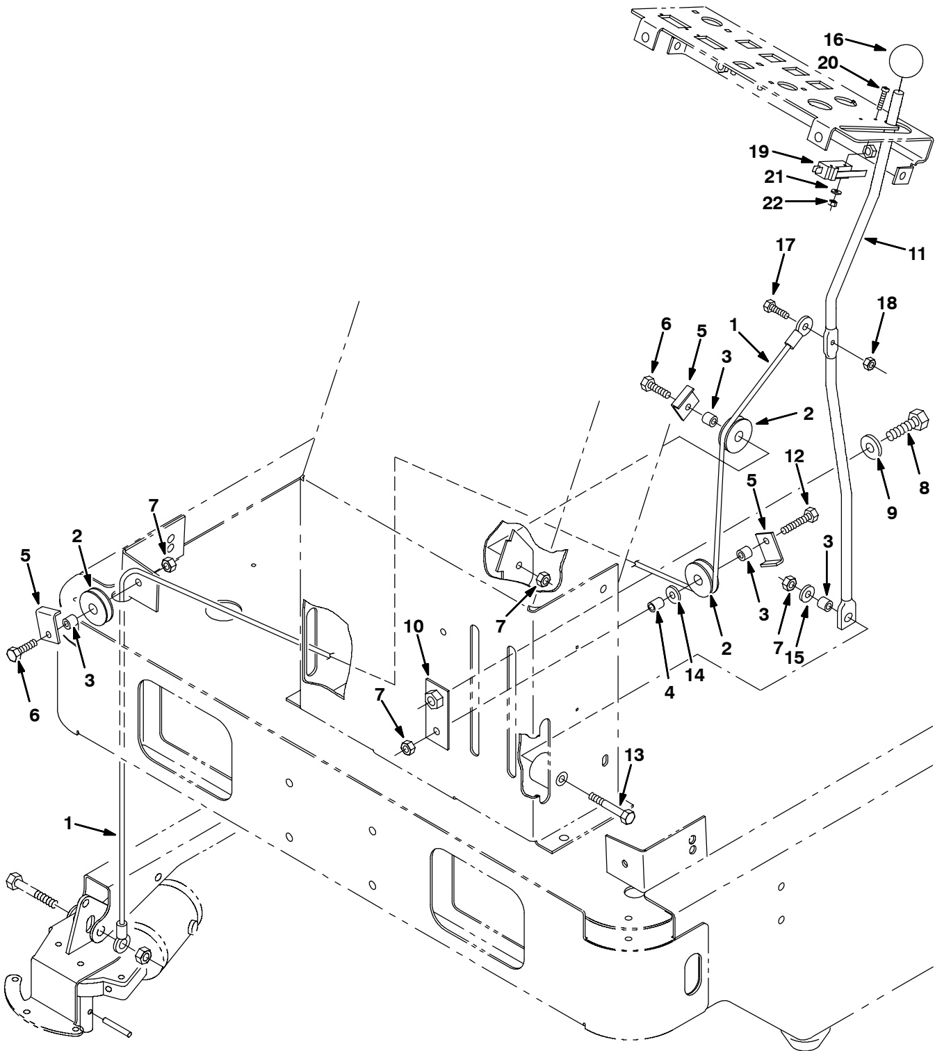
Fig. 18 - Side Brush Lift Group
