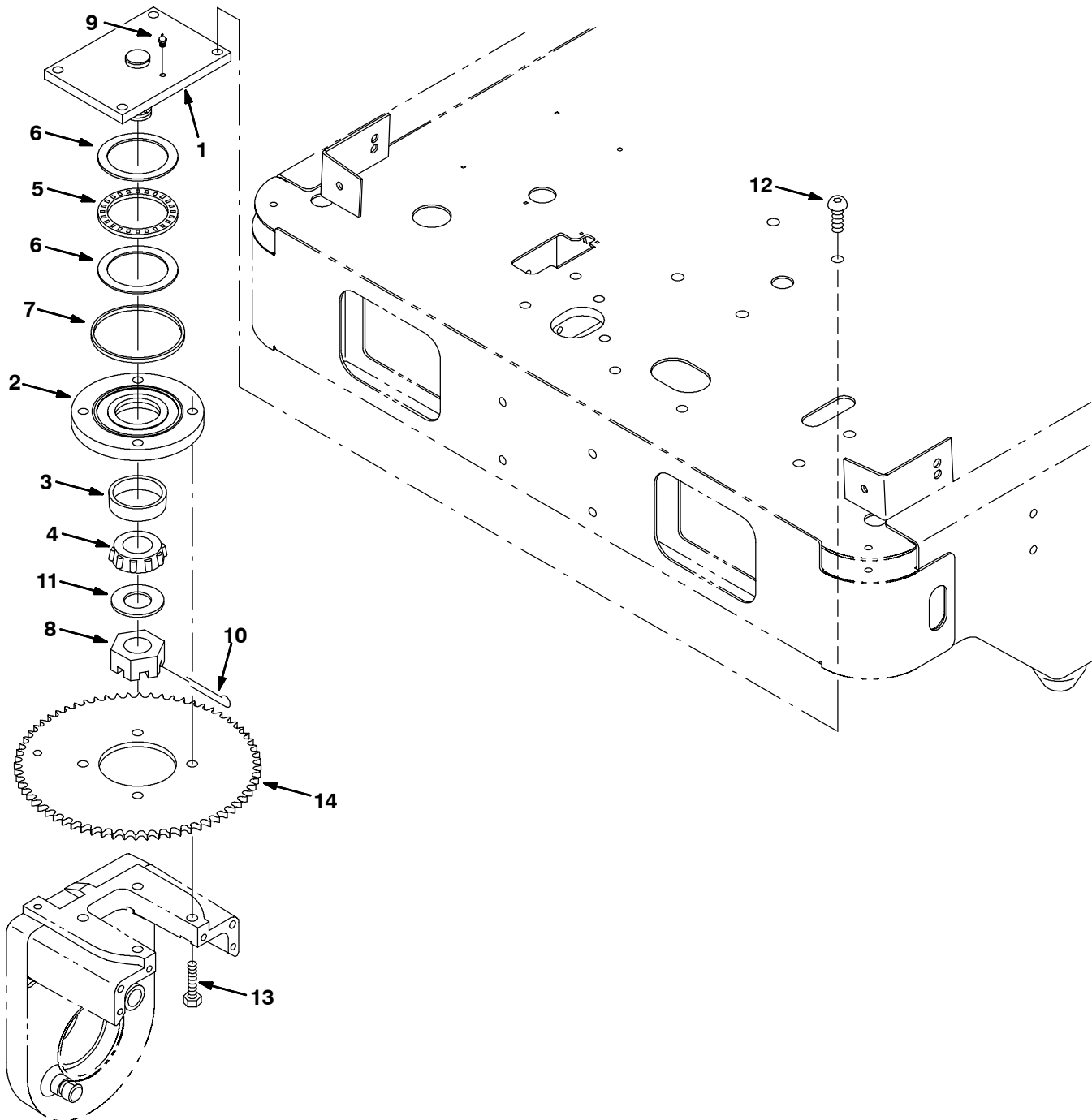
Fig. 9 - Front Wheel Pivot Group
