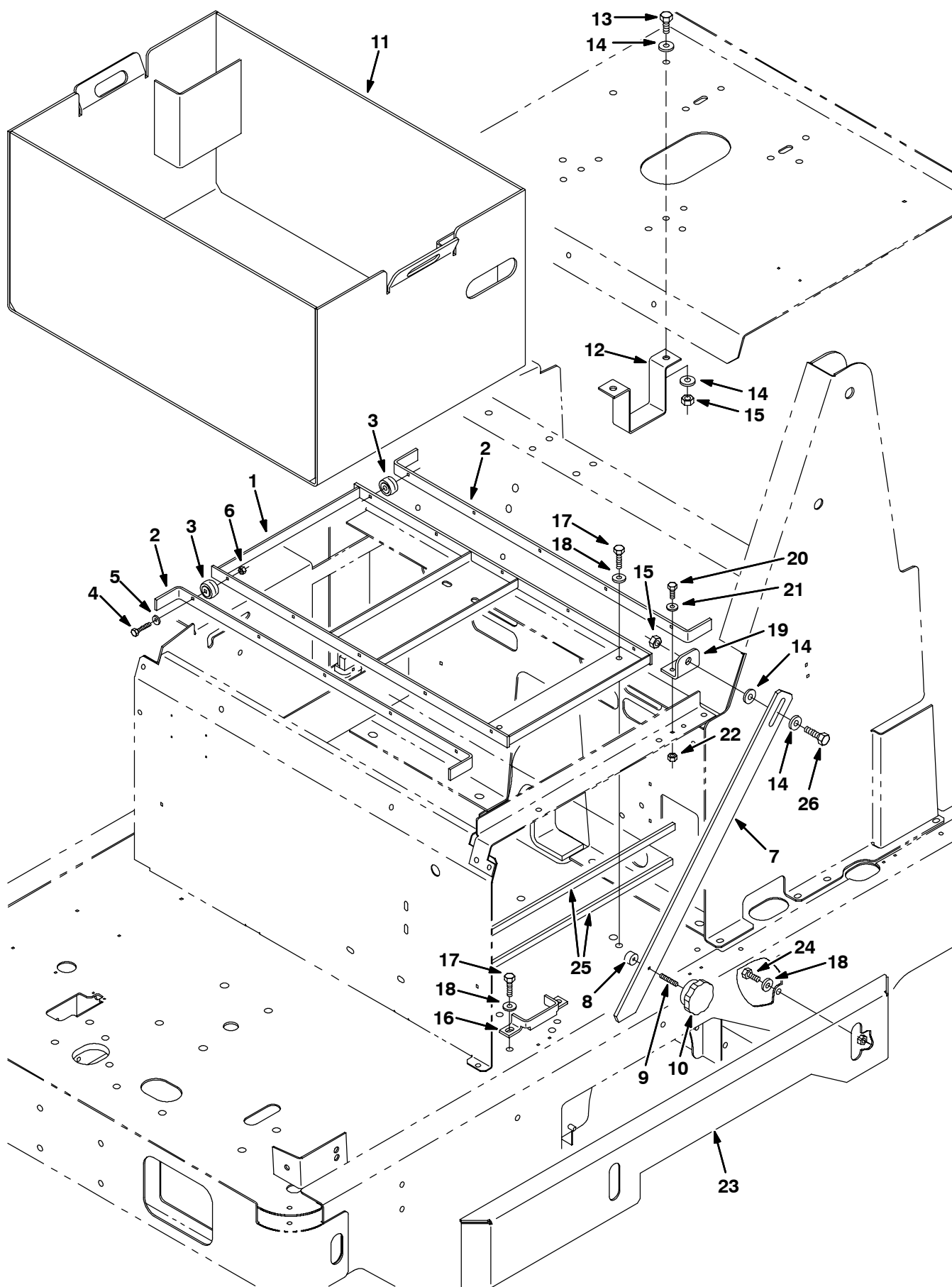
Fig. 7 - Rollout Battery Case Kit
