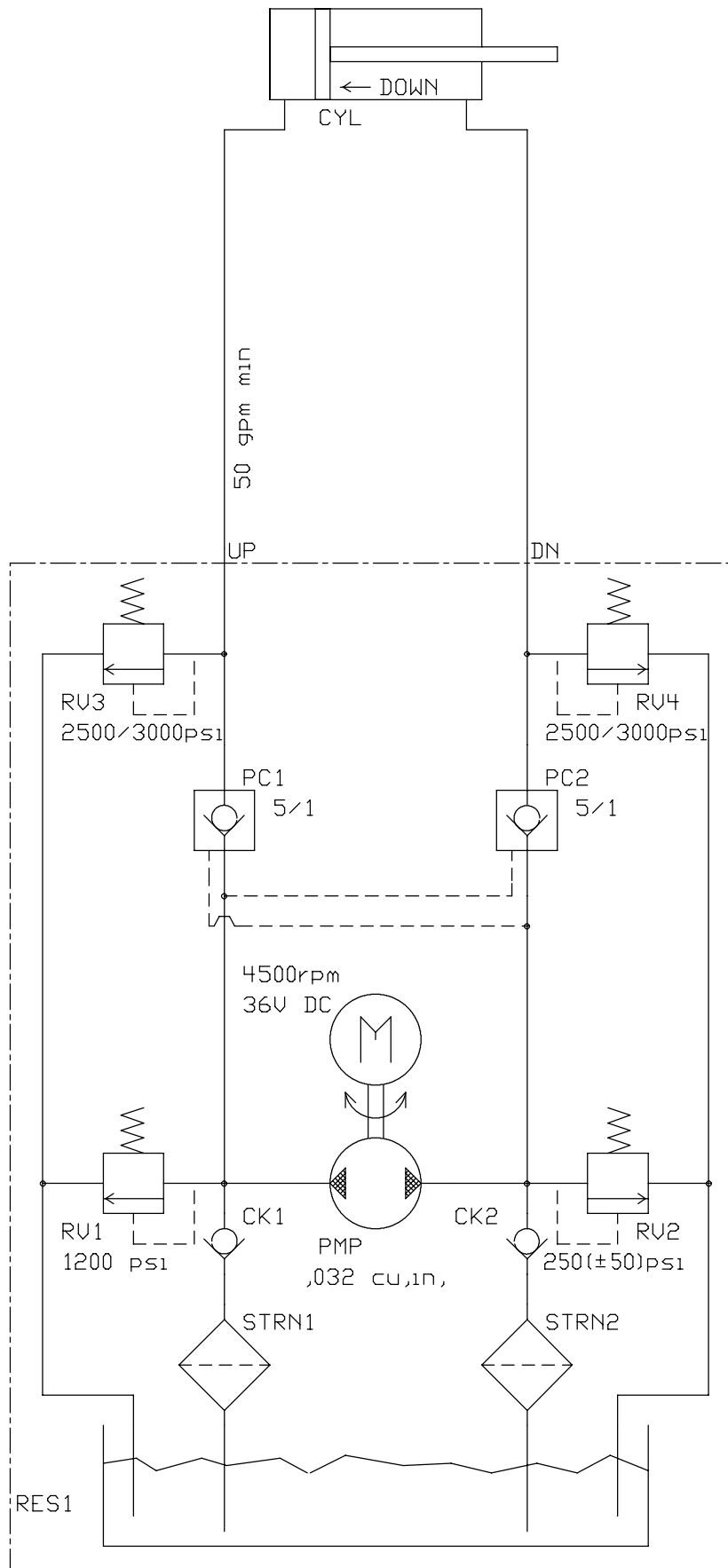
Fig. 26 - Hydraulic Schematic
