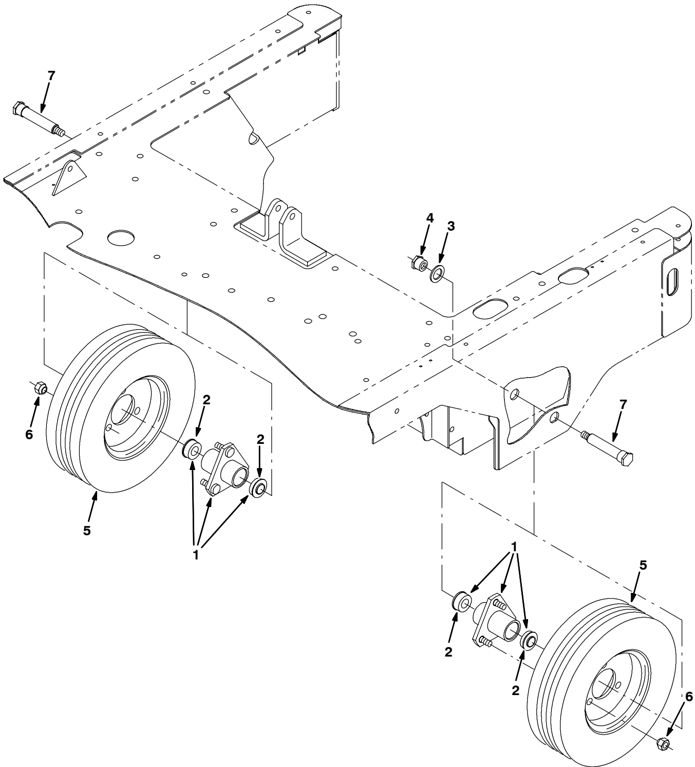
Fig. 13 - Rear Wheel Group
