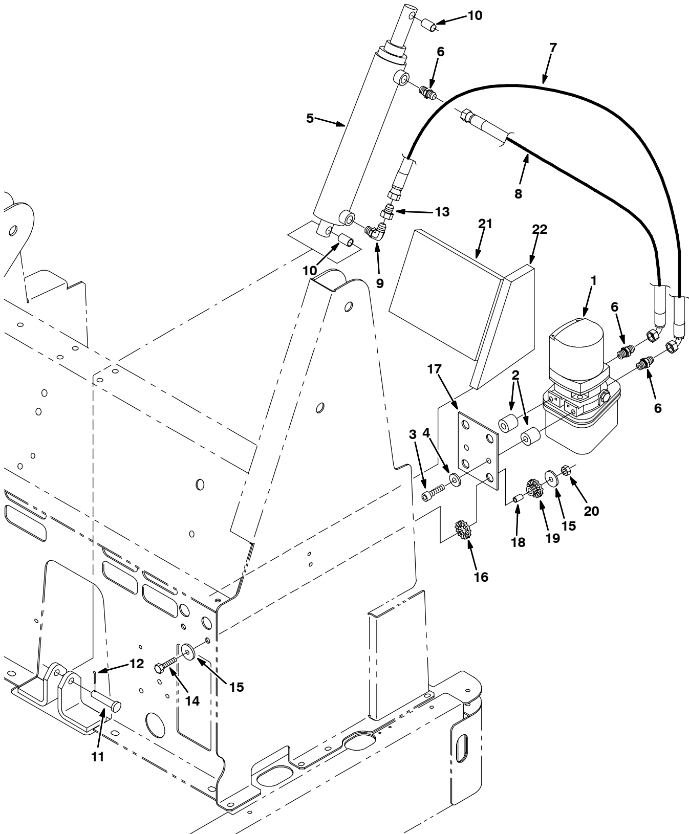
Fig. 24 - Hydraulic Hopper Lift Group
