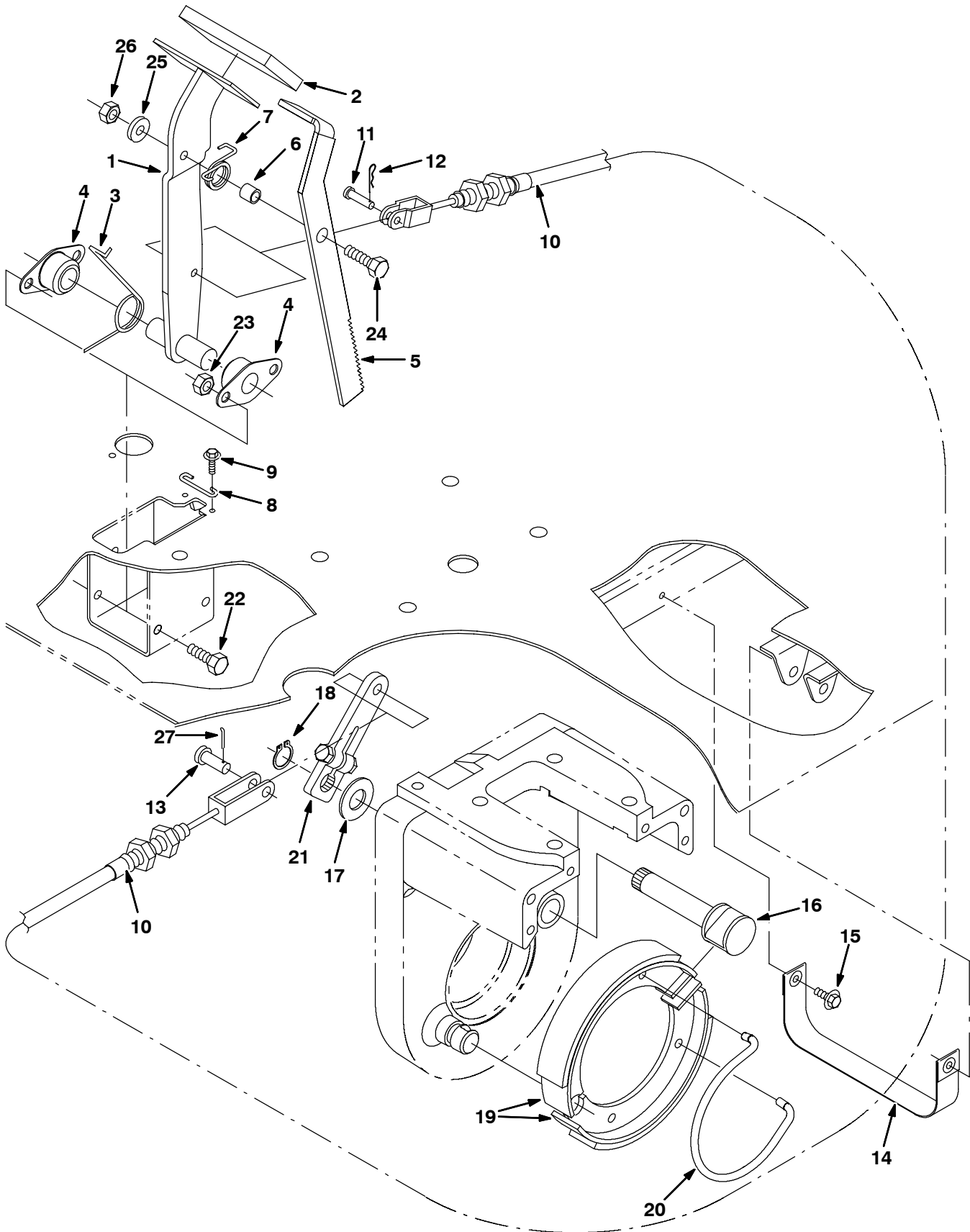
Fig. 11 - Brake Group
