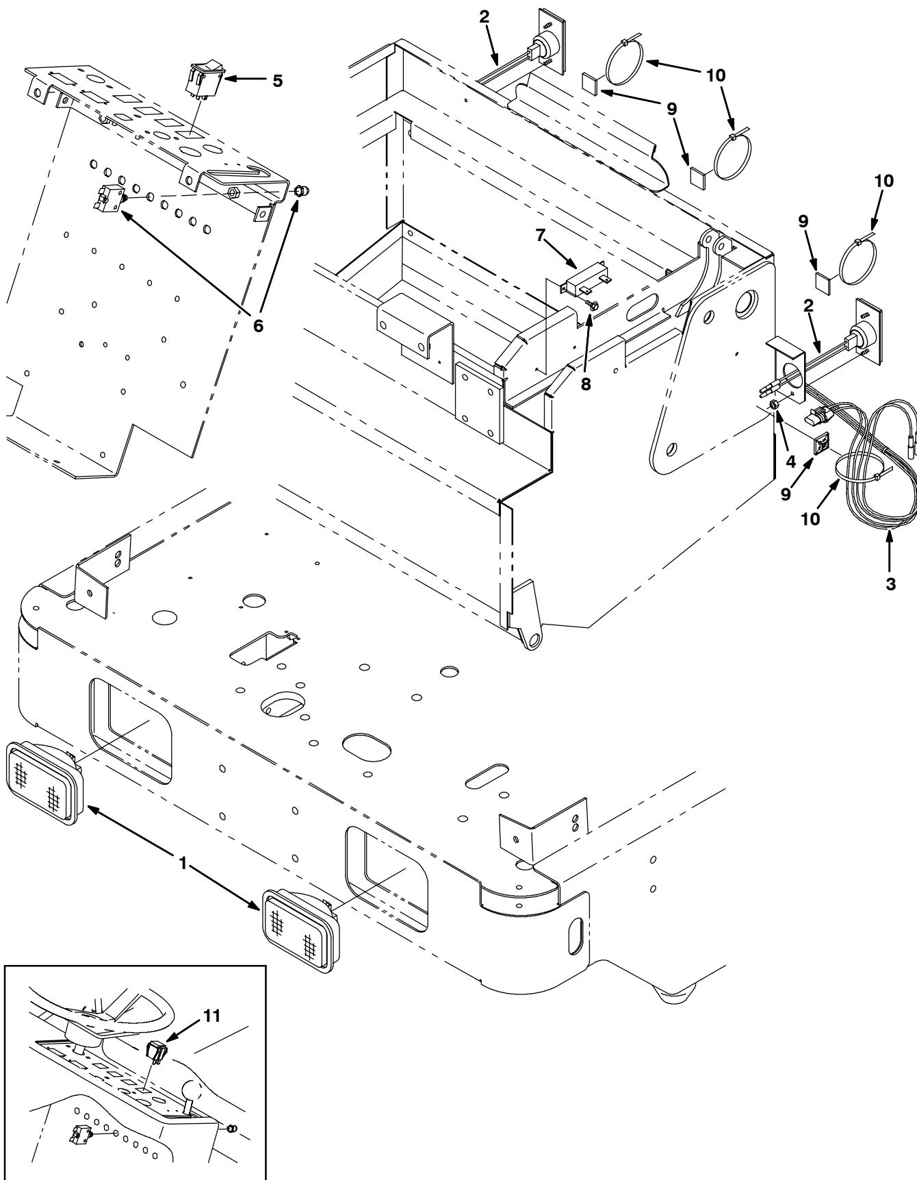
Fig. 15 - Light Kit
