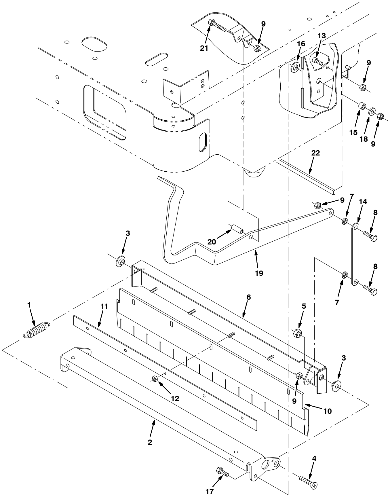
Fig. 15 - Main Brush Front Flap Group
