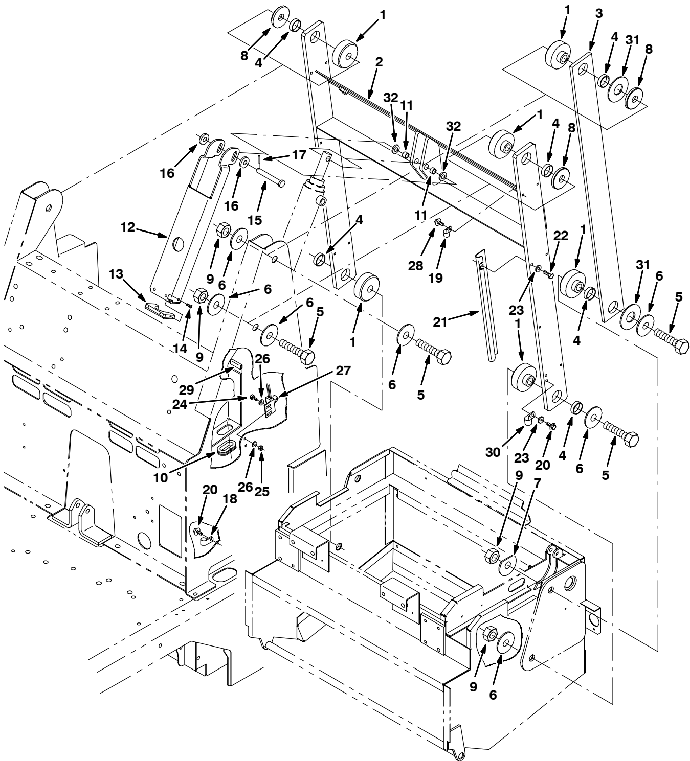
Fig. 22 - Hopper Lift Arms Group
