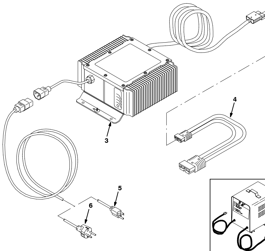
Fig. 21 - Battery Charger and Harness Group, International Only
