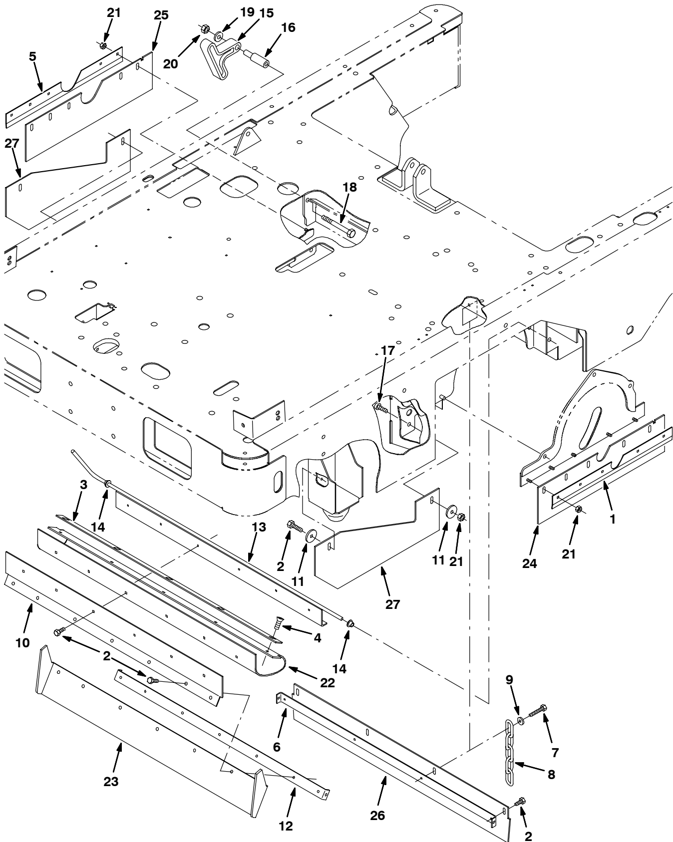
Fig. 14 - Main Brush Skirts Group
