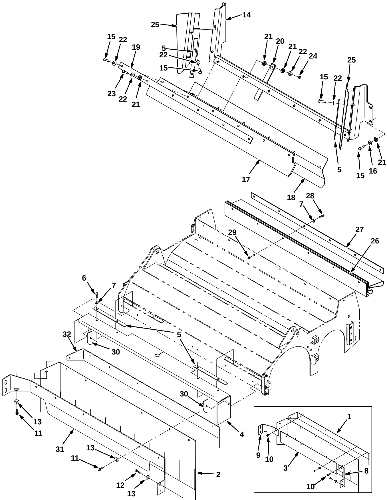
Fig. 46 – Cylindrical Brush Head Skirt Group
