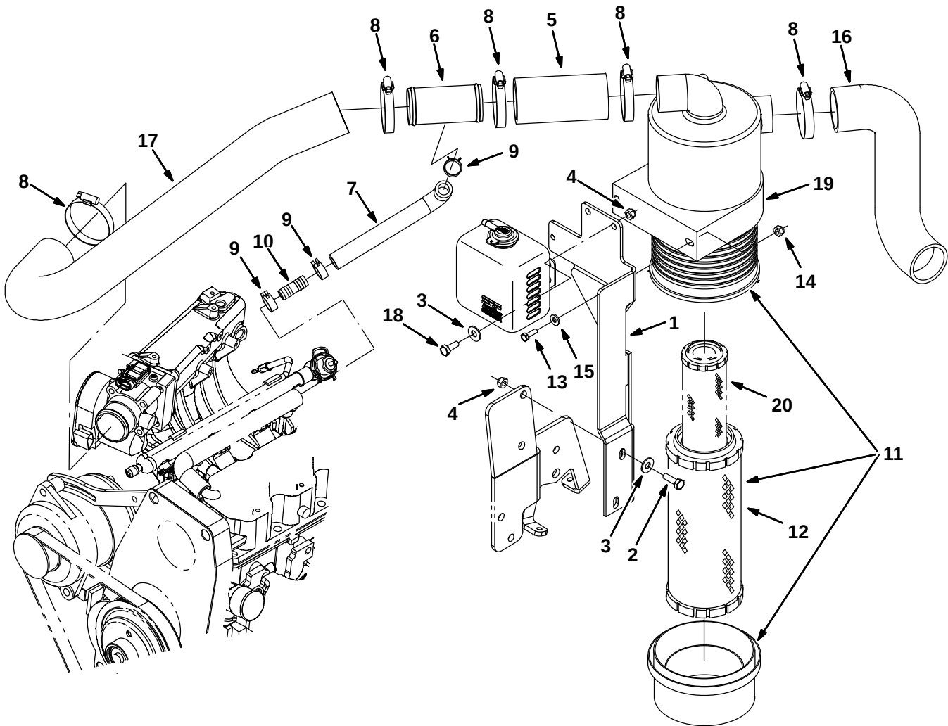
Fig. 22 – Engine Air Cleaner Group, Gasoline (000000–001999)
