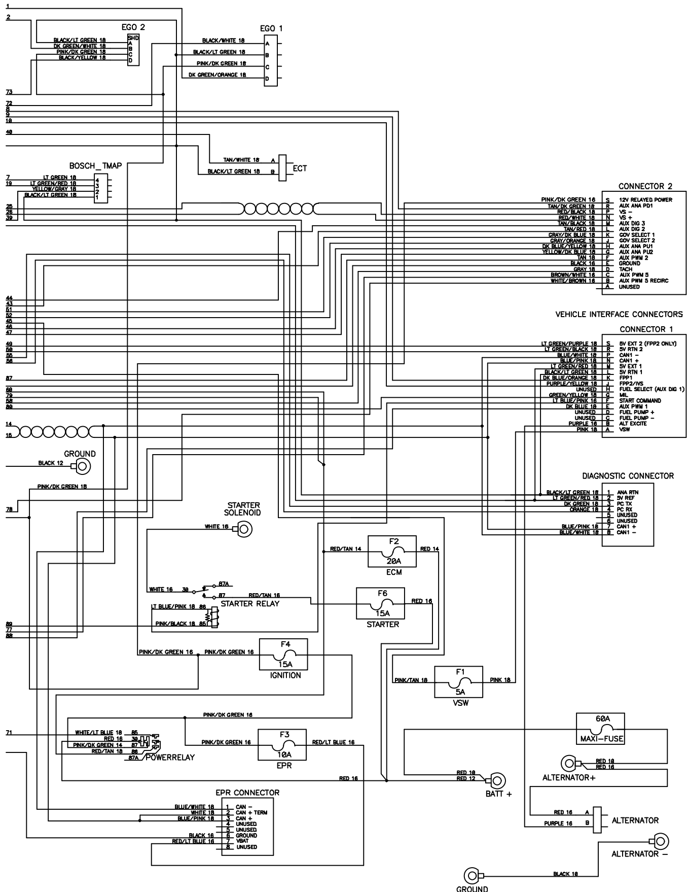
Fig. 81 – Electrical Schematic, LPG Engine Harness (003123- )
