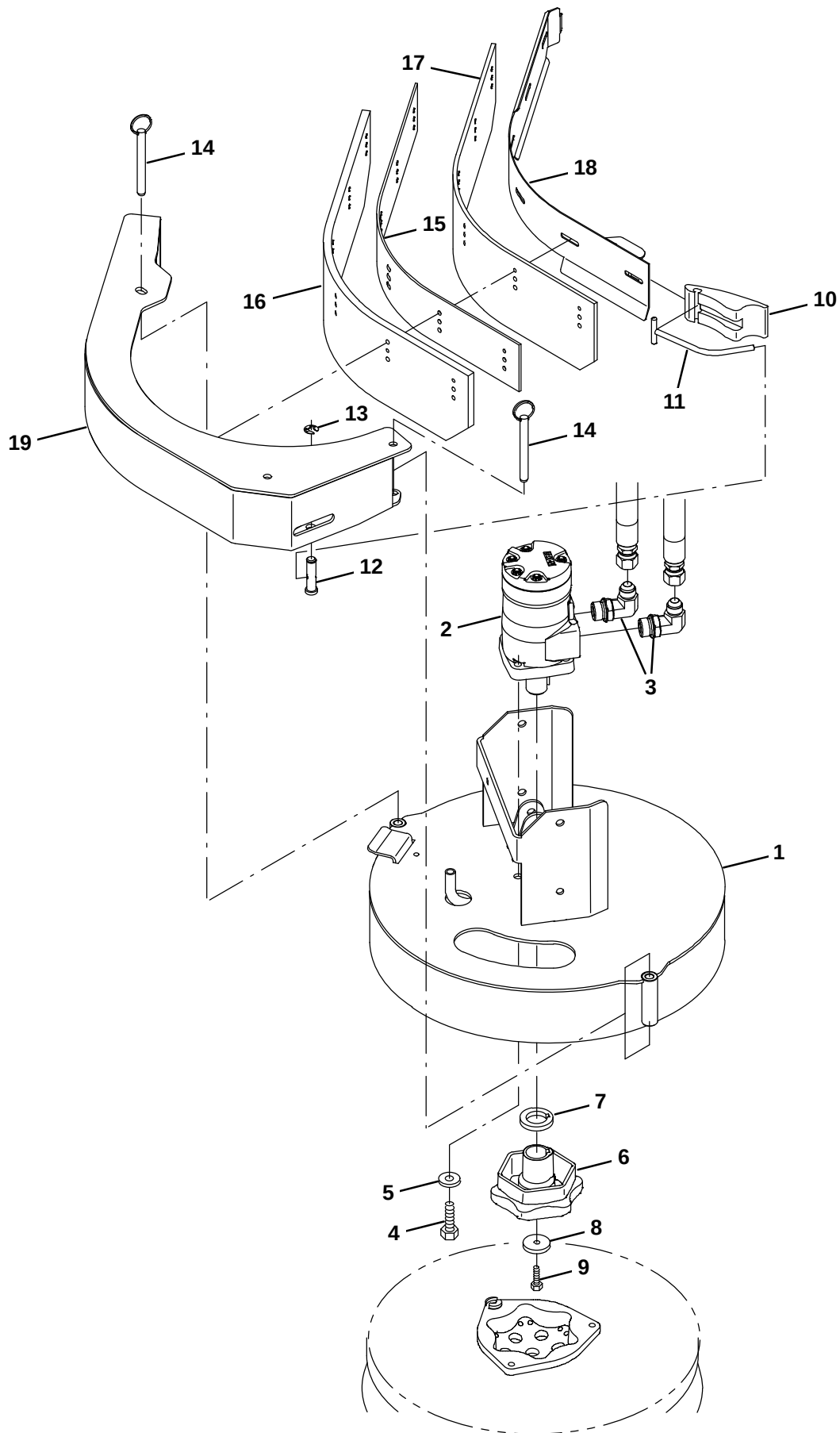
Fig. 4 – Side Brush Motor Group (003077– )
