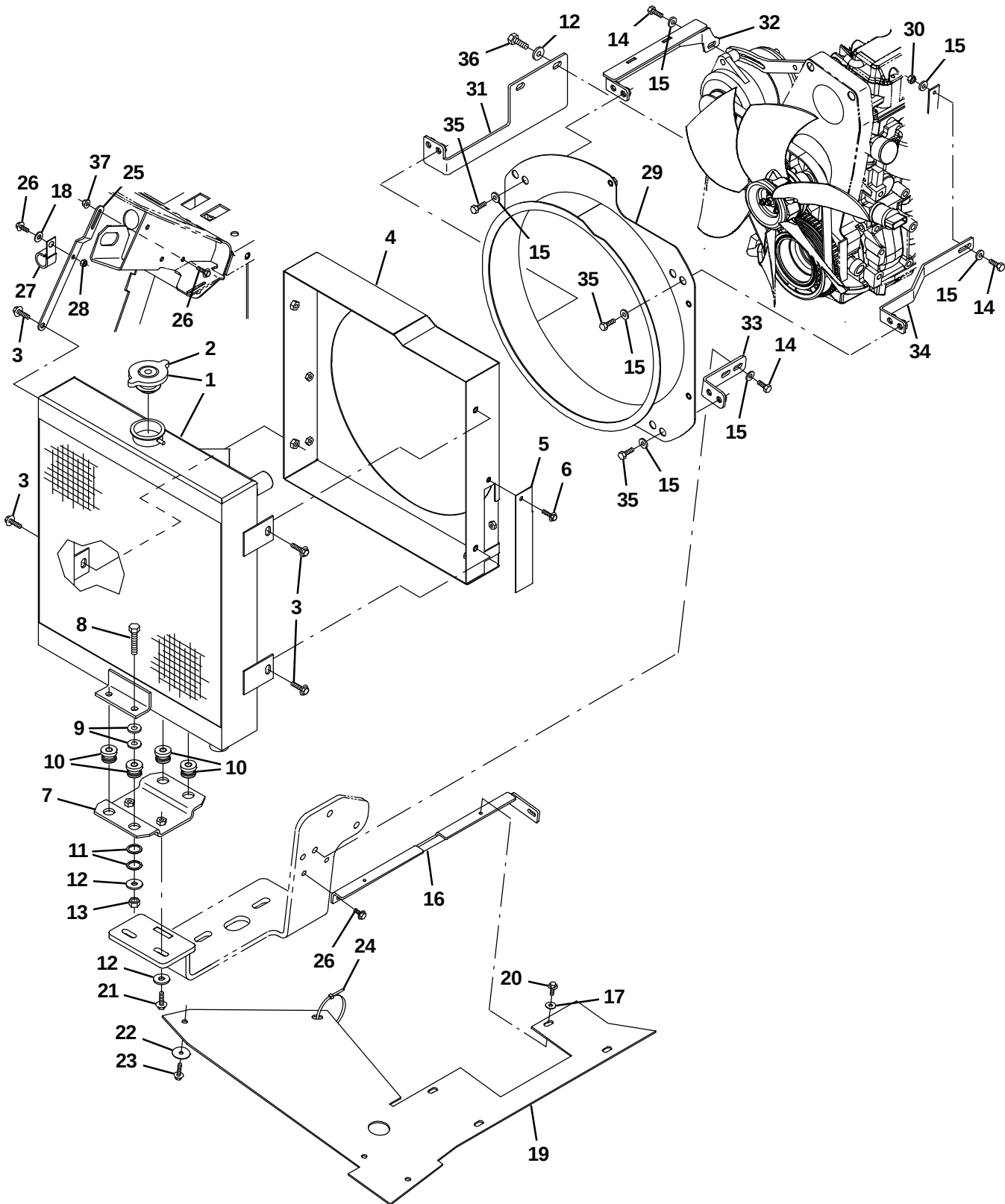
Fig. 30 – Engine Radiator and Mount Group (003039– )
