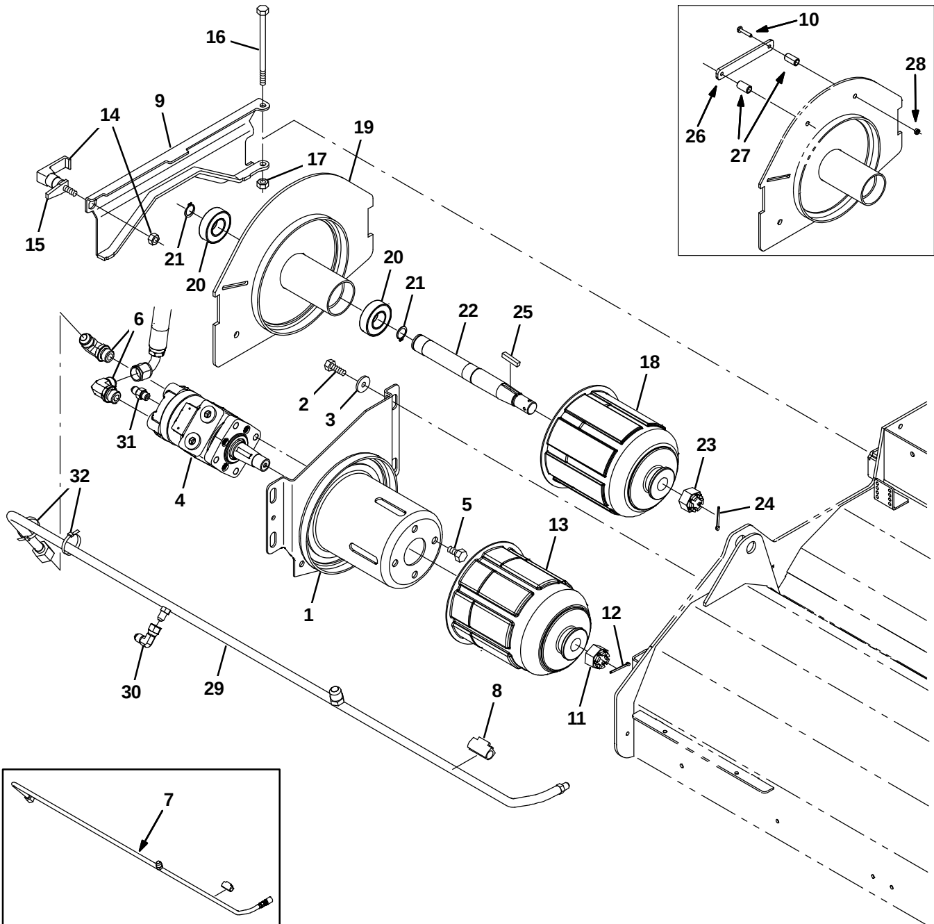
Fig. 44 – Cylindrical Scrub Brush Drive Group, Right Side
