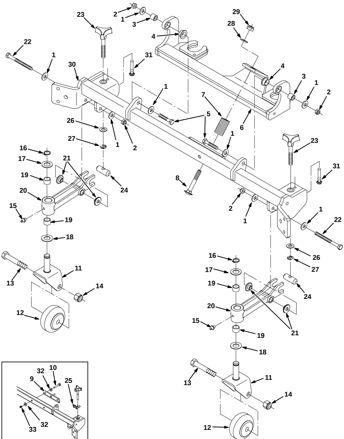
Fig. 49 – Squeegee Linkage Group, Rear
