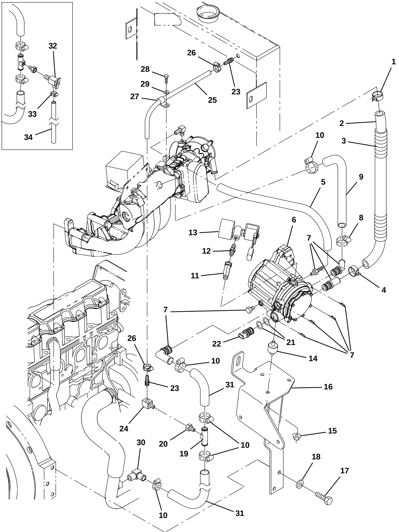
Fig. 17 – Engine Vaporizer Group, LPG (002000–003122)
