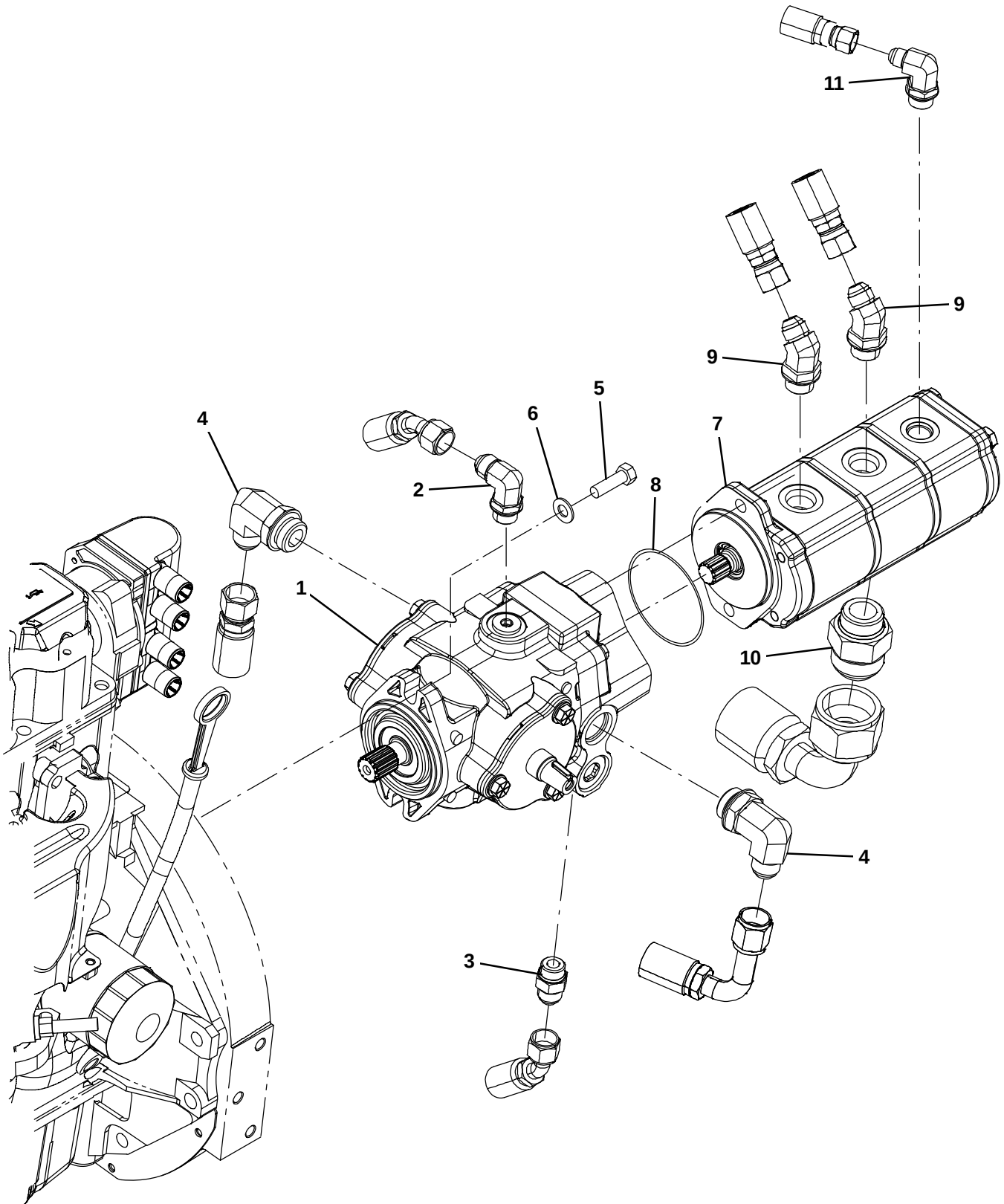
Fig. 68 – Hydraulic Pumps Group
