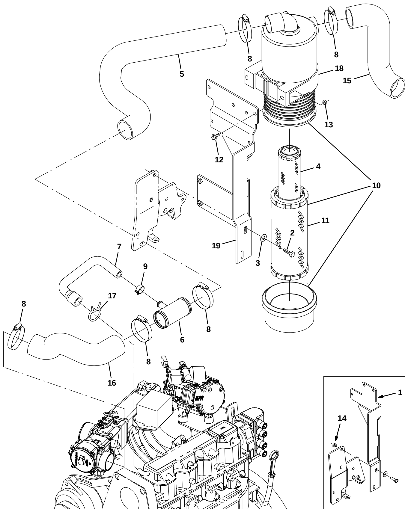
Fig. 25 – Engine Air Cleaner Group, LPG (002000– )
