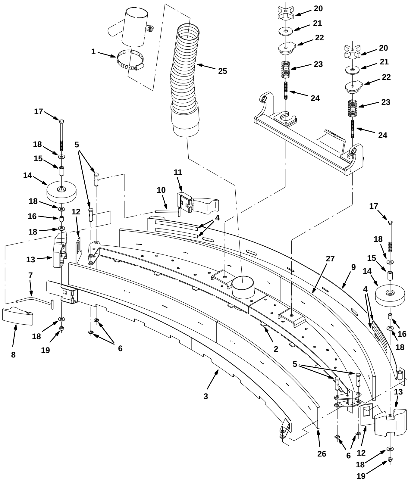
Fig. 48 – Squeegee Group, Rear
