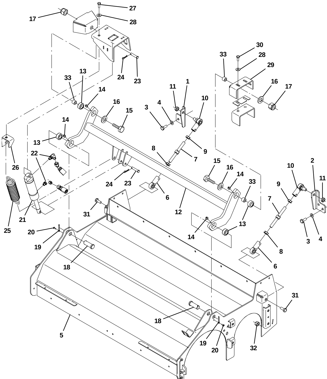
Fig. 45 – Cylindrical Scrub Brush Head Lift Group
