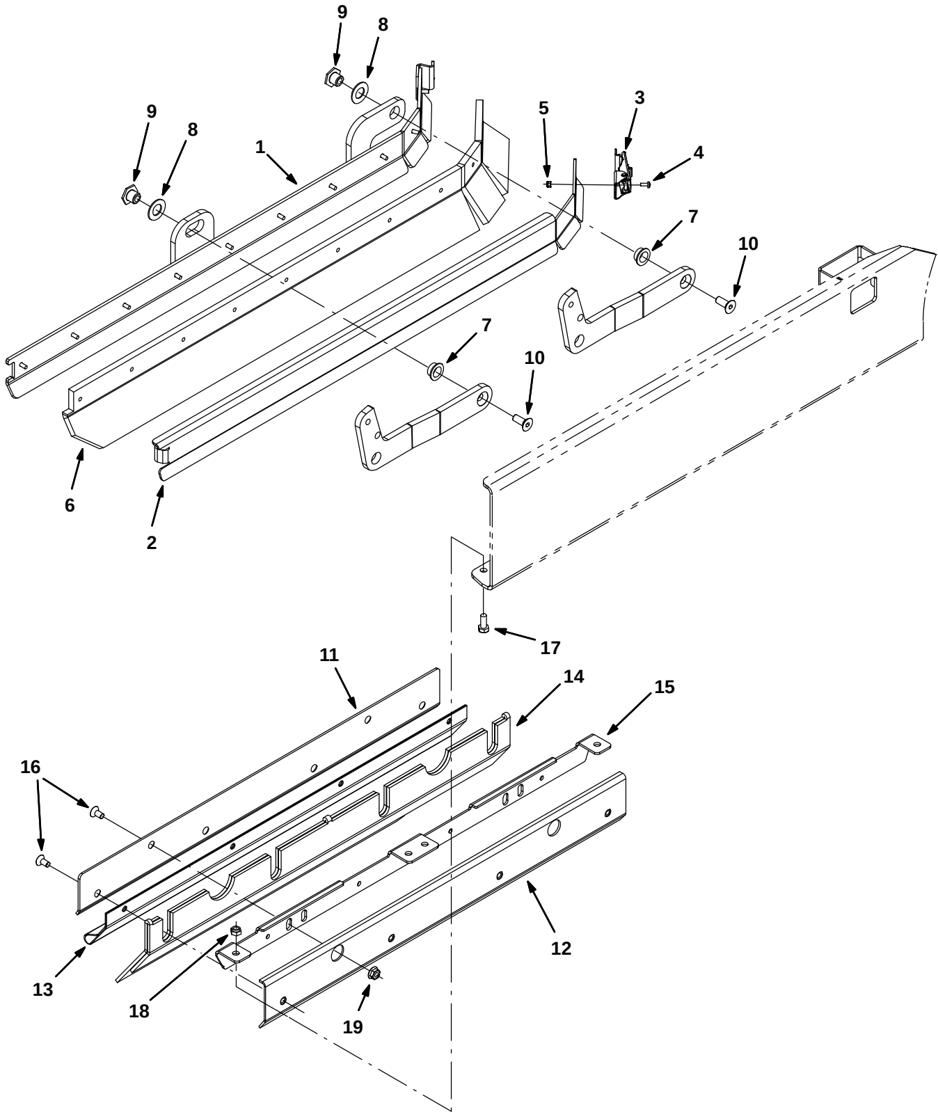
Fig. 52 – Squeegee Group, Left Side
