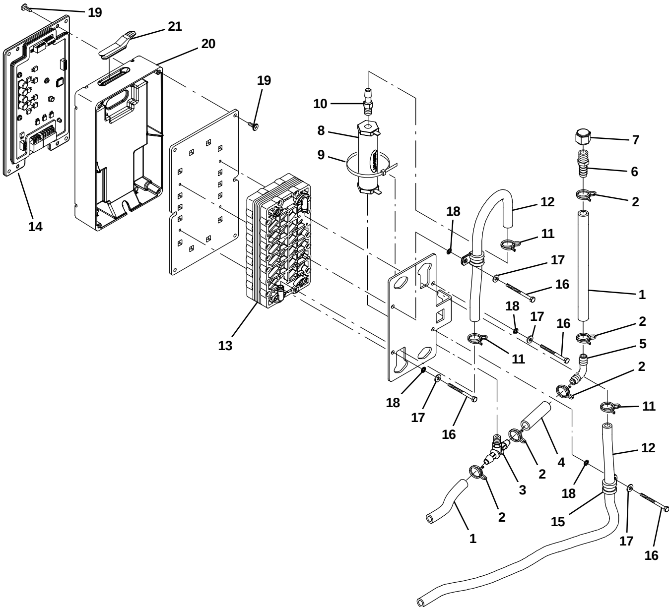
Fig. 15 – ec-H2O Module Assembly Breakdown, 9007882
