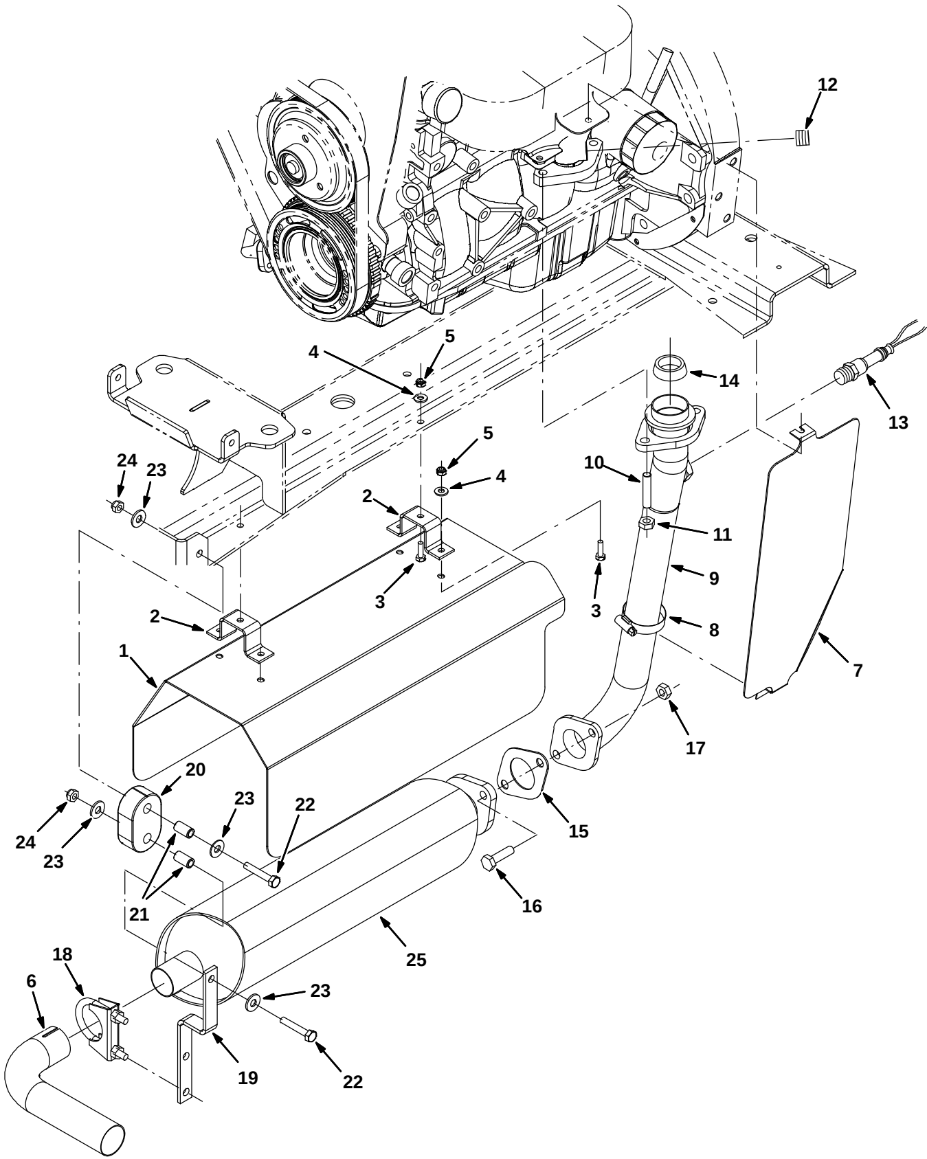
Fig. 27 – Engine Muffler Group (000000–001999)
