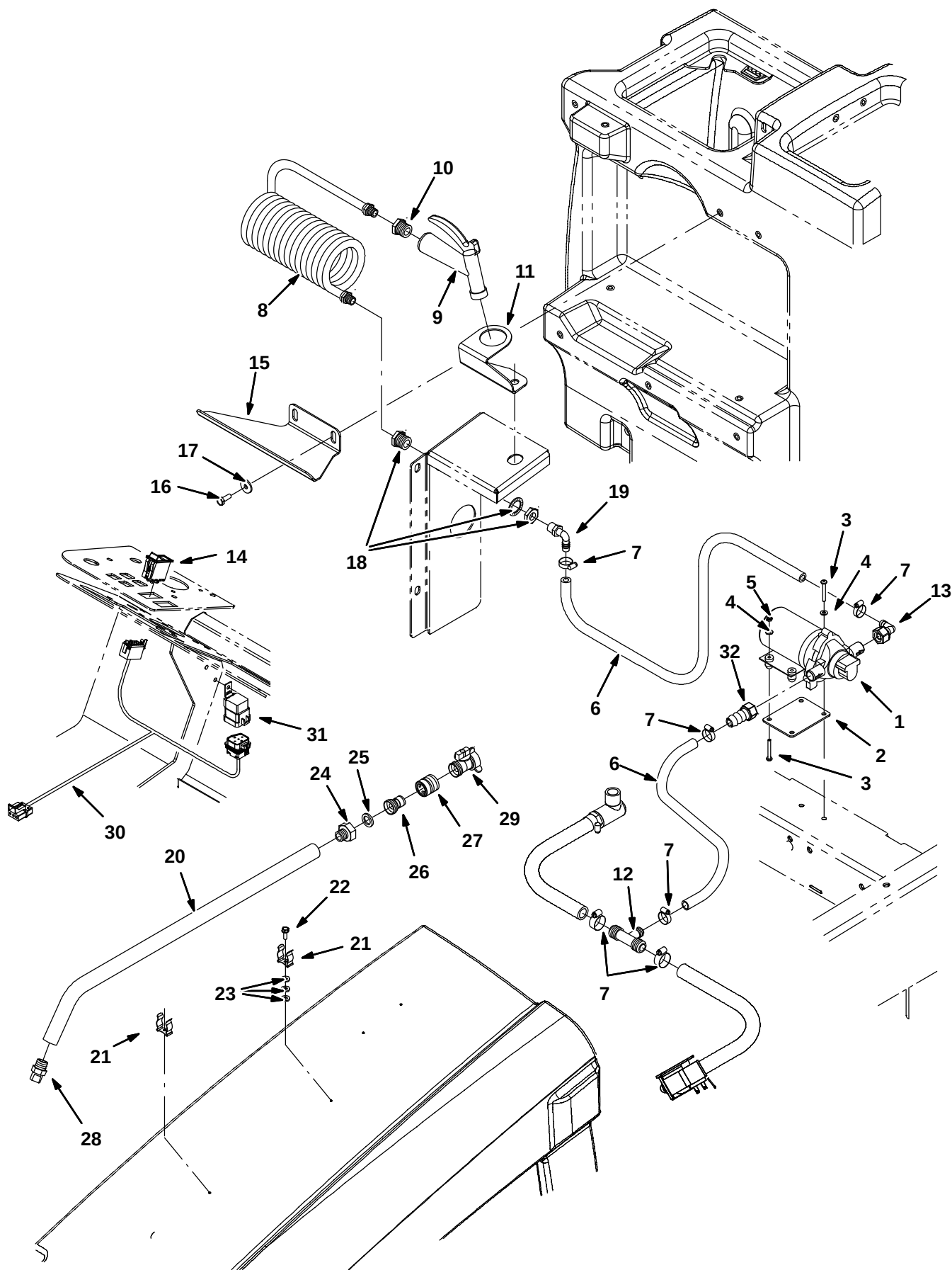
Fig. 31 – Spray Nozzle Kit
