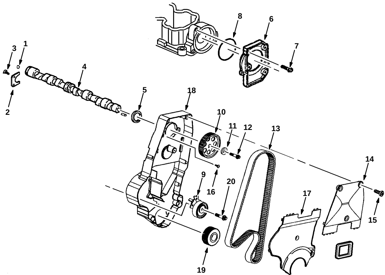
Fig. 6 – Camshaft Group
