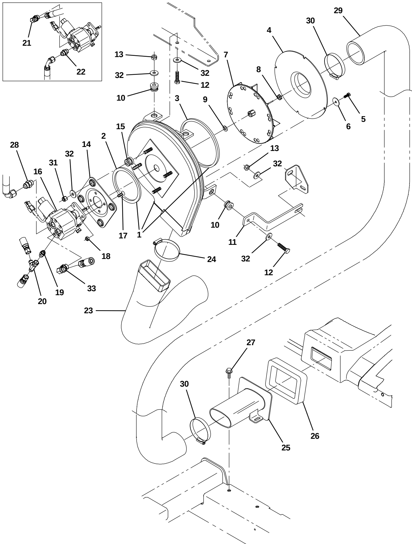
Fig. 60 – Vacuum Fan Group, Sweeping
