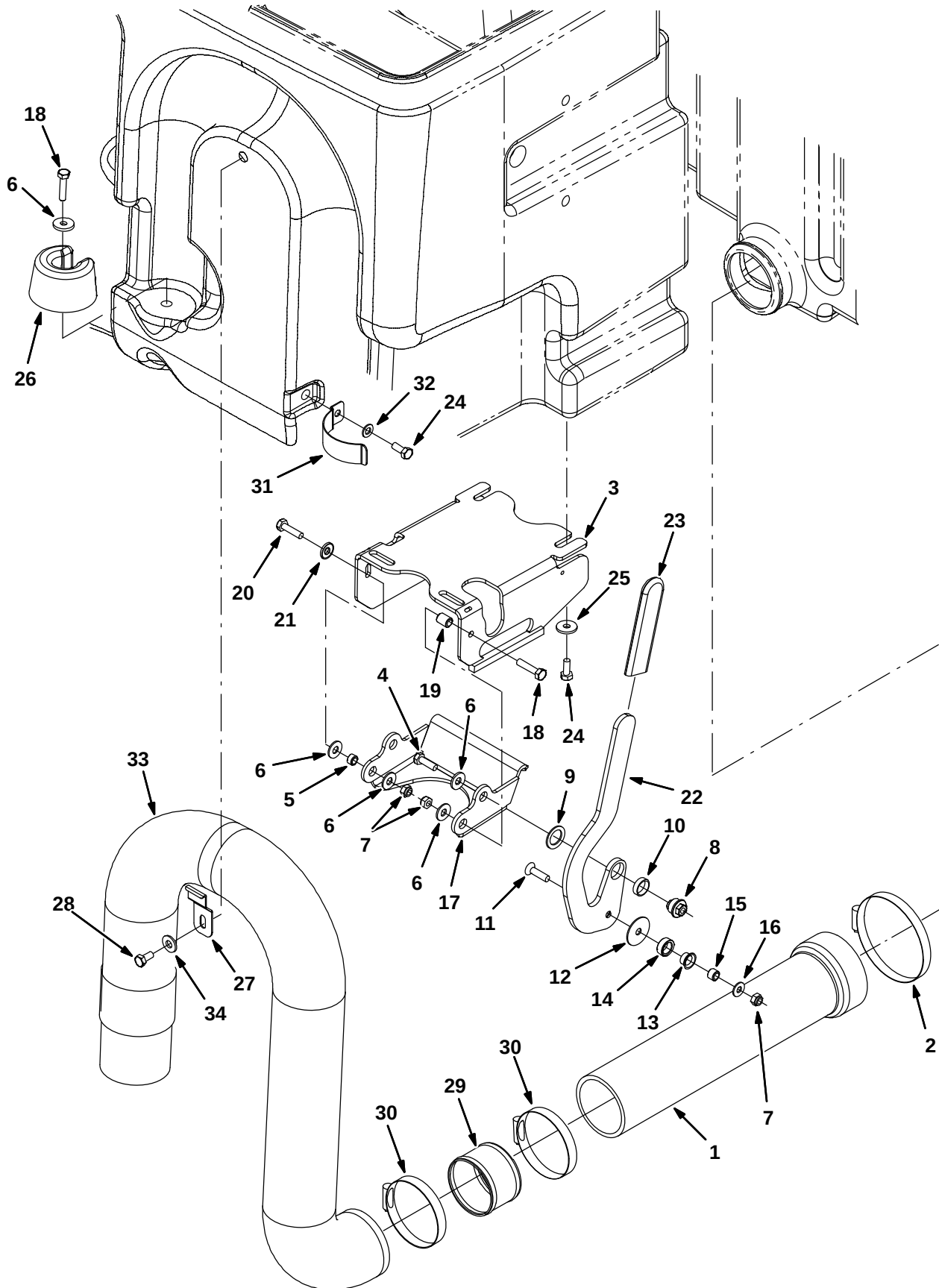
Fig. 55 – Solution Tank Drain Group
