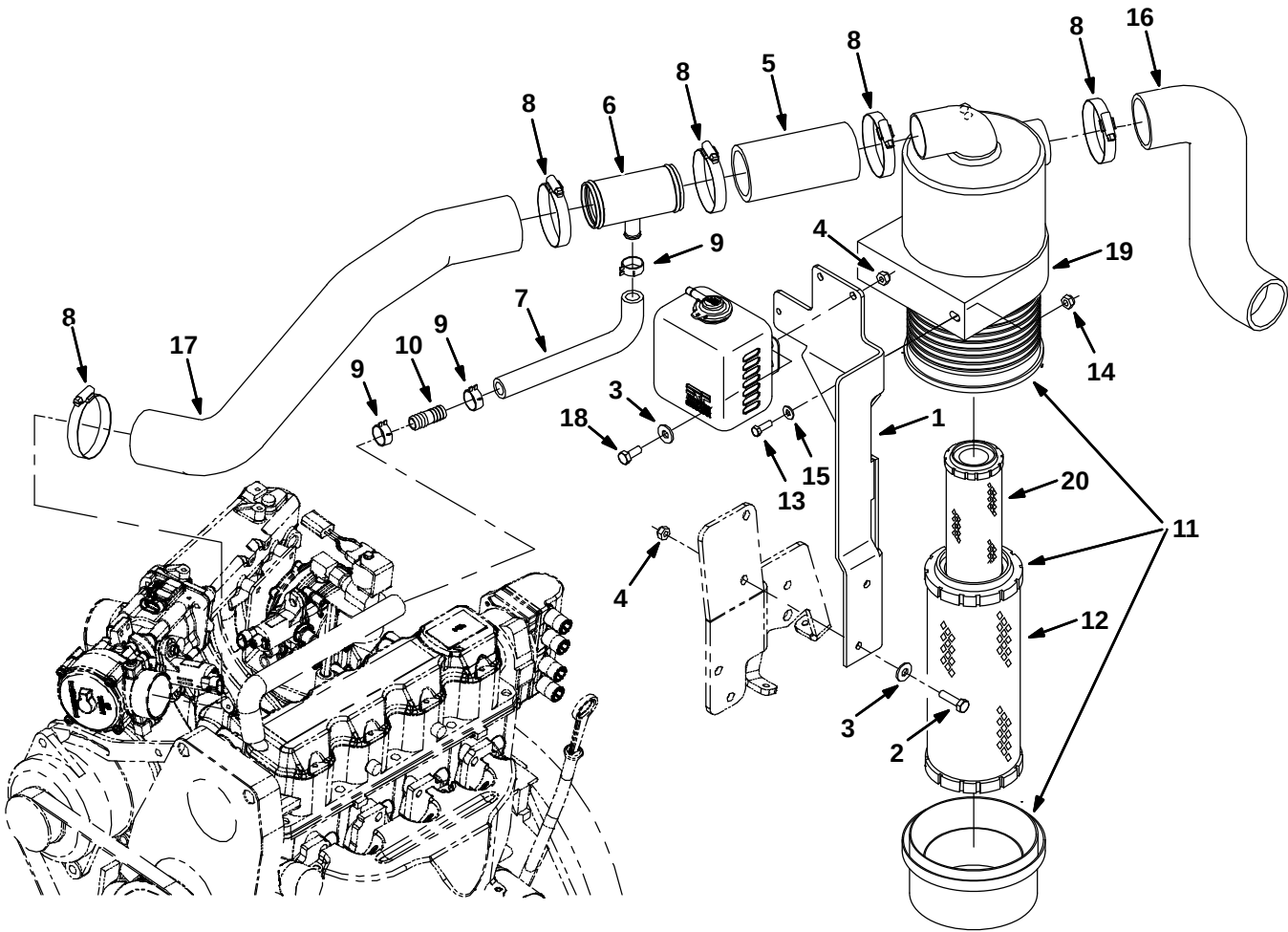
Fig. 24 – Engine Air Cleaner Group, LPG (000000–001999)
