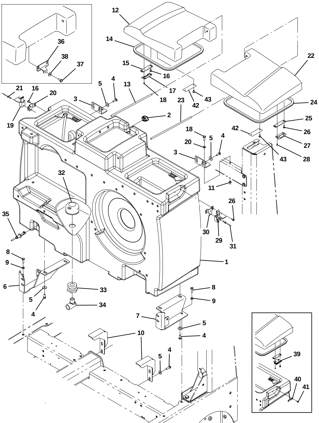
Fig. 54 – Solution Tank Group
