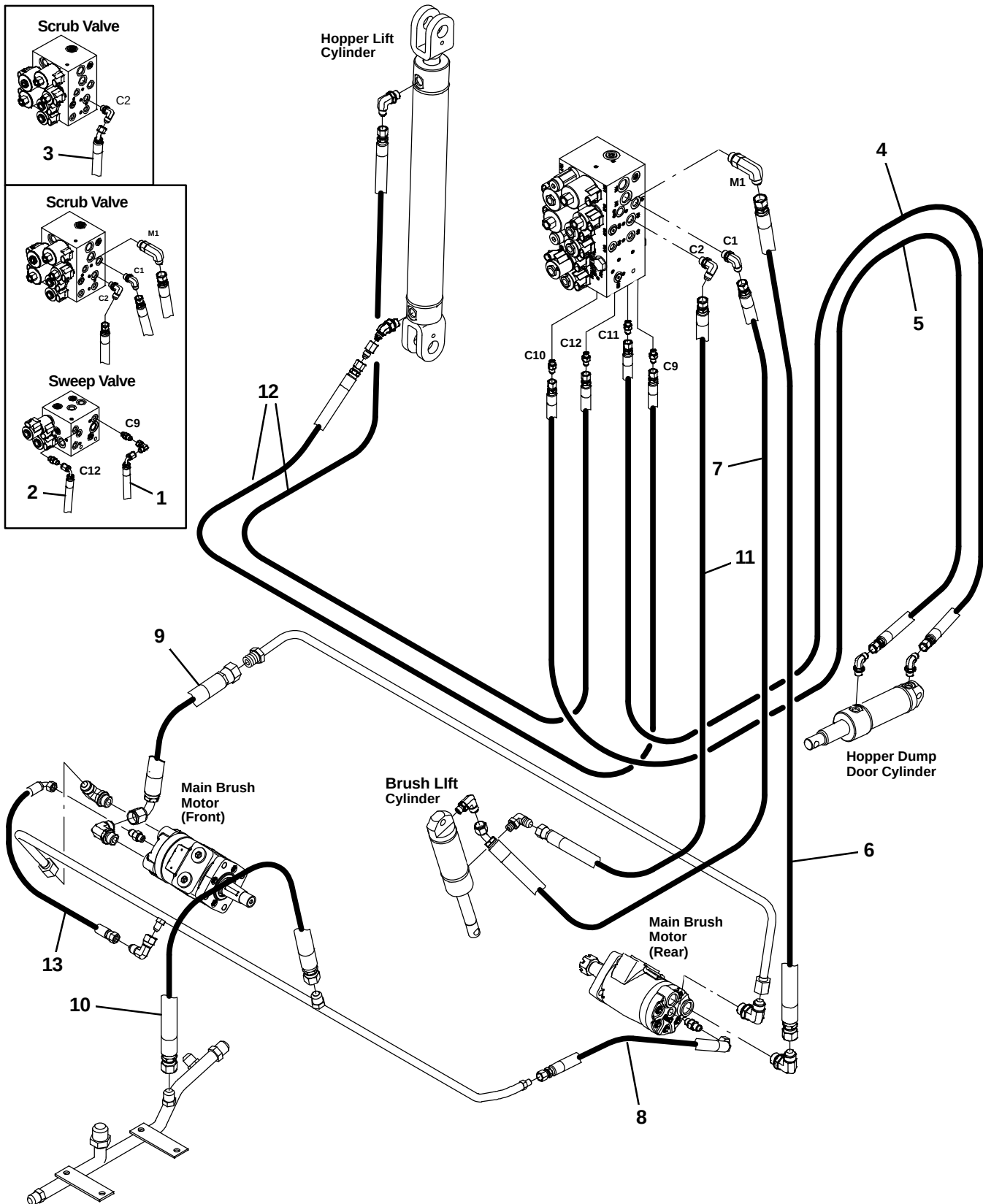
Fig. 66 – Hydraulic Hose Group, Brush and Hopper
