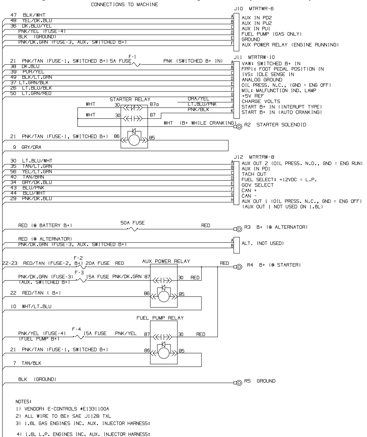
Fig. 77 – Electrical Schematic, Gas/LPG Engine Harness (000000-001999)
