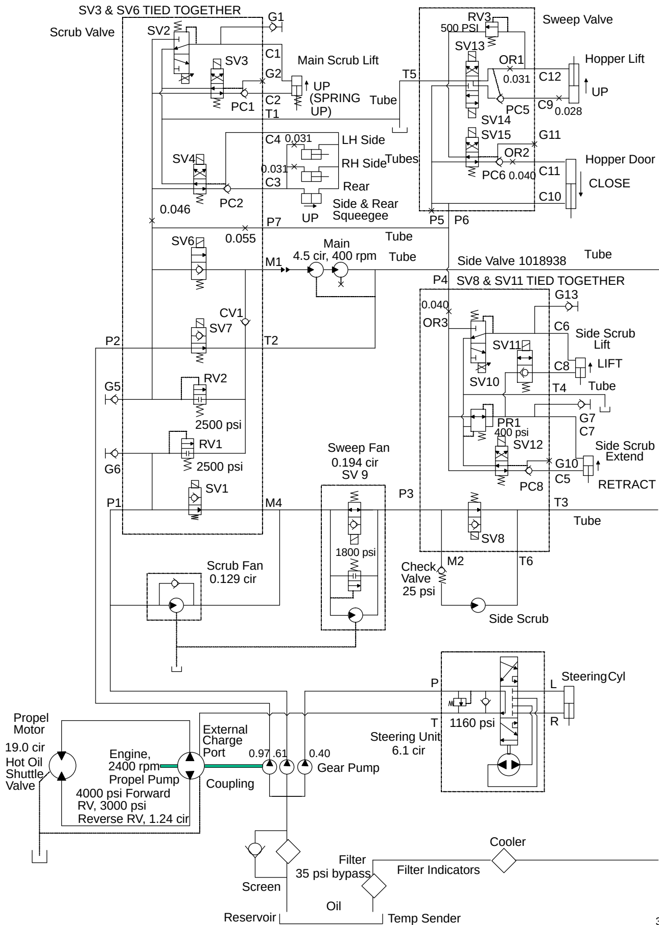
Fig. 61 – Hydraulic Schematic (000000–002699)
