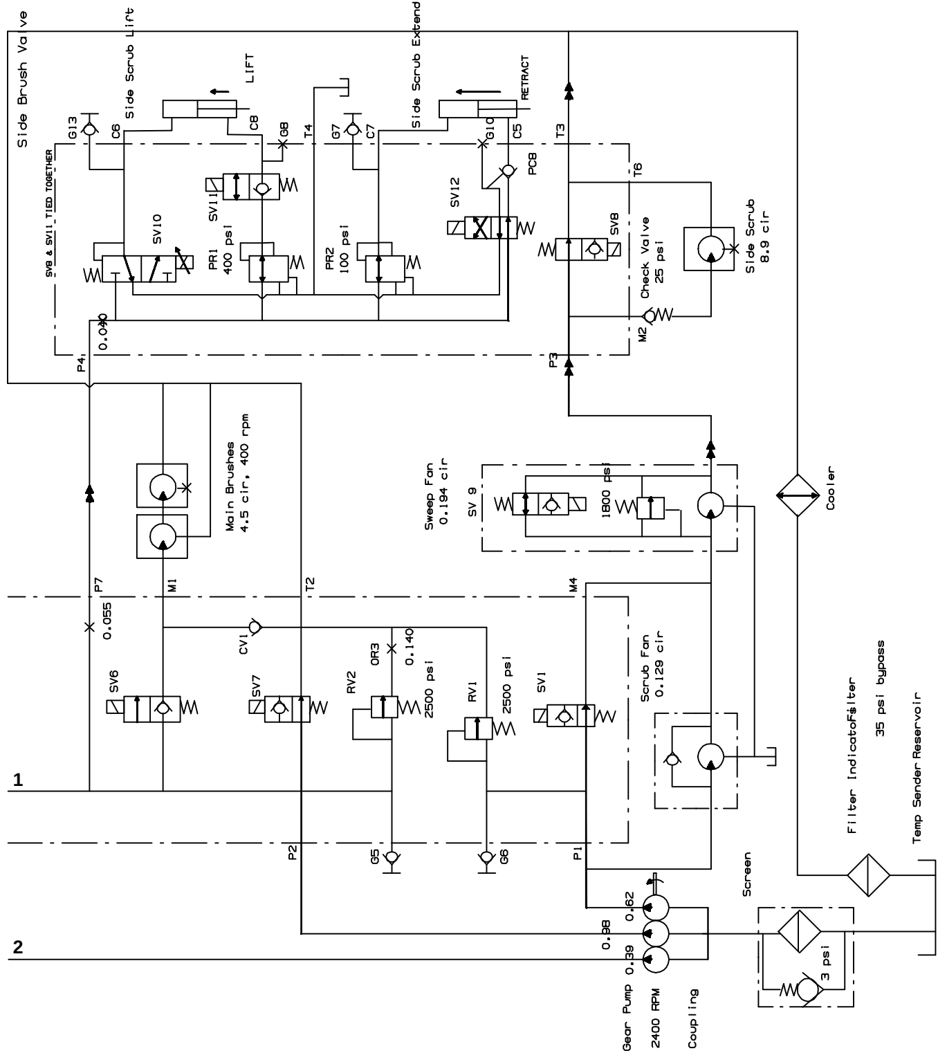
Fig. 63 – Hydraulic Schematic (003298– )
