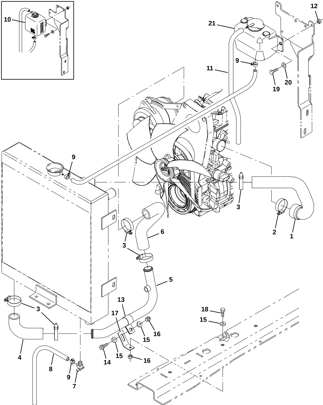
Fig. 31 – Engine Radiator Hose Group (003039– )
