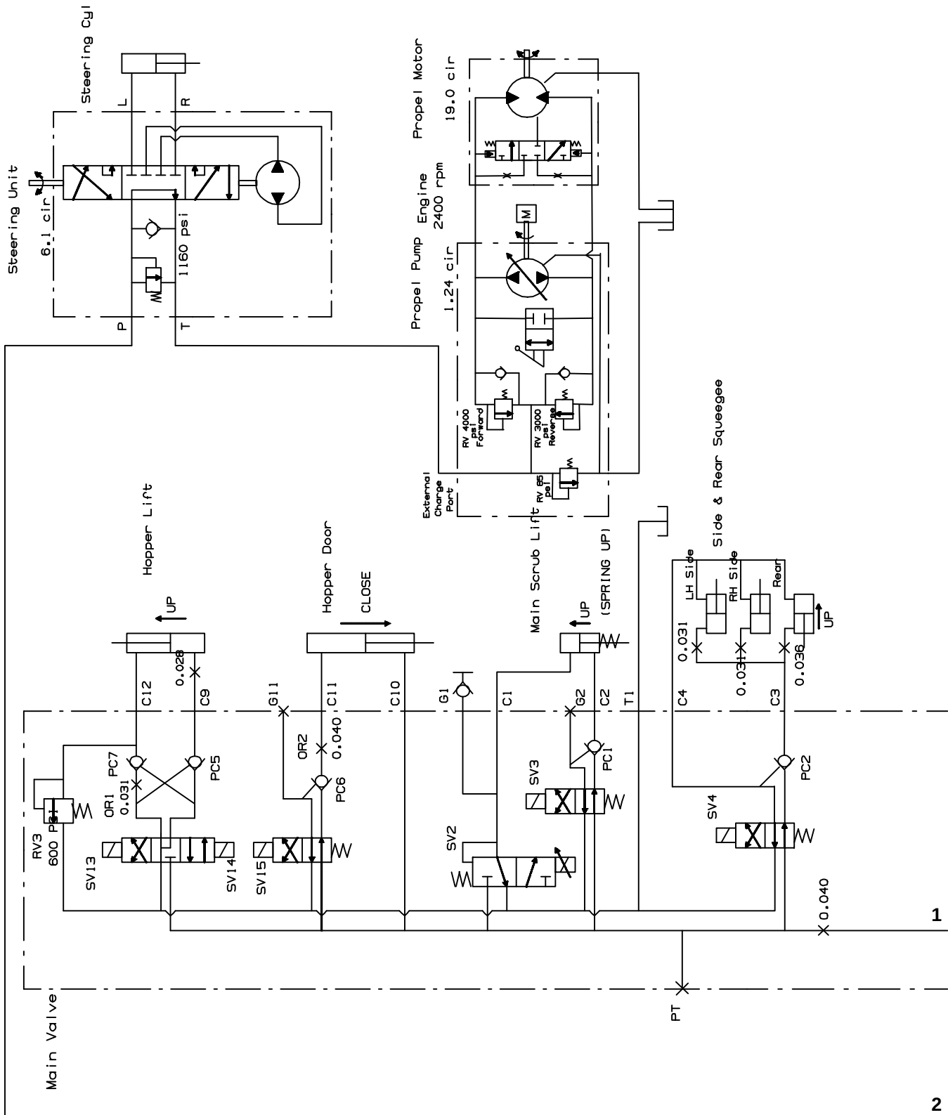
Fig. 62 – Hydraulic Schematic (002700–003297)
