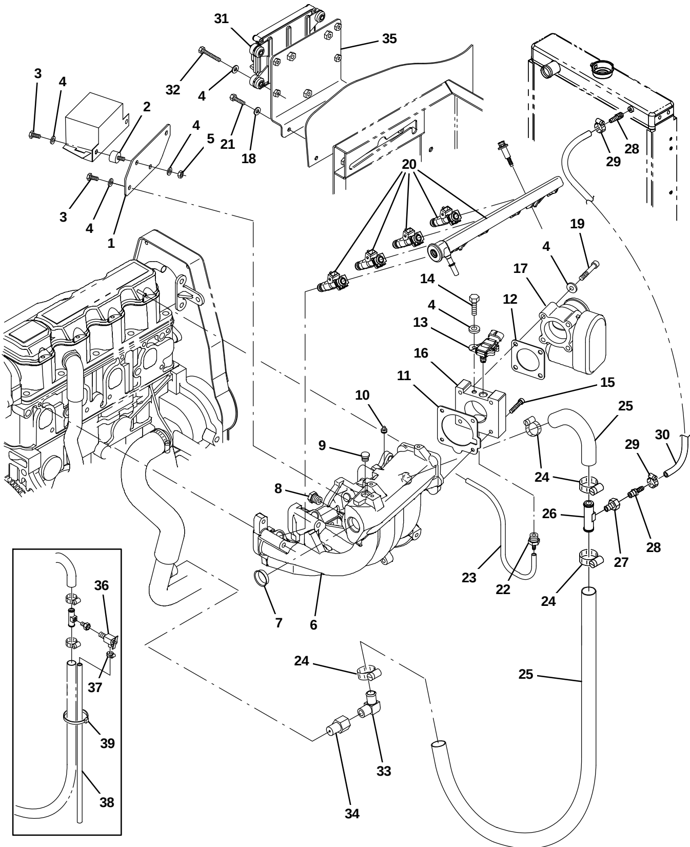
Fig. 13 – Engine EFI Group, Gasoline (002000–003122)
