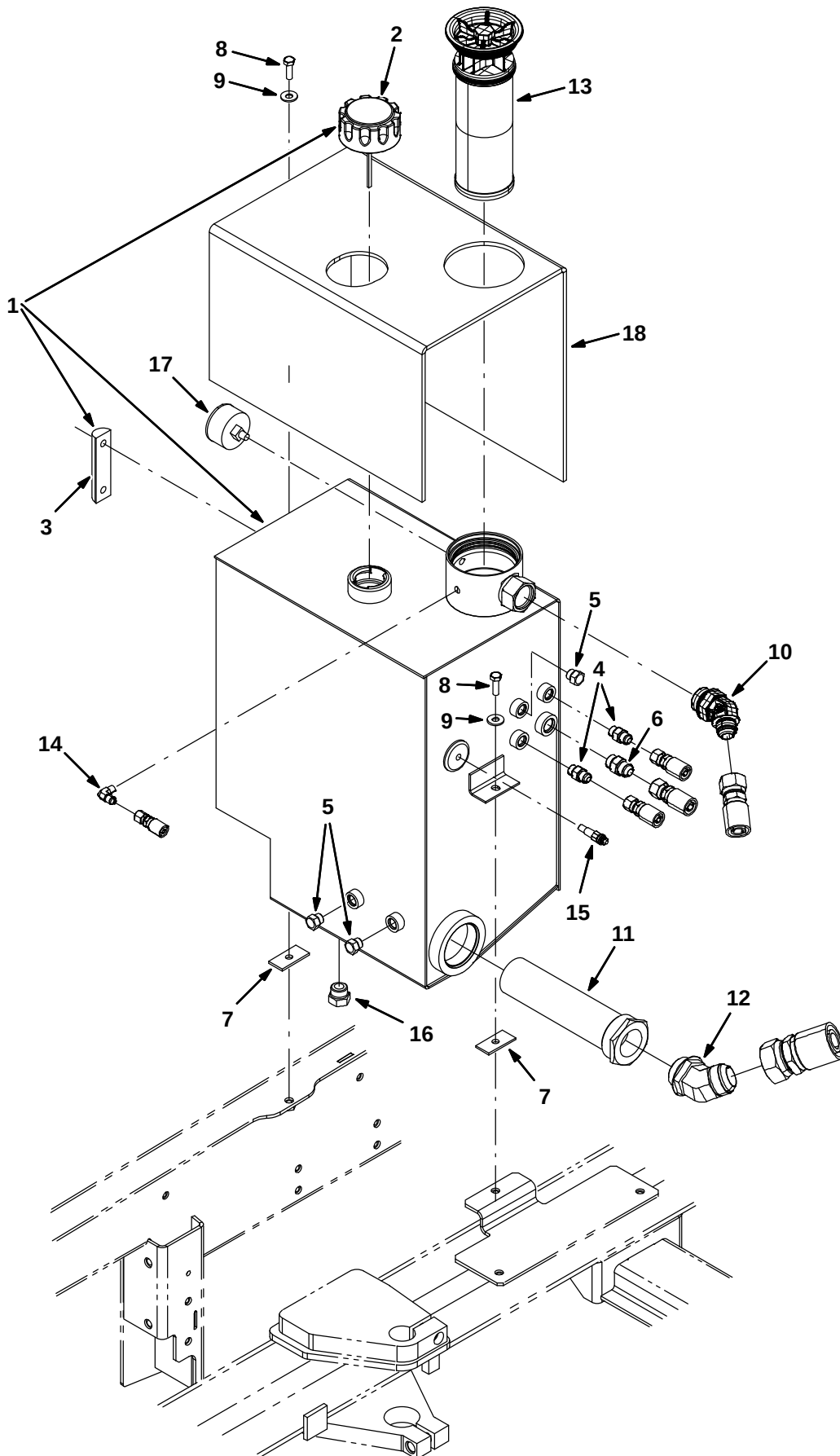
Fig. 70 – Hydraulic Reservoir Group
