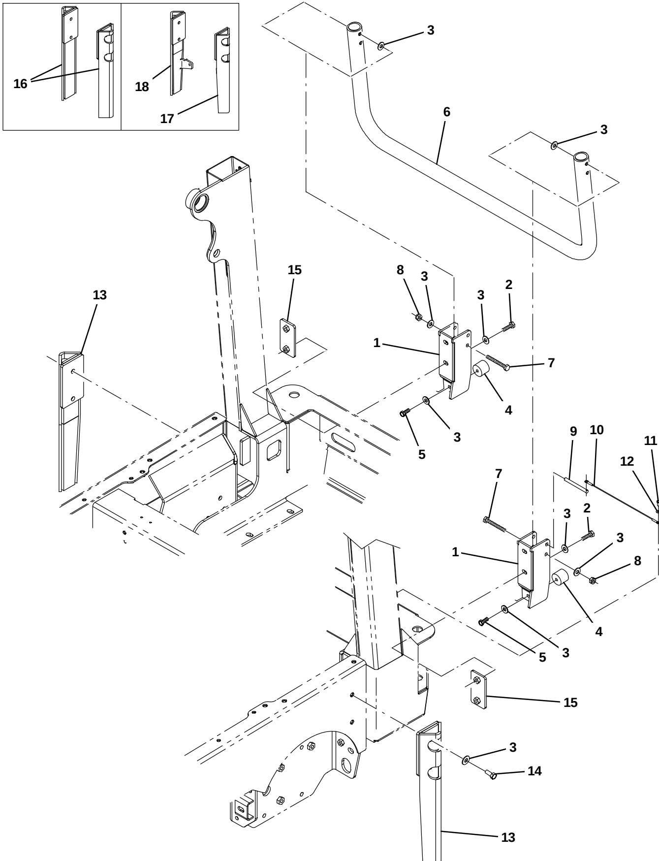
Fig. 33 – Squeegee Guard Kit
