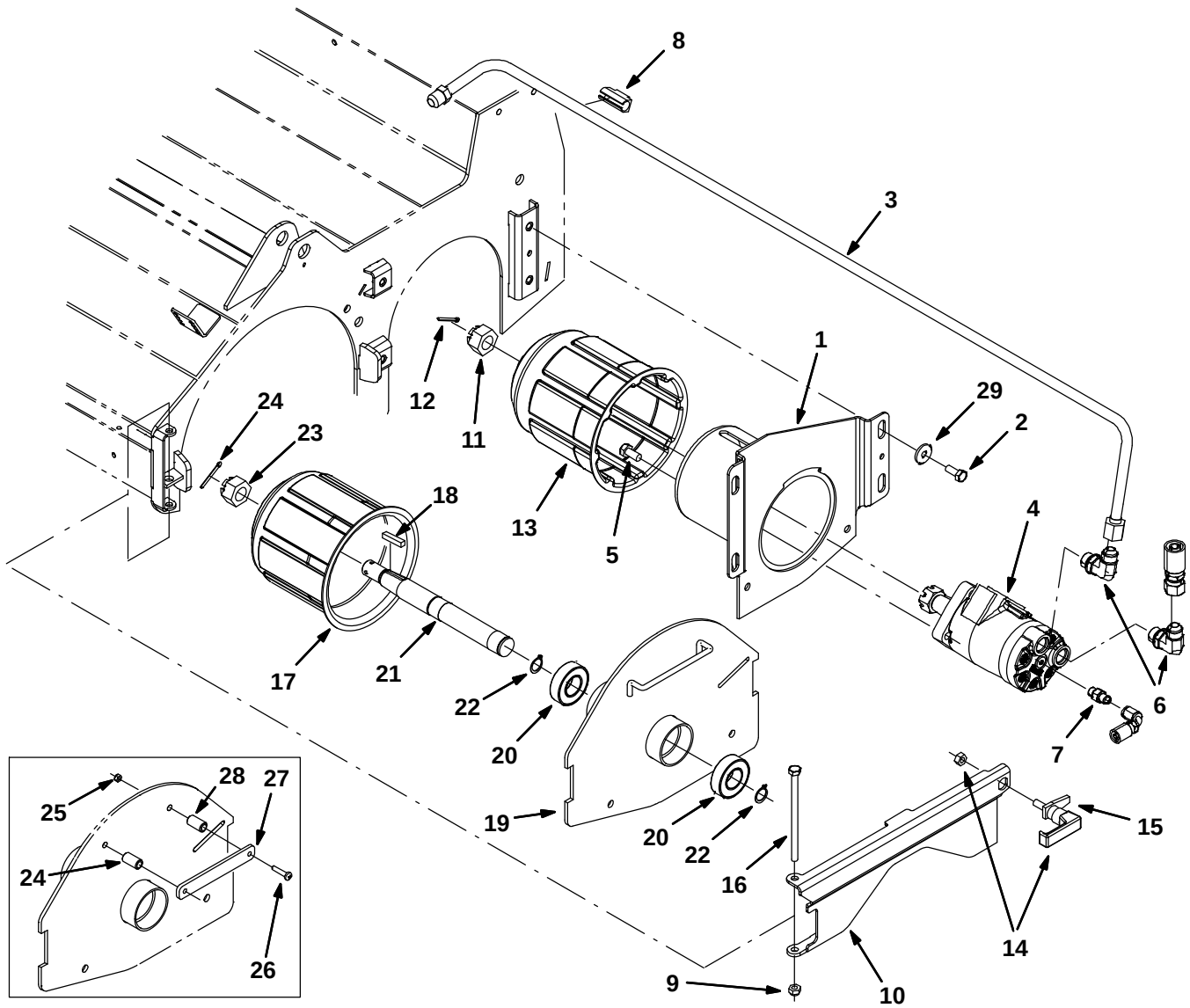
Fig. 43 – Cylindrical Scrub Brush Drive Group, Left Side
