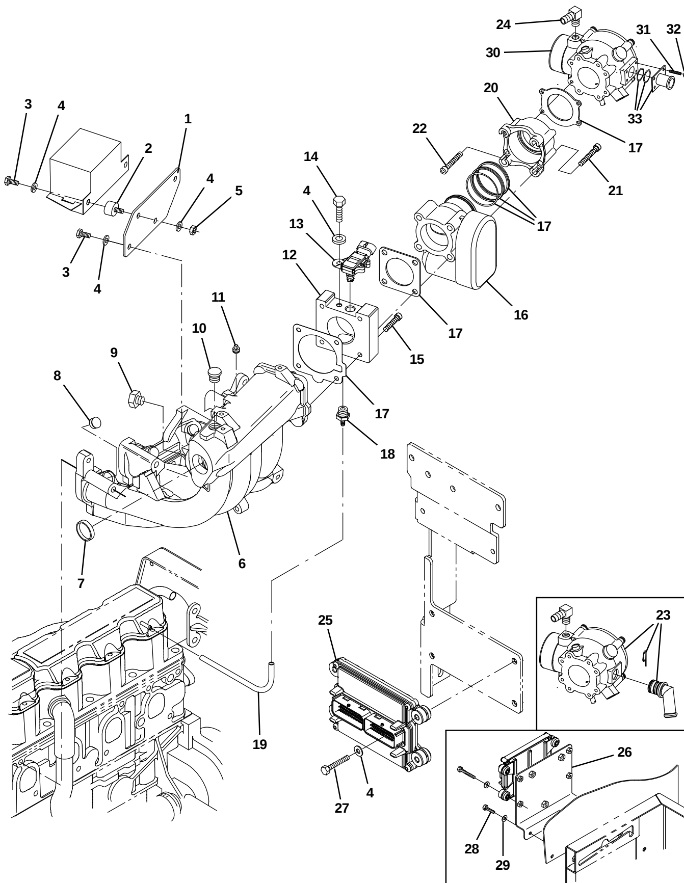
Fig. 16 – Engine EFI Group, LPG (002000– )
