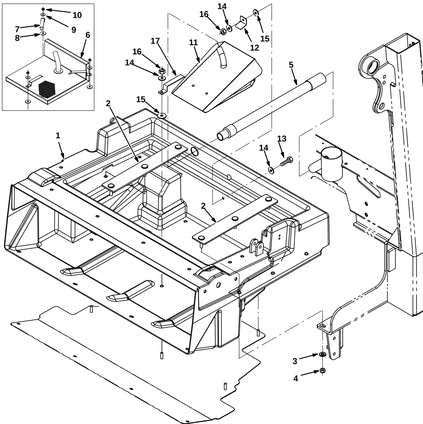
Fig. 38 – Hopper and Debris Screen Group
