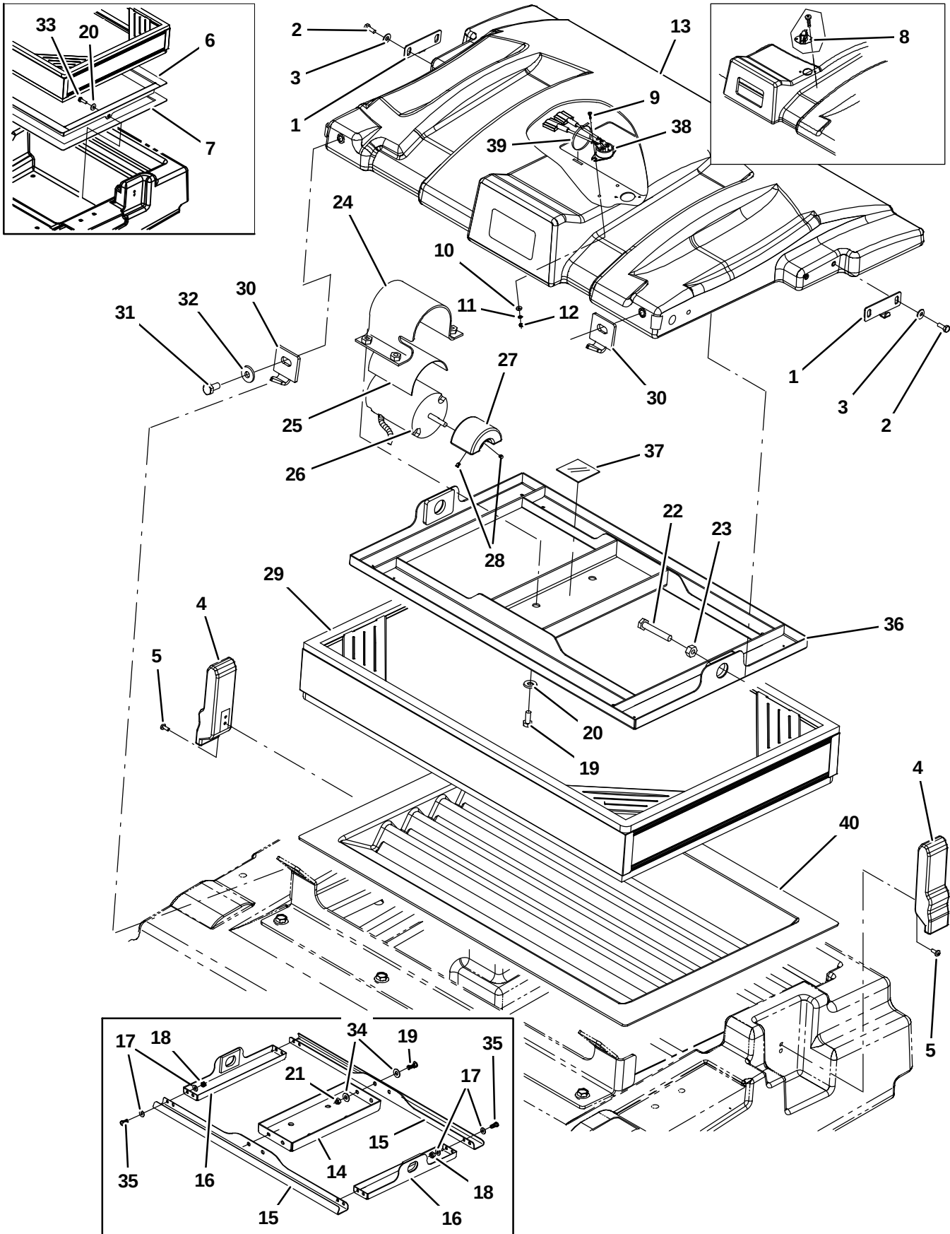
Fig. 39 – Hopper Cover and Dust Filter Group
