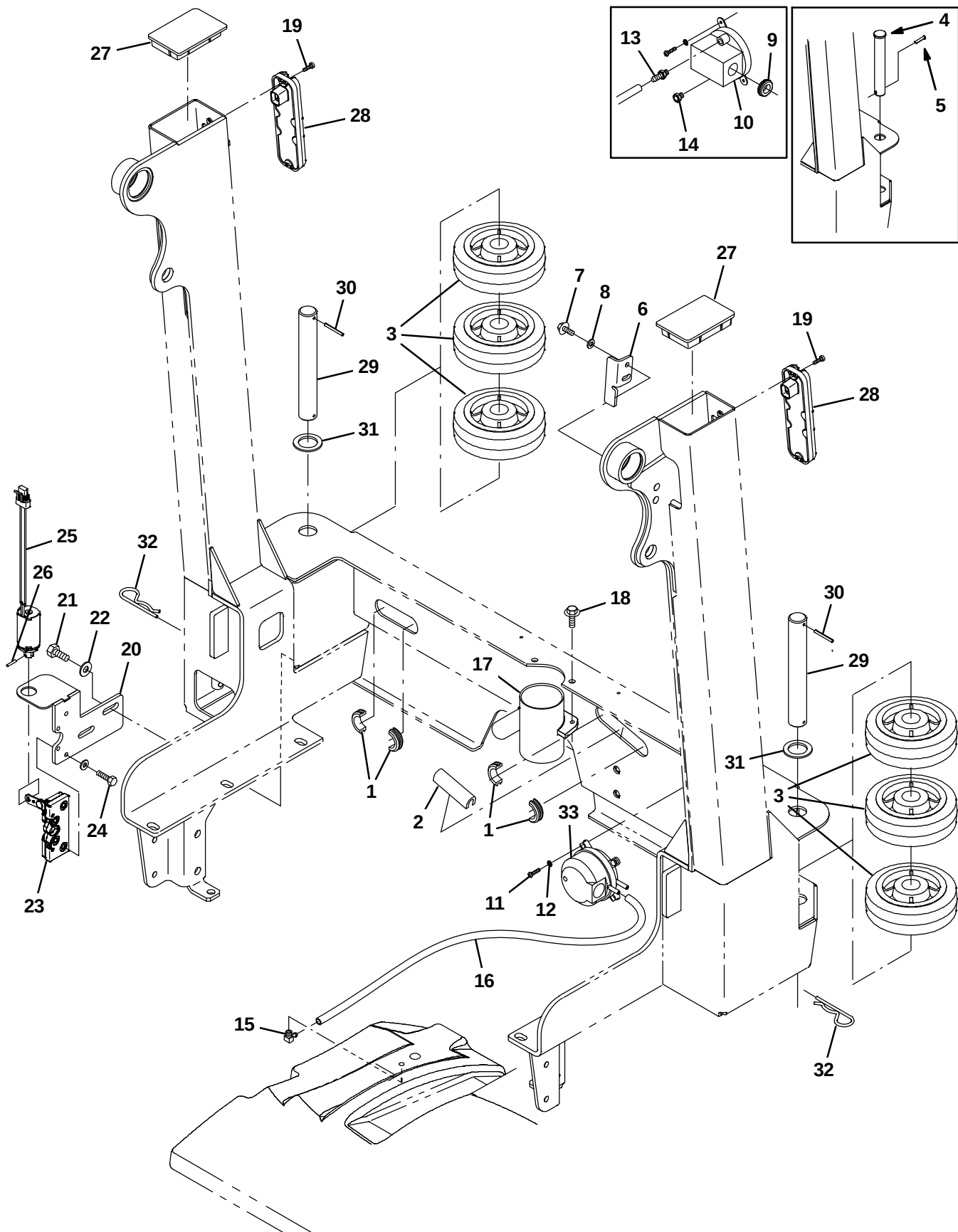
Fig. 40 – Hopper Bumper Group
