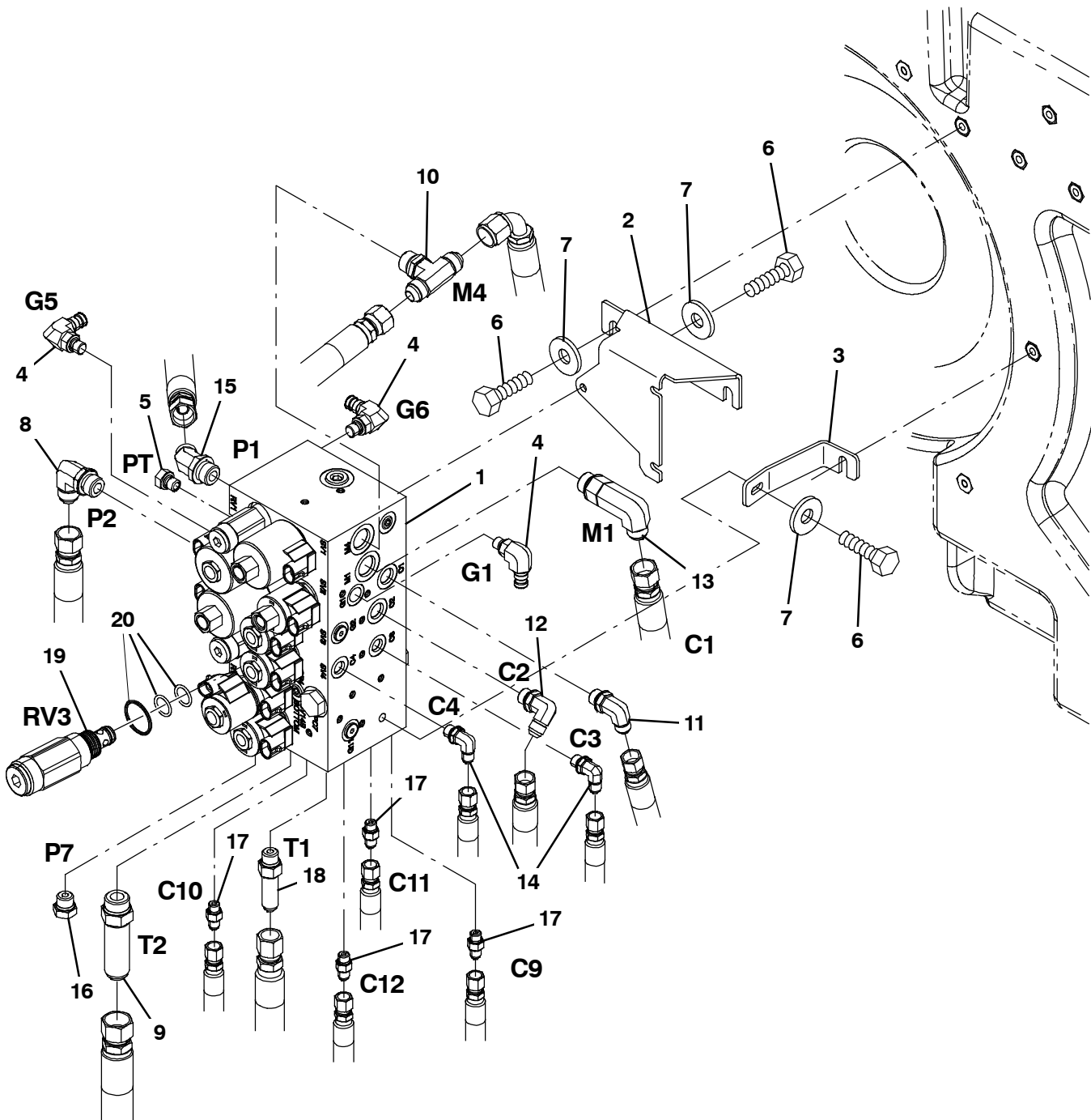
Fig. 72 - Hydraulic Valve Group (002700- )
