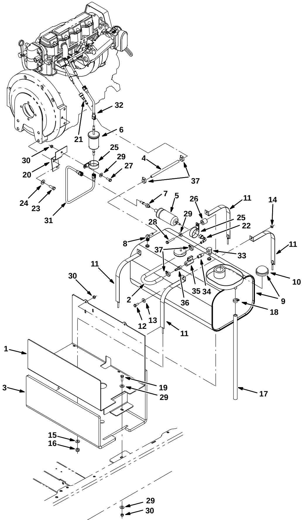
Fig. 19 – Engine Fuel Tank Group, Gasoline (000000–001999)
