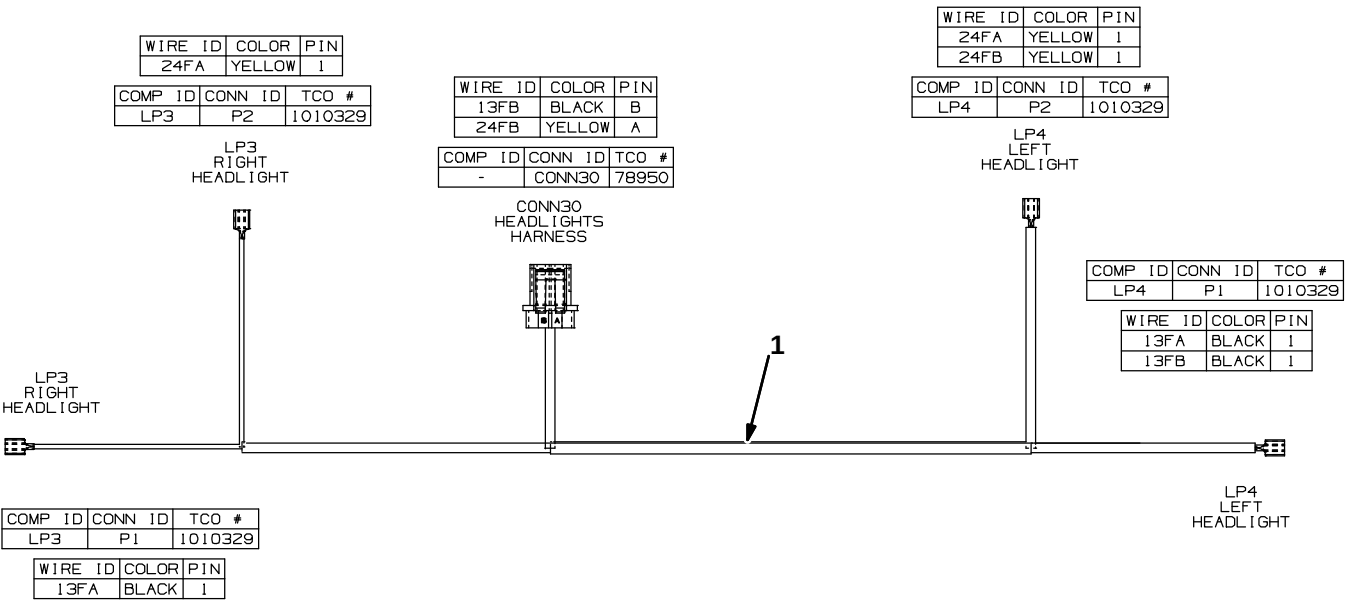
Fig. 83 – Electrical Wire Harness Group, Headlight
