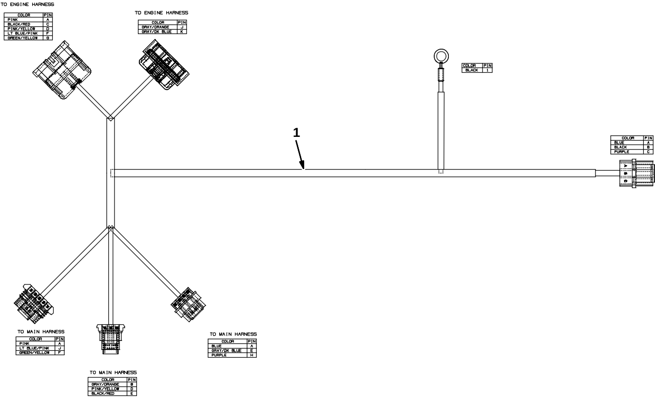
Fig. 87 – Electrical Wire Harness Group, Gasoline/LPG Engine Adapter Harness
