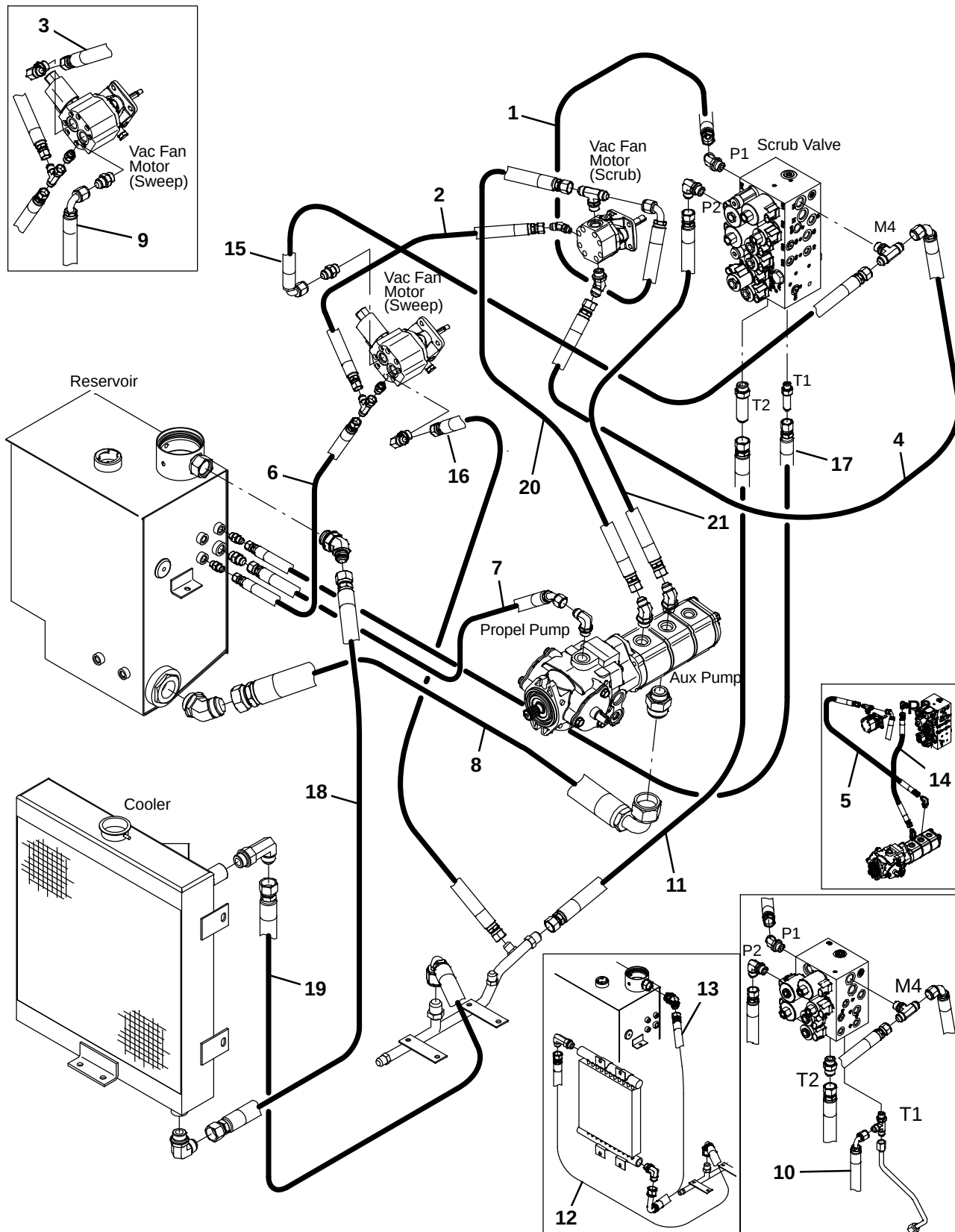
Fig. 65 – Hydraulic Hose Group, Pump and Vacuum Fans
