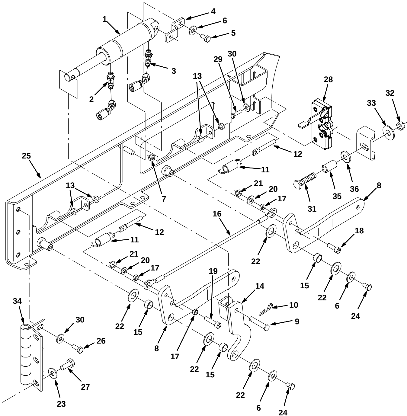
Fig. 51 – Squeegee Lift Group, Right Side
