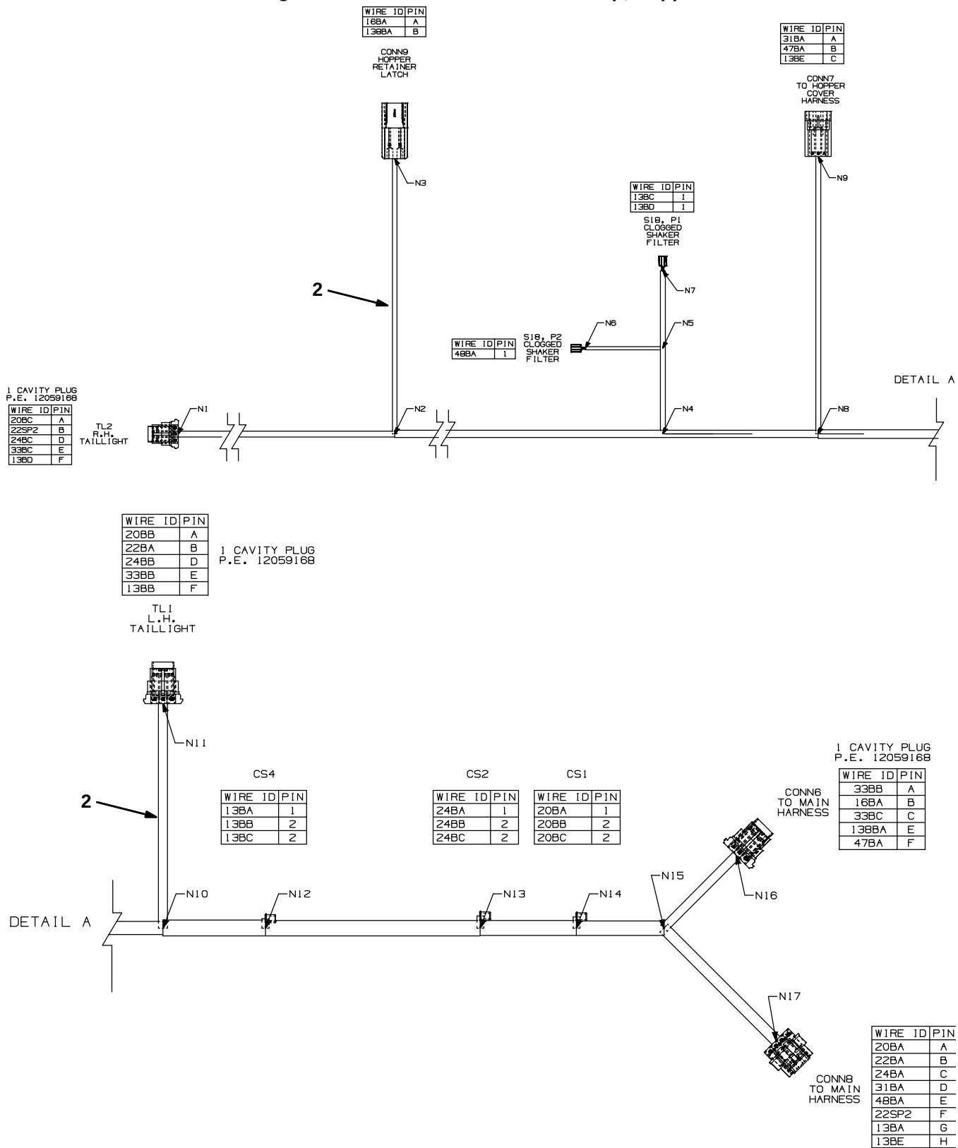
Fig. 84 – Electrical Wire Harness Group, Hopper
