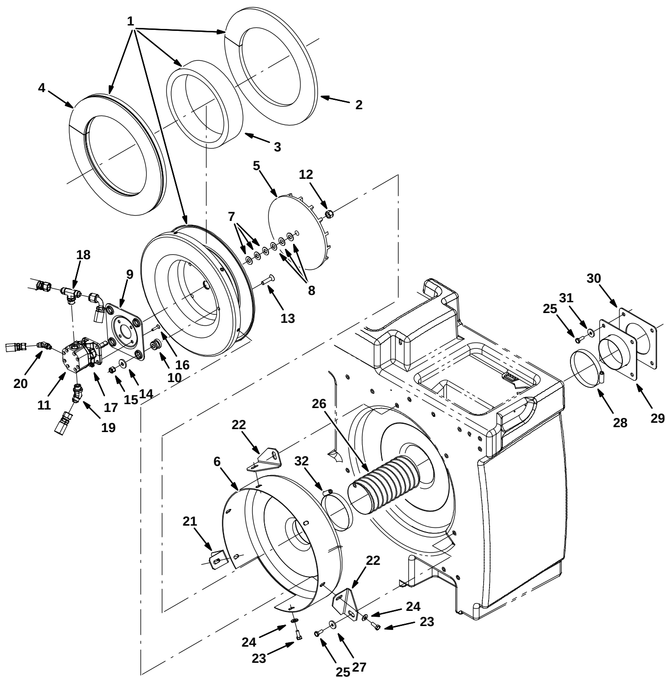
Fig. 59 – Vacuum Fan Group, Scrubbing
