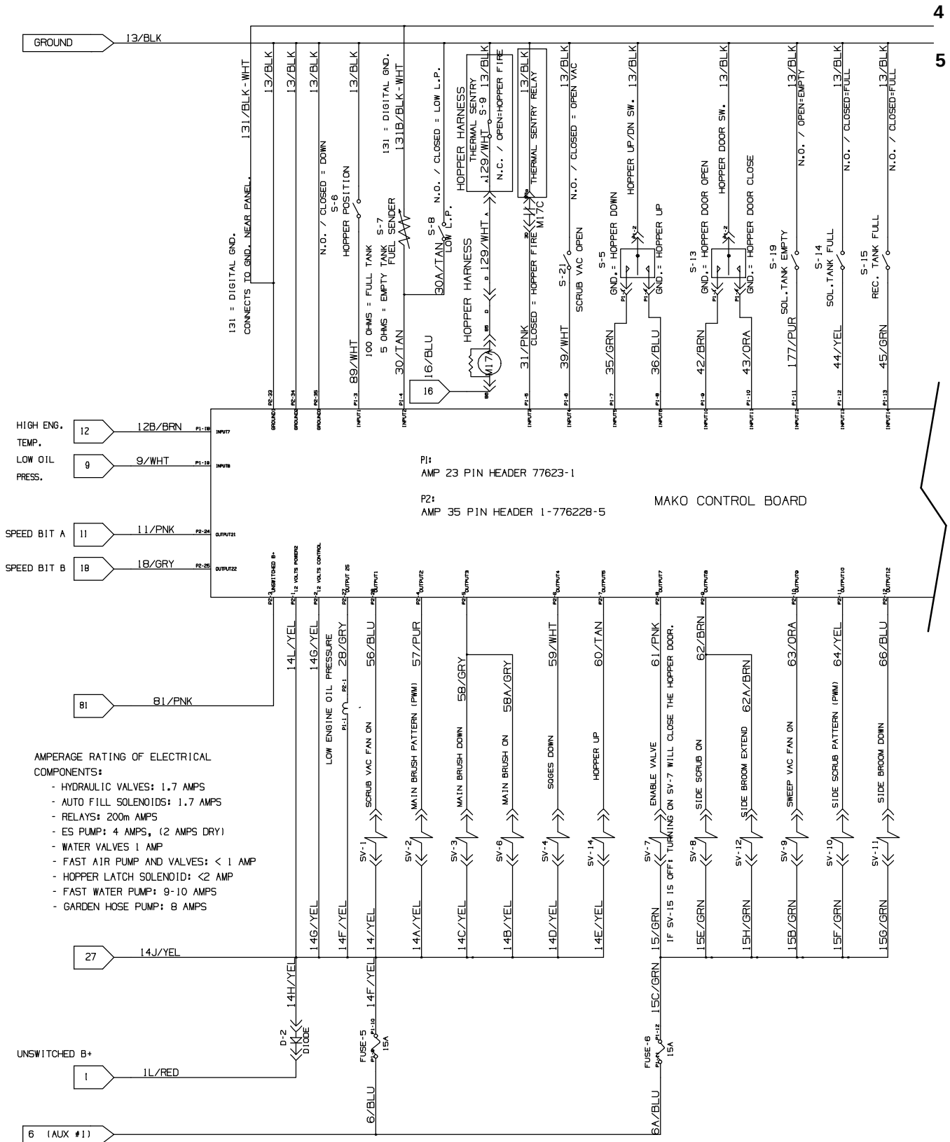
Fig. 76 – Electrical Schematic (003479- )
