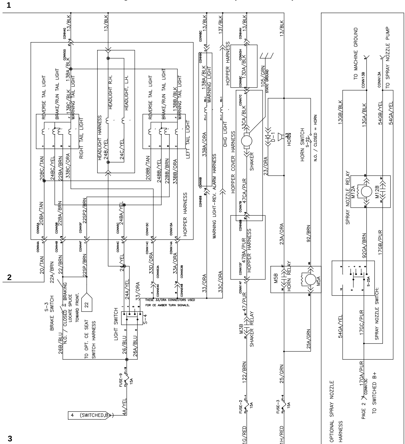
Fig. 76 – Electrical Schematic (003479–
