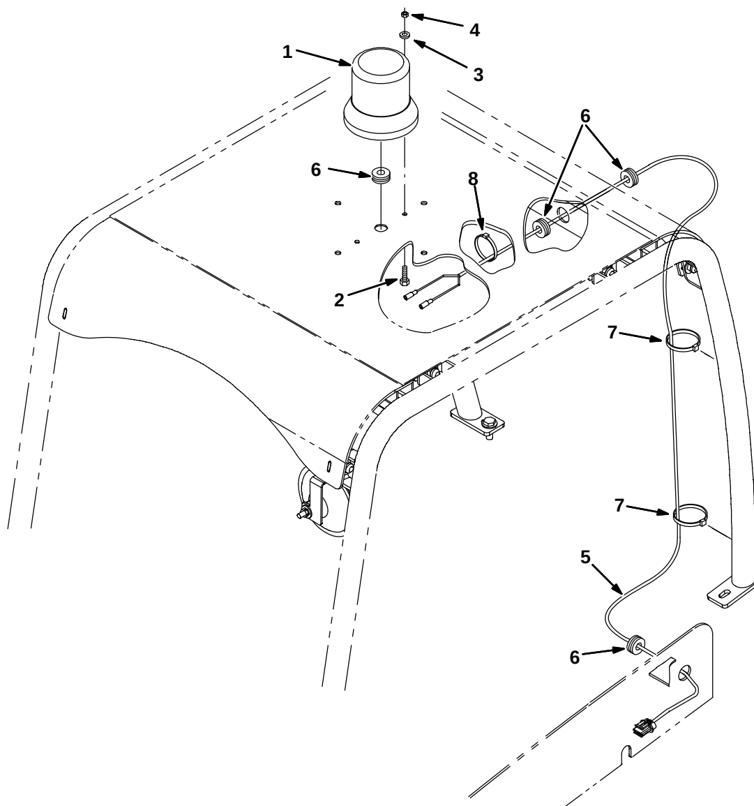
Fig. 27 – Light Kit, Revolving Overhead Guard
