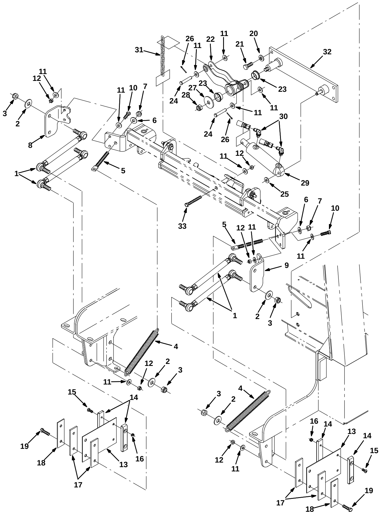
Fig. 47 – Squeegee Lift Group, Rear
