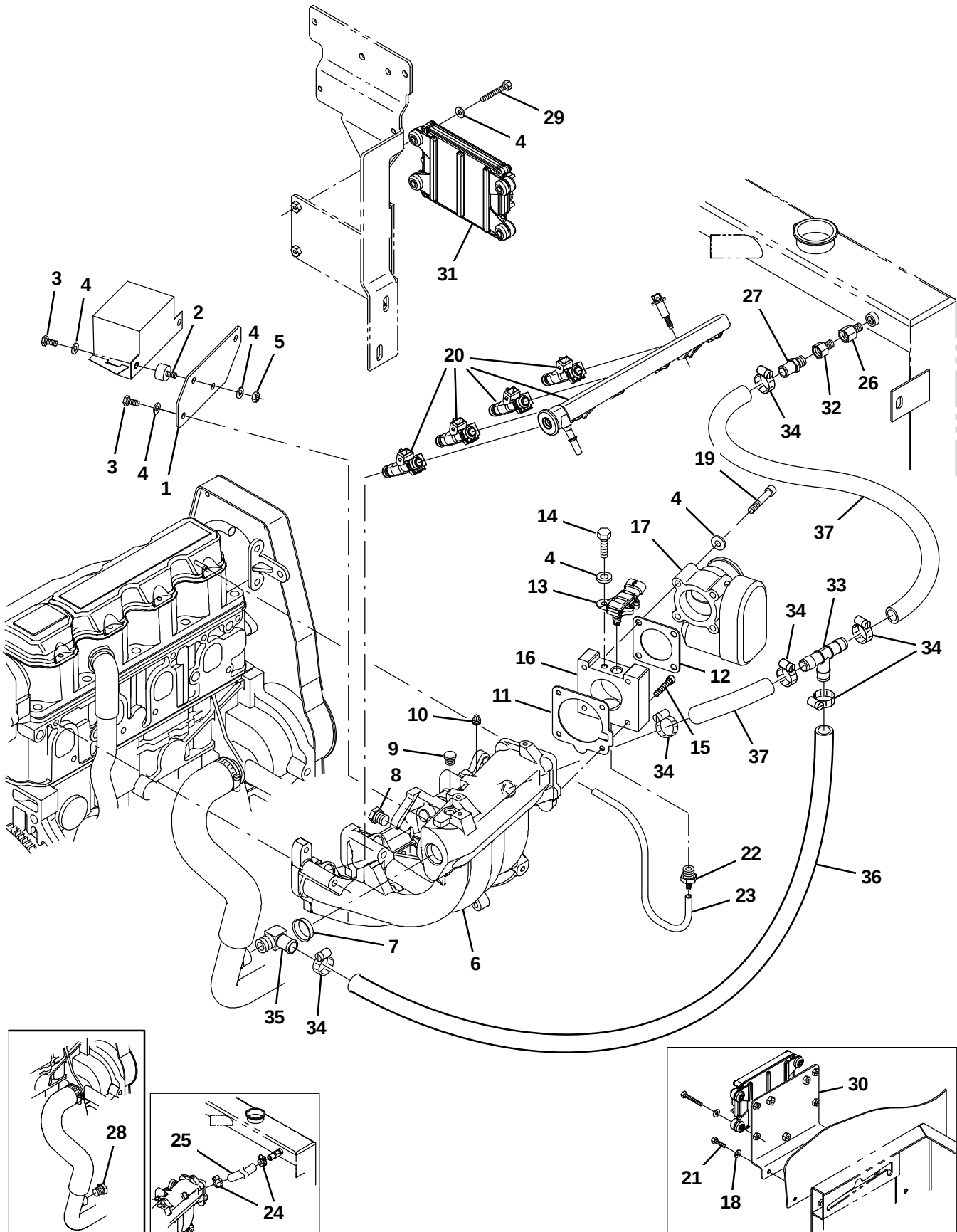
Fig. 14 – Engine EFI Group, Gasoline (003123– )
