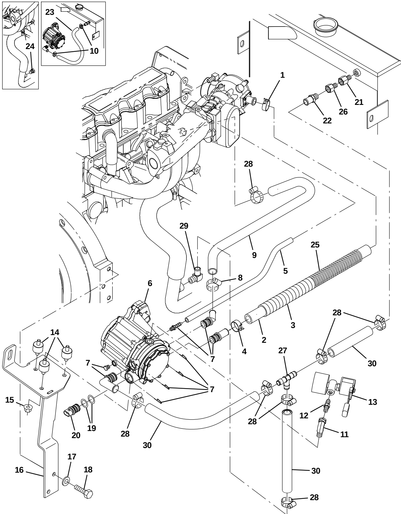
Fig. 18 – Engine Vaporizer Group, LPG (003123– )
