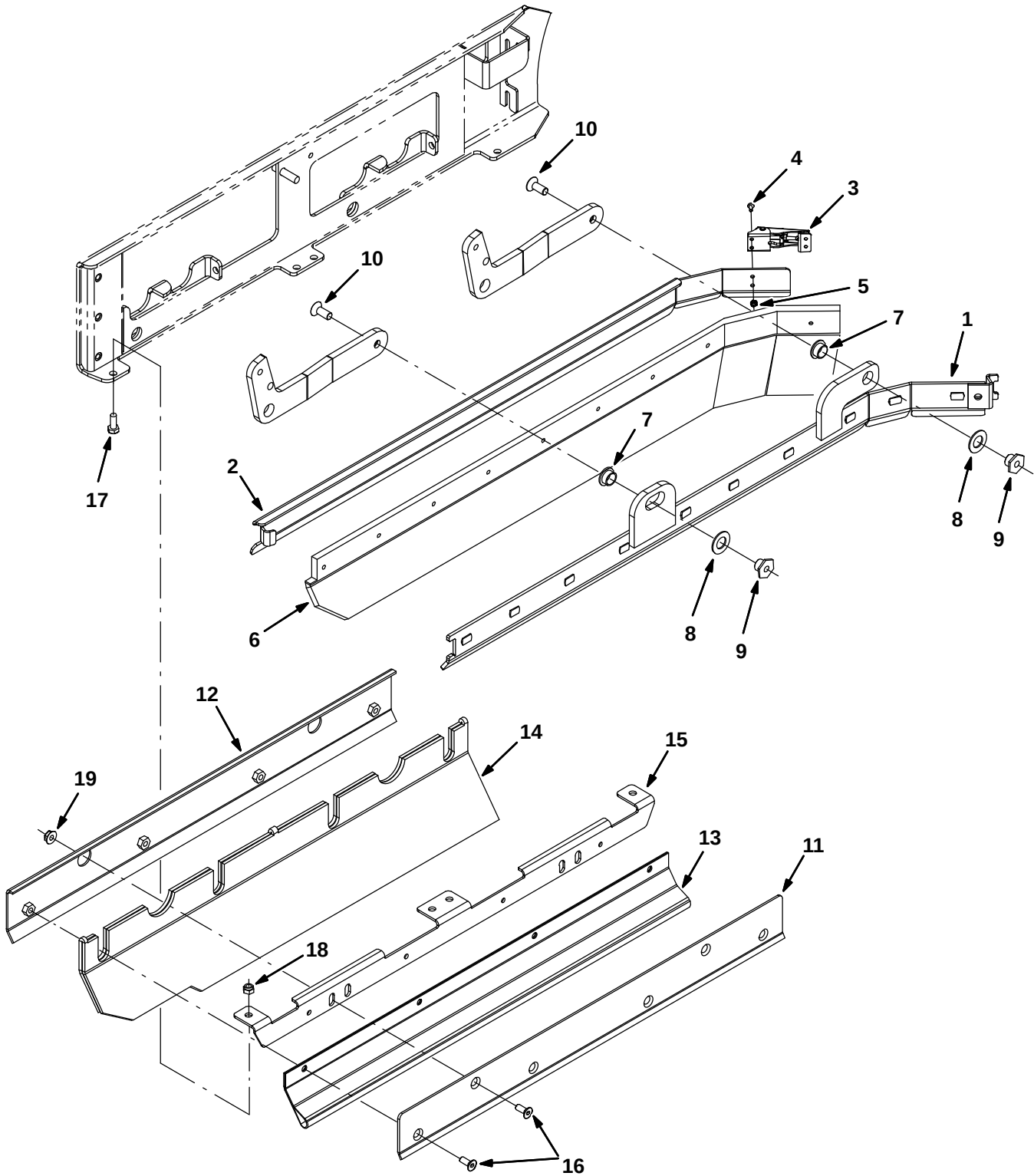
Fig. 50 – Squeegee Group, Right Side
