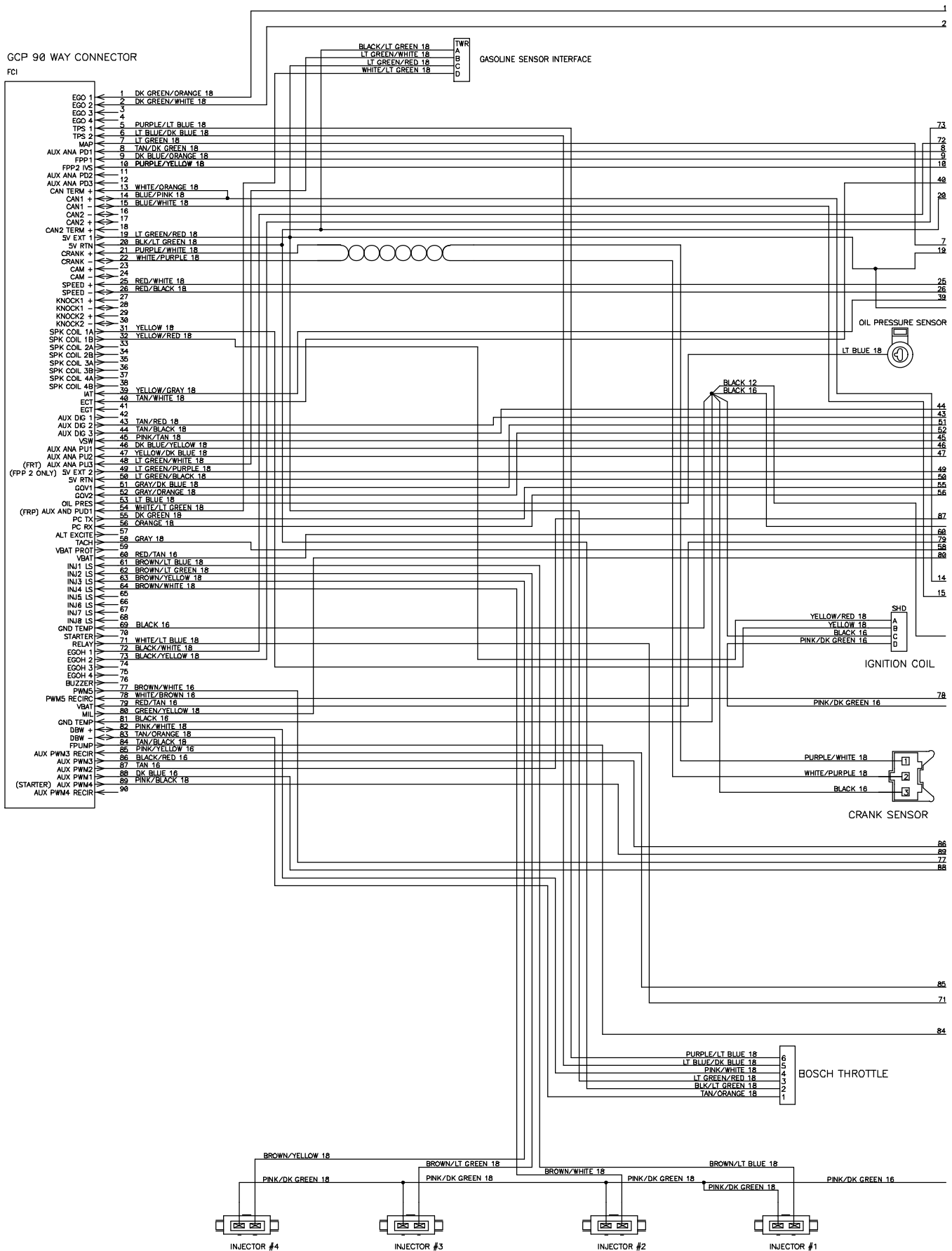
Fig. 78 – Electrical Schematic, Gas Engine Harness (002000-003122)
