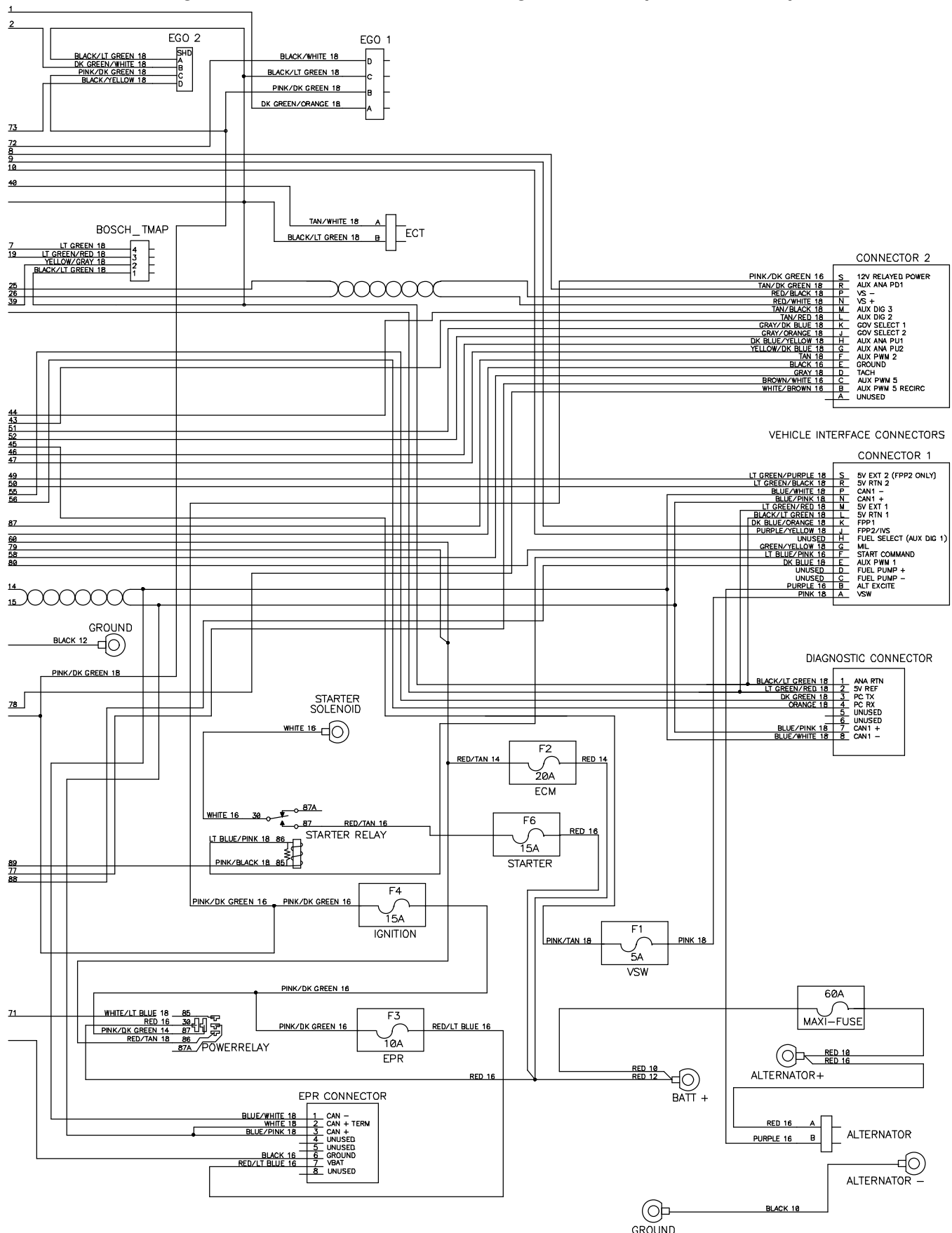
Fig. 80 – Electrical Schematic, LPG Engine Harness (002000-003122)
