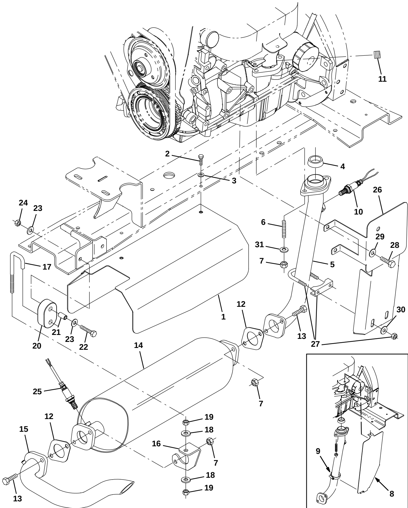
Fig. 28 – Engine Muffler Group (002000– )
