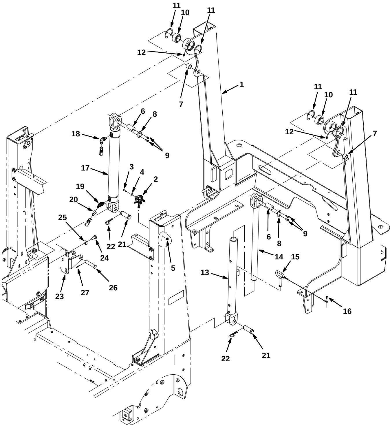
Fig. 37 – Hopper Lift Arms Group
