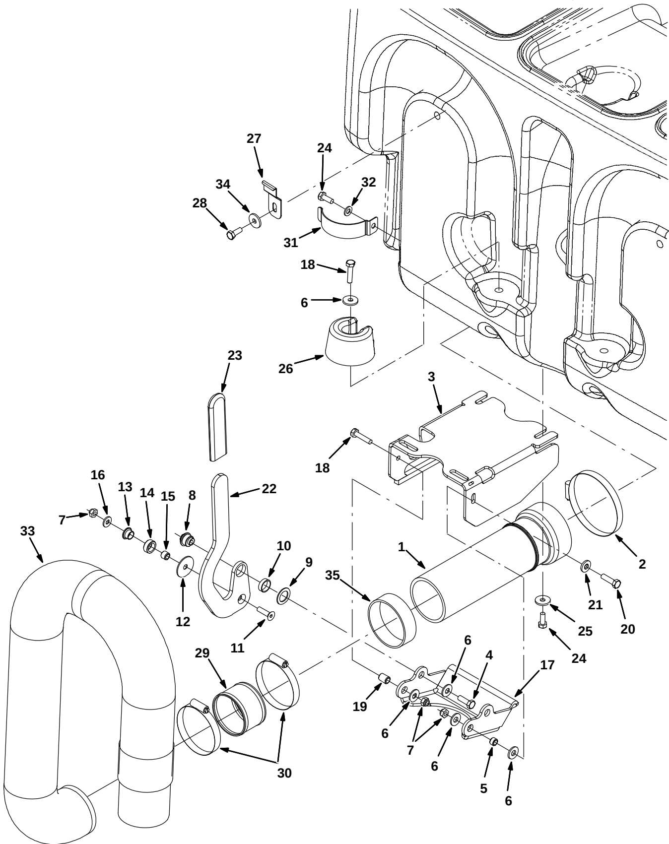
Fig. 58 – Recovery Tank Drain Group
