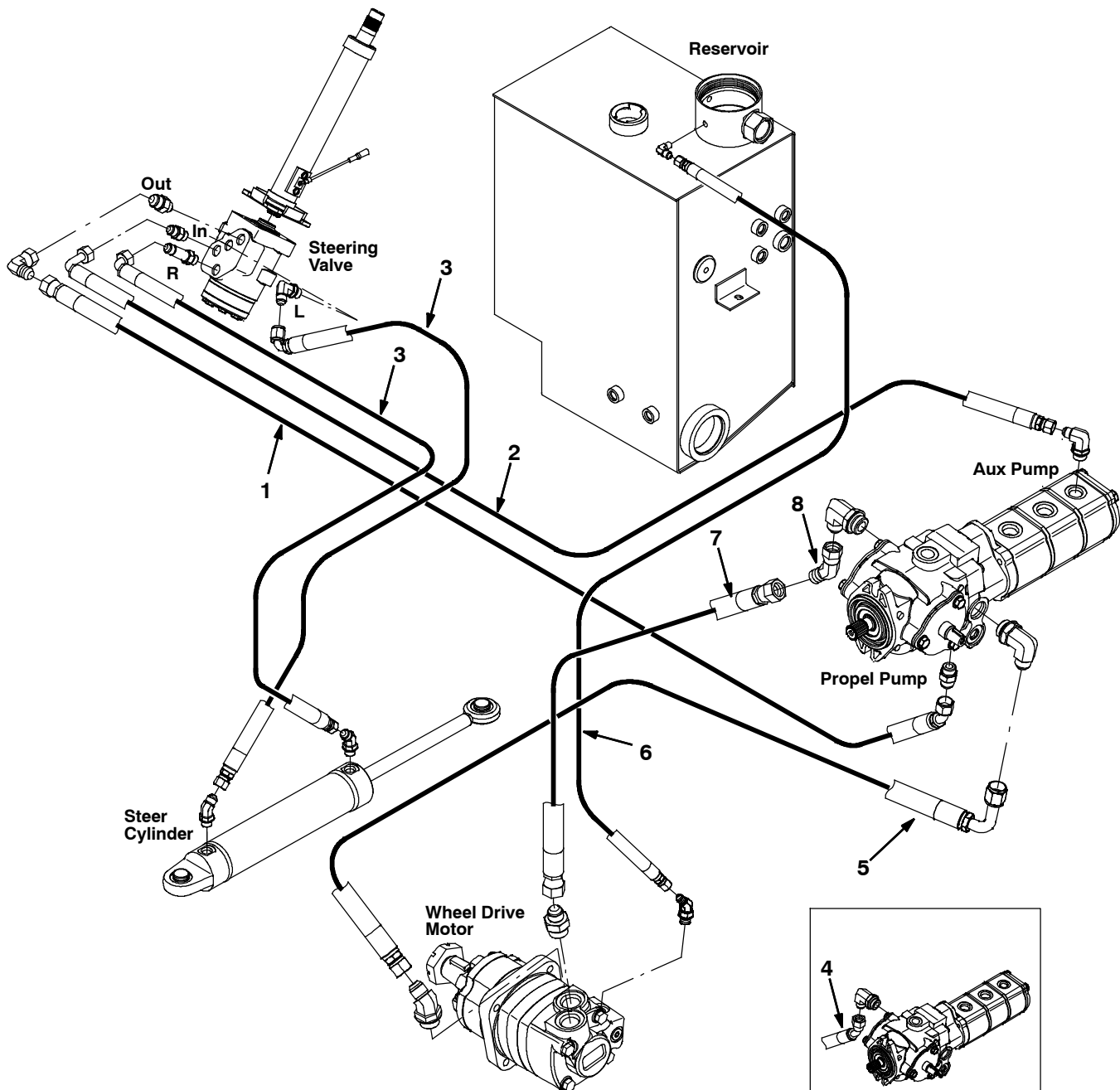
Fig. 64 - Hydraulic Hose Group, Steering and Propel
