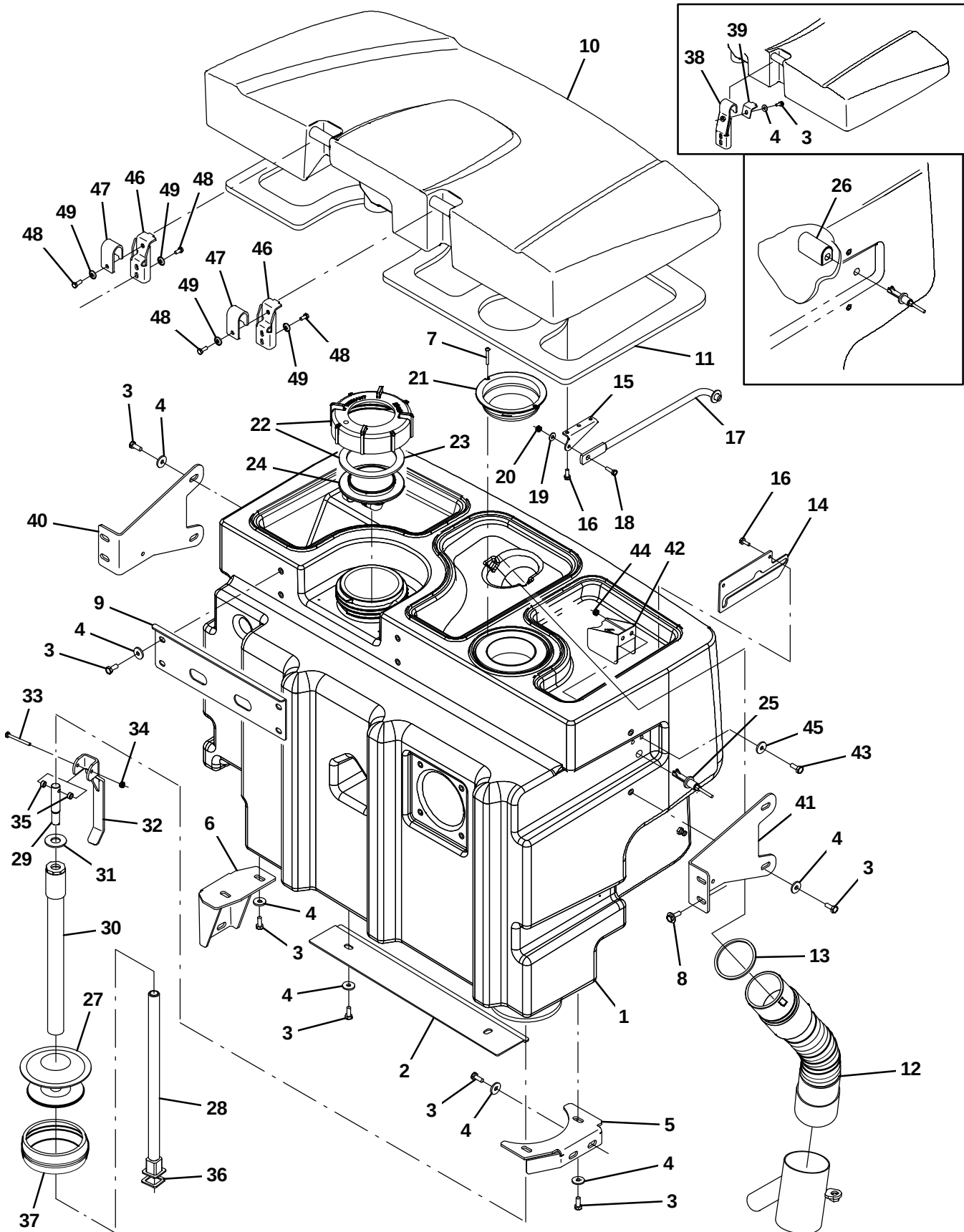
Fig. 57 – Recovery Tank Group
