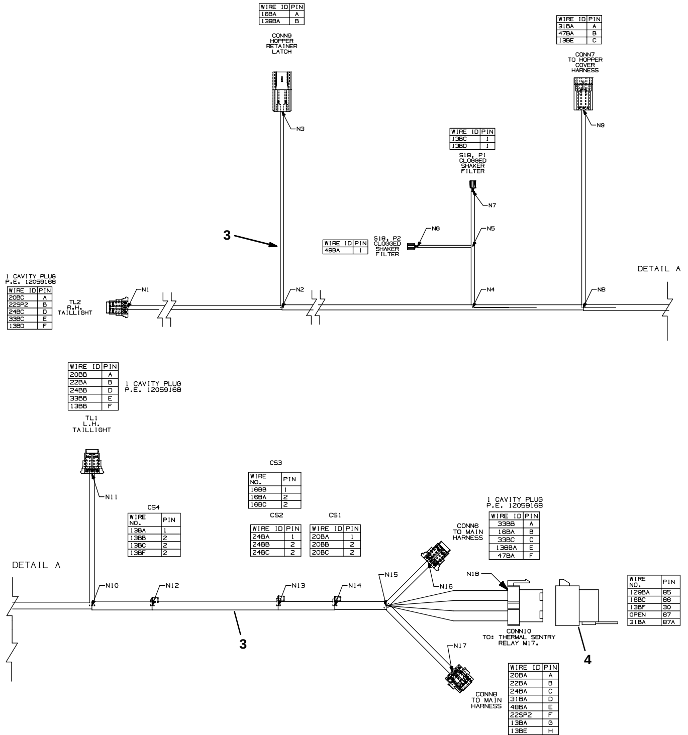
Fig. 84 – Electrical Wire Harness Group, Hopper
