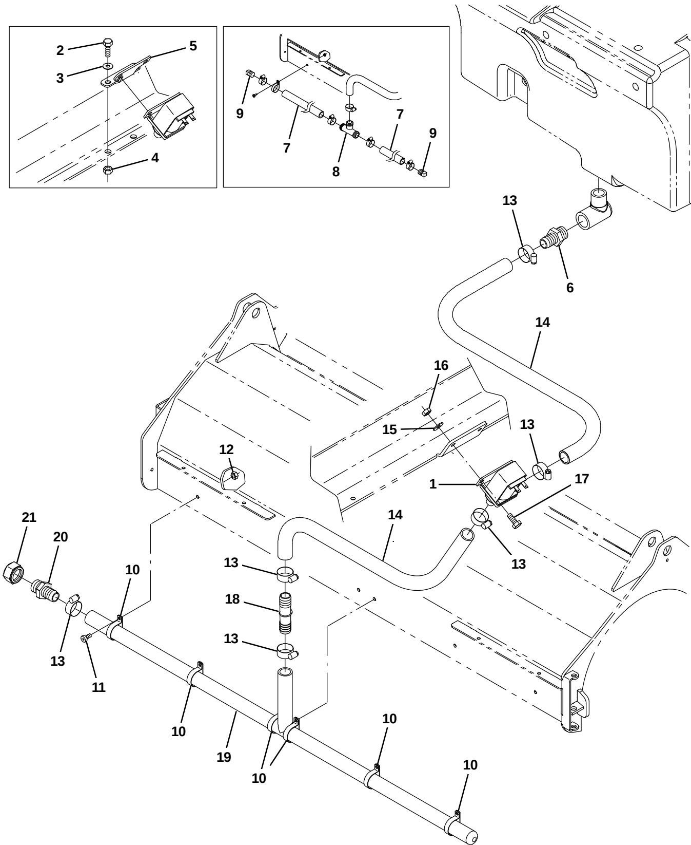
Fig. 56 – Solution Control Group
