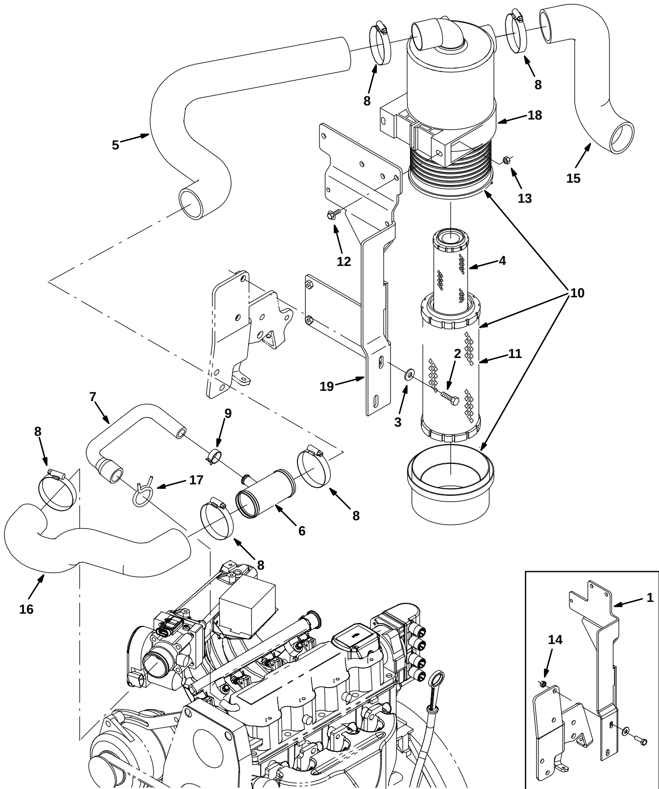
Fig. 23 – Engine Air Cleaner Group, Gasoline (002000– )
