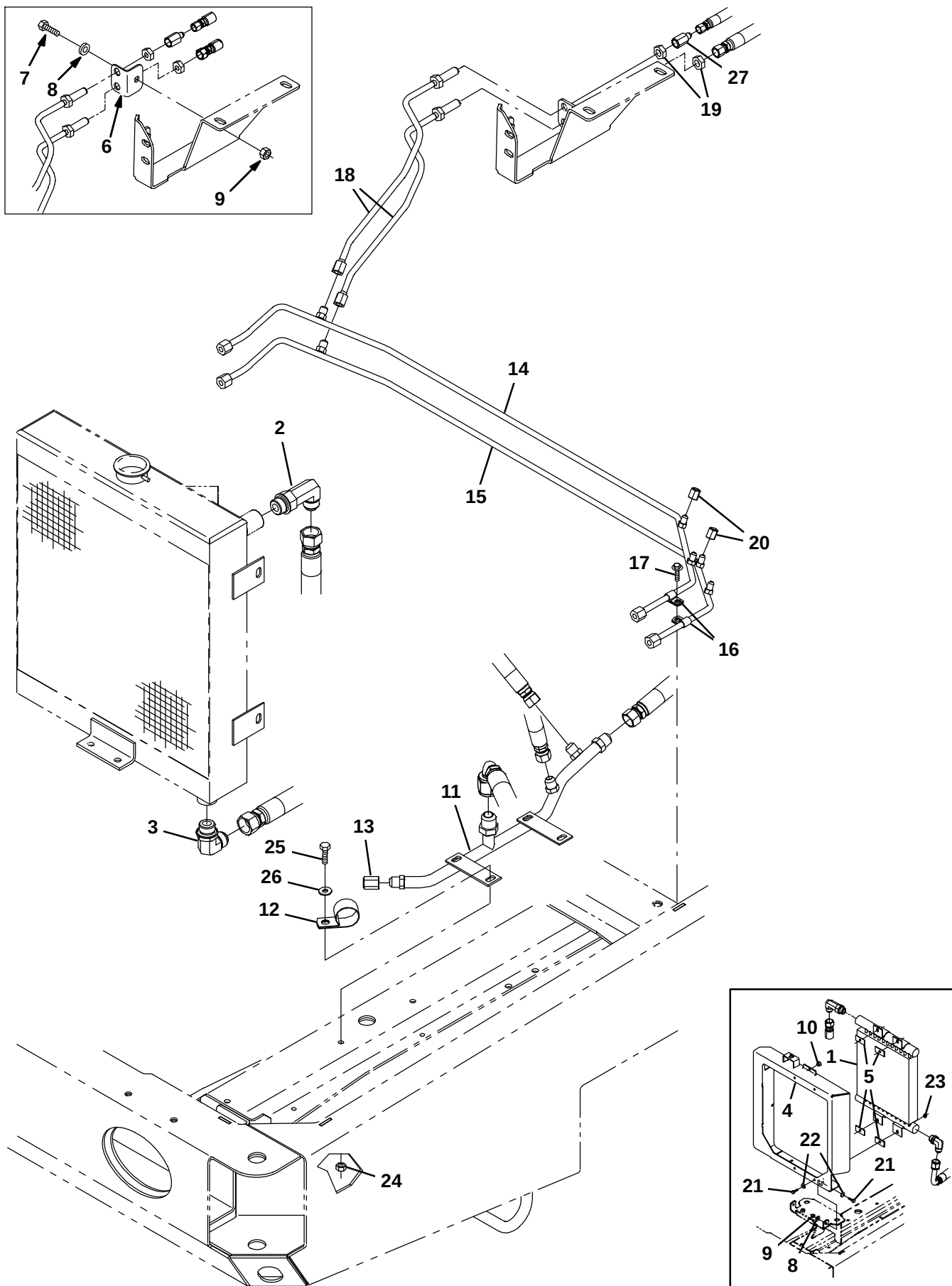
Fig. 69 – Hydraulic Cooler and Tubes Group
