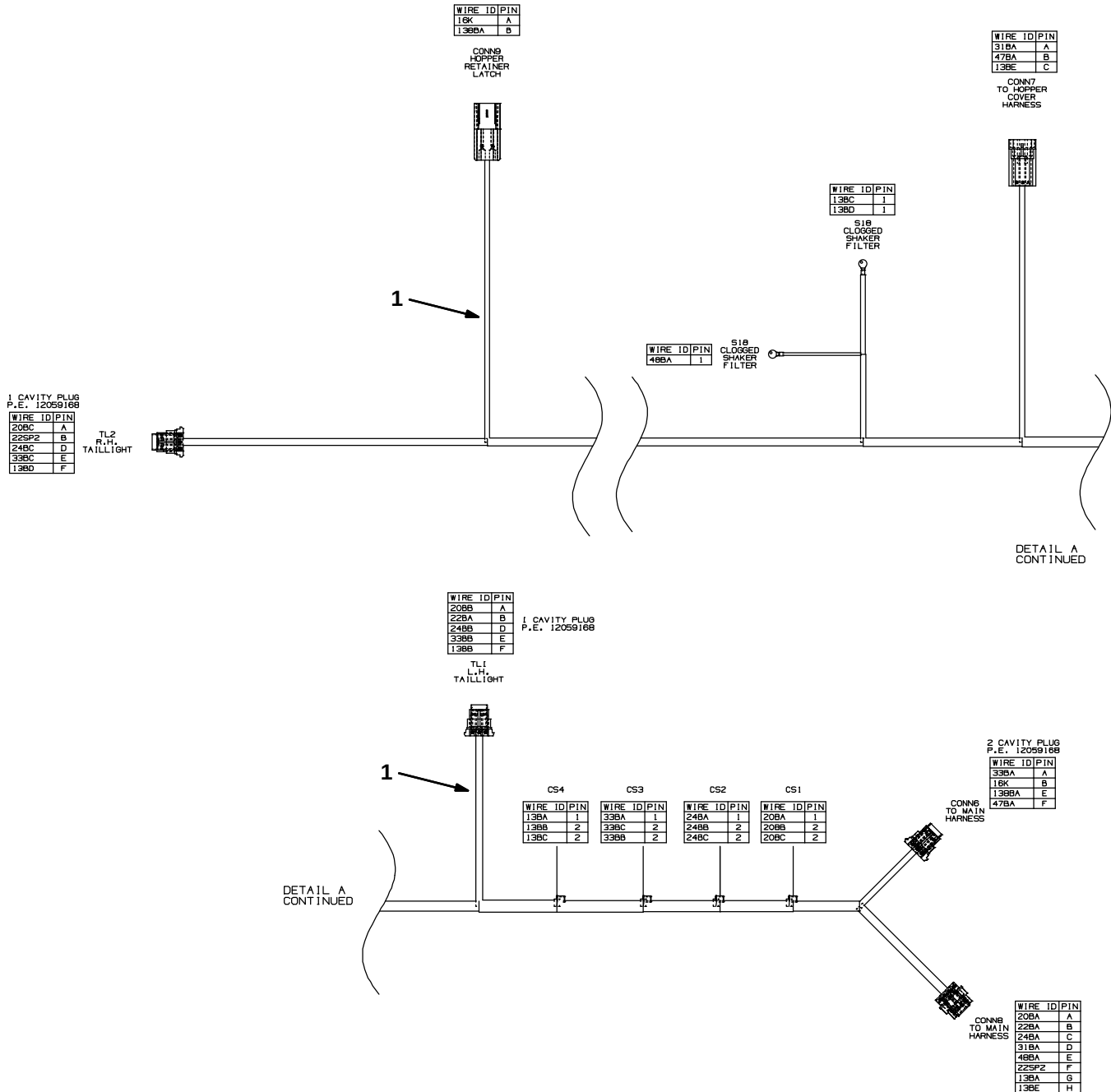
Fig. 84 – Electrical Wire Harness Group, Hopper
