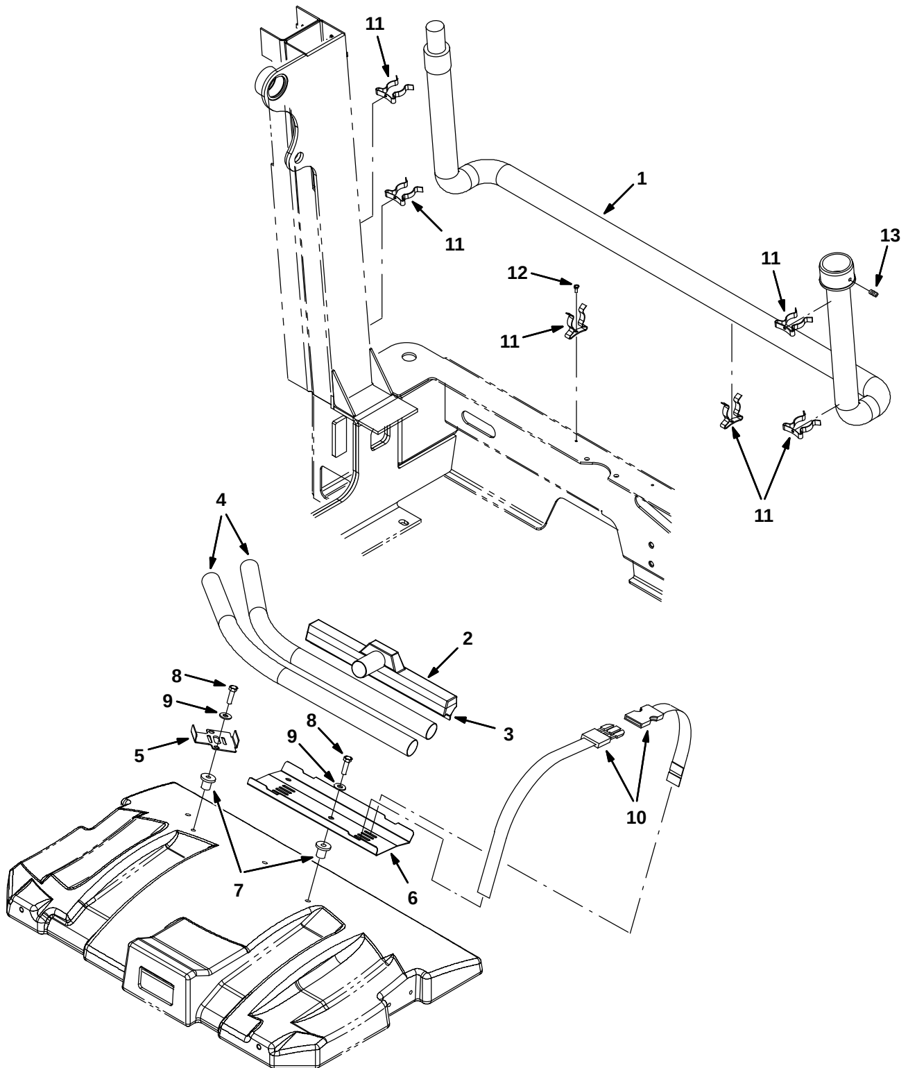
Fig. 29 – Vacuum Wand Kit (000000-002406)
