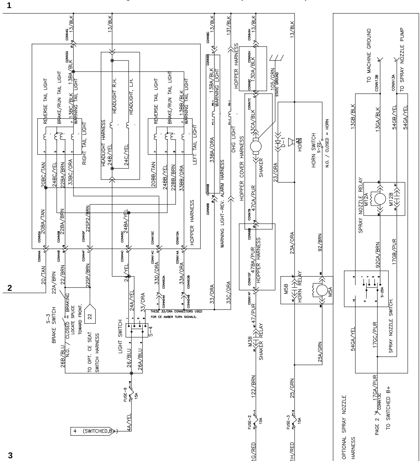
Fig. 75 – Electrical Schematic (002533–003478)
