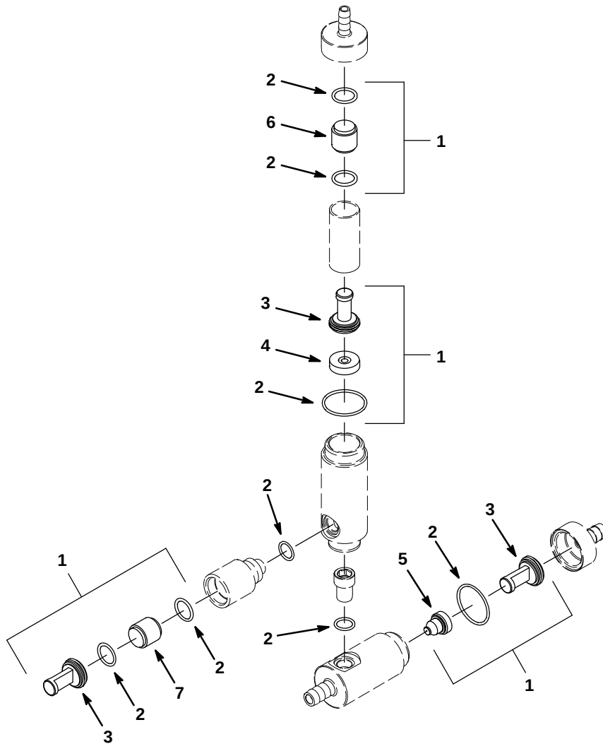
Fig. 16 – FaST Injector Assembly Breakdown, 9004515
