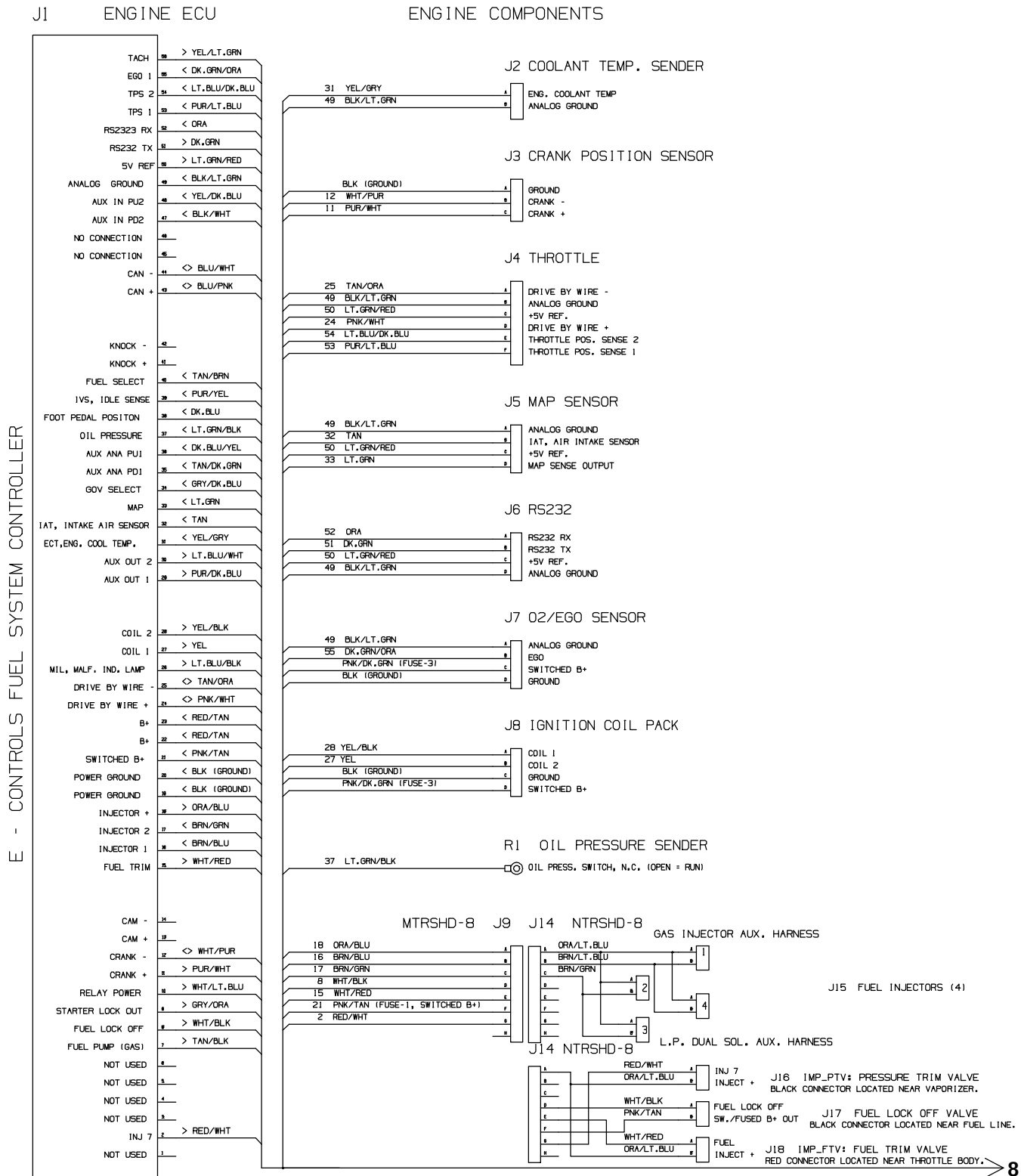
Fig. 77 – Electrical Schematic, Gas/LPG Engine Harness (000000–001999)
