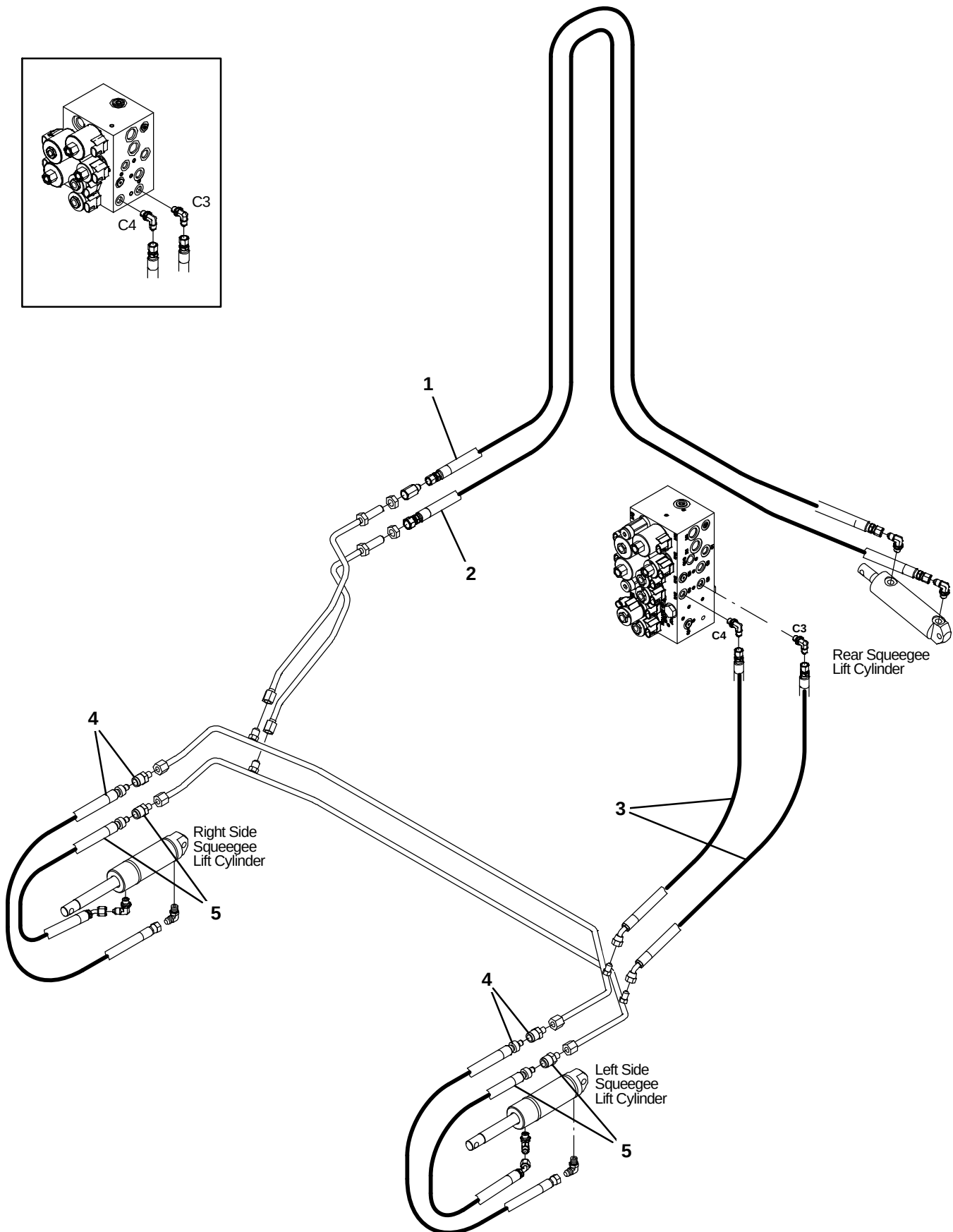
Fig. 67 – Hydraulic Hose Group, Squeegee Lift
