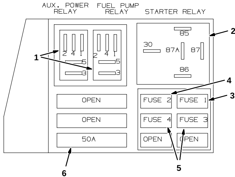
Fig. 86 – Electrical Wire Harness Group, Gasoline/LPG Engine
