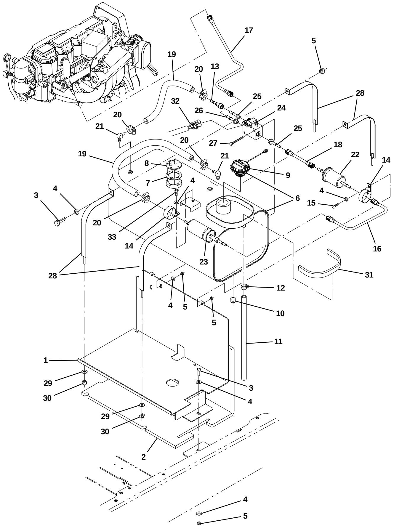
Fig. 20 – Engine Fuel Tank Group, Gasoline (002000– )
