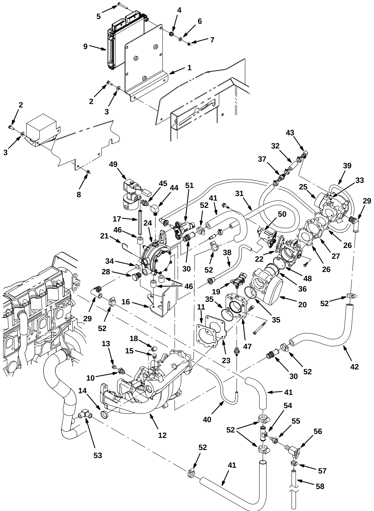
Fig. 15 – Engine EFI Group, LPG (000000–001999)
