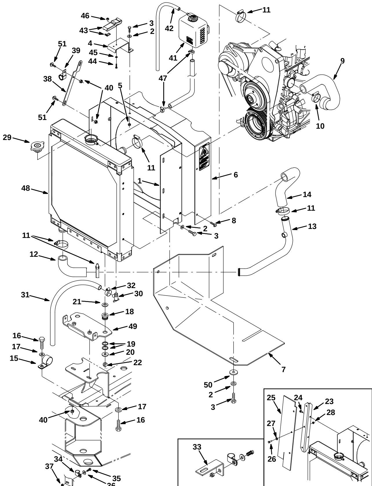
Fig. 29 – Engine Radiator Group (000000–003038)
