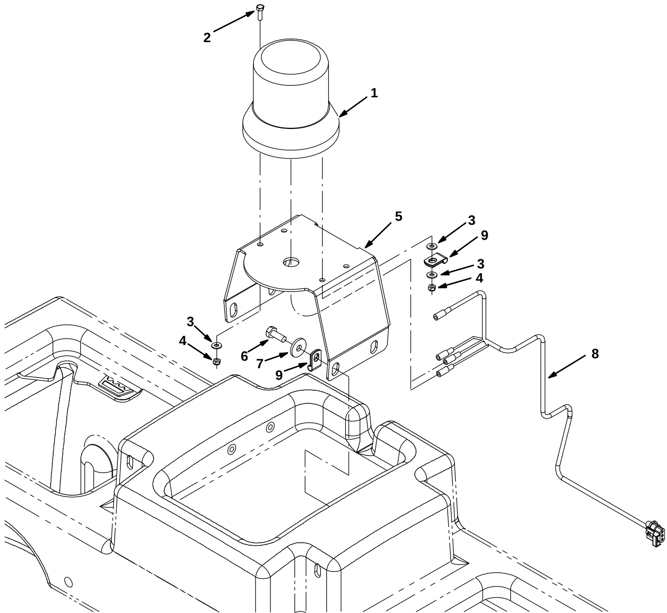
Fig. 25 – Light Kit, Revolving
