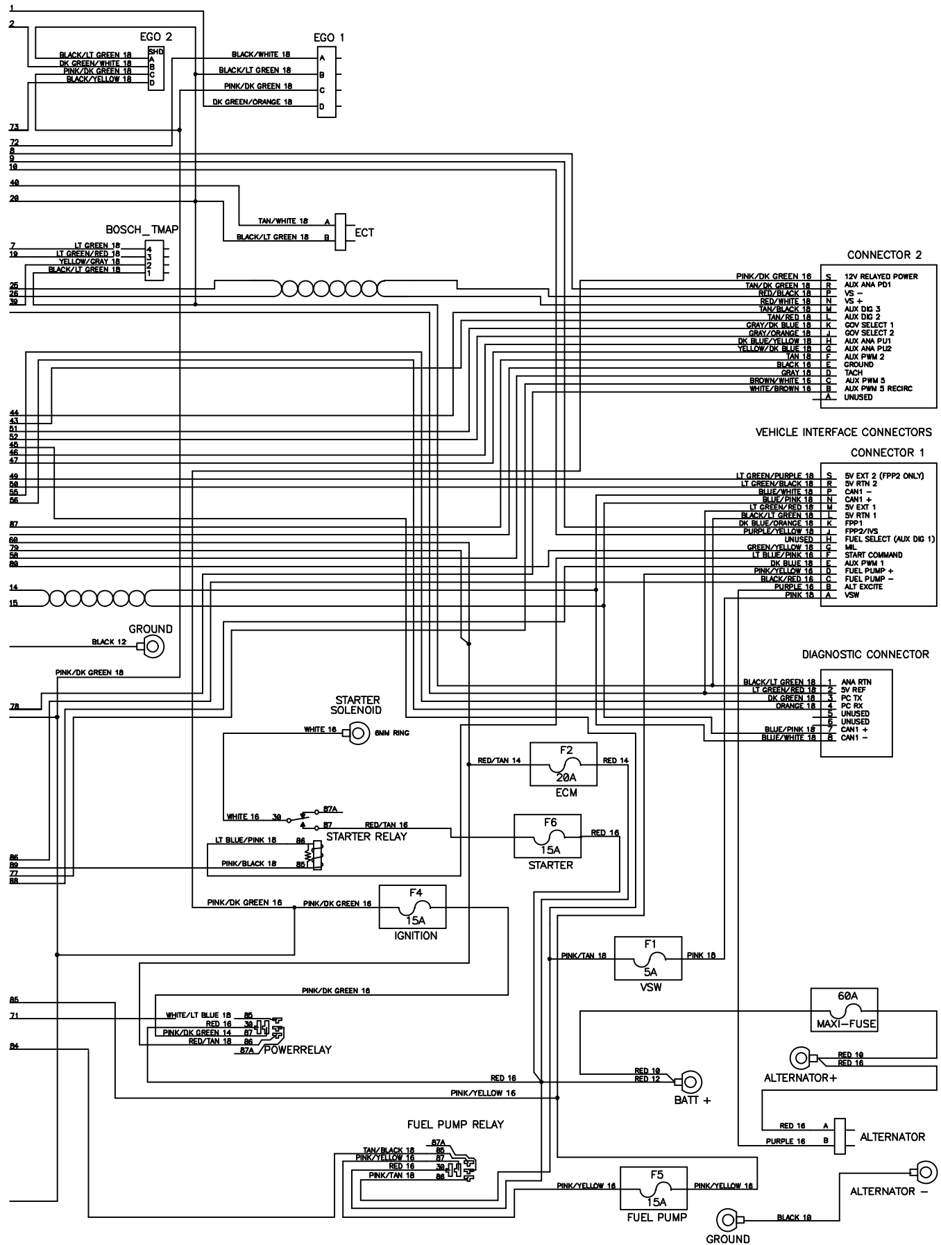
Fig. 79 – Electrical Schematic, Gas Engine Harness (003123– )
