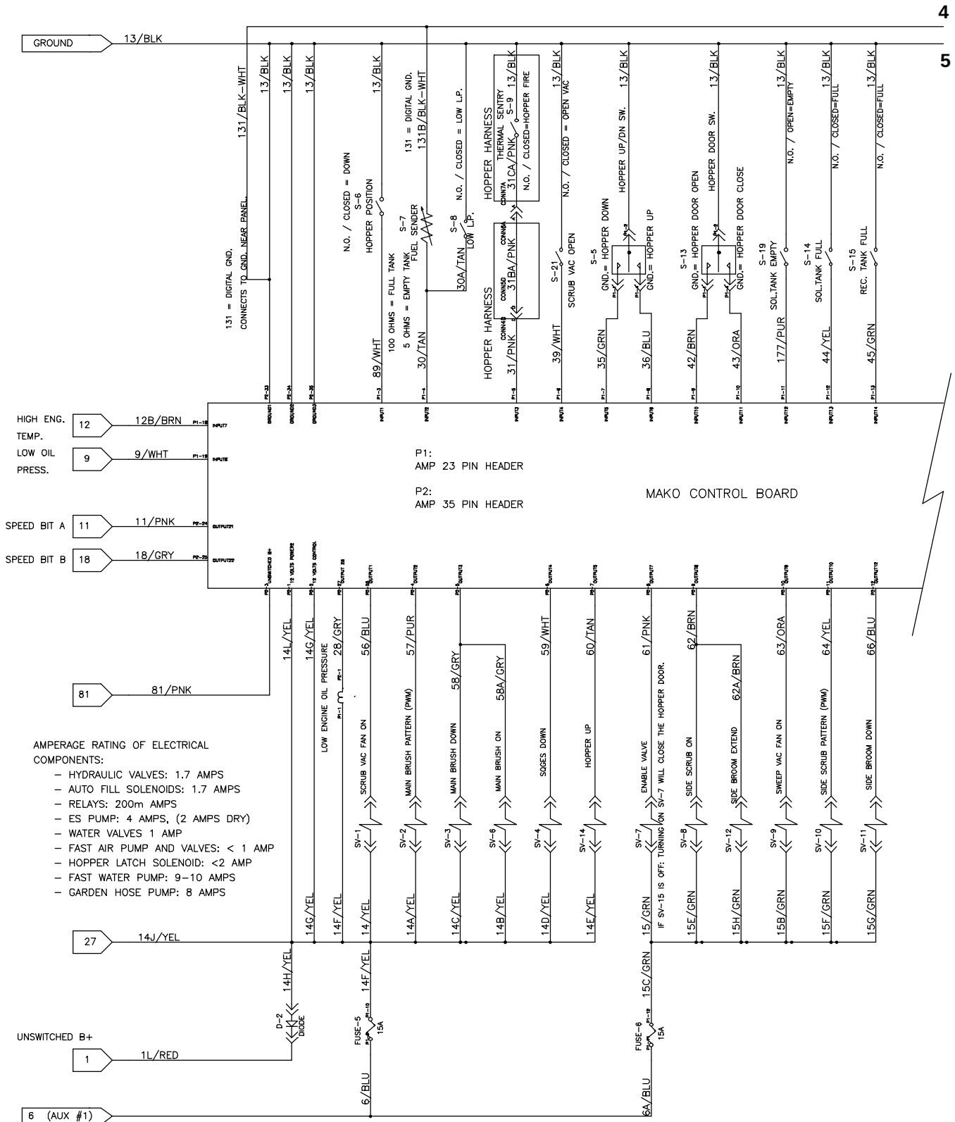
Fig. 75 – Electrical Schematic (002533–003478)
