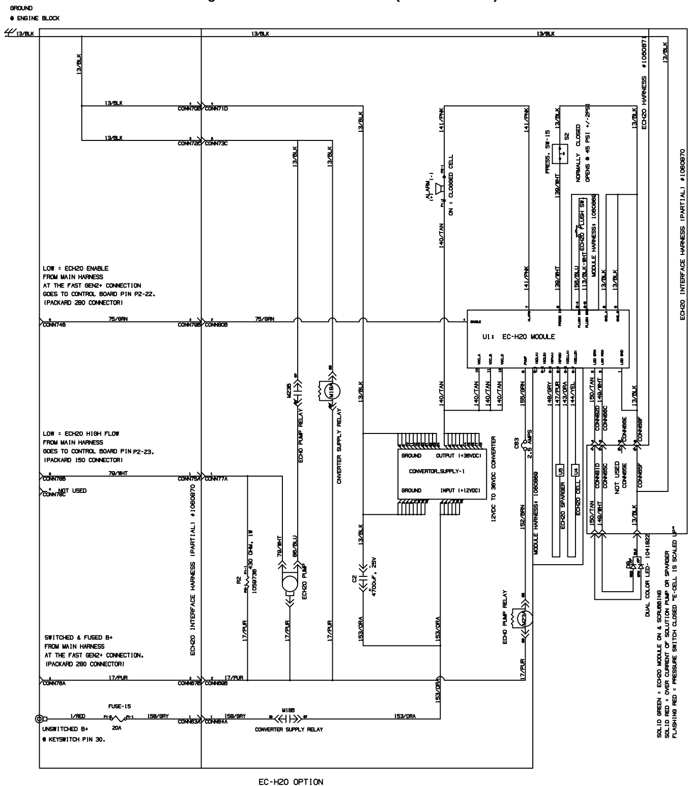
Fig. 76 – Electrical Schematic (003479– )
