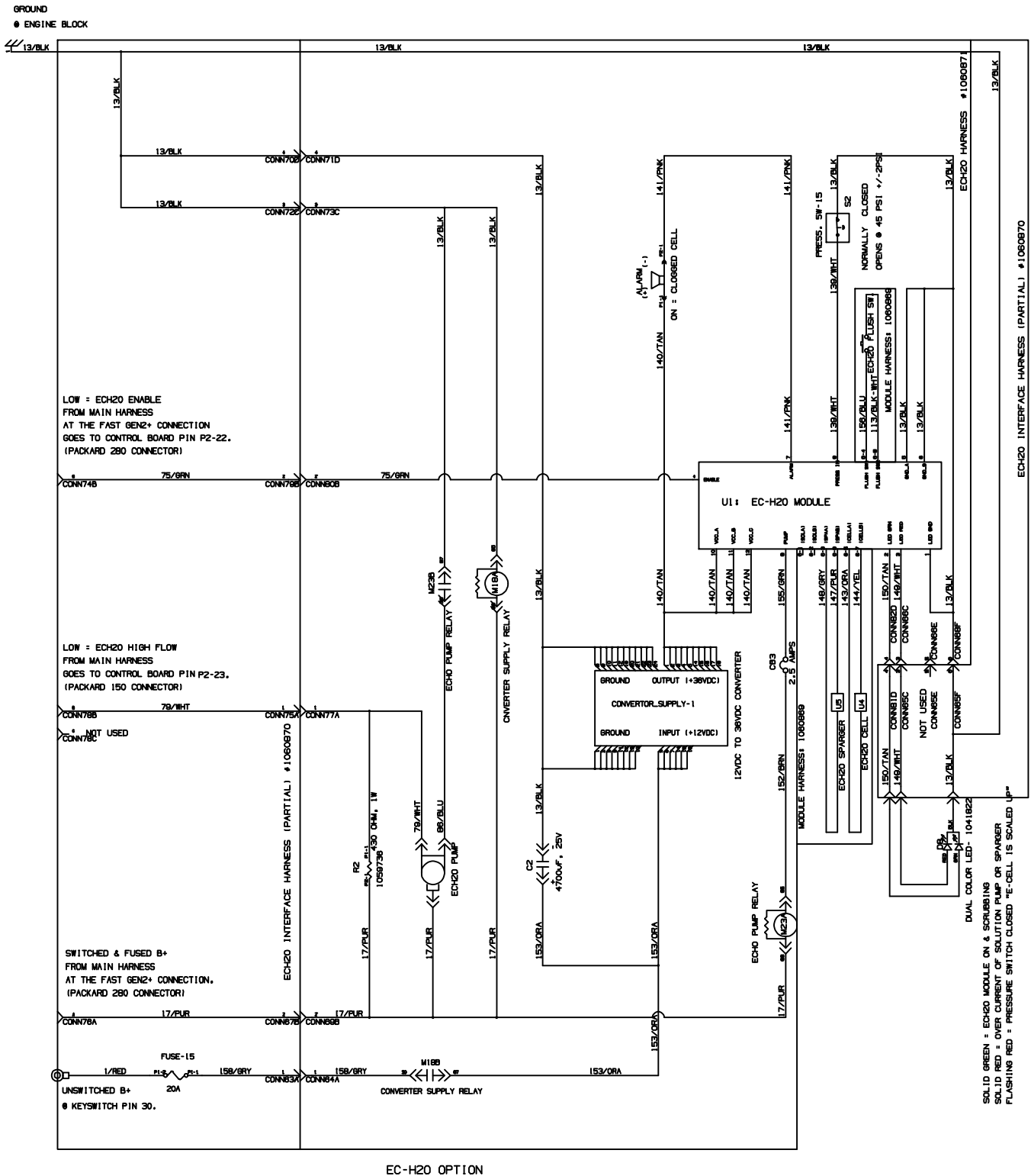
Fig. 75 – Electrical Schematic (002533–003478)
