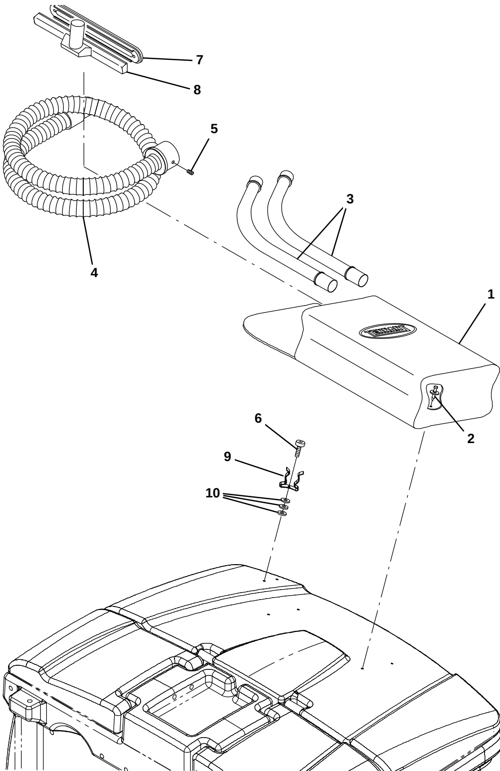
Fig. 30 – Vacuum Wand Kit (002407– )
