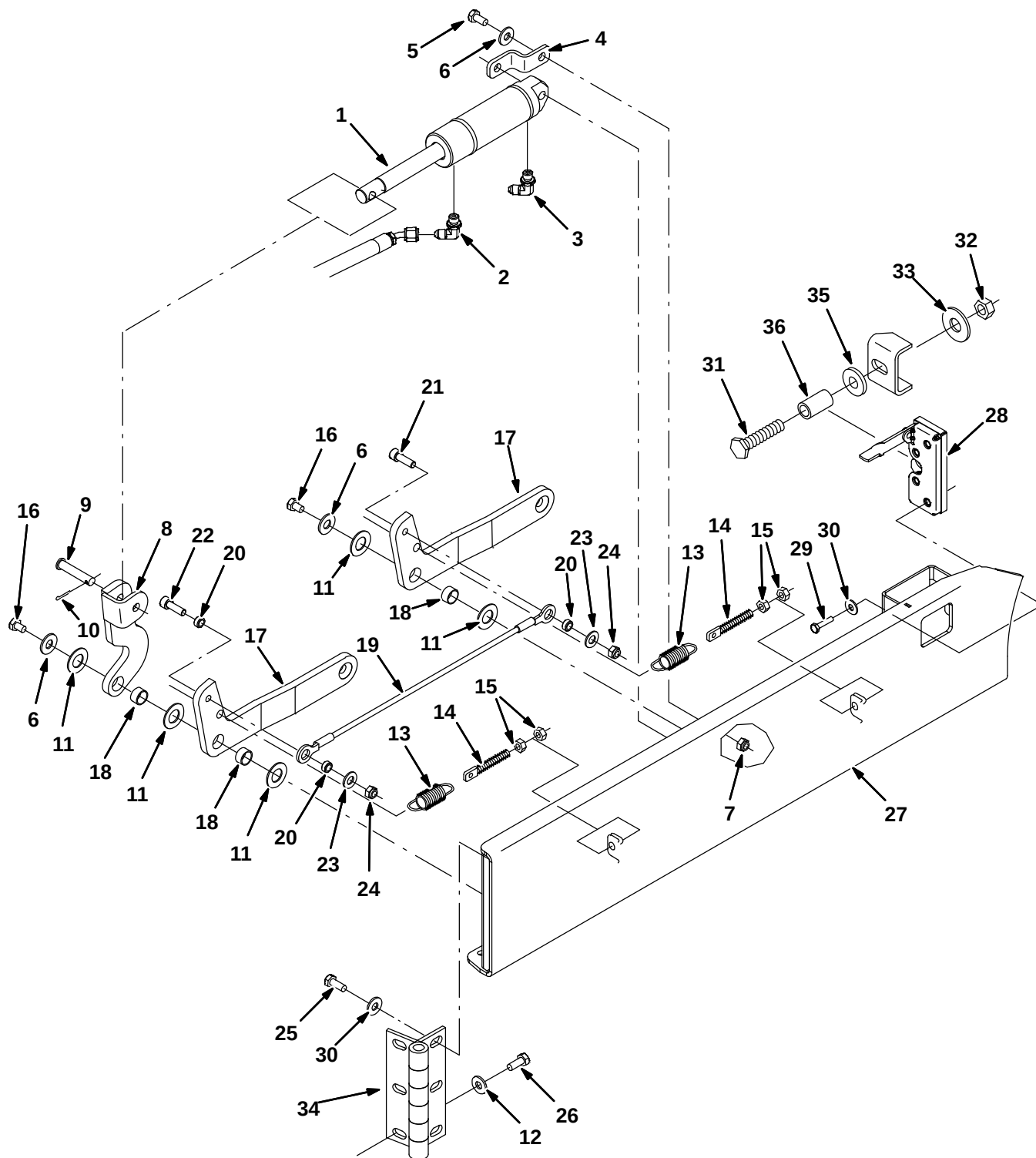
Fig. 53 – Squeegee Lift Group, Left Side
