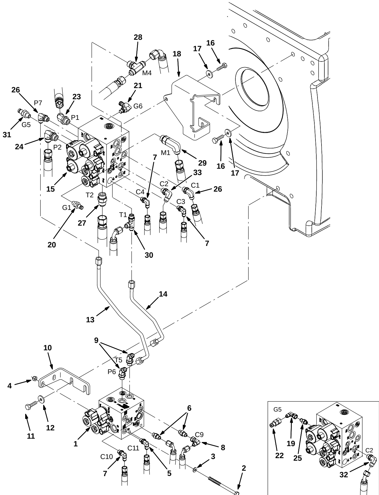
Fig. 71 – Hydraulic Valves Group (000000–002699)
