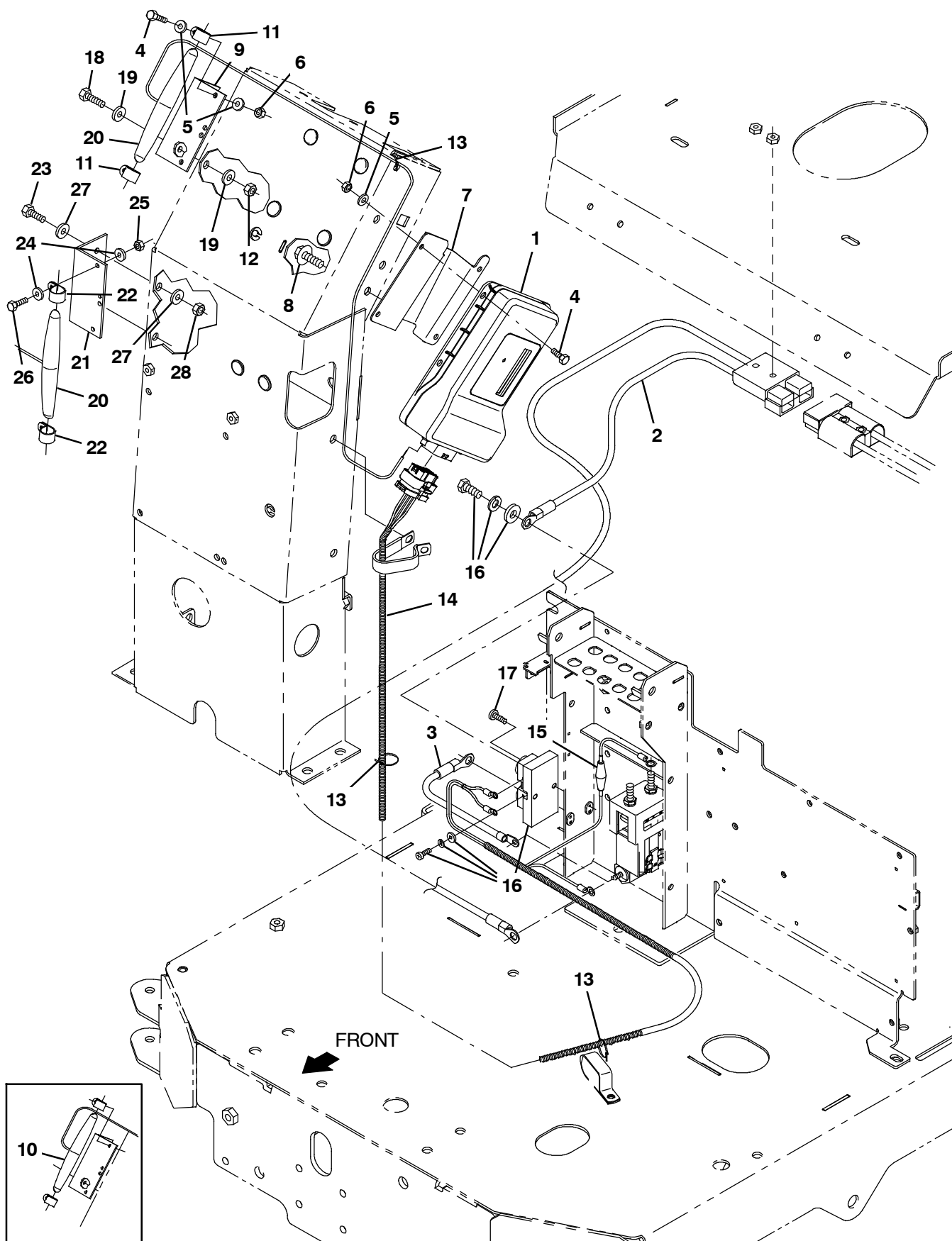
Fig. 51 - Rollout Battery Telemetry Group
