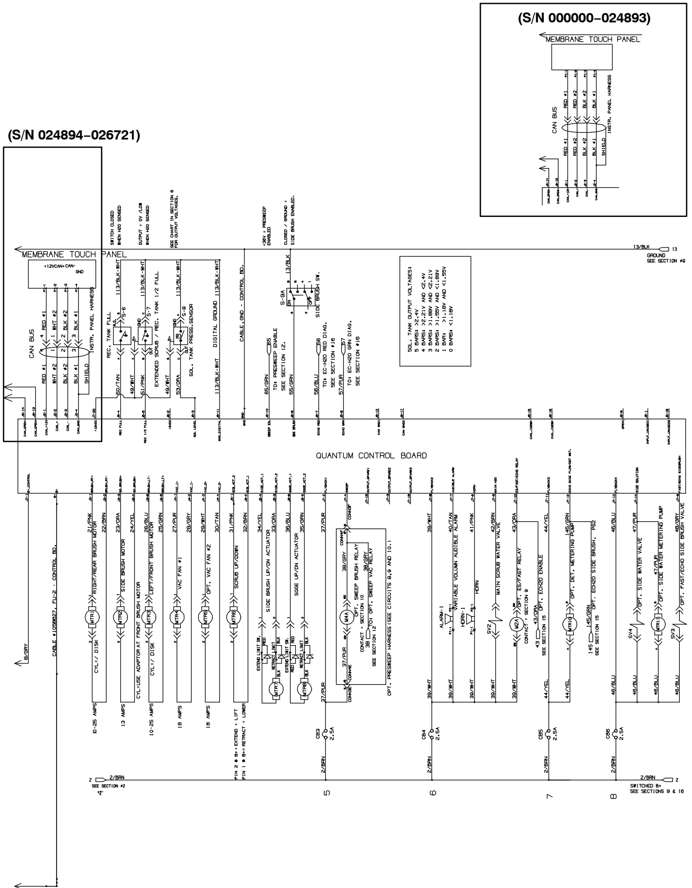
Fig. 22 – Electrical Schematic (2 of 5) (S/N 000000–026721)
