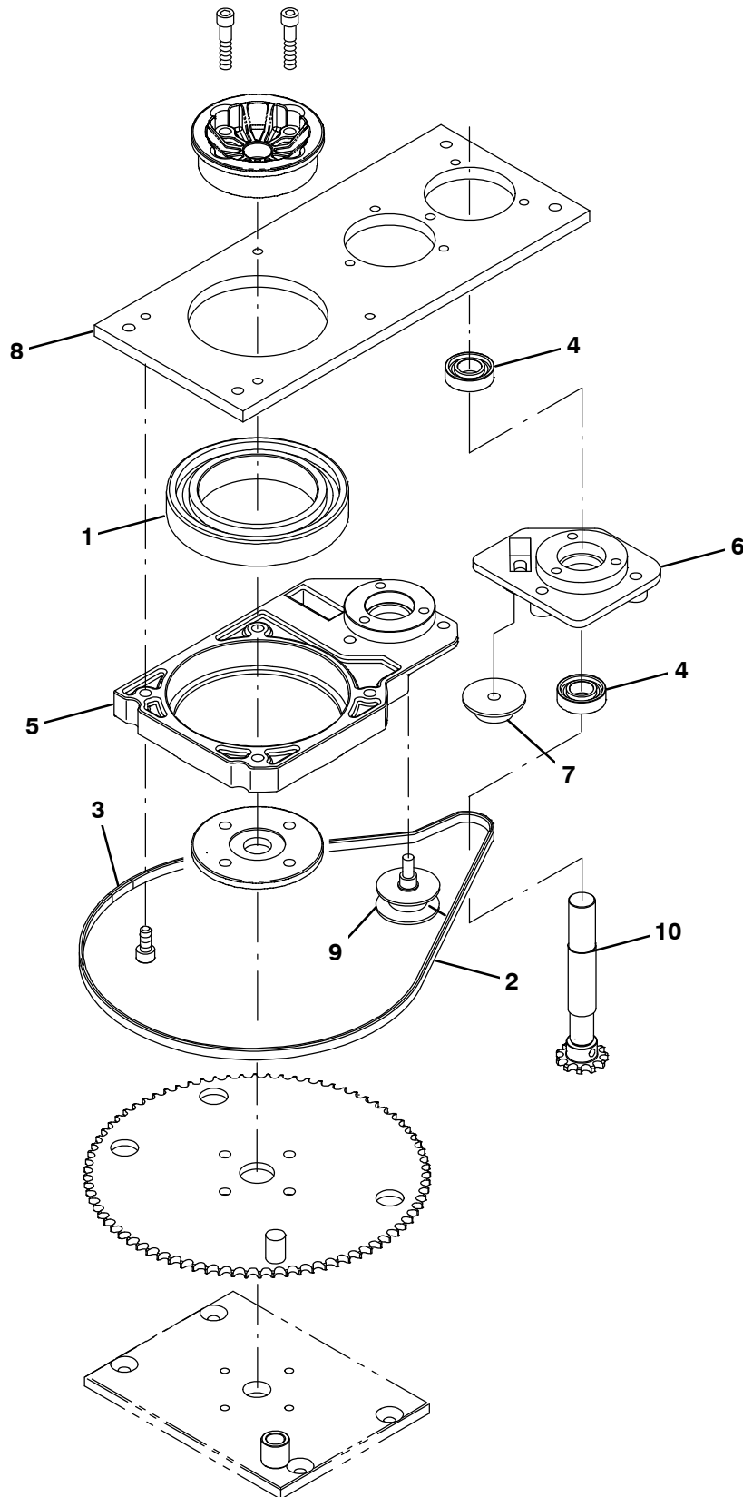
Fig. 1 – Steering Control Breakdown, 1053418 (000000–022671)
