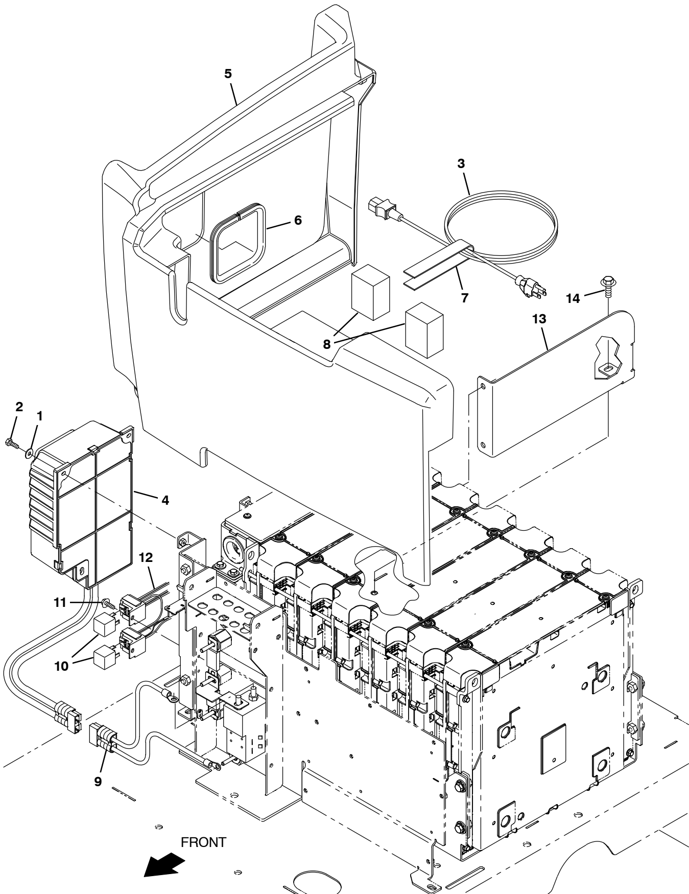
Fig. 47 – Lithium-Ion Onboard Battery Charger Group
