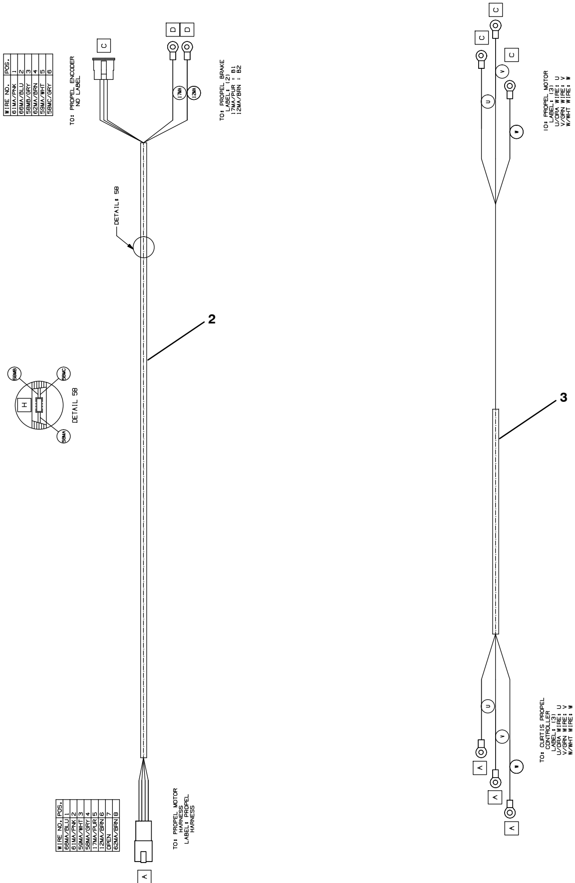
Fig. 24 – Wire Harnesses Group (S/N 000000–026721)
