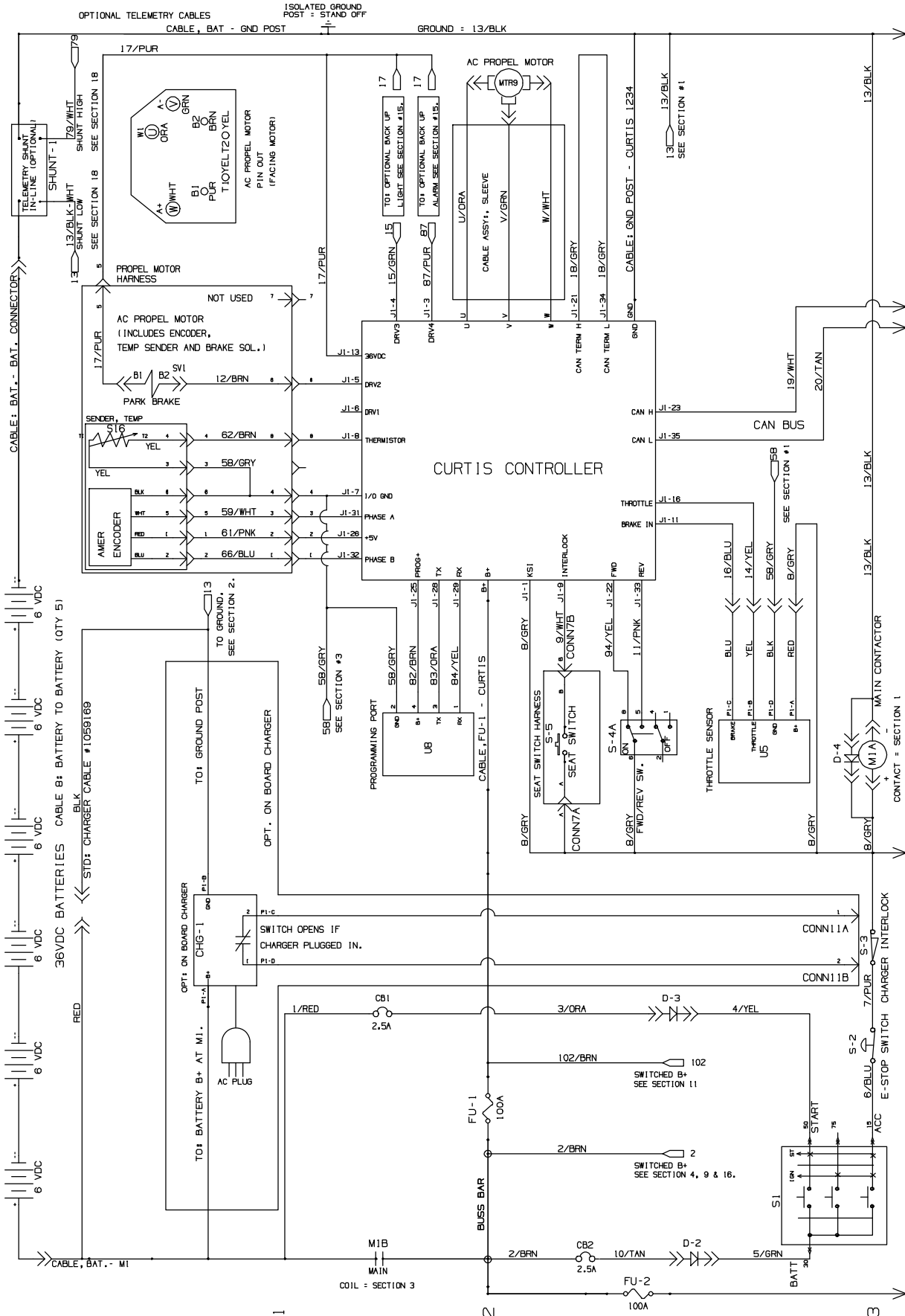
Fig. 22 – Electrical Schematic (1 of 5) (S/N 000000–026721)
