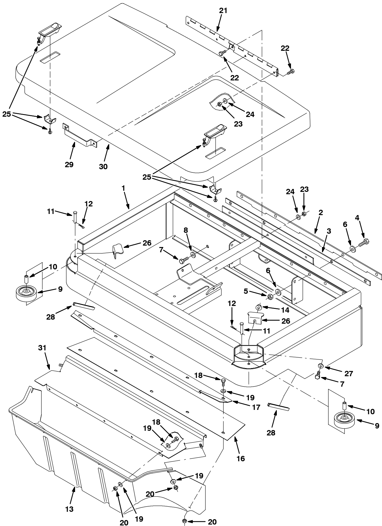
Fig. 33 - Pre-Sweep Frame and Hopper Group
