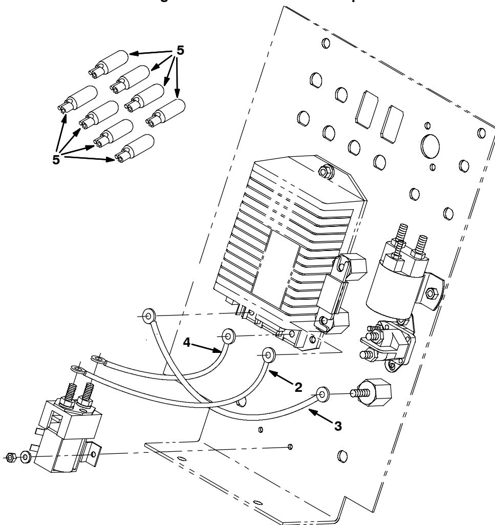
Fig. 32 - Wire Harnesses Group
