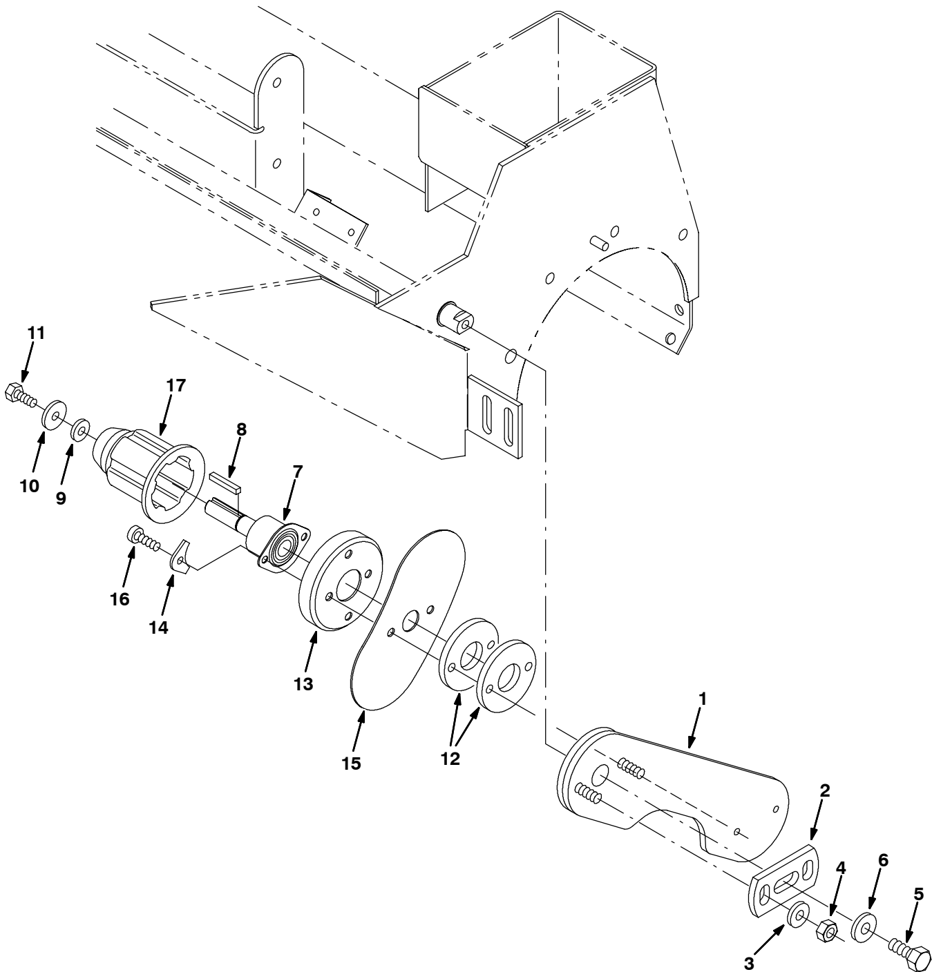
Fig. 37 - Pre-Sweep Brush Idler Group
