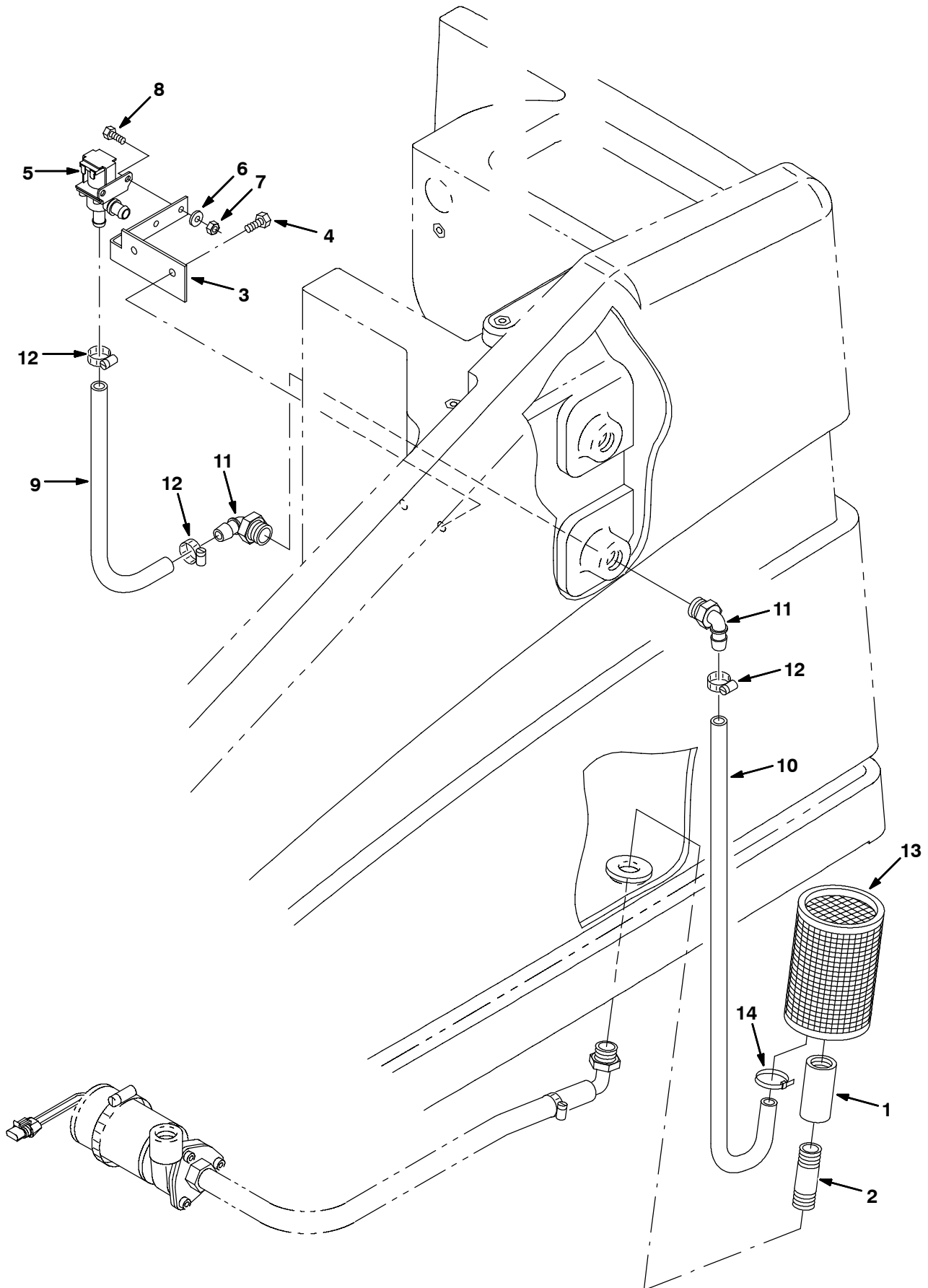
Fig. 10 - ES Filter Backflush Kit
