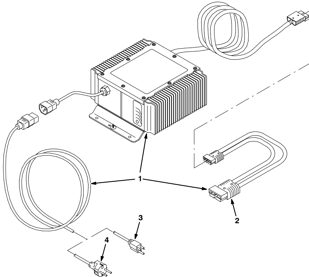
Fig. 25 - Battery Charger Group, International Only
