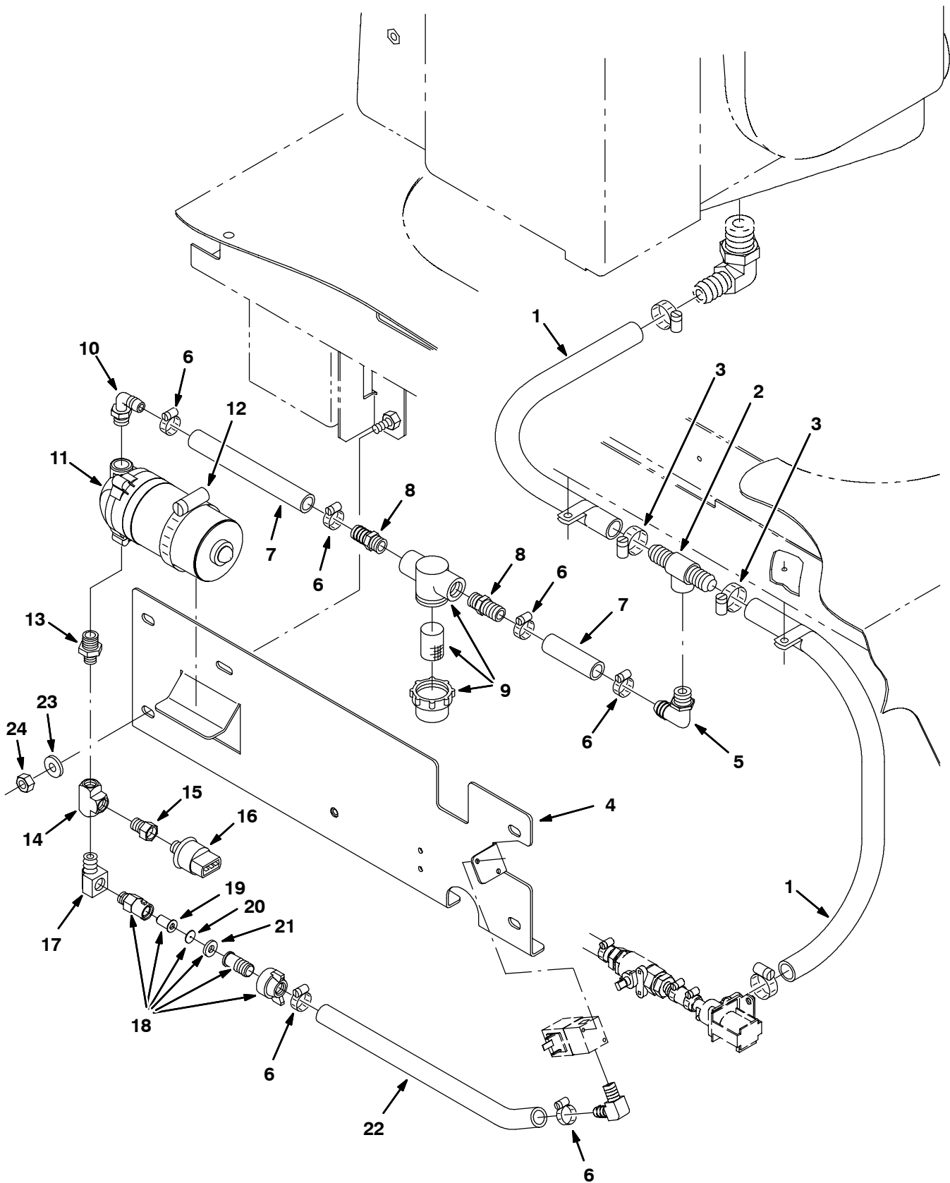
Fig. 21 - FaST Solution Pump Group
