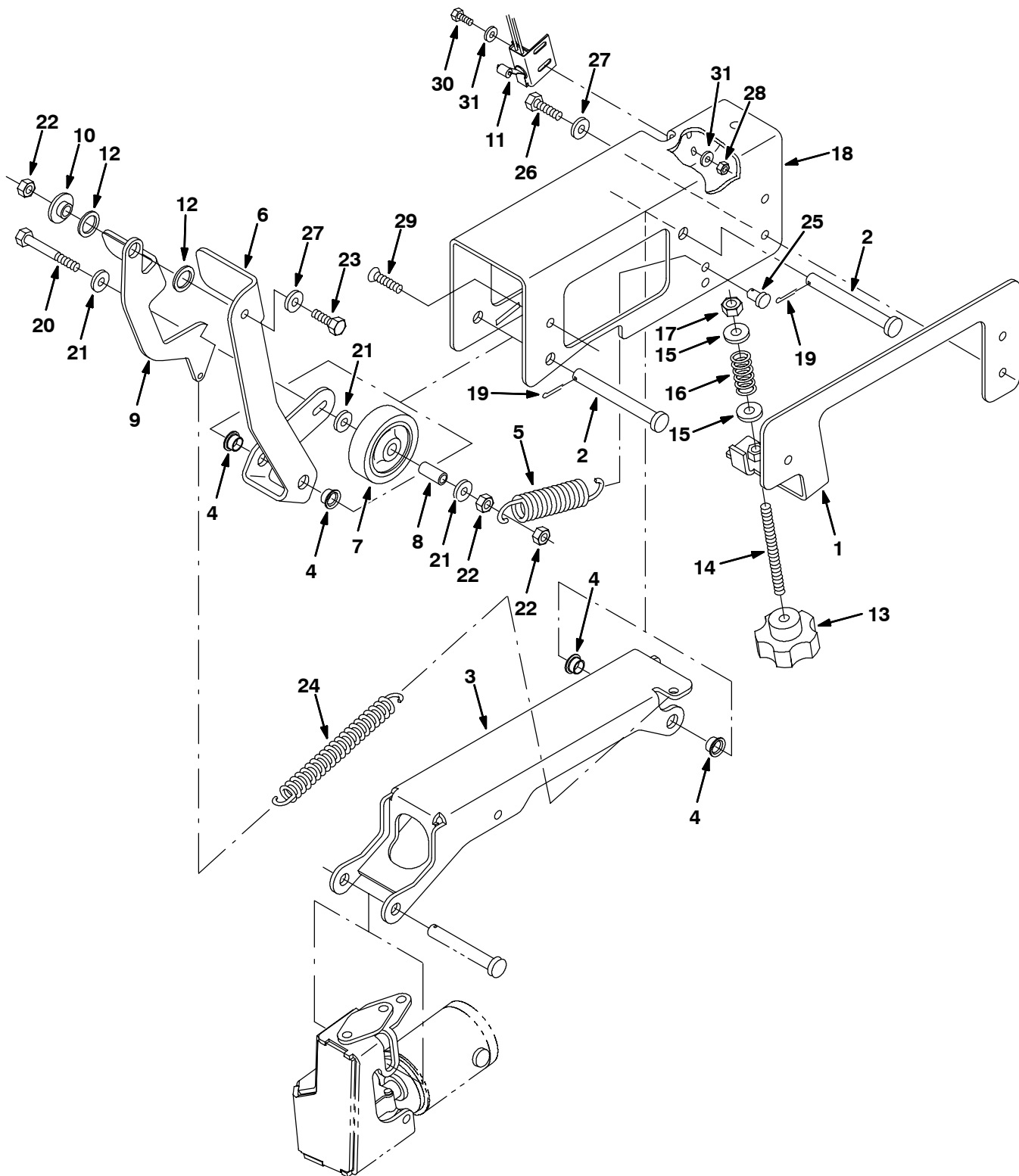
Fig. 45 - Side Brush Lift Group
