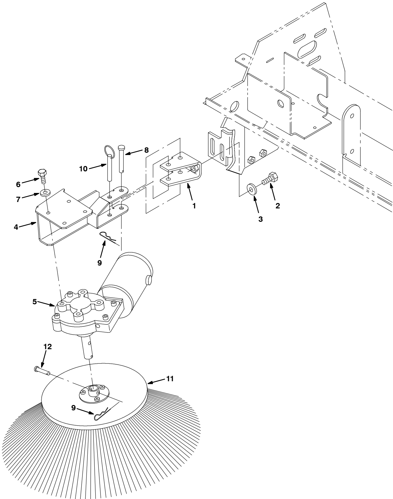
Fig. 38 - Pre-Sweep Side Brush Group
