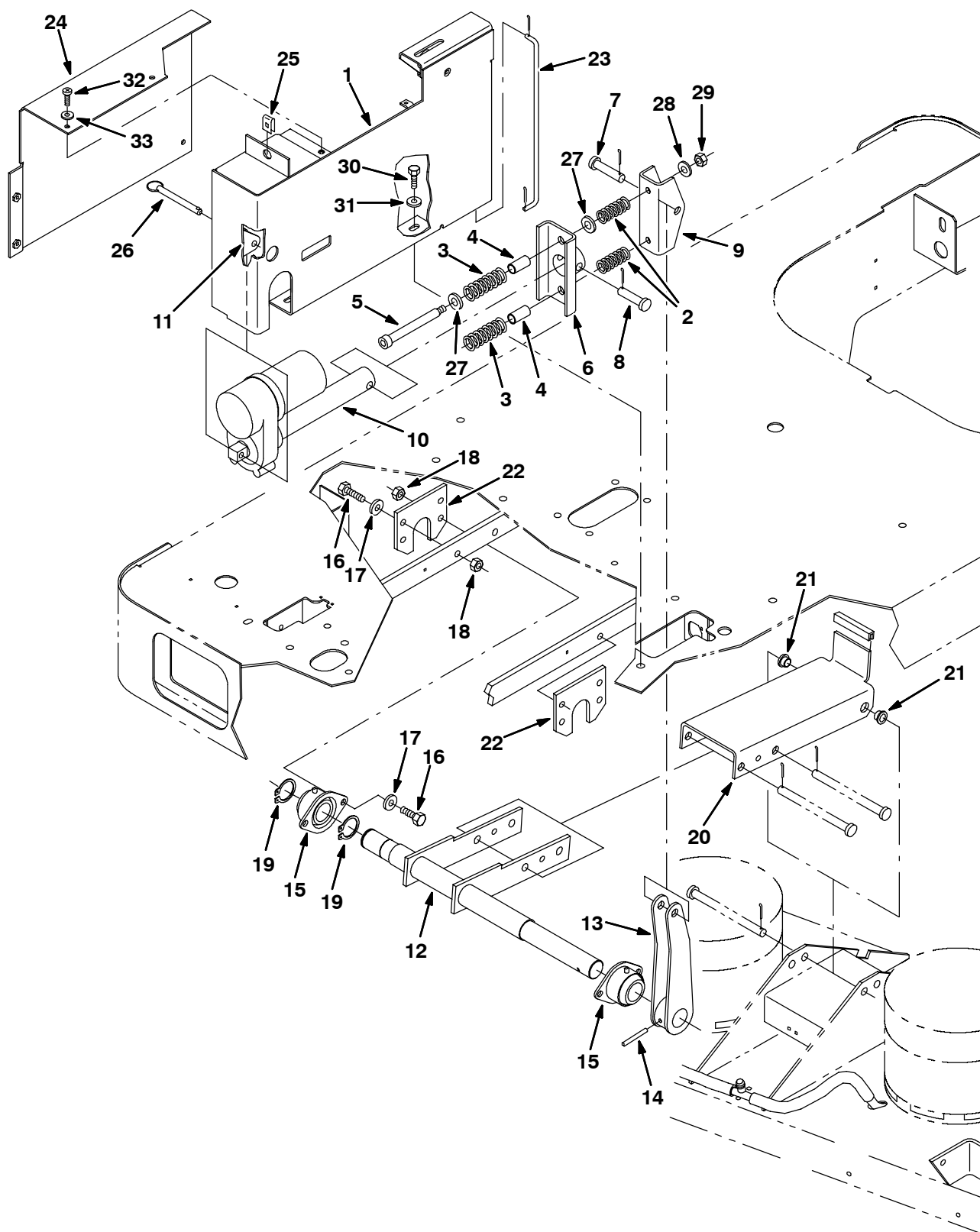
Fig. 26 - Rollout Battery Scrub Head Lift Group
