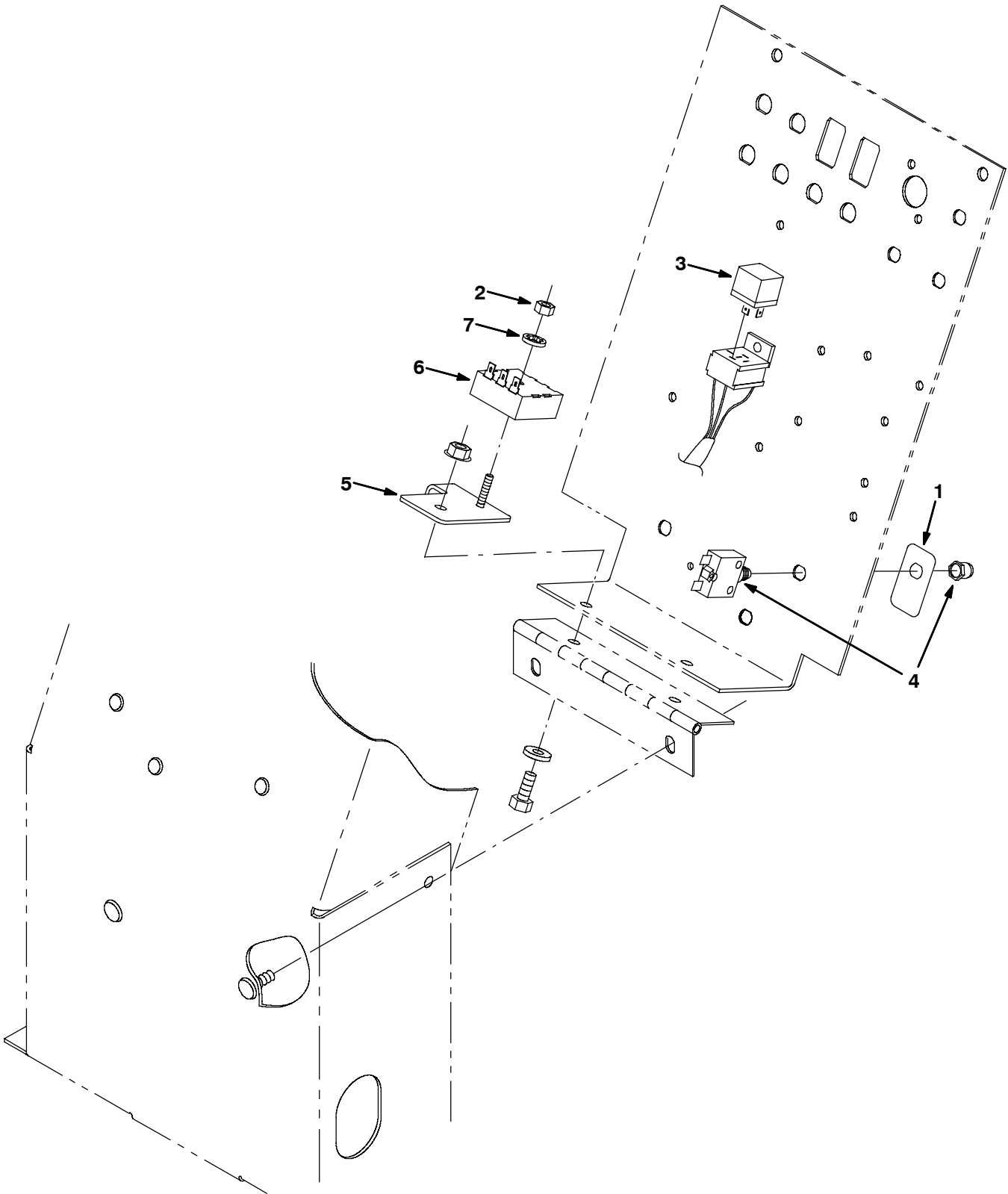
Fig. 24 - FaST Electrical Panel Group
