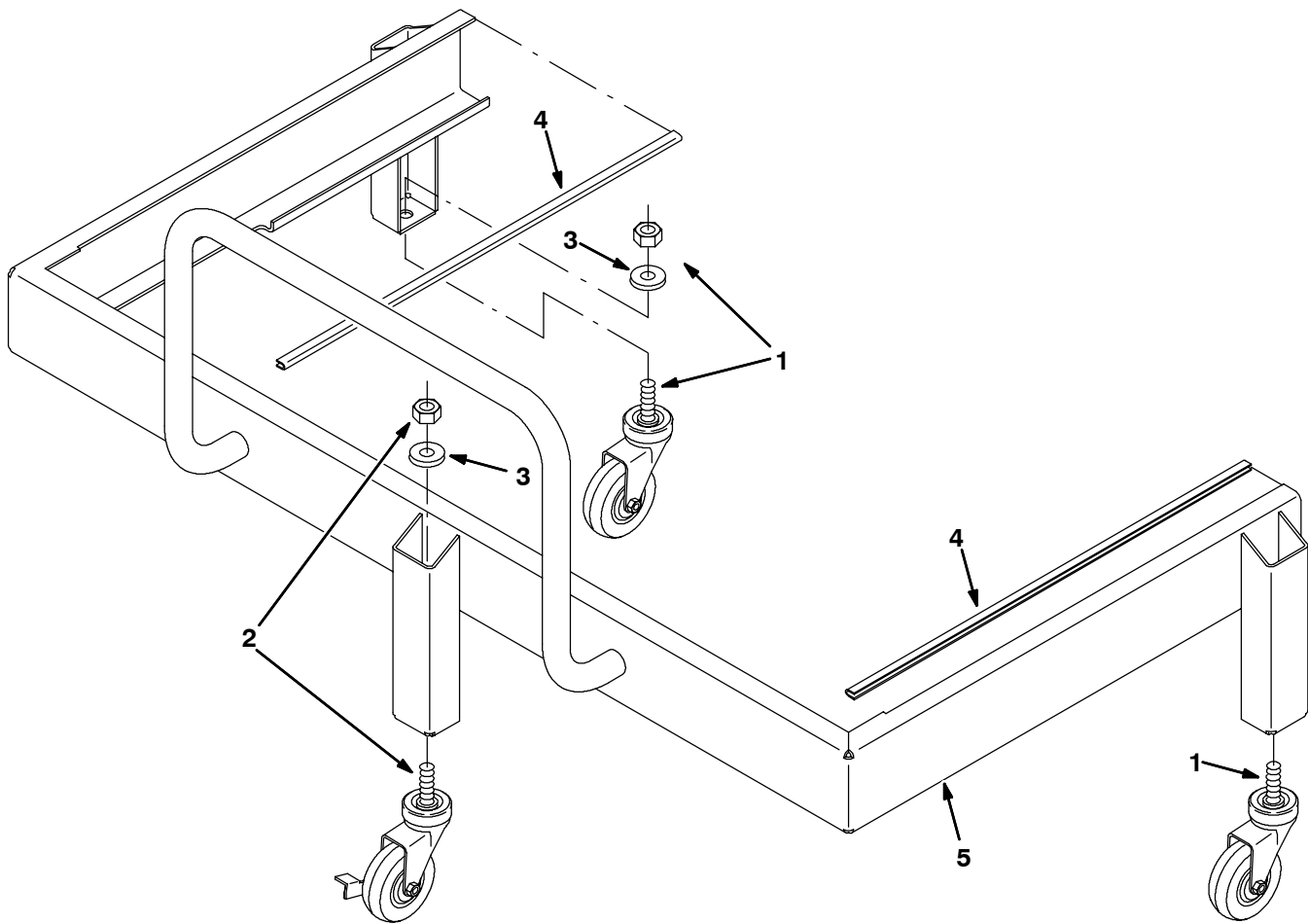
Fig. 44 - Pre-Sweep Dolly Kit
