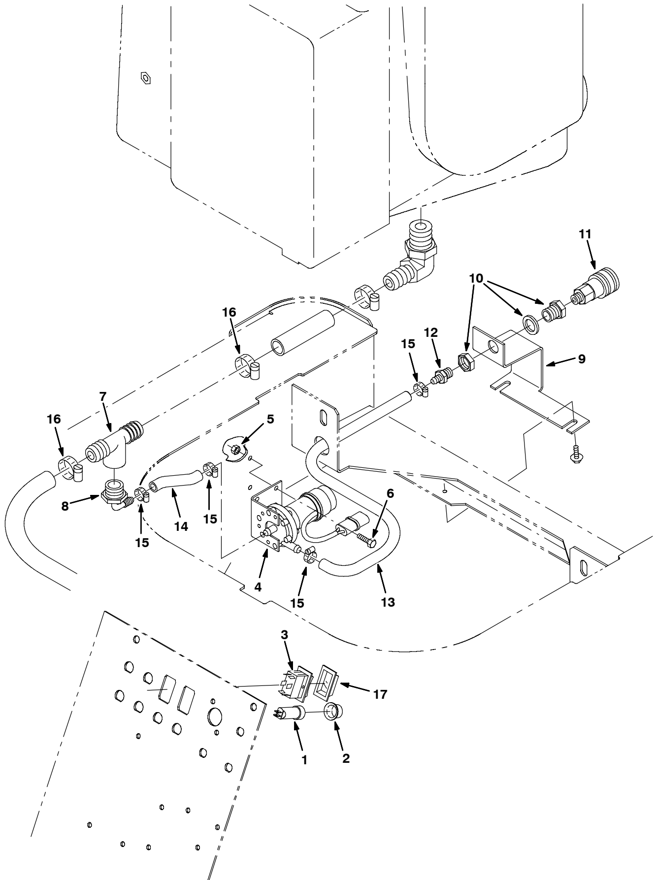
Fig. 13 - Power Wand Pump and Fittings Group
