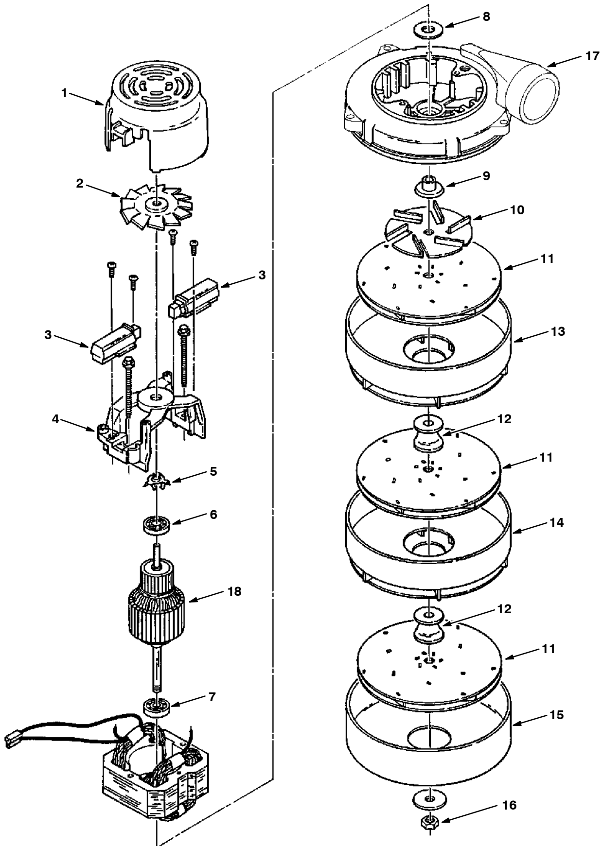
Fig. 5 - Electric Motor Breakdown, 398520
