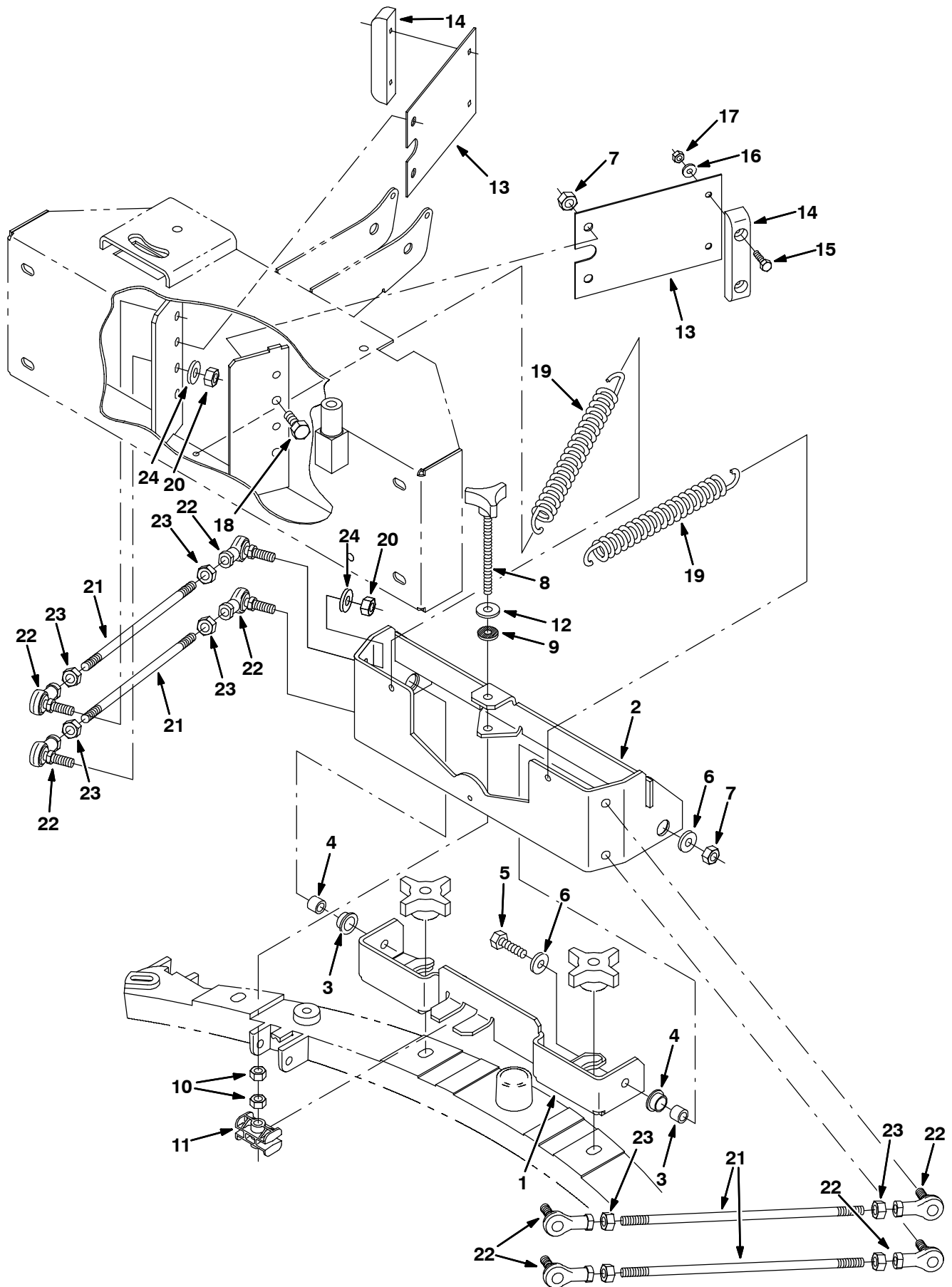
Fig. 29 - Rear Squeegee Linkage Group
