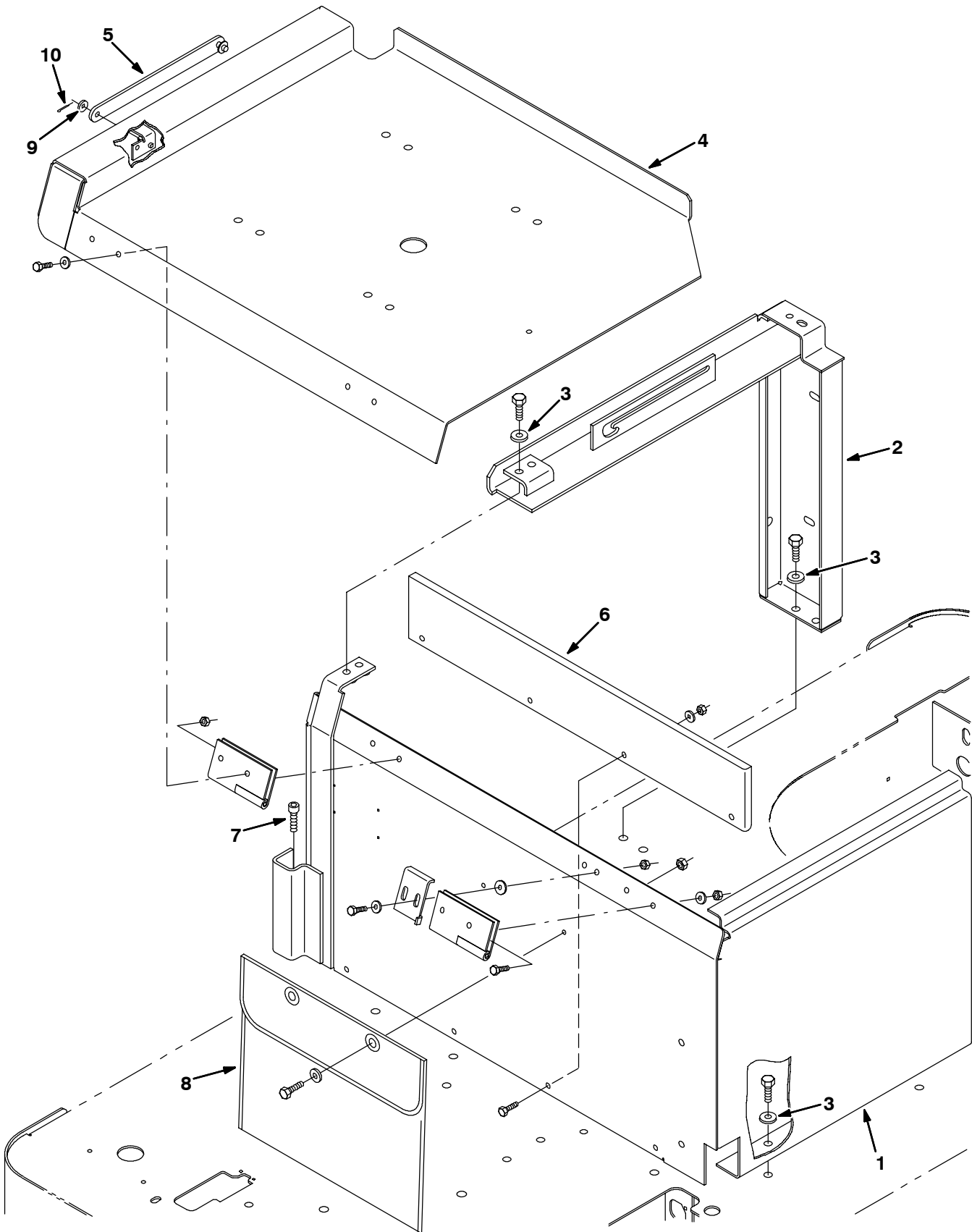
Fig. 27 - Rollout Battery Seat Support Group
