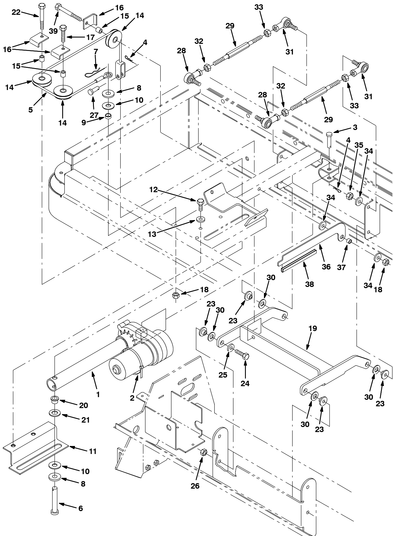
Fig. 34 - Pre-Sweep Brush Lift Group
