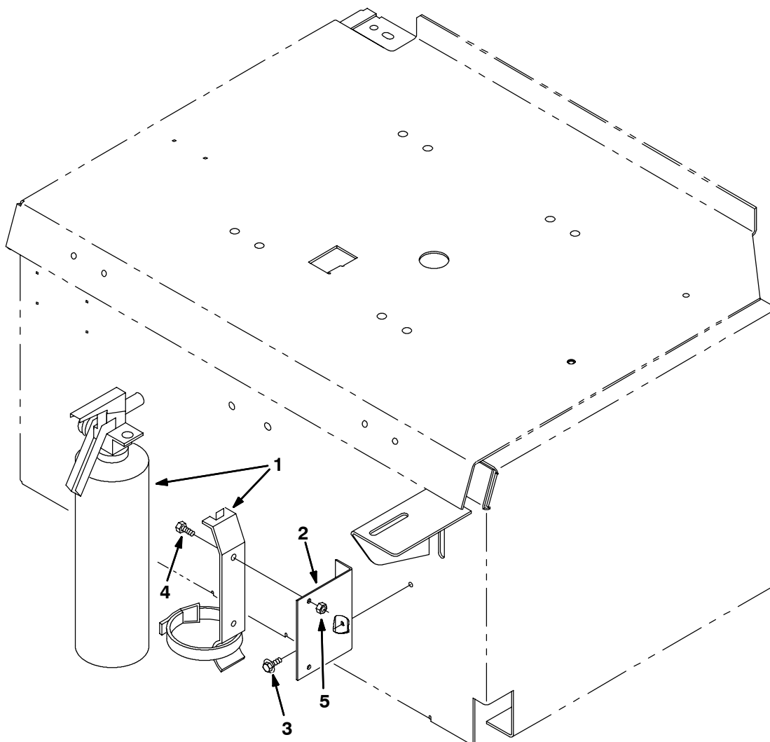
Fig. 52 - Fire Extinguisher Kit
