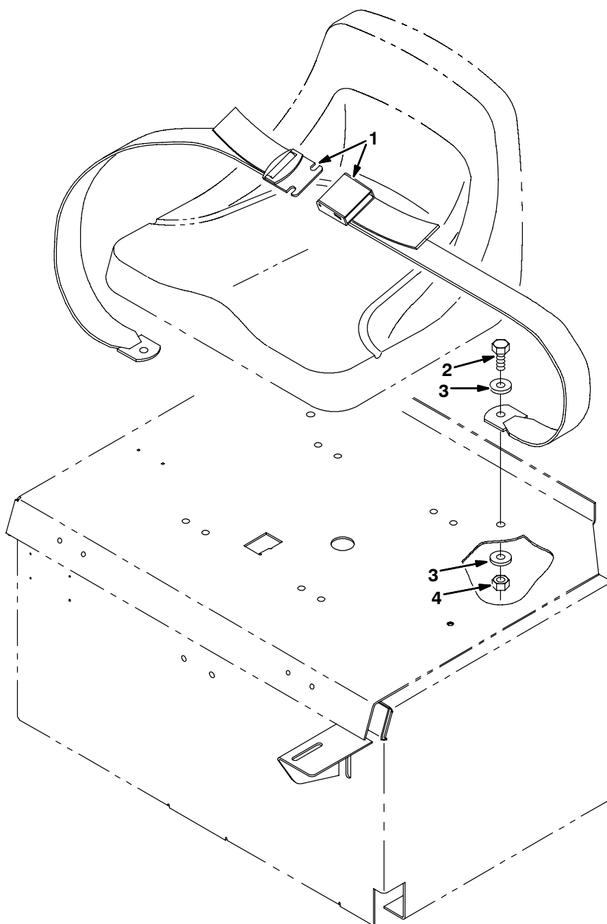
Fig. 50 - Seat Belt Kit
