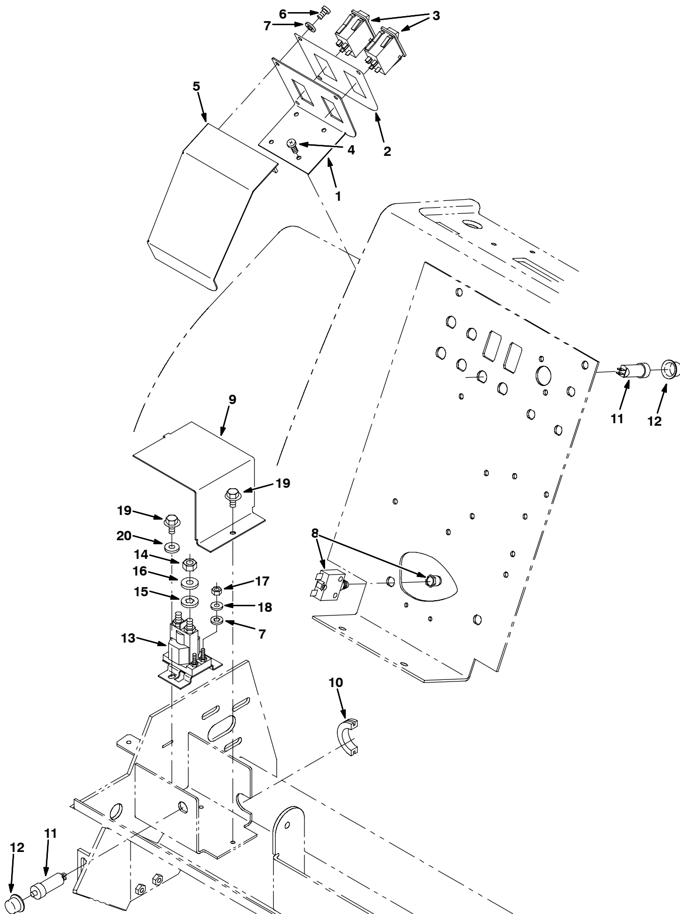
Fig. 40 - Pre-Sweep Electrical Group
