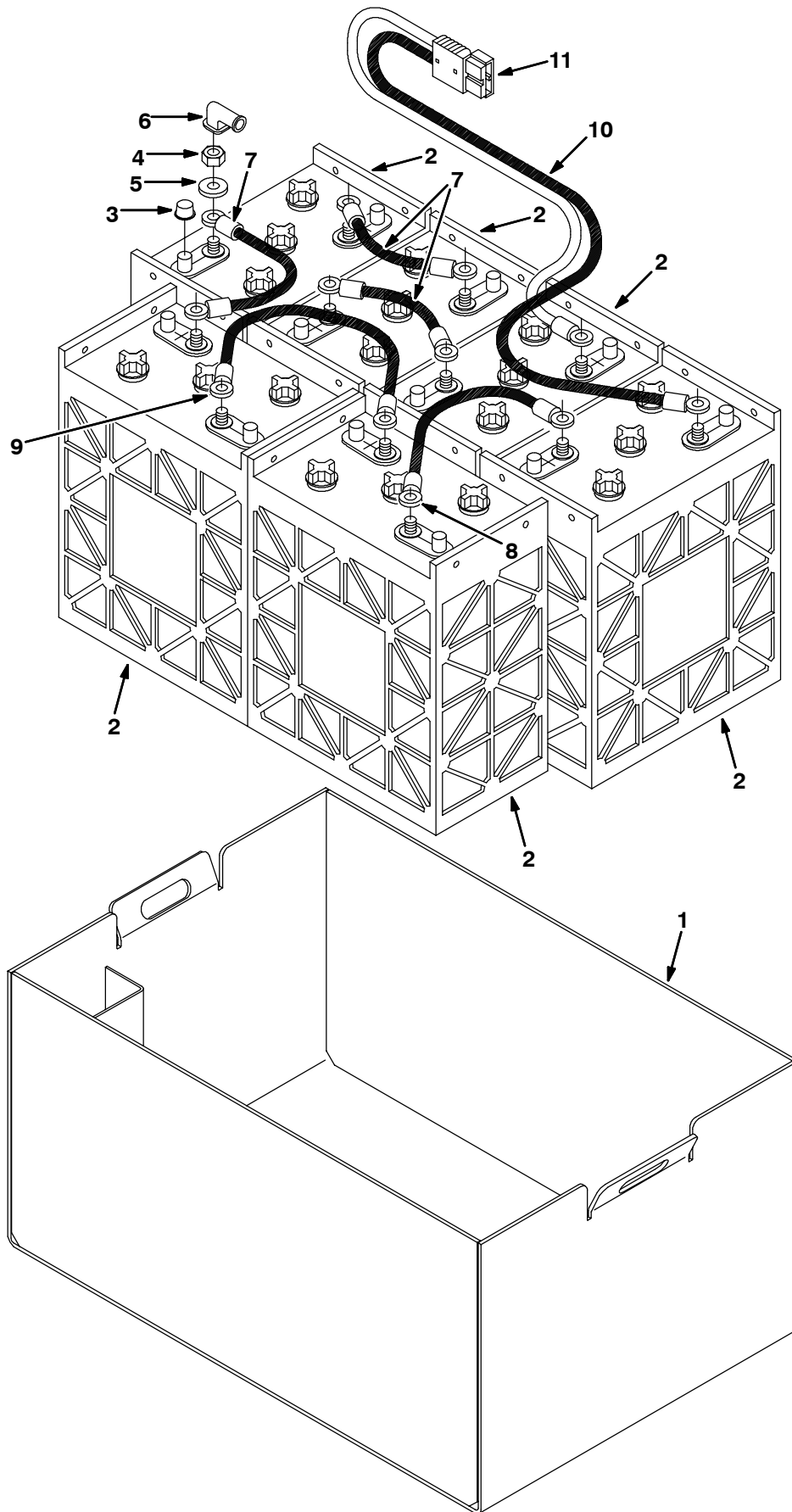
Fig. 32 - Rollout Battery Pack Kit
