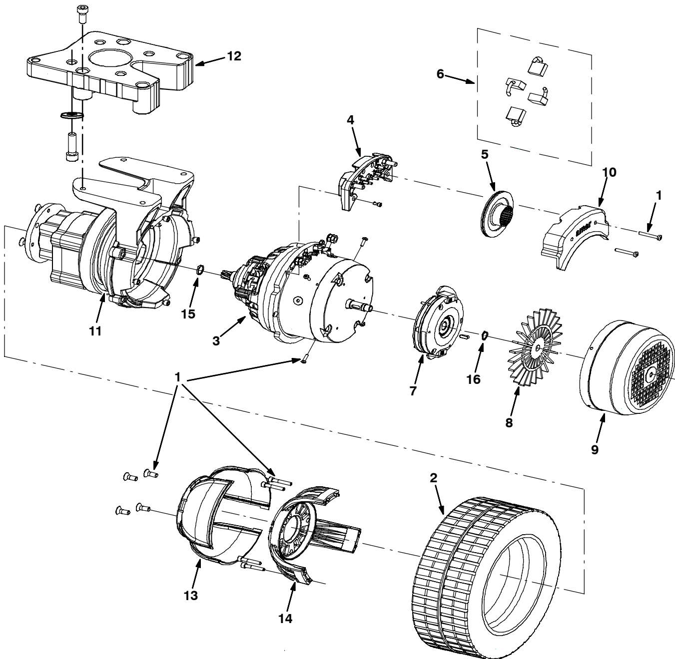
Fig. 6 - Drive Wheel Breakdown, 1033016
