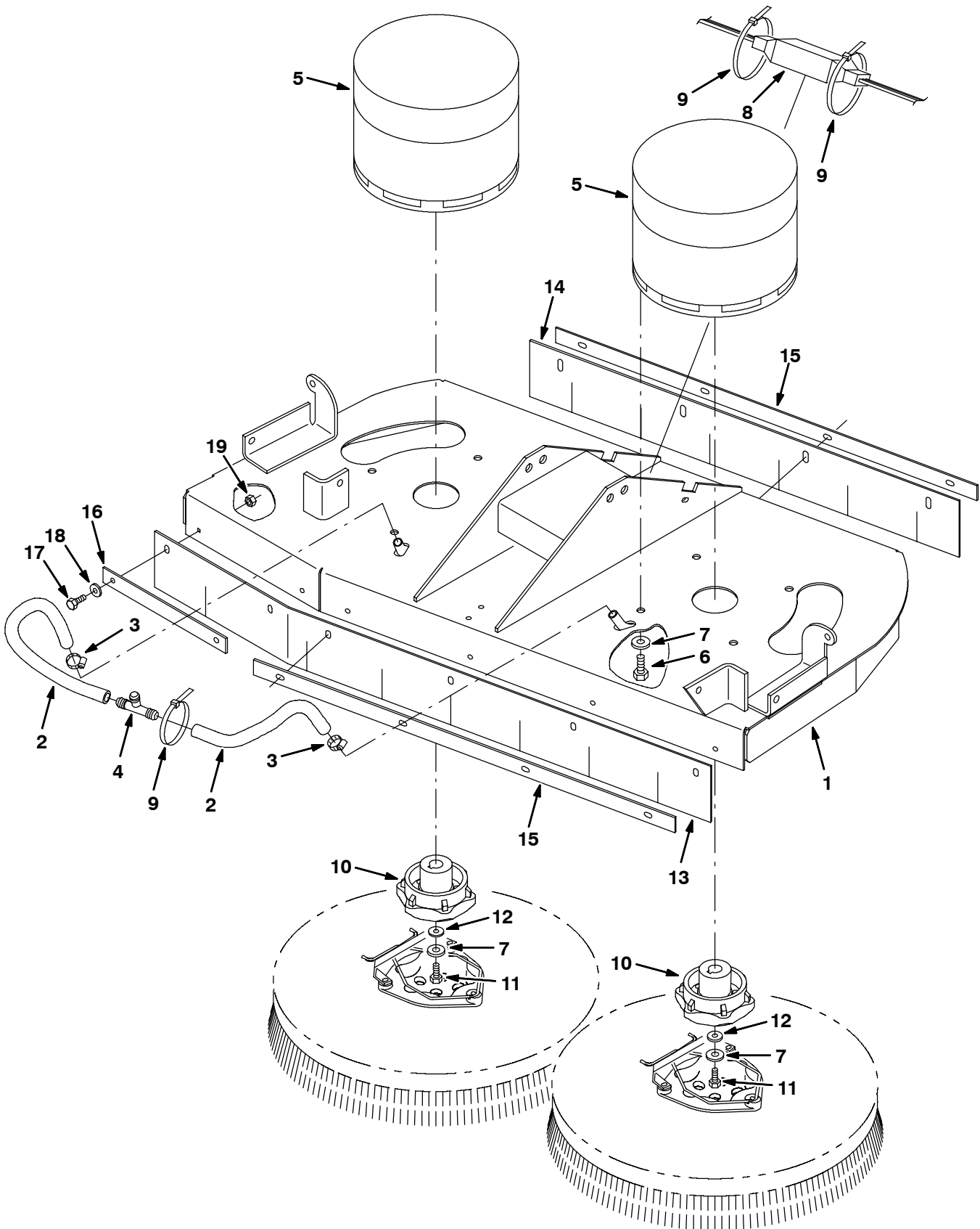
Fig. 11 - Disk Scrub Head Drive Motor Group, 900 mm (36 in)
