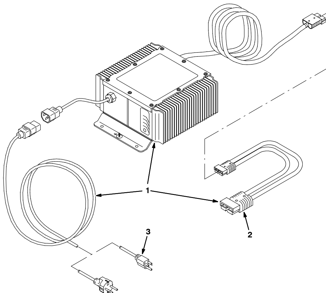
Fig. 24 - Battery Charger Group
