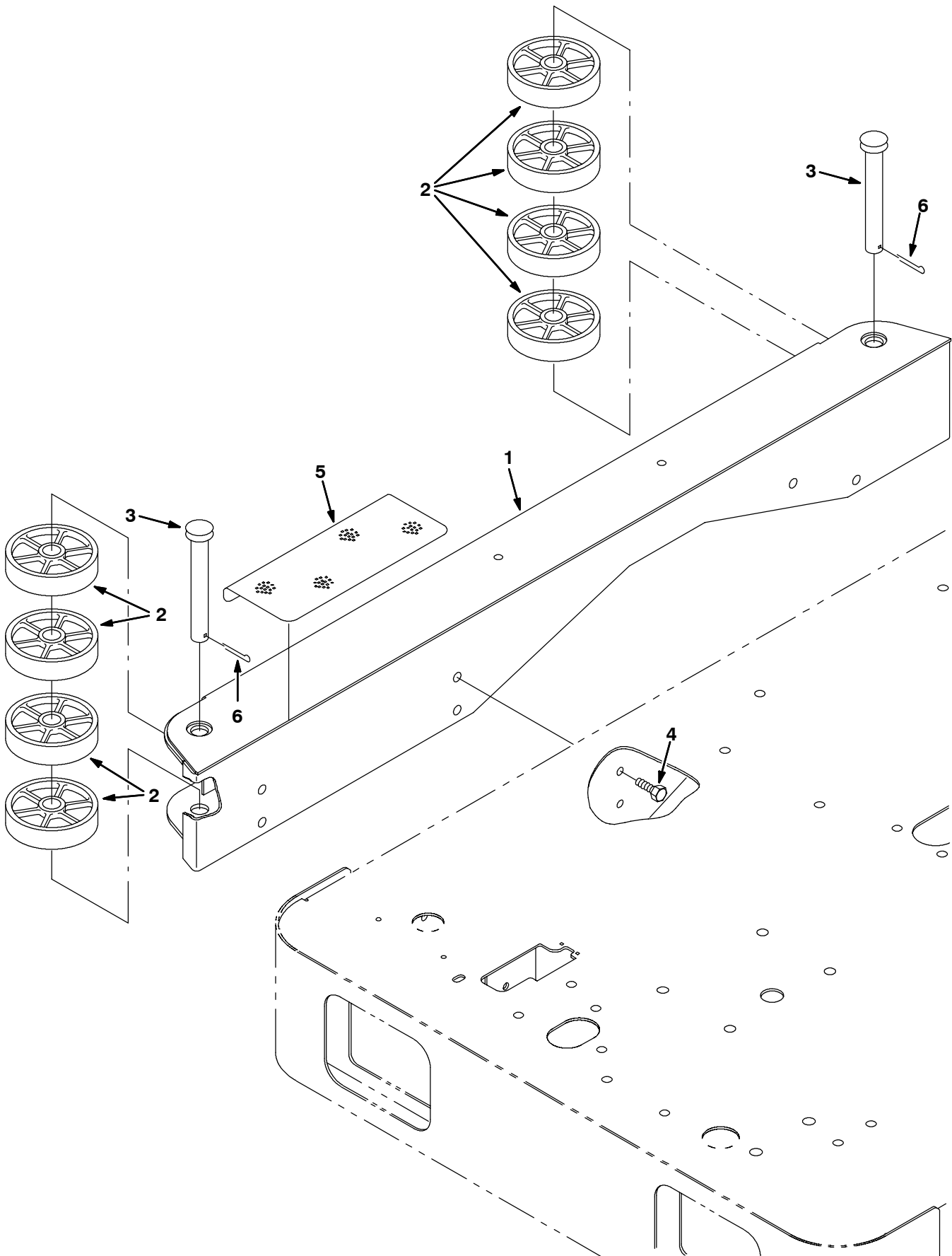
Fig. 19 - Side Roller Bumper Kit
