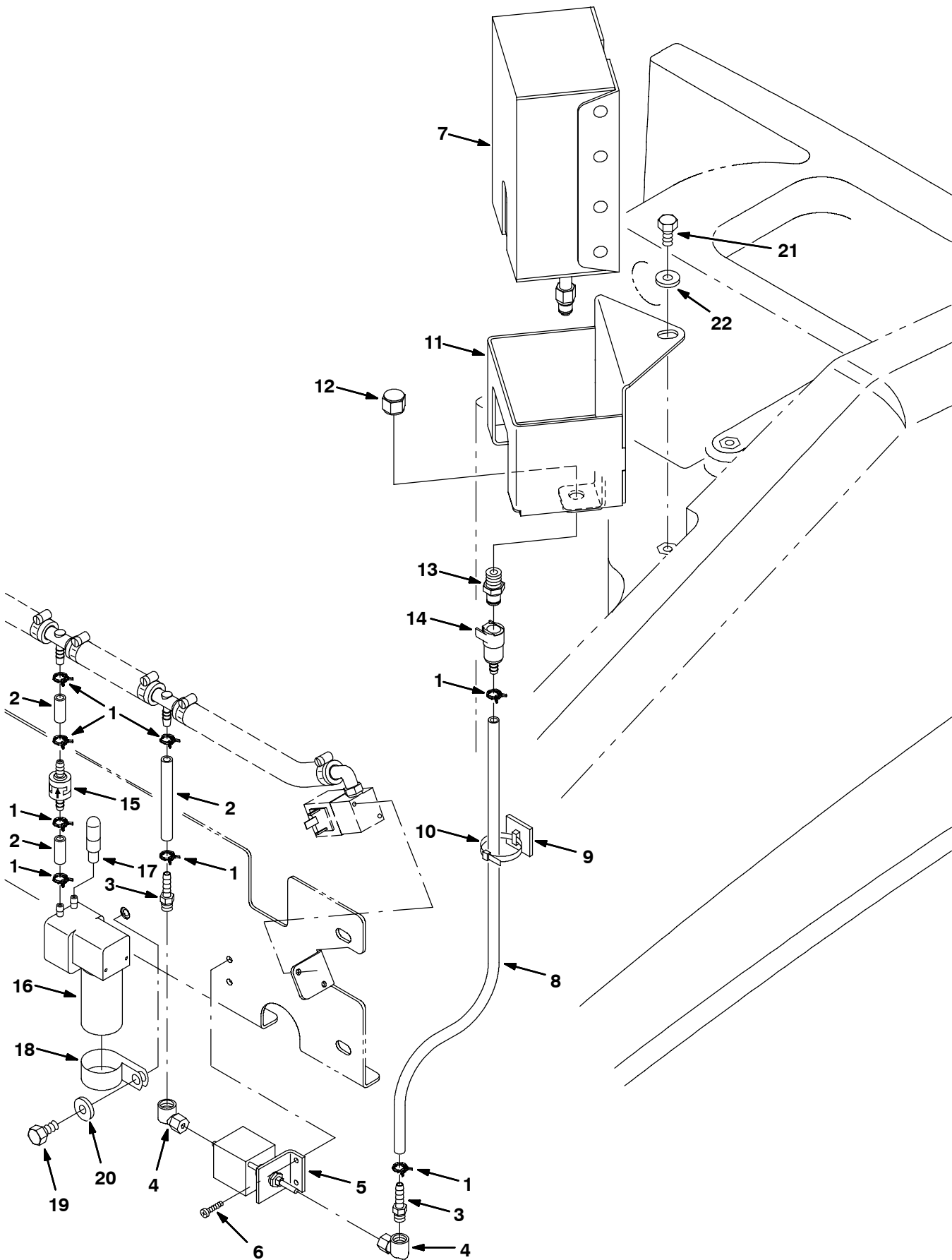
Fig. 20 - FaST Air Pump and Detergent Group
