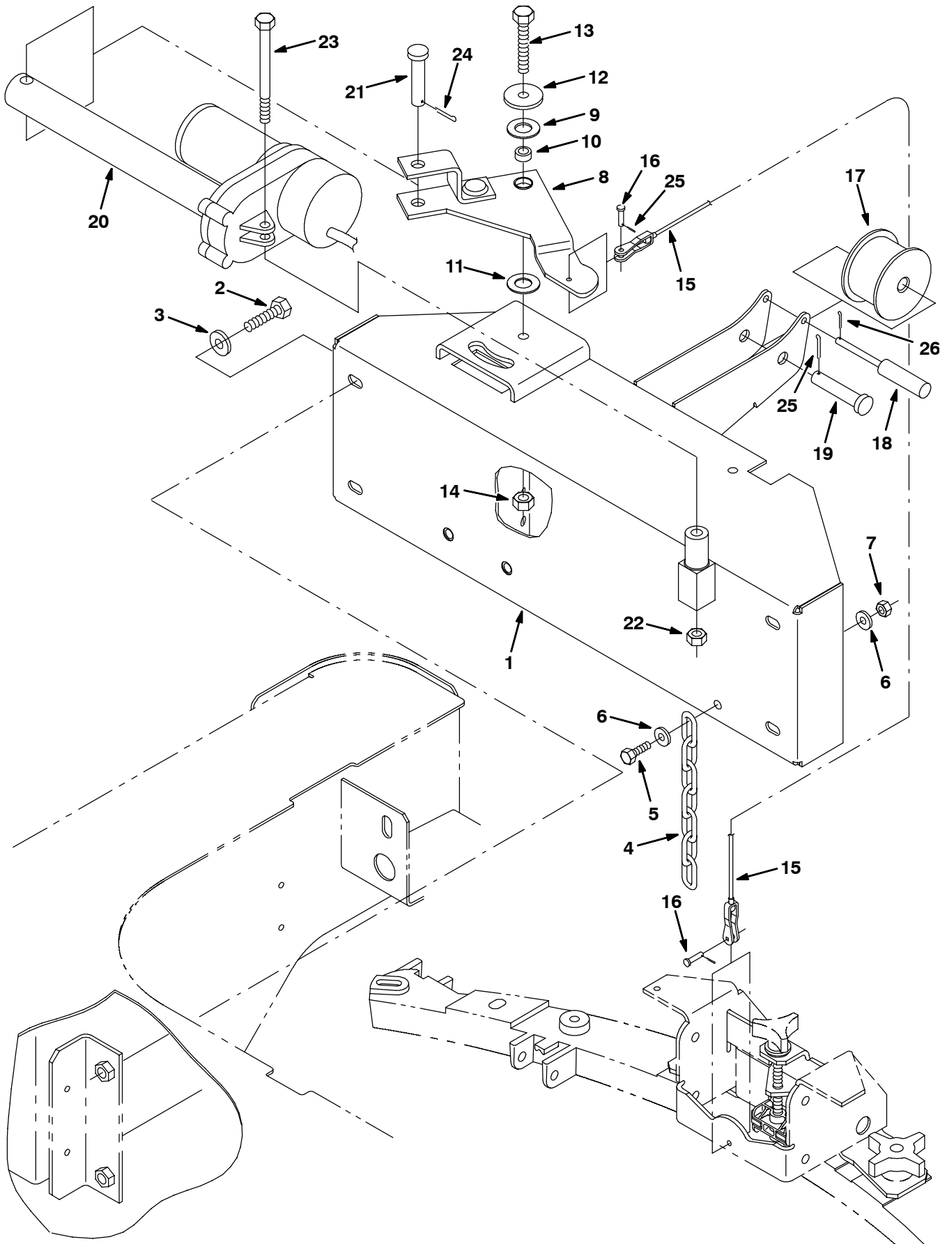
Fig. 28 - Rear Squeegee Lift Group
