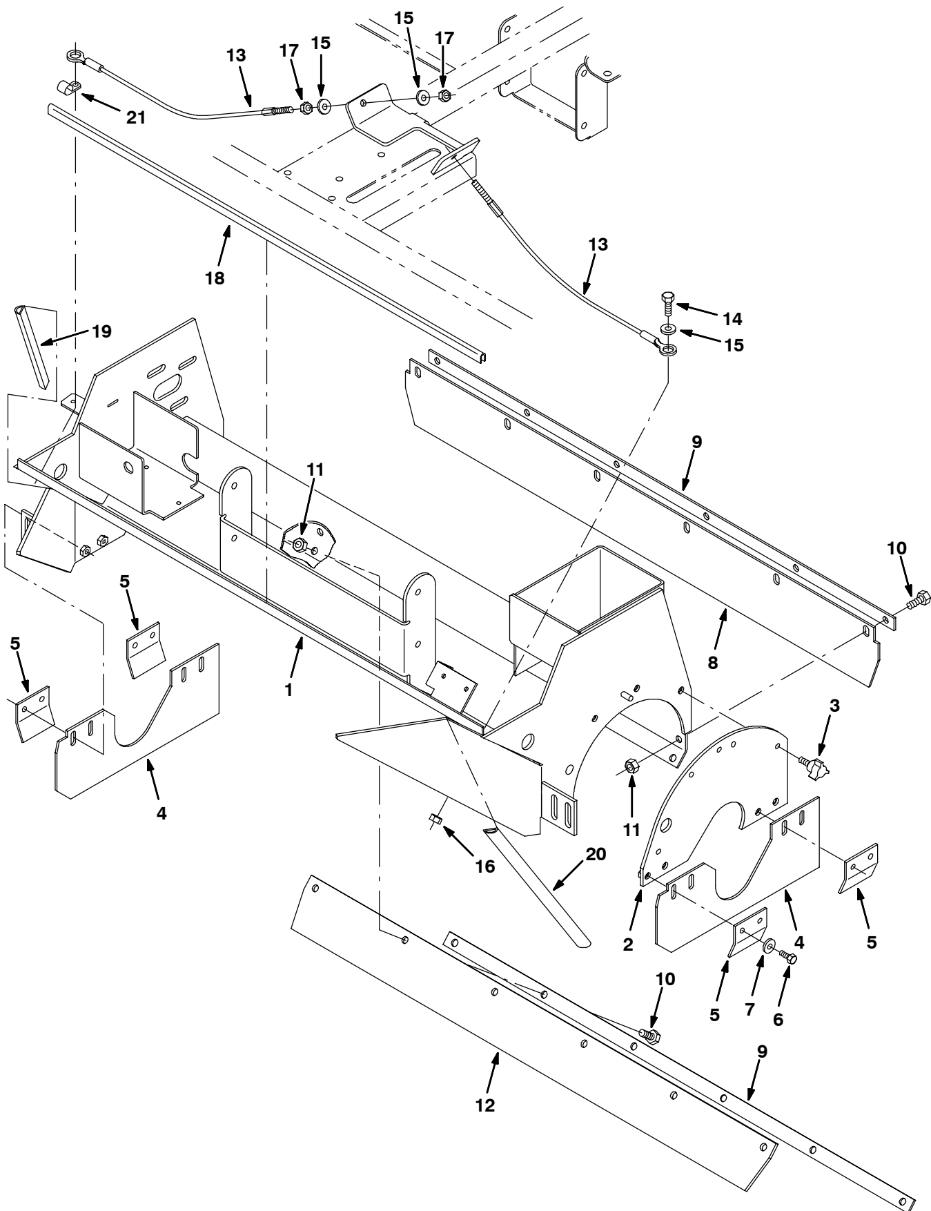
Fig. 35 - Pre-Sweep Brush Housing and Skirts Group
