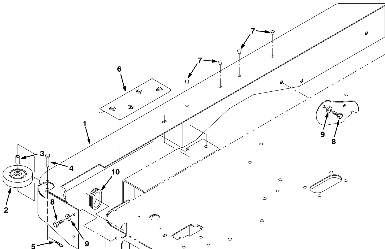
Fig. 47 - Side Brush Bumper Group
