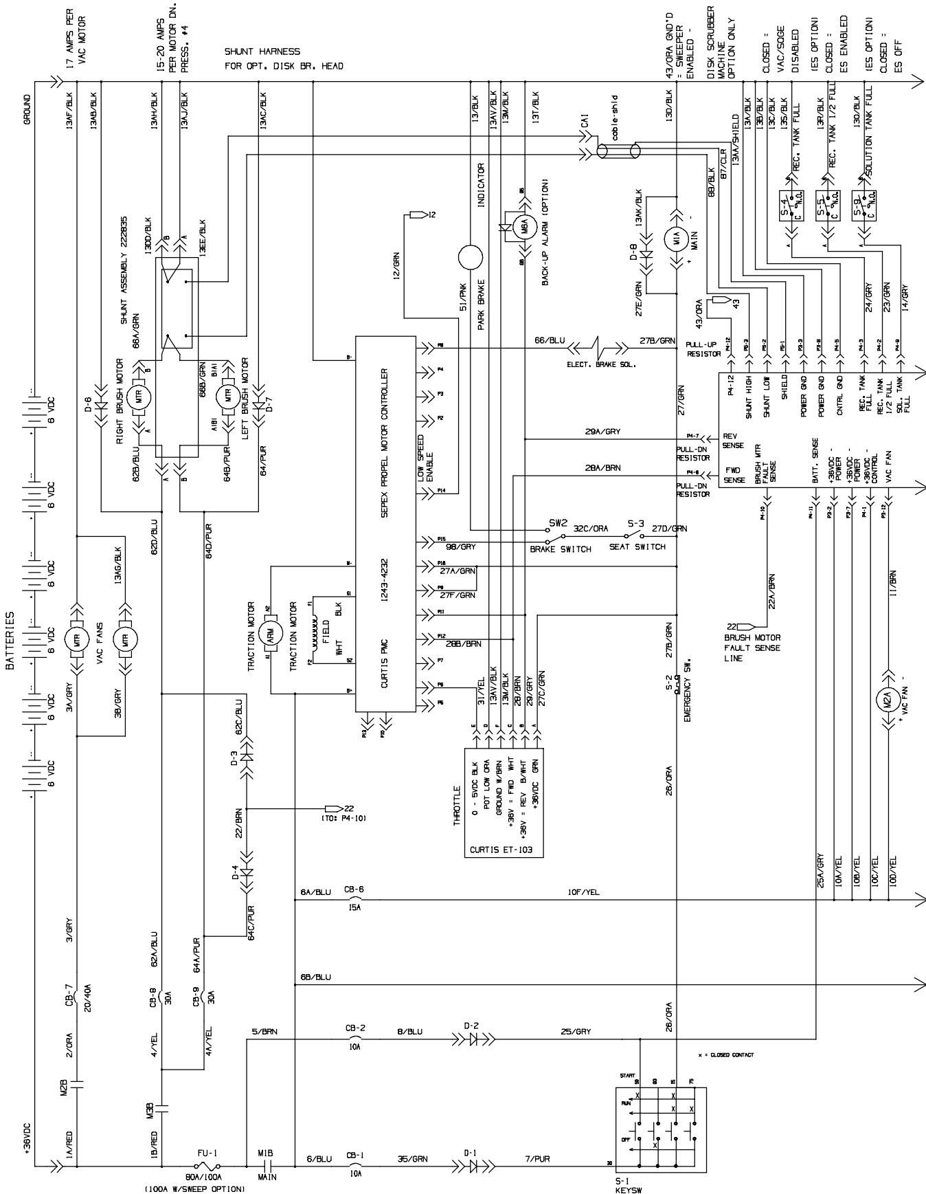
Fig. 31 - Electrical Schematic
