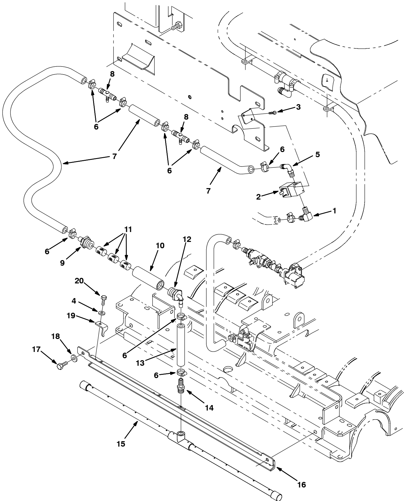
Fig. 23 - FaST Foam Filter Group, Cylindrical Scrub Head, 900mm (36 in)
