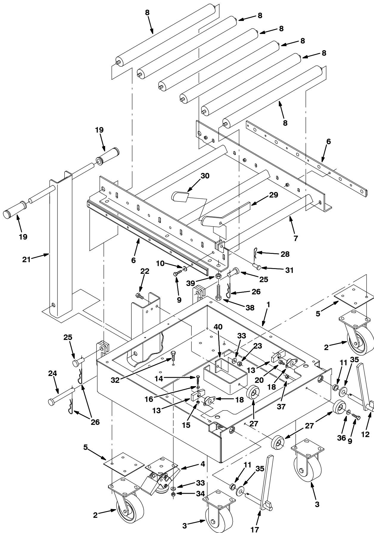
Fig. 31 - Rollout Battery Cart Kit
