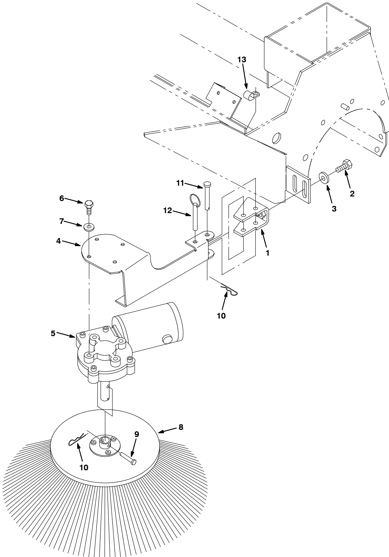
Fig. 43 - Pre-Sweep Side Brush Kit, Left Hand
