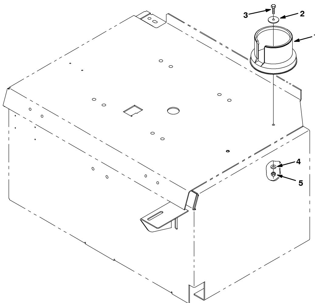
Fig. 51 - Cup Holder Kit
