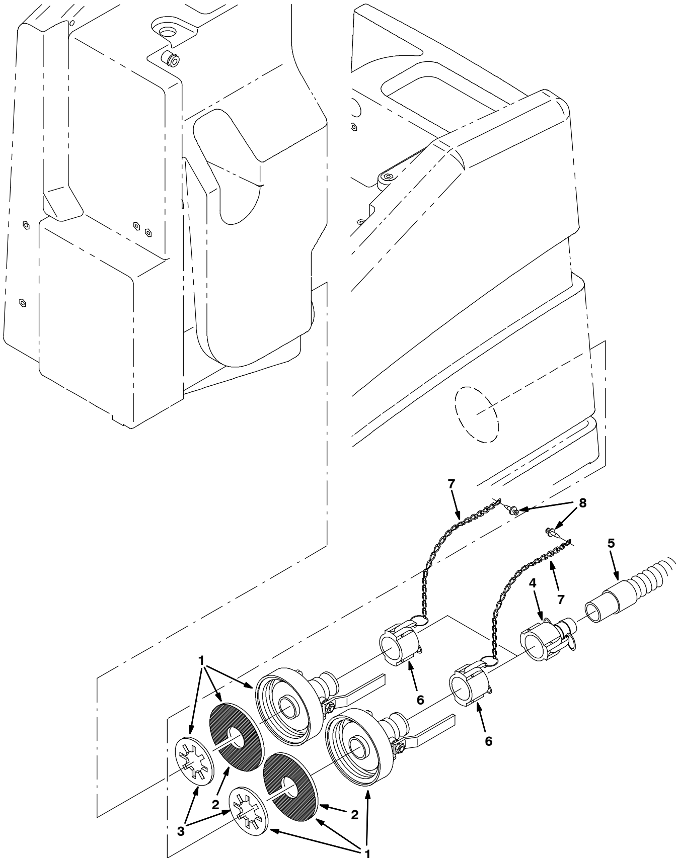
Fig. 21 - Positive Solution Control Drain Kit, ES
