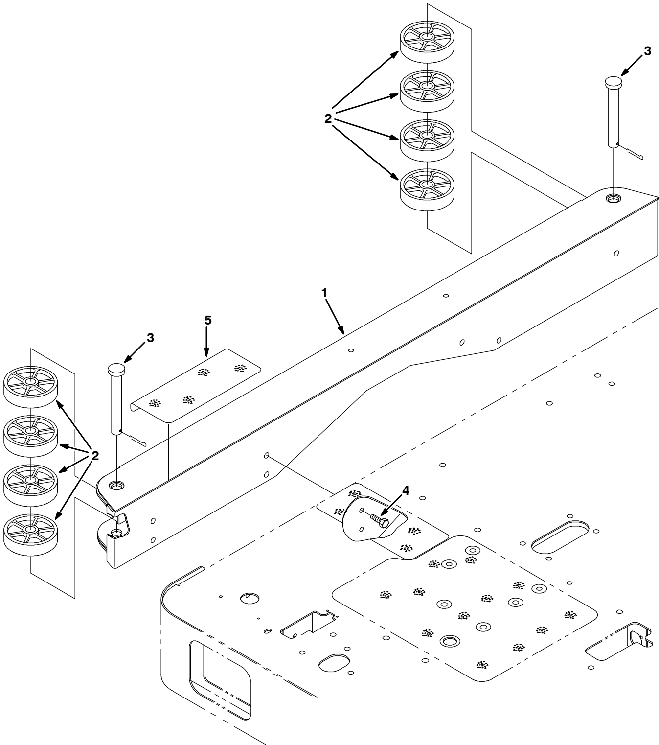
Fig. 29 - Rollout Battery Side Bumper Group, 900 mm (36 in)
