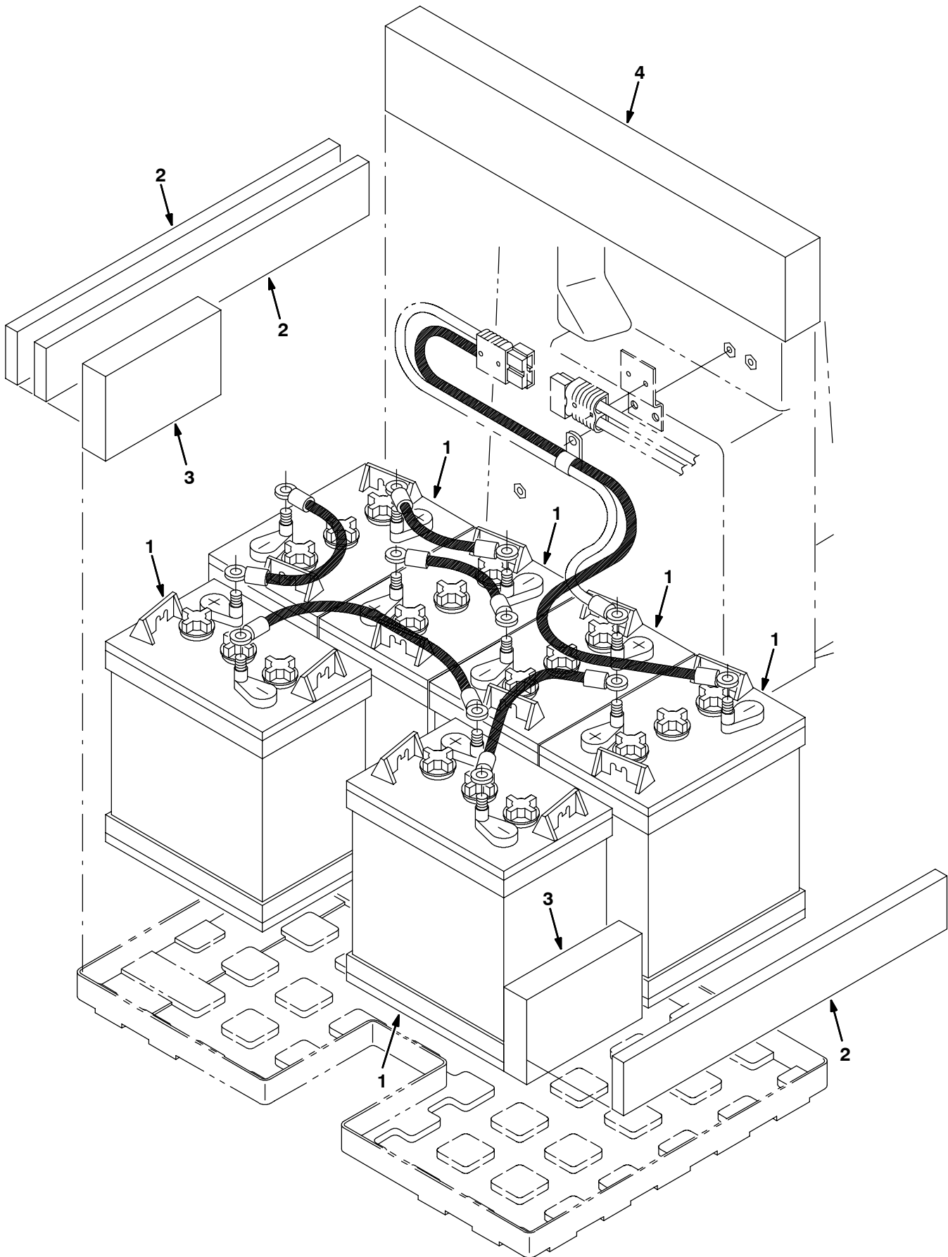
Fig. 22 - Battery Kit, Wet, 235AH
