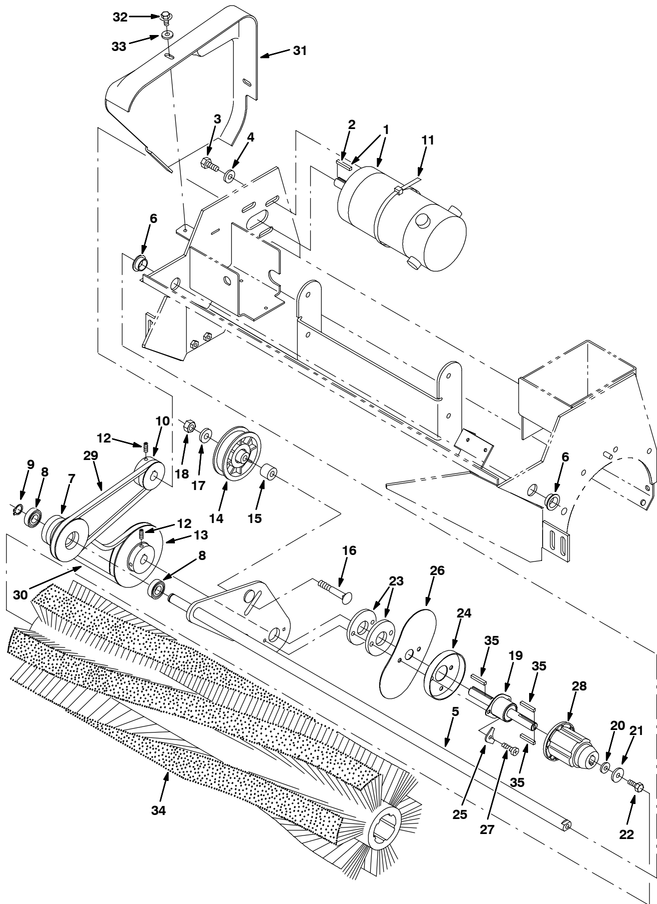
Fig. 36 - Pre-Sweep Brush Drive Group
