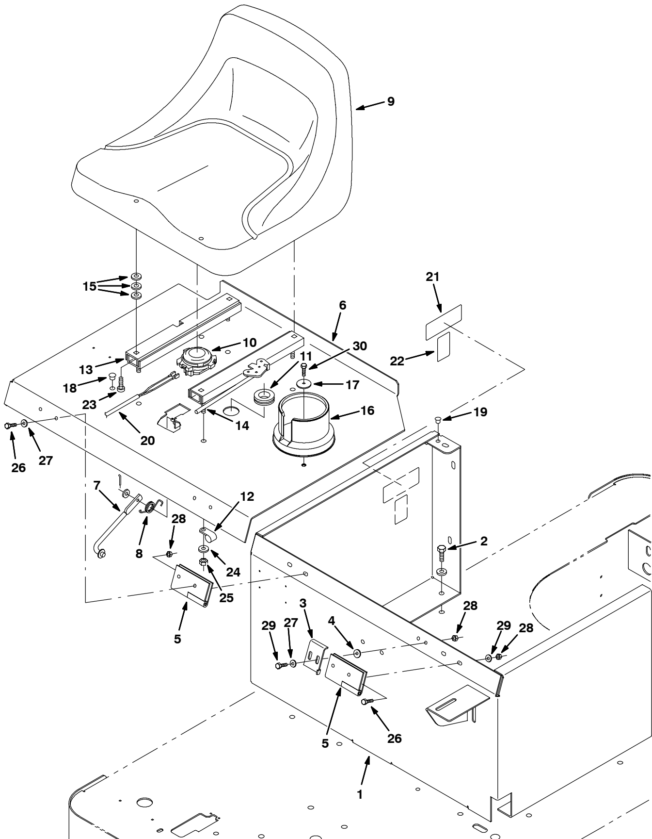
Fig. 3 - Seat Group
