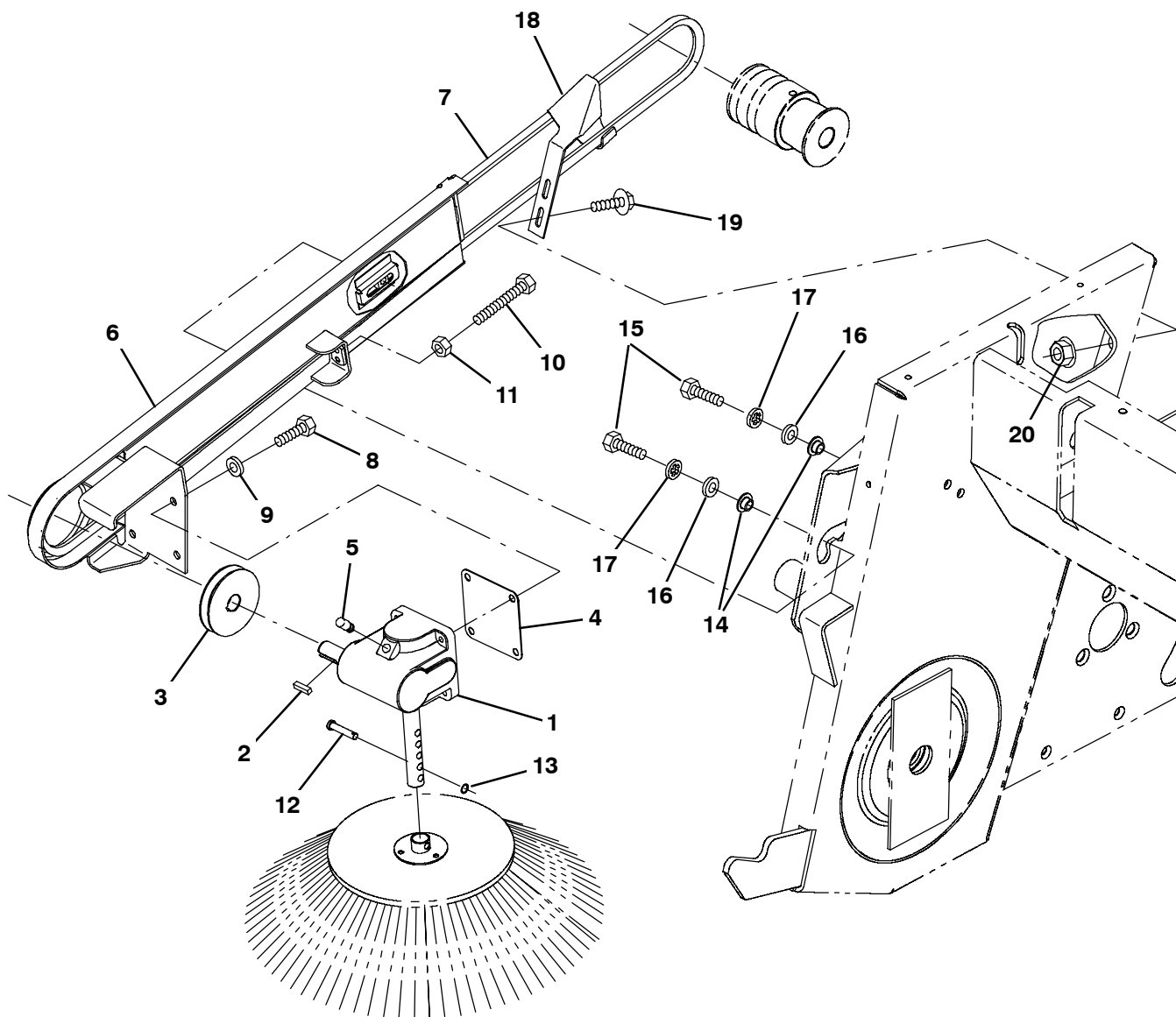
Fig. 7 - Side Brush Group
