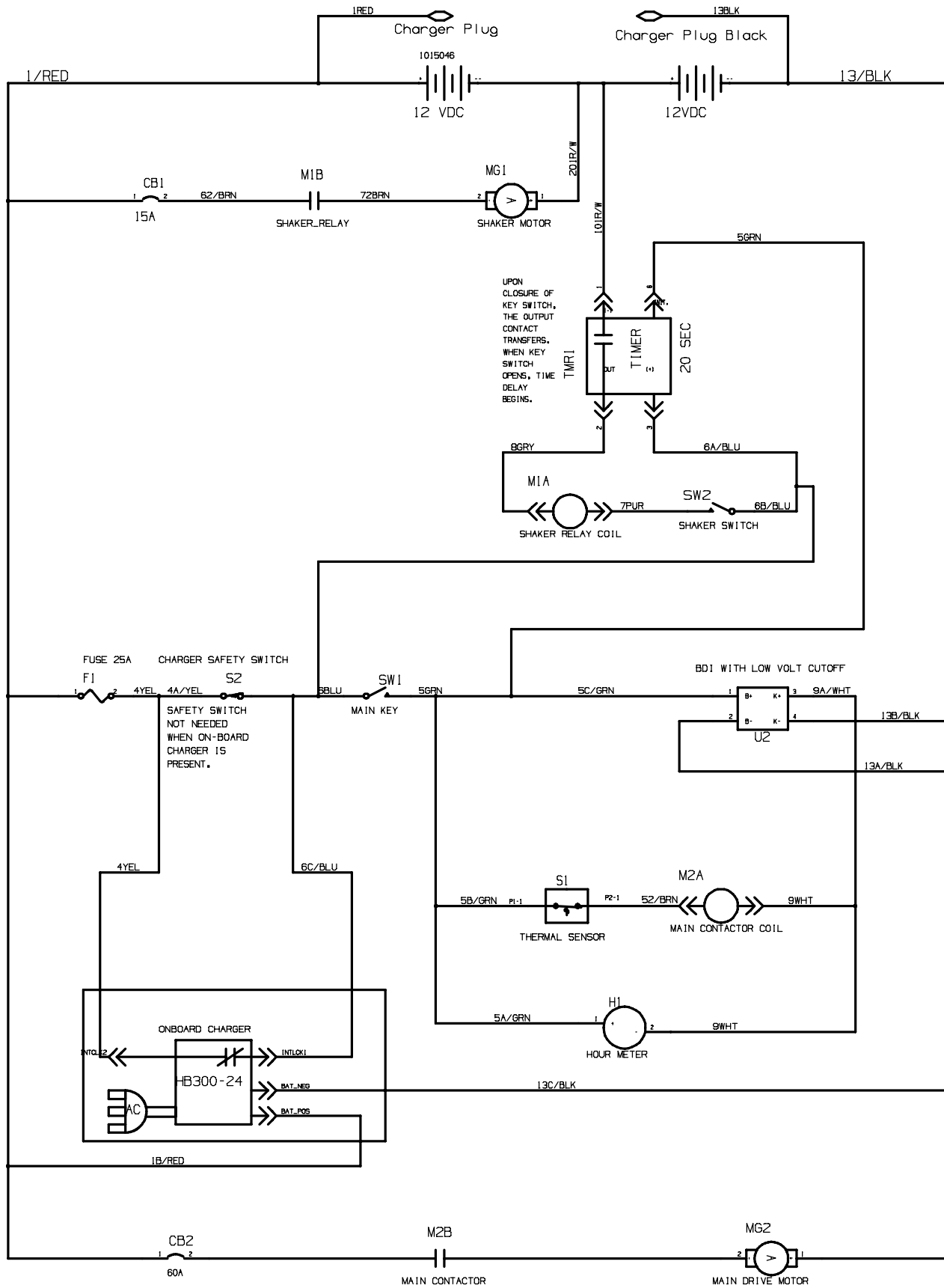
Fig. 16 - Electrical Schematic
