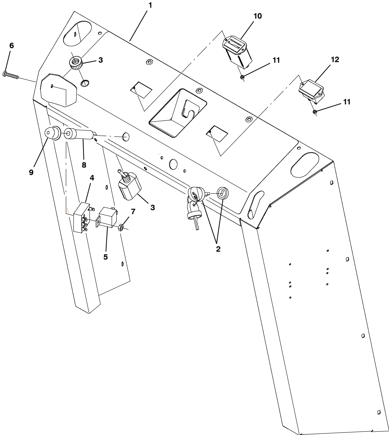
Fig. 10 - Instrument Panel Group
