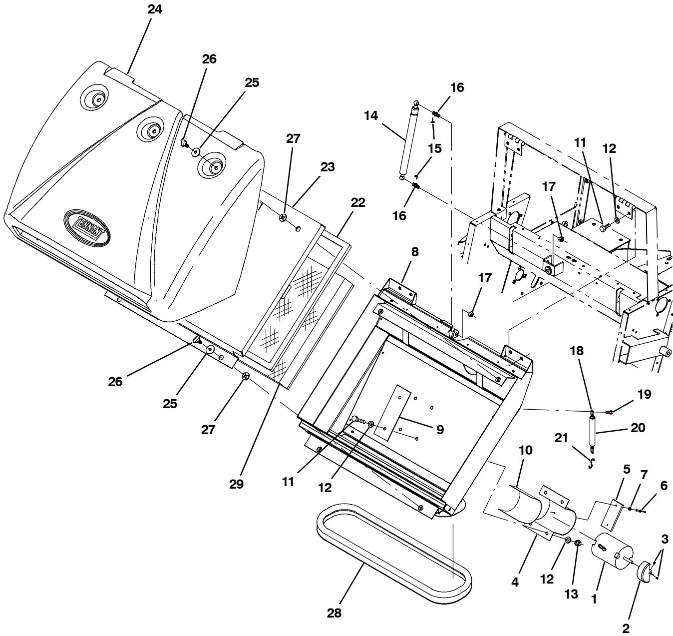
Fig. 13 - Filter and Shaker Motor Group
