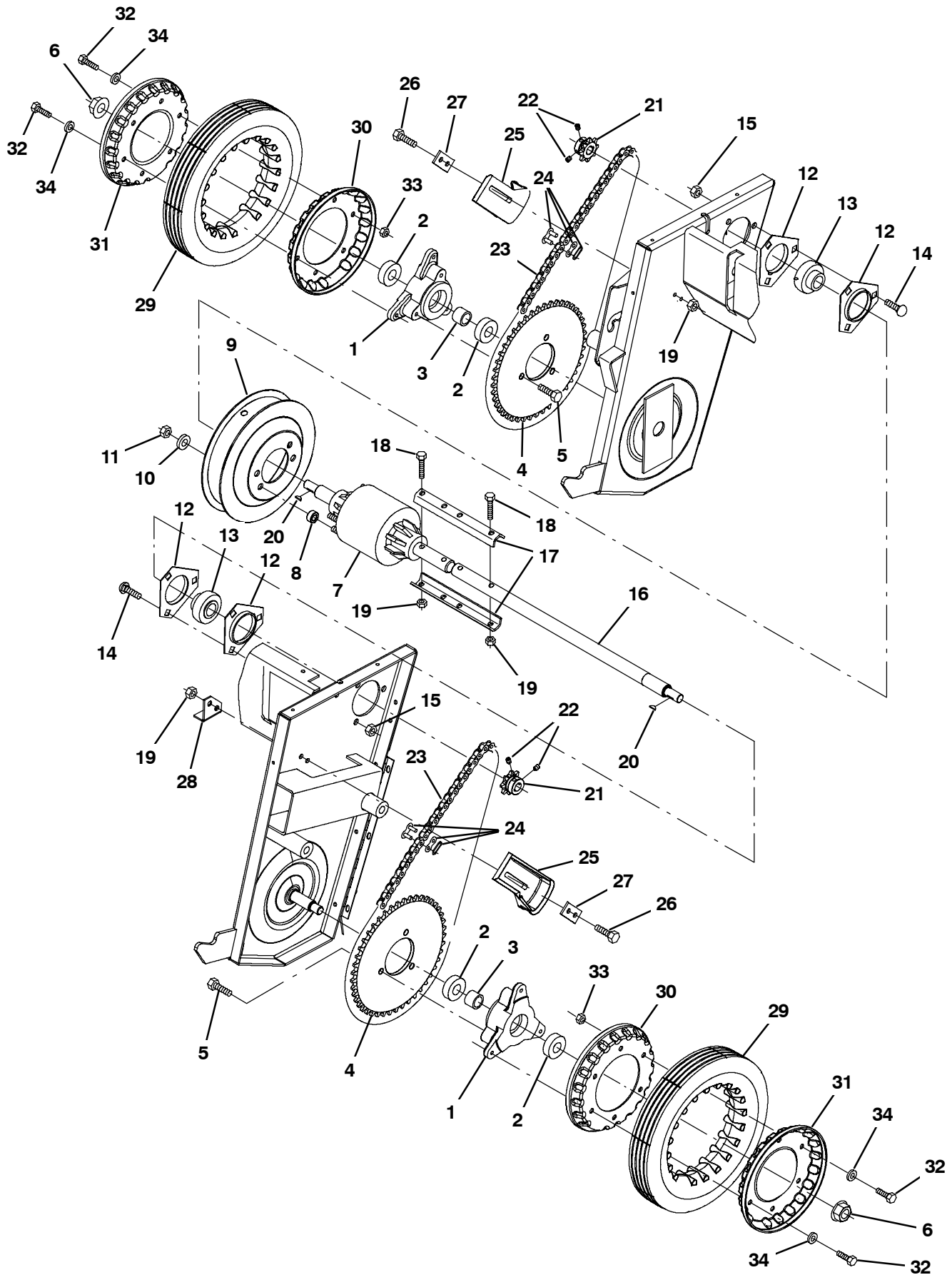
Fig. 4 - Wheel Group, Drive
