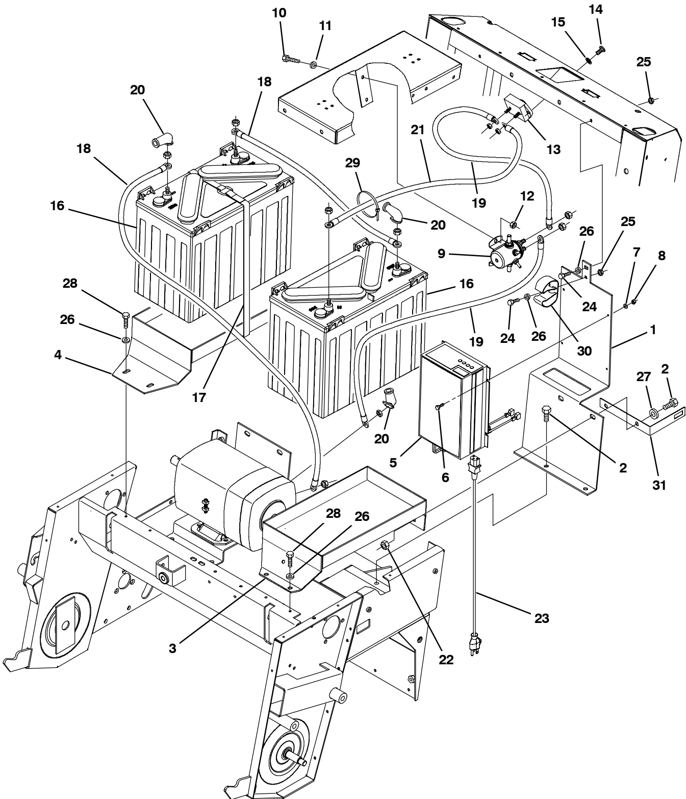
Fig. 9 - Battery and Charger Group
