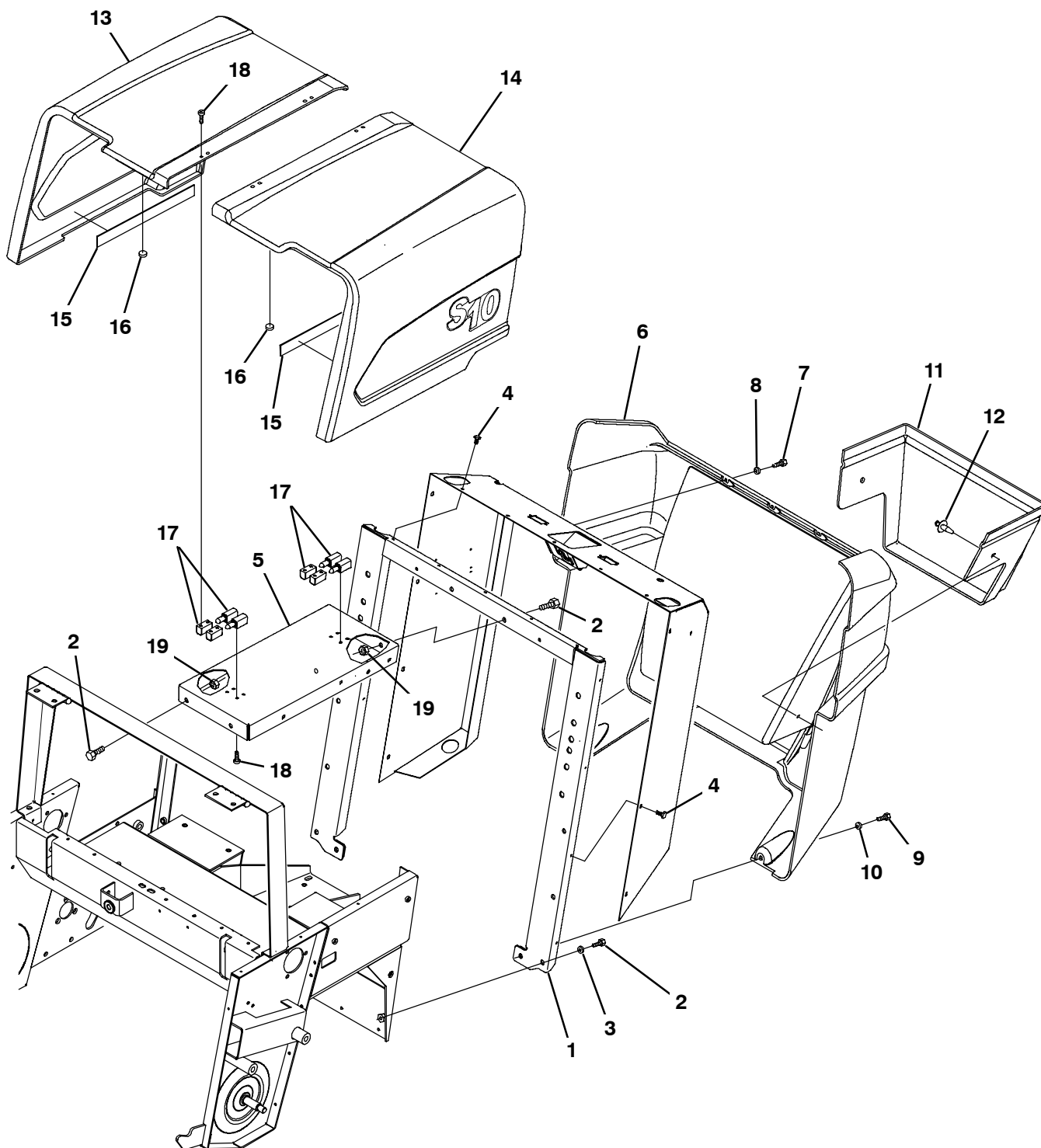
Fig. 15 - Covers Group
