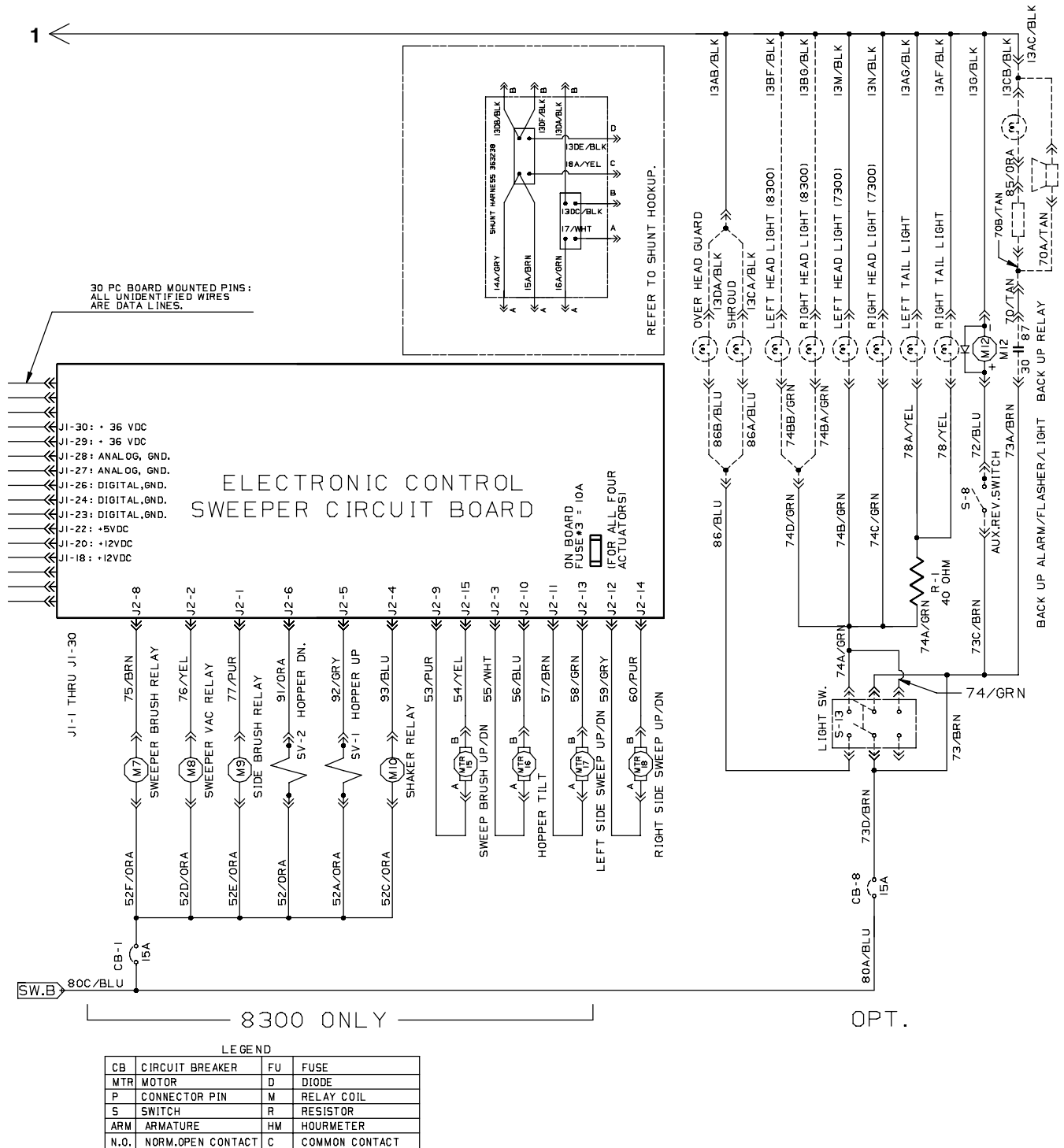
Fig. 55 - Electrical Schematic
