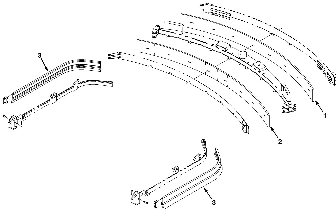
Fig. 51 - Max Pro 1200 Urethane Squeegee Kit
