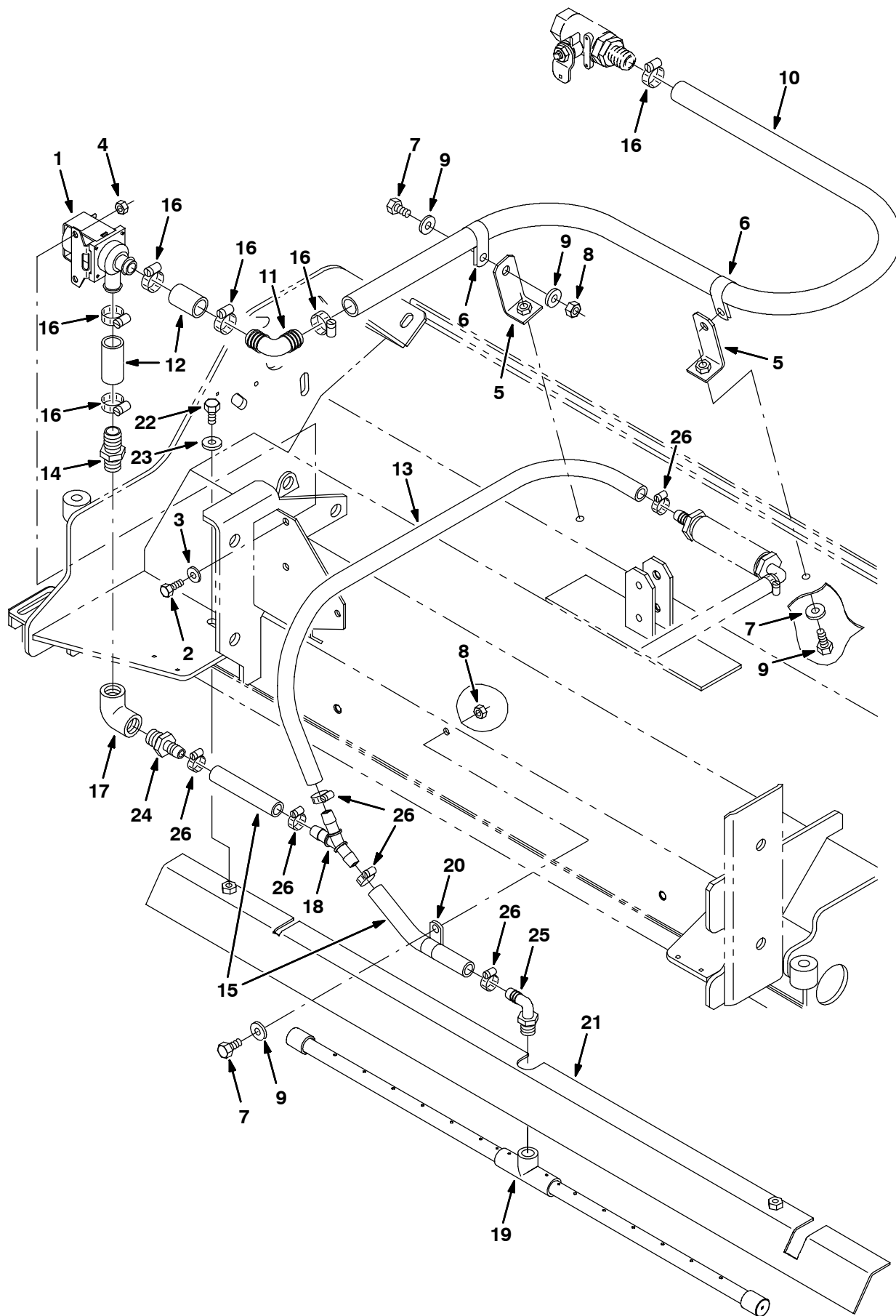
Fig. 30 - Max Pro 1200 (Cylindrical Brush) Solution Valve Group (FaST)
