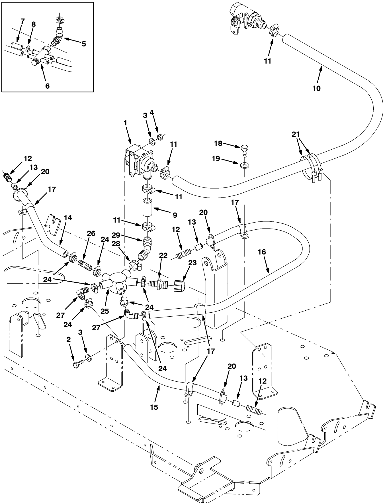
Fig. 12 - Max Pro 1200 (Disc-Brush) Solution Valve Group (Non FaST)
