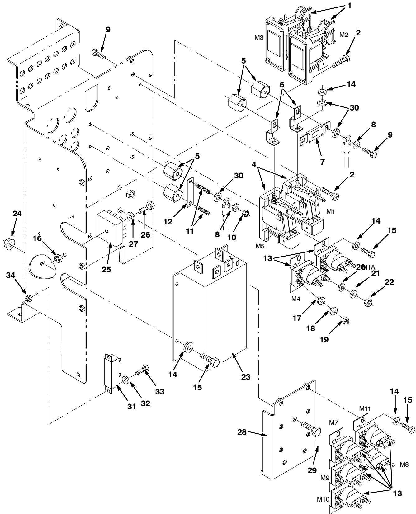
Fig. 49 - Electrical Control Box Contactor Group (000000-003545)
