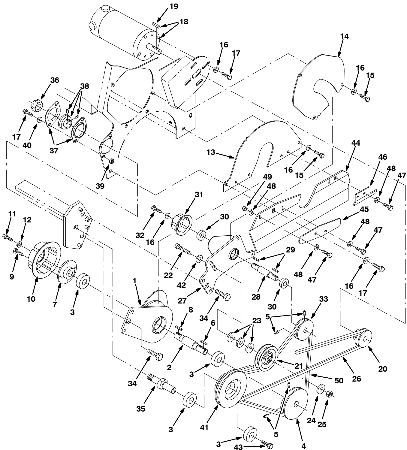
Fig. 36 - Sweeper Main Brush Drive Group
