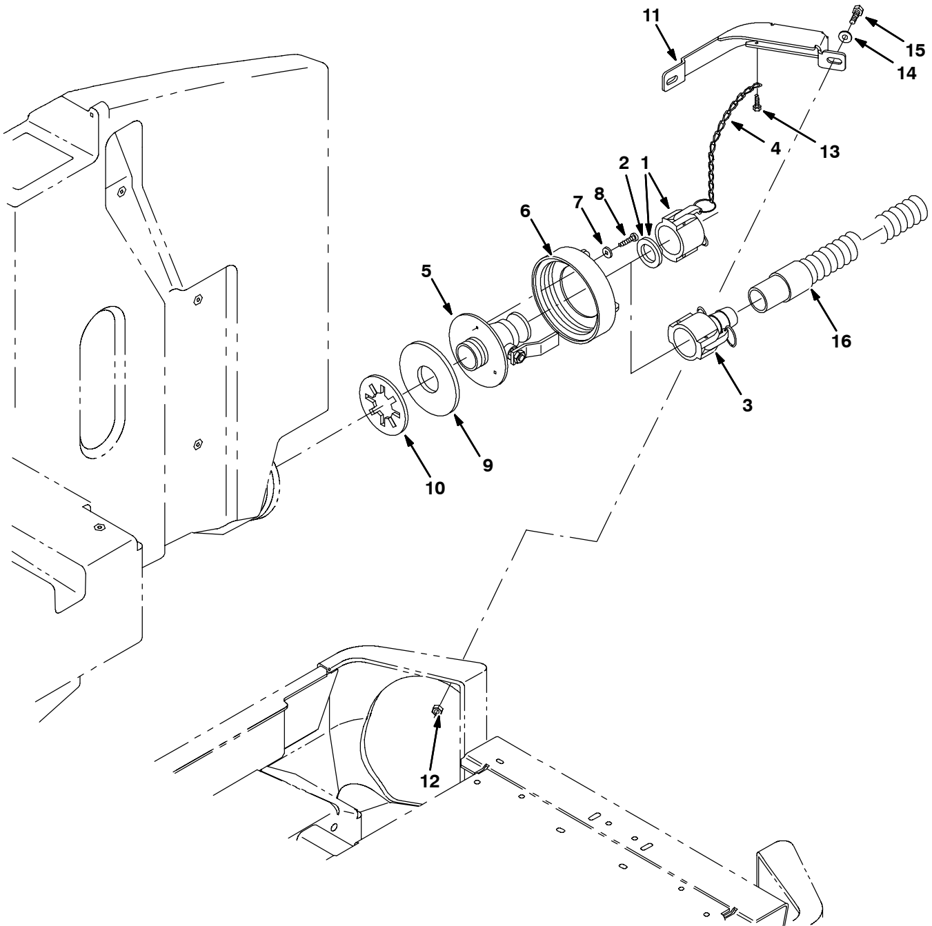
Fig. 40 - Positive Solution Control Drain Kit, Solution Tank
