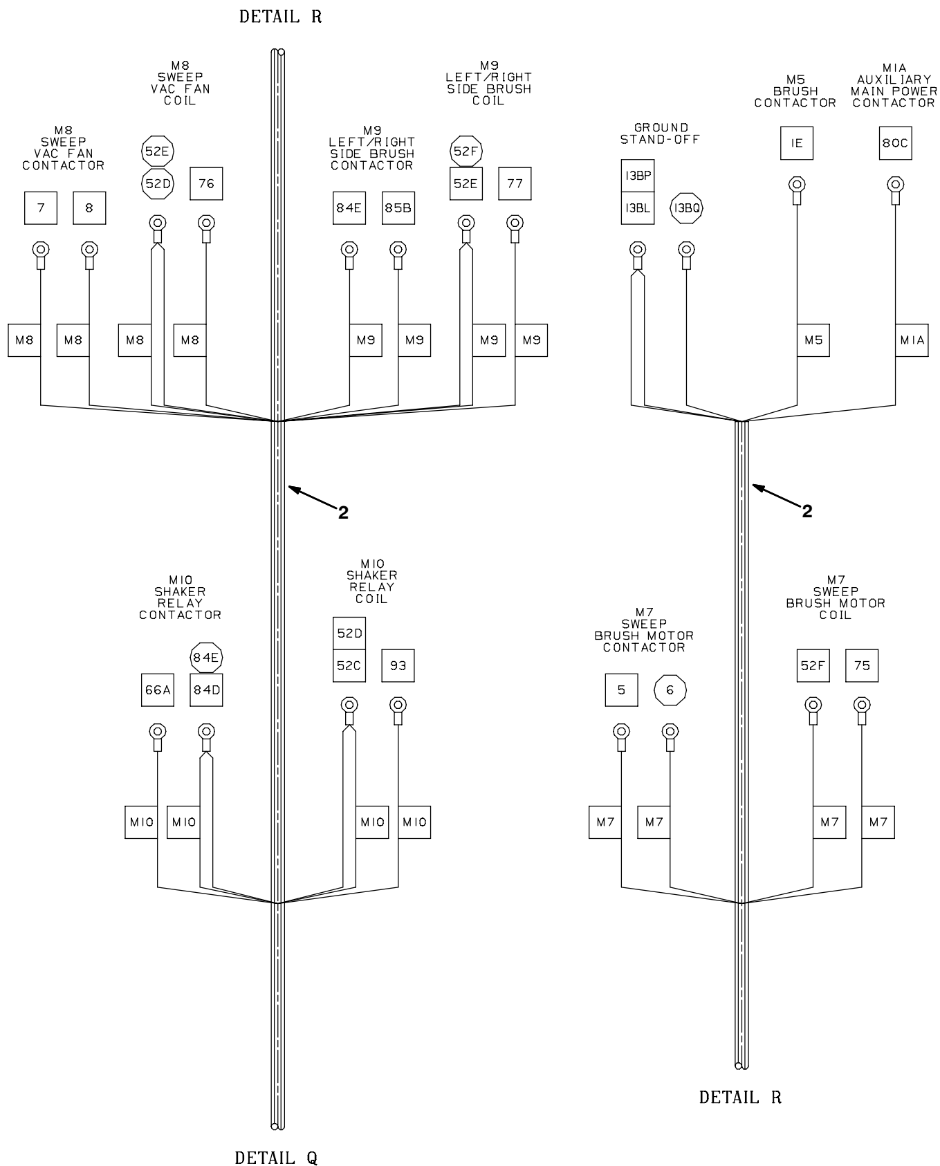
Fig. 56 - Electrical Wire Harnesses Group Hopper Harness Group
