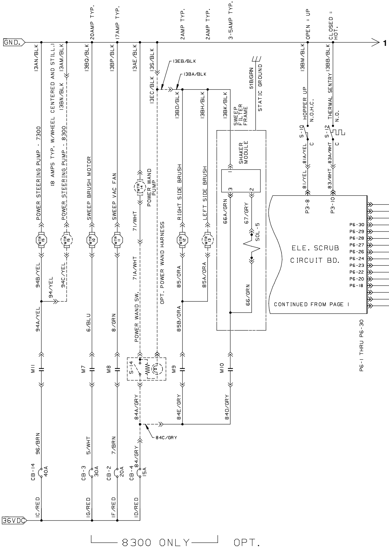
Fig. 55 - Electrical Schematic
