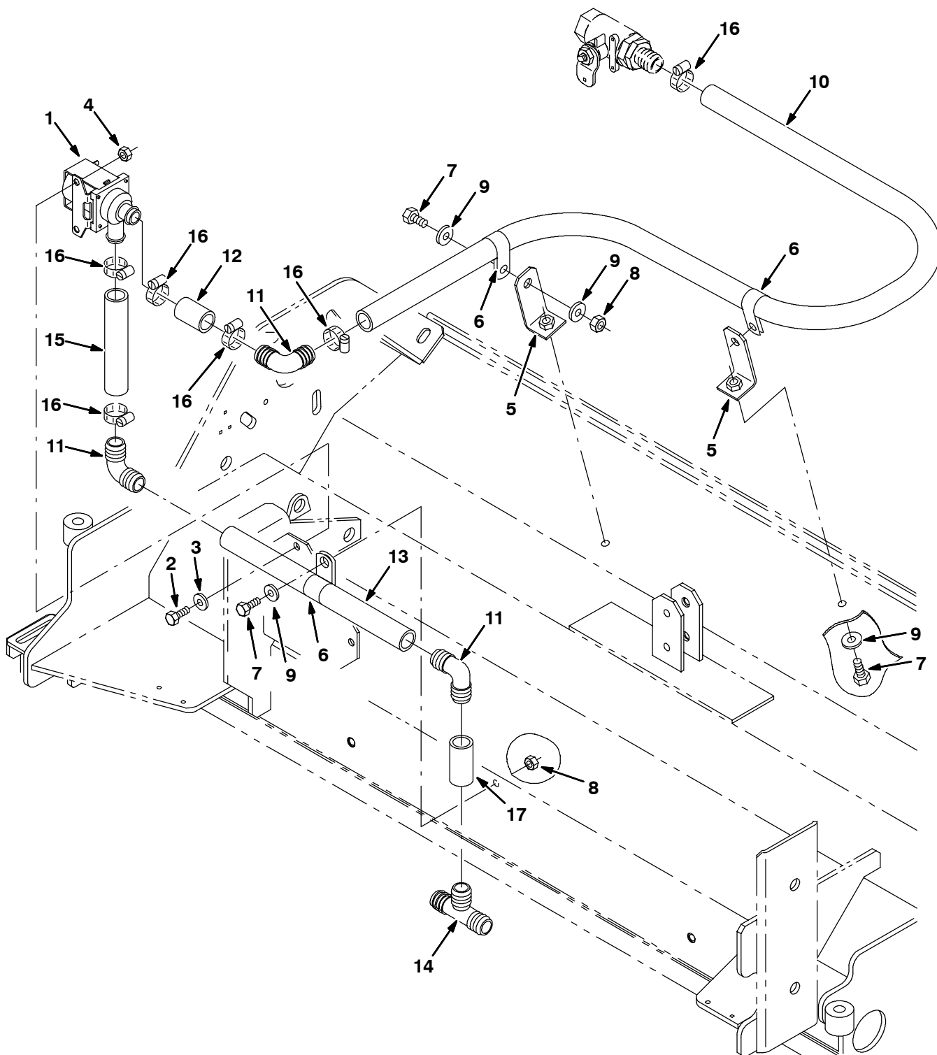
Fig. 29 - Max Pro 1200 (Cylindrical Brush) Solution Valve Group (Non FaST)
