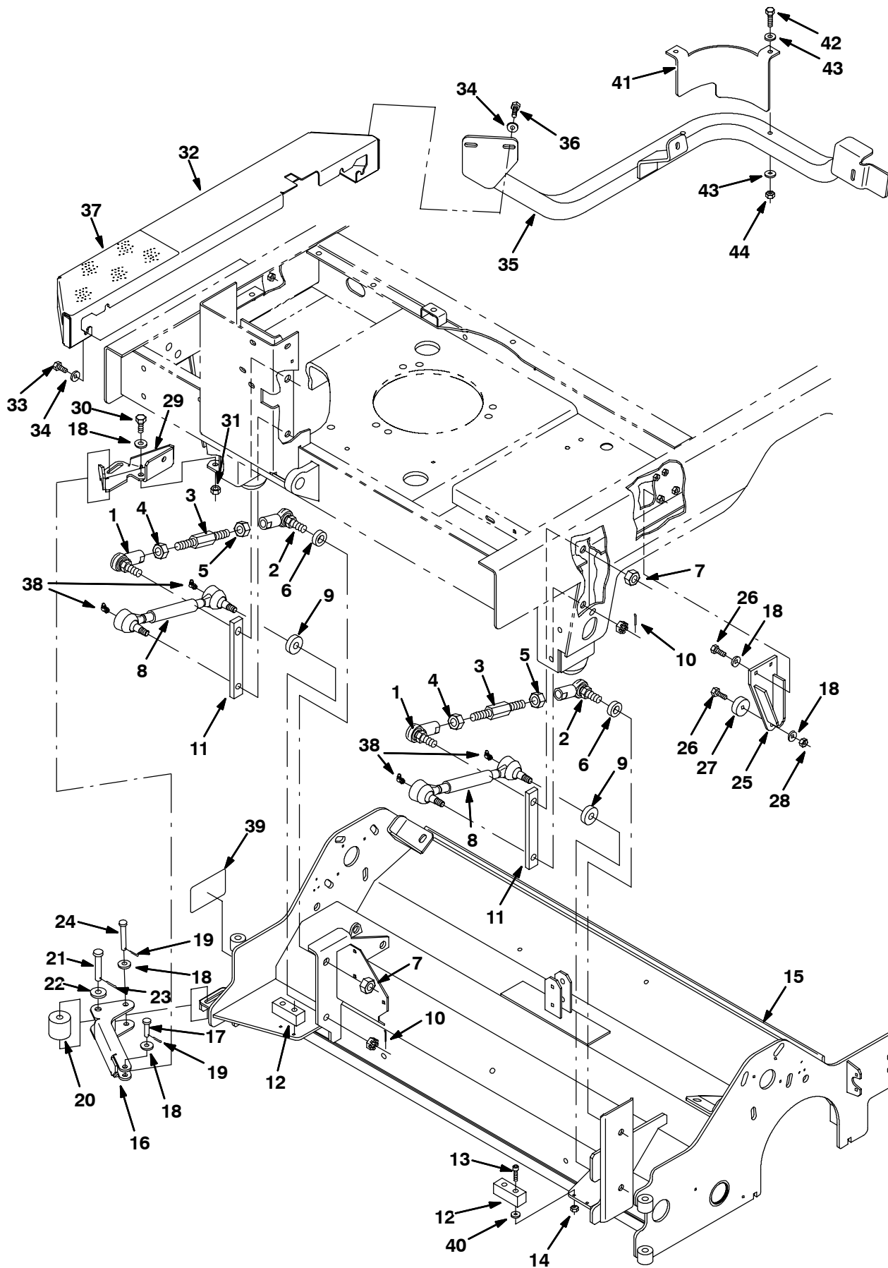
Fig. 27 - Max Pro 1200 (Cylindrical Brush) Scrub Head Frame and Linkage Group
