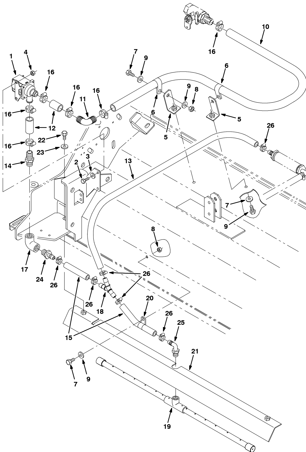
Fig. 21 - Max Pro 1000 (Cylindrical Brush) Solution Valve Group (FaST)
