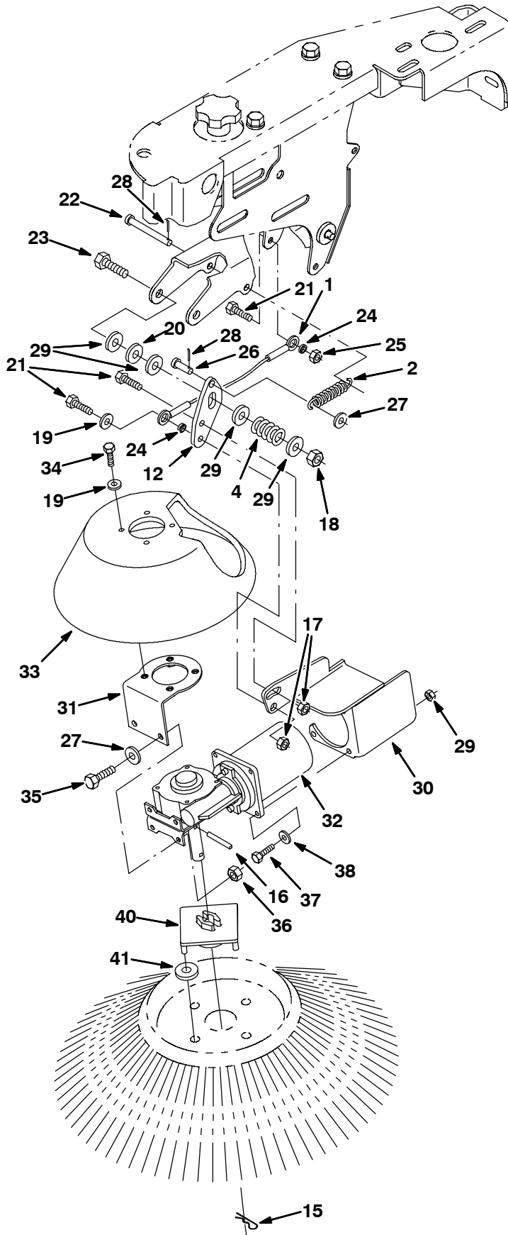
Fig. 34 - Sweeper Side Brush Motor and Pivot Group
