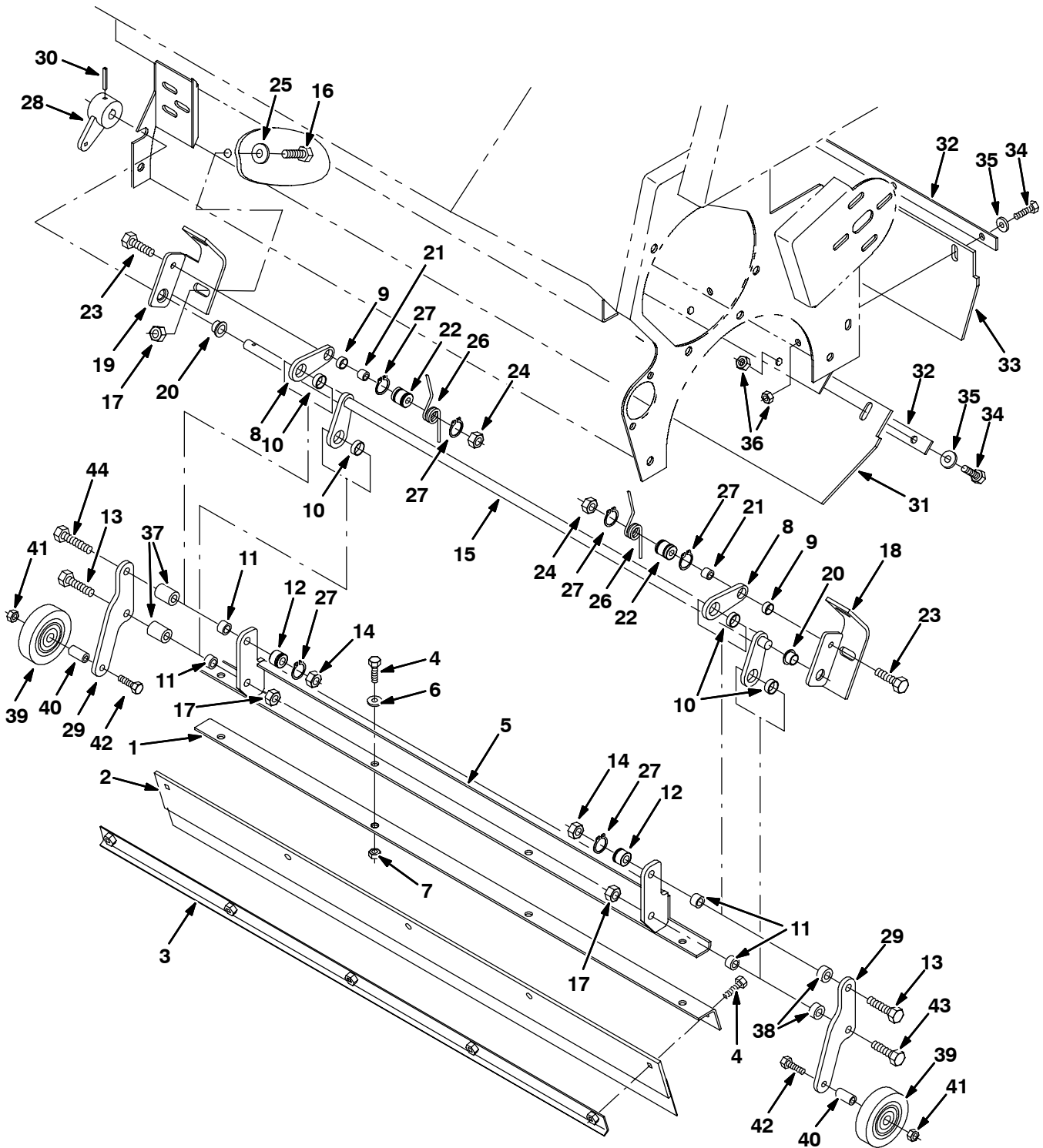
Fig. 40 - Sweeper Main Brush Skirts Group
