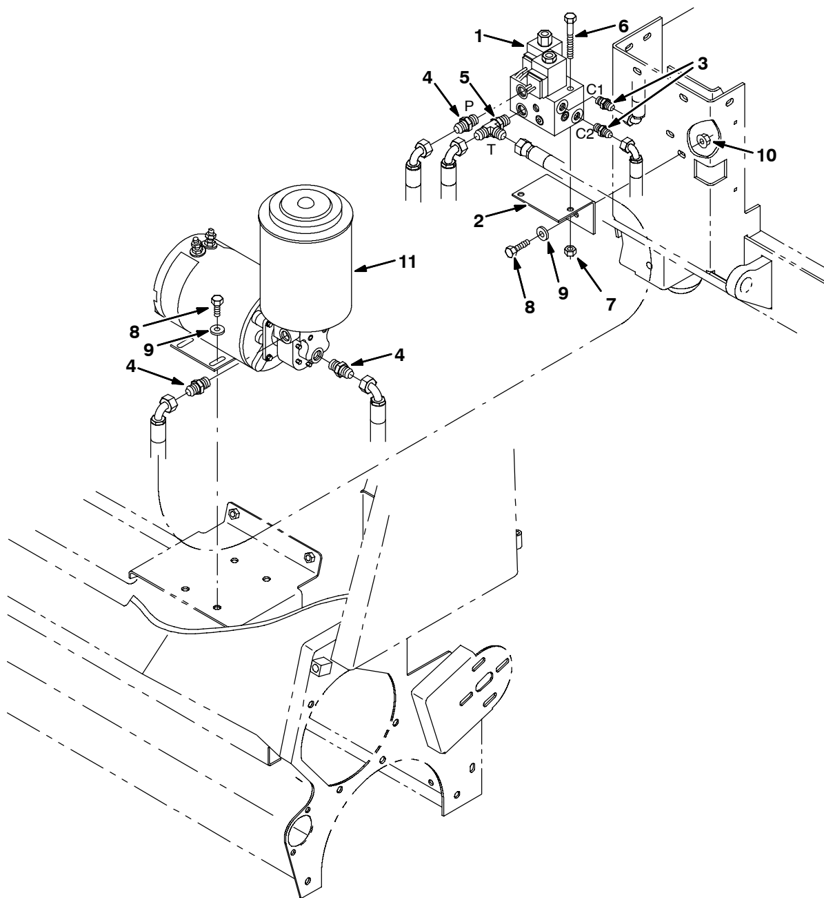
Fig. 45 - Hydraulic Power Unit and Solenoid Valve Group
