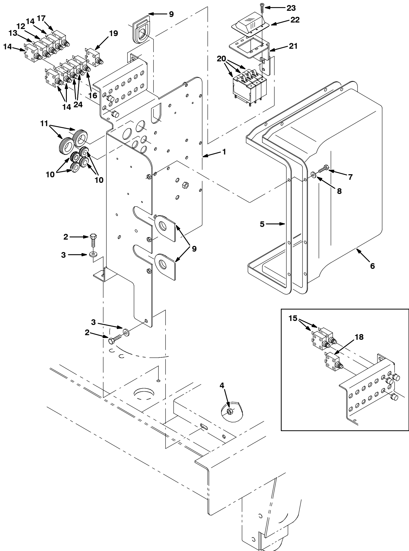
Fig. 48 - Electrical Control Box Circuit Breaker Group
