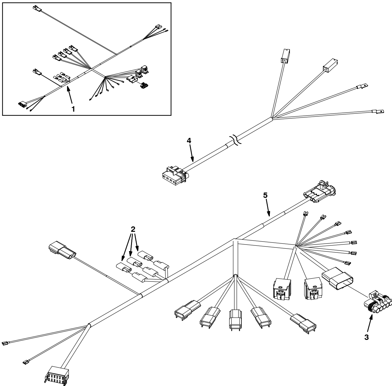
Fig. 57 - Electrical Wire Harness Group, FaST
