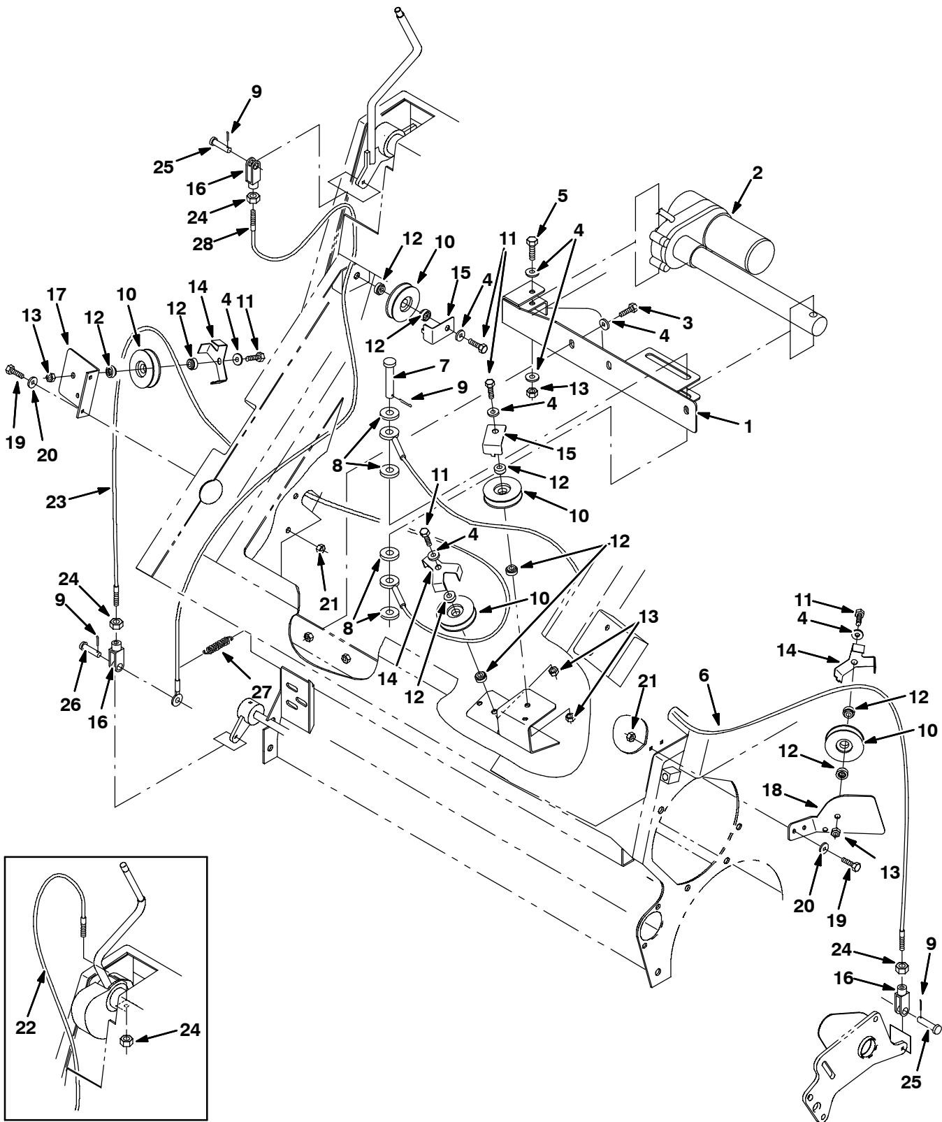
Fig. 38 - Sweeper Main Brush Lift Group
