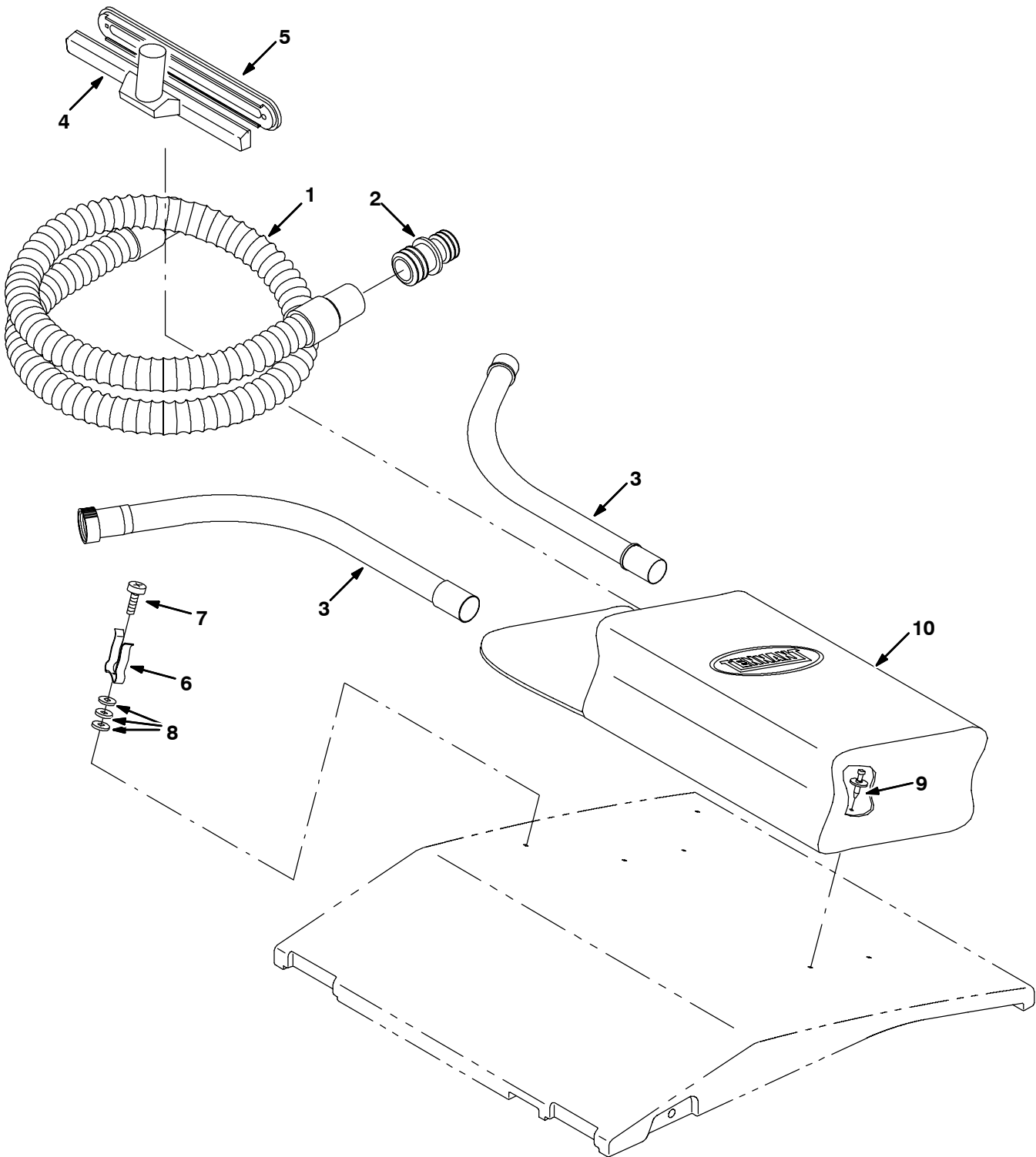
Fig. 47 - Vacuum Wand Kit
