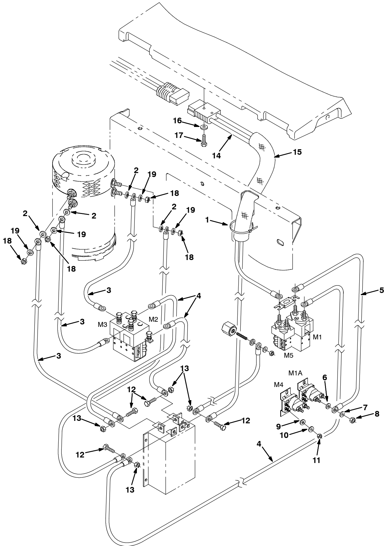
Fig. 52 - Electrical Control Box Wires Group (003546- )
