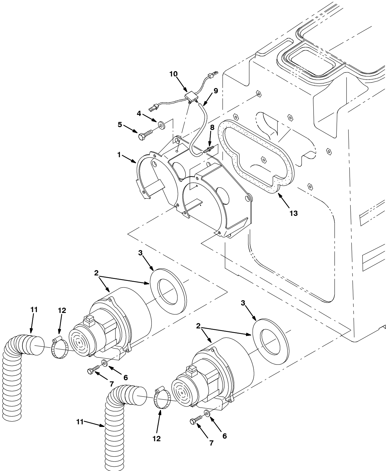
Fig. 21 - Scrubber Vacuum Fan Group
