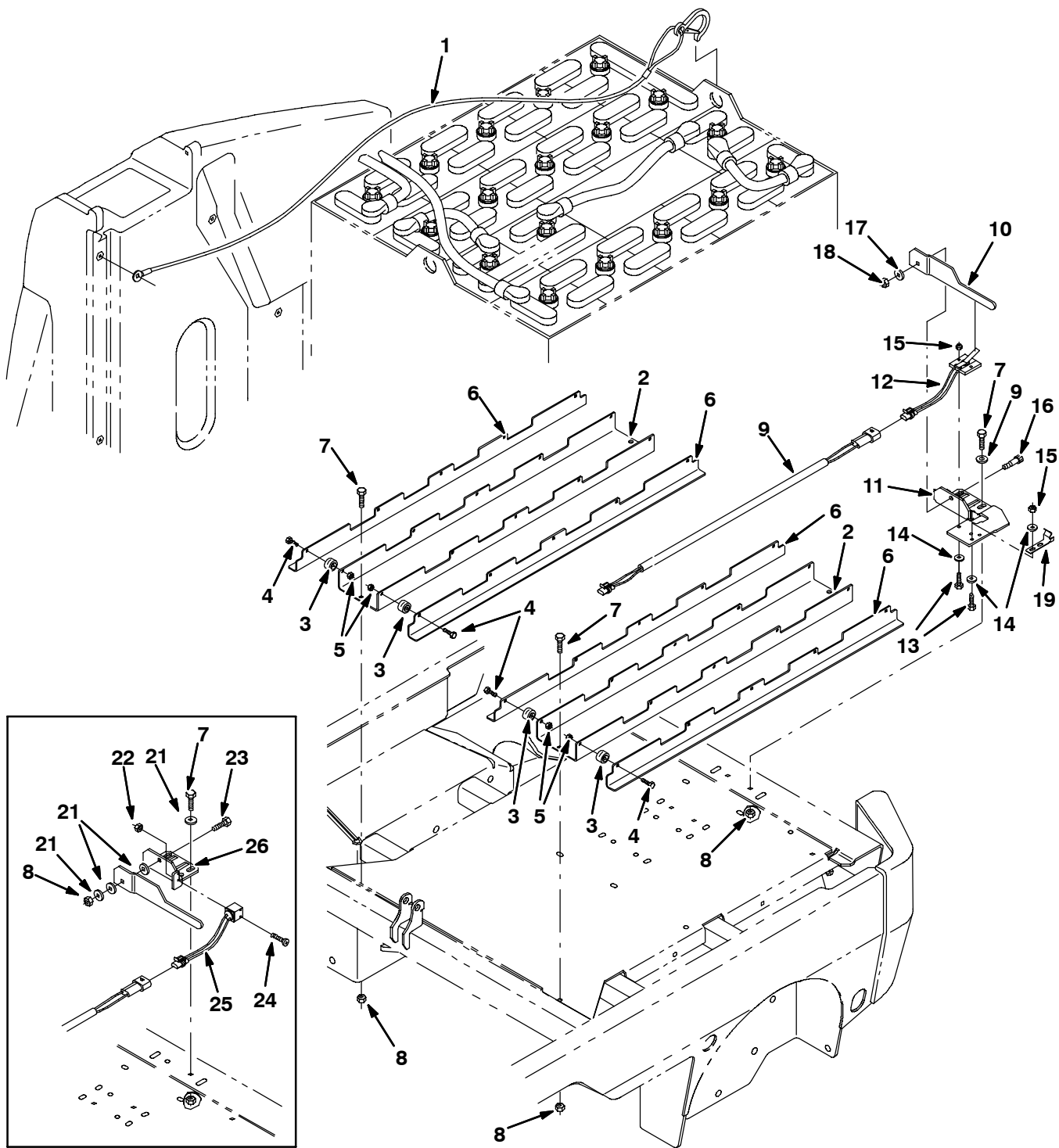
Fig. 52 - Battery Rollout Kit
