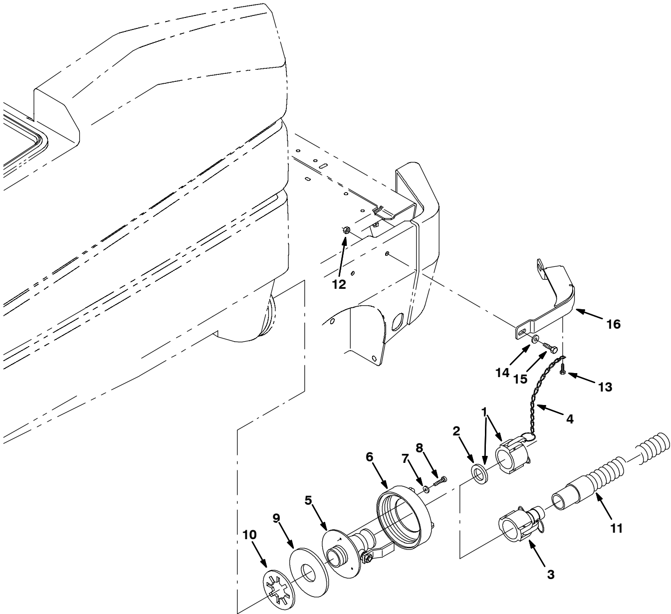
Fig. 39 - Positive Solution Control Drain Kit, Recovery Tank
