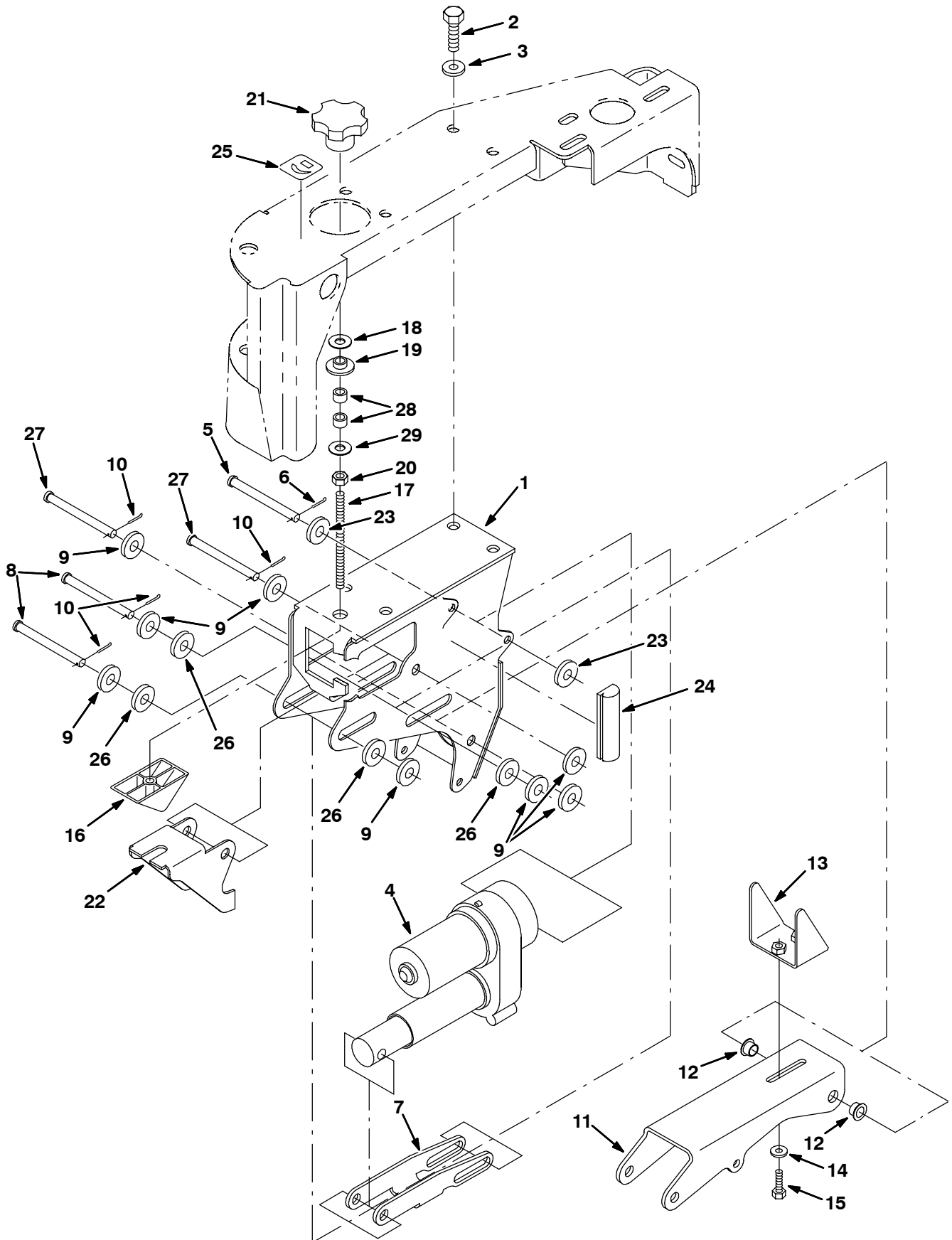
Fig. 35 - Sweeper Side Brush Lift Group
