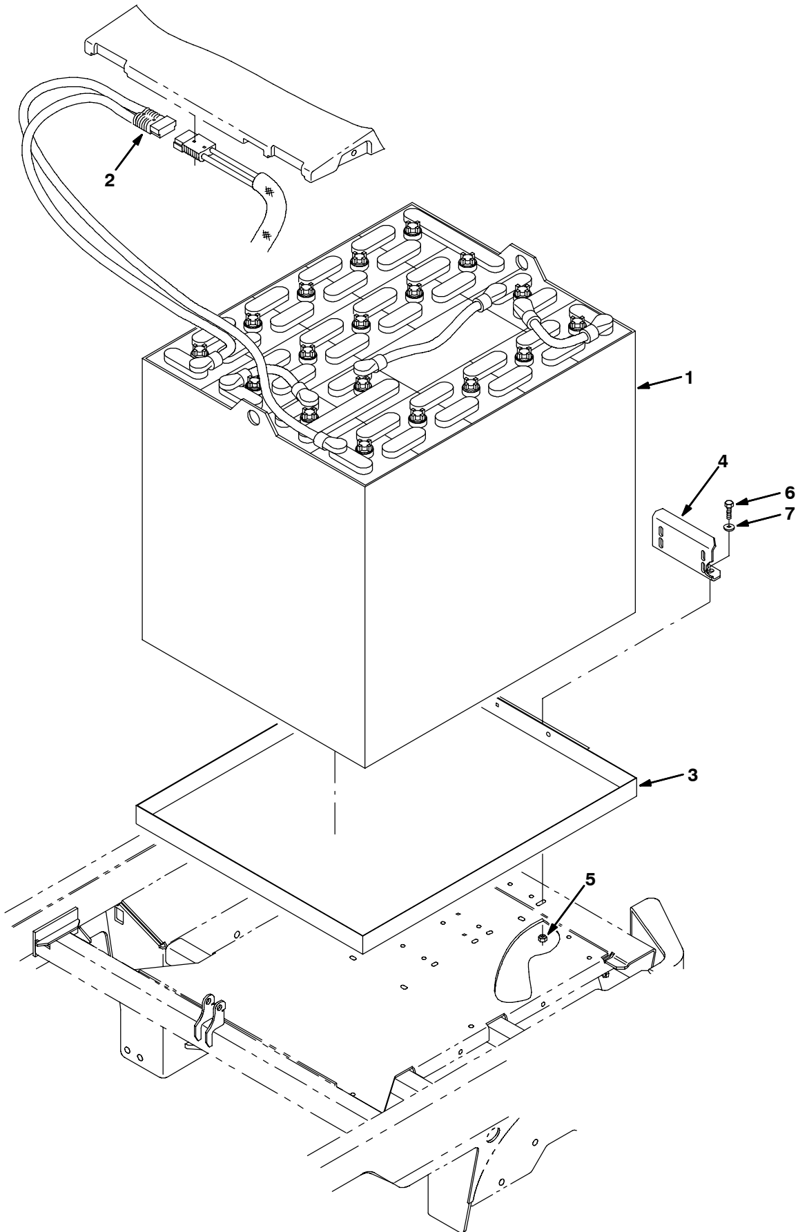
Fig. 57 - Battery Kit, 1000AH Wet
