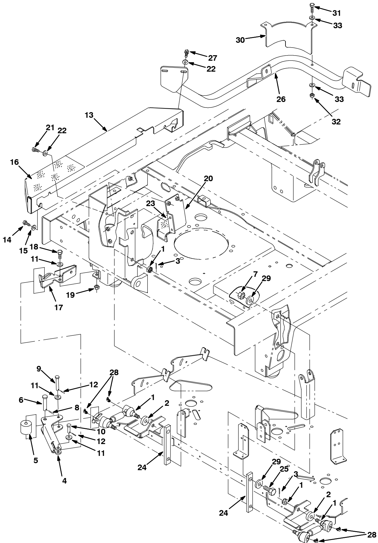
Fig. 11 - Max Pro 1200 (Disc-Brush) Scrub Head Linkage Group
