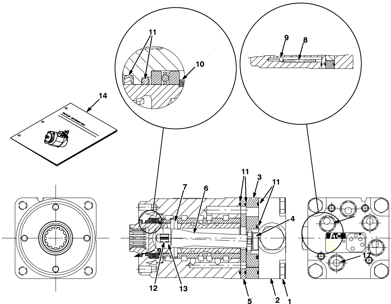
Fig. 15 - Steering Control Valve Breakdown, 373495
