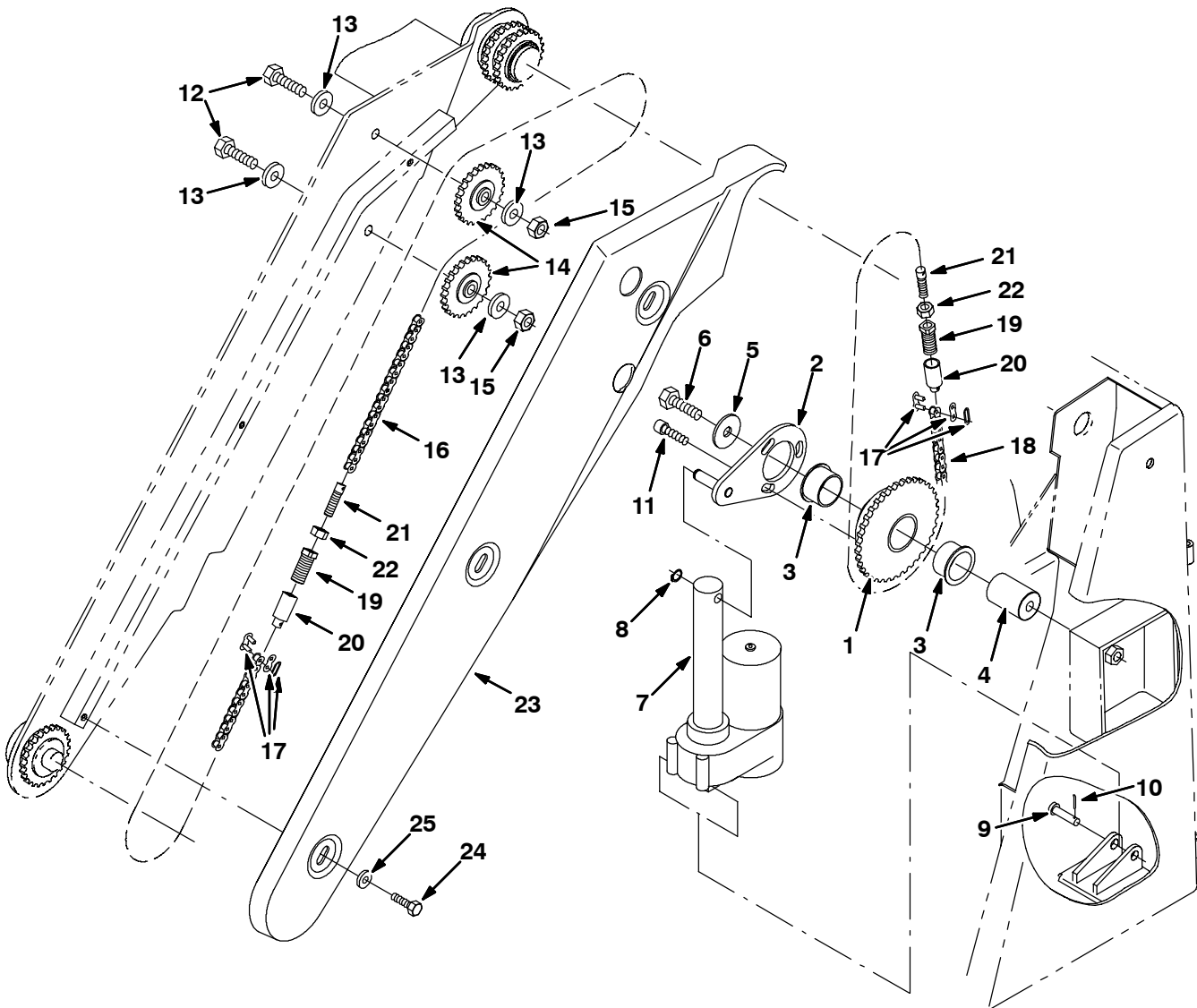
Fig. 42 - Hopper Chain and Cover Group
