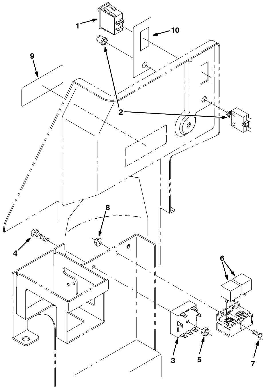
Fig. 54 - Electrical Group, FaST
