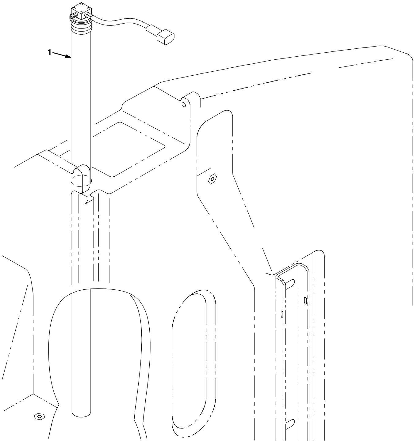
Fig. 41 - Low Water Level Kit
