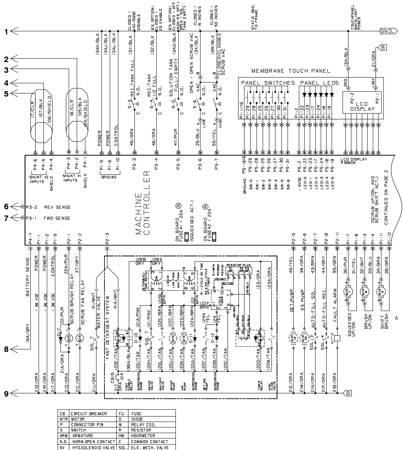
Fig. 55 - Electrical Schematic
