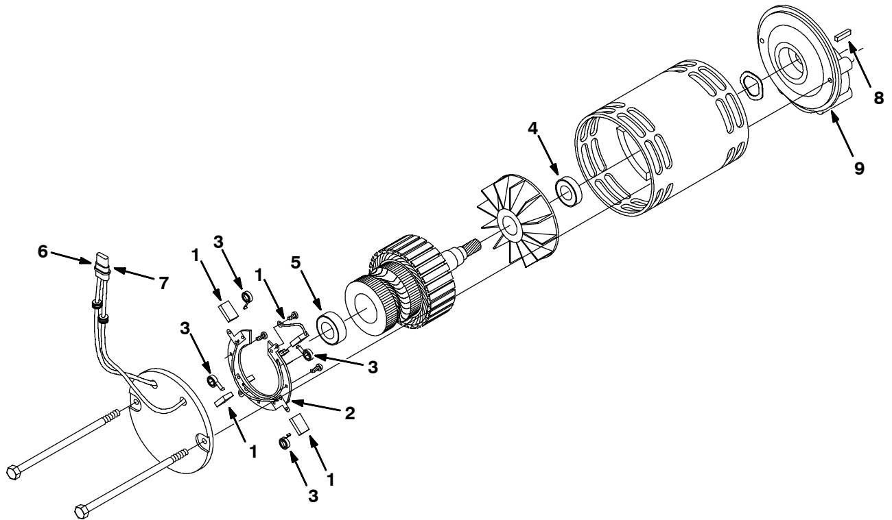
Fig. 16 - Electric Motor Breakdown, 387585
