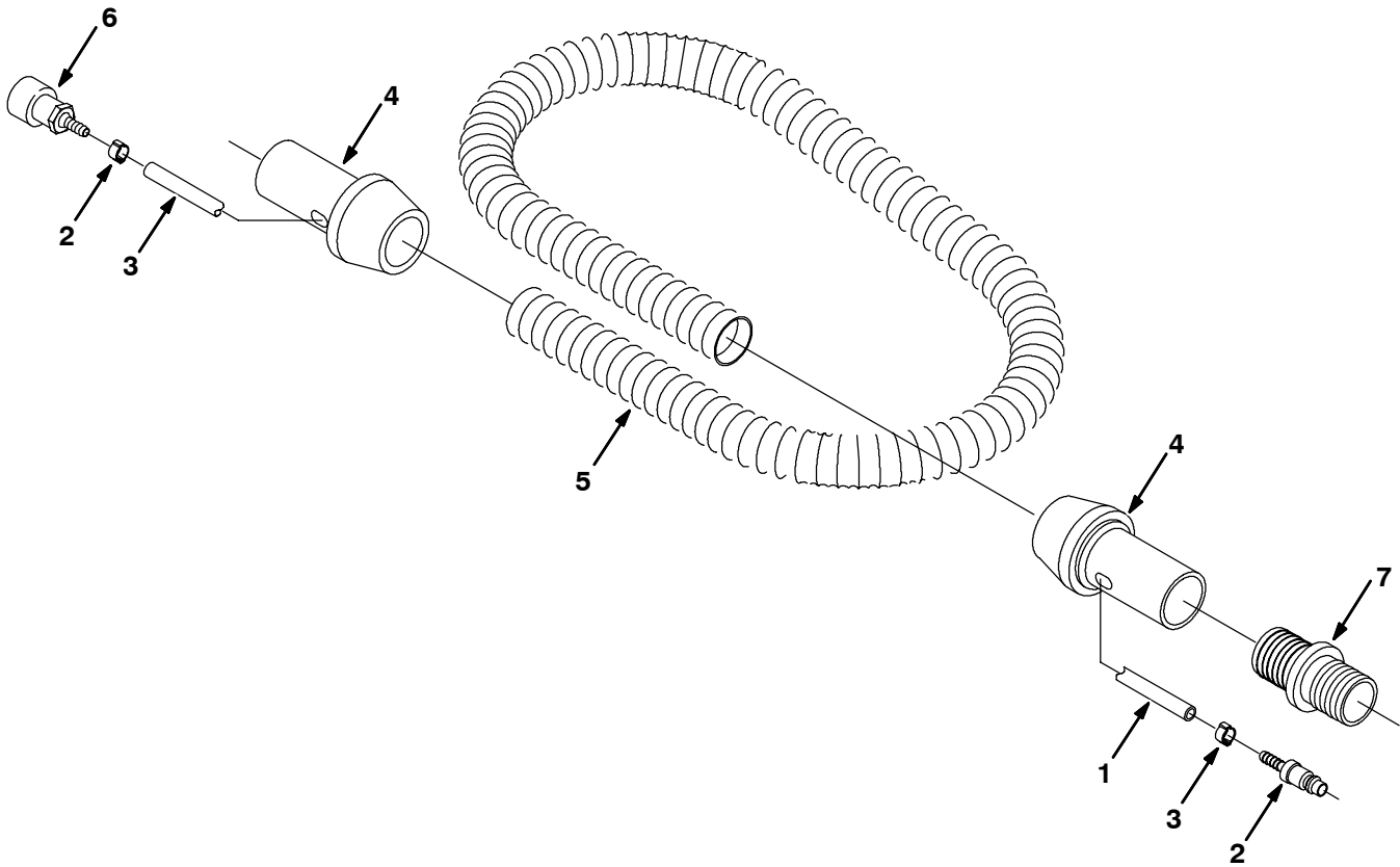
Fig. 43 - Power Wand Hose Assembly
