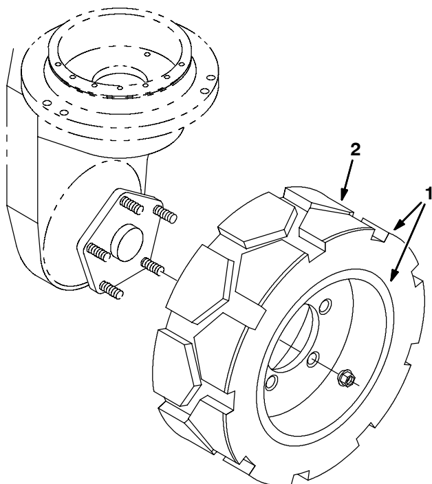
Fig. 64 - Tire, Non-Mark, Non-Skid, Front Drive
