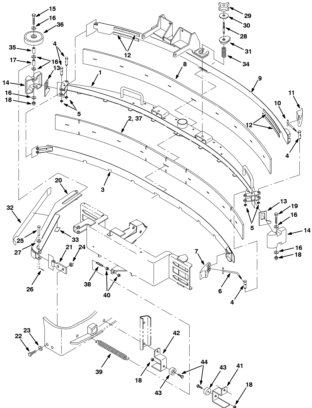
Fig. 48 - Max Pro 1200 Rear Squeegee Group
