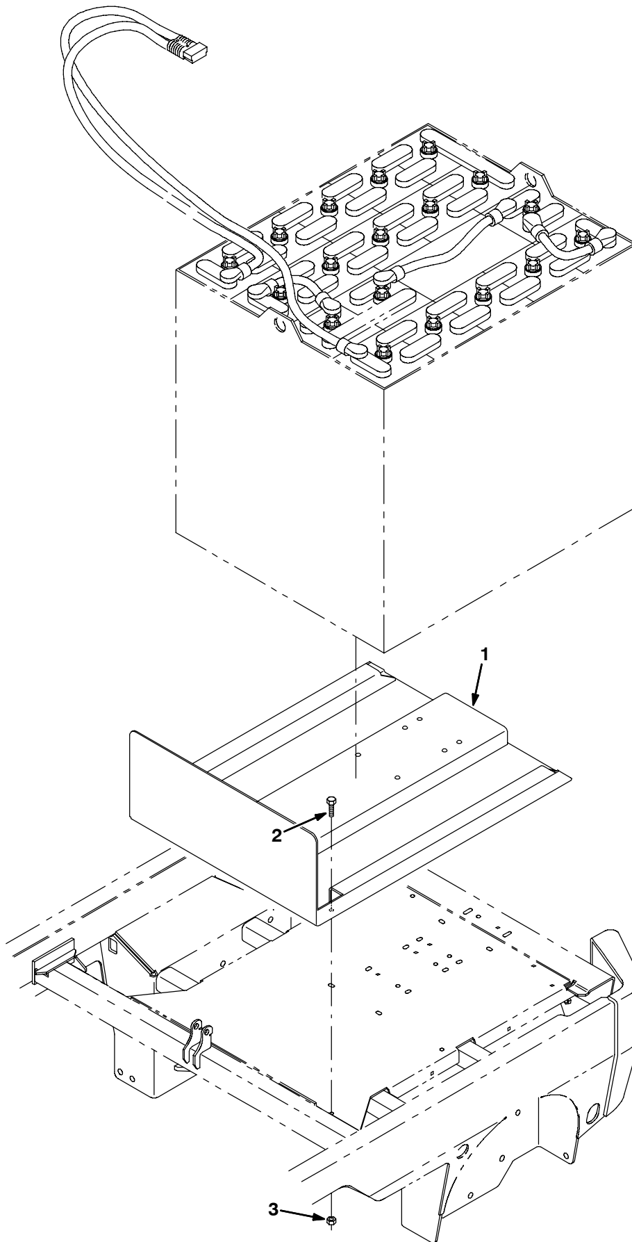
Fig. 53 - Battery Forklift Kit
