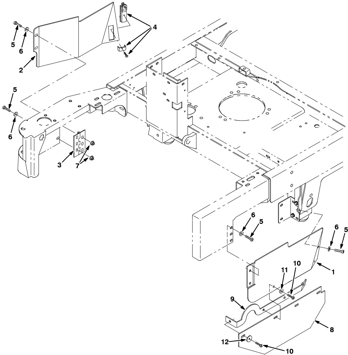
Fig. 33 - Sweeper Main Brush Doors Group
