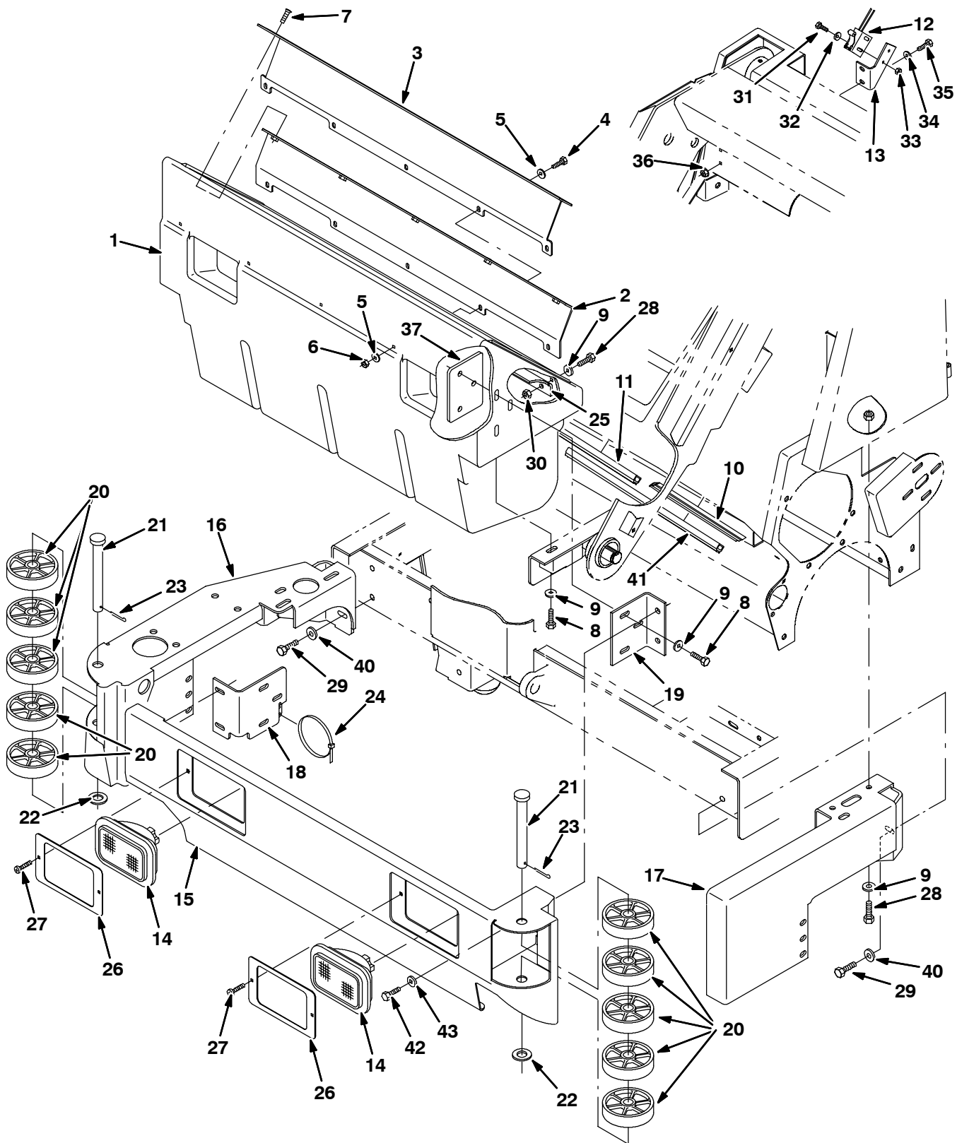
Fig. 39 - Hopper and Bumper Group
