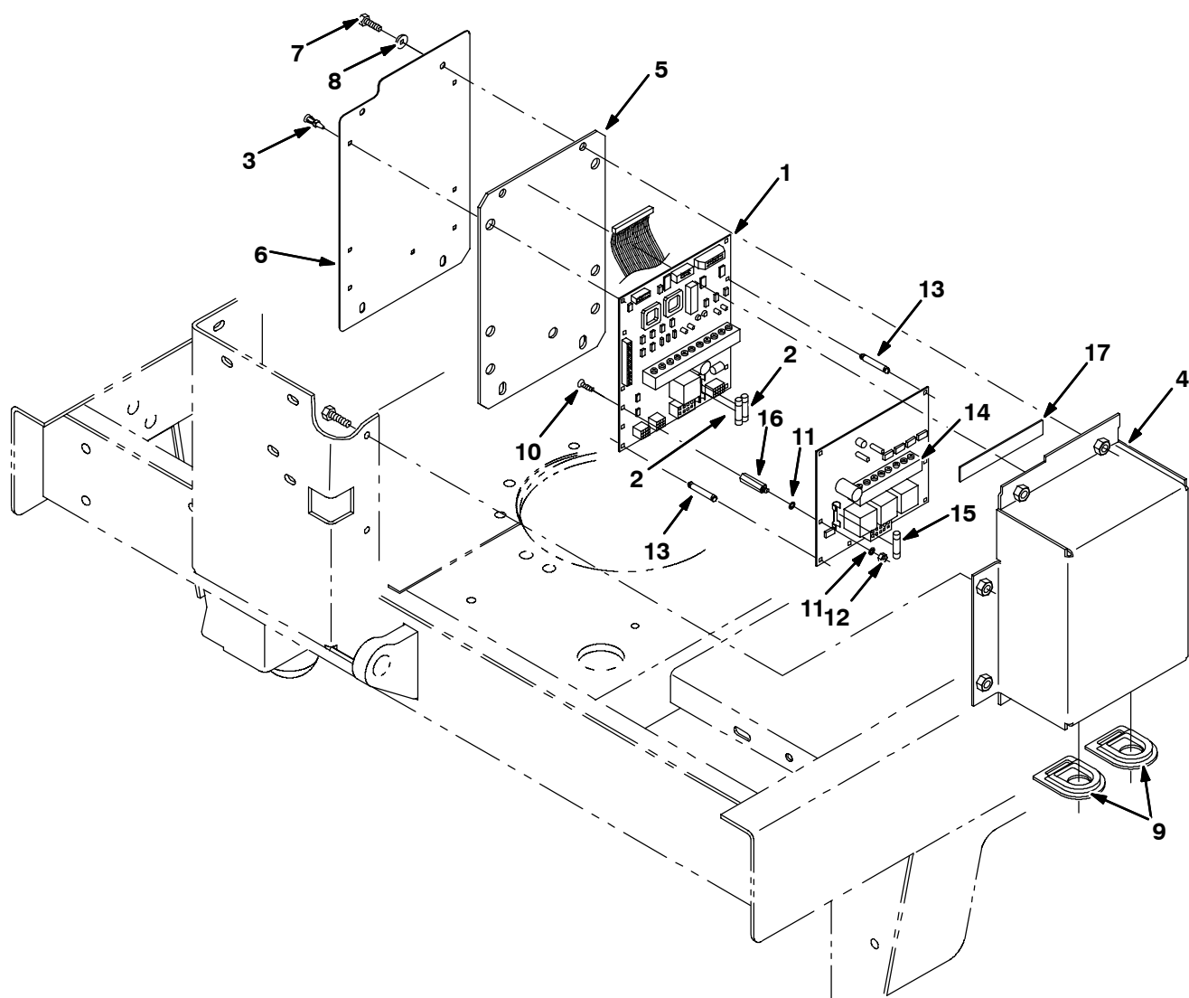
Fig. 53 - Electrical Circuit Board Group
