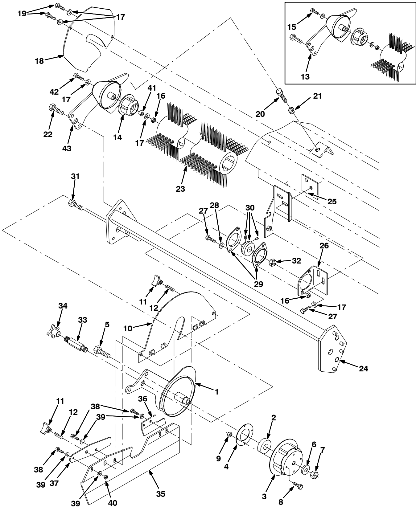
Fig. 37 - Sweeper Main Brush Idler Group
