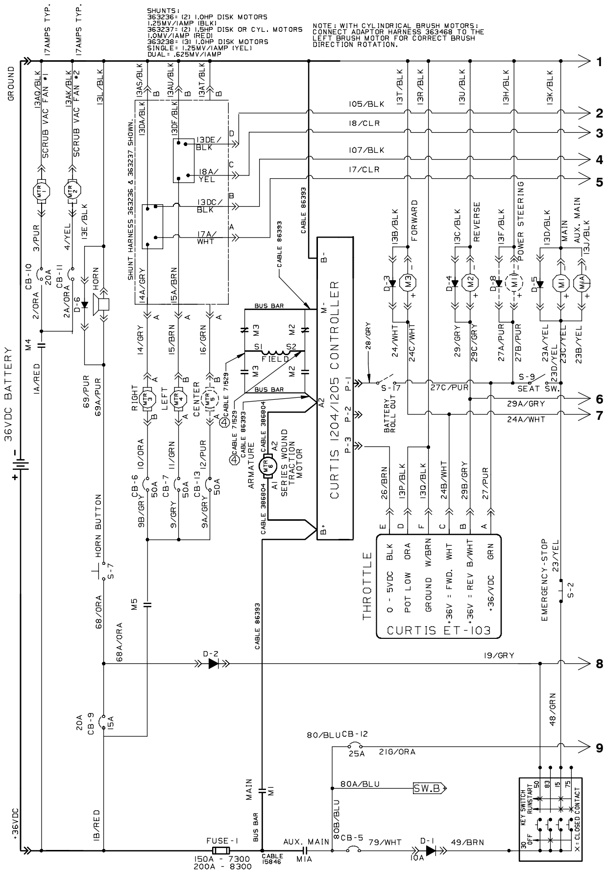
Fig. 55 - Electrical Schematic
