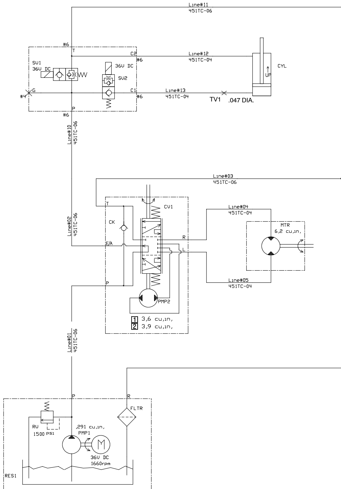
Fig. 46 - Hydraulic Schematic
