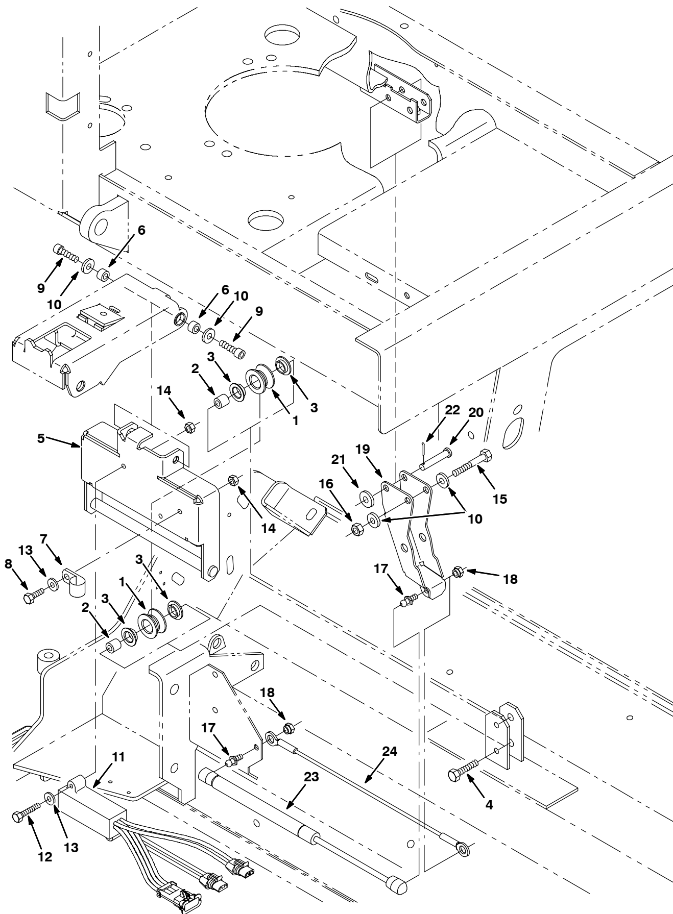
Fig. 31 - Max Pro 1200 (Cylindrical Brush) Edge Scrub Group
