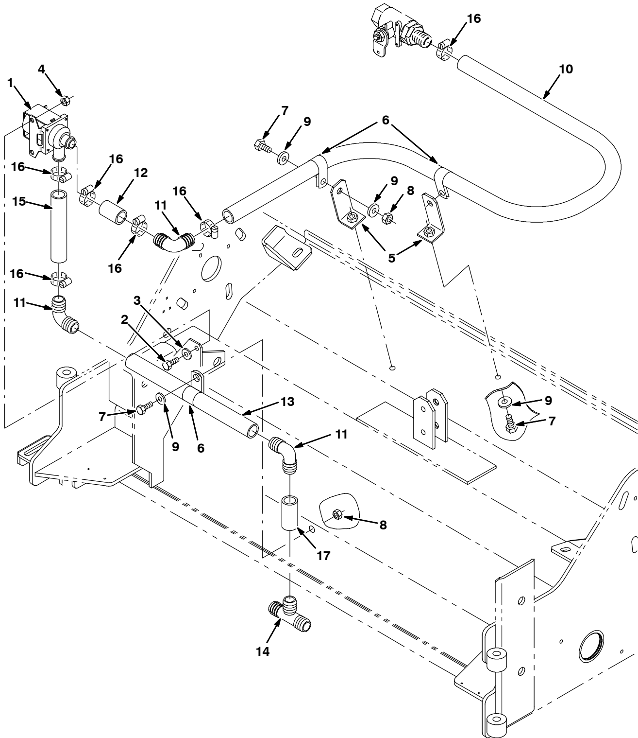
Fig. 20 - Max Pro 1000 (Cylindrical Brush) Solution Valve Group (Non FaST)
