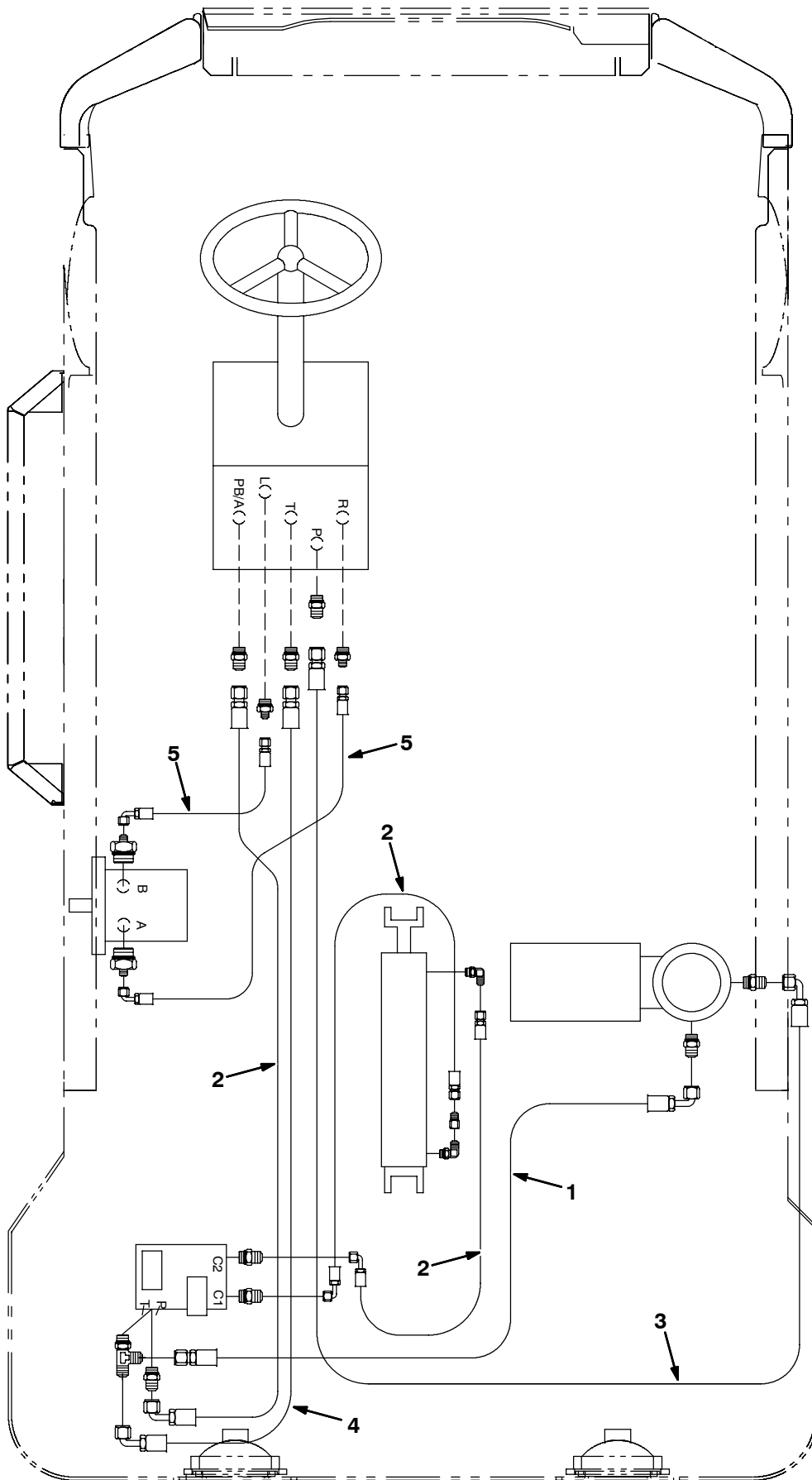
Fig. 47 - Hydraulic Hose Group
