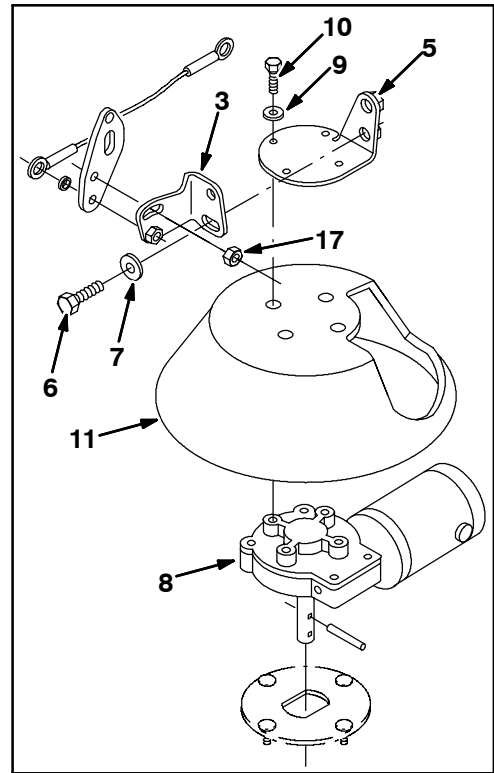
Fig. 34 - Sweeper Side Brush Motor and Pivot Group
