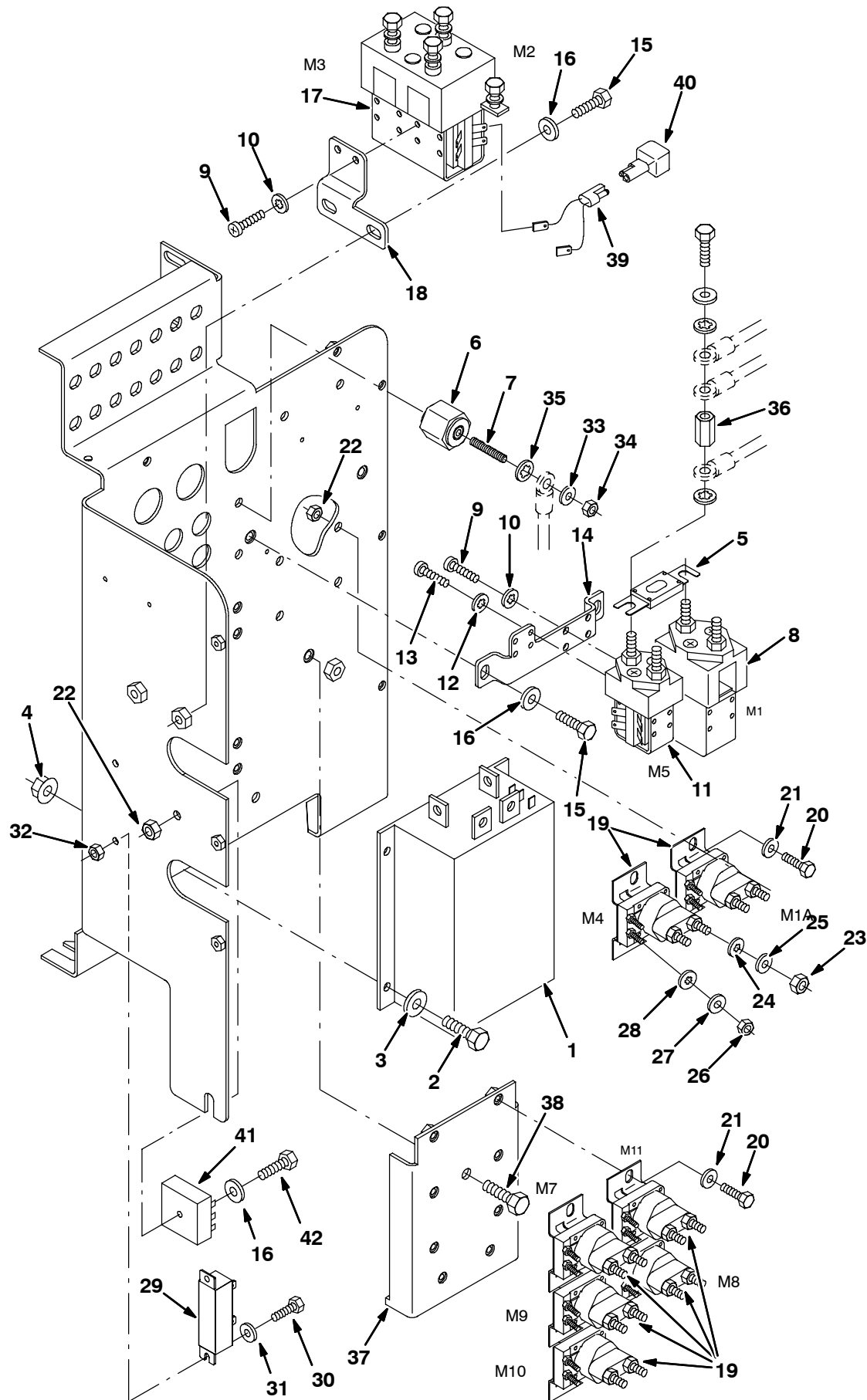
Fig. 50 - Electrical Control Box Contactor Group (003546- )
