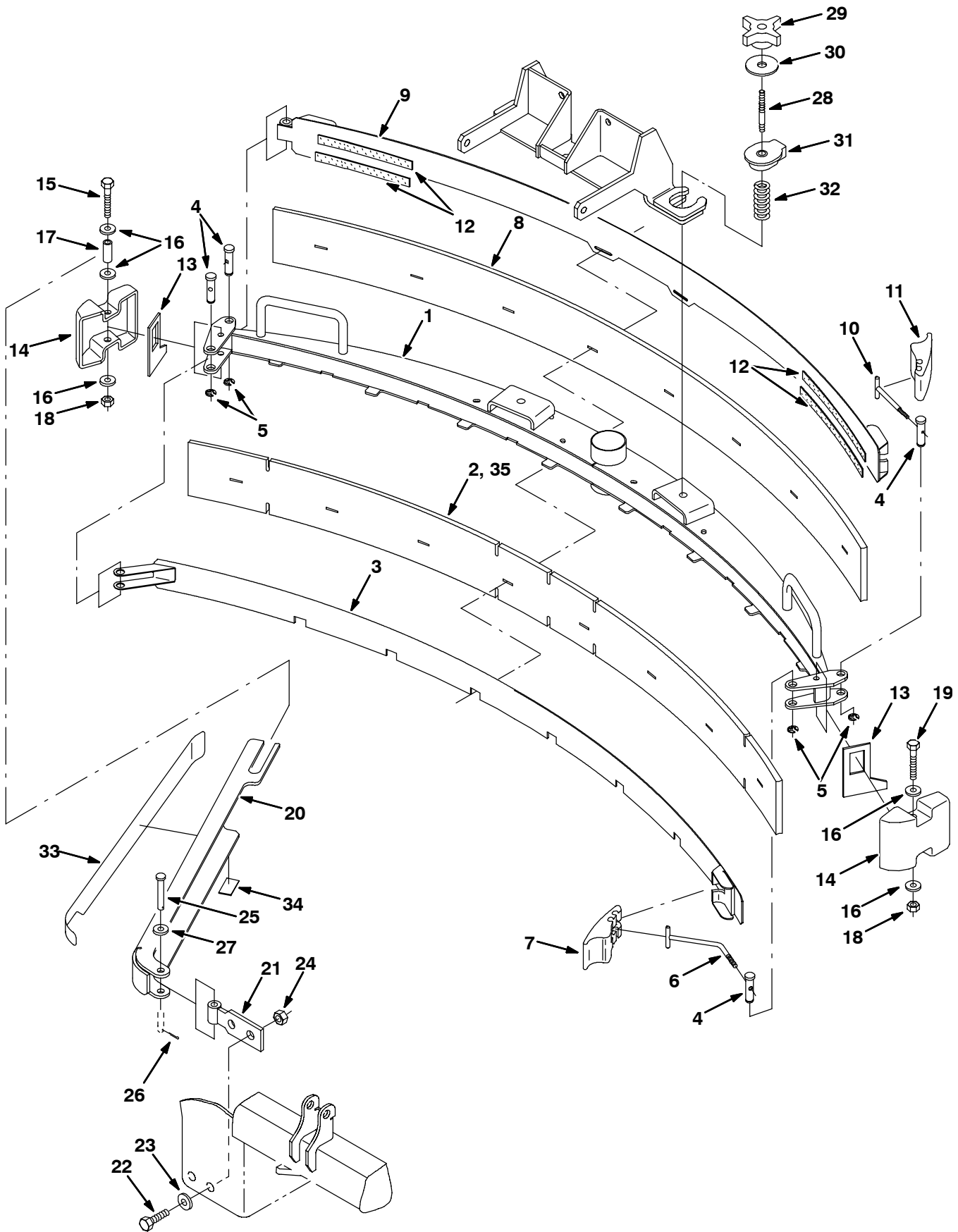
Fig. 49 - Max Pro 1200 Rear Squeegee Group (For Vacuumized Side Squeegee)
