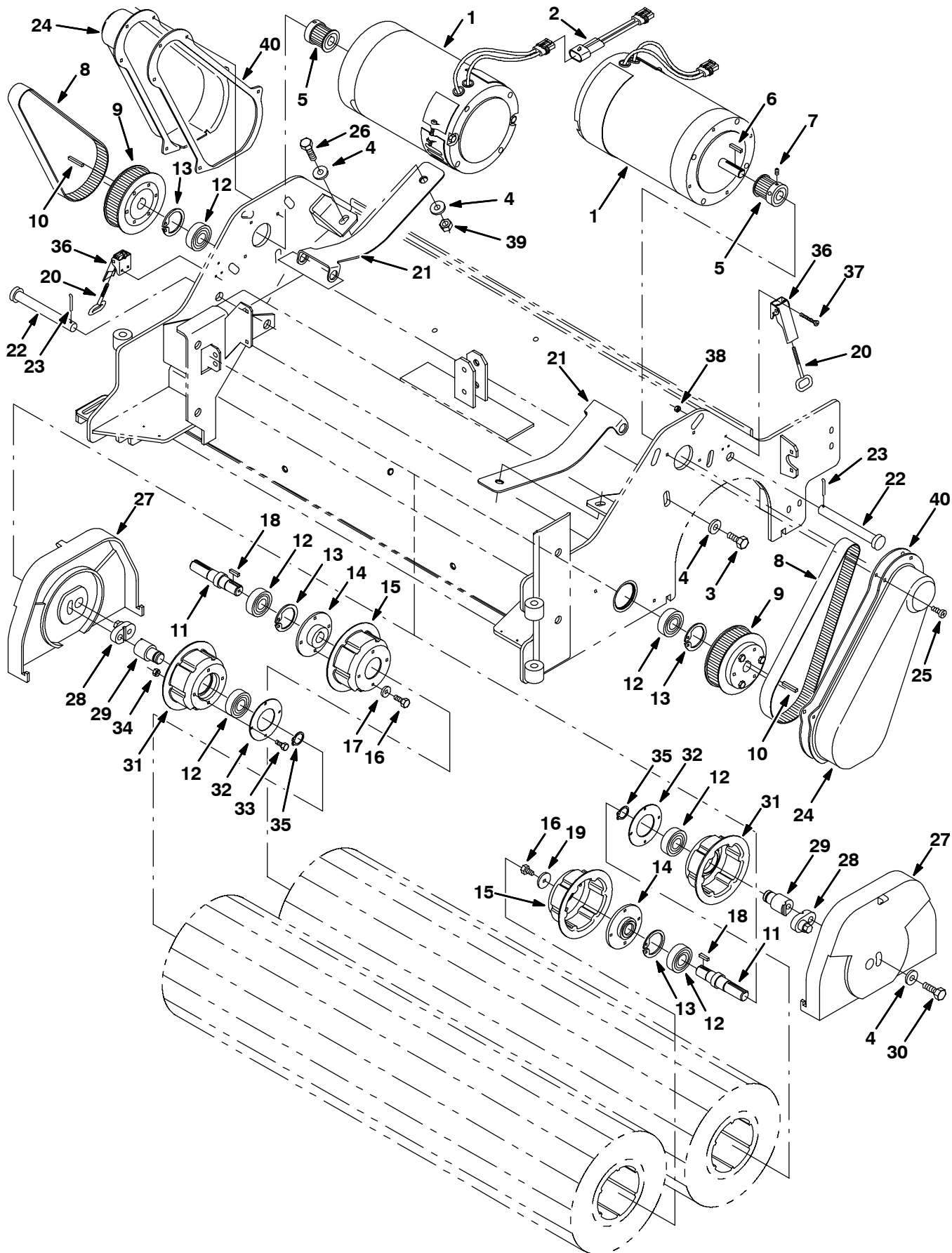
Fig. 19 - Max Pro 1000 (Cylindrical Brush) Scrub Head Drive Group
