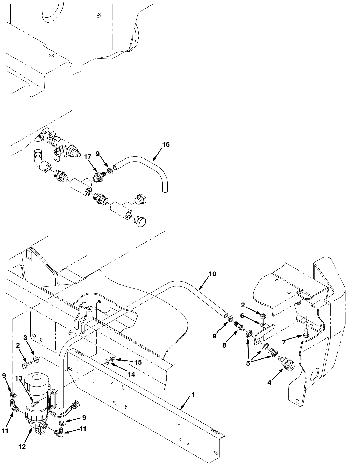
Fig. 45 - Power Wand Pump and Fittings Group
