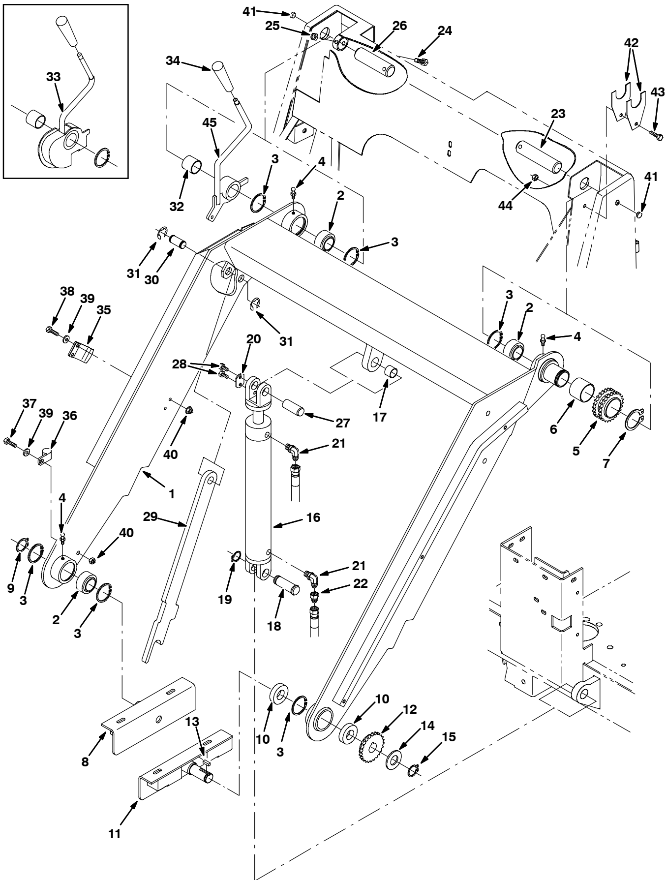
Fig. 41 - Hopper Lift Arms Group
