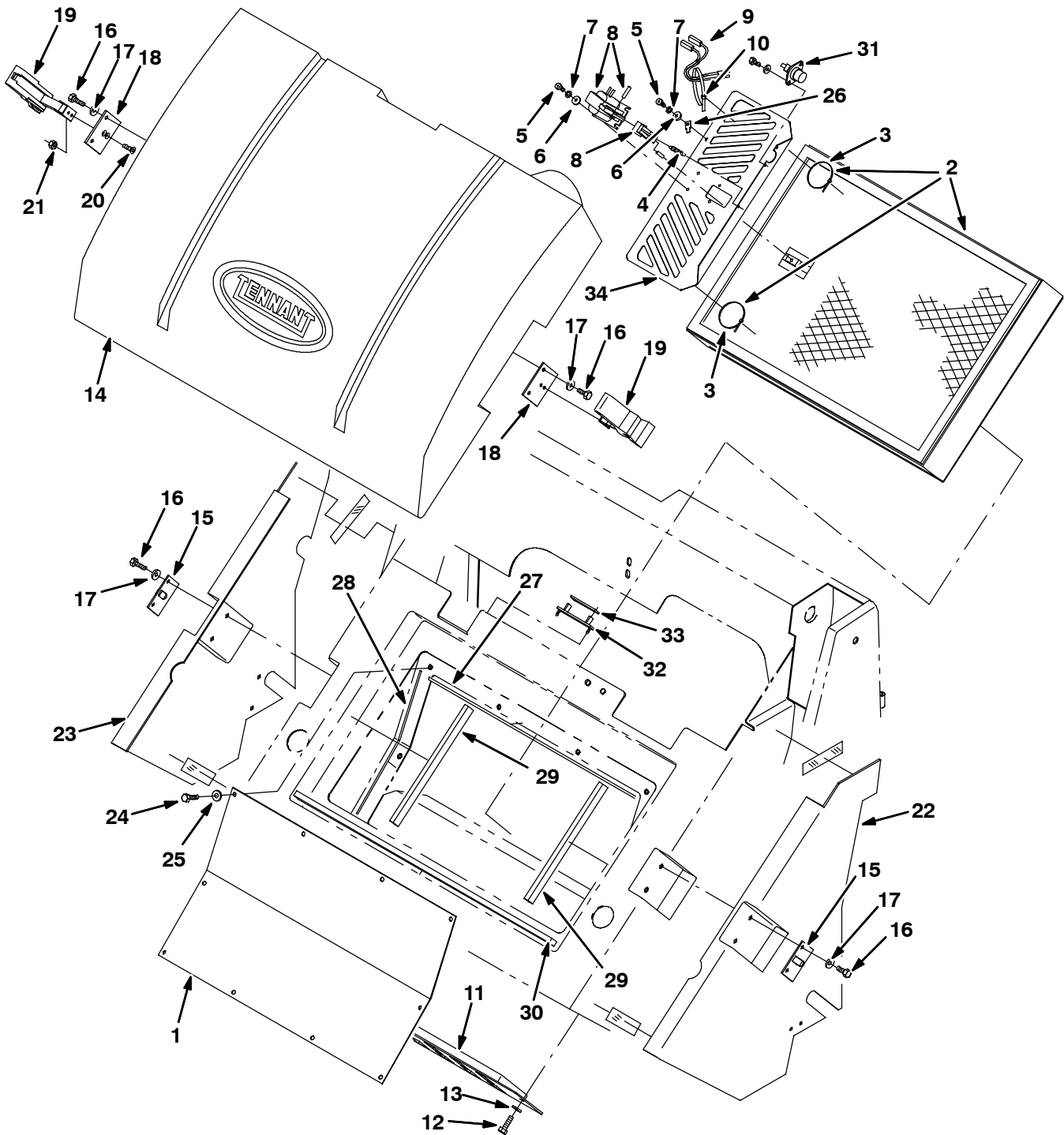
Fig. 43 - Hopper Filter Box Group
