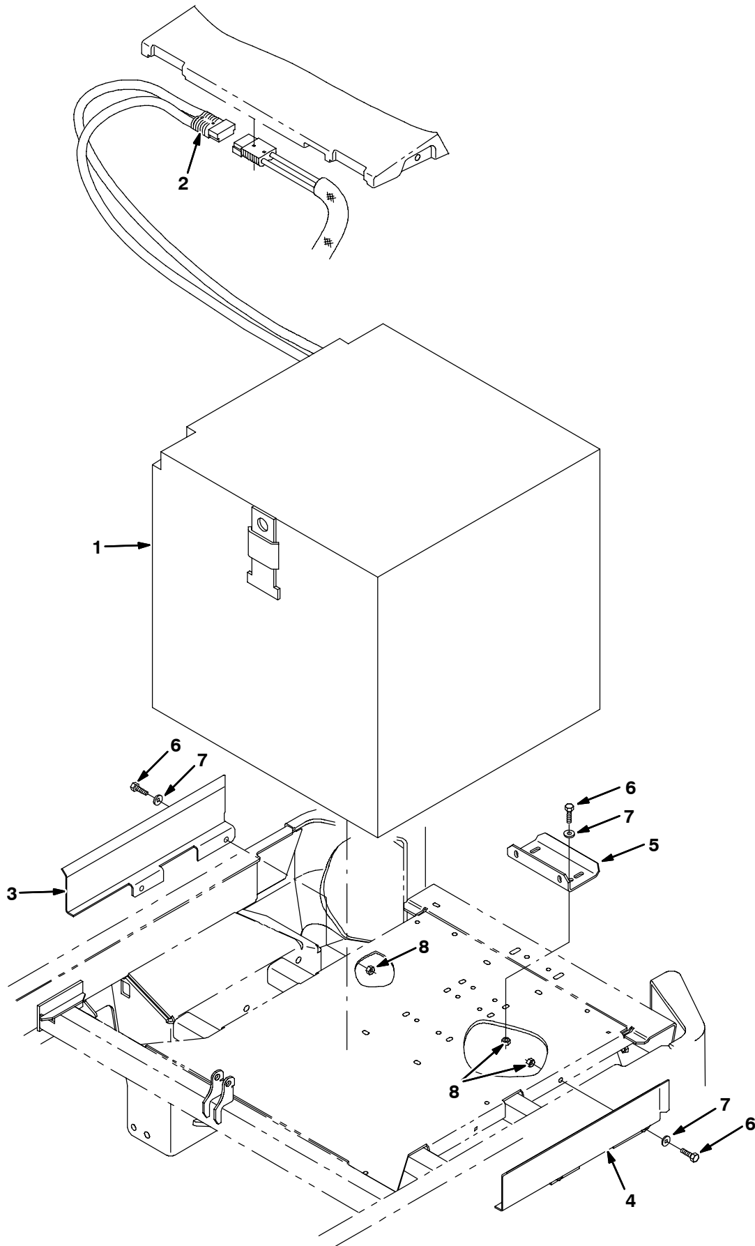
Fig. 55 - Battery Kit, 600AH
