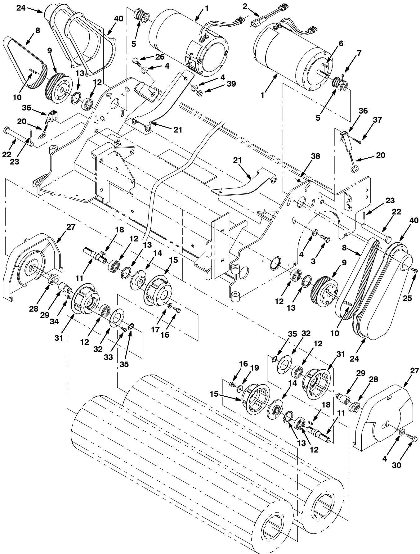
Fig. 28 - Max Pro 1200 (Cylindrical Brush) Scrub Head Drive Group
