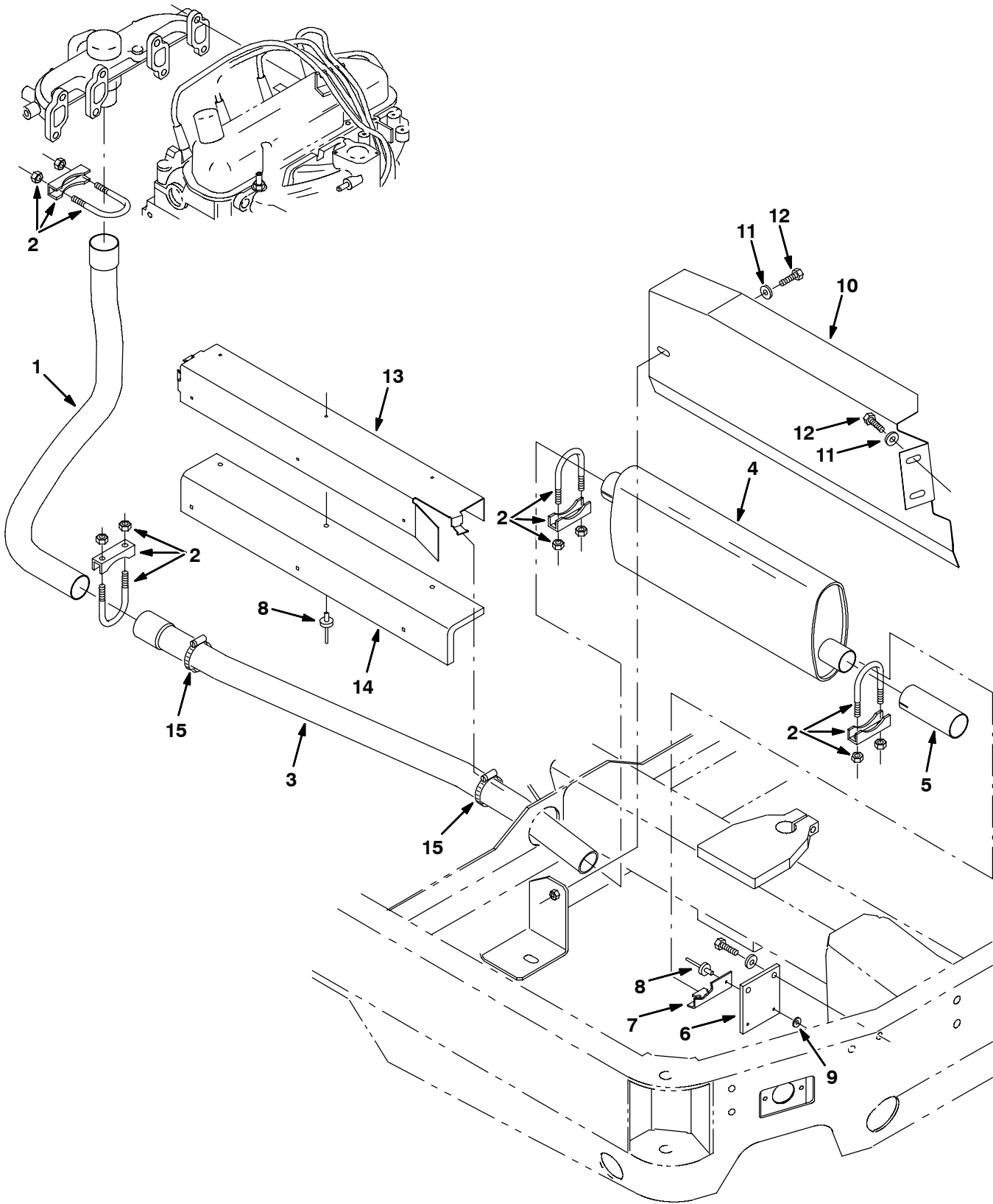
Fig. 32 - Engine Muffler Group (000000-009999)
