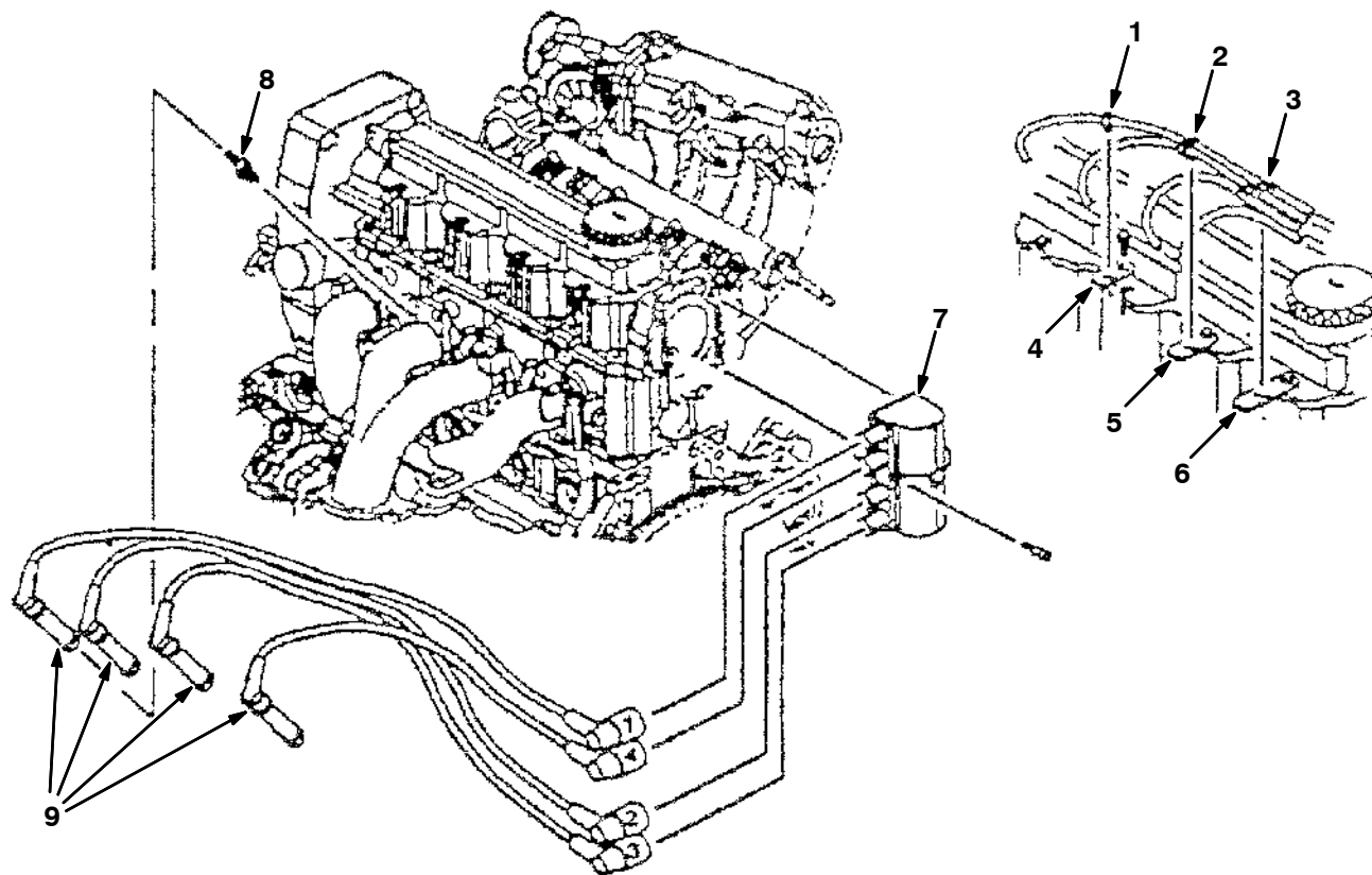
Fig. 4 - Ignition Group
