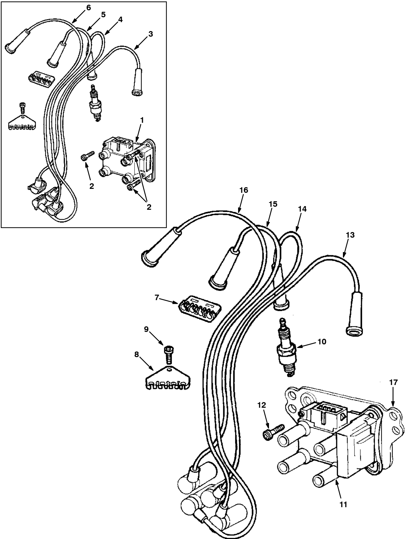
Fig. 10 - Distributorless Ignition Group
