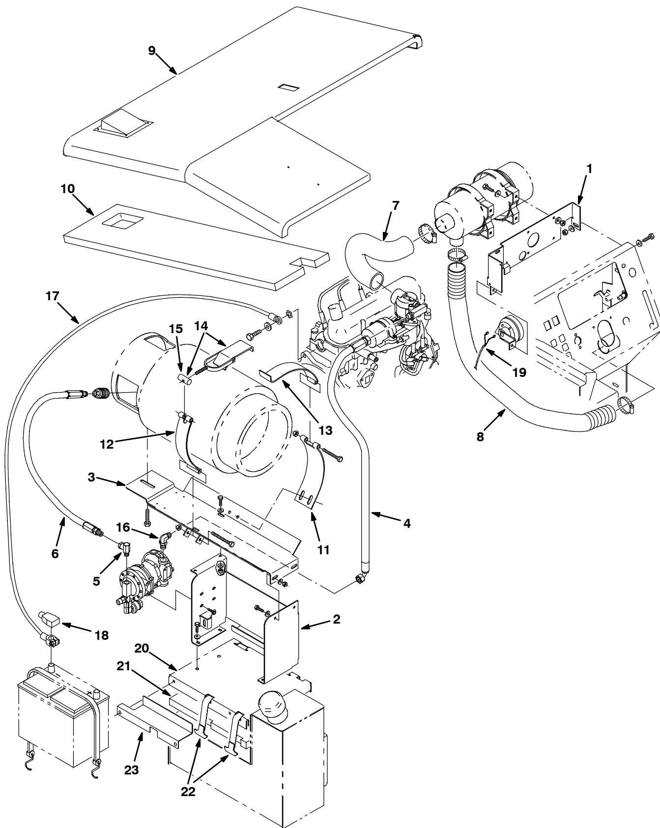
Fig. 26 - Fuel Tank and Engine Cover Group, Horizontal LPG (000000-001139)
