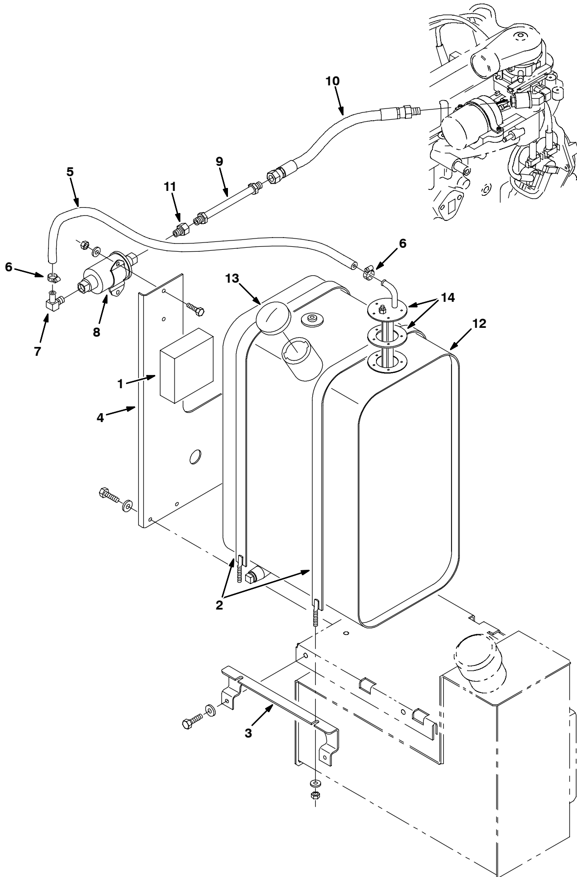
Fig. 22 - Engine Fuel Tank Group, Gasoline (000000-009999)
