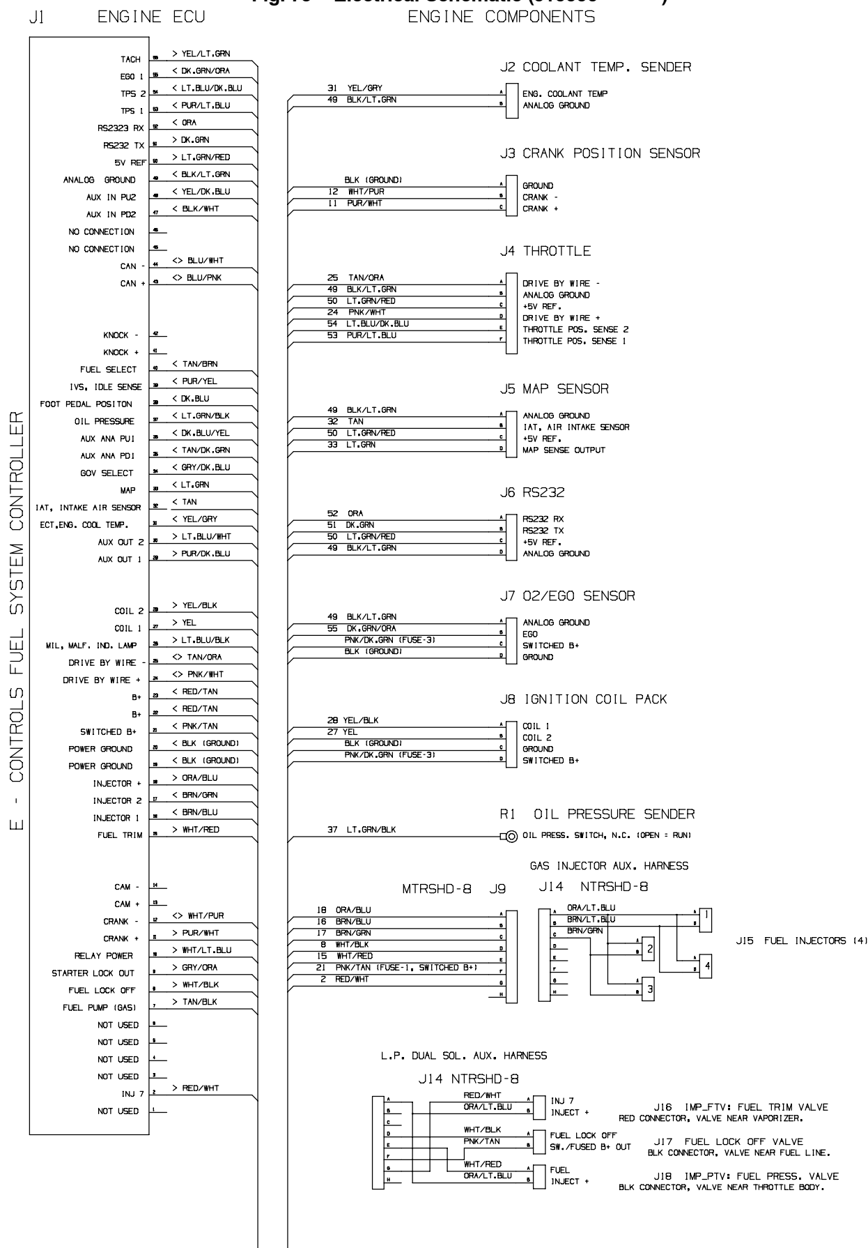
Fig. 79 - Electrical Schematic (010000- )
