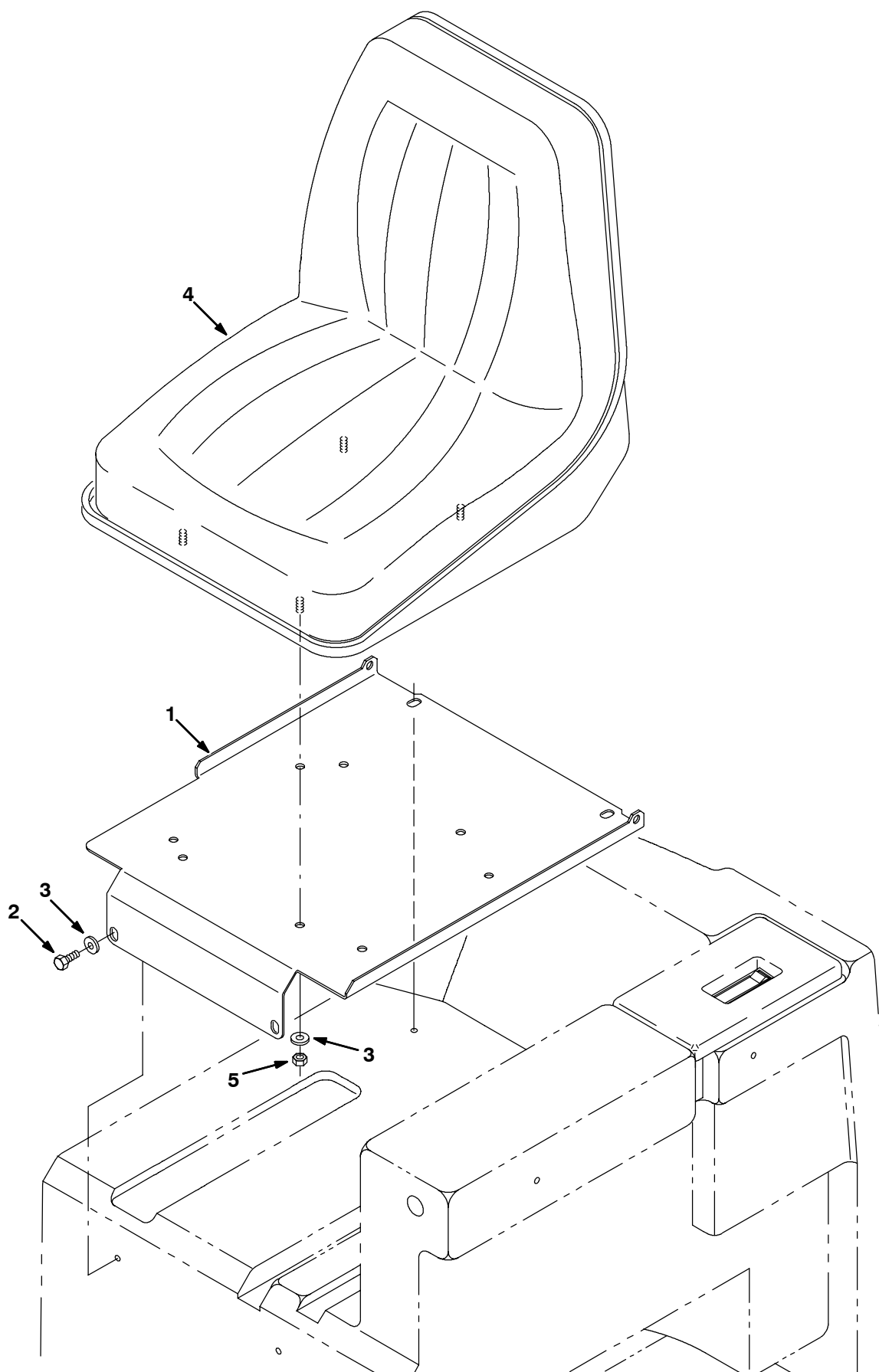
Fig. 9 - Seat Group
