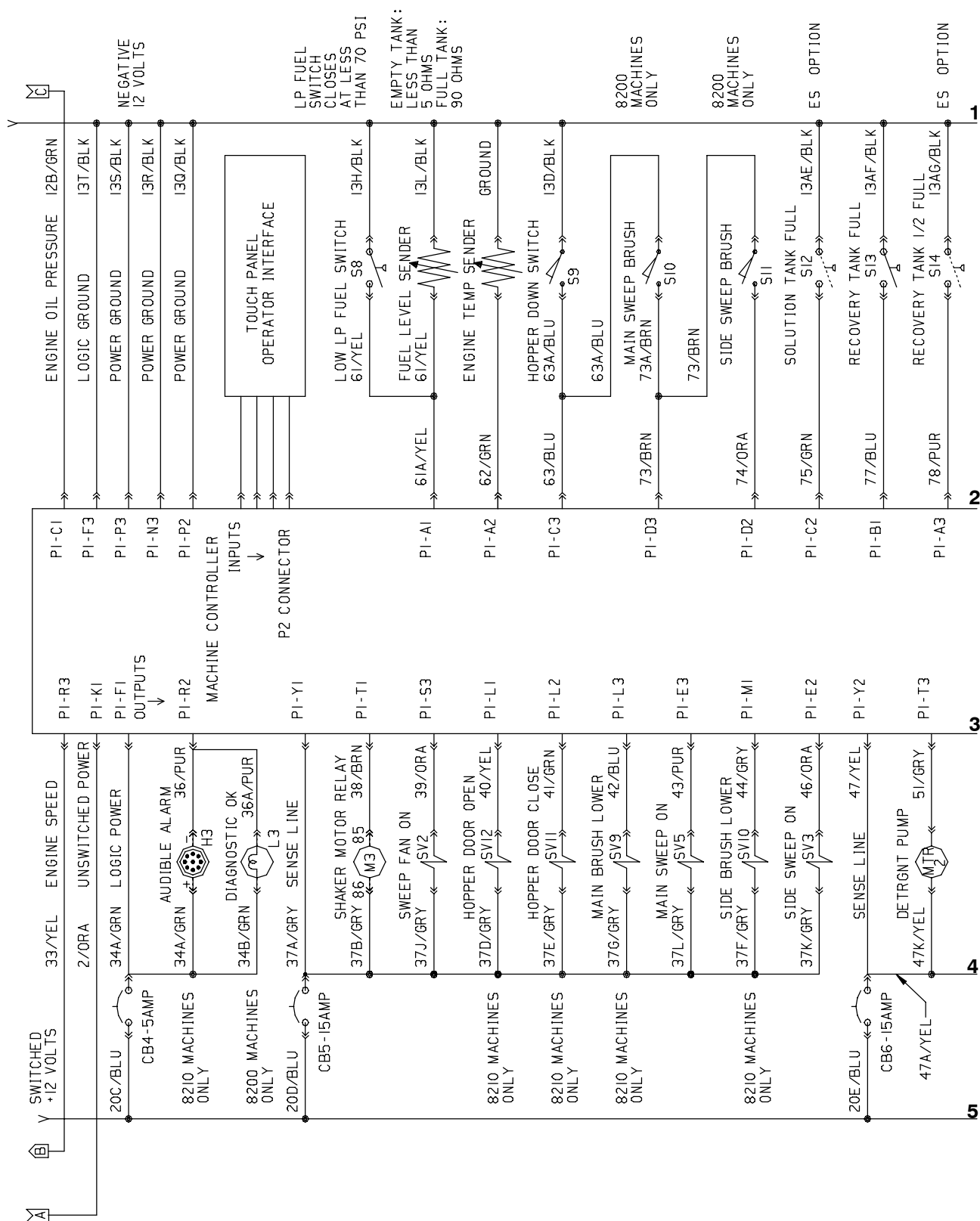
Fig. 78 - Electrical Schematic (000000-009999)
