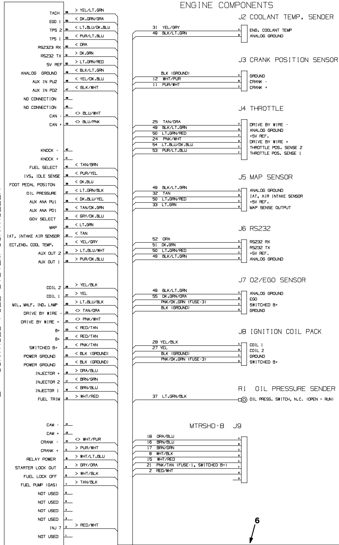
Fig. 80 - Electrical Wire Harness Group
