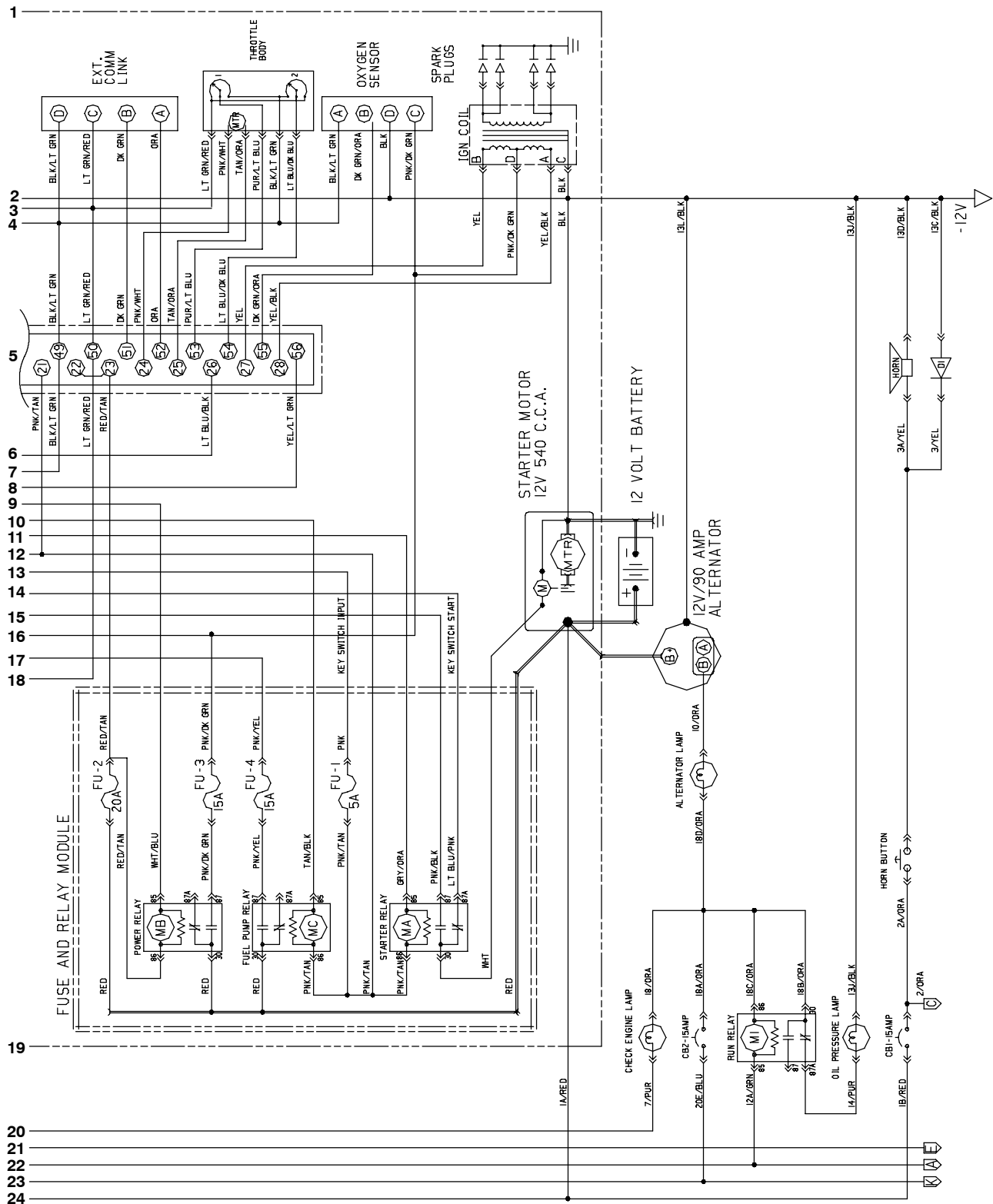
Fig. 79 - Electrical Schematic (010000- )
