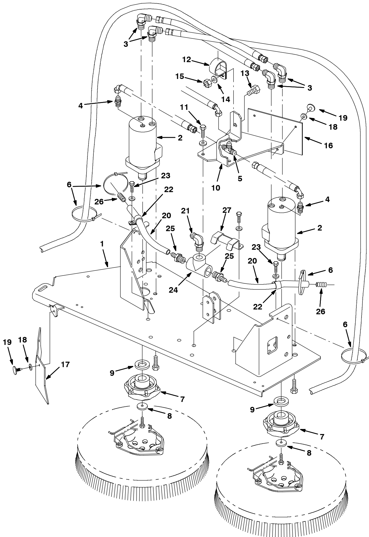
Fig. 52 - Scrub Head Group, Max Pro 1000 (Two-Brush)
