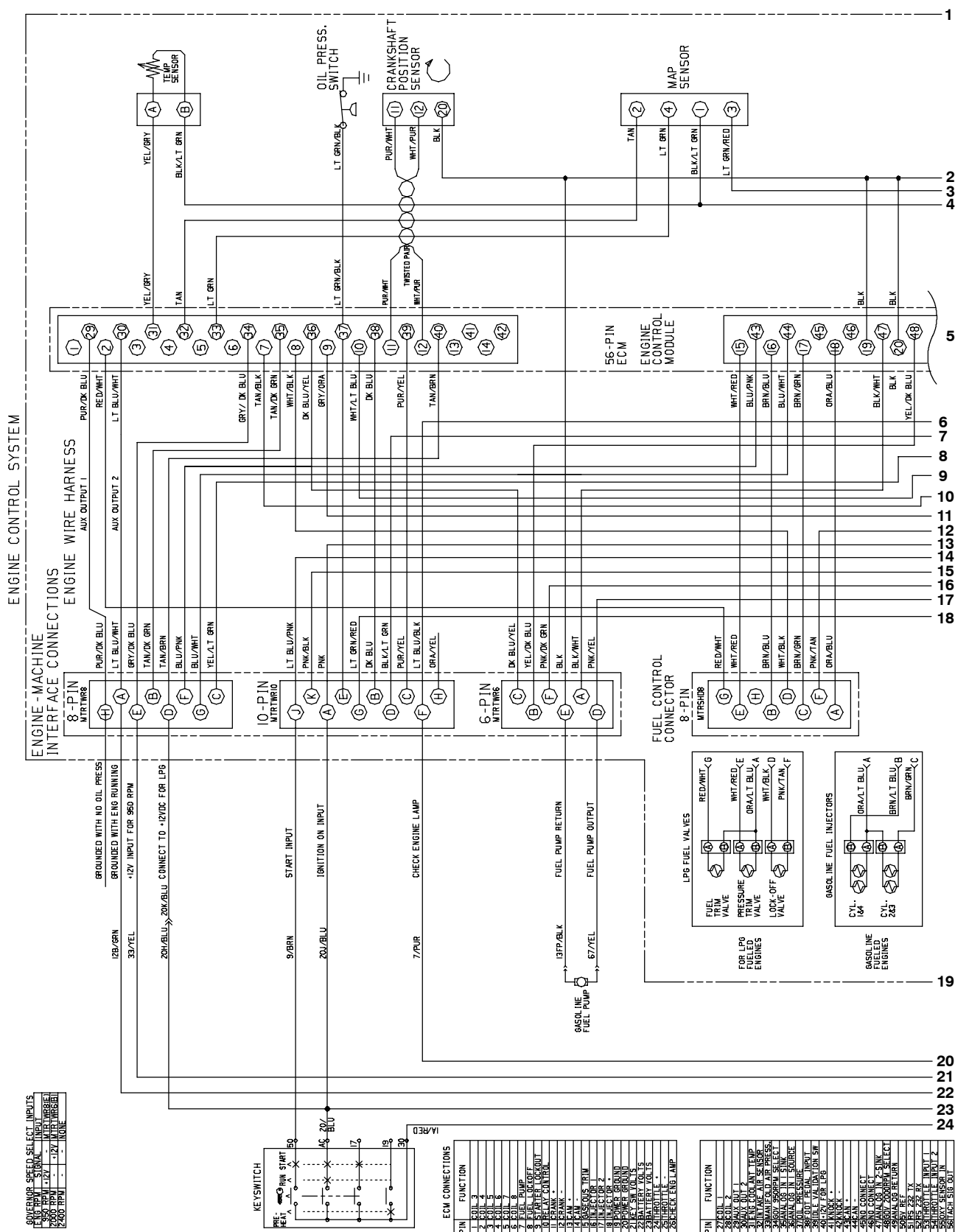
Fig. 79 - Electrical Schematic (010000- )
