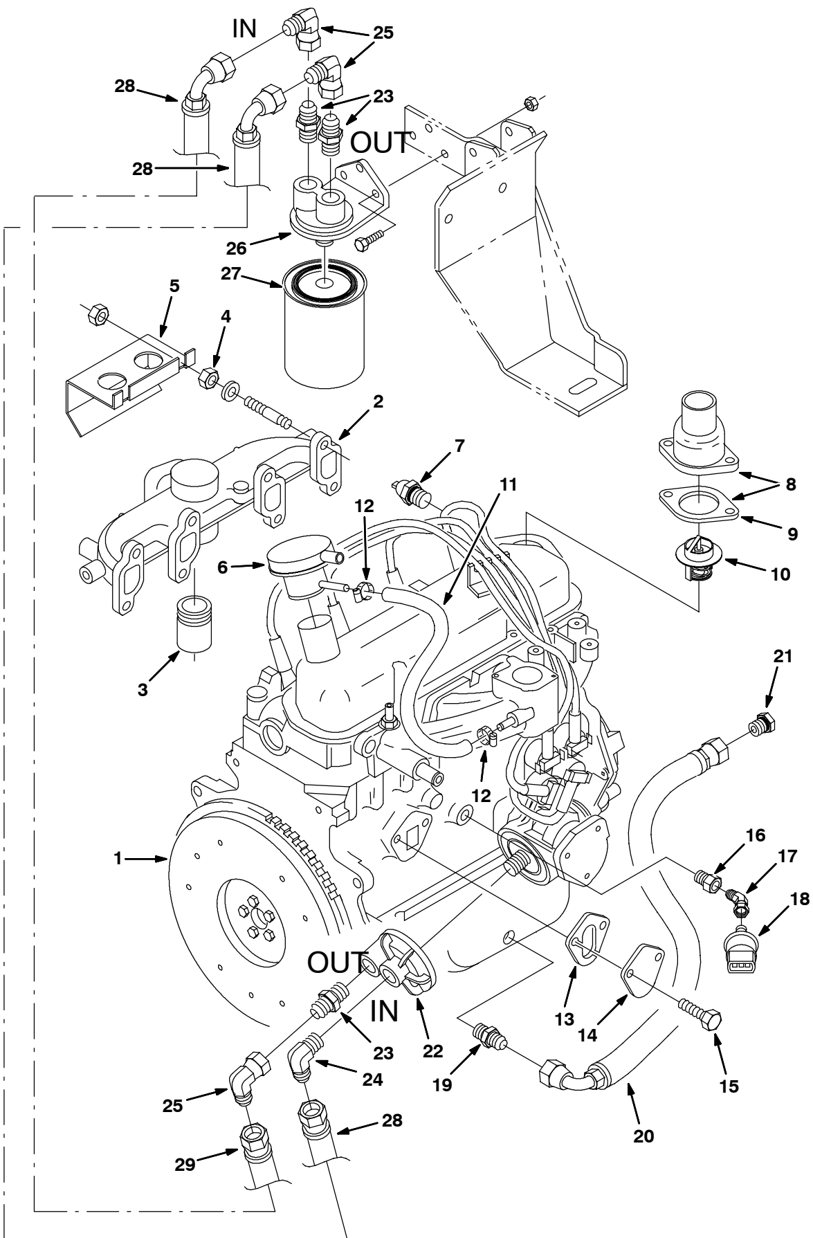
Fig. 14 - Engine Group, Gasoline & LPG (000000-009999)
