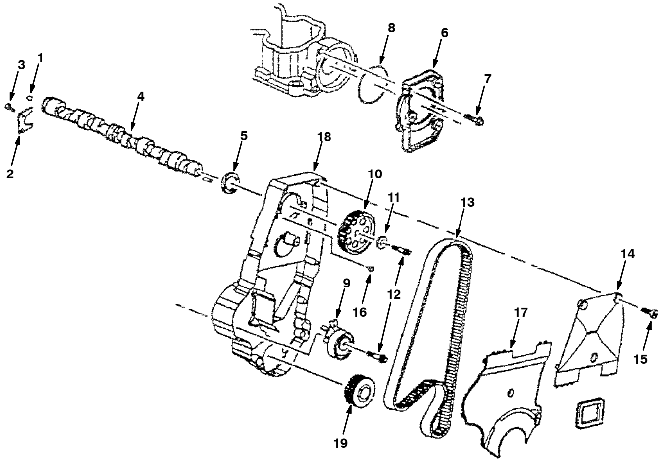
Fig. 3 - Camshaft Group
