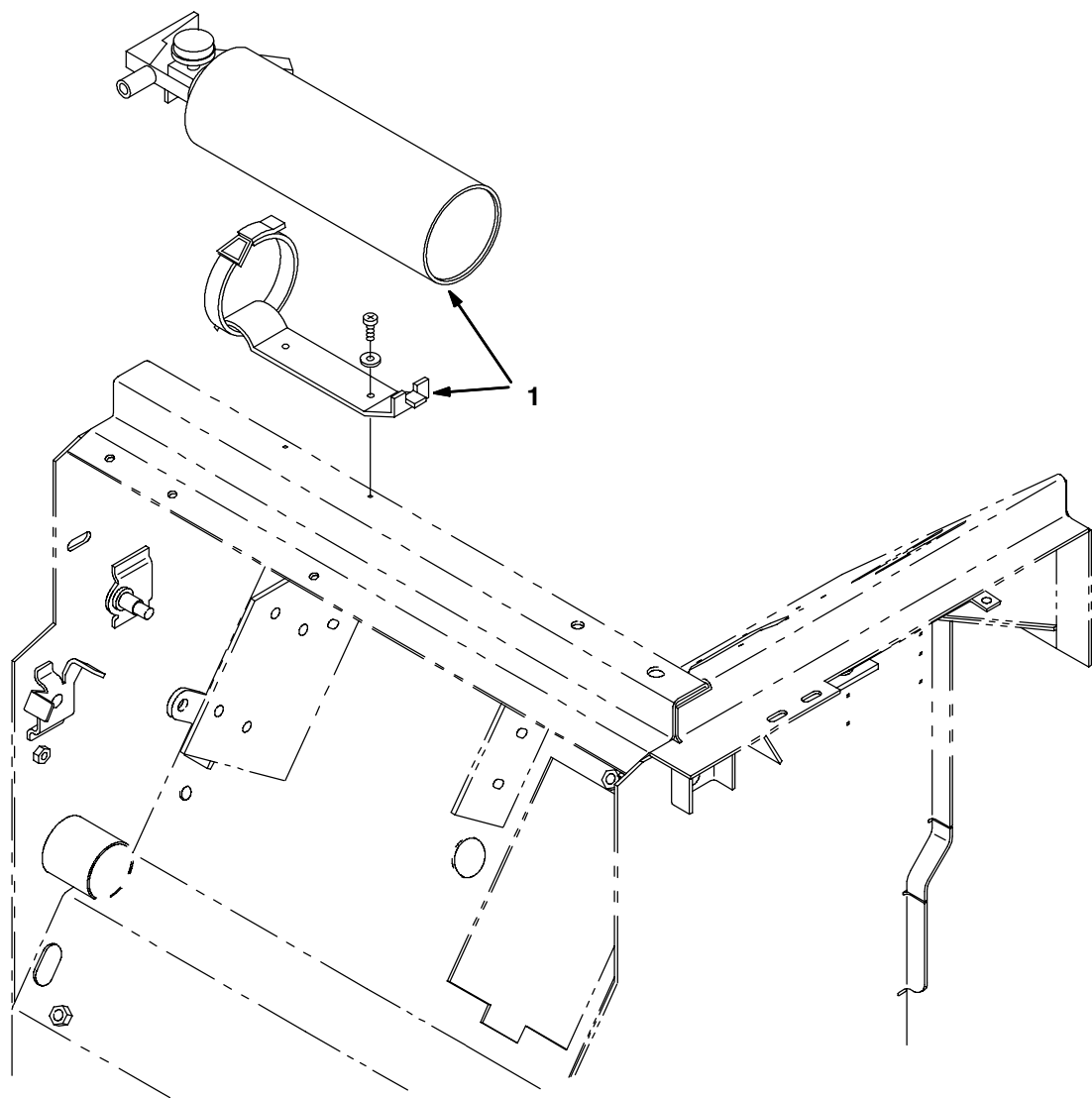
Fig. 34 - Fire Extinguisher Kit
