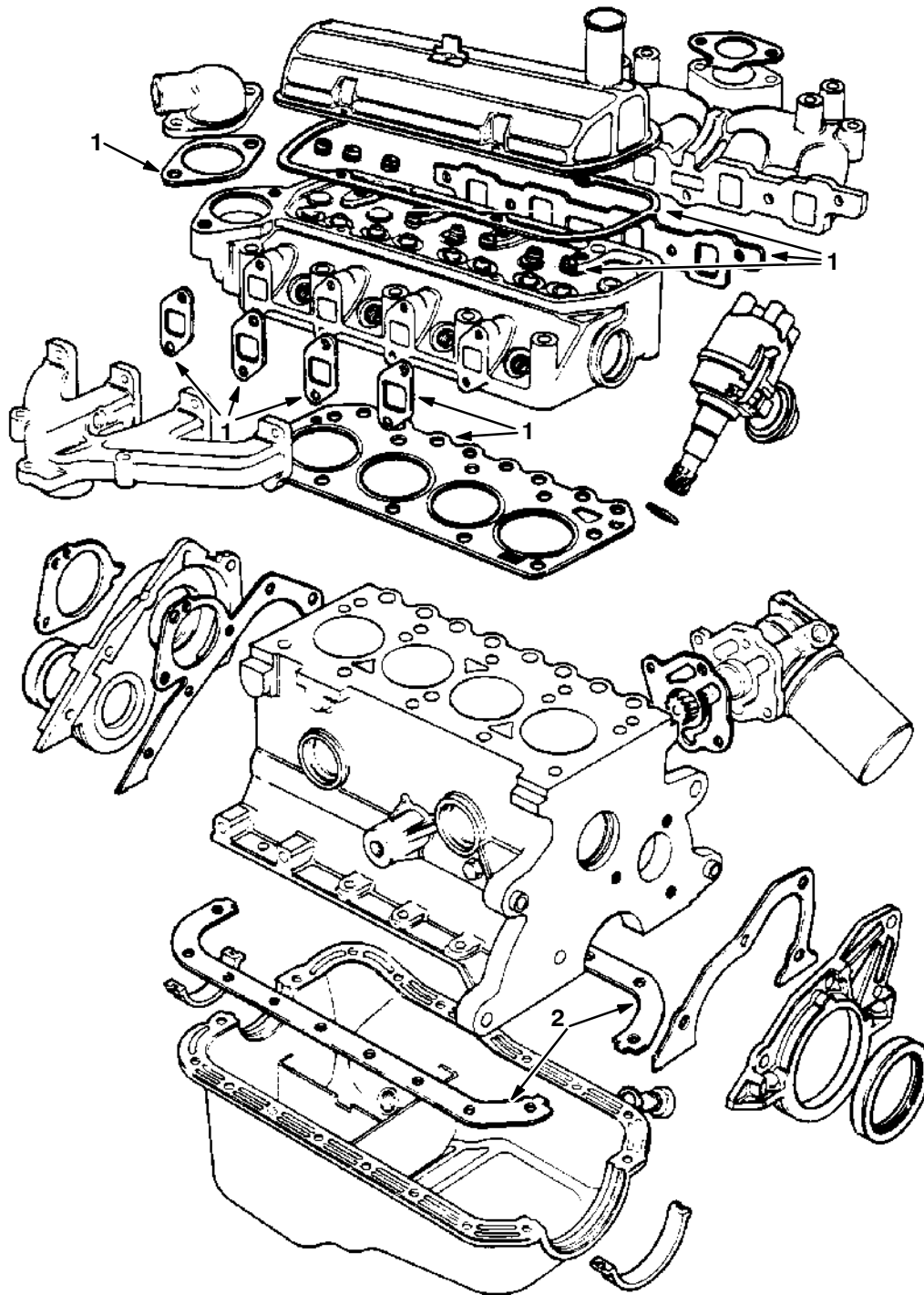
Fig. 9 - Gaskets Group
