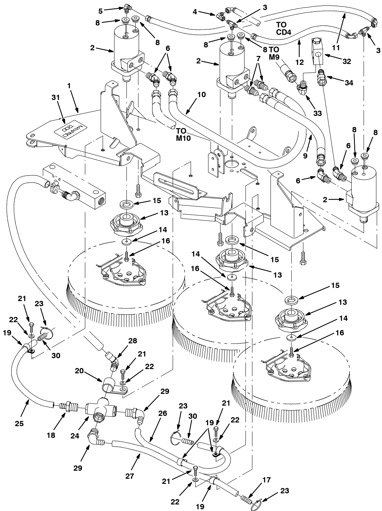
Fig. 16 - Scrub Head Group, Max Pro 1200 (Three-Brush)
