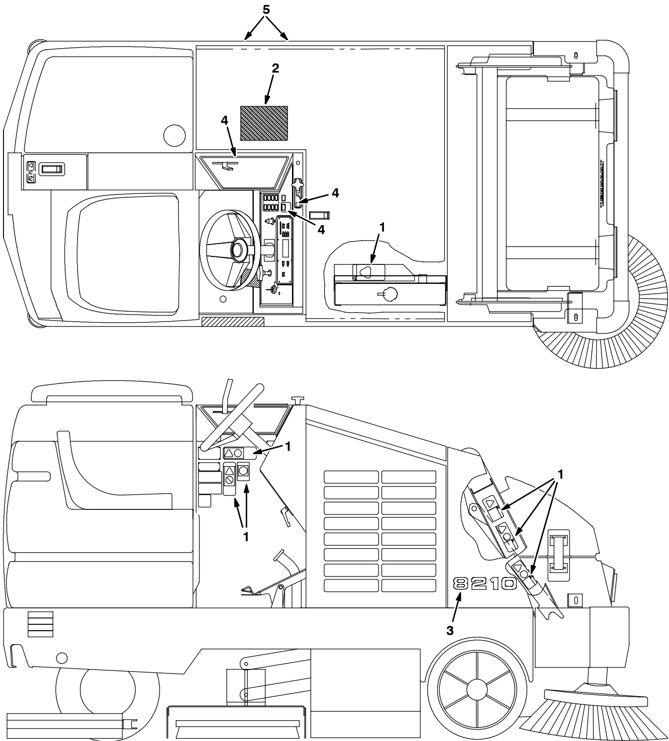
Fig. 81 - Label Group
