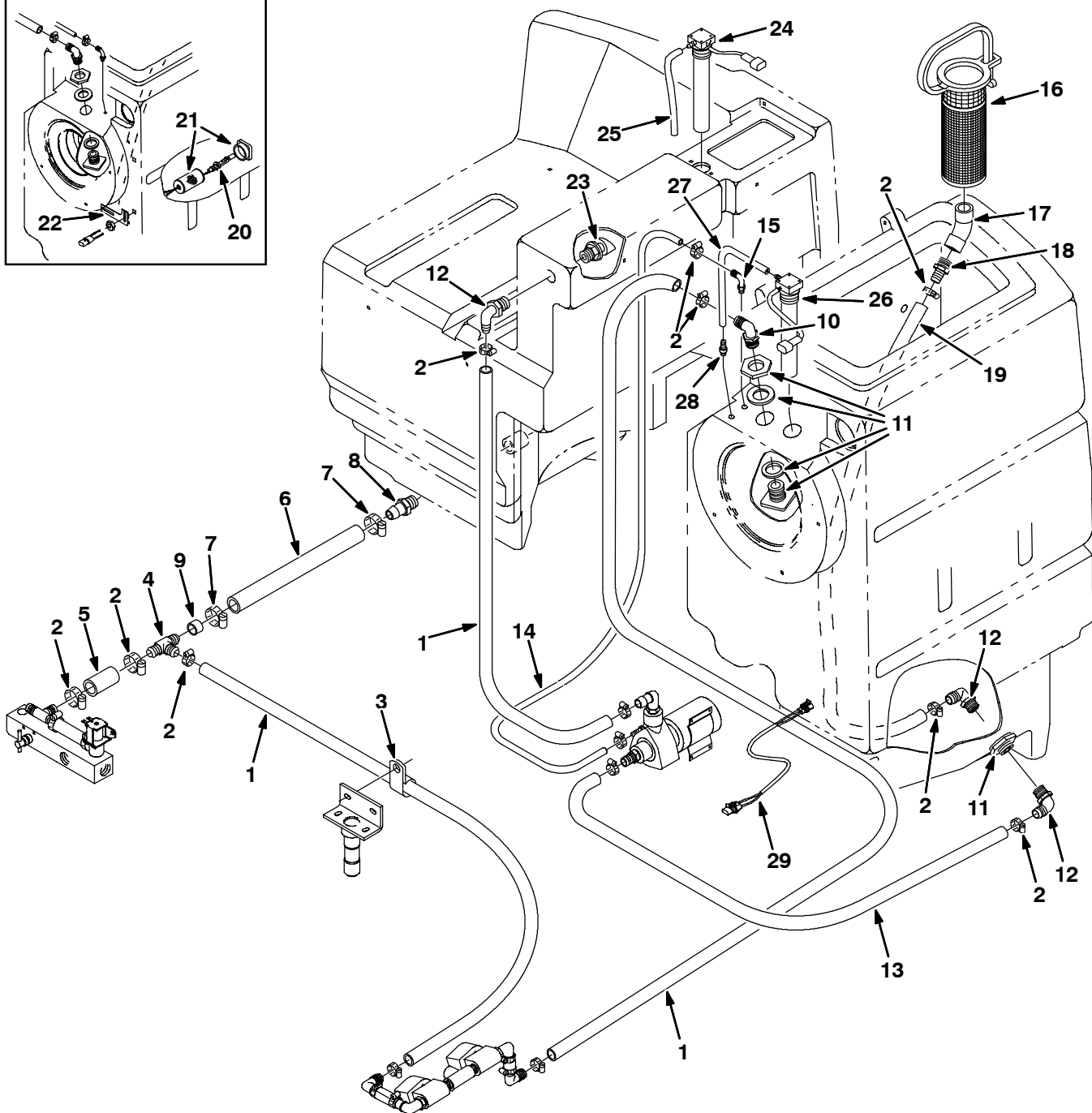
Fig. 6 - ES Tanks Group (010000- )
