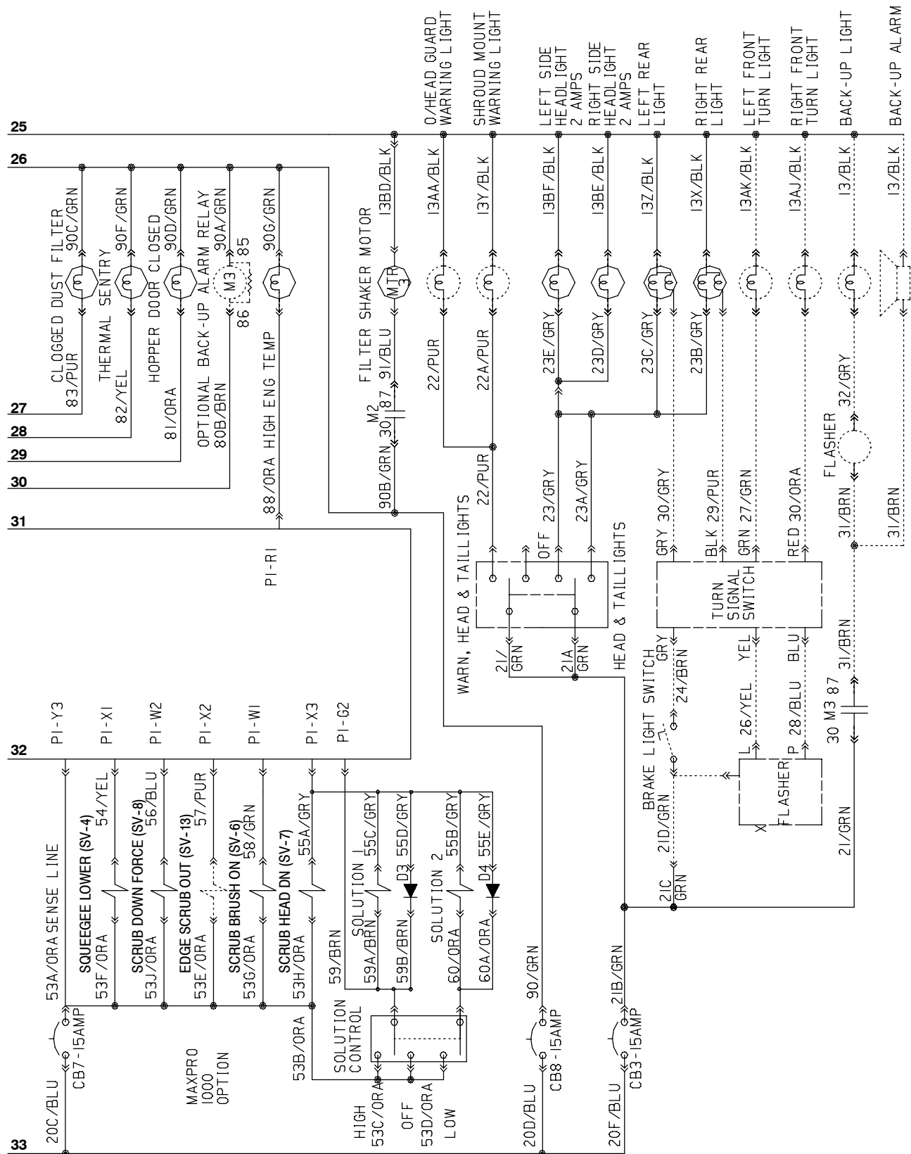
Fig. 79 - Electrical Schematic (010000- )
