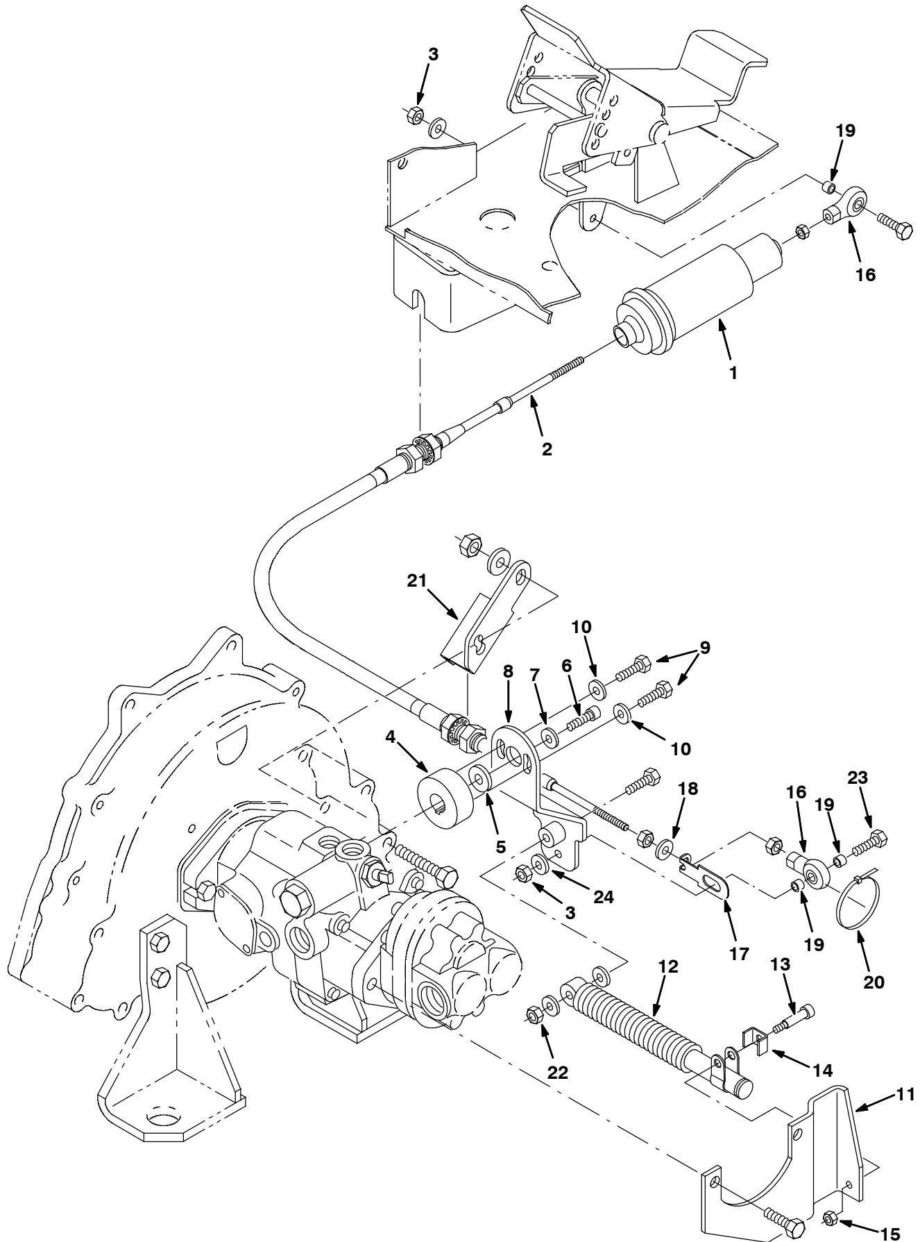
Fig. 68 - Hydraulic Pump Linkage Group (000000-009999)
