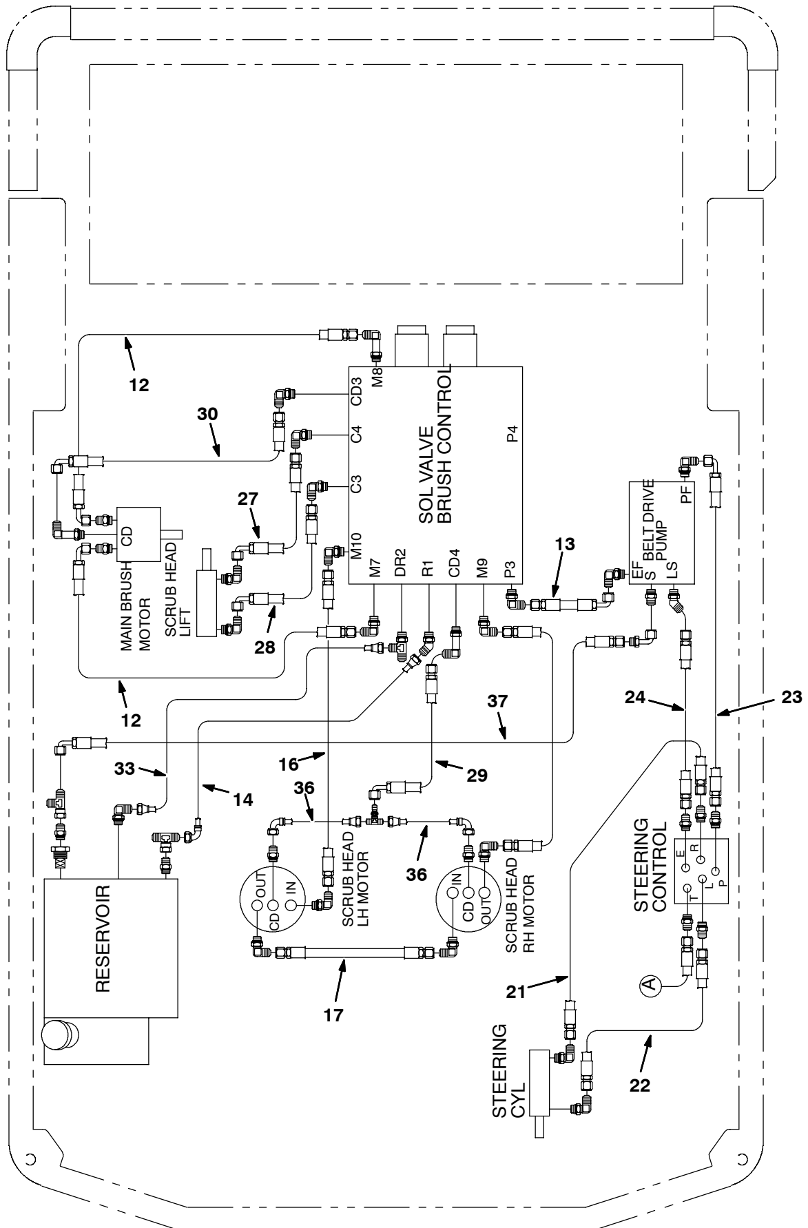
Fig. 67 - Hydraulic Hose Group
