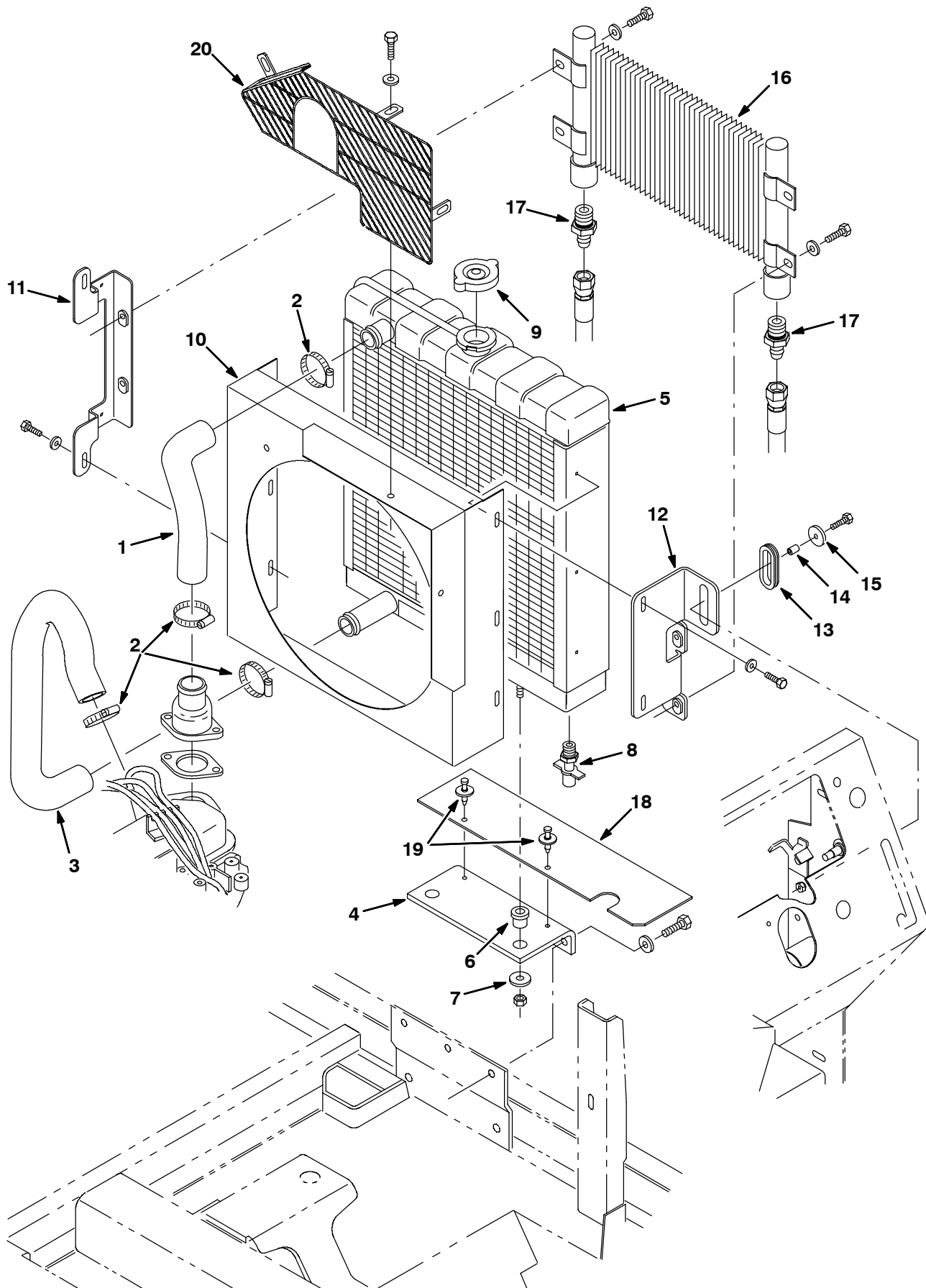
Fig. 34 - Enigne Radiator Group (000000-009999)
