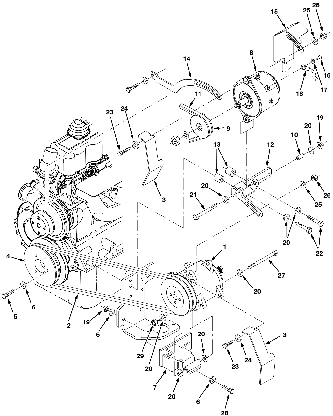
Fig. 26 - Cab AC Compressor Group, GM (007000-
