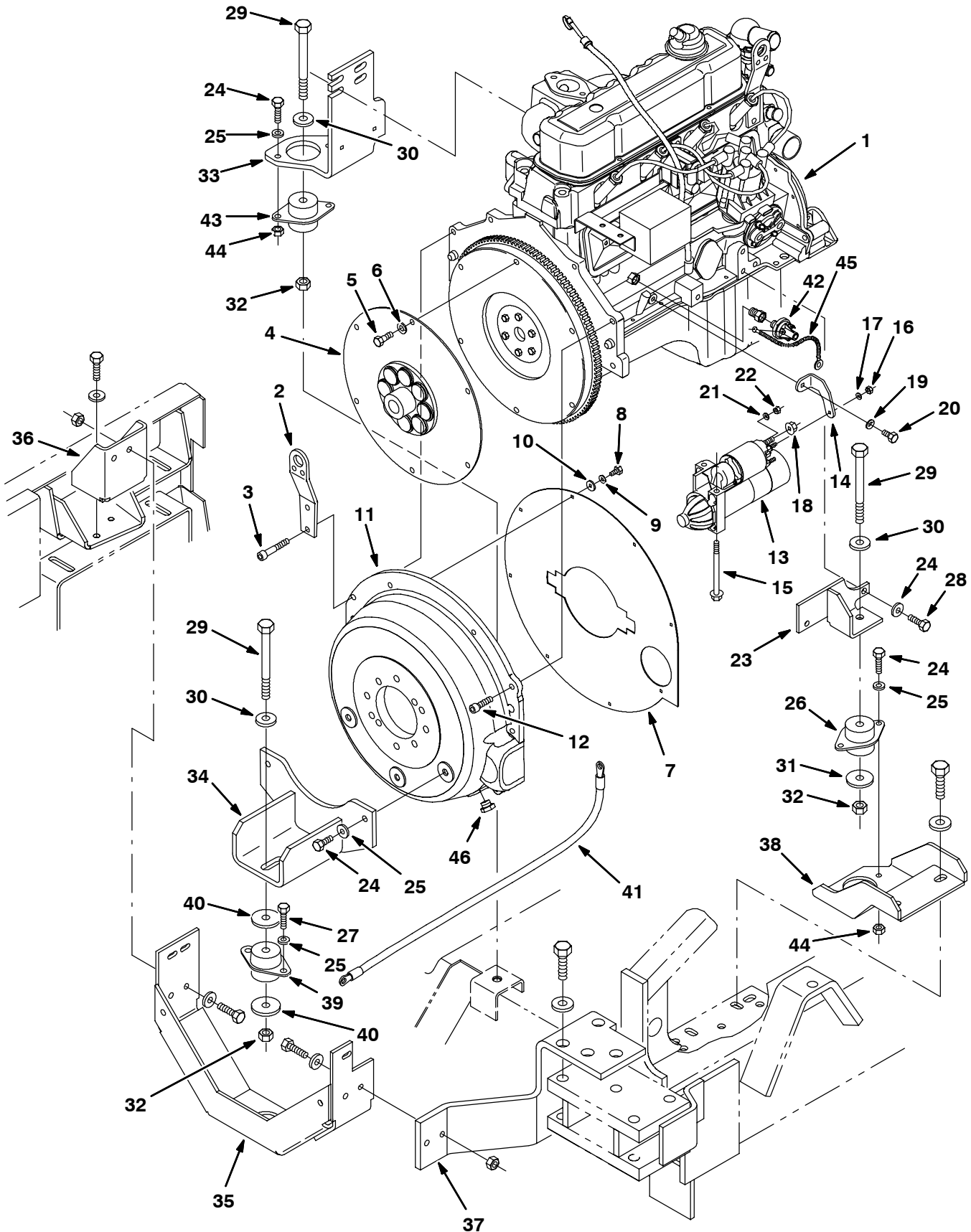
Fig. 22 - Engine Group (006000-006999)
