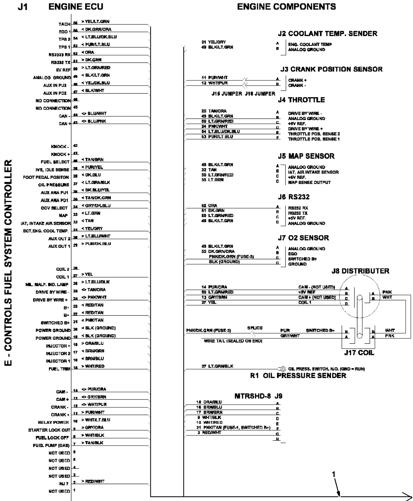
Fig. 96 - Wire Harnesses Group, Gas/LPG Engine (006000-006999)
