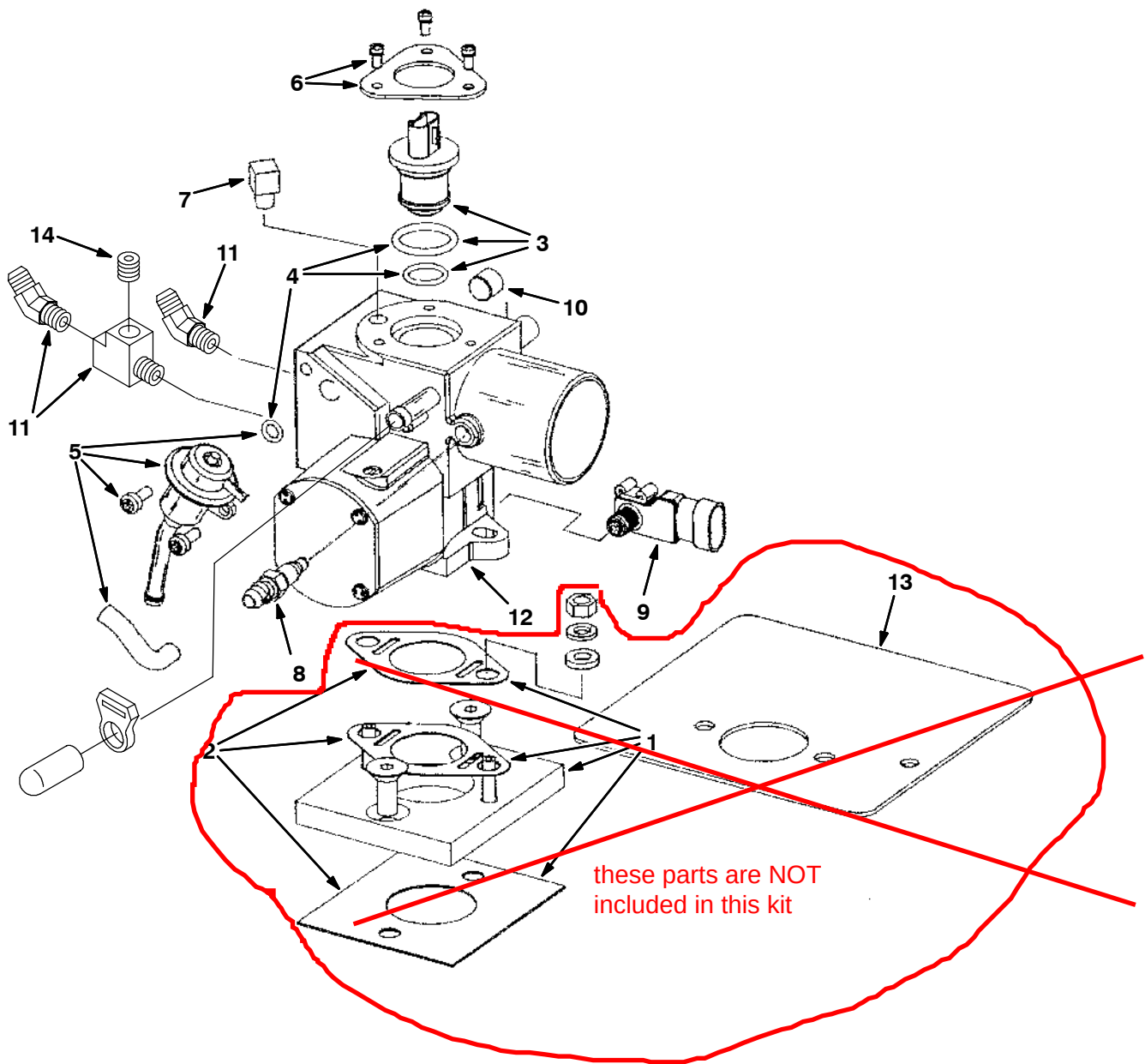
Fig. 39 - Gasoline Electronic Fuel Ignition Breakdown, 371897
