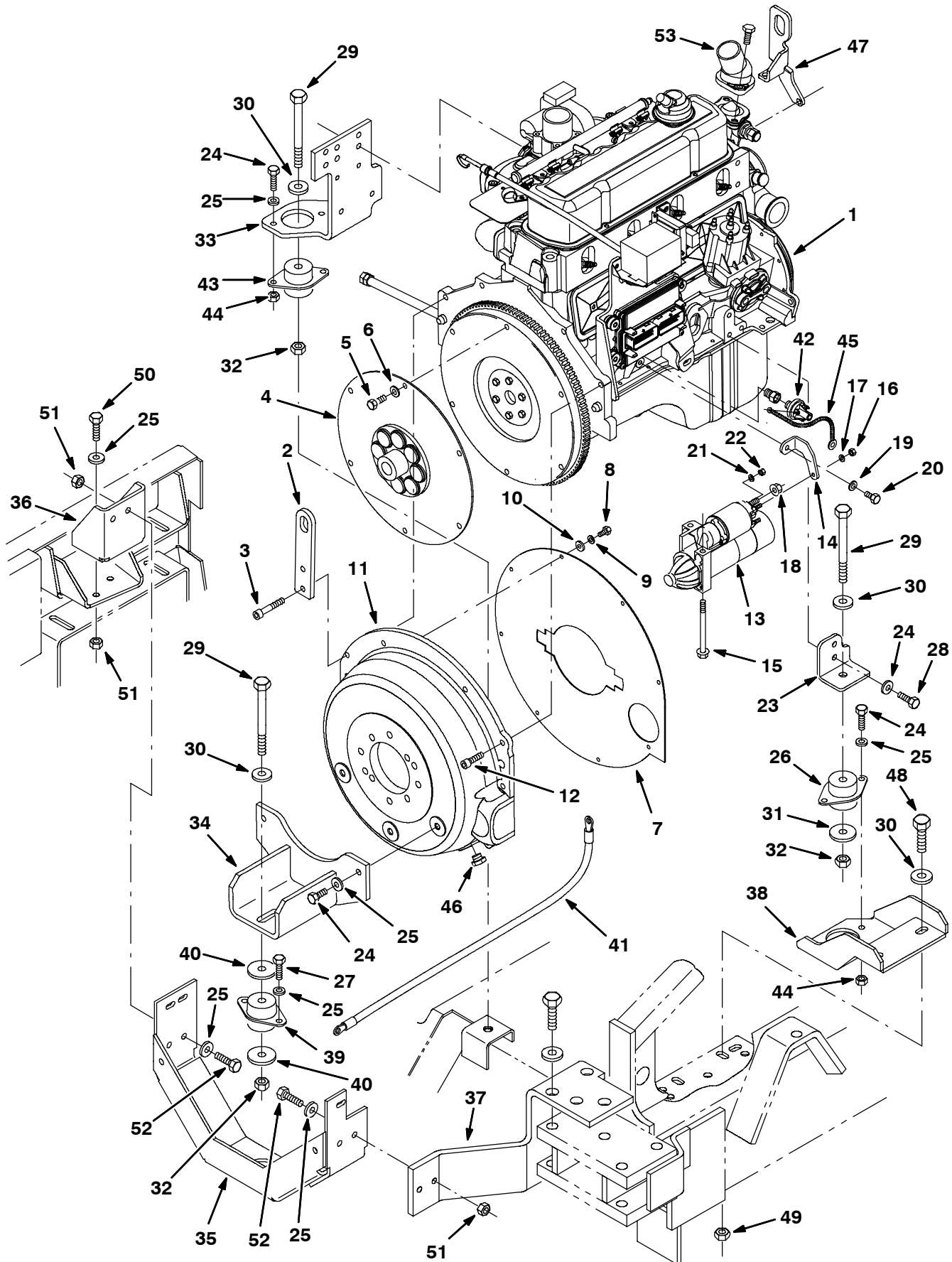
Fig. 23 - Engine Group (007000- )
