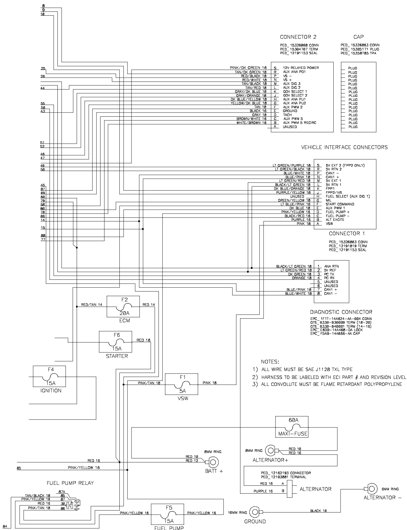
Fig. 99 - Wire Harnesses Schematic, Gas Engine (007000- )
