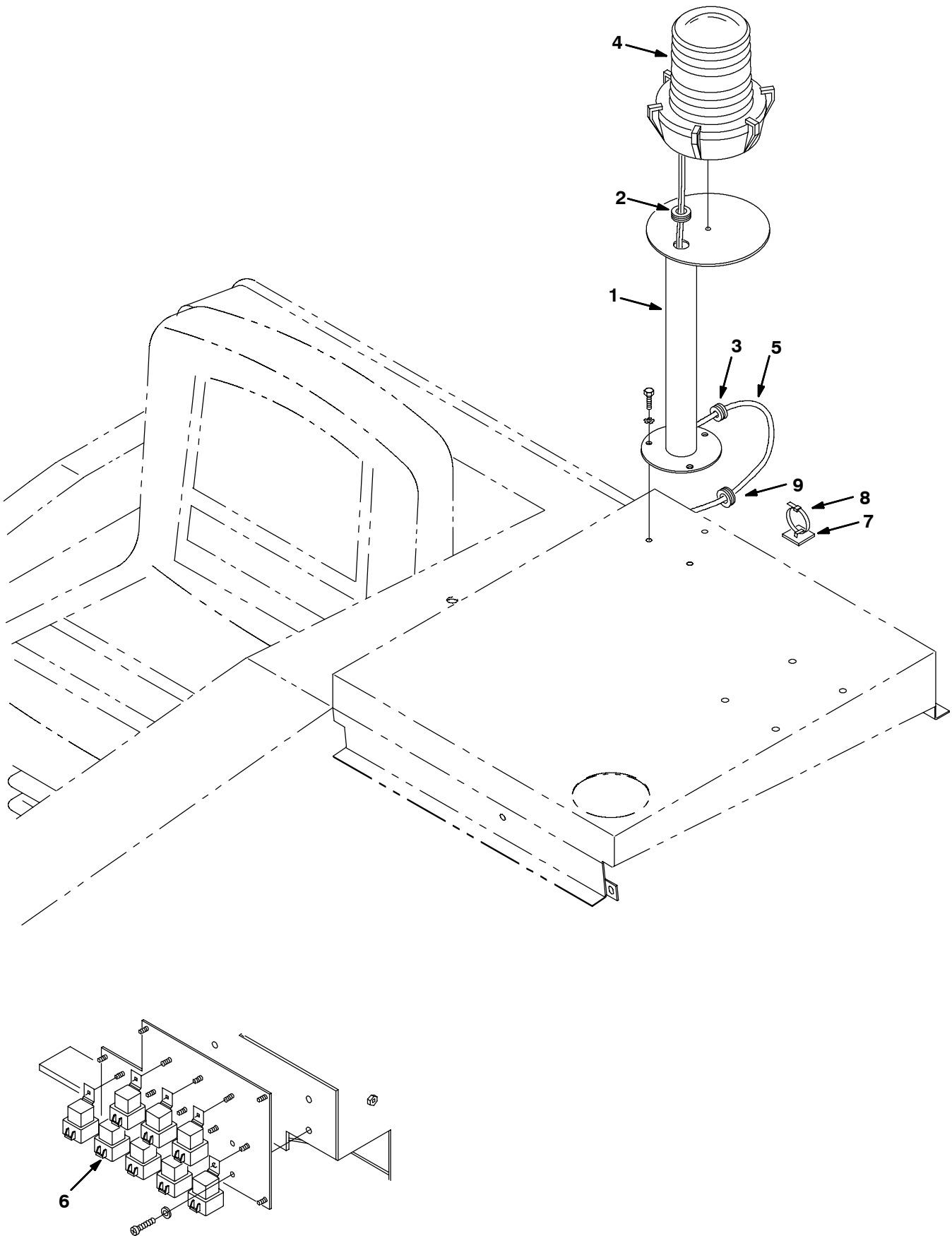
Fig. 5 - Light Kit, Flashing Low
