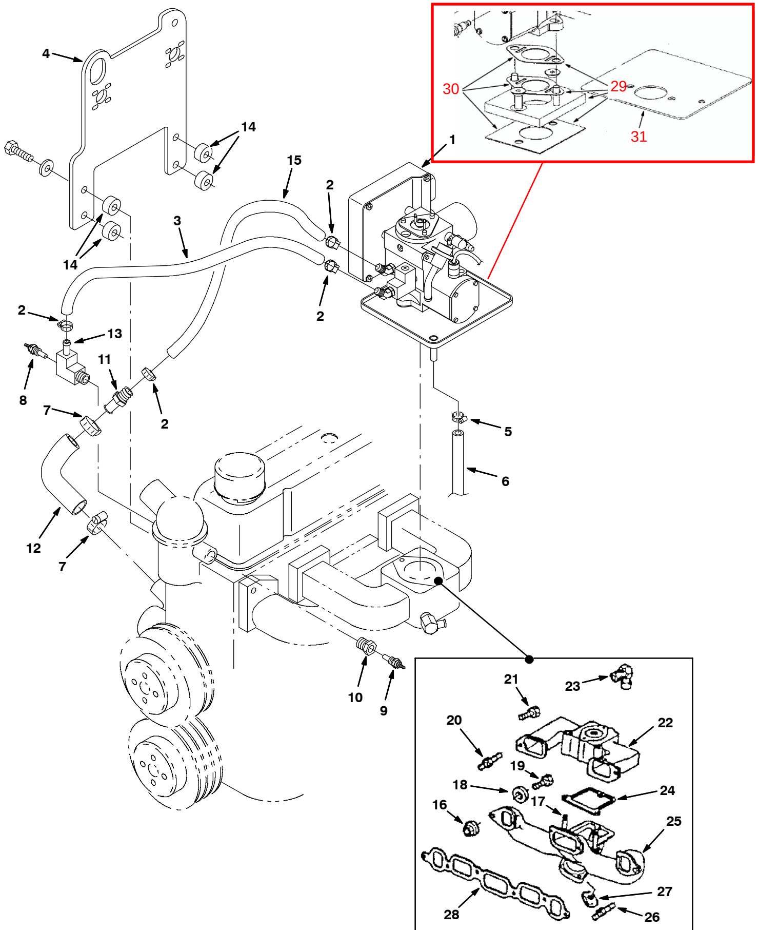
Fig. 29 - Engine Electronic Fuel Ignition Group, Gas (004937-005999)
