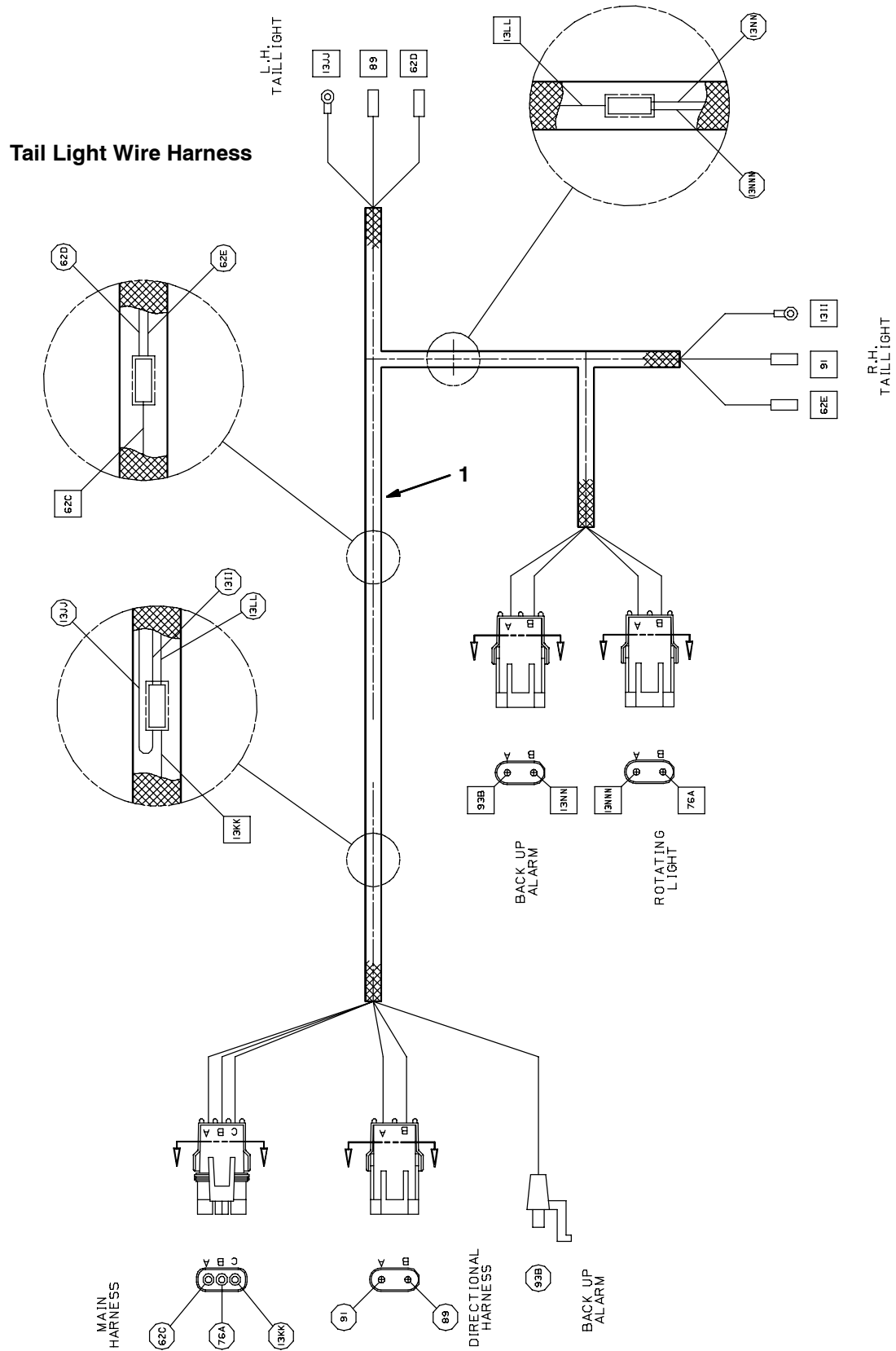
Fig. 93 - Wire Harnesses Group, Gas/LPG, Tail Lights (004000- )
