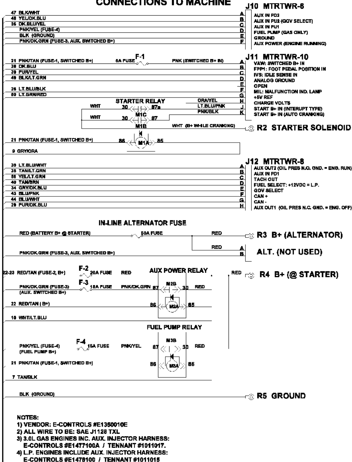
Fig. 89 - Electrical Schematic (006000- )
