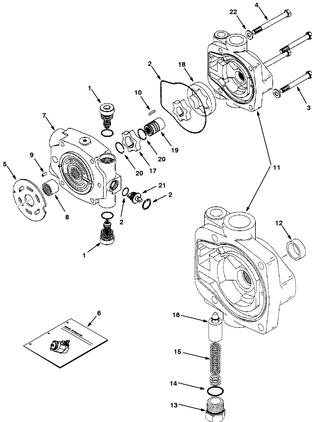
Fig. 4 - Hydraulic Piston Pump Breakdown, 373404
