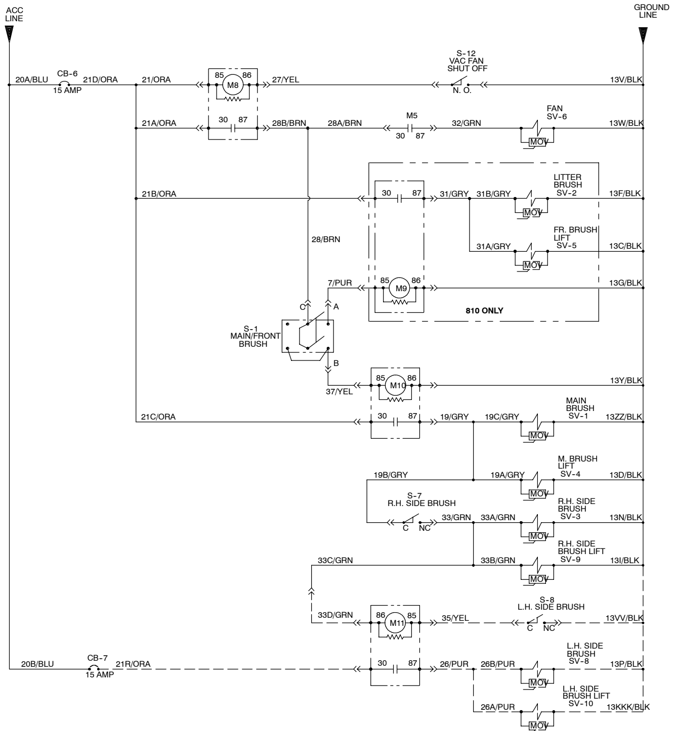
Fig. 87 - Electrical Schematic (004000-004936)
