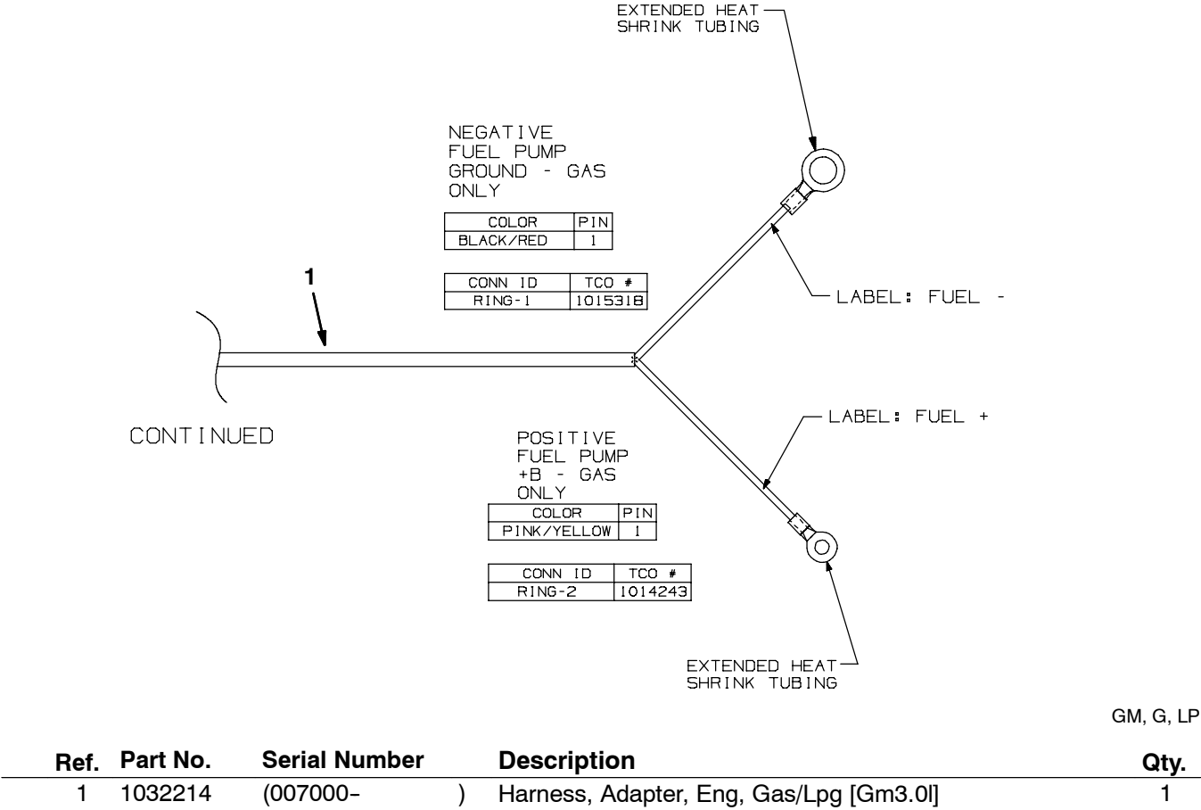
Fig. 102 - Wire Harnesses Group, Gas/LPG, Adaptor (007000- )
