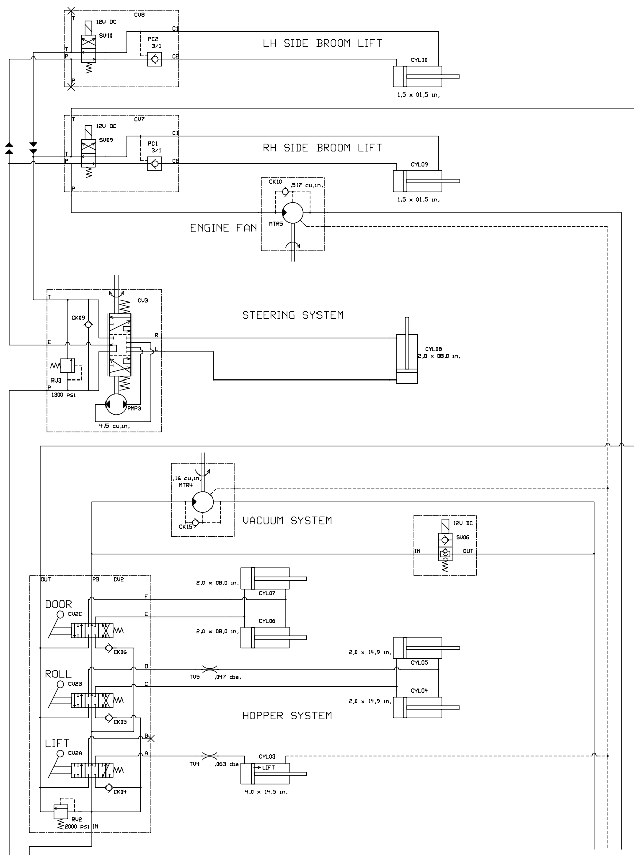
Fig. 71 - Hydraulic Schematic
