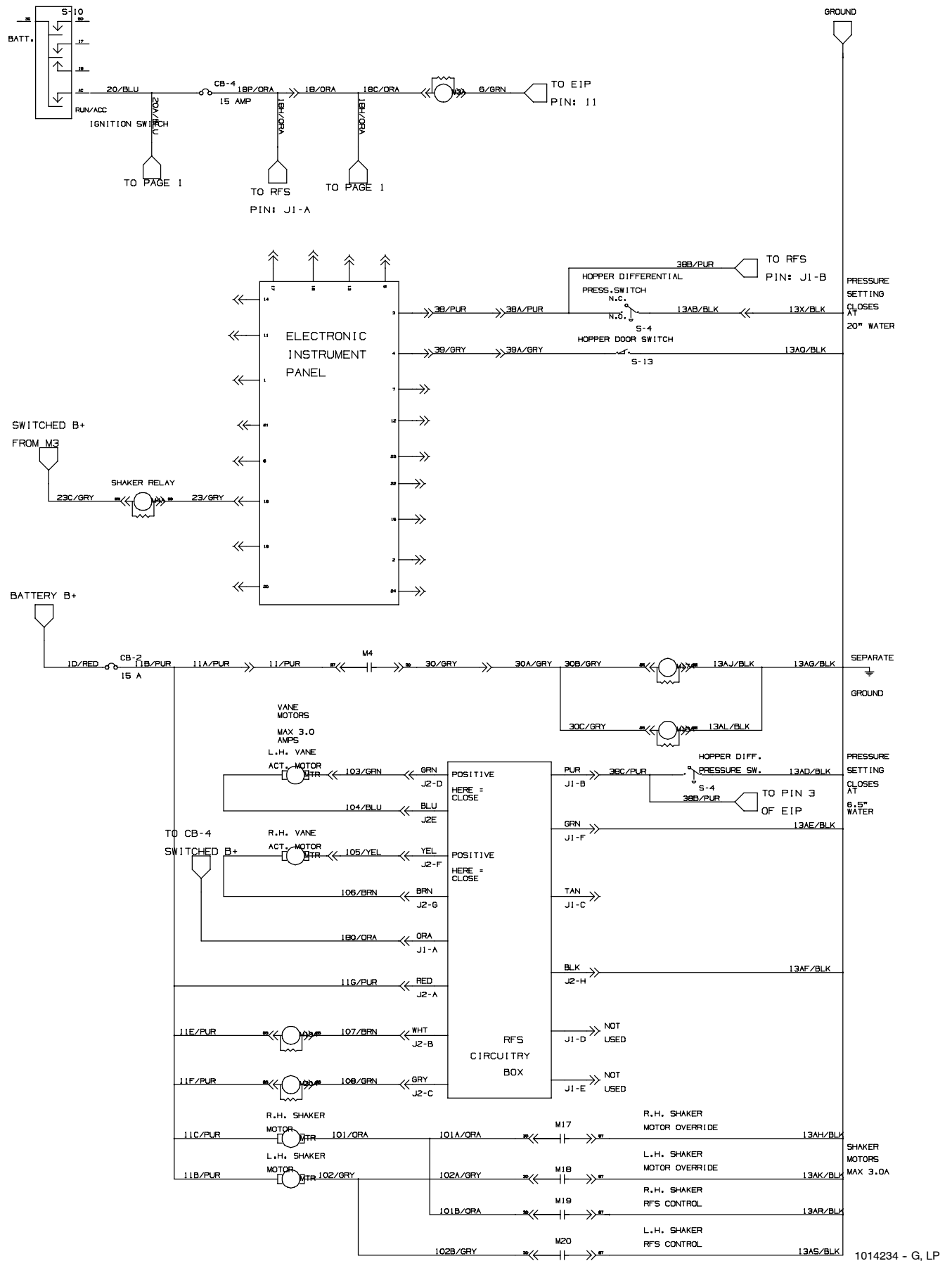
Fig. 90 - Electrical Schematic (006000- )
