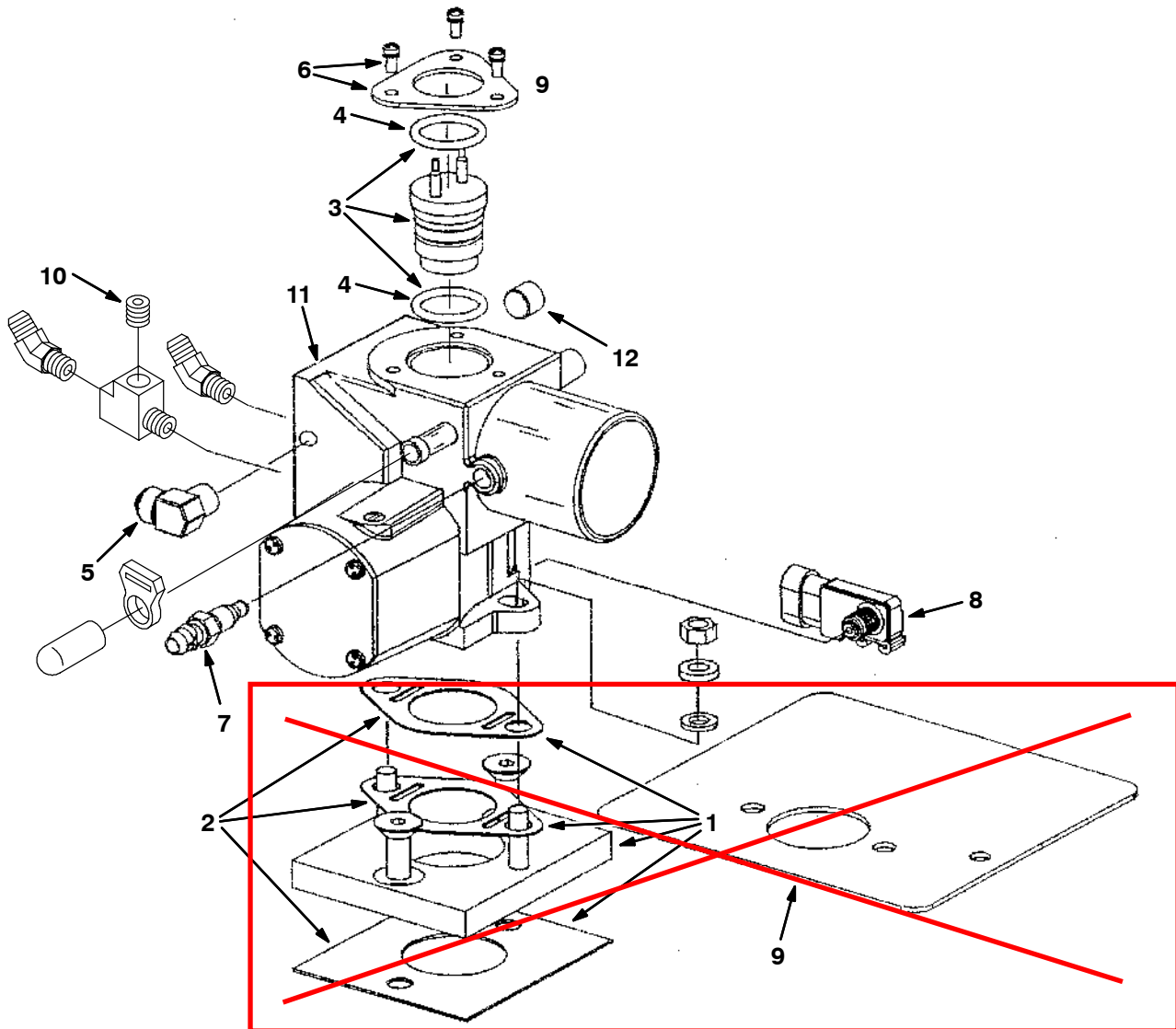
Fig. 37 - LPG EFI Breakdown, 371895
