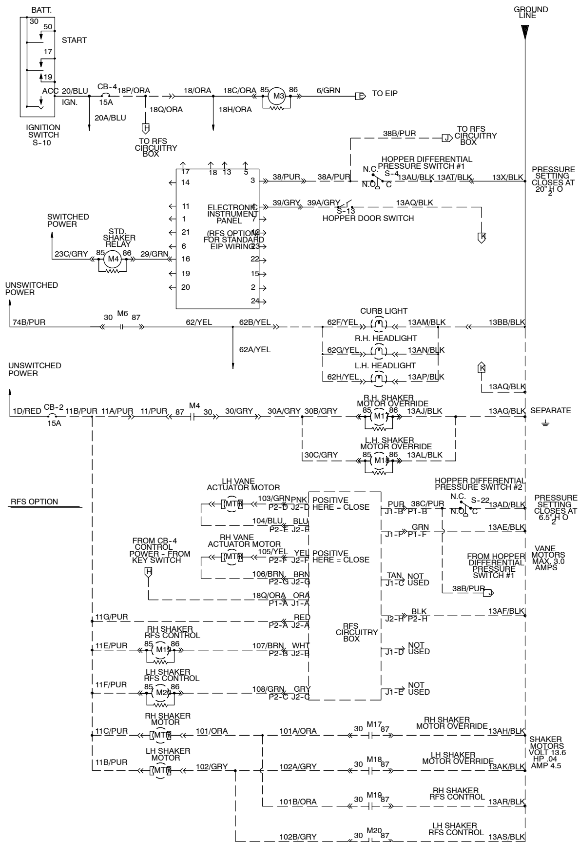
Fig. 87 - Electrical Schematic (004000-004936)
