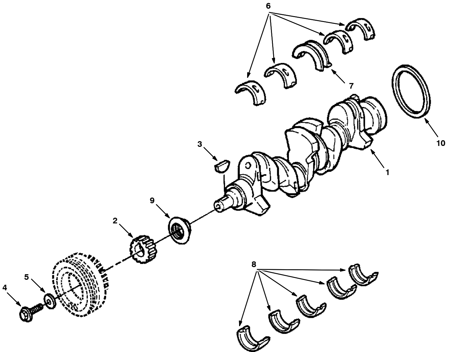
Fig. 7 - Crankshaft Group
