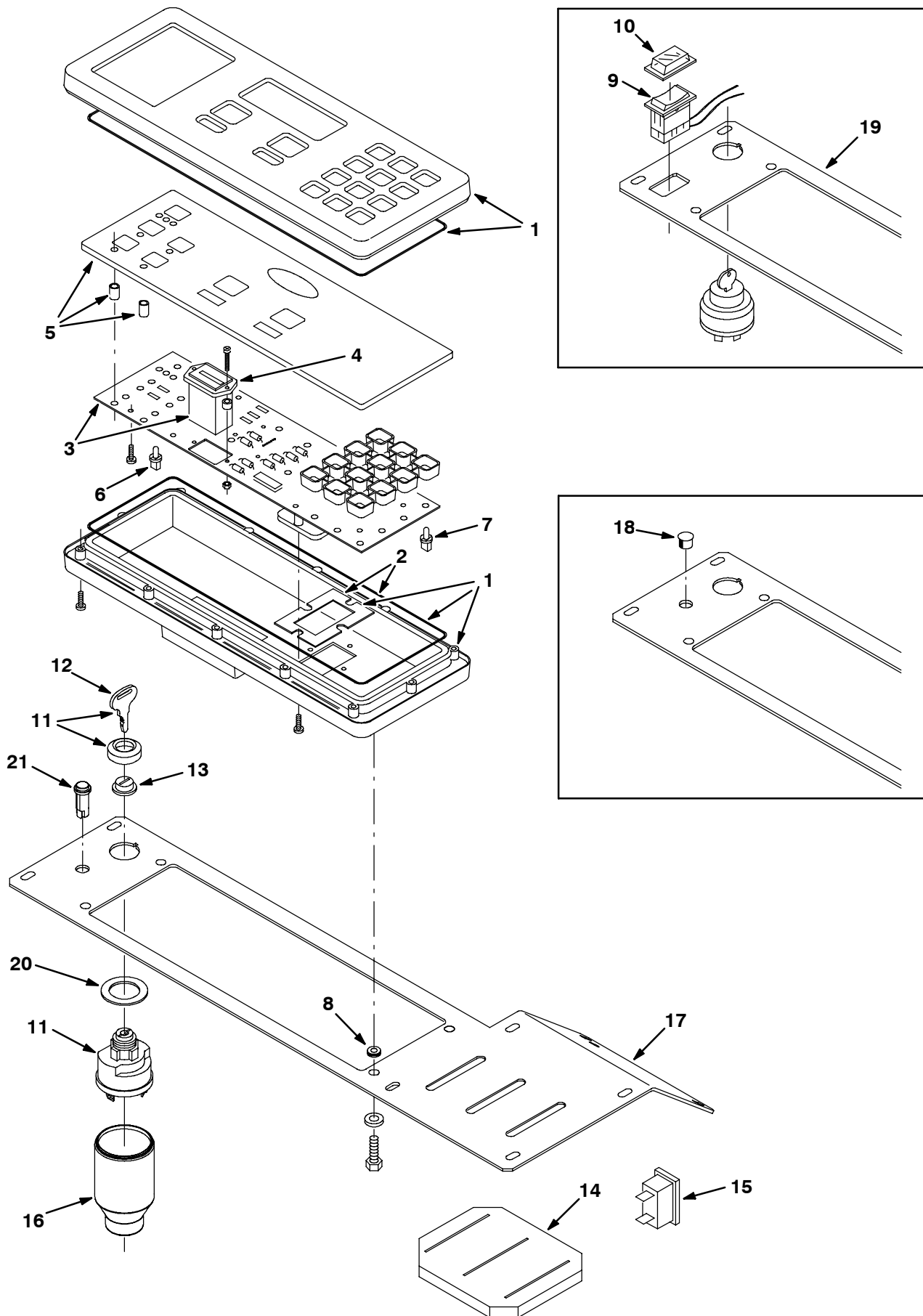
Fig. 85 - Electrical Instrument Panel Assembly
