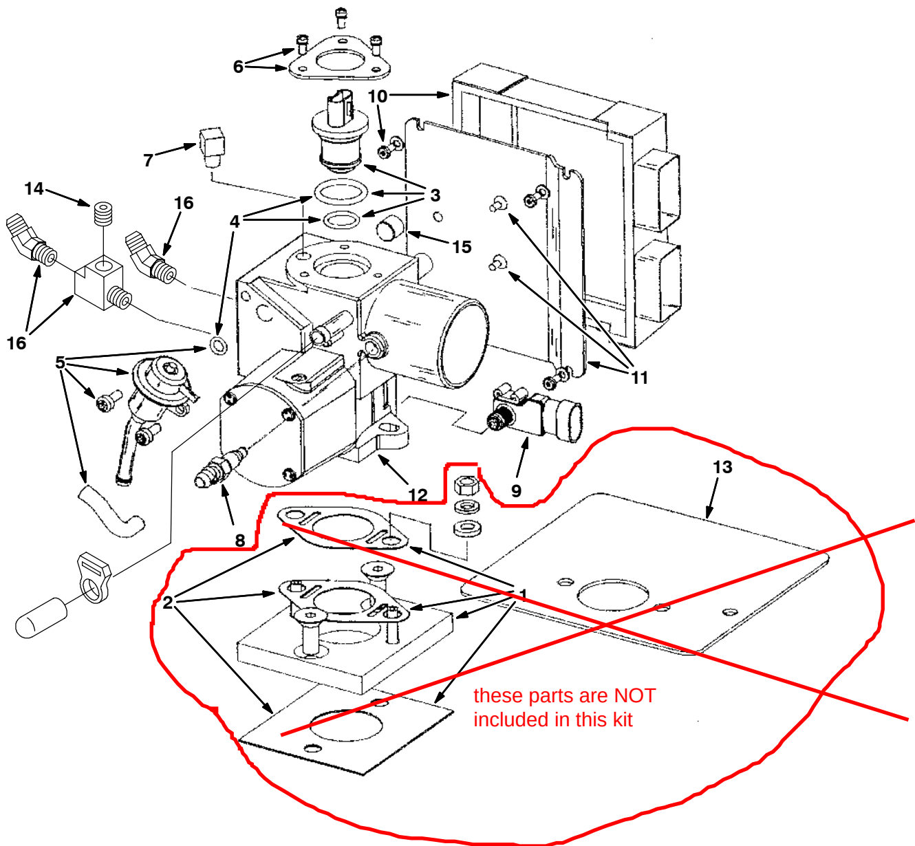
Fig. 38 - Gasoline EFI Breakdown, 371896
