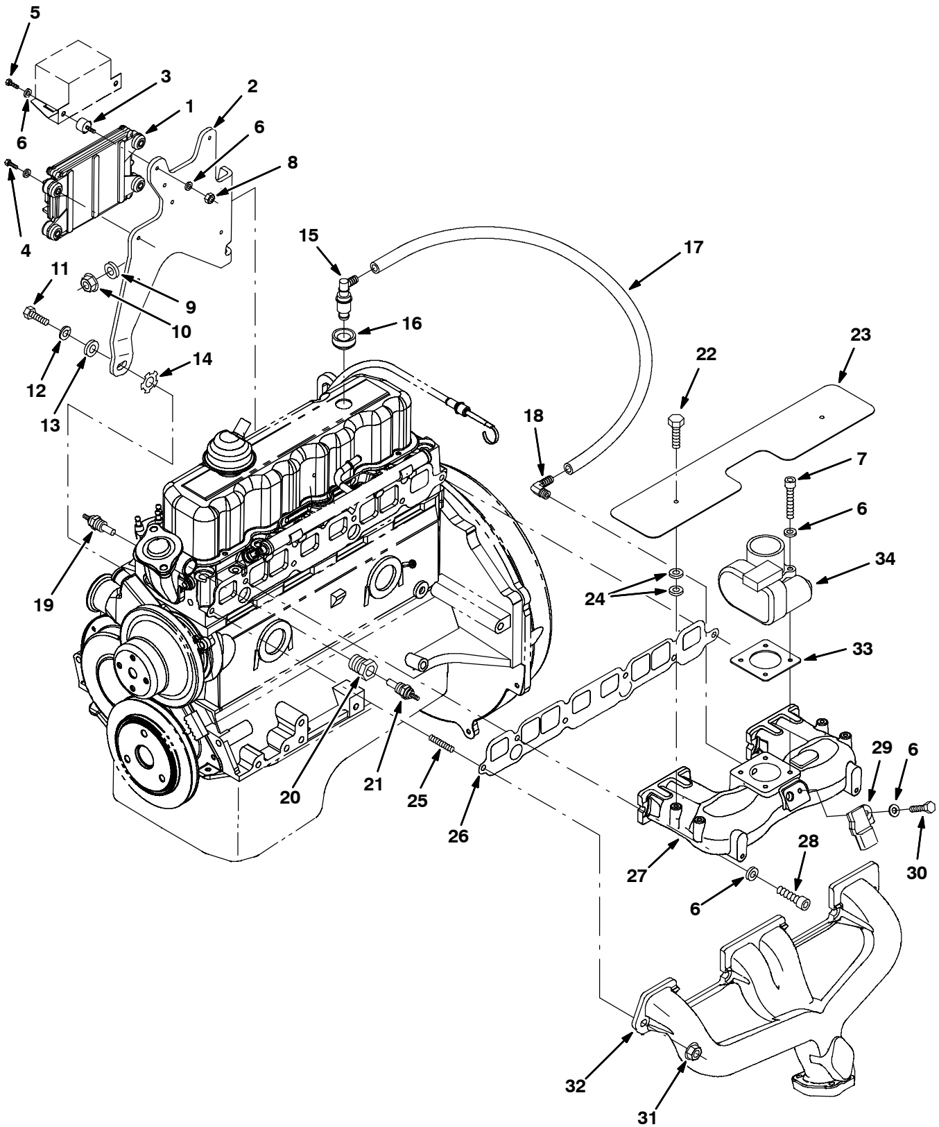
Fig. 31 - Engine Electronic Fuel Ignition Group, Gas (007000- )
