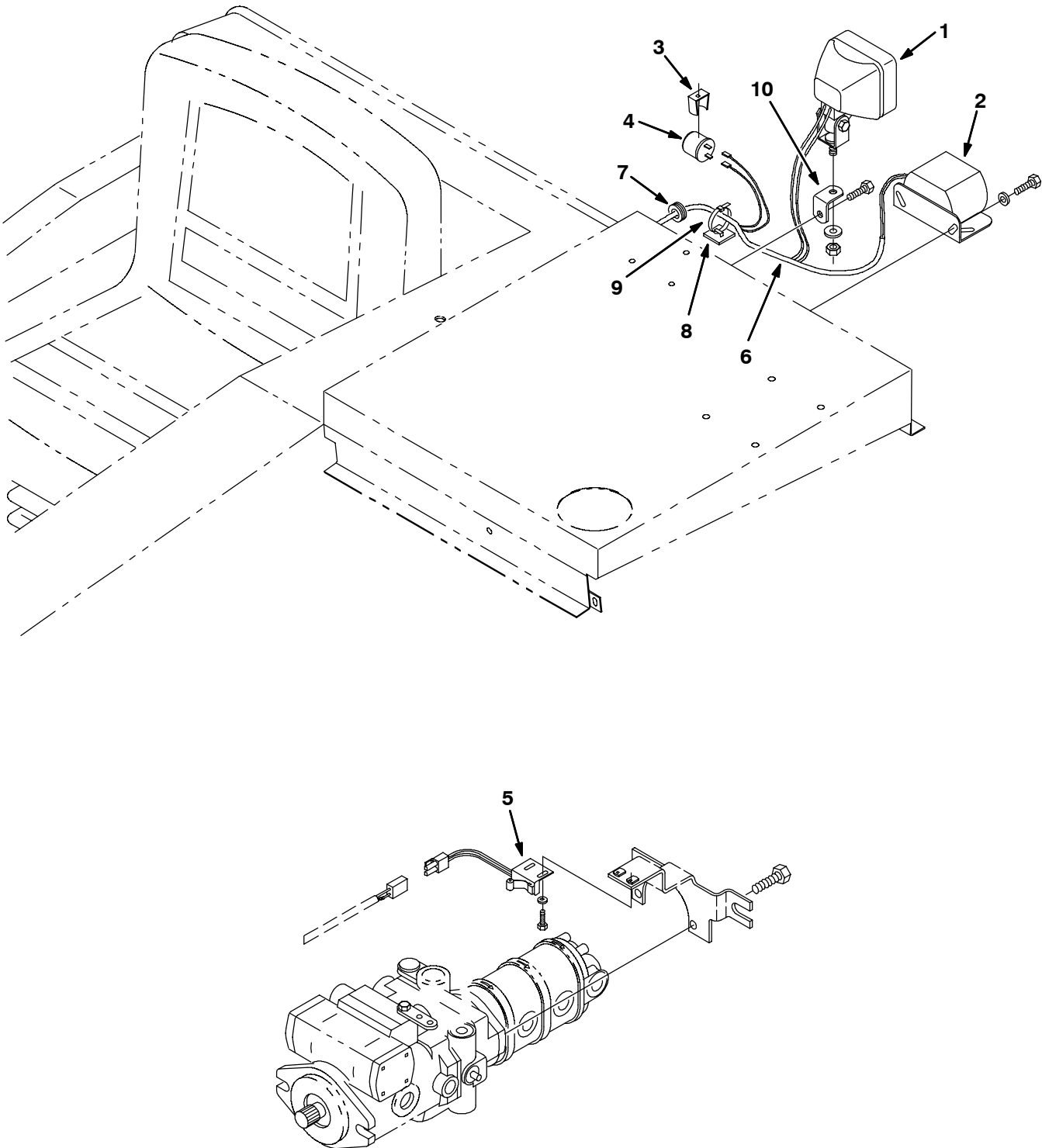
Fig. 7 - Back-Up Alarm Kit
