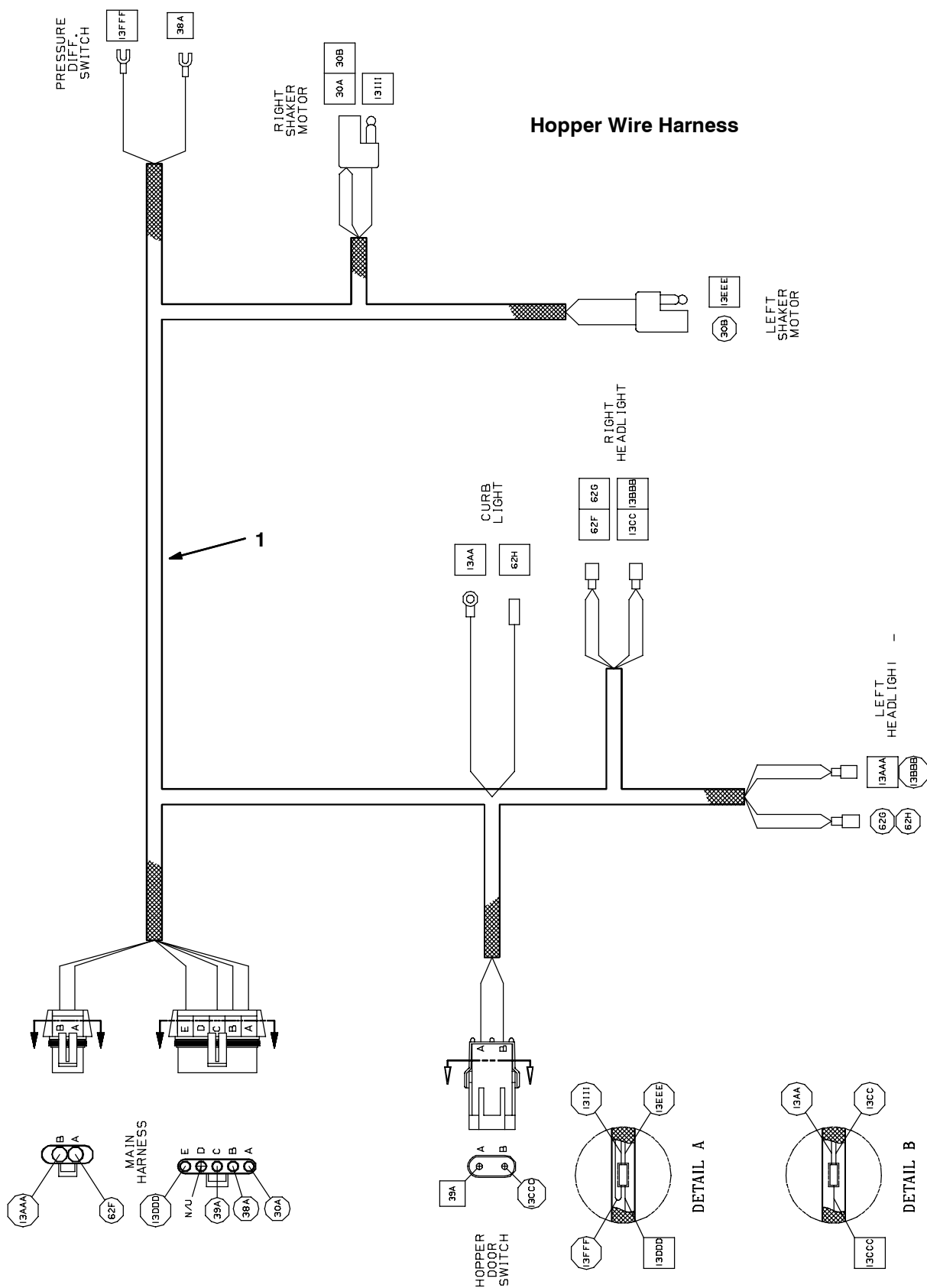
Fig. 92 - Wire Harnesses Group, Gas/LPG, Hopper (004000- )
