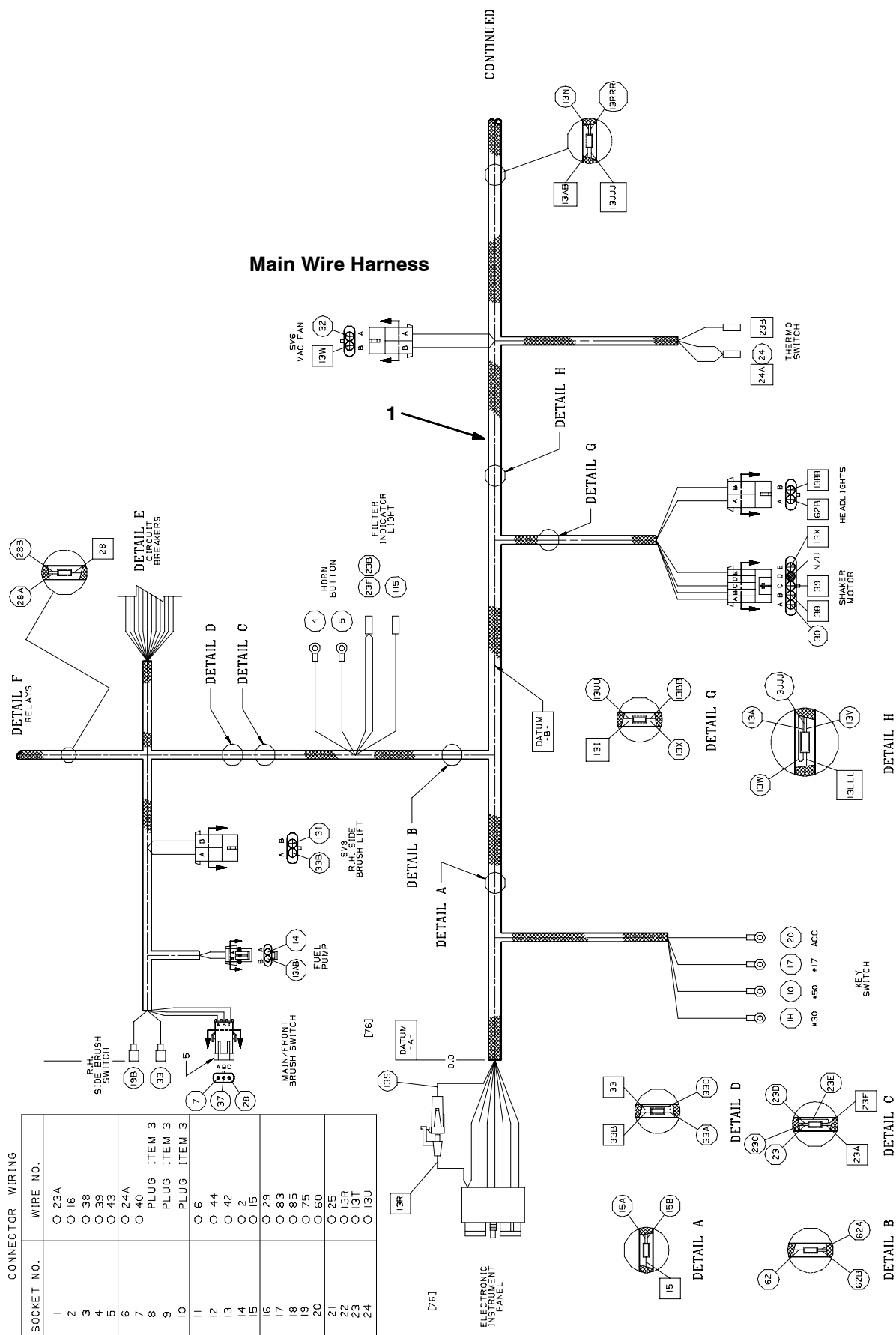
Fig. 94 - Wire Harnesses Group, Gas/LPG, Main (004275-004936)
