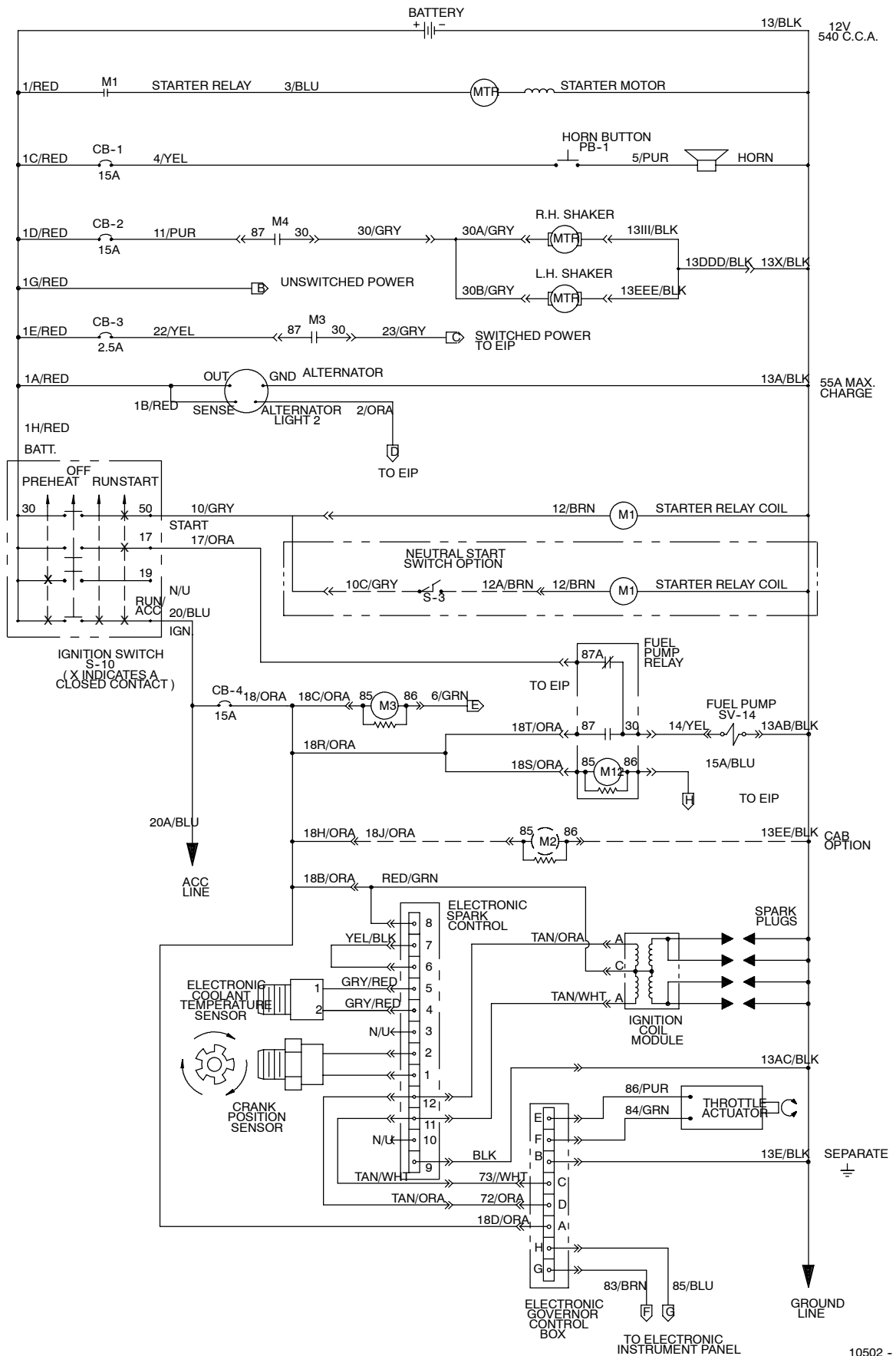
Fig. 87 - Electrical Schematic (004000-004936)
