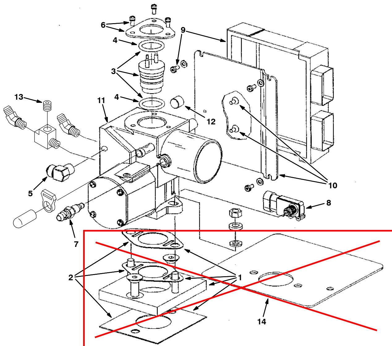
Fig. 36 - LPG EFI Breakdown, 371894
