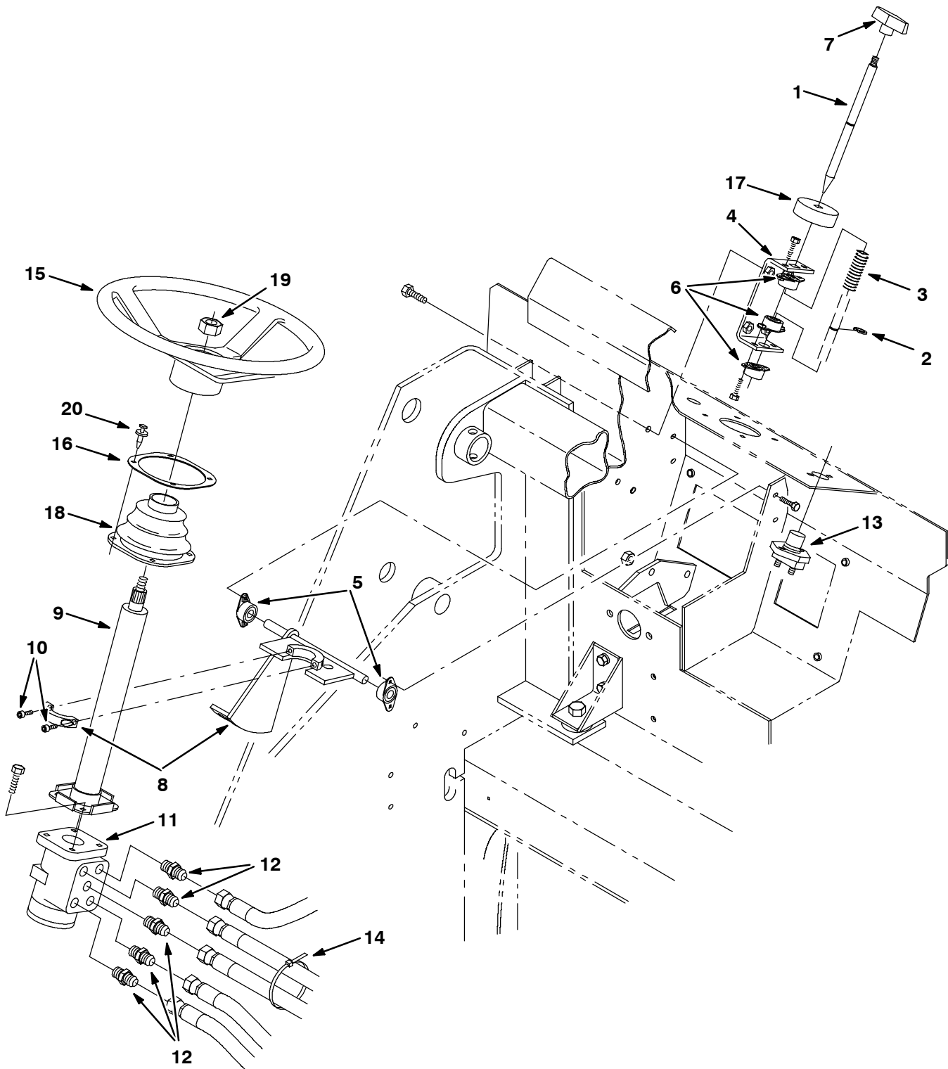
Fig. 84 - Steering Group
