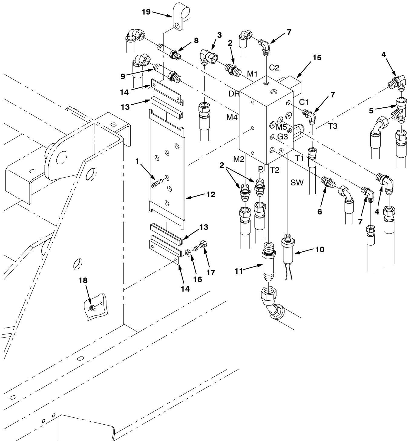
Fig. 75 - Hydraulic Solenoid Valve Group
