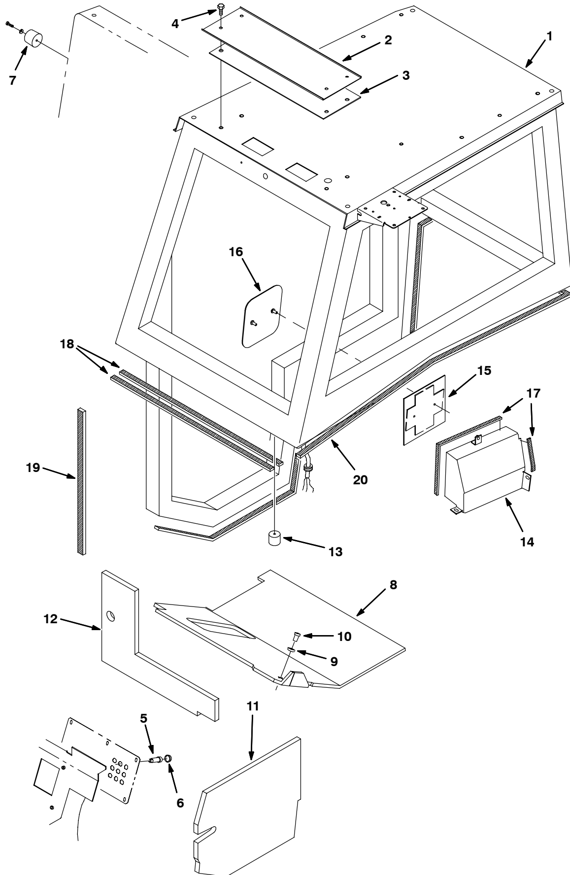
Fig. 17 - Cab Kit
