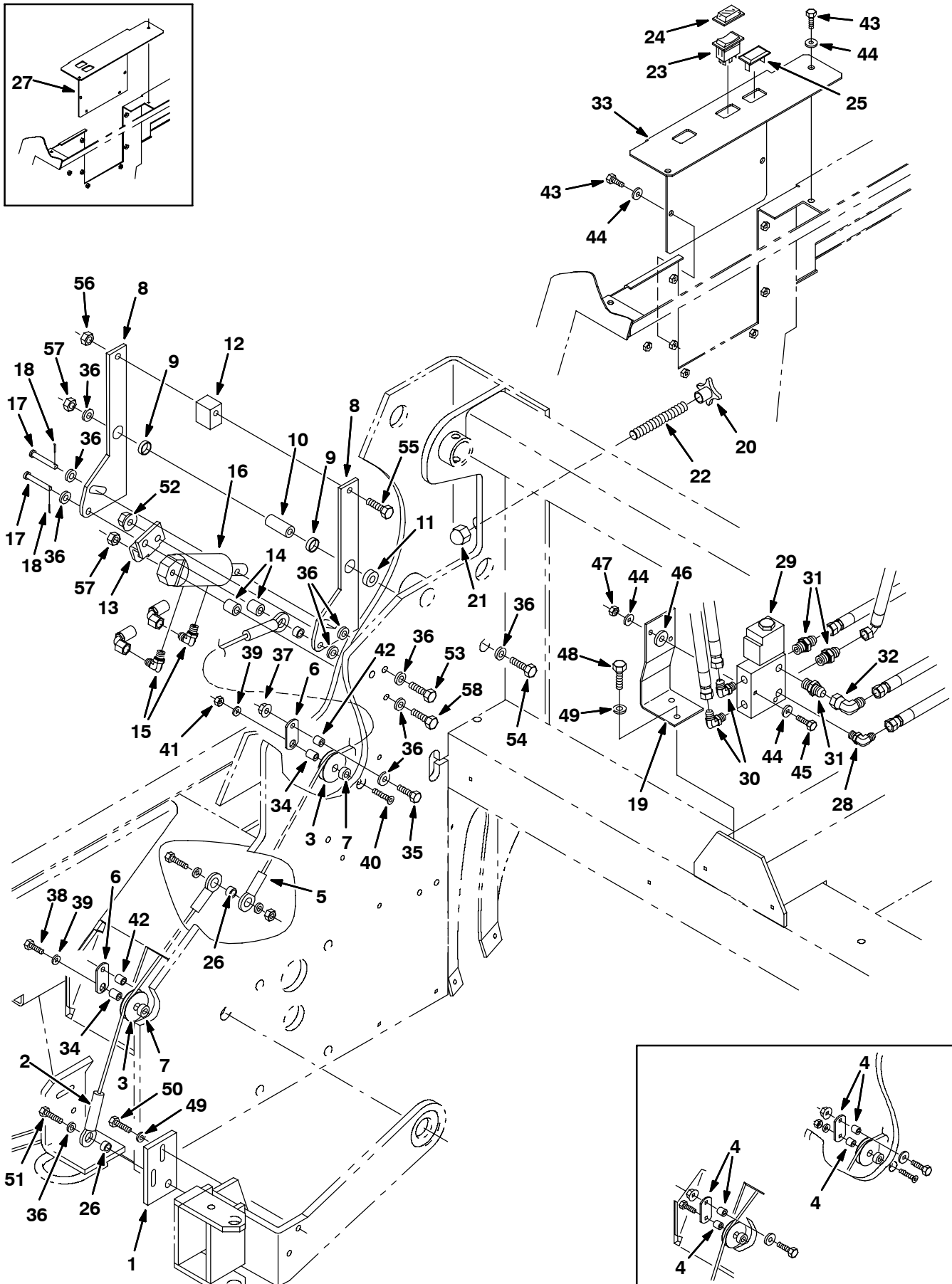
Fig. 78 - Brush Lift Group, Side
