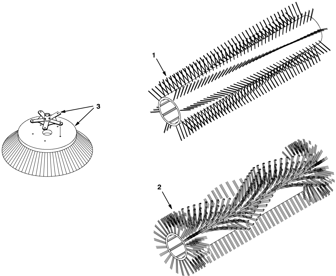
Fig. 2 - Brushes, Replacement
