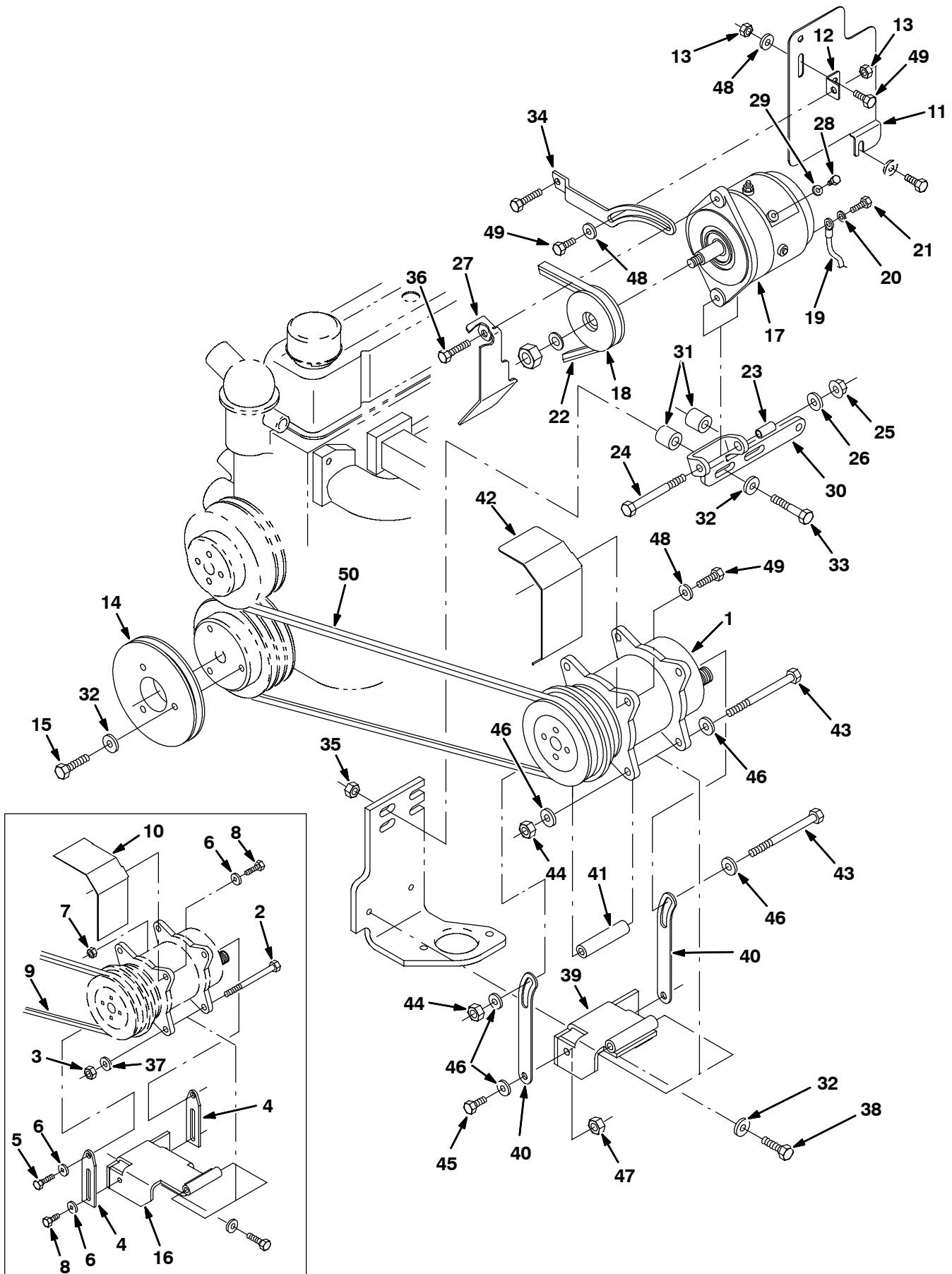
Fig. 25 - Cab AC Compressor Group, GM GM (004937-006999)
