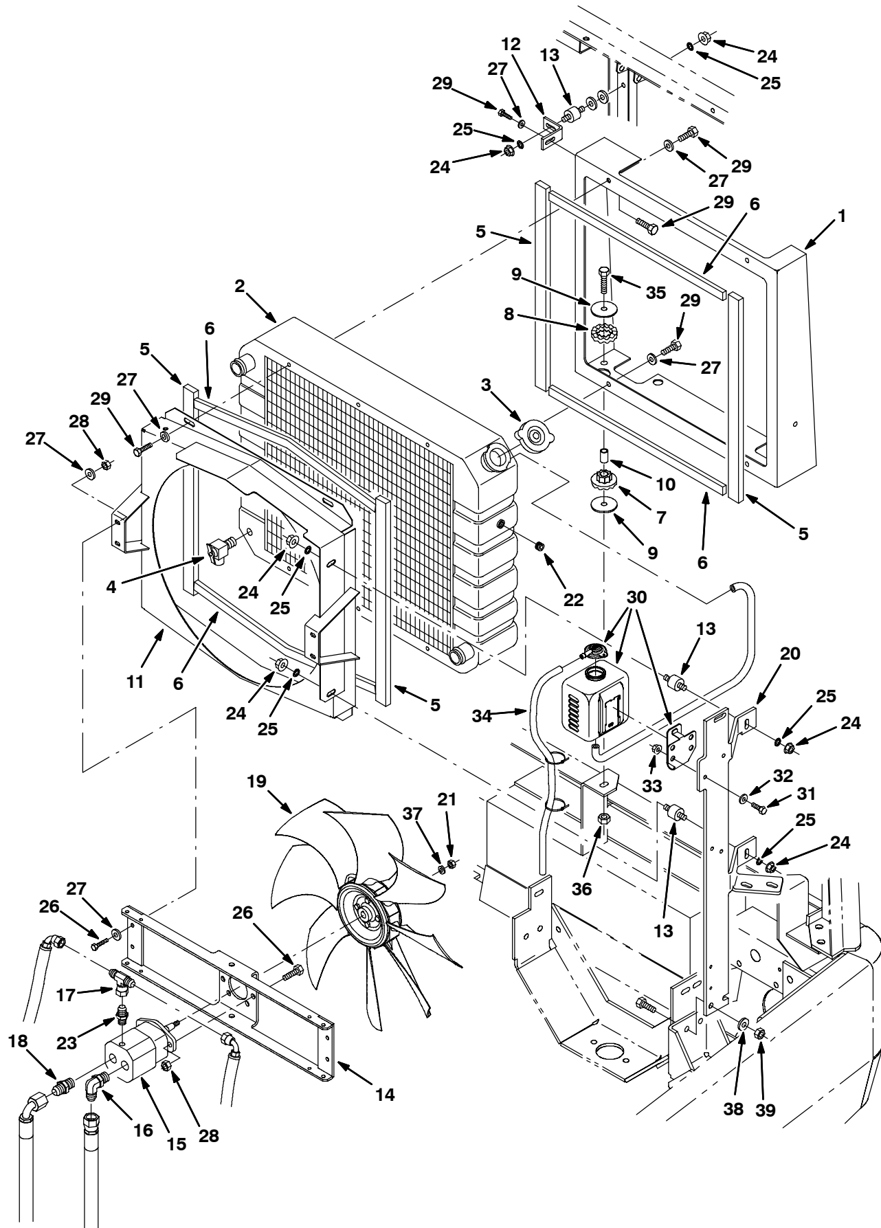
Fig. 62 - Engine Radiator and Cooling Fan Group (007000- )
