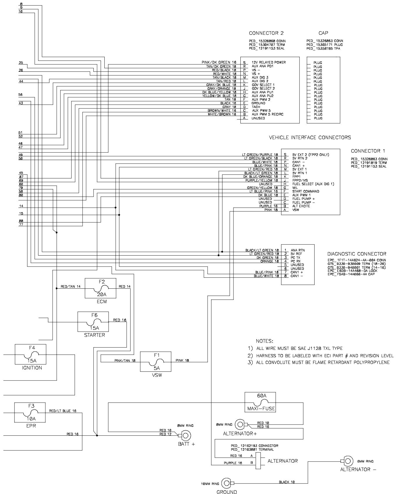
Fig. 100 - Wire Harnesses Schematic, LPG Engine (007000- )
