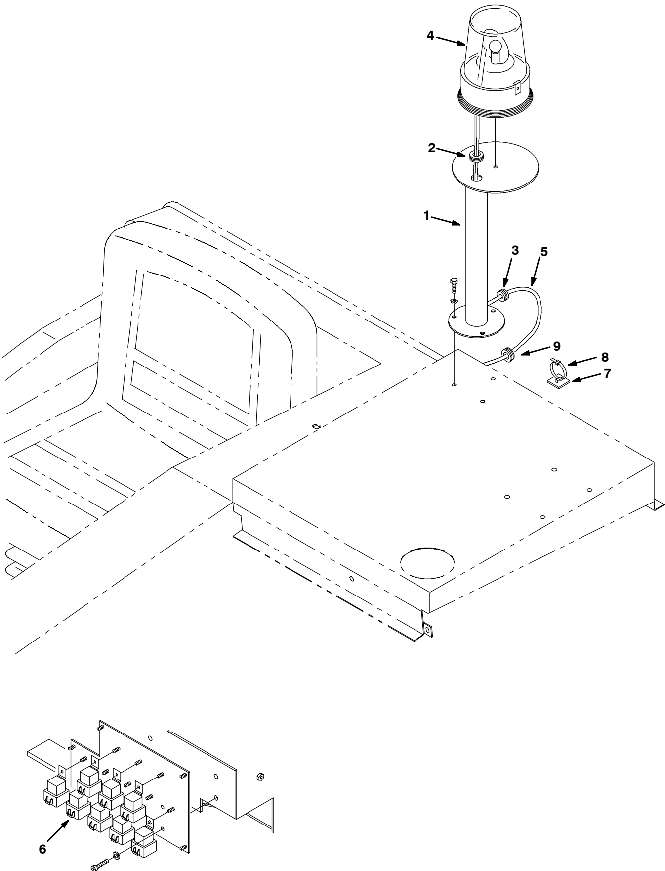
Fig. 6 - Light Kit, Revolving Low
