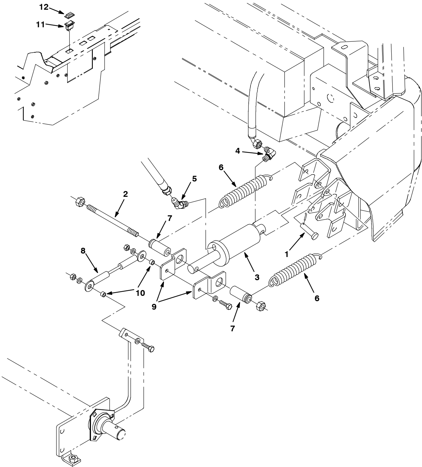
Fig. 80 - Brush Lift Group, Main
