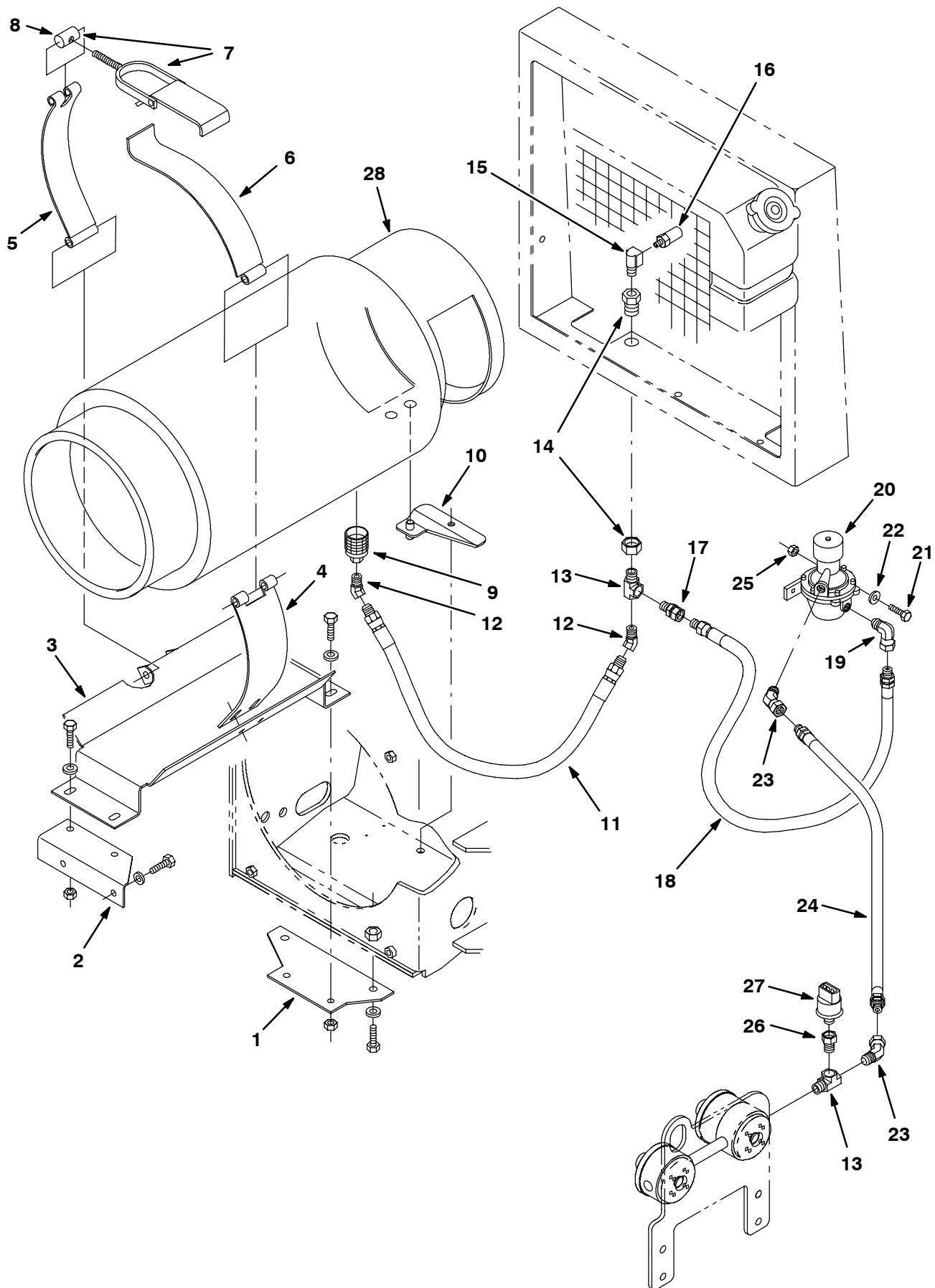
Fig. 53 - Engine Fuel Tank Group, LPG (004937-005999)
