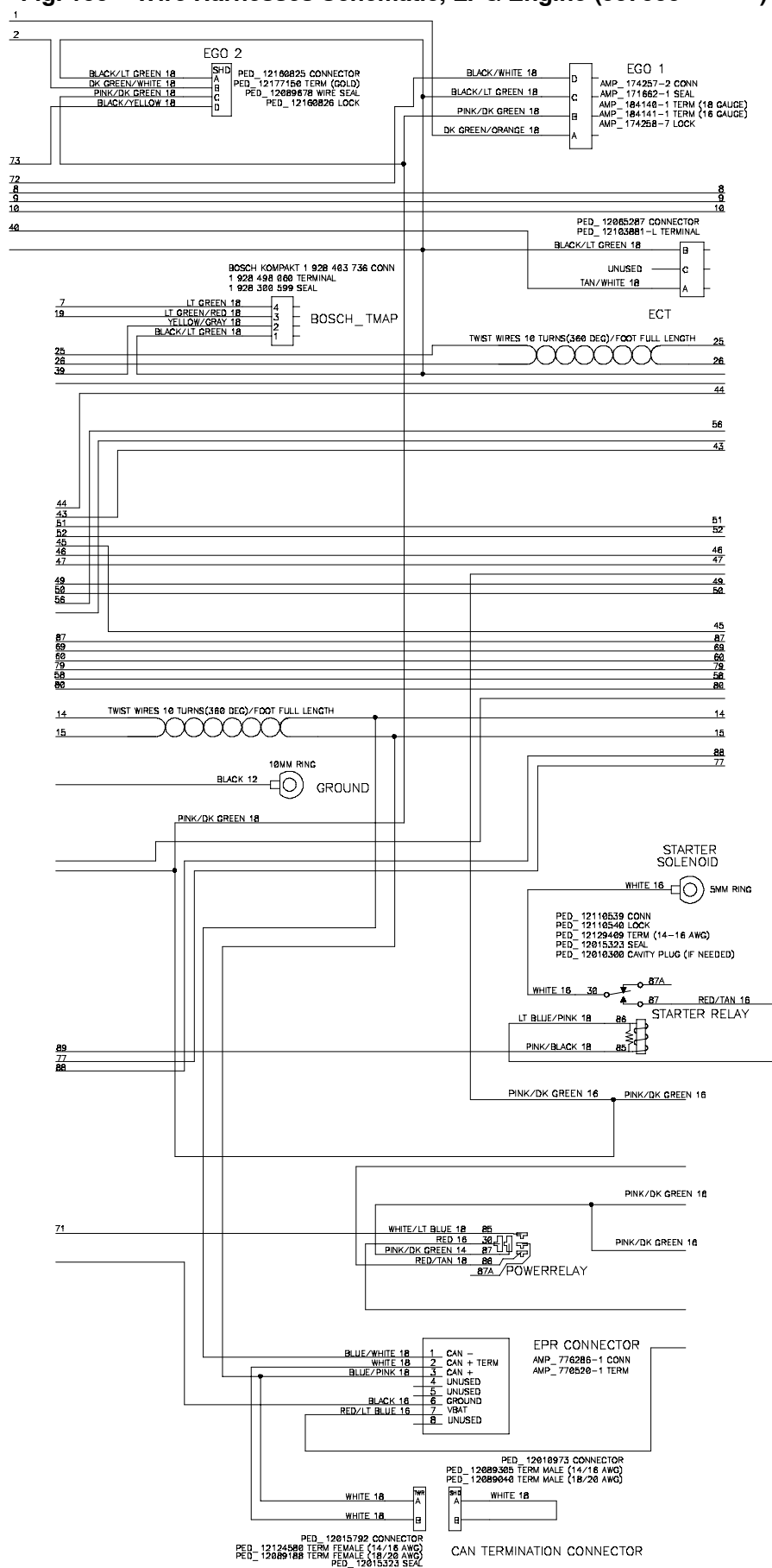
Fig. 100 - Wire Harnesses Schematic, LPG Engine (007000- )
