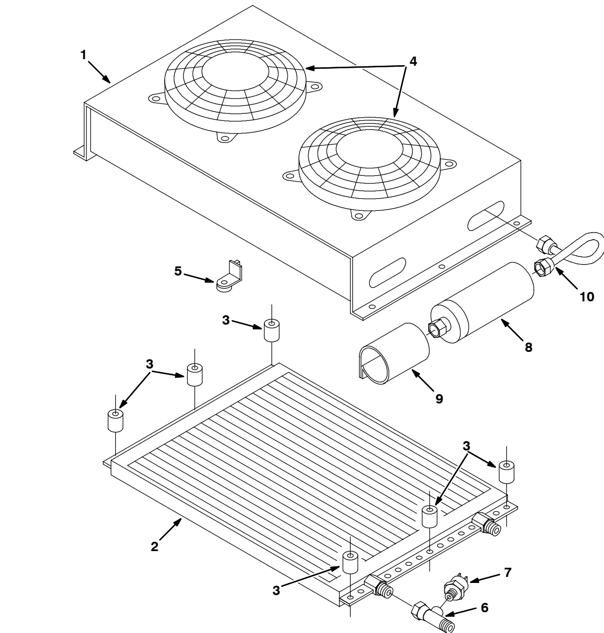
Fig. 31 - AC Condenser Box Breakdown, 380625
