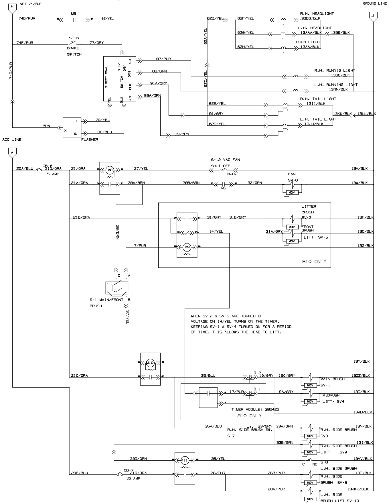
Fig. 89 - Electrical Schematic (006000- )
