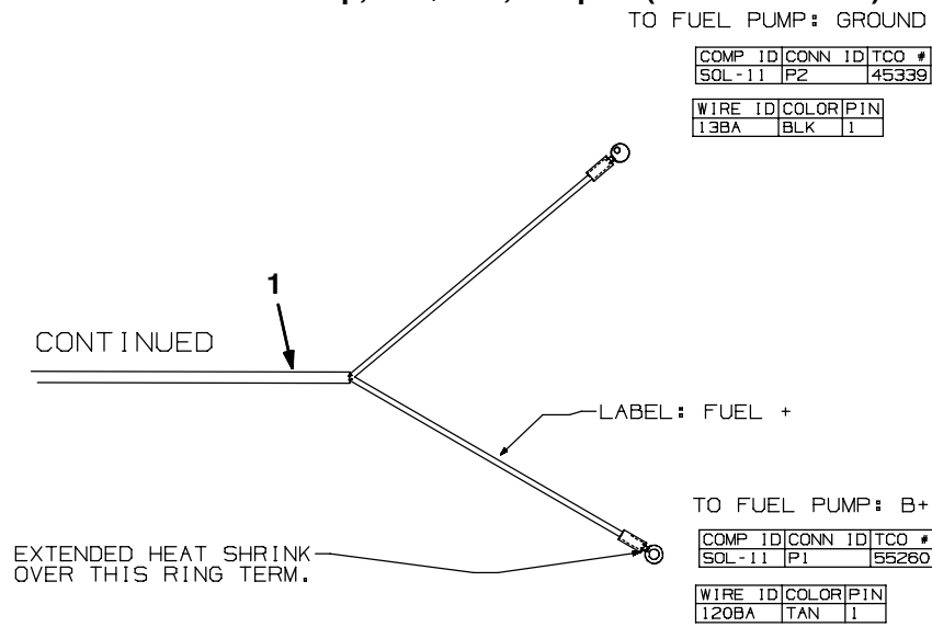
Fig. 101 - Wire Harnesses Group, Gas/LPG, Adaptor (006000-006999)
