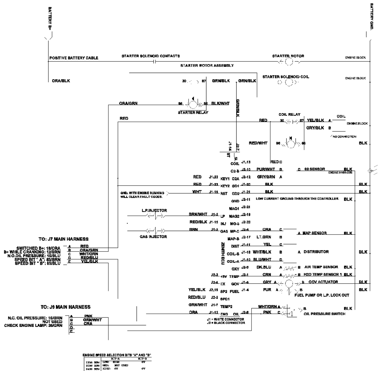
Fig. 88 - Electrical Schematic (004937-005999)
