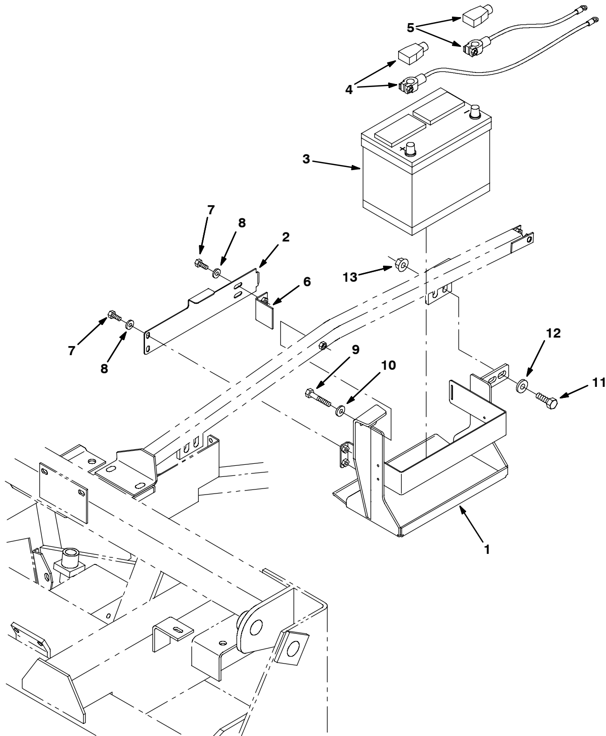
Fig. 64 - Engine Battery Group (007000- )
