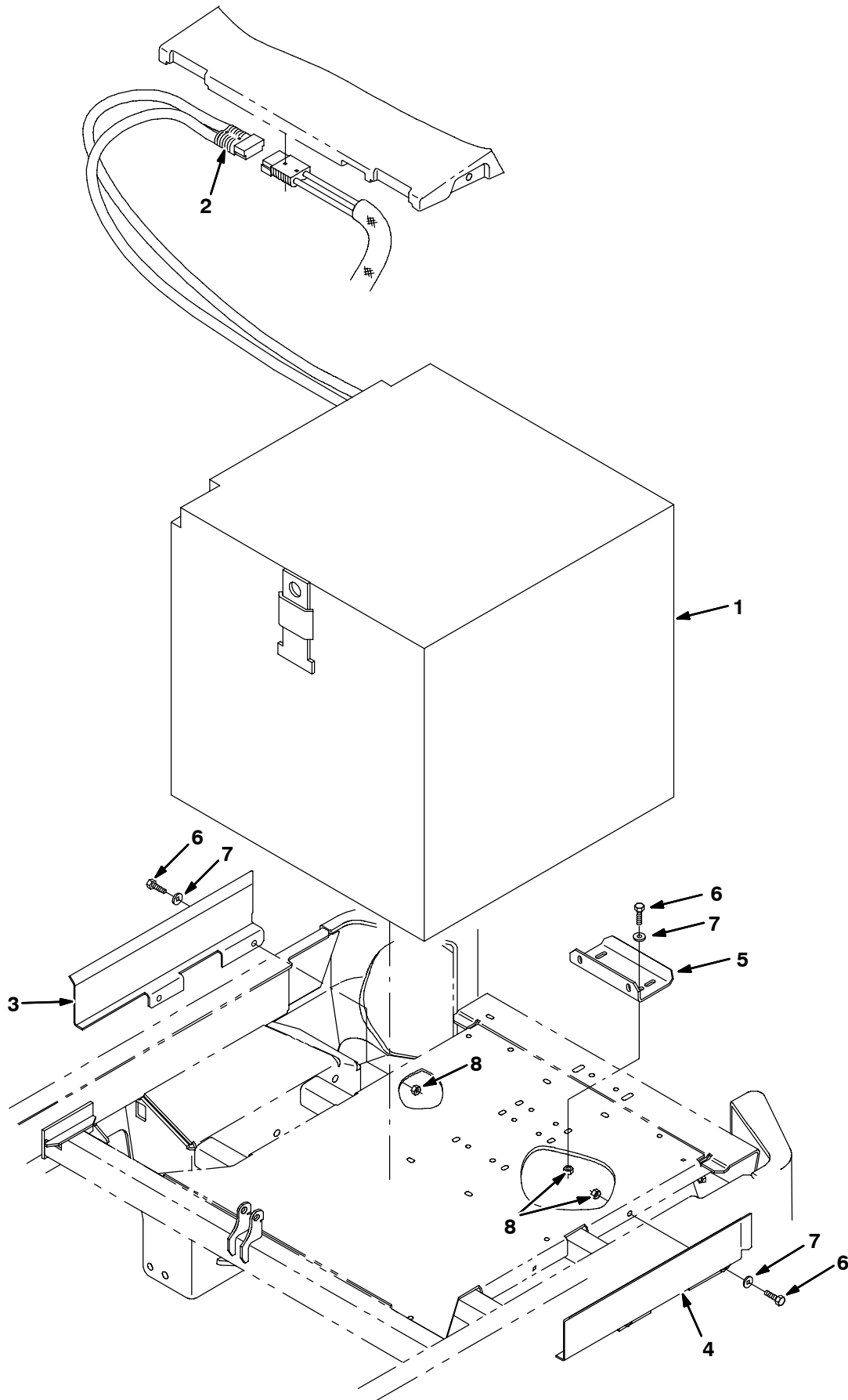
Fig. 63 - Battery Kit, 600AH
