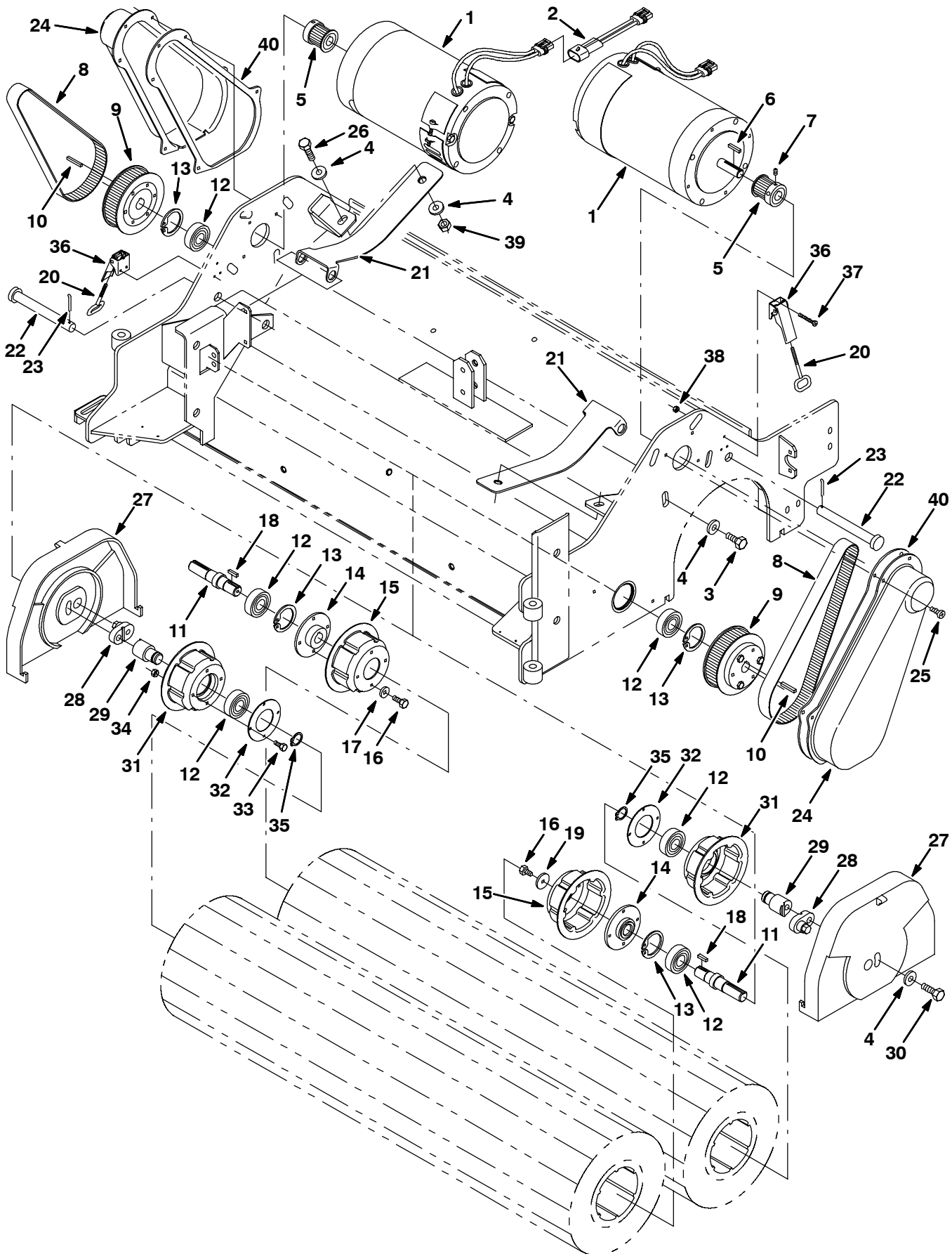
Fig. 26 - Max Pro 1000 (Cylindrical Brush) Scrub Head Drive Group
