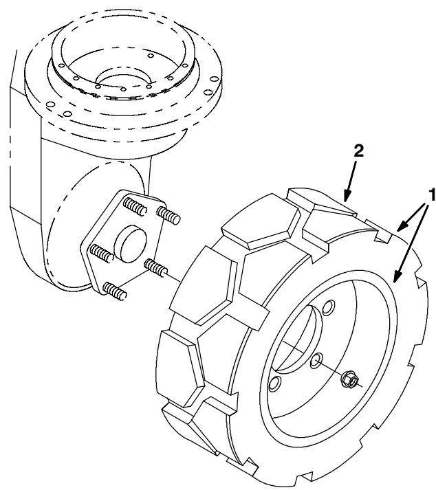
Fig. 72 - Tire, Non-Mark, Non-Skid, Front Drive
