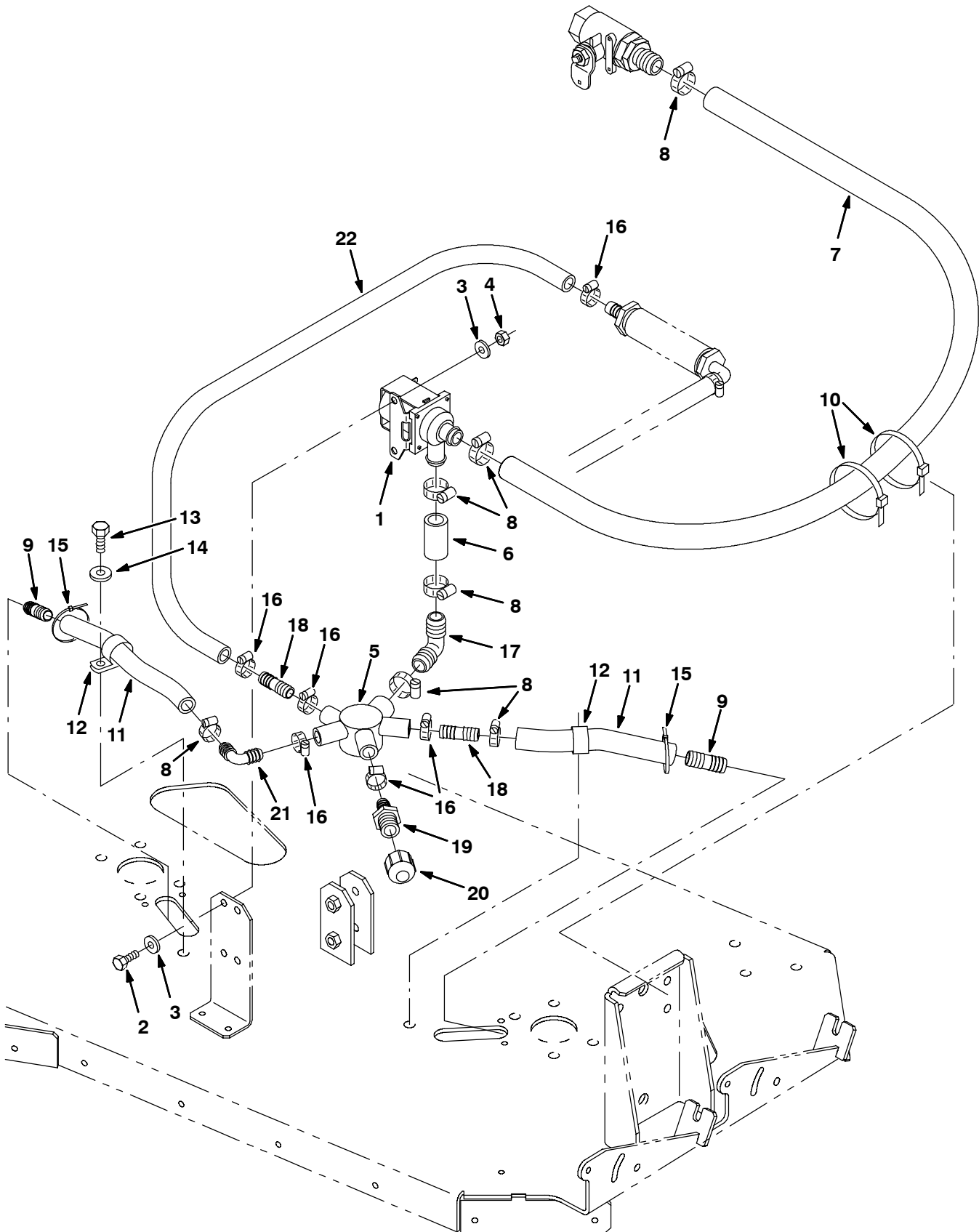
Fig. 26 - Max Pro 1000 (Disc-Brush) Solution Valve Group (FaST)
