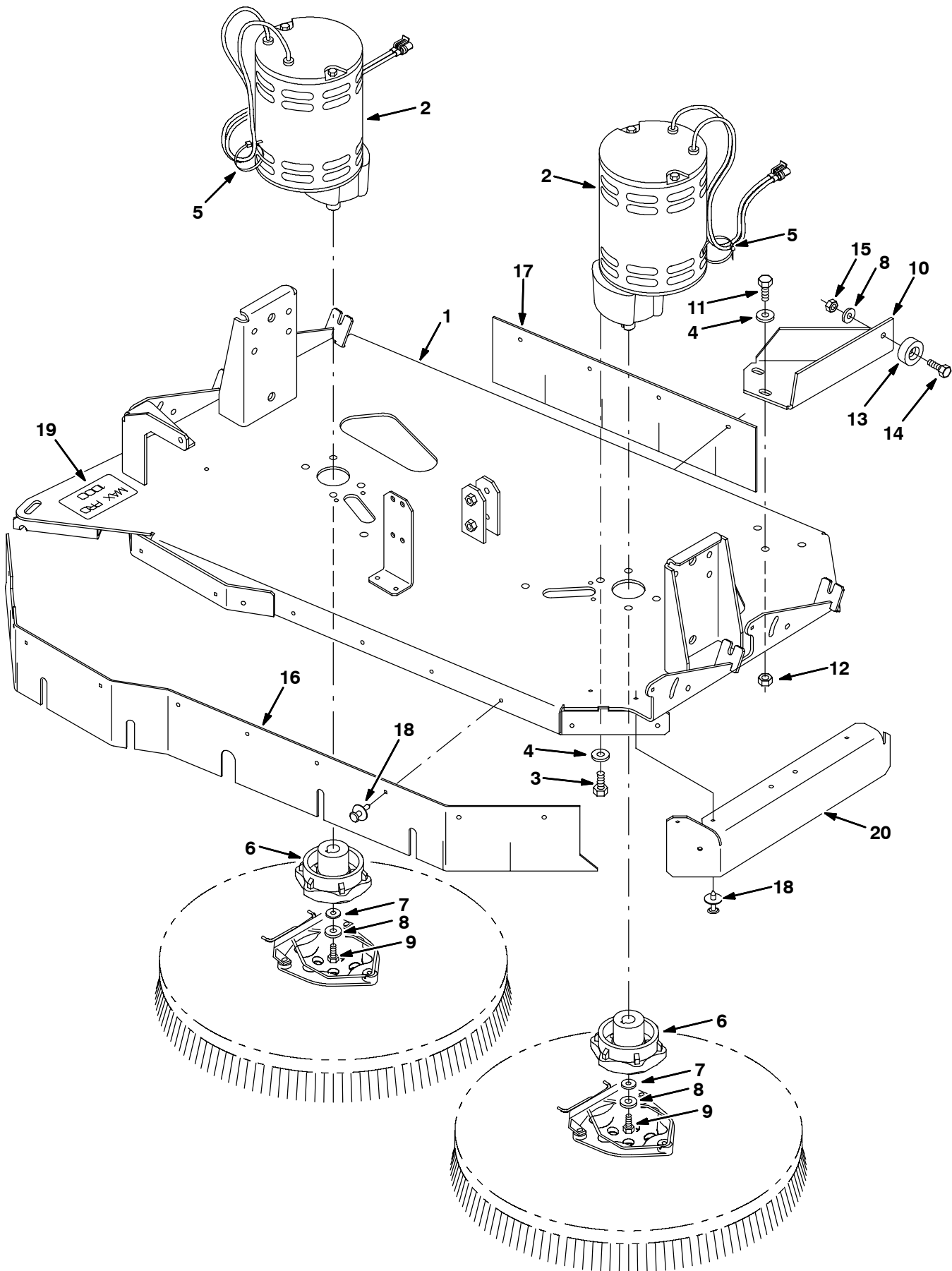
Fig. 23 - Max Pro 1000 (Disc-Brush) Scrub Head Frame Group
