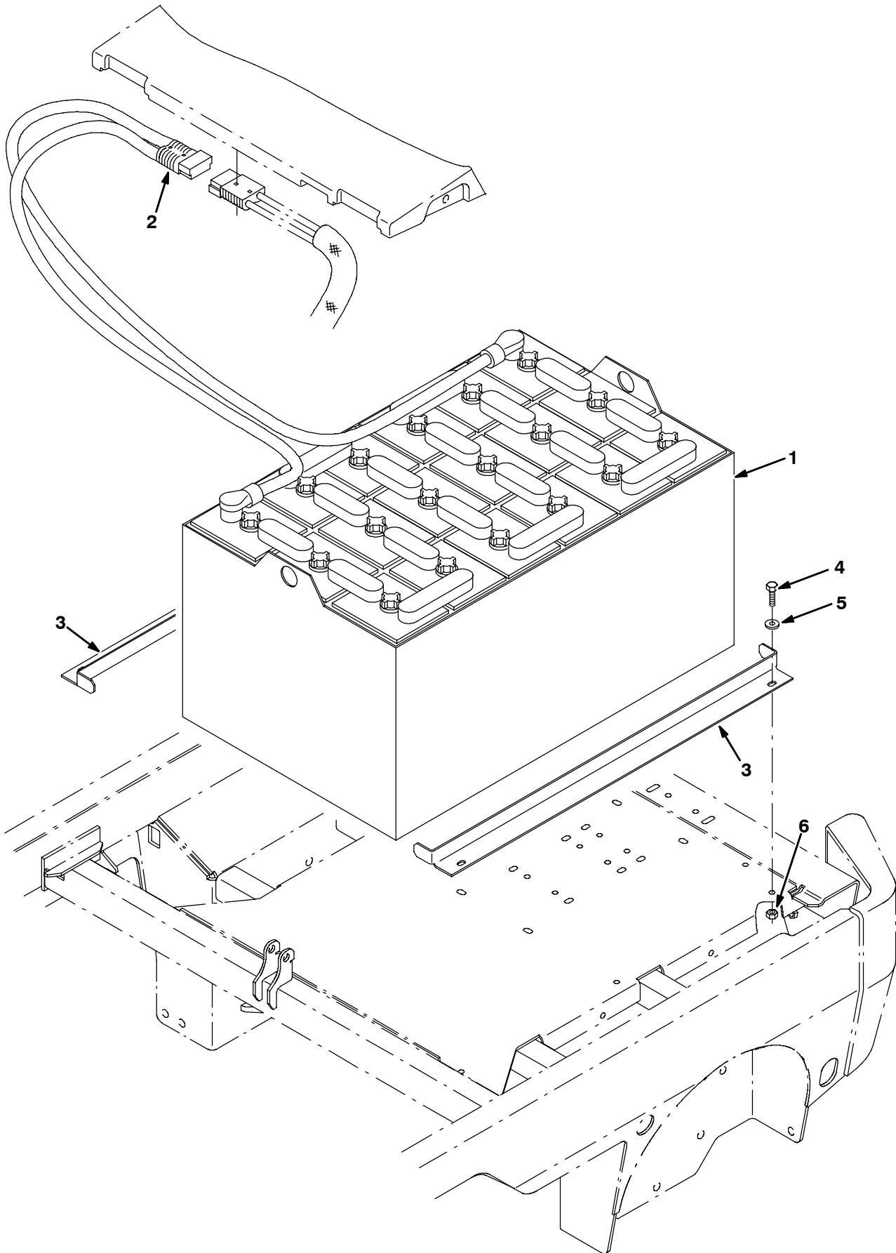
Fig. 61 - Battery Kit, 380AH Wet
