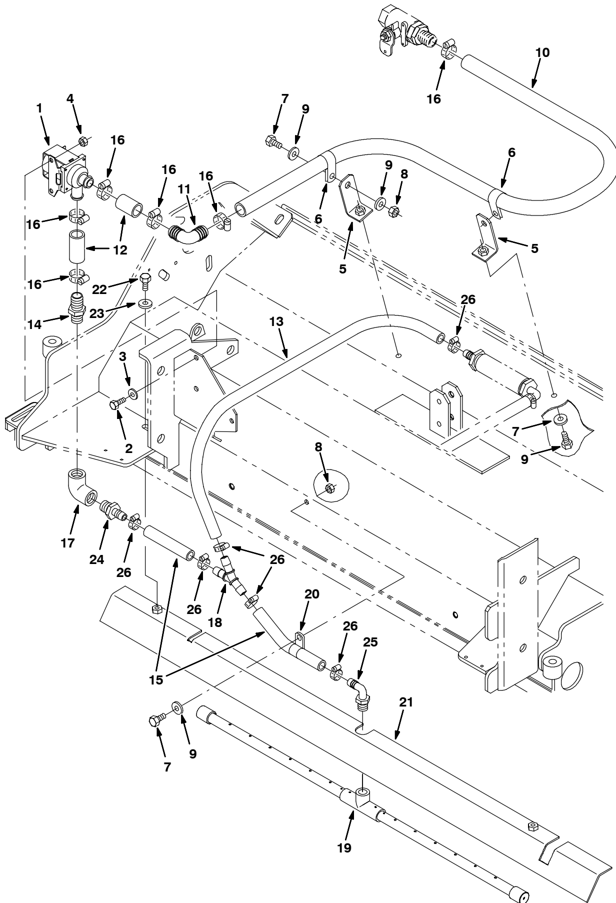
Fig. 37 - Max Pro 1200 (Cylindrical Brush) Solution Valve Group (FaST)
