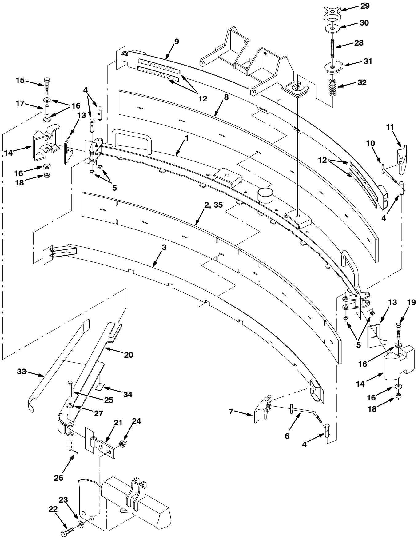
Fig. 56 - Max Pro 1200 Rear Squeegee Group (For Vacuumized Side Squeegee)
