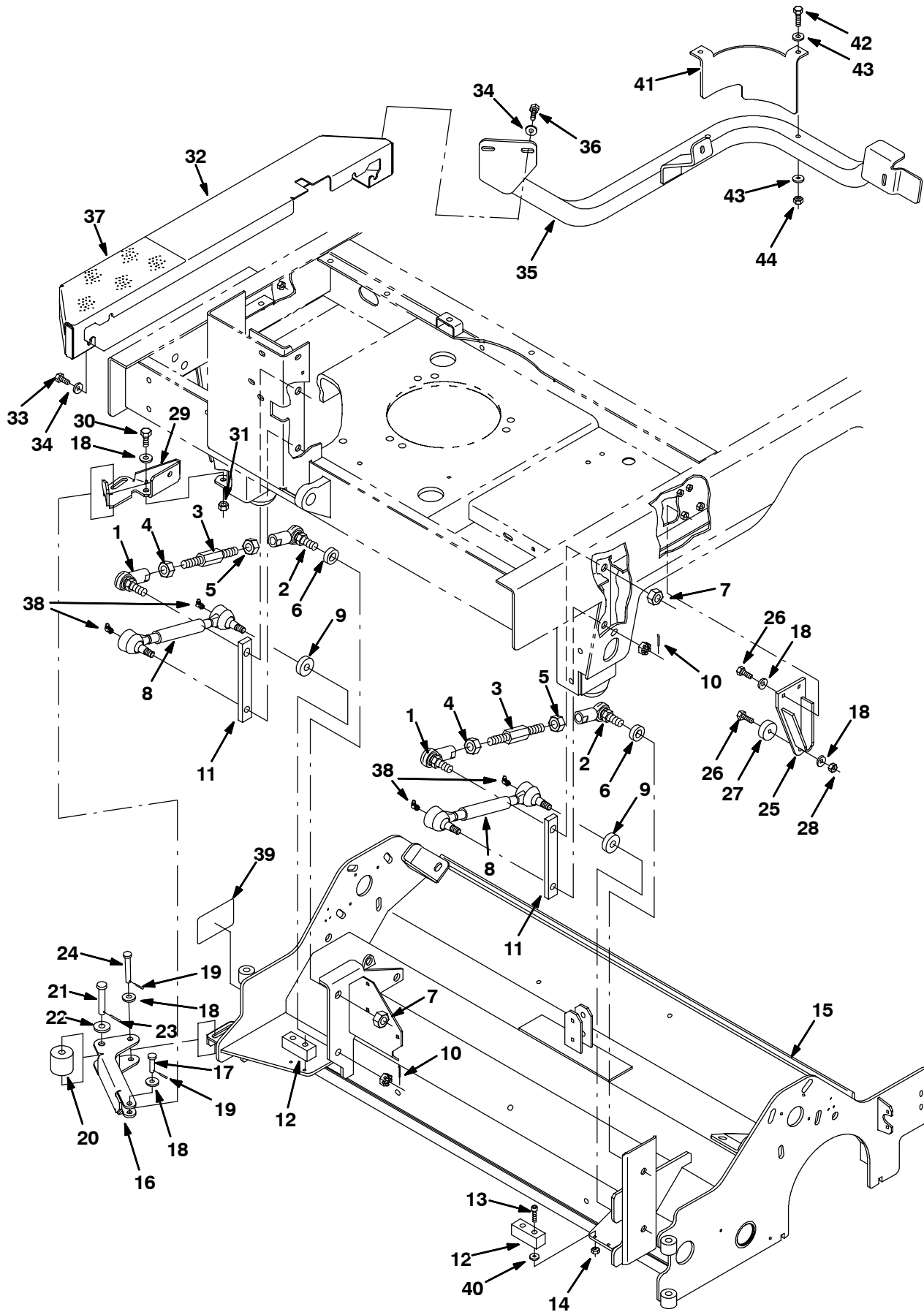
Fig. 34 - Max Pro 1200 (Cylindrical Brush) Scrub Head Frame and Linkage Group
