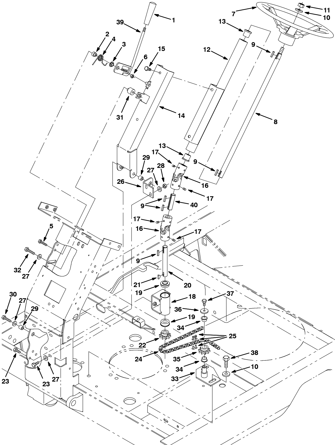
Fig. 8 - Steering Group
