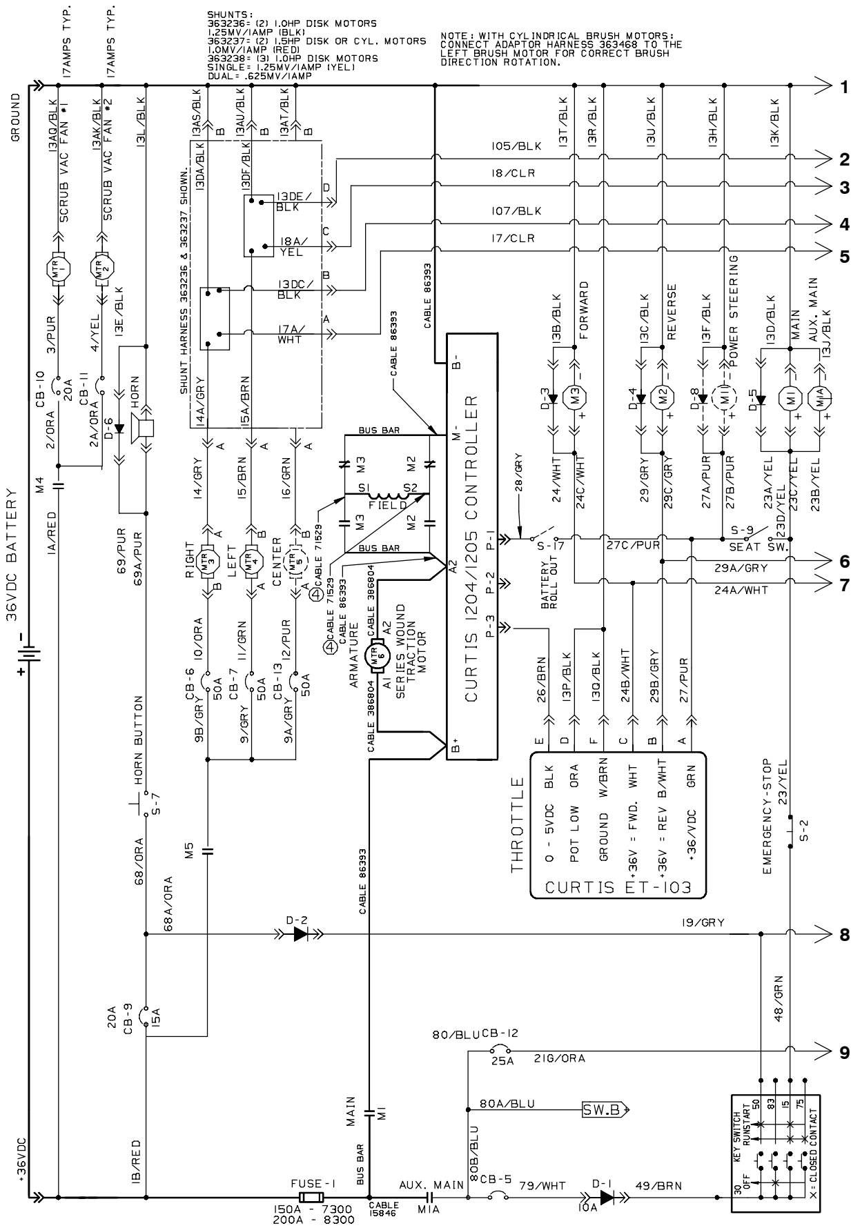
Fig. 40 - Electrical Schematic
