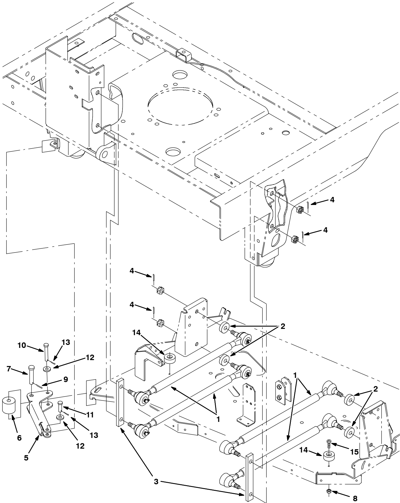
Fig. 24 - Max Pro 1000 (Disc-Brush) Scrub Head Linkage Group
