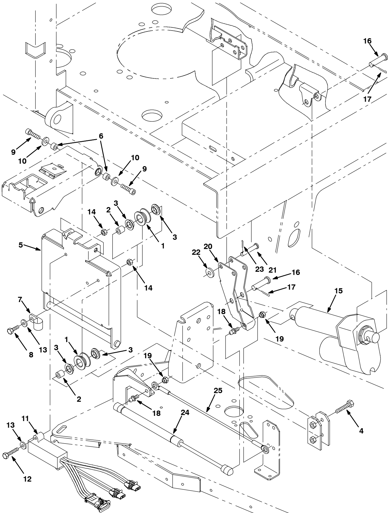
Fig. 27 - Max Pro 1000 (Disc-Brush) Edge Scrub Group
