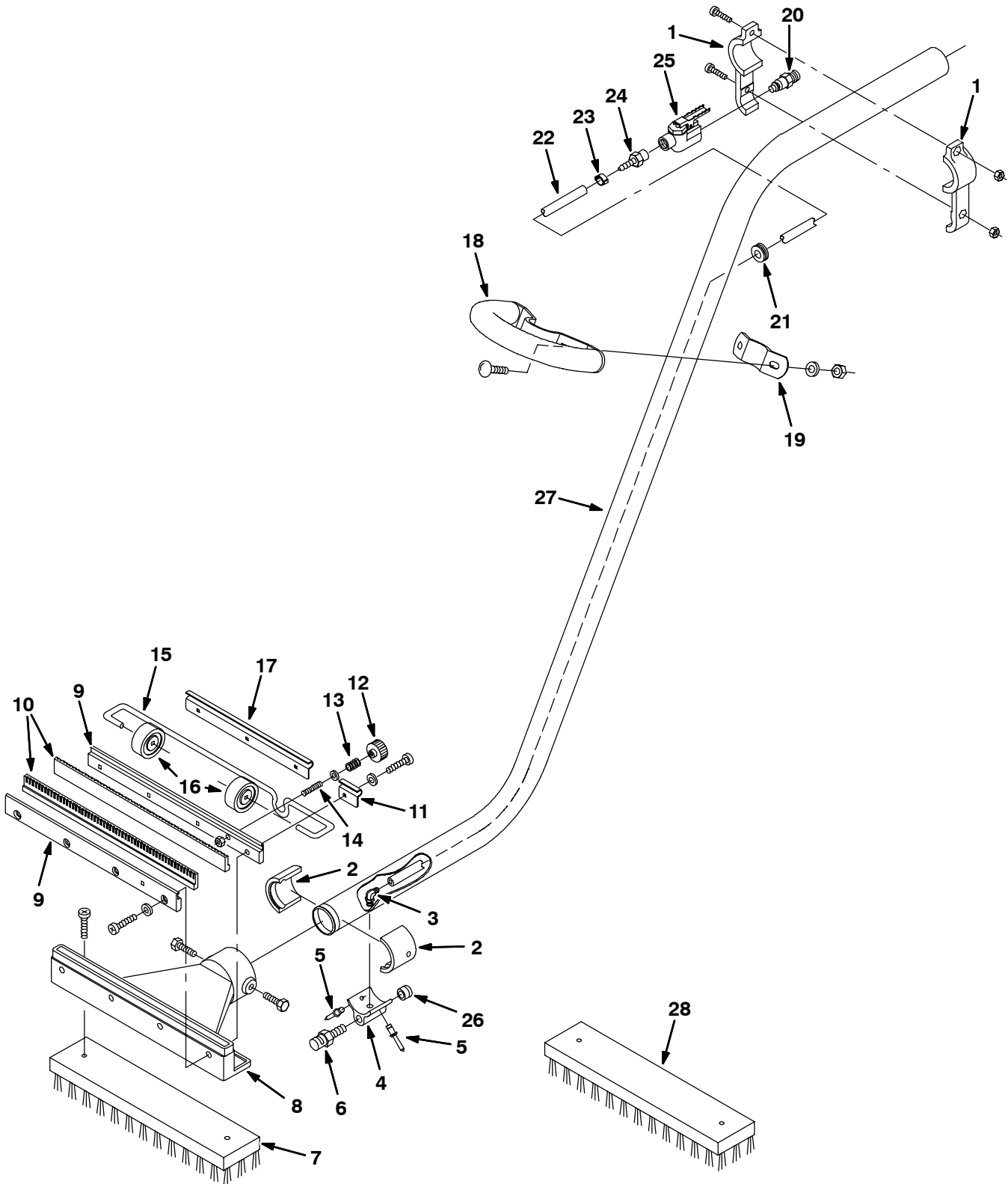
Fig. 51 - Power Wand Assembly
