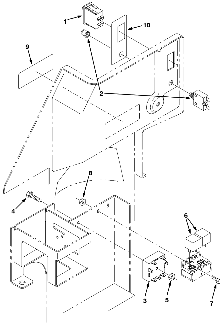
Fig. 39 - Electrical Group, FaST
