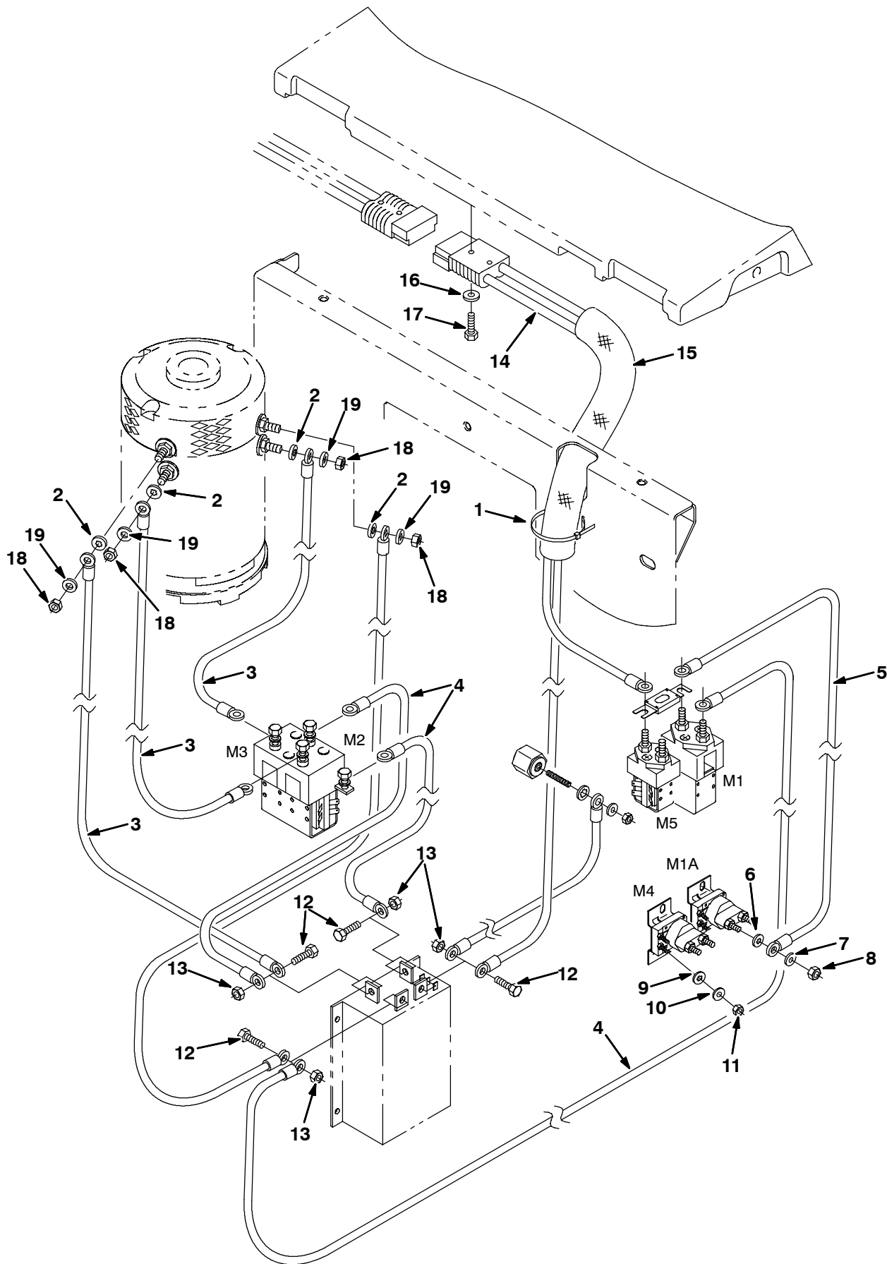
Fig. 37 - Eleectrical Control Box Wires Group (001706- )
