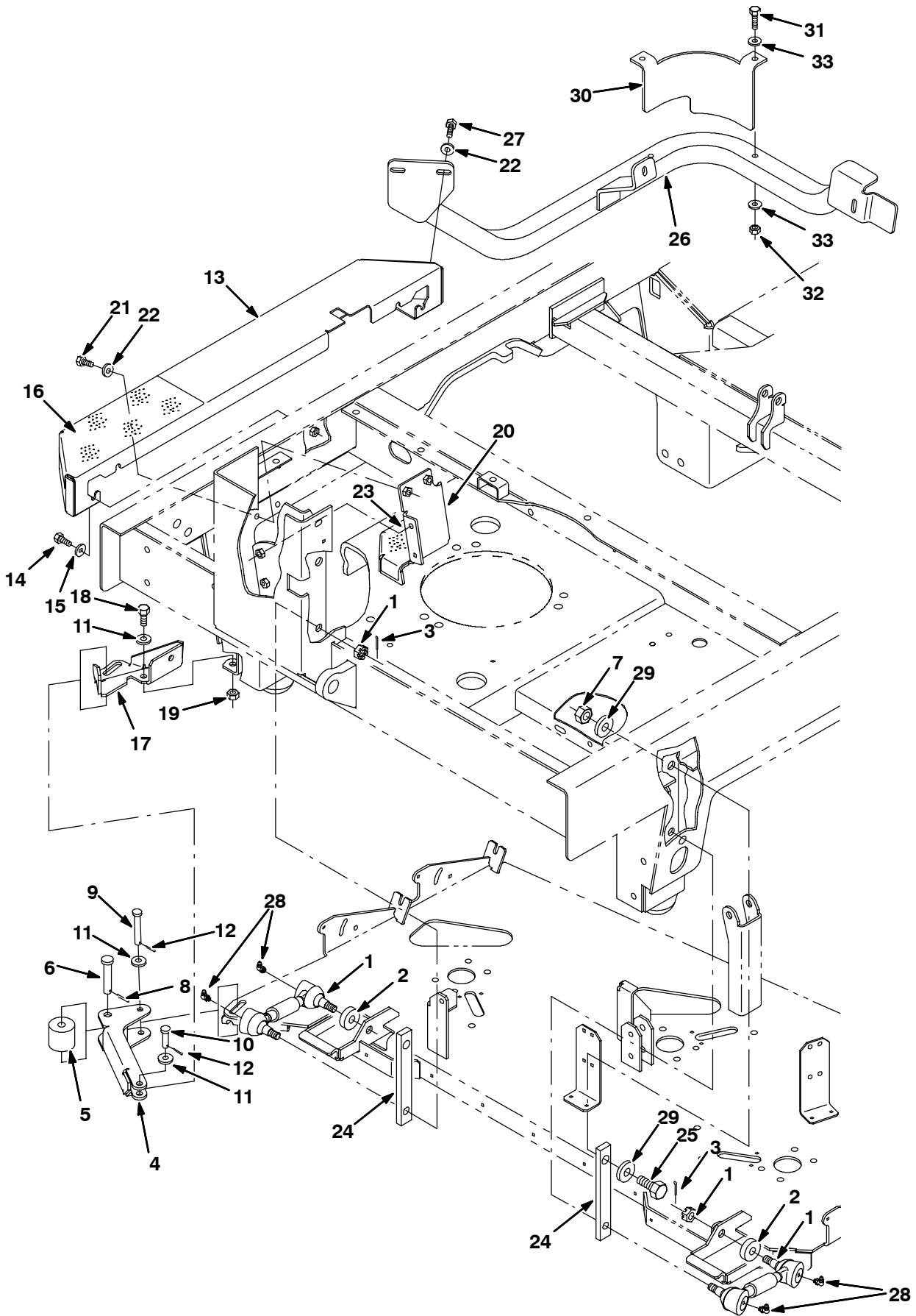
Fig. 18 - Max Pro 1200 (Disc-Brush) Scrub Head Linkage Group
