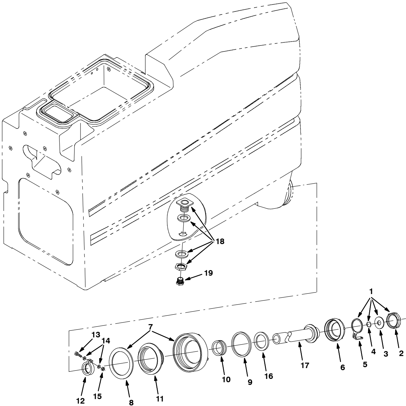
Fig. 20 - Recovery Tank Drain Assembly
