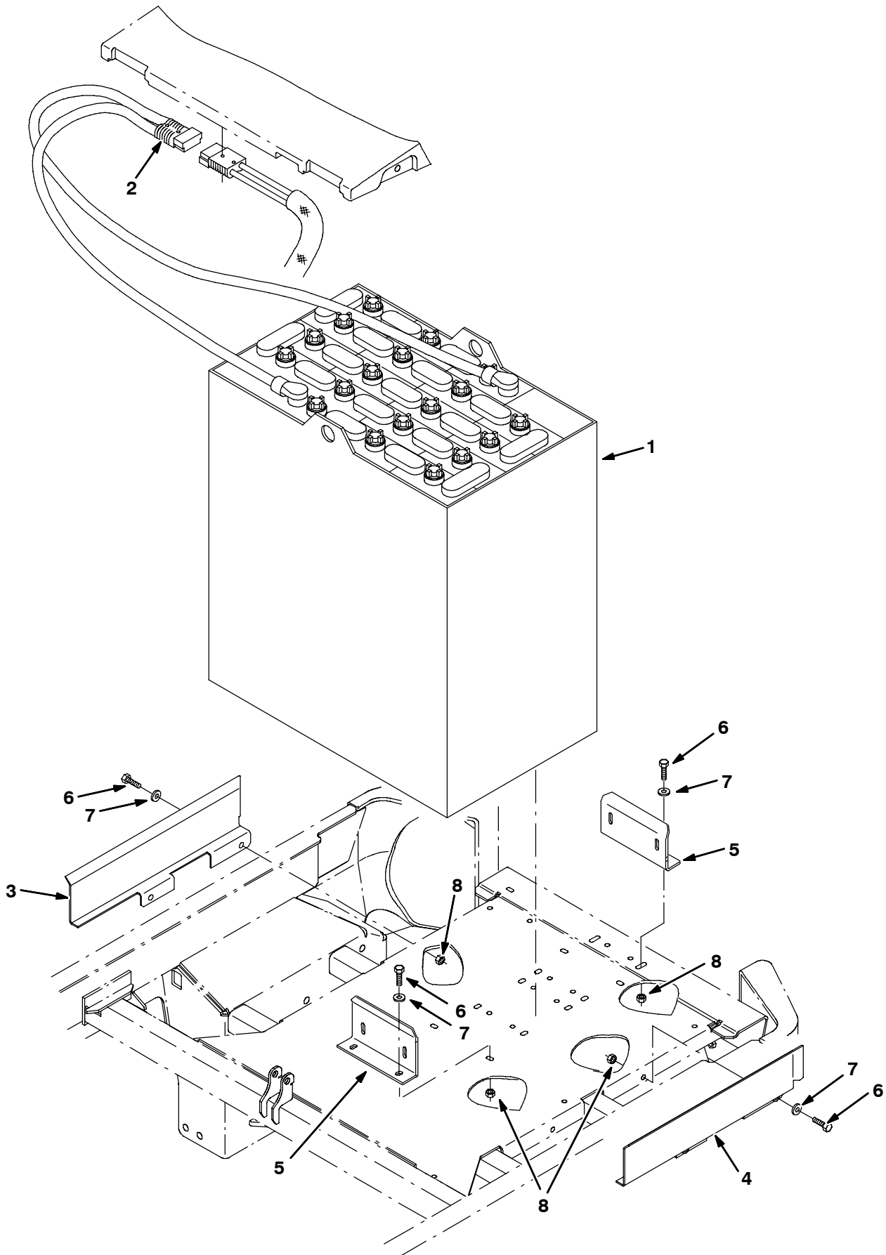
Fig. 62 - Battery Kit, 500AH Wet
