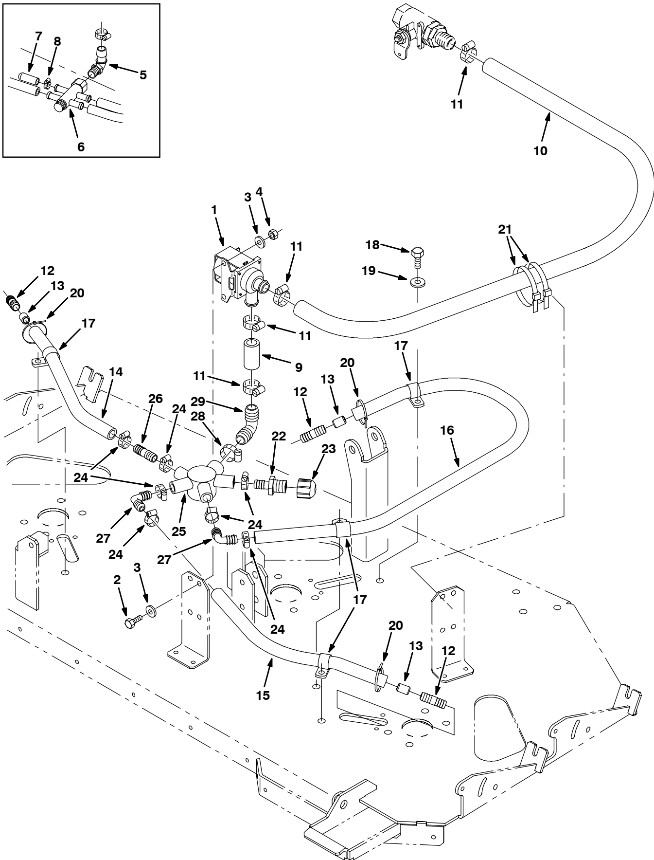
Fig. 19 - Max Pro 1200 (Disc-Brush) Solution Valve Group (Non FaST)
