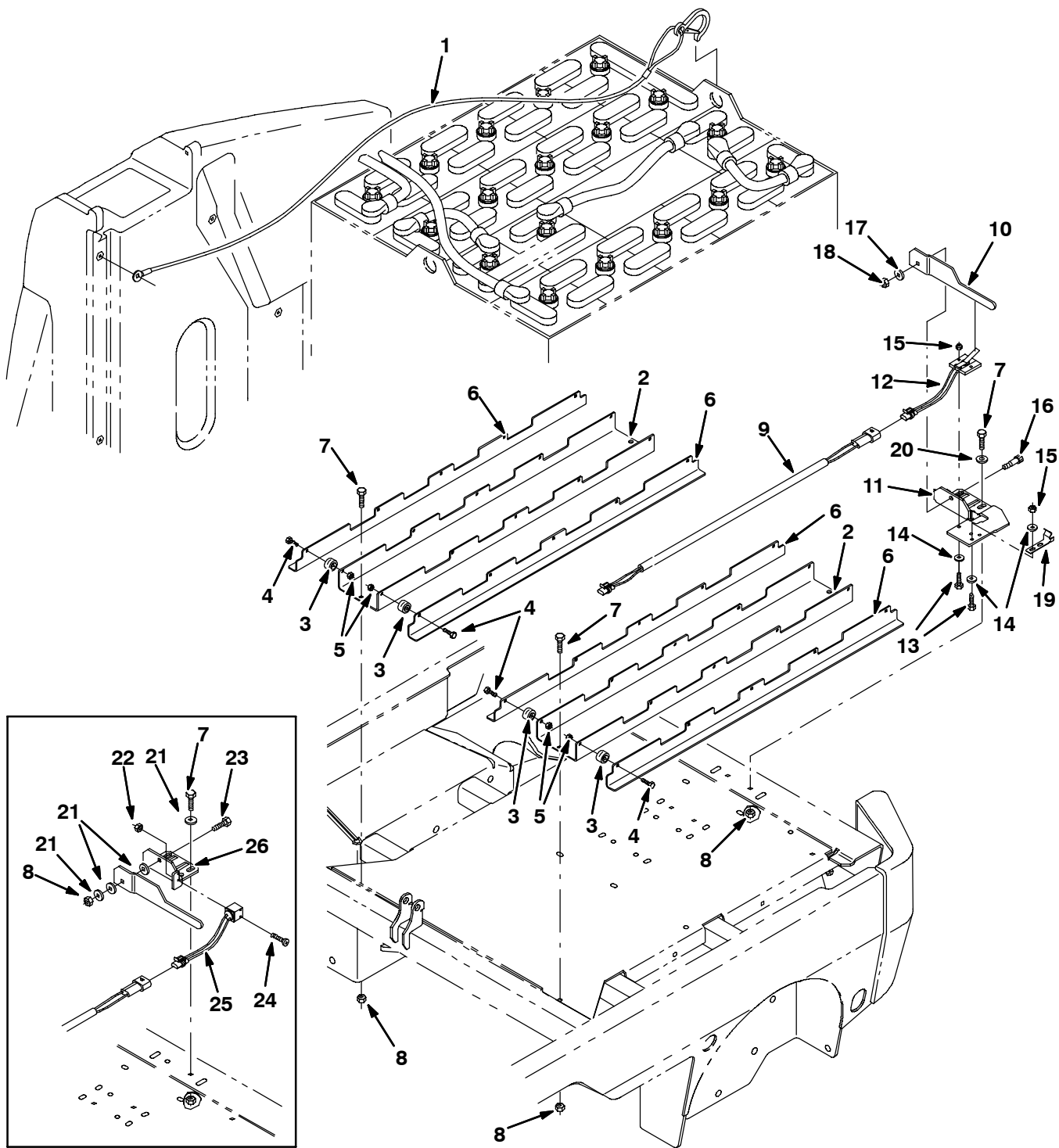
Fig. 59 - Battery Rollout Kit
