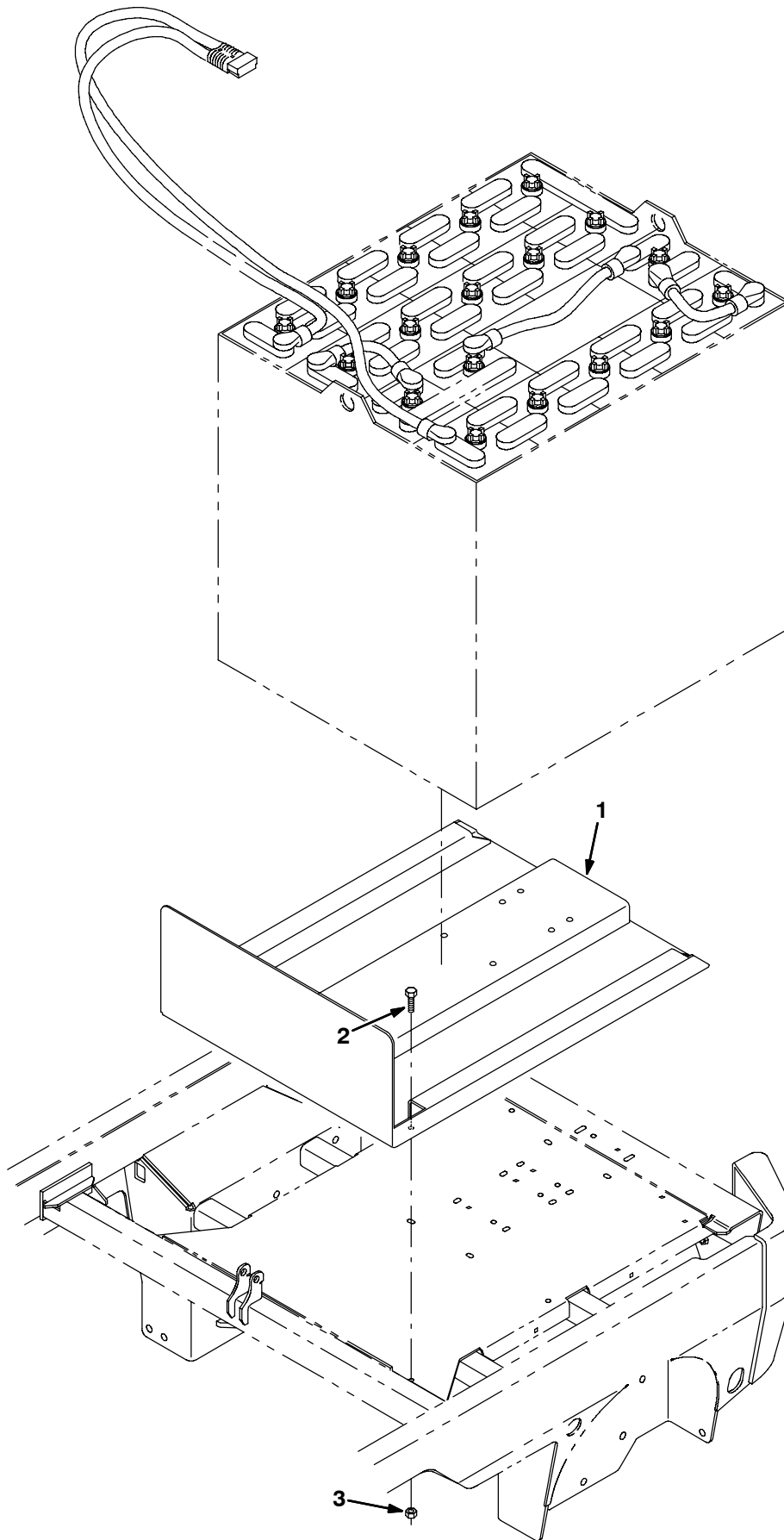
Fig. 60 - Battery Forklift Kit
