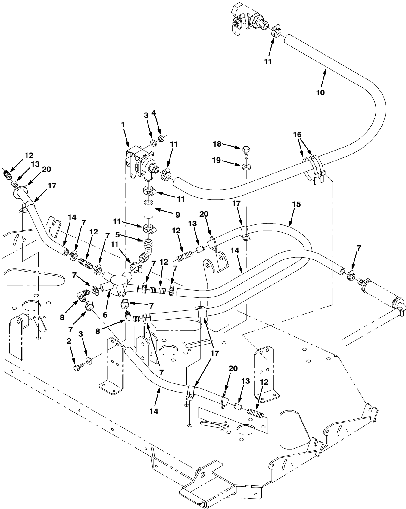
Fig. 20 - Max Pro 1200 (Disc-Brush) Solution Valve Group (FaST)
