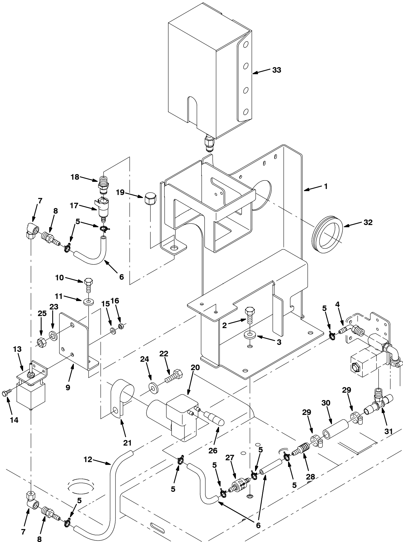
Fig. 16 - FaST Air Pump and Detergent Group
