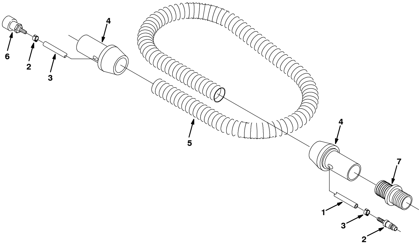
Fig. 50 - Power Wand Hose Assembly
