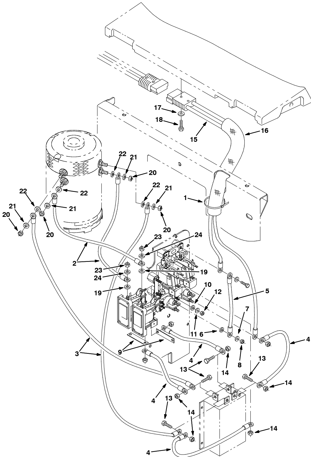
Fig. 36 - Electrical Control Box Wires Group (000000- 001705)
