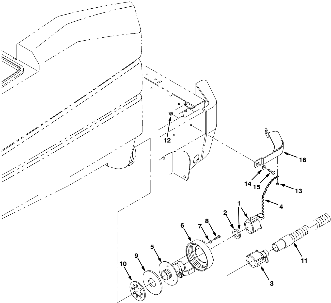
Fig. 46 - Positive Solution Control Drain Kit, Recovery Tank
