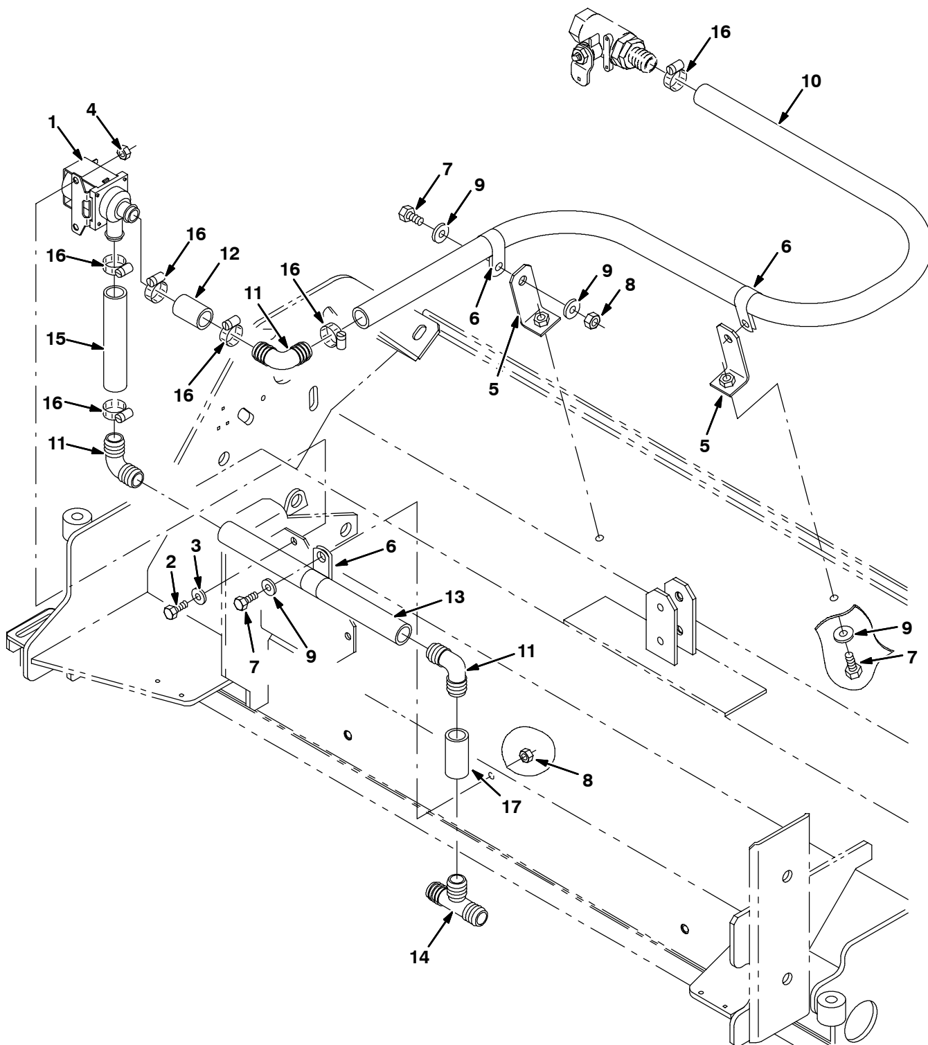
Fig. 36 - Max Pro 1200 (Cylindrical Brush) Solution Valve Group (Non FaST)
