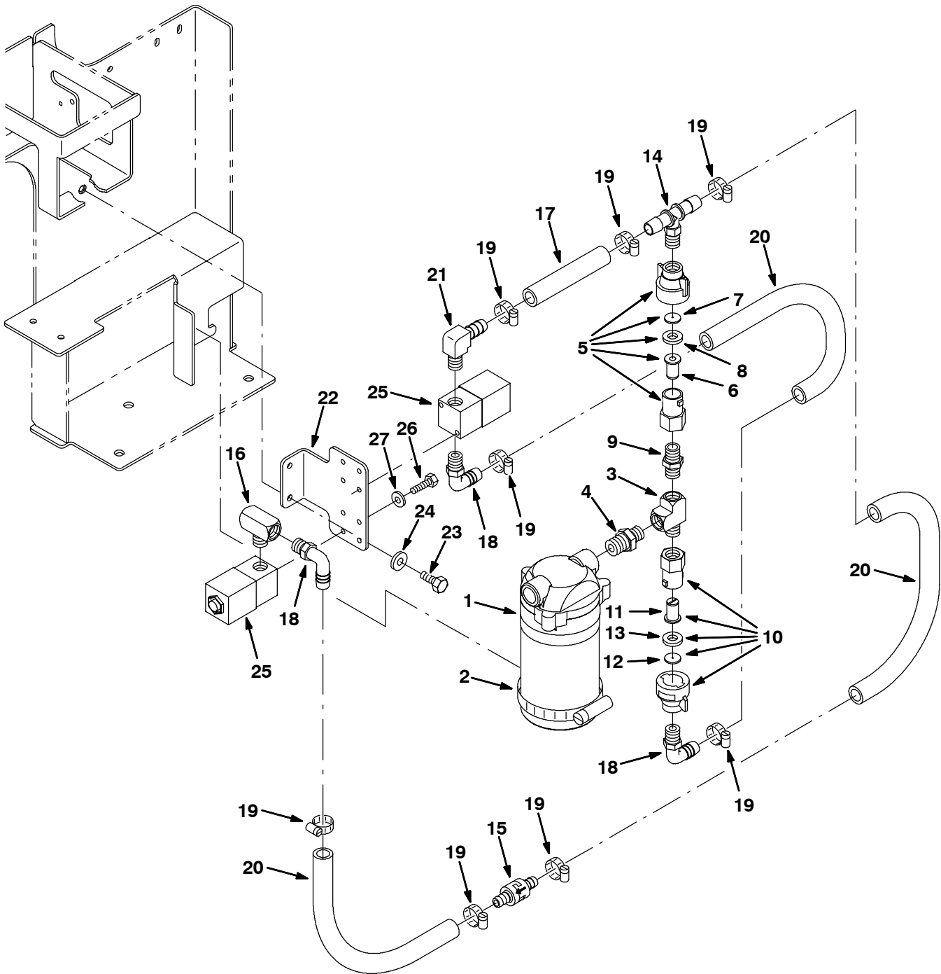
Fig. 15 - FaST Solution Pump Group
