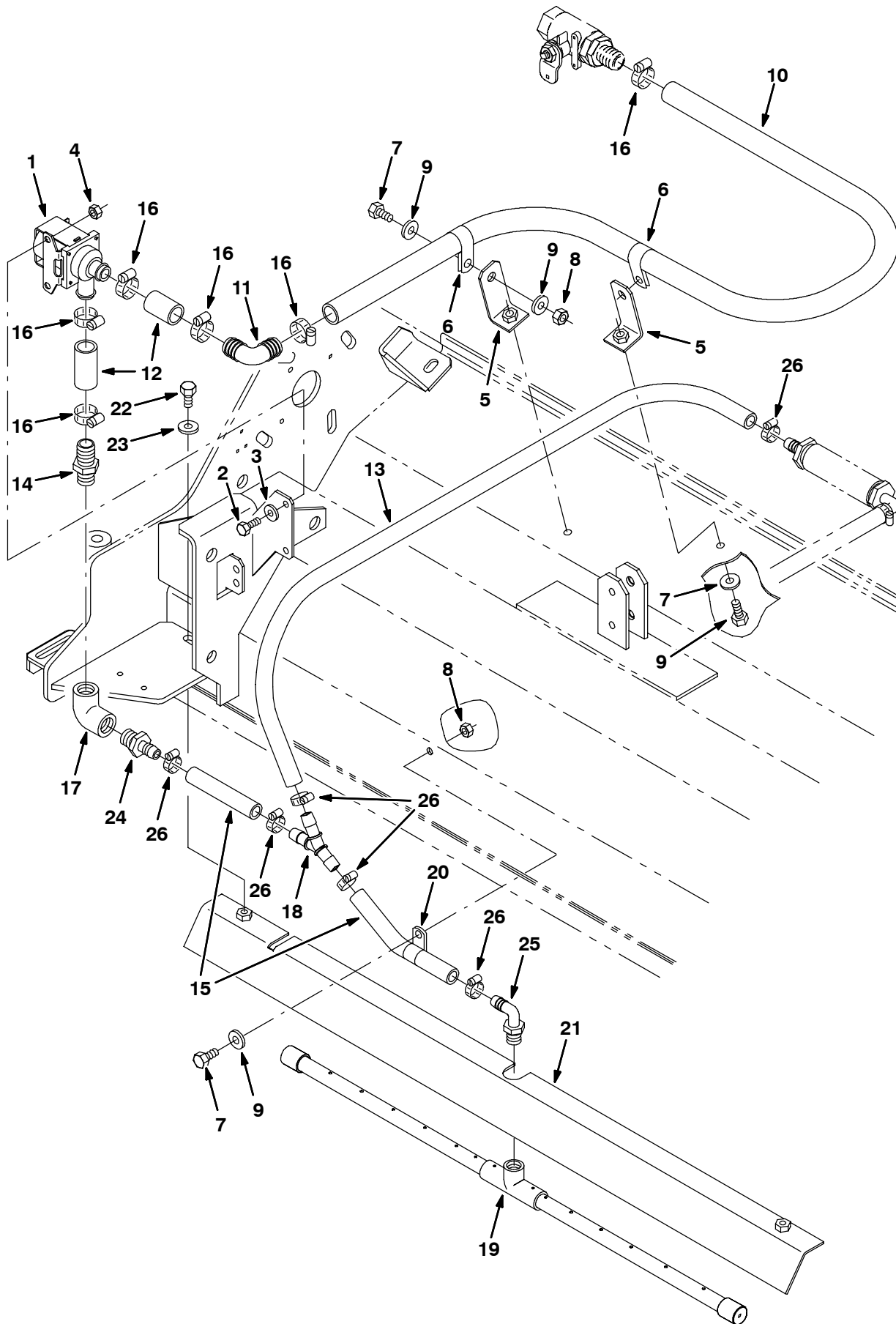
Fig. 28 - Max Pro 1000 (Cylindrical Brush) Solution Valve Group (FaST)
