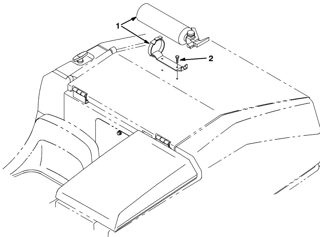
Fig. 74 - Fire Extinguisher Kit
