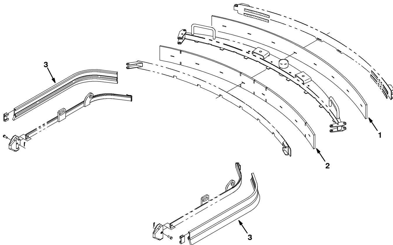
Fig. 58 - Max Pro 1200 Urethane Squeegee Kit
