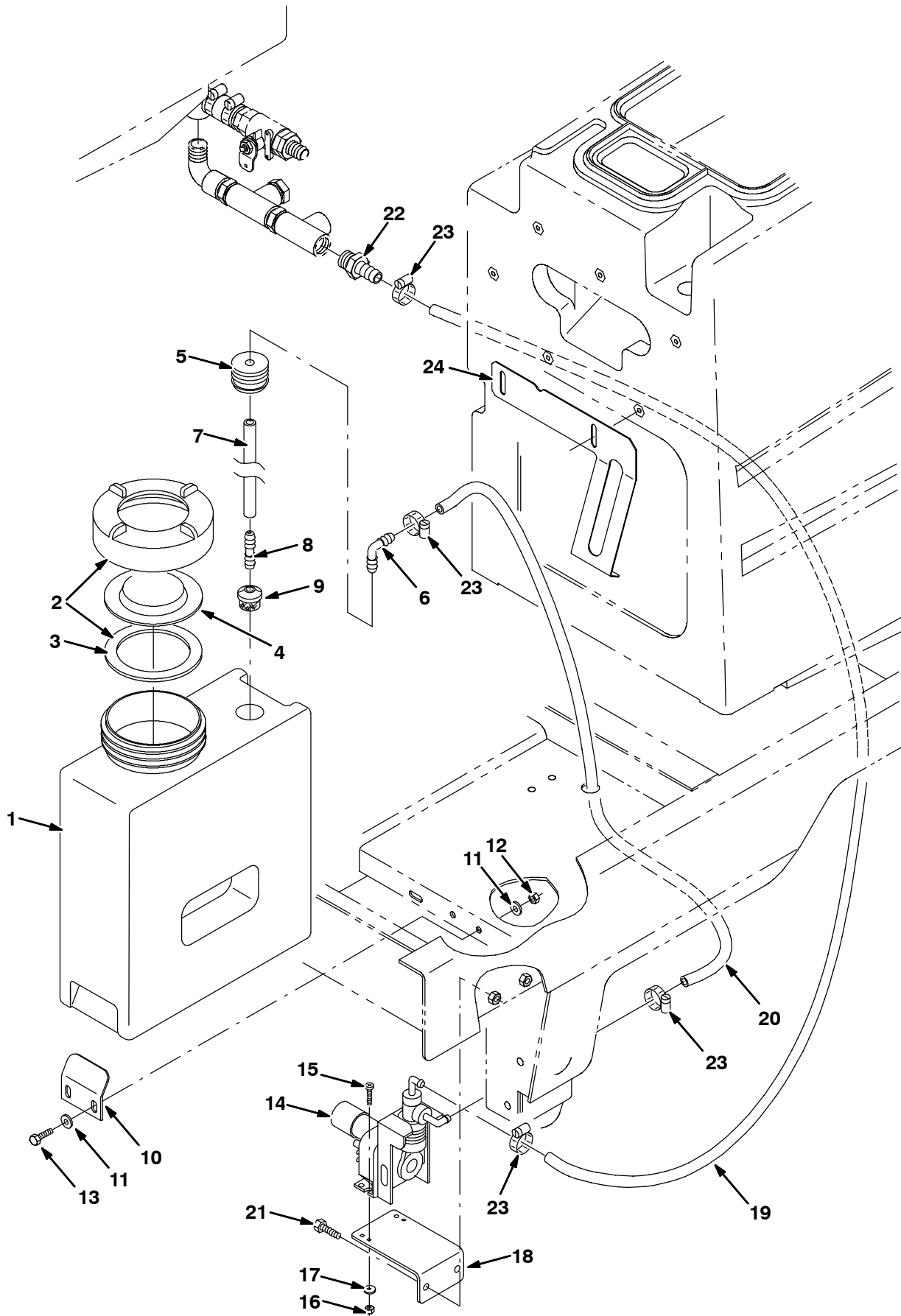
Fig. 49 - Detergent Metering Kit
