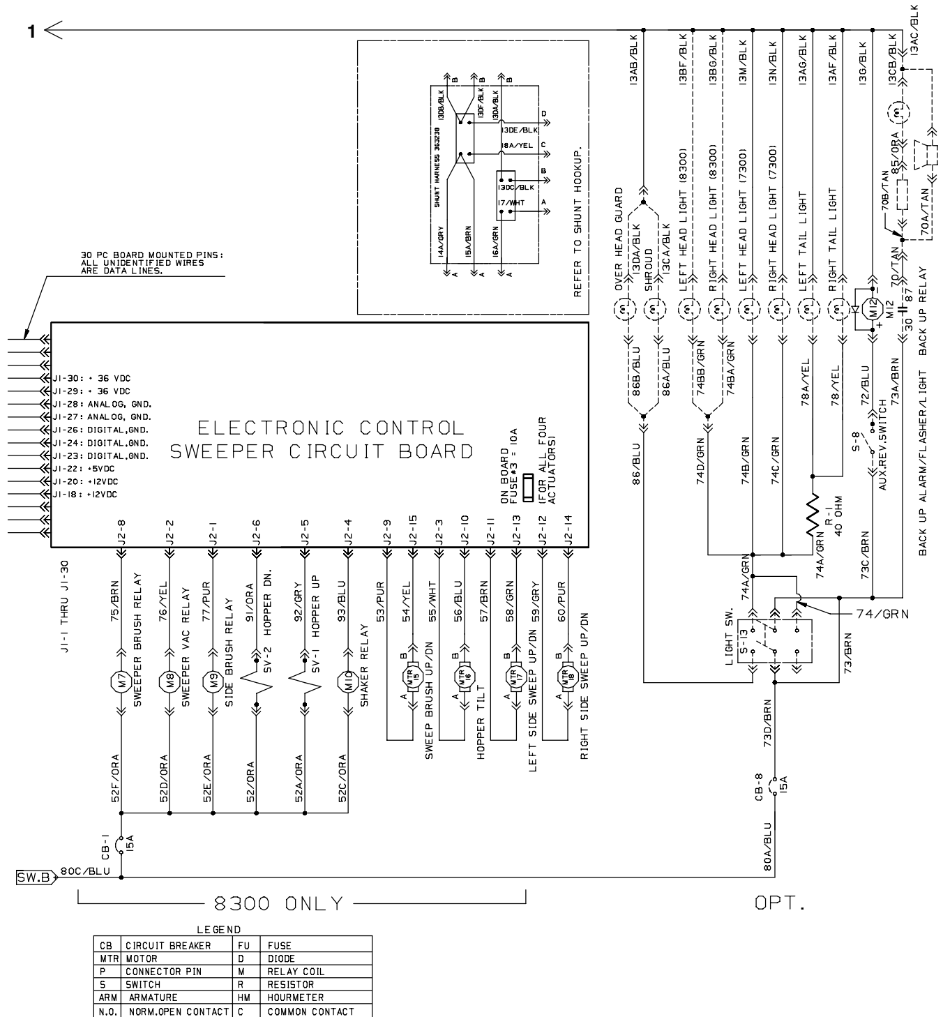
Fig. 40 - Electrical Schematic
