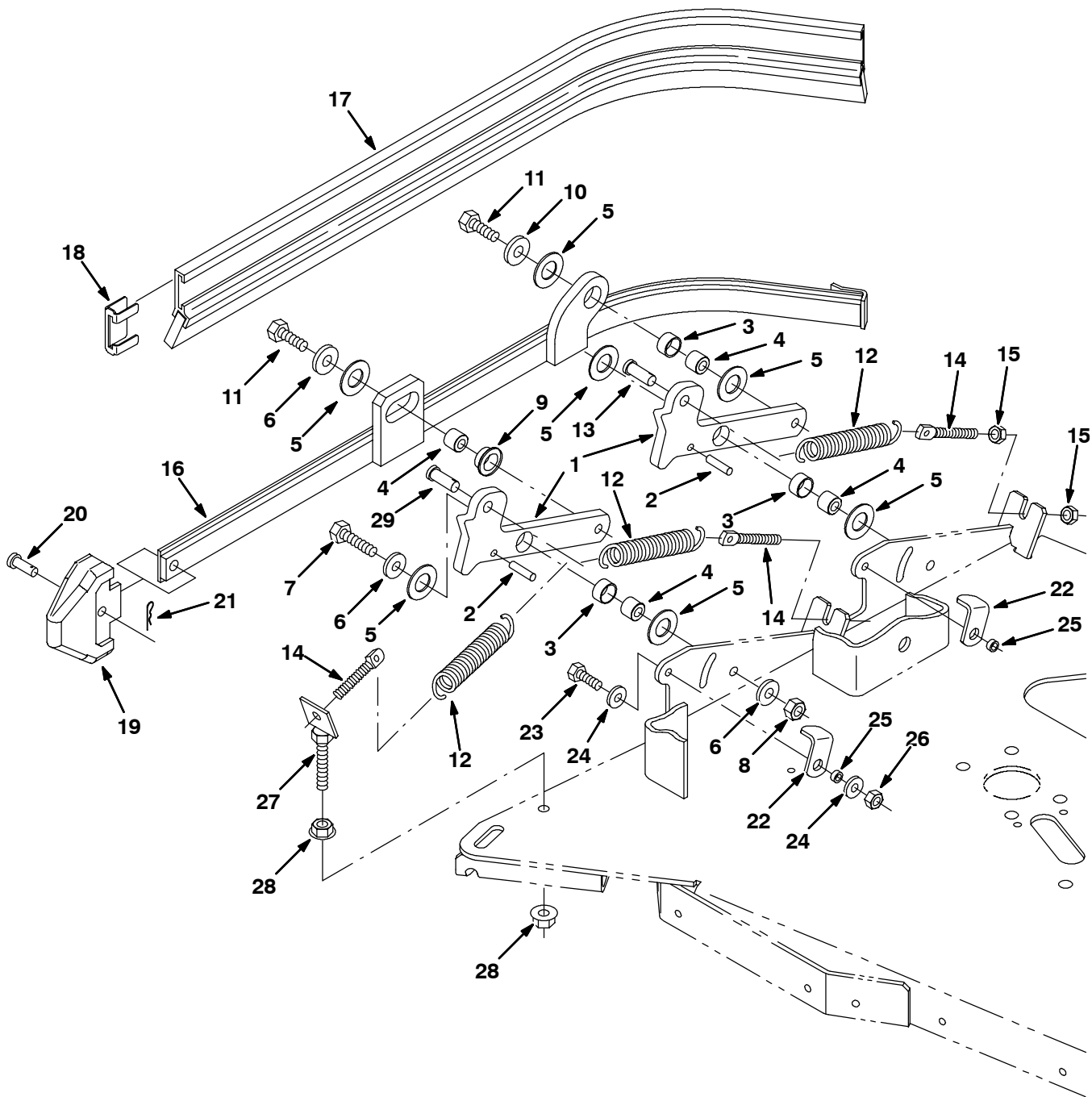
Fig. 28 - Max Pro 1000 (Disc-Brush) Right Side Squeegee Group
