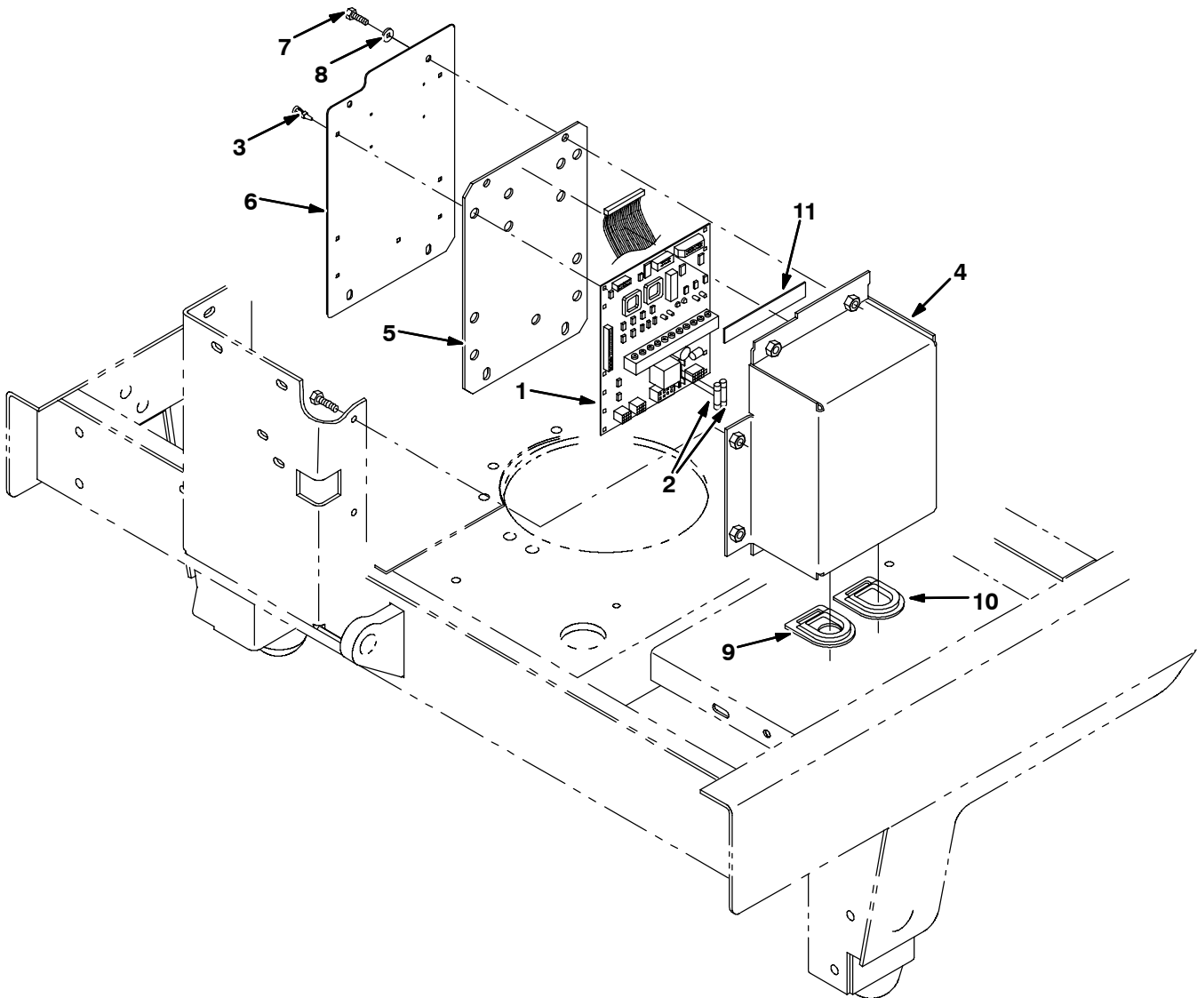
Fig. 38 - Electrical Circuit Board Group
