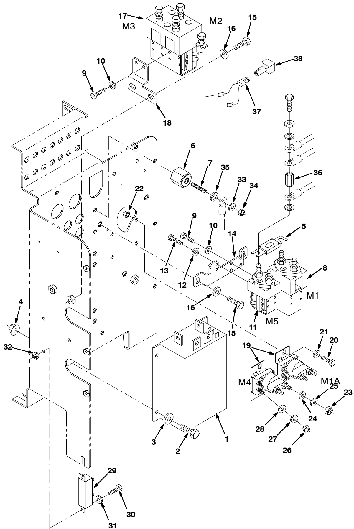
Fig. 35 - Electrical Control Box Contactor Group (001706- )
