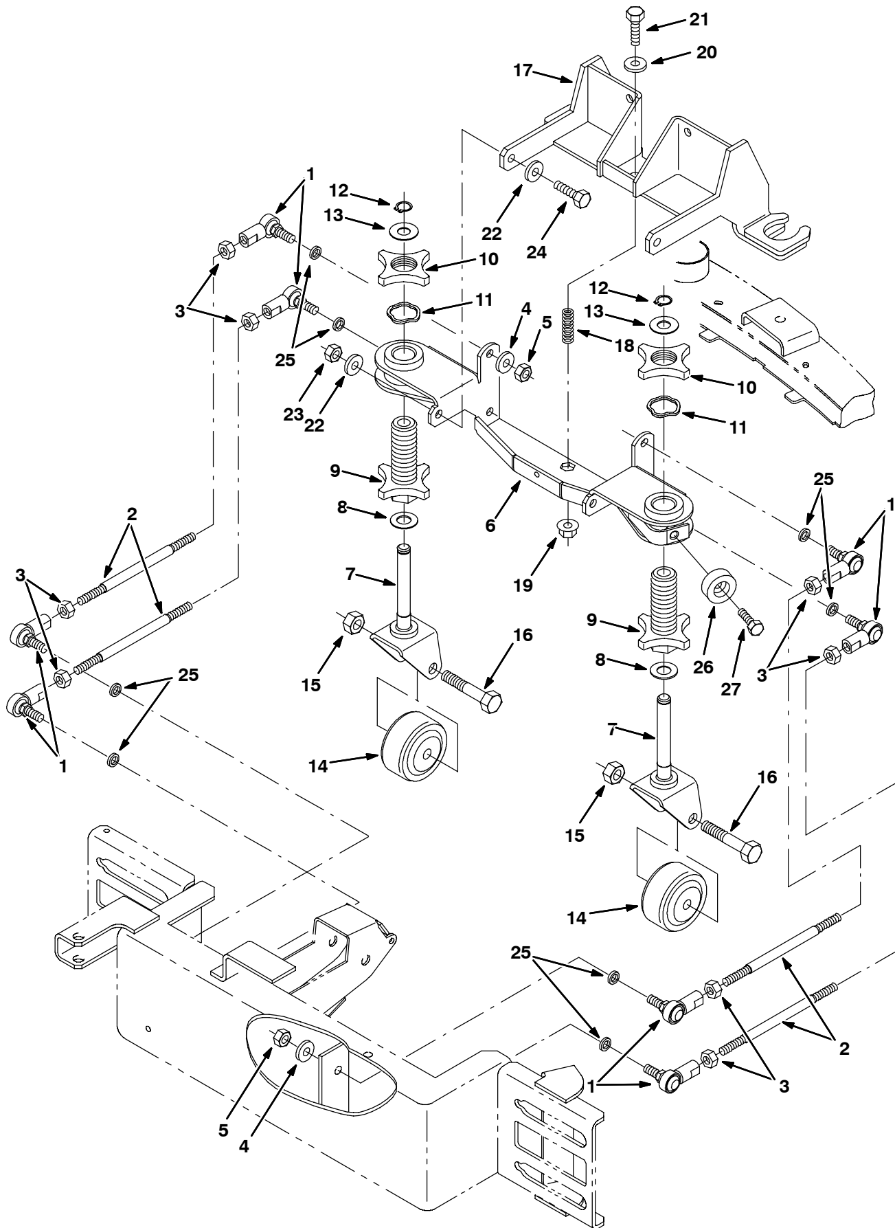
Fig. 30 - Squeegee Linkage Group, Rear
