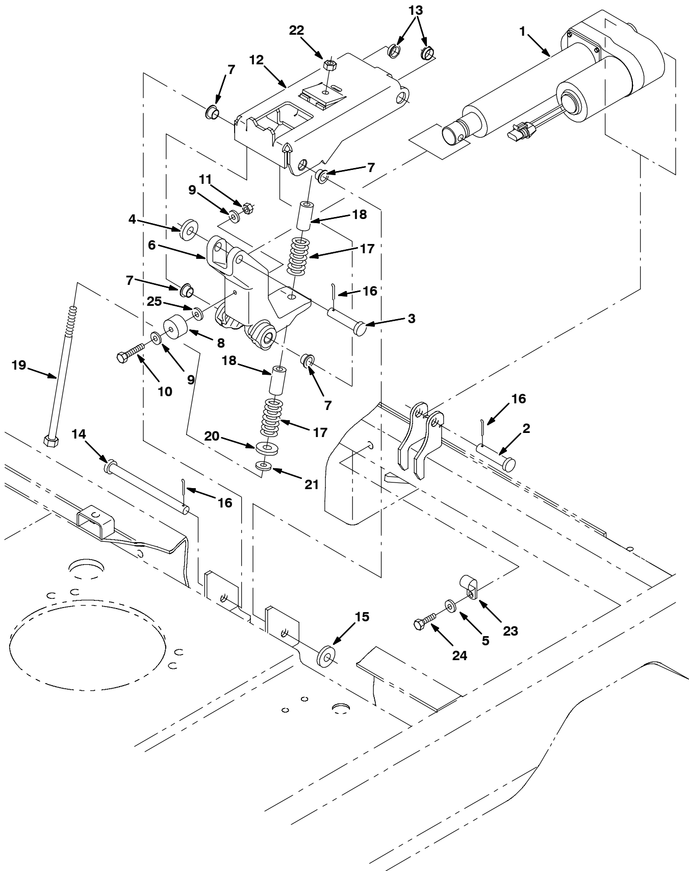
Fig. 22 - Scrub Head Lift Group
