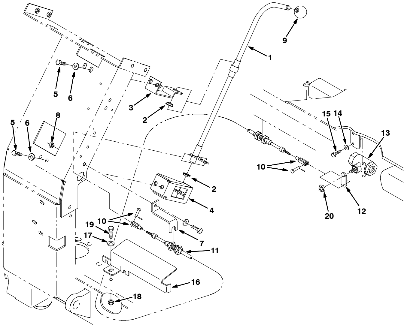
Fig. 18 - Solution Control Group
