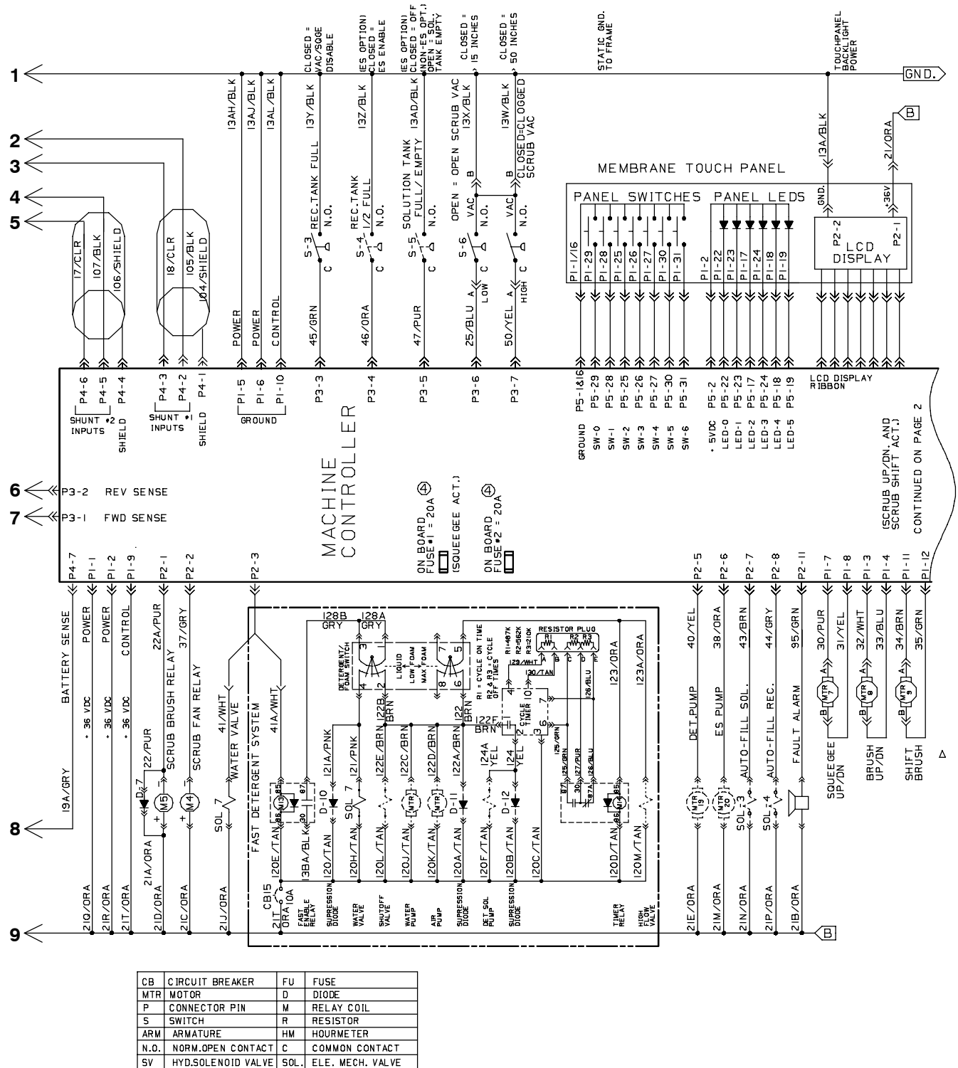
Fig. 40 - Electrical Schematic
