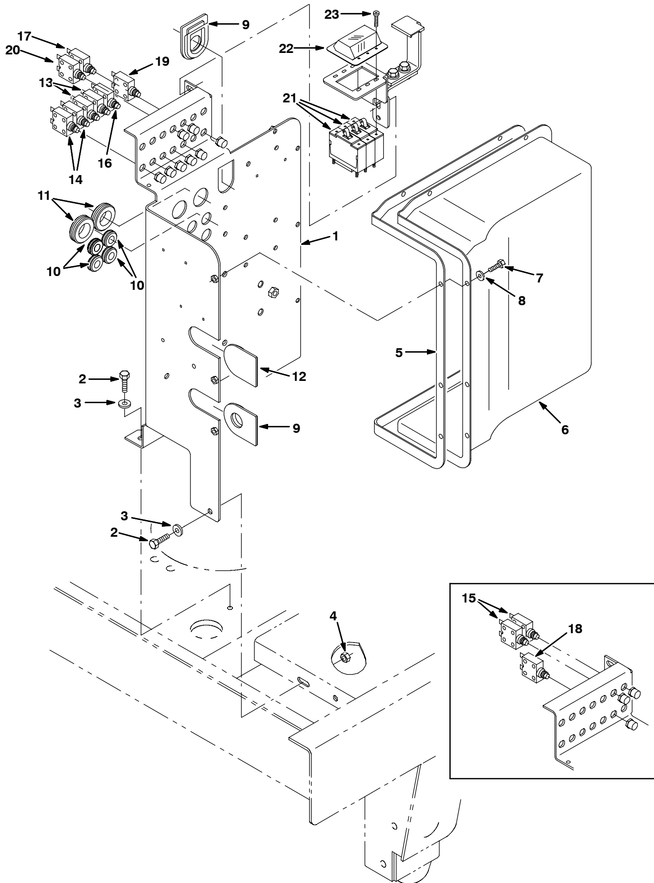
Fig. 33 - Electrical Control Box Circuit Breaker Group
