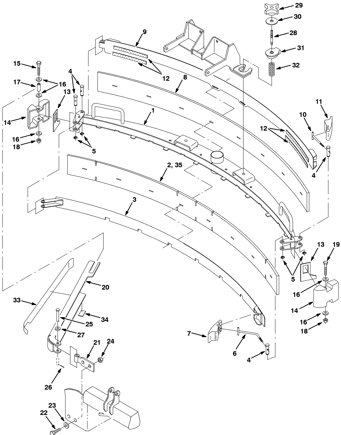
Fig. 32 - Max Pro 1000 Rear Squeegee Group
