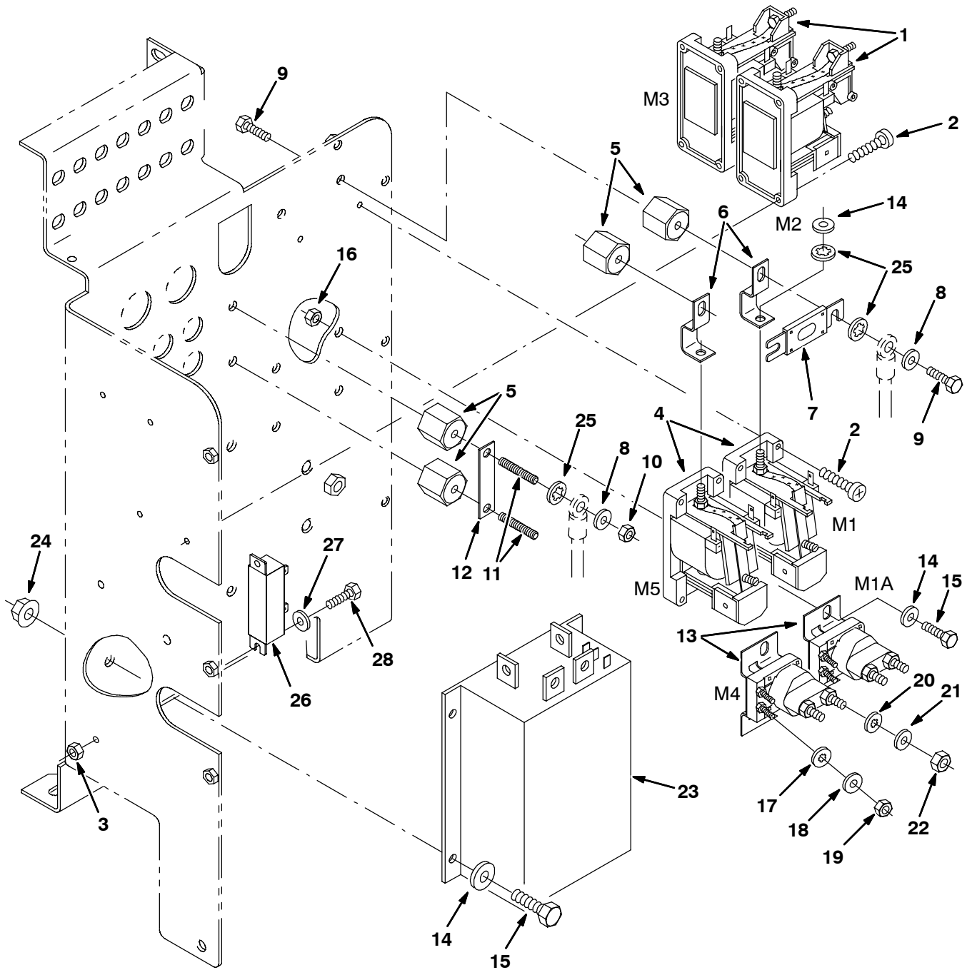
Fig. 34 - Electrical Control Box Contactor Group (000000- 001705)
