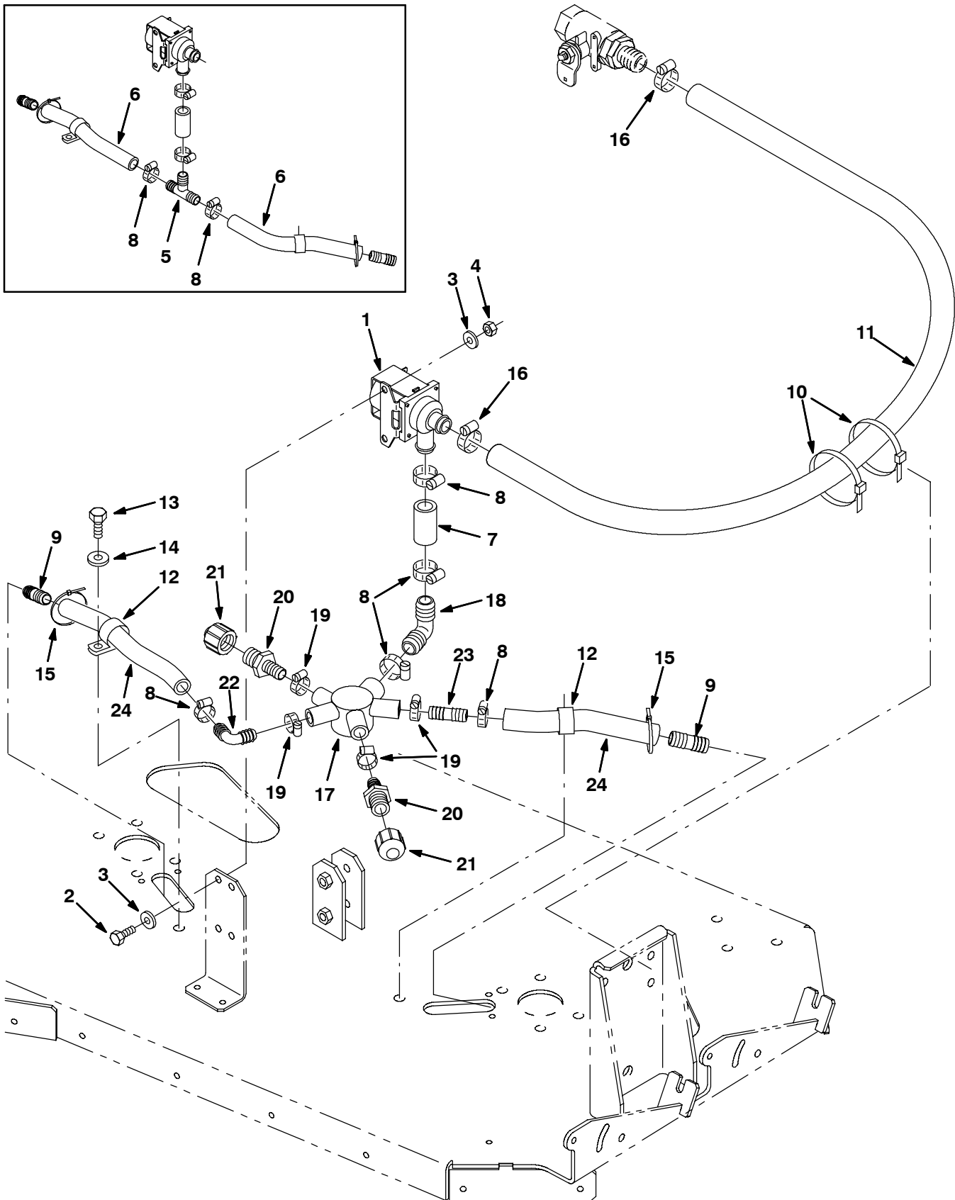
Fig. 25 - Max Pro 1000 (Disc-Brush) Solution Valve Group (Non FaST)
