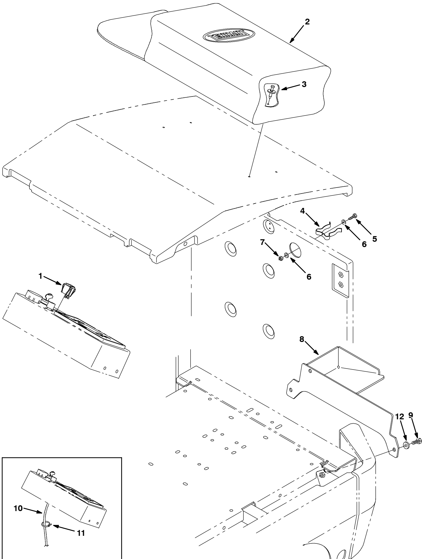
Fig. 53 - Power Wand Mount Group
