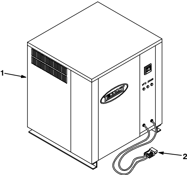
Fig. 68 - Battery Charger Group, 120A, 36V, 60Hz 3Ph (500Ah Batteries)
