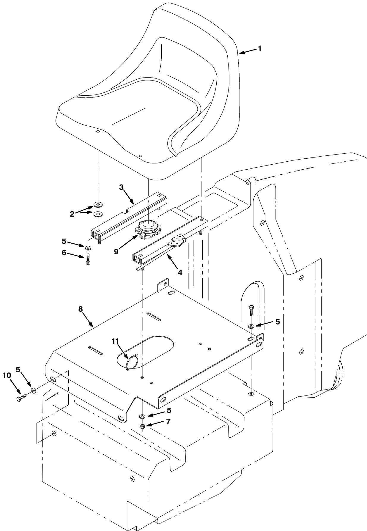
Fig. 9 - Seat Group
