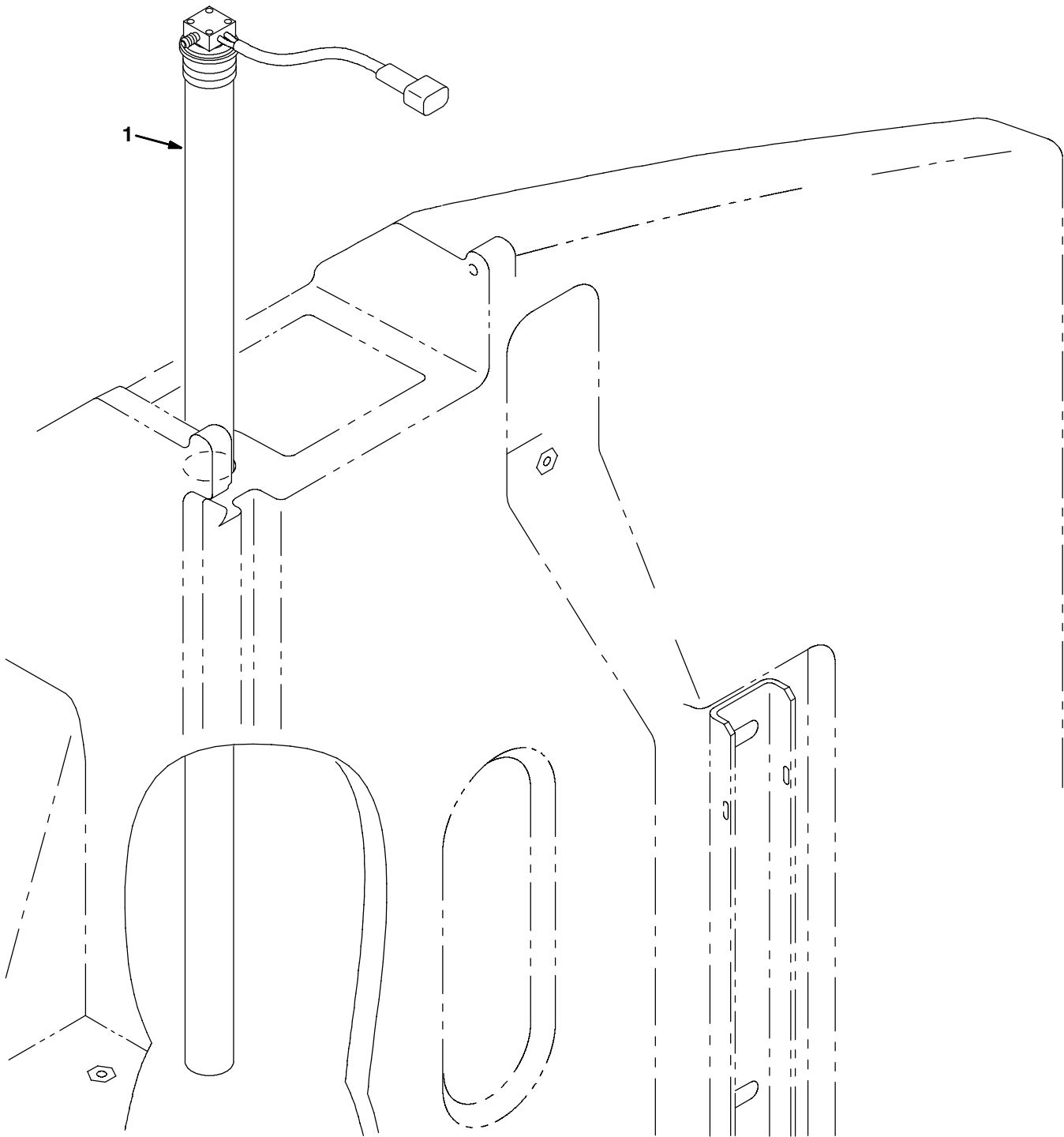
Fig. 48 - Low Water Level Kit
