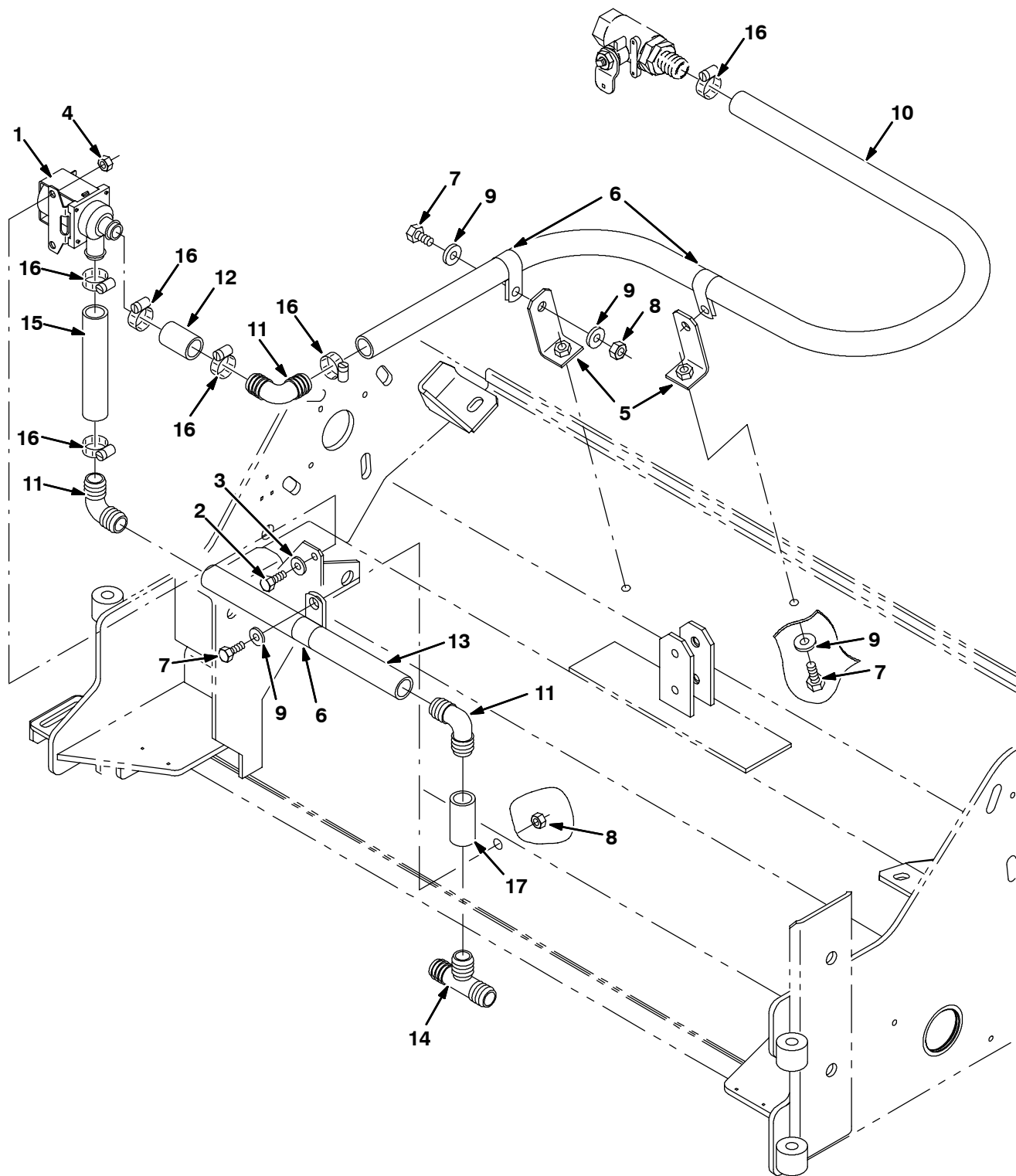
Fig. 27 - Max Pro 1000 (Cylindrical Brush) Solution Valve Group (Non FaST)
