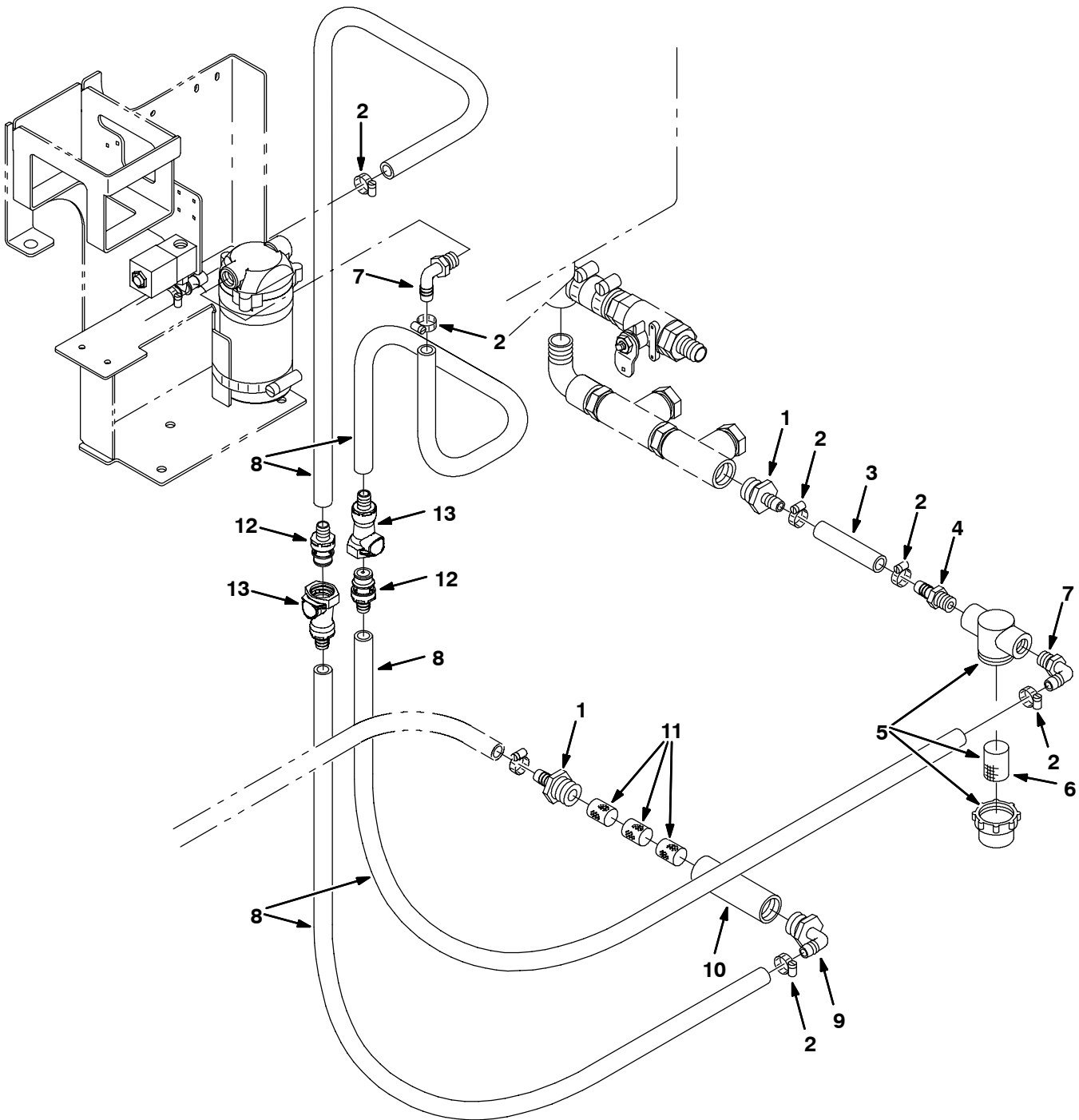
Fig. 17 - FaST Foam Filter Group
