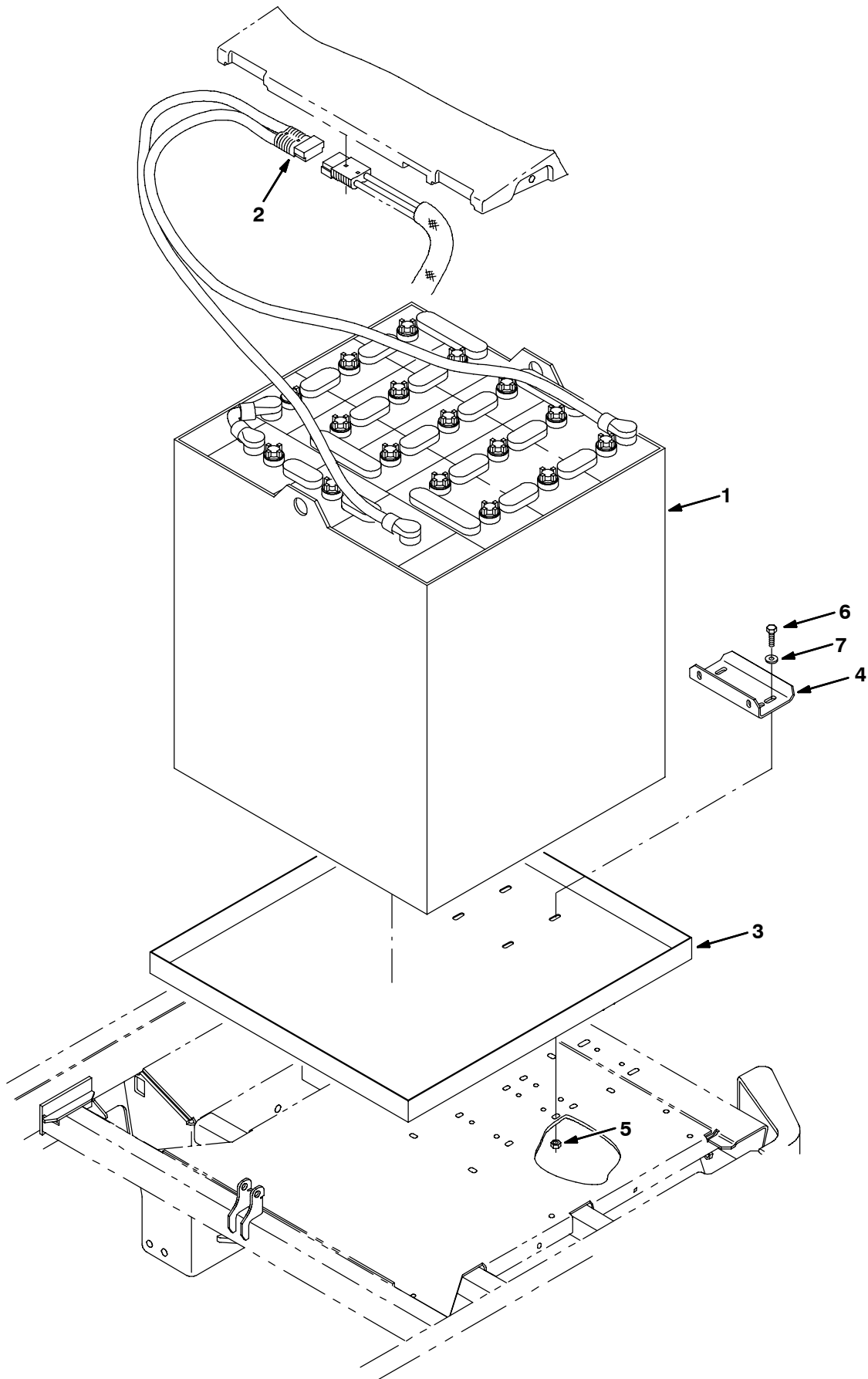
Fig. 64 - Battery Kit, 750AH Wet
