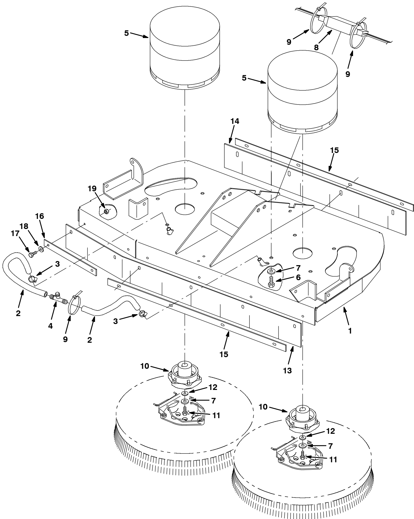
Fig. 14 - Disk Scrub Head Drive Motor Group, 900 mm (36 in)
