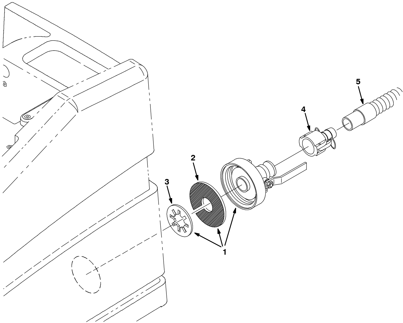
Fig. 23 - Positive Solution Control Drain Kit, Std
