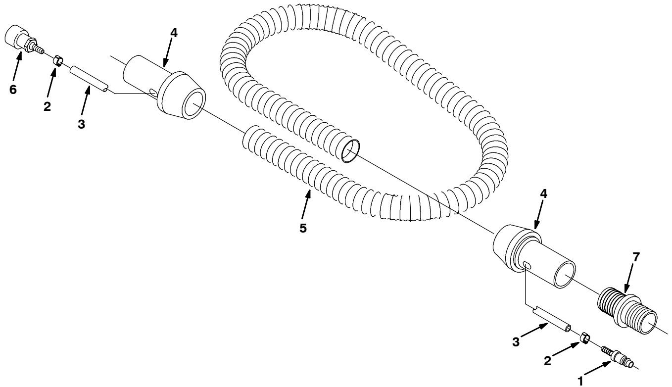
Fig. 15 - Power Wand Hose Assembly
