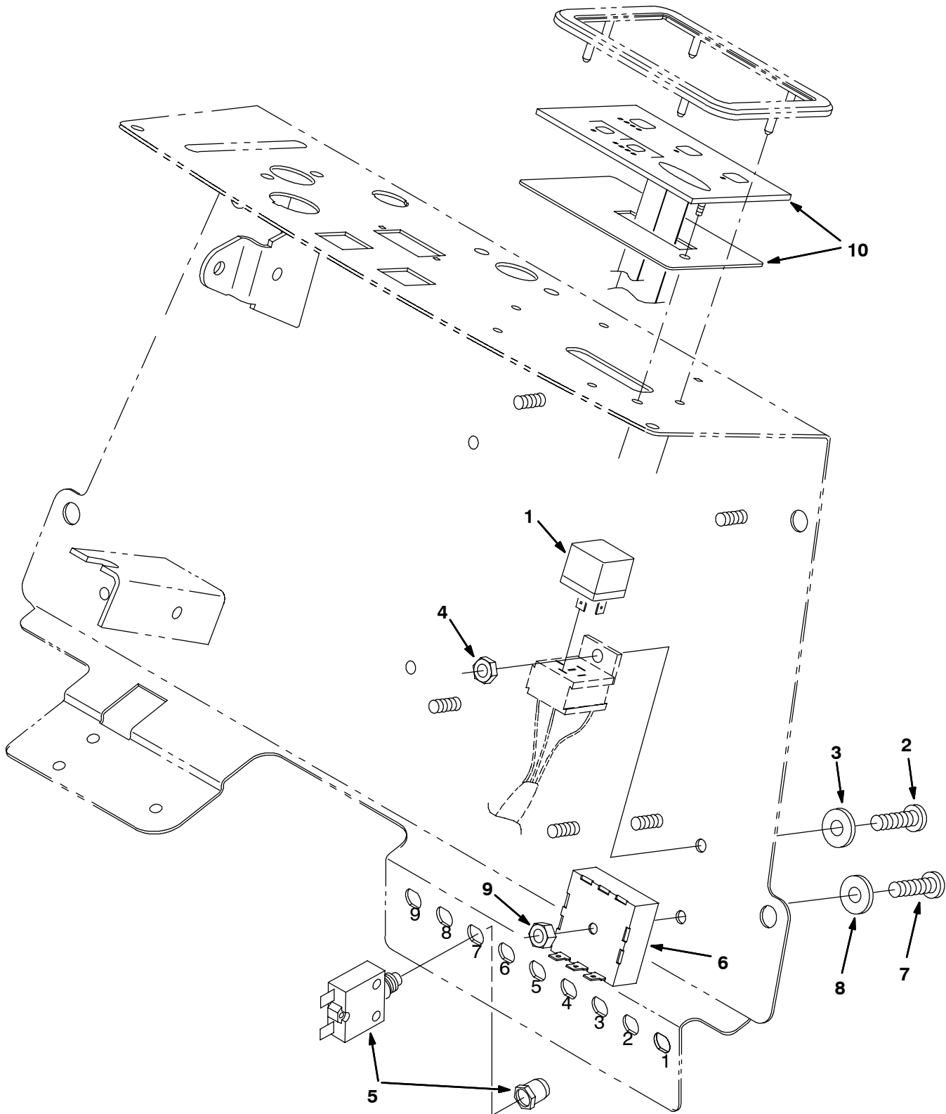
Fig. 9 - FaST Instrument Panel Group
