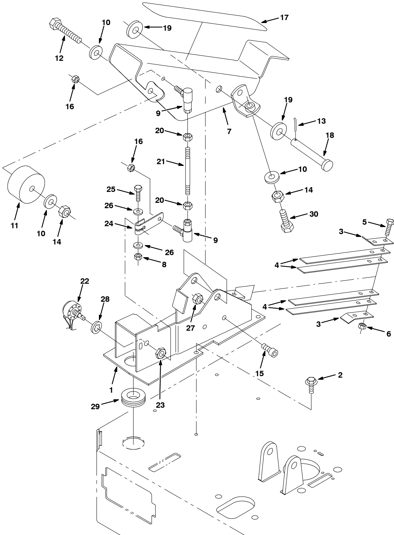
Fig. 16 - Directional Pedal Group (00000000-10117237)
