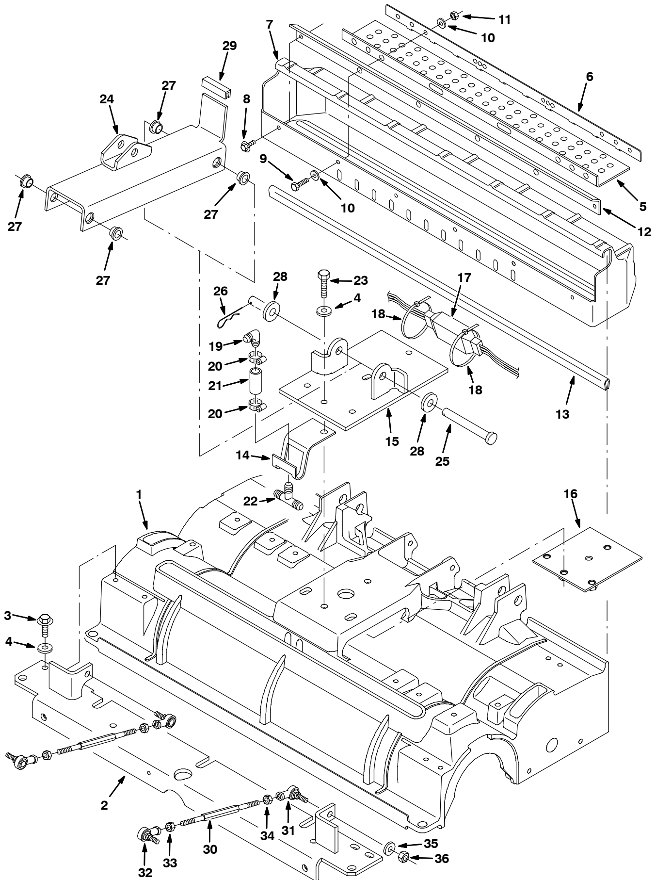
Fig. 23 - Cylindrical Scrub Head Frame Group, 700 mm (28 in)
