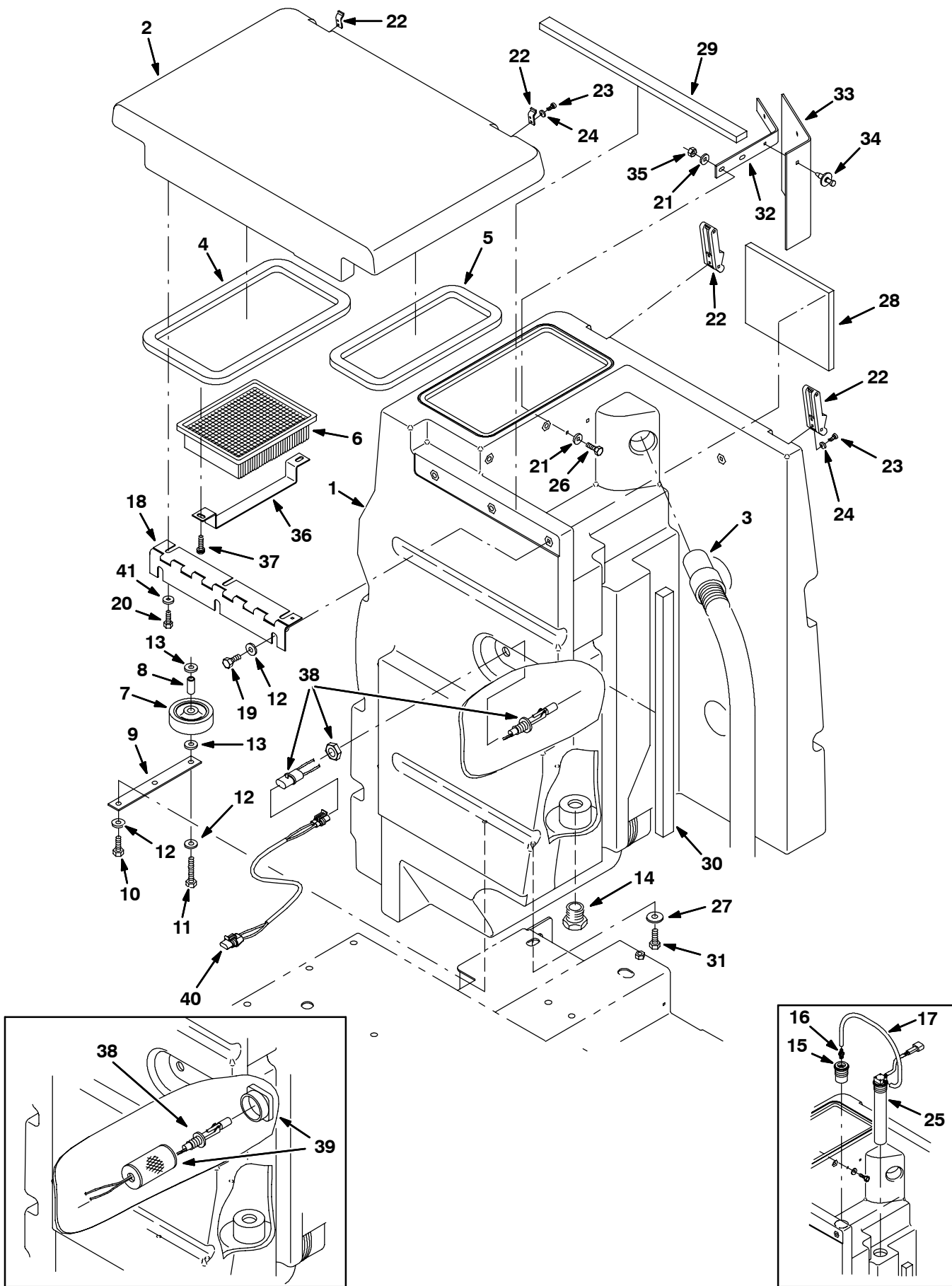
Fig. 20 - Recovery Tank Group
