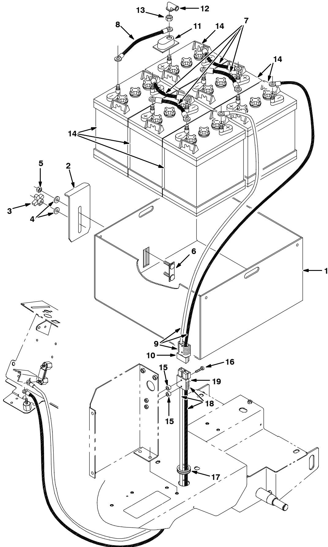
Fig. 37 - Rollout Battery Pack Kit
