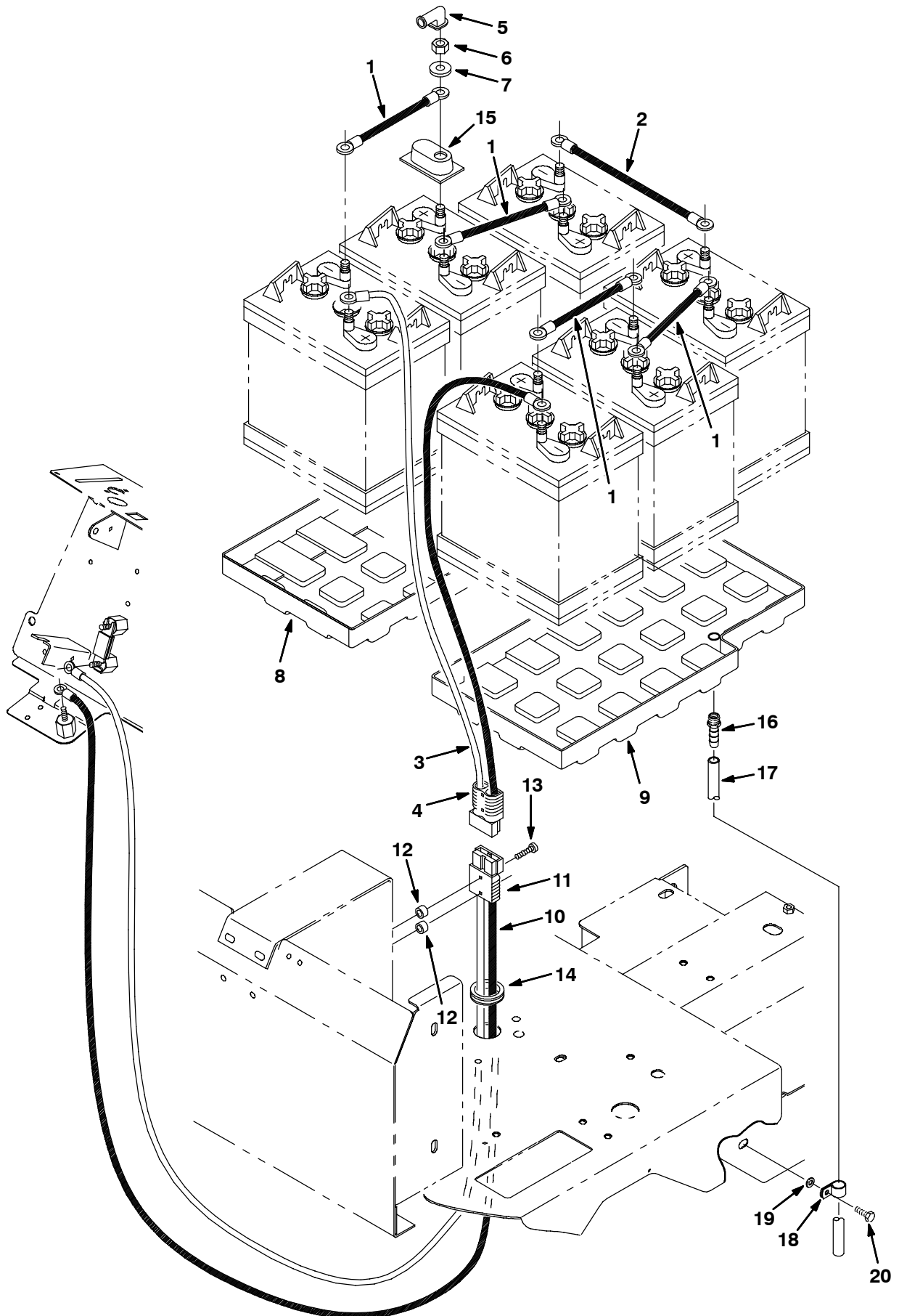
Fig. 25 - Battery Cable Group
