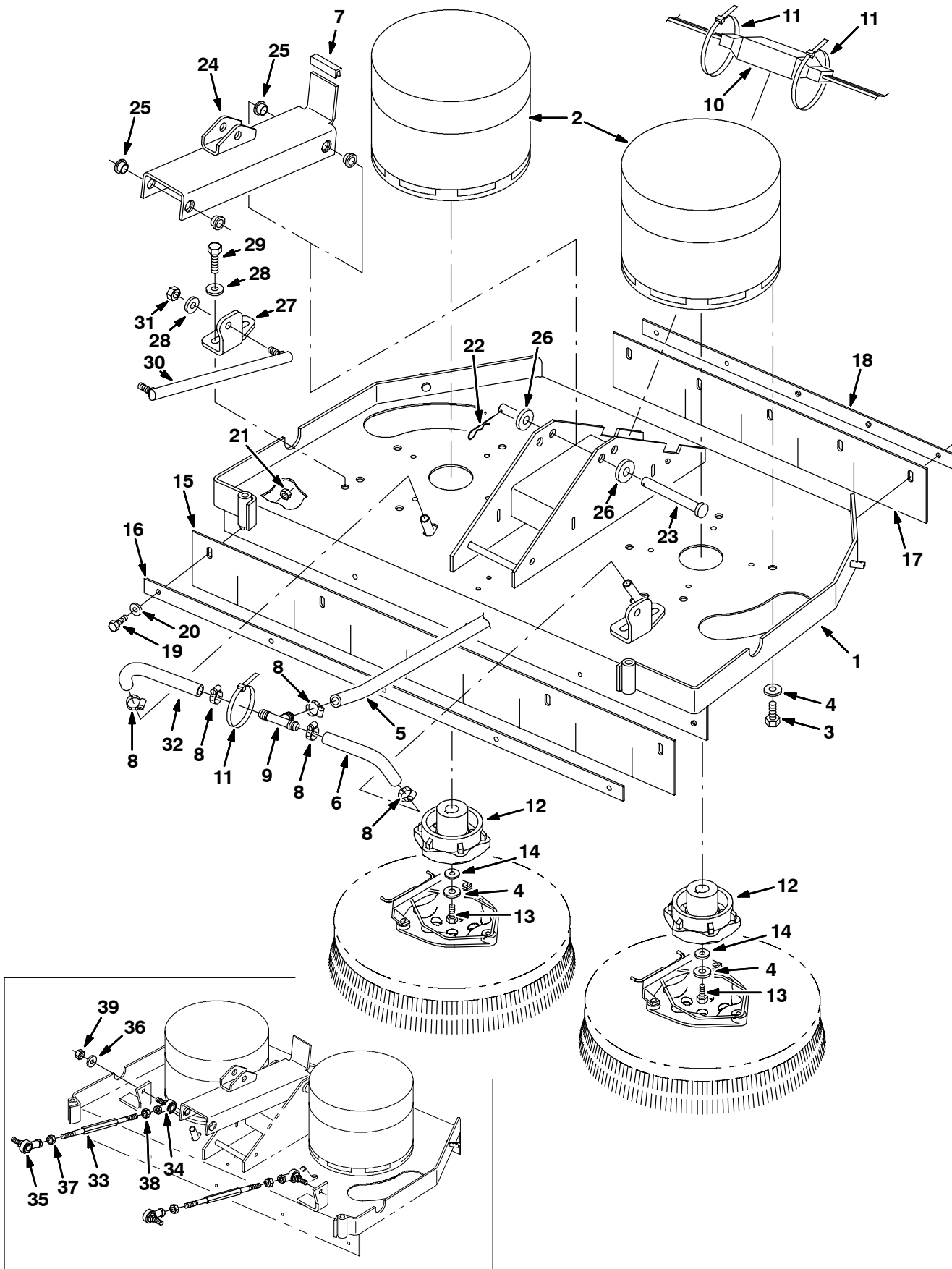
Fig. 20 - Disk Scrub Head Drive Motor Group, 800 mm (32 in)
