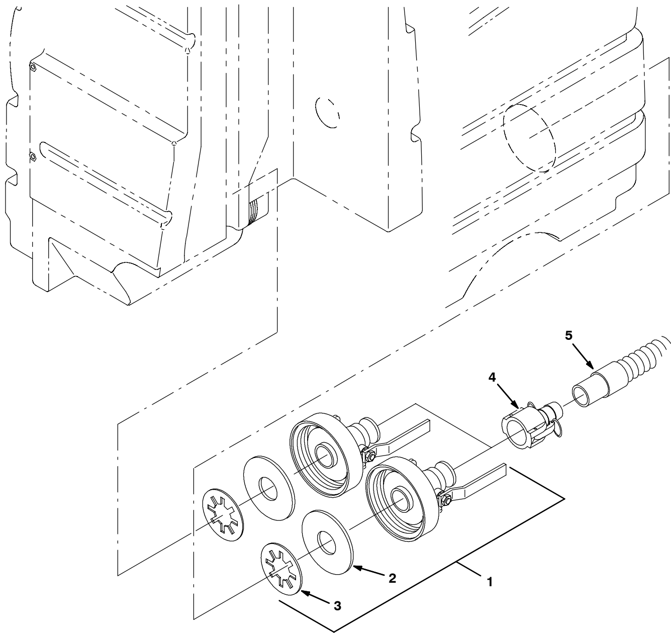
Fig. 49 - Positive Solution Control Drain Kit, ES (Extended Scrub)
