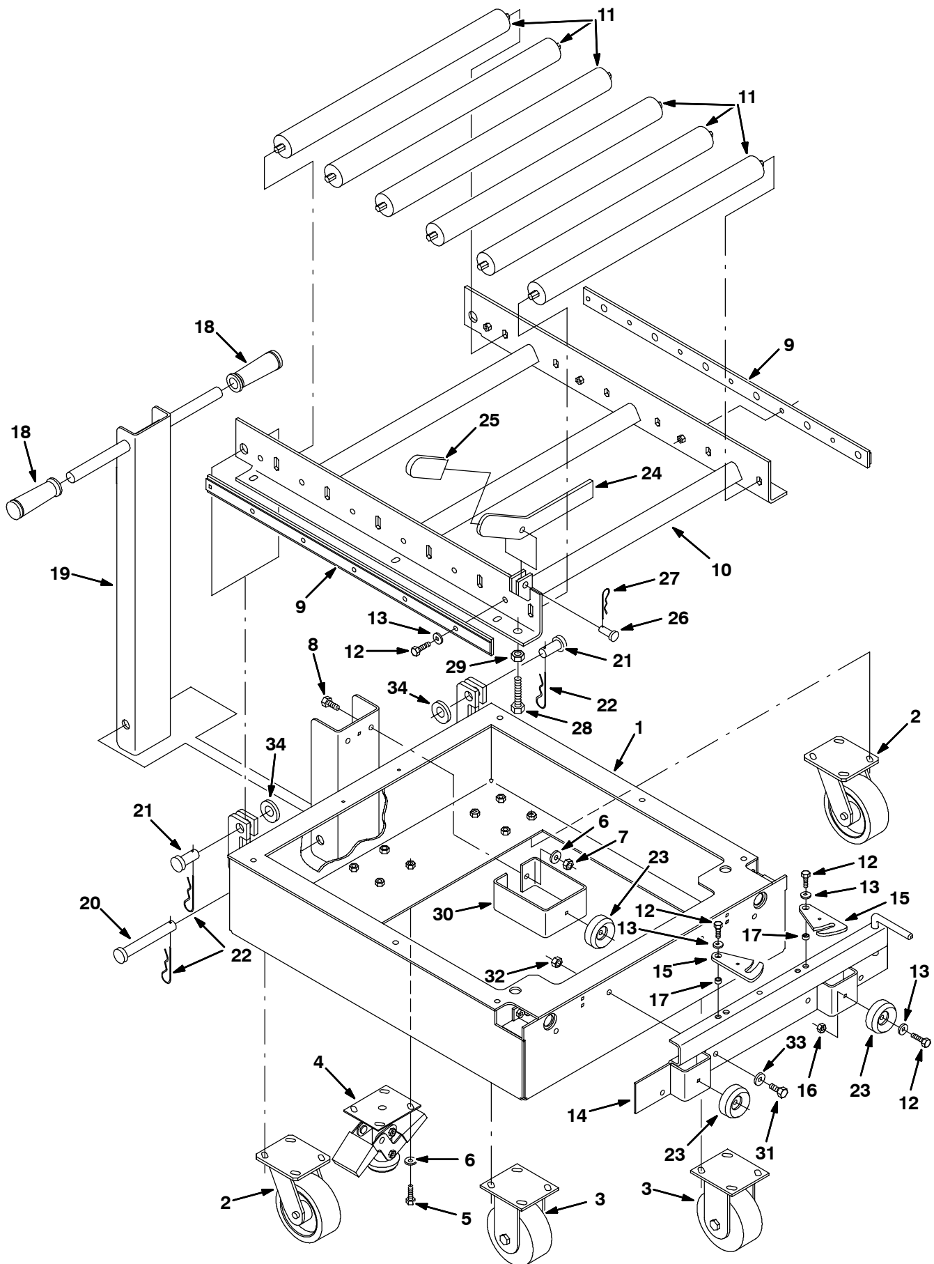
Fig. 38 - Rollout Battery Cart Kit
