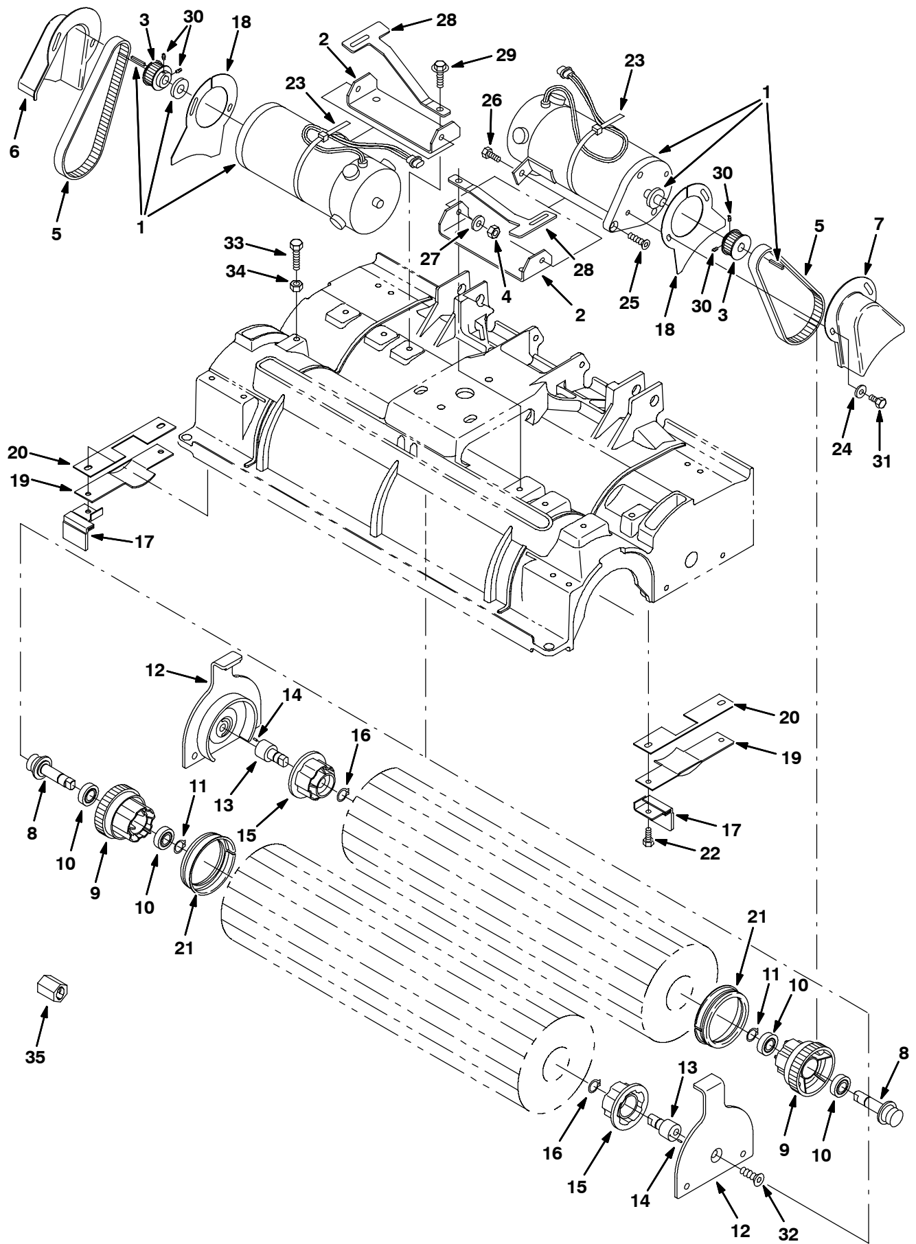
Fig. 25 - Cylindrical Scrub Head Drive Motor Group, 800 mm (32 in)
