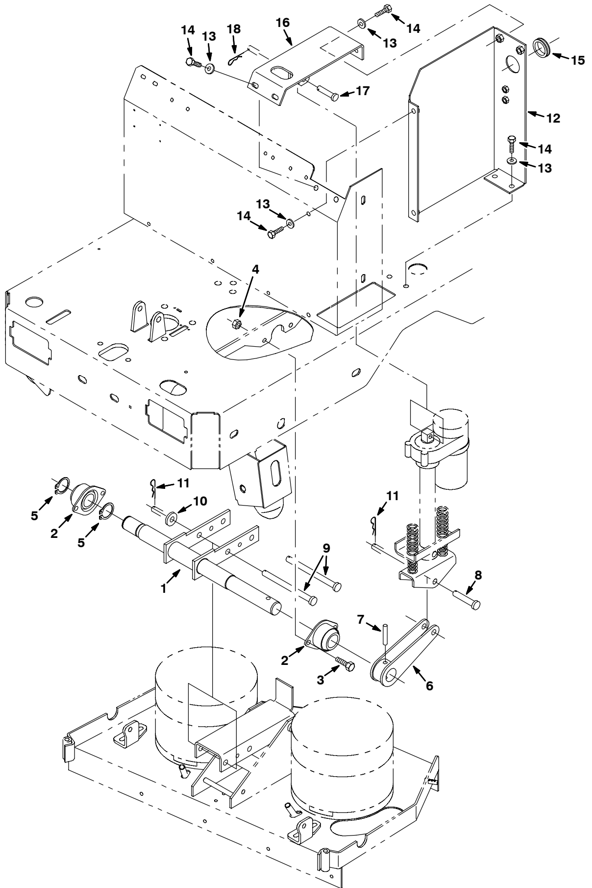
Fig. 36 - Rollout Battery Scrub Head Lift Group
