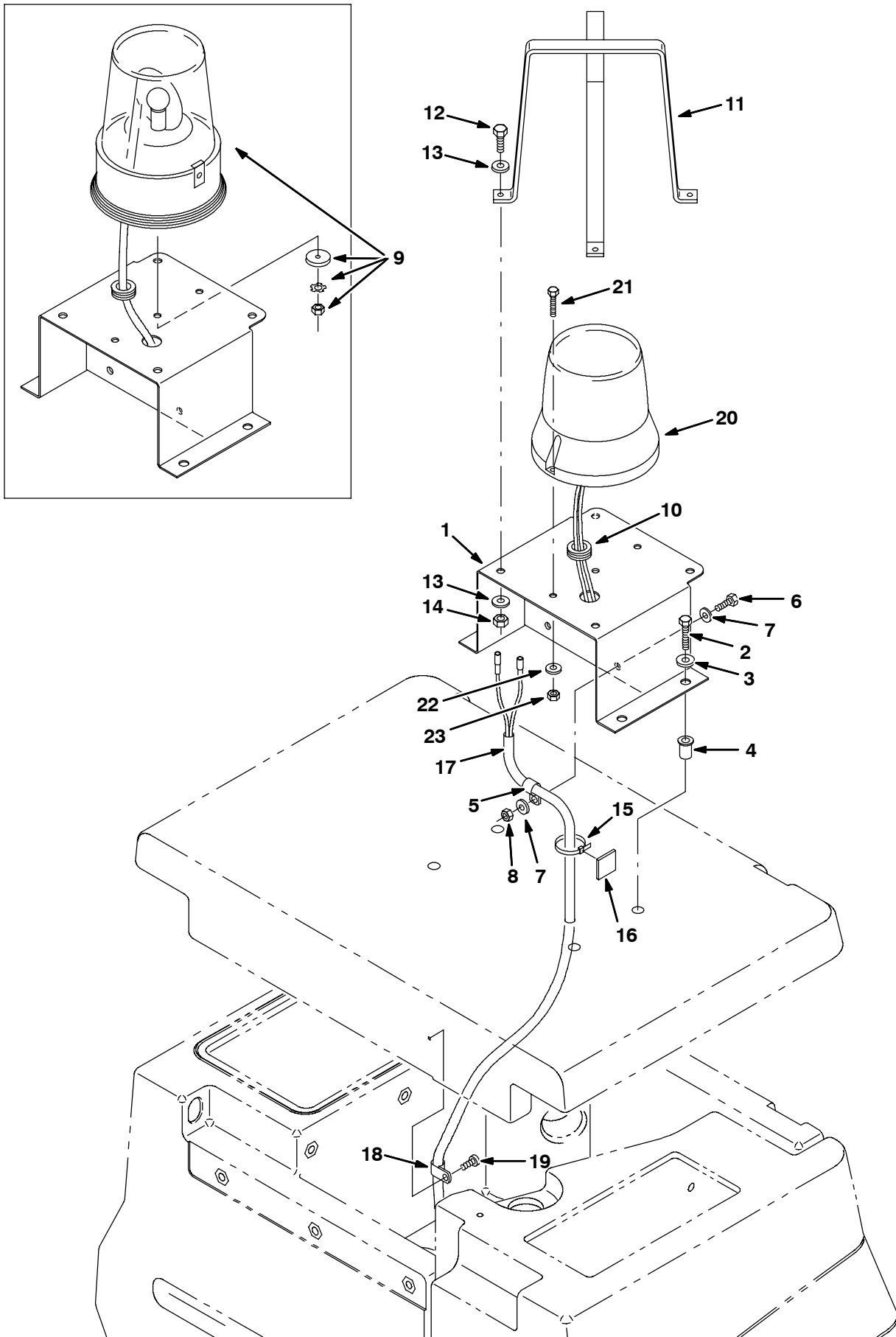
Fig. 44 - Revolving Light Kit
