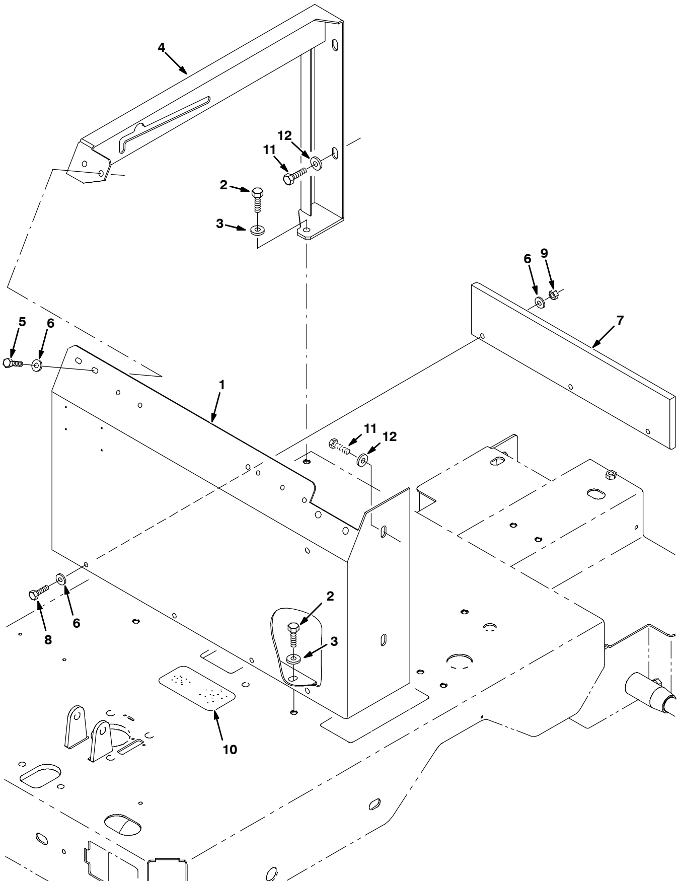
Fig. 35 - Rollout Battery Seat Support Group
