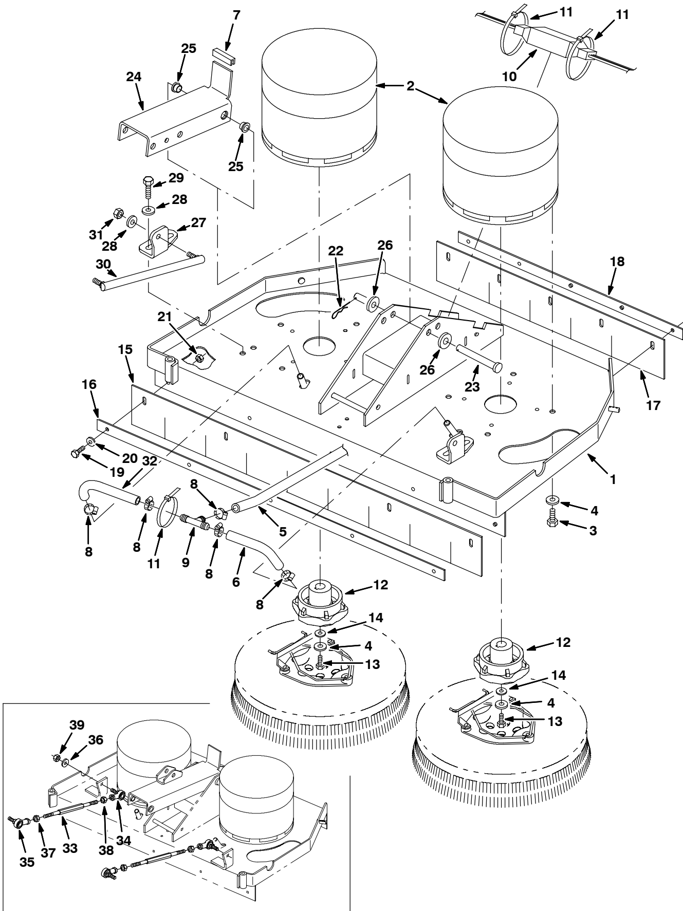
Fig. 30 - Rollout Battery Disk Scrub Head Drive Motor Group, 800 mm (32 in)
