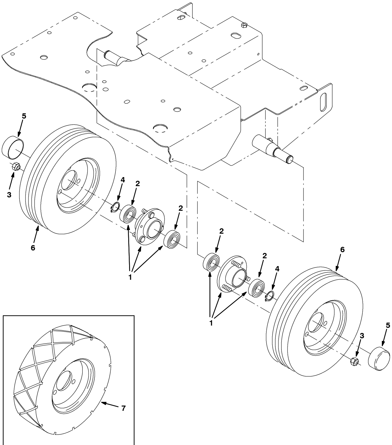
Fig. 15 - Rear Wheel Group
