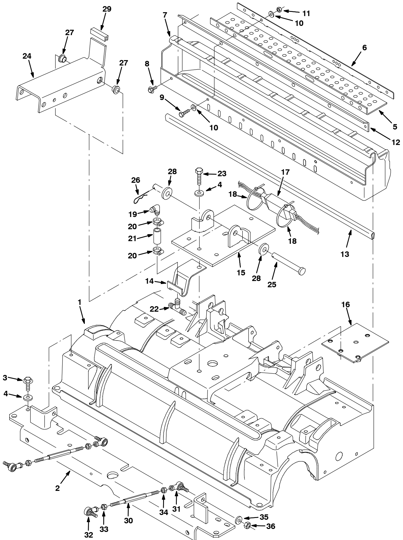
Fig. 31 - Rollout Battery Cylindrical Scrub Head Frame Group, 700 mm (28 in)
