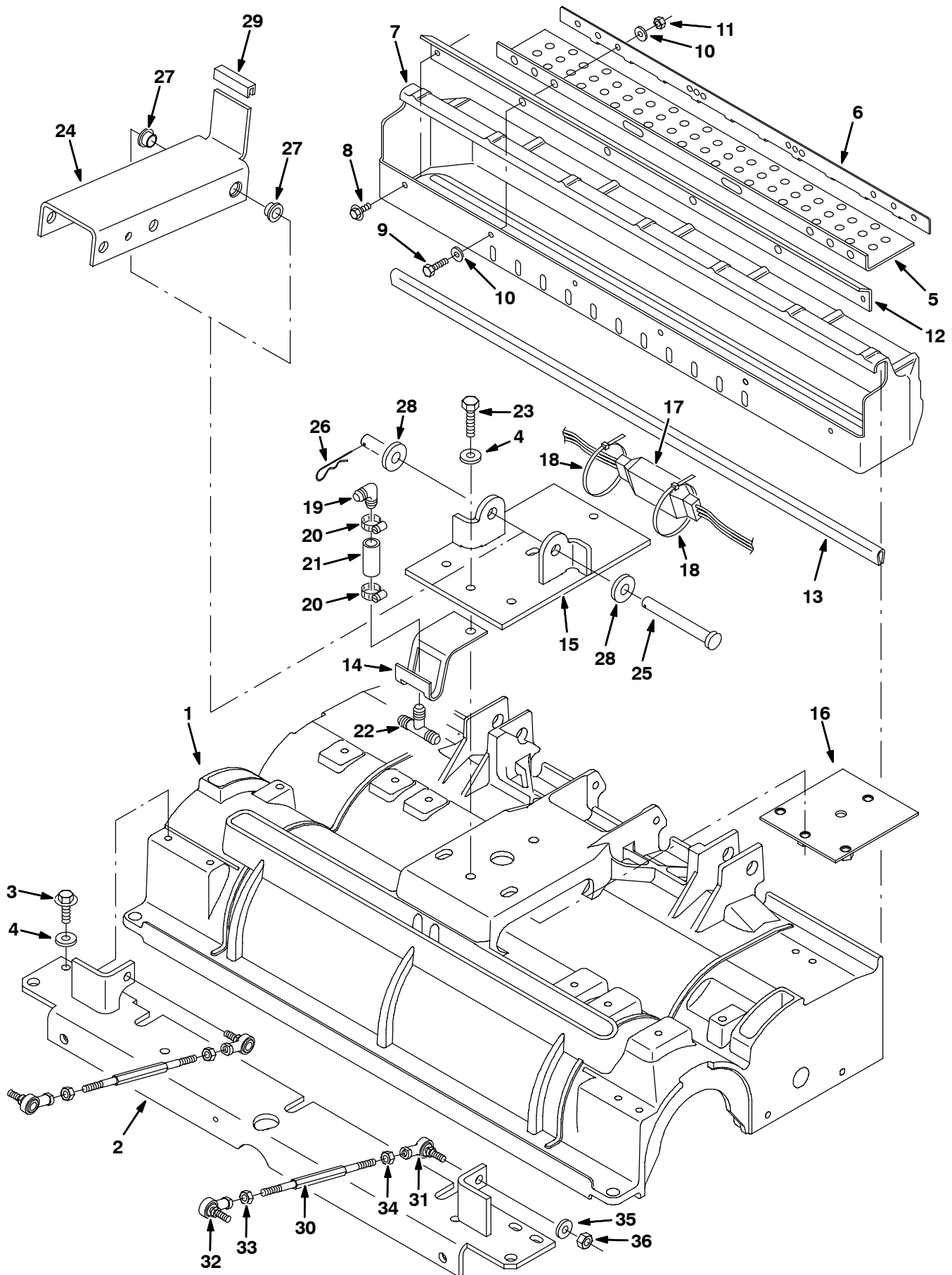
Fig. 32 - Rollout Battery Cylindrical Scrub Head Frame Group, 800 mm (32 in)
