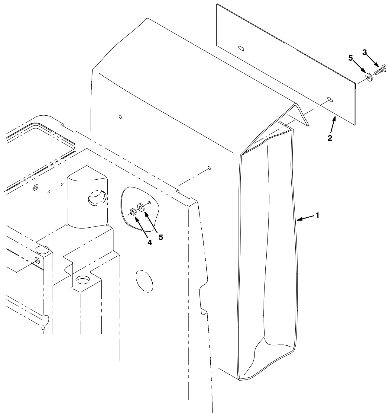
Fig. 50 - Storage Bag Kit
