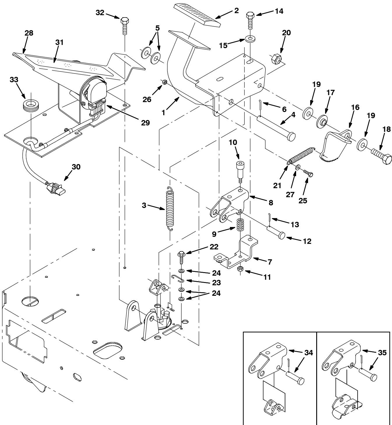
Fig. 14 - Brake Pedal and Directional Pedal Group
