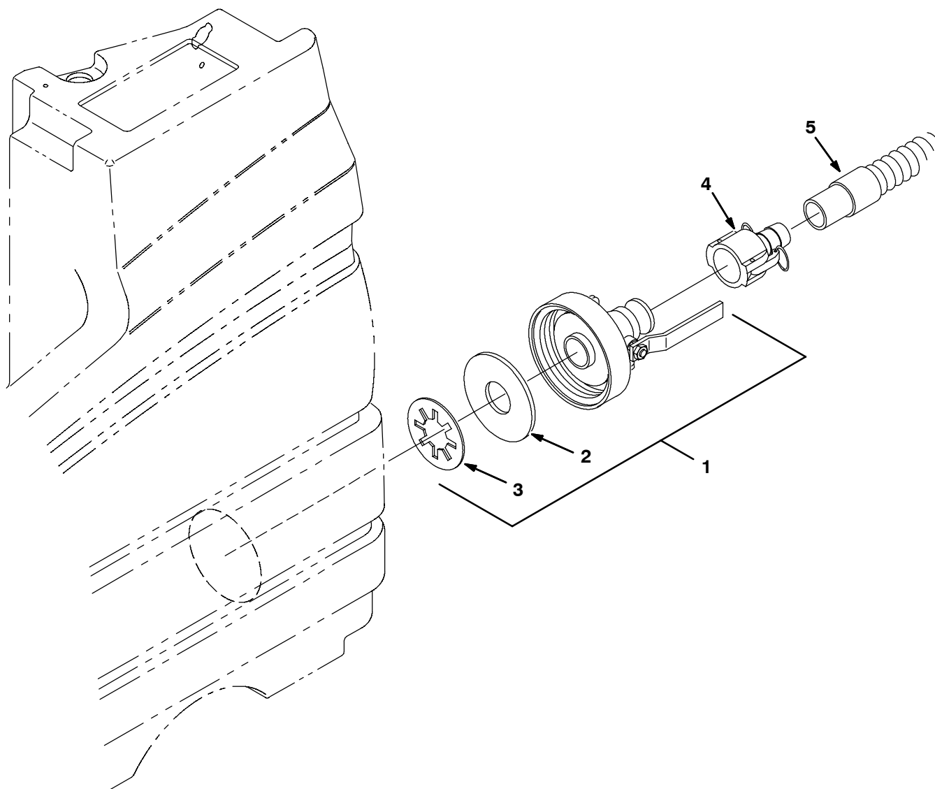
Fig. 48 - Positive Solution Control Drain Kit, Std
