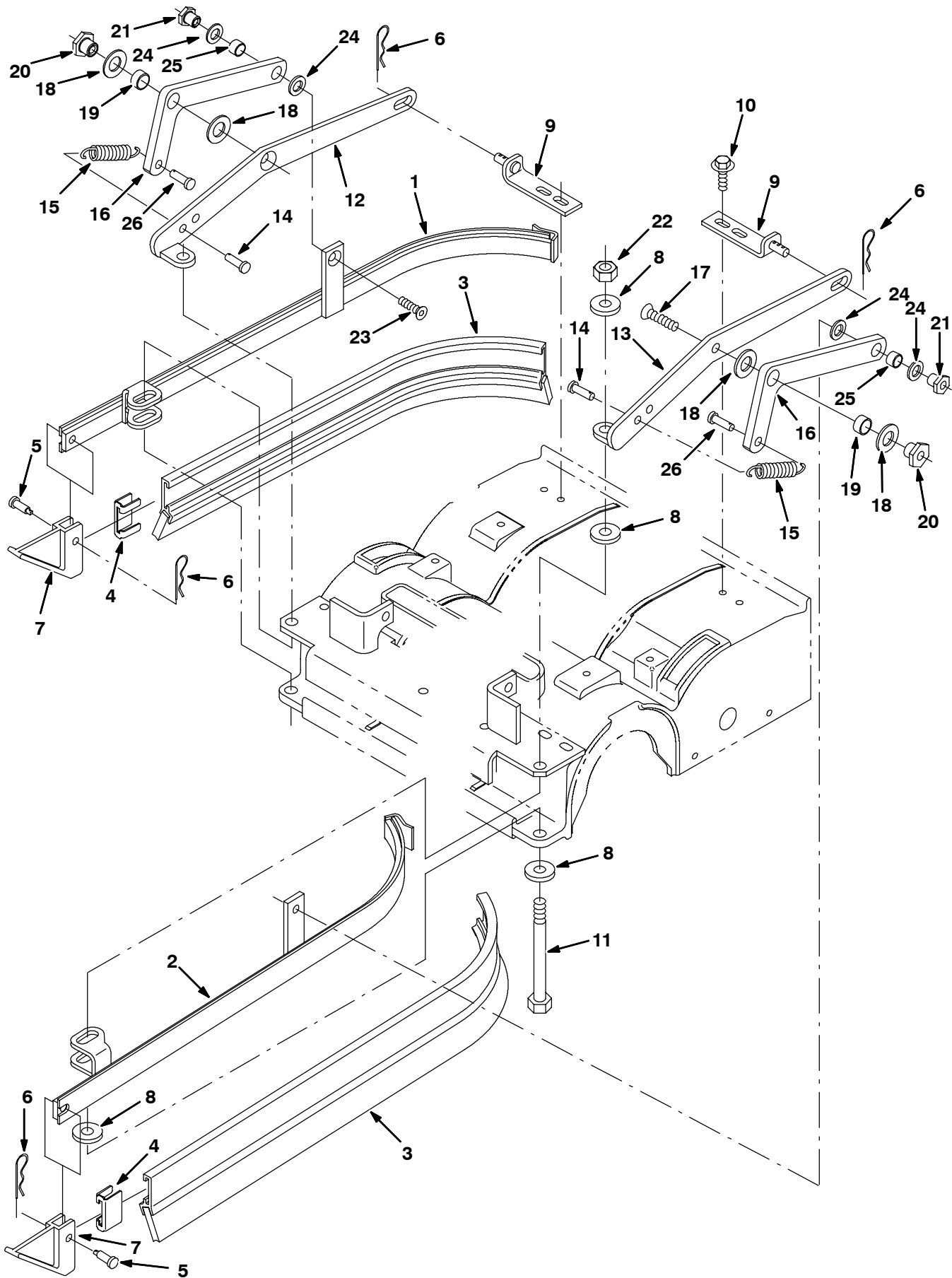
Fig. 27 - Cylindrical Scrub Head Squeegee Group, 800 mm (32 in)
