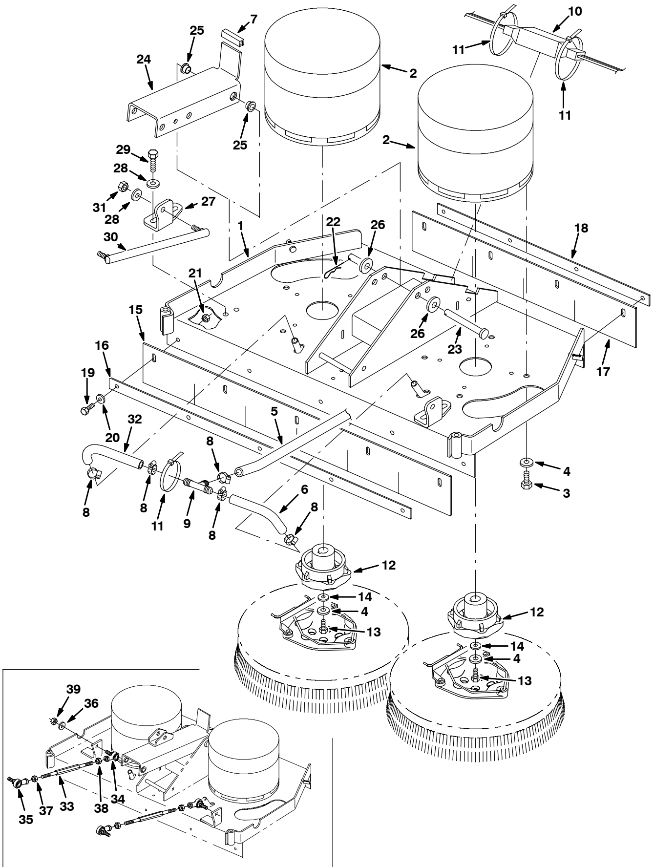
Fig. 28 - Rollout Battery Disk Scrub Head Drive Motor Group, 700 mm (28 in)
