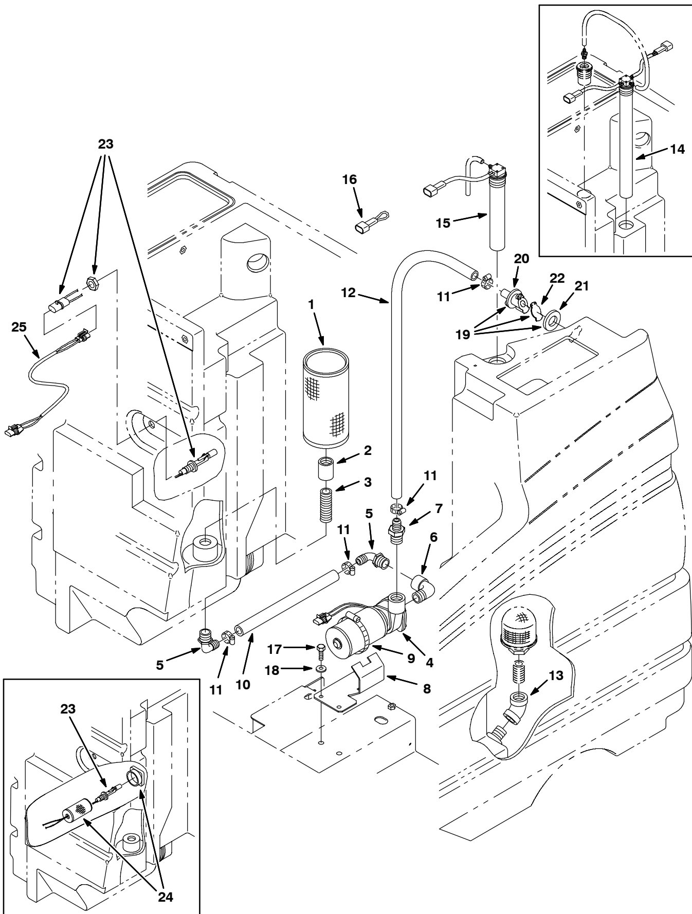
Fig. 2 - ES (Extended Scrub) Pump Group
