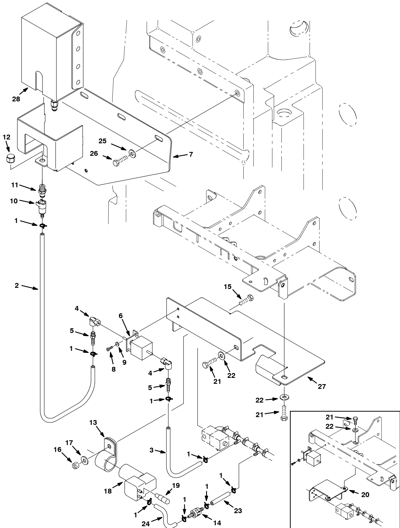
Fig. 4 - FaST Air Pump and Detergent Group
