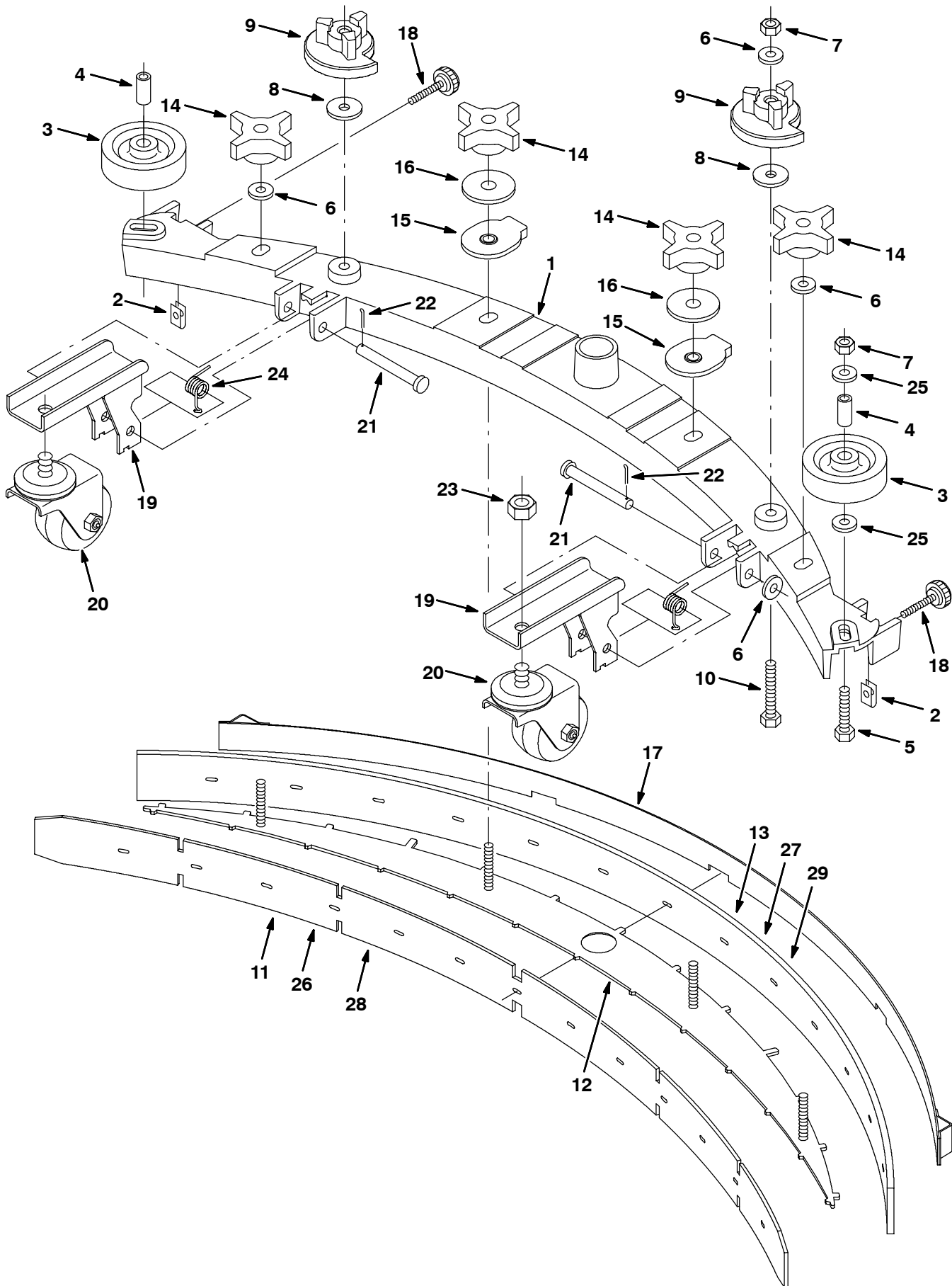
Fig. 39 - Rear Squeegee Group, 800 mm (32 in)
