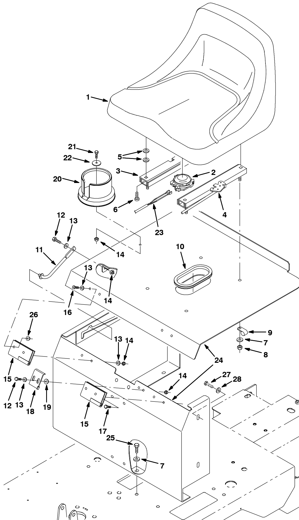
Fig. 5 - Seat Group (0000000-10108251)
