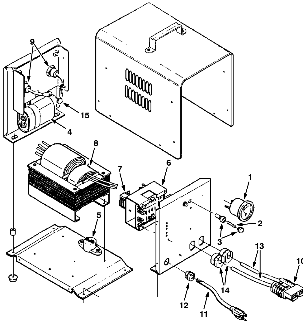
Fig. 5 - Battery Charger Breakdown, 50 Hz (305 Ah batteries), 222691
