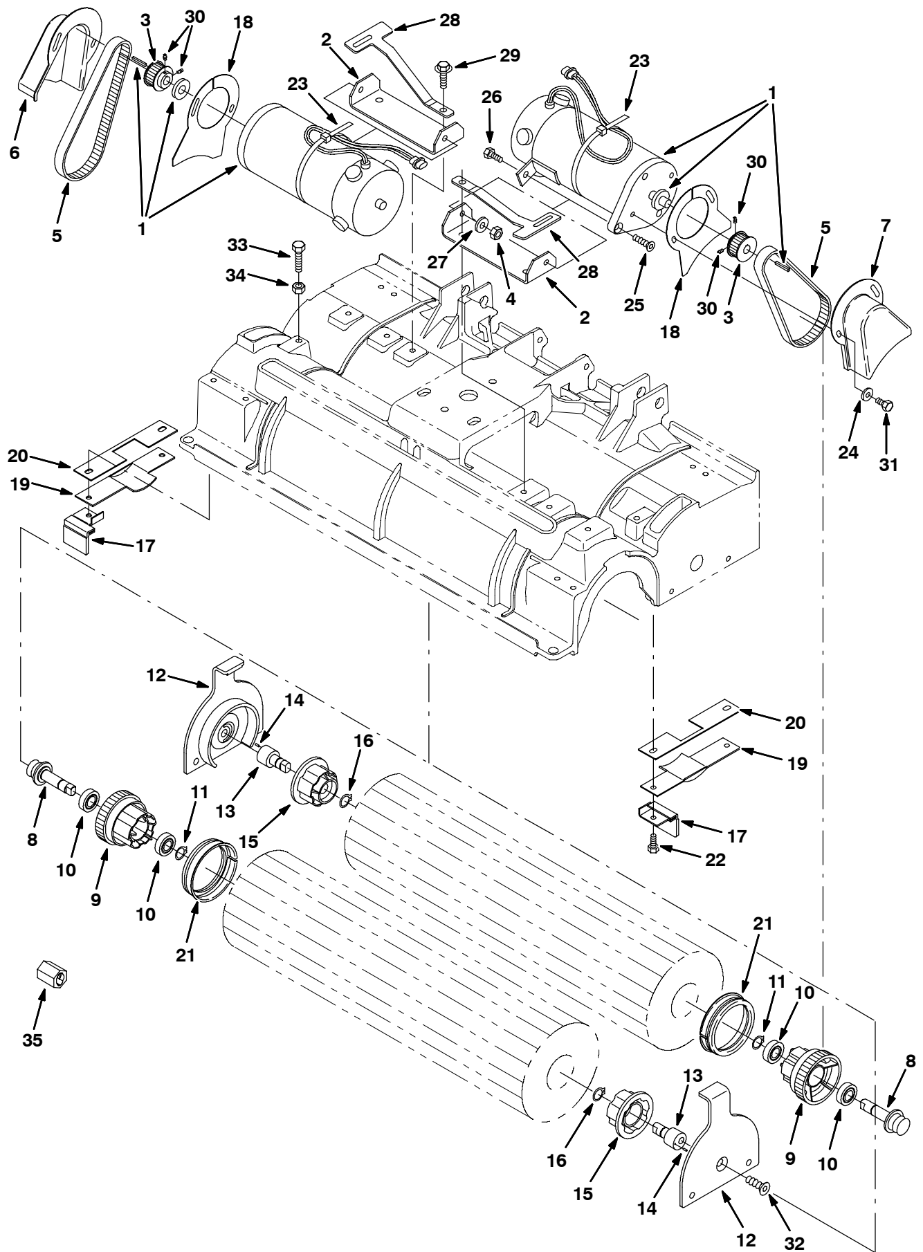
Fig. 22 - Cylindrical Scrub Head Drive Motor Group, 700 mm (28 in)
