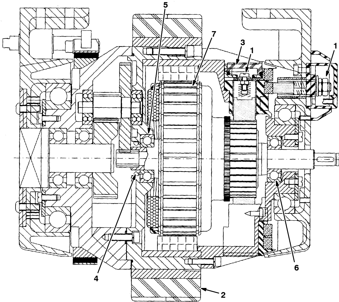
Fig. 7 - Front Wheel Gearbox Breakdown, 390851 (10046634-10160409)
