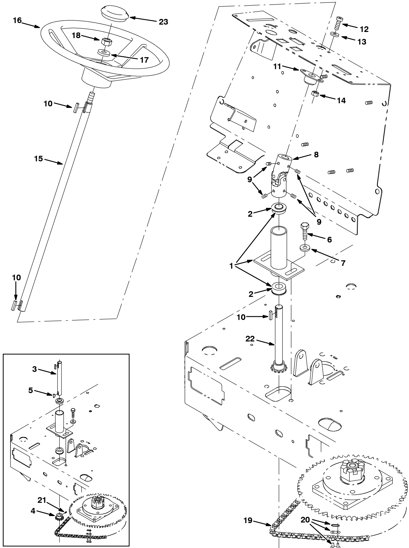
Fig. 7 - Steering Group
