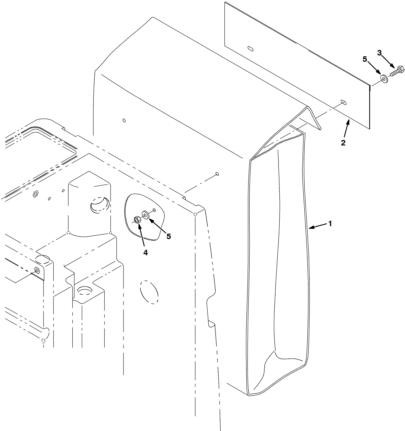
Fig. 14 - Power Wand Mount Group
