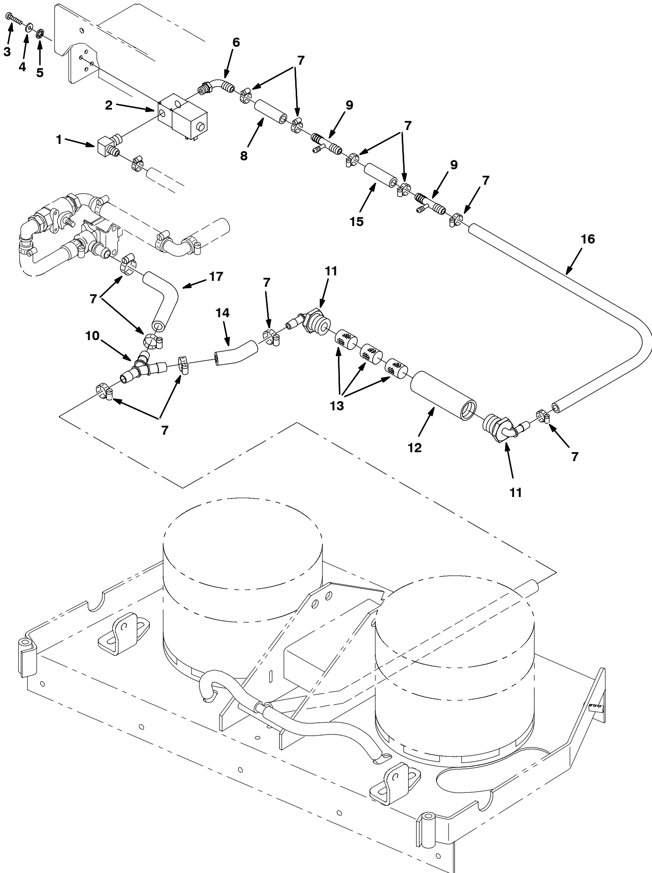
Fig. 6 - FaST Foam Filter Group, Disk Scrub Head
