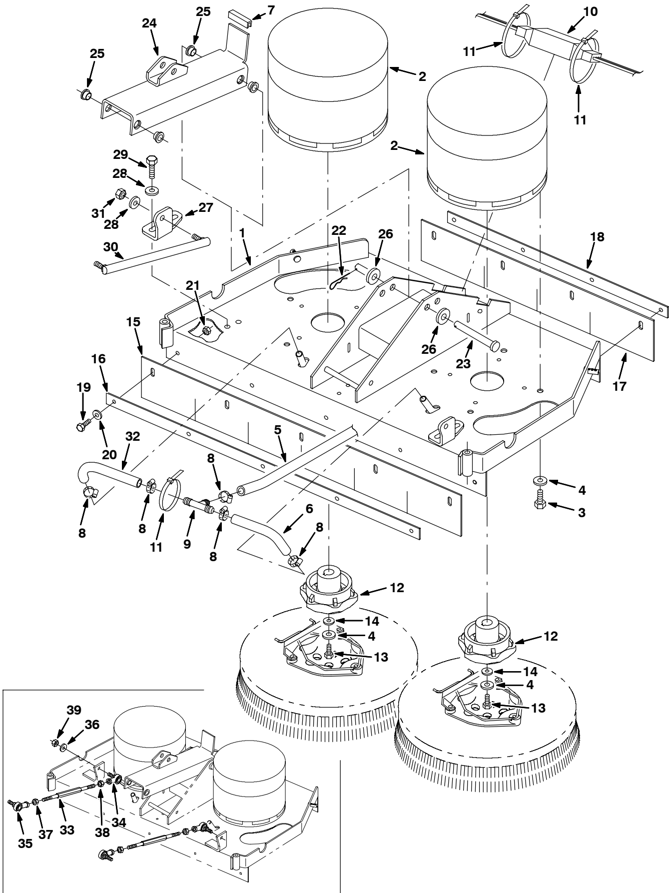
Fig. 18 - Heavy Duty Disk Scrub Head Drive Motor Group, 700 mm (28 in)
