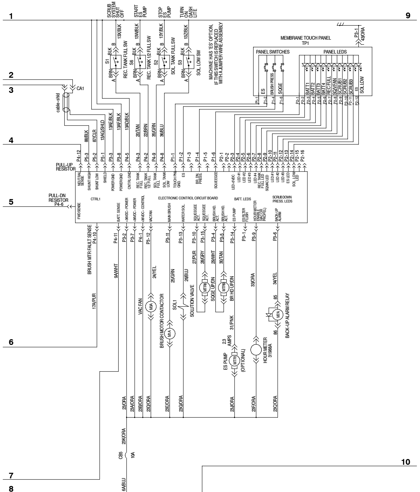
Fig. 29 - Electrical Schematic
