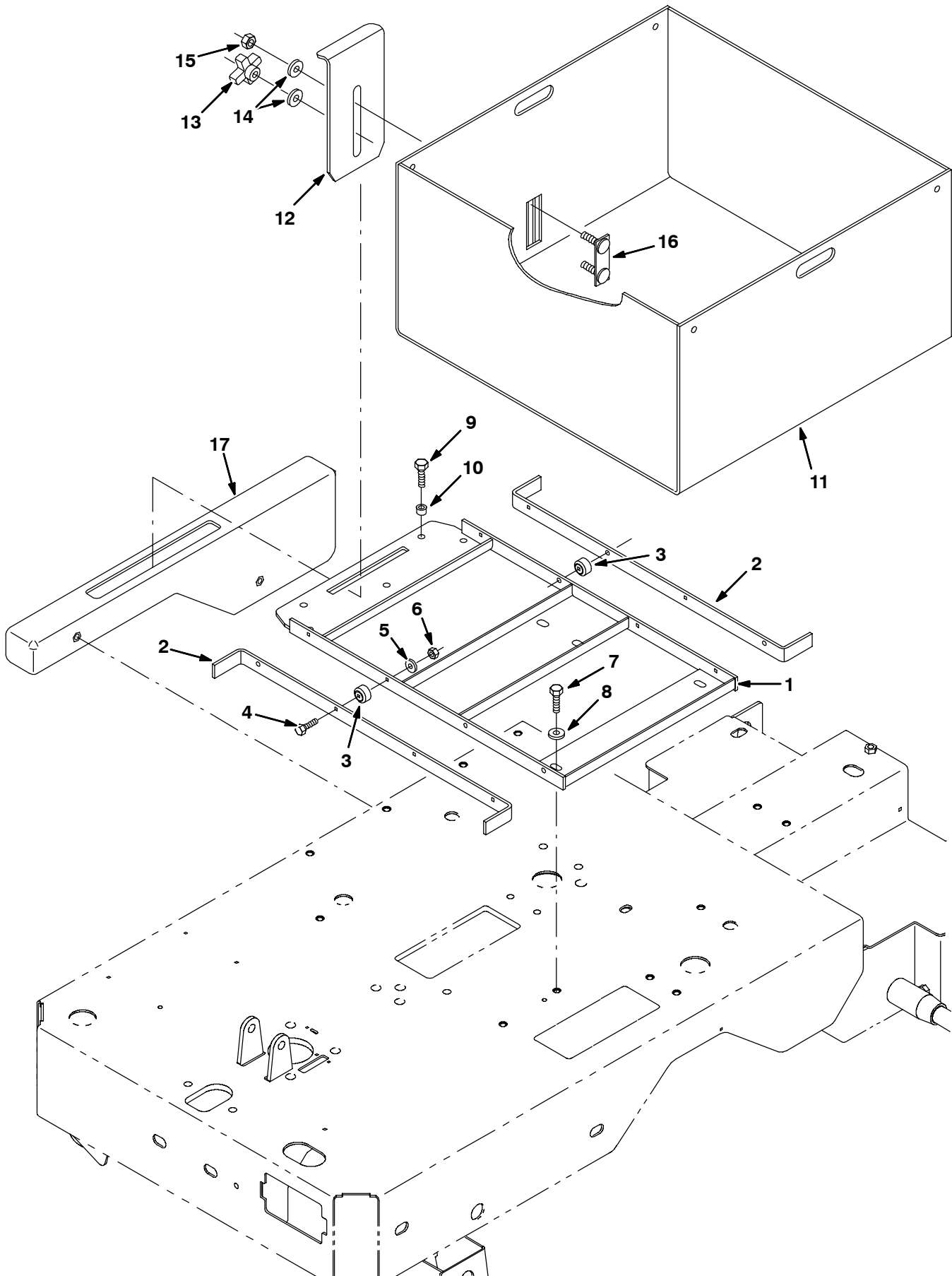
Fig. 33 - Rollout Battery Case Group
