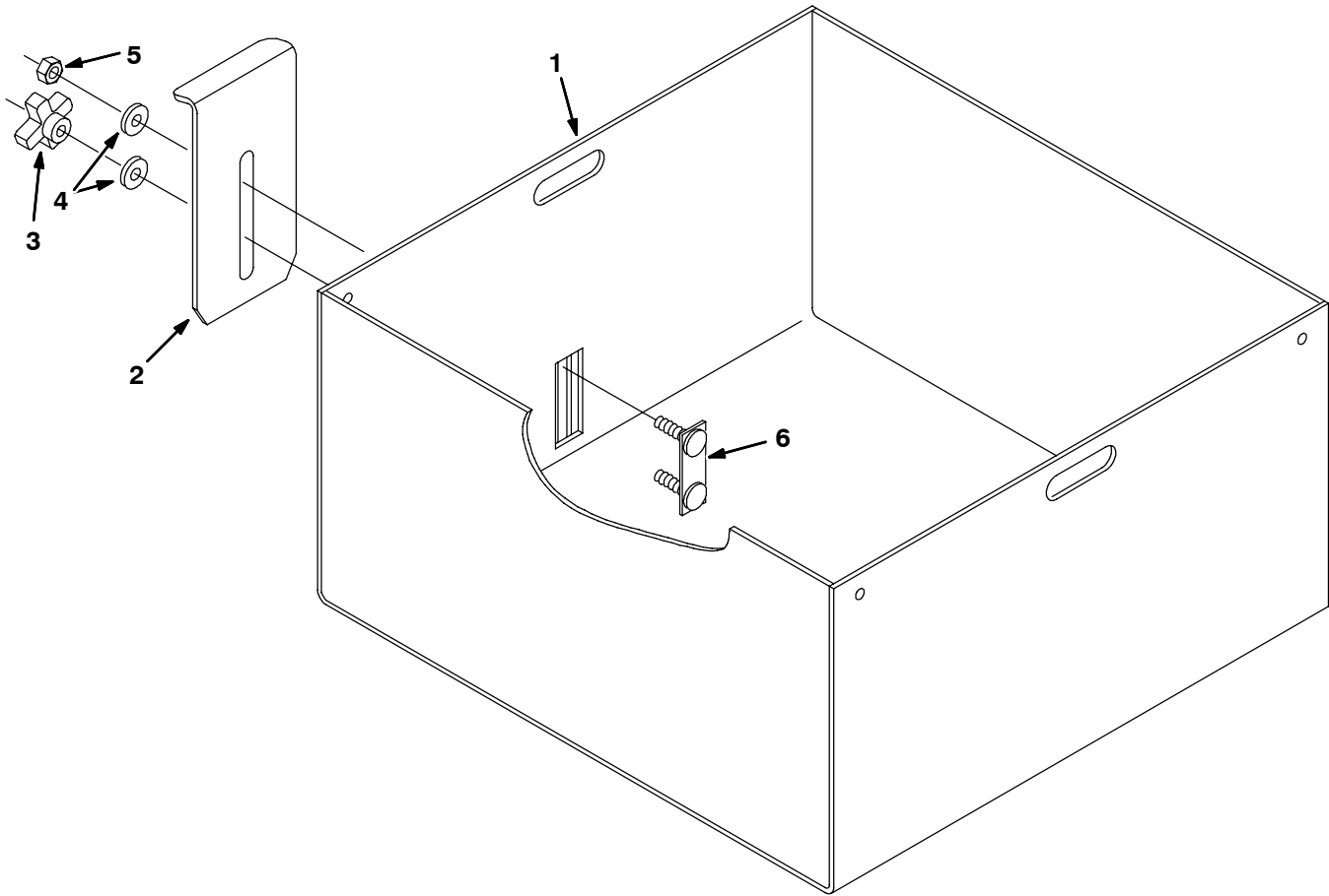
Fig. 34 - Rollout Battery Extra Case Kit
