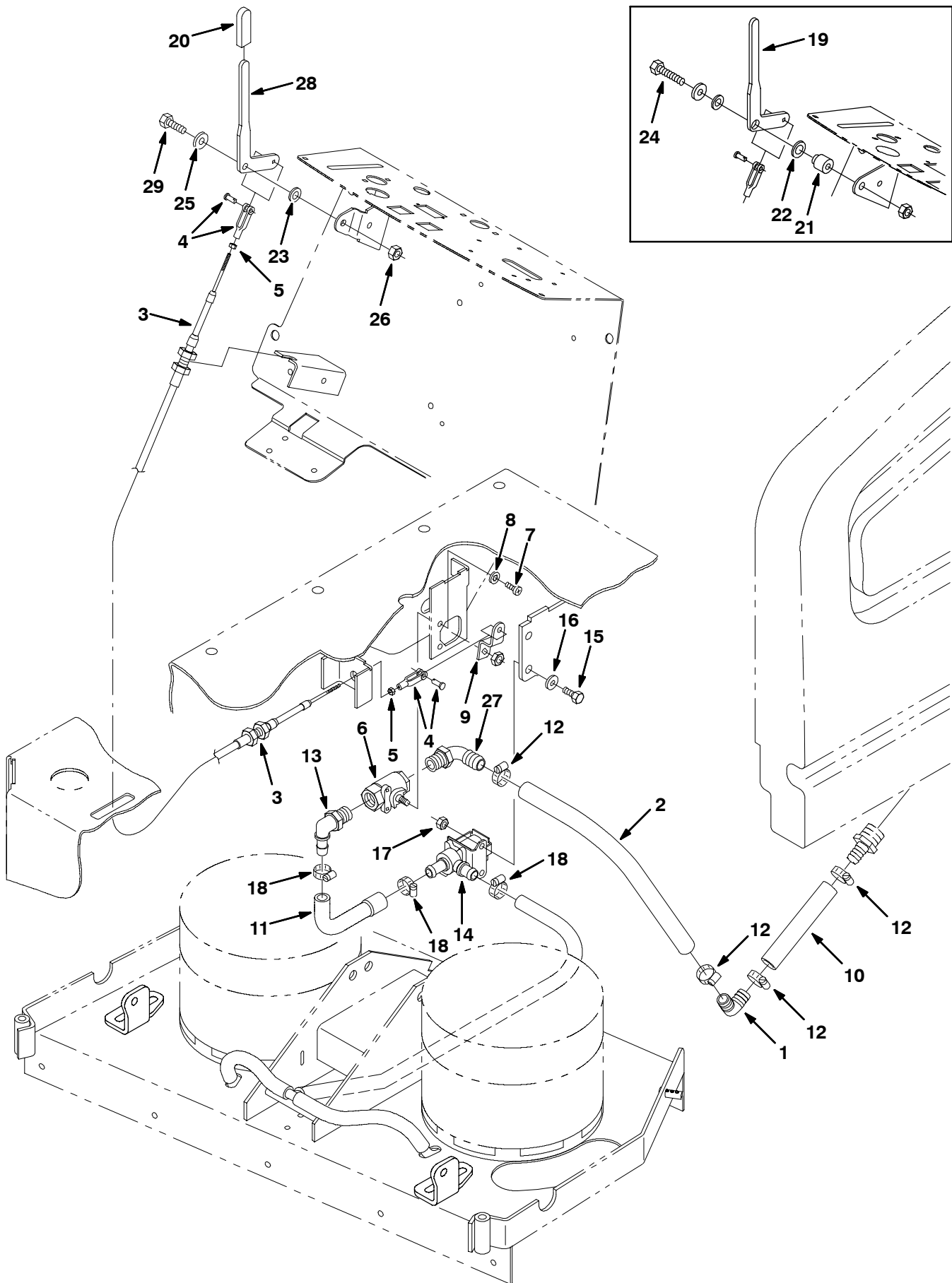
Fig. 24 - Solution Control Group
