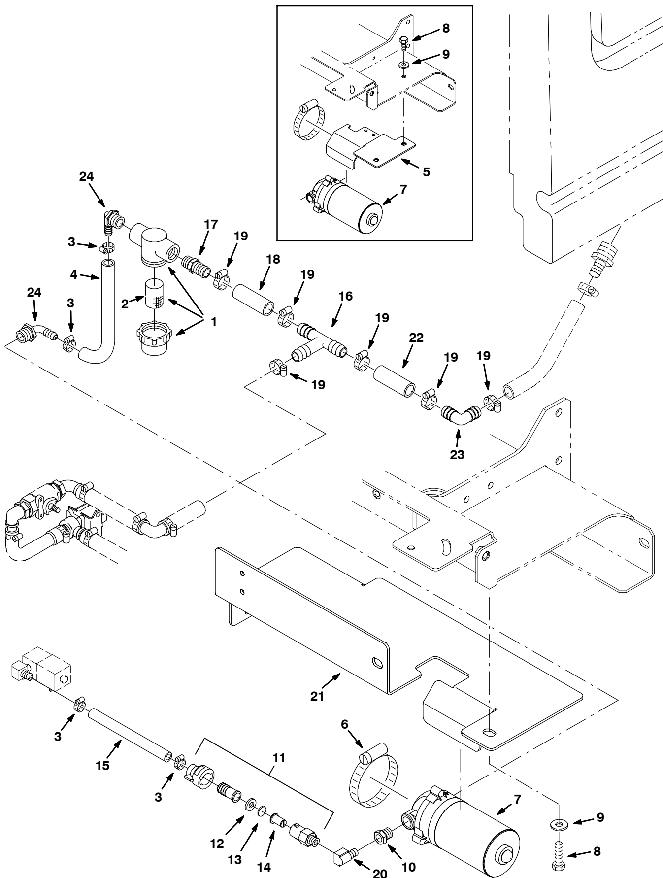
Fig. 5 - FaST Solution Pump Group
