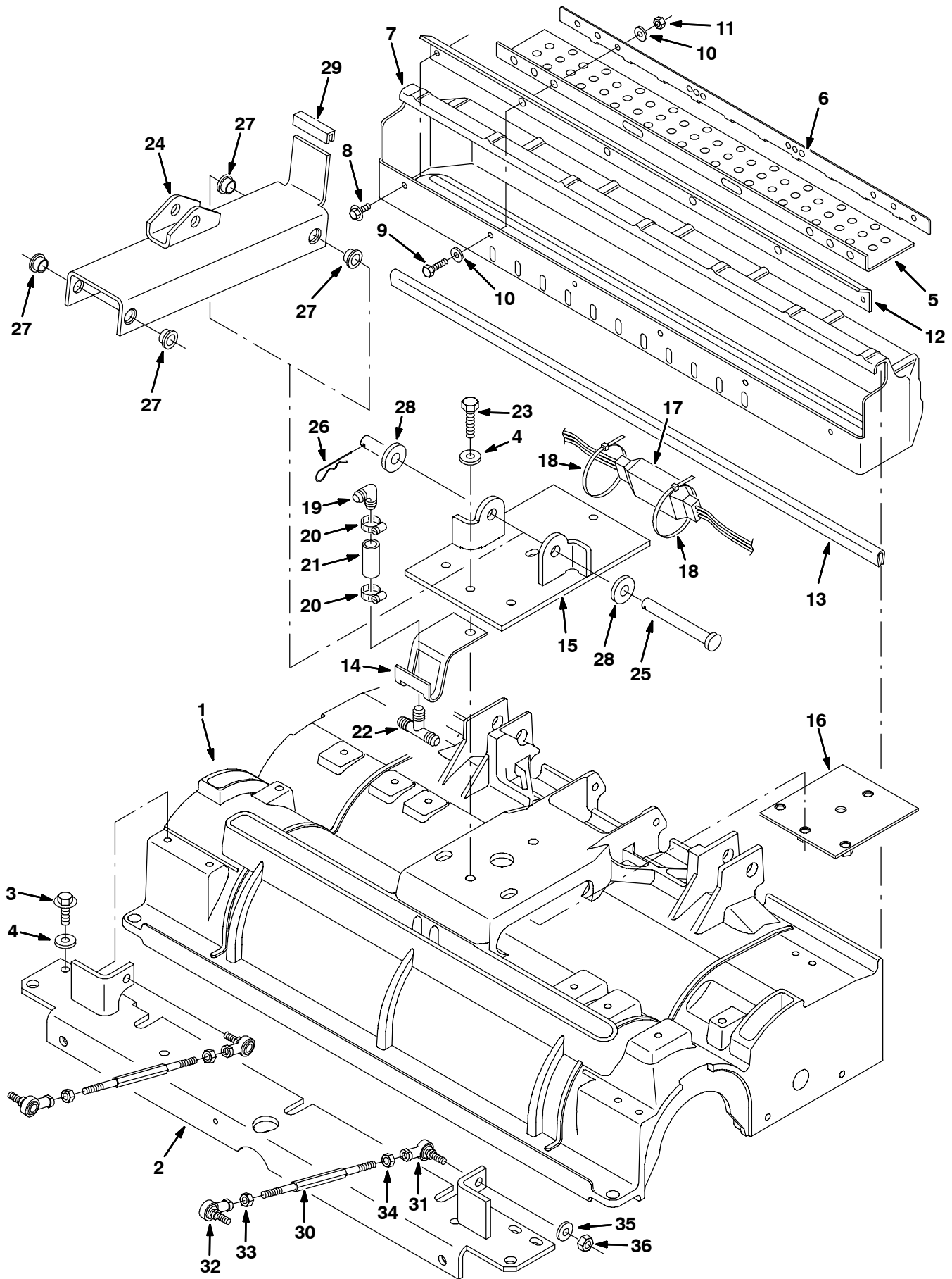
Fig. 26 - Cylindrical Scrub Head Frame Group, 800 mm (32 in)
