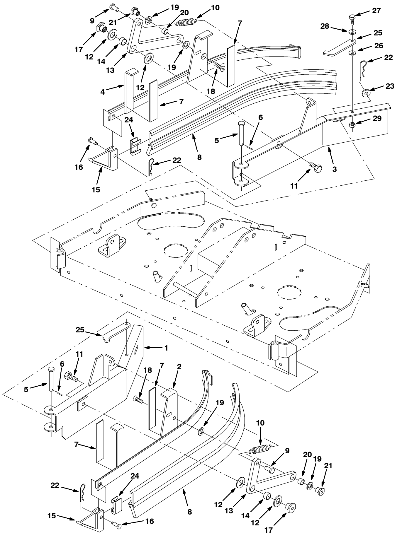
Fig. 29 - Rollout Battery Disk Scrub Head Squeegee Group, 700 mm (28 in)
