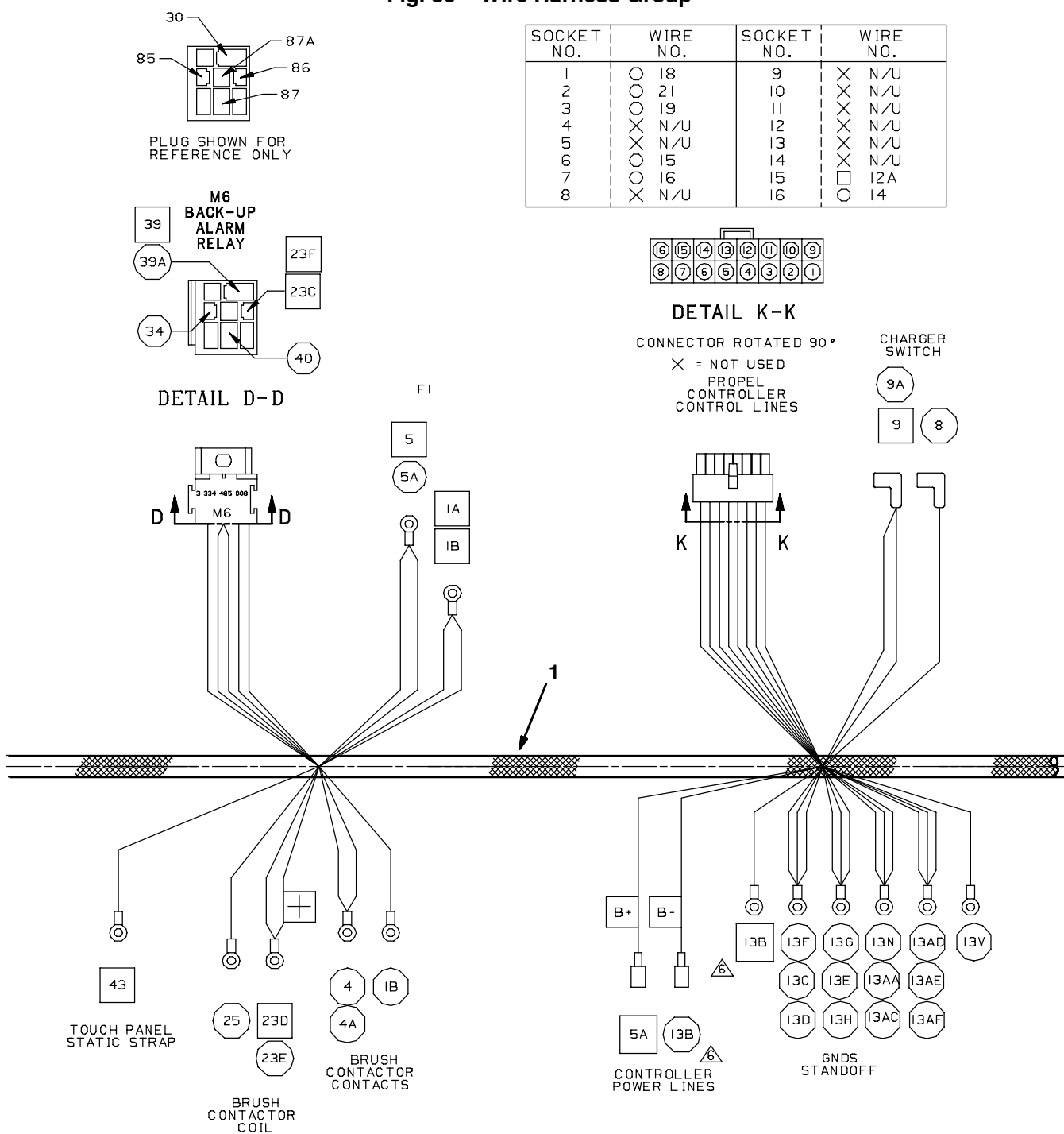
Fig. 30 - Wire Harness Group
