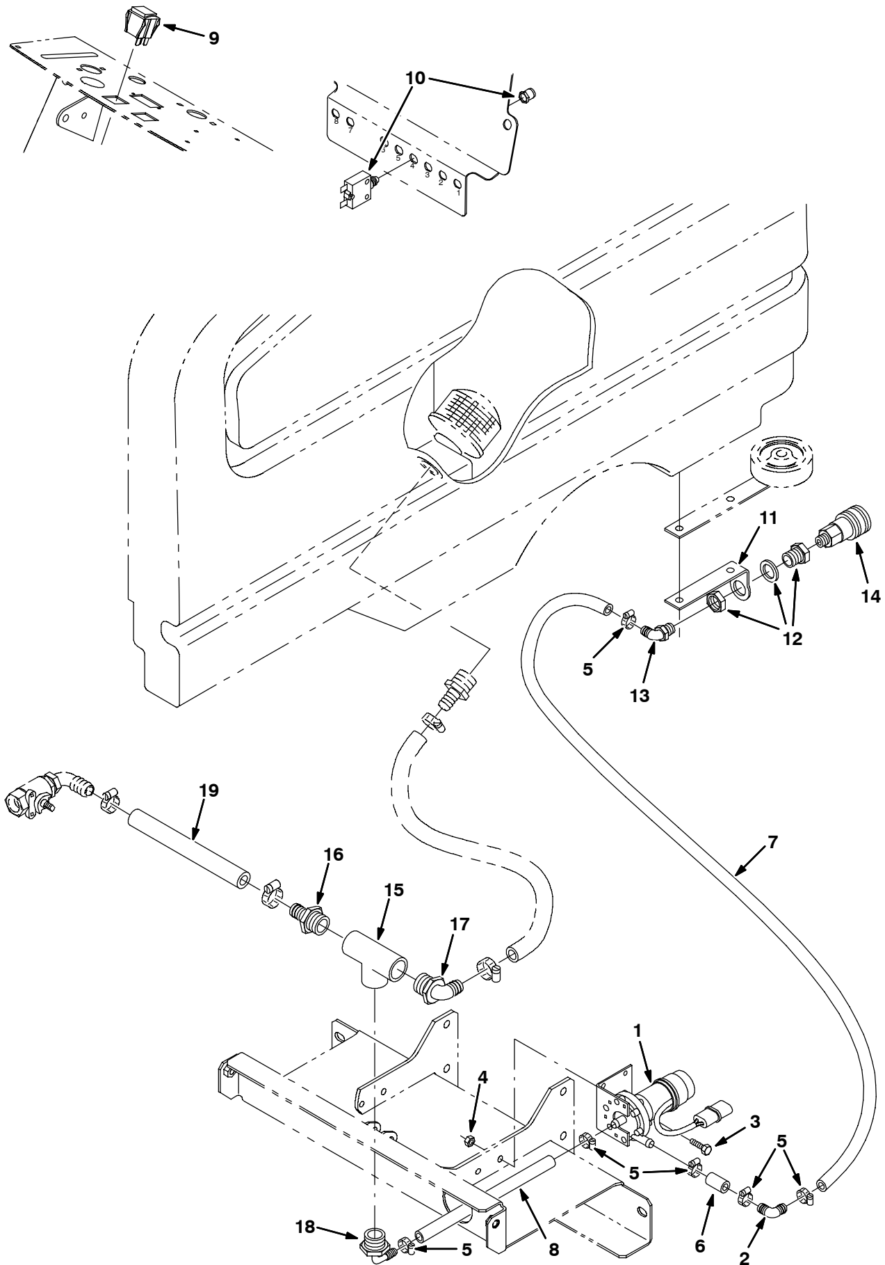
Fig. 13 - Power Wand Pump and Fittings Group
