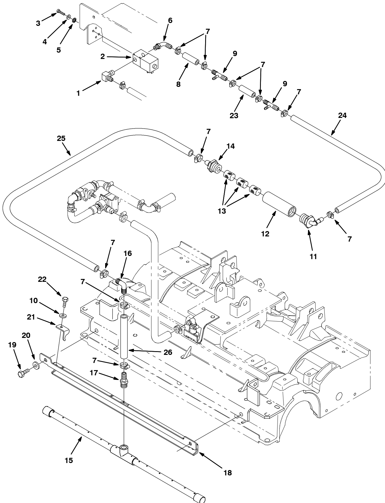
Fig. 7 - FaST Foam Filter Group, Cylindrical Scrub Head, 700 mm (28 in)
