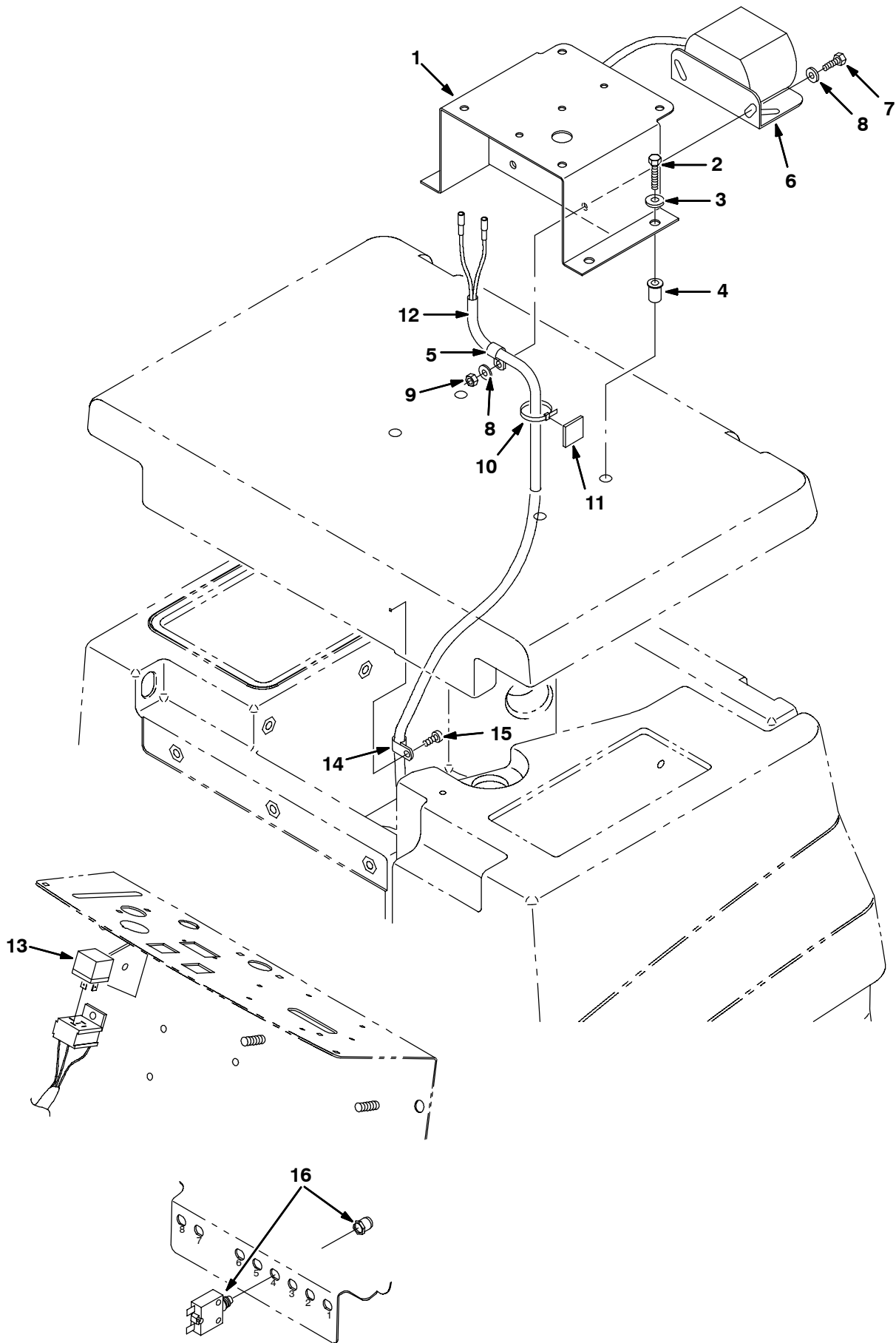
Fig. 46 - Backup Alarm Kit
