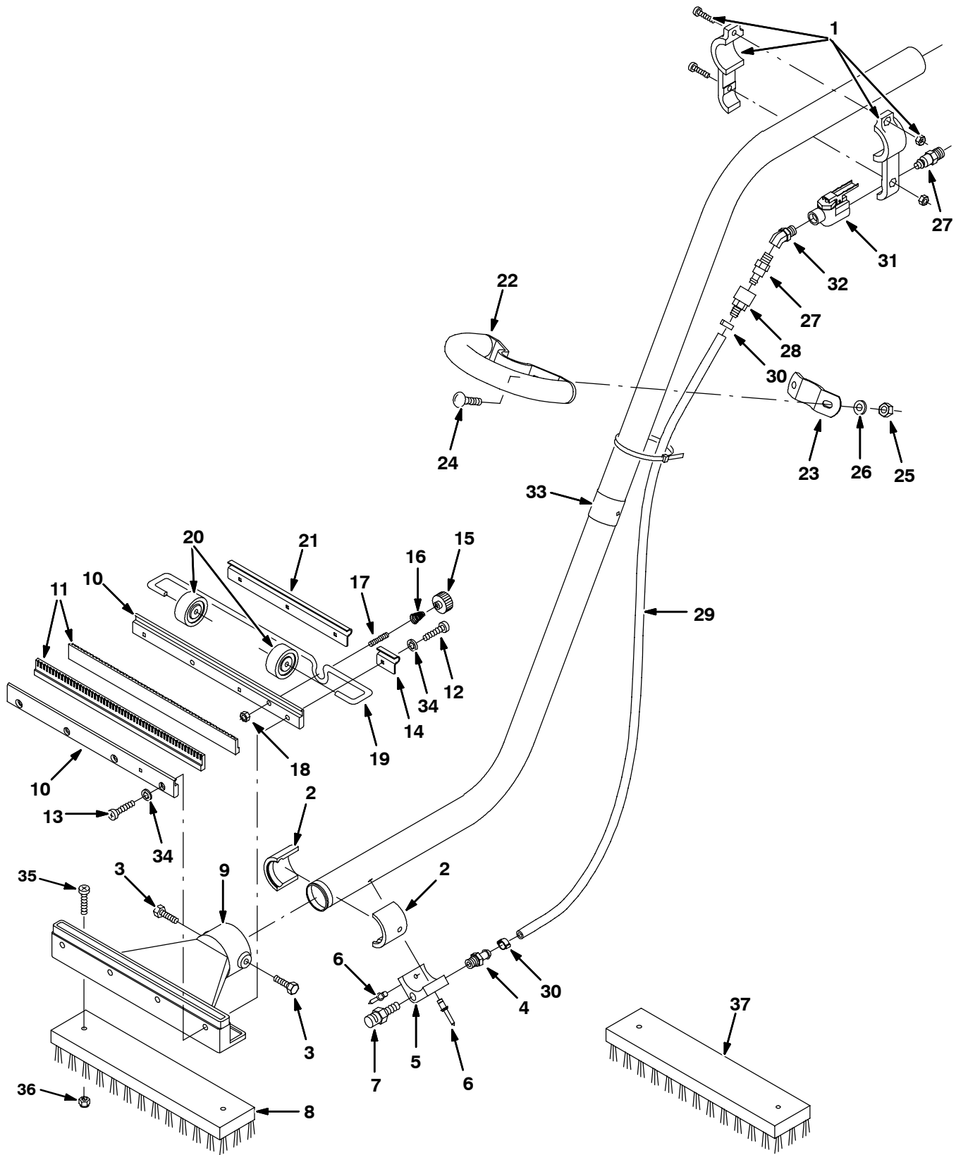
Fig. 16 - Power Wand Assembly
