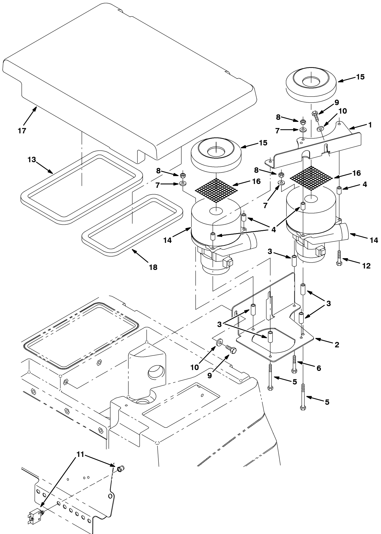
Fig. 17 - Heavy Duty Vacuum Fan Kit
