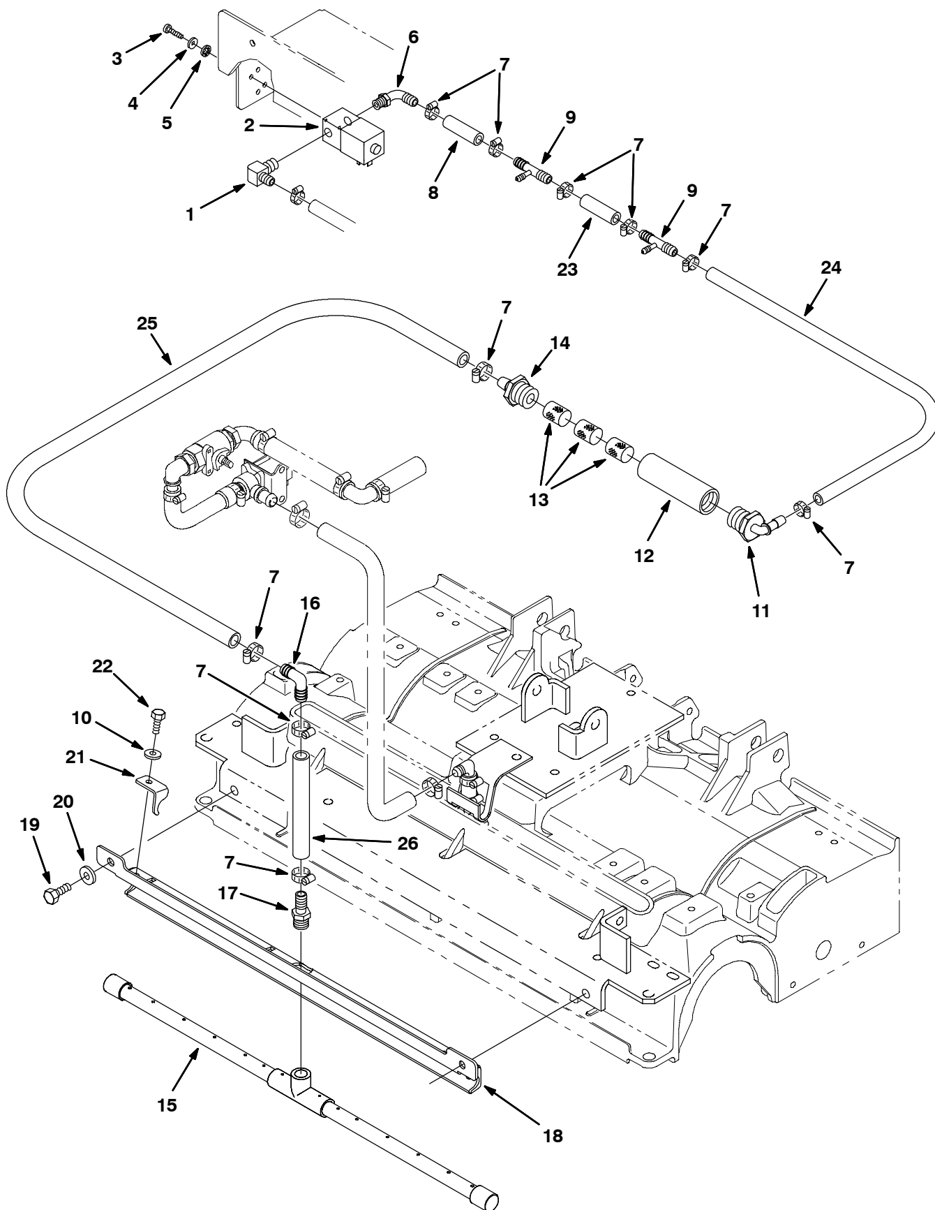
Fig. 8 - FaST Foam Filter Group, Cylindrical Scrub Head, 800 mm (32 in)
