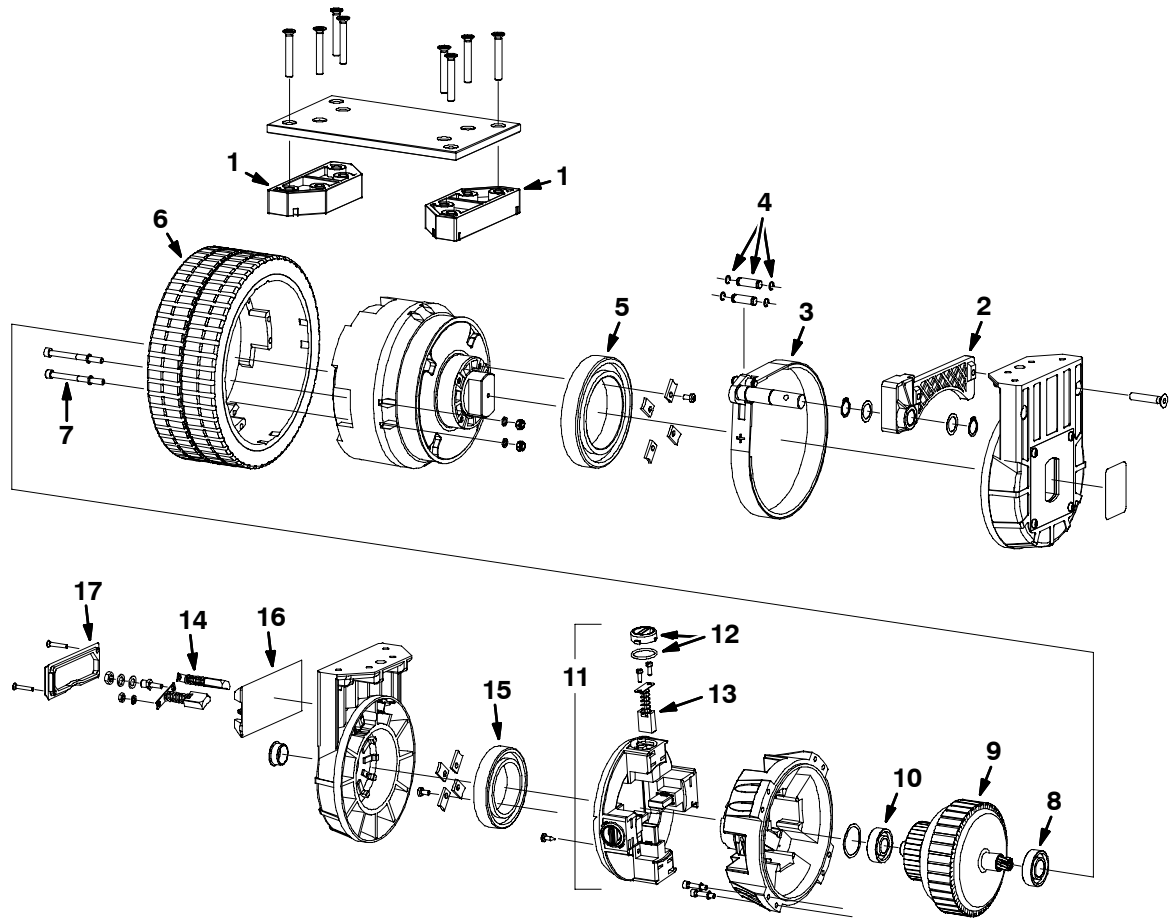
Fig. 9 - Front Wheel Gearbox Breakdown, 374346 (10262872-
