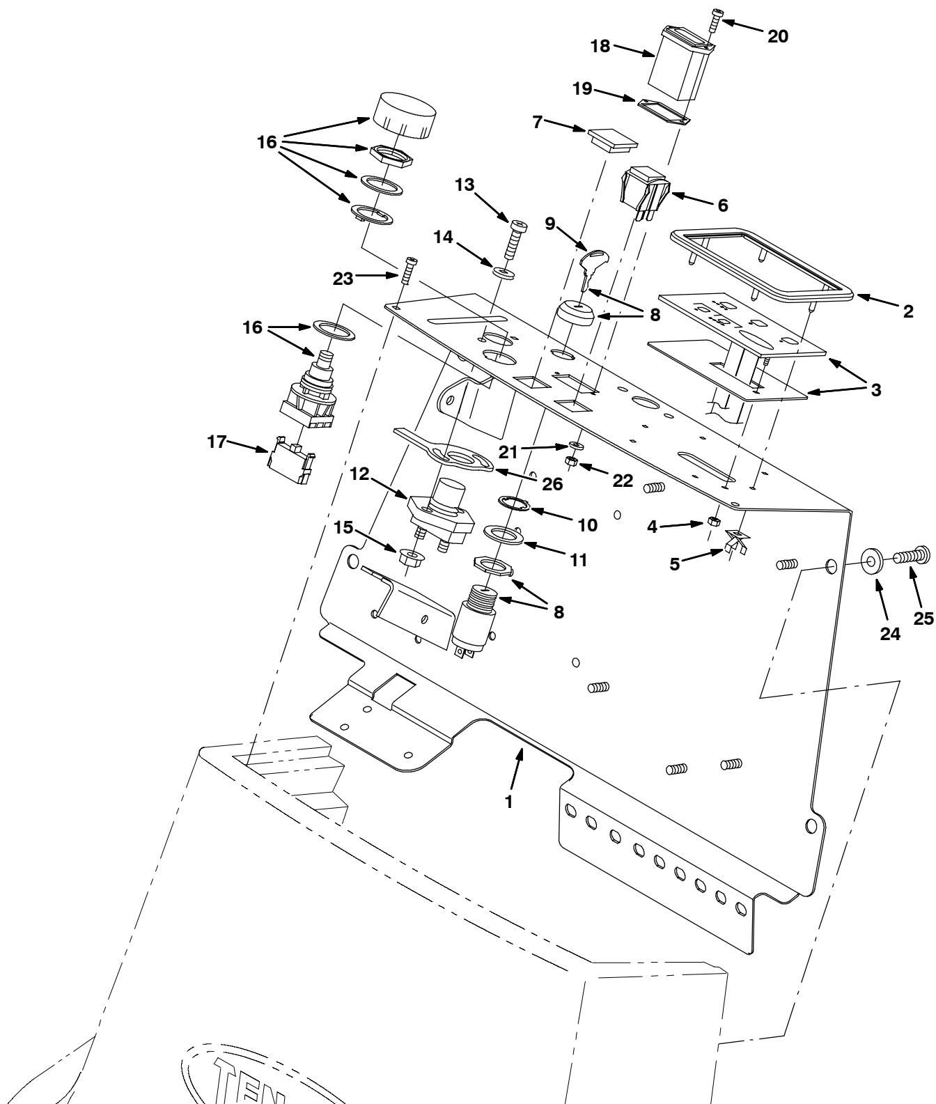
Fig. 8 - Instrument Panel
