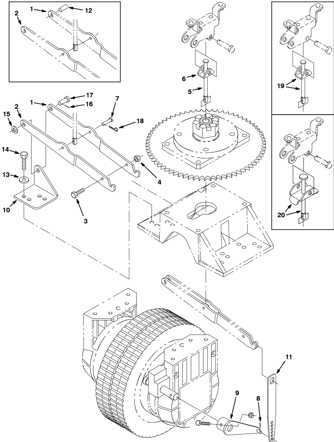
Fig. 13 - Front Brake Linkage Group (10160410-
