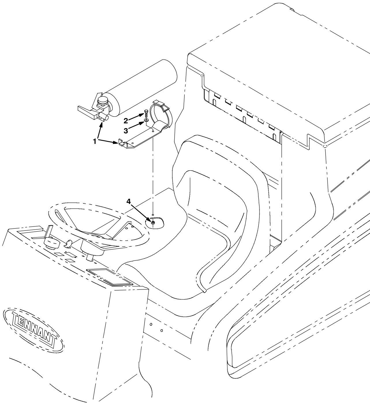
Fig. 47 - Fire Extinguisher Kit
