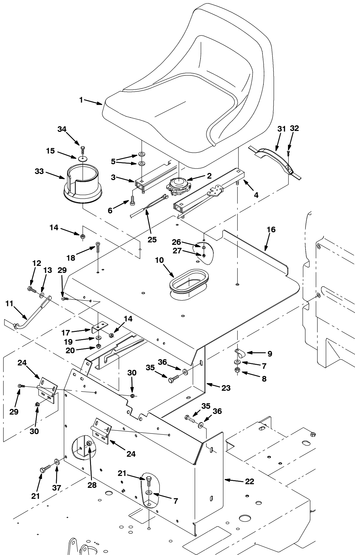
Fig. 6 - Seat Group (10108252- )
