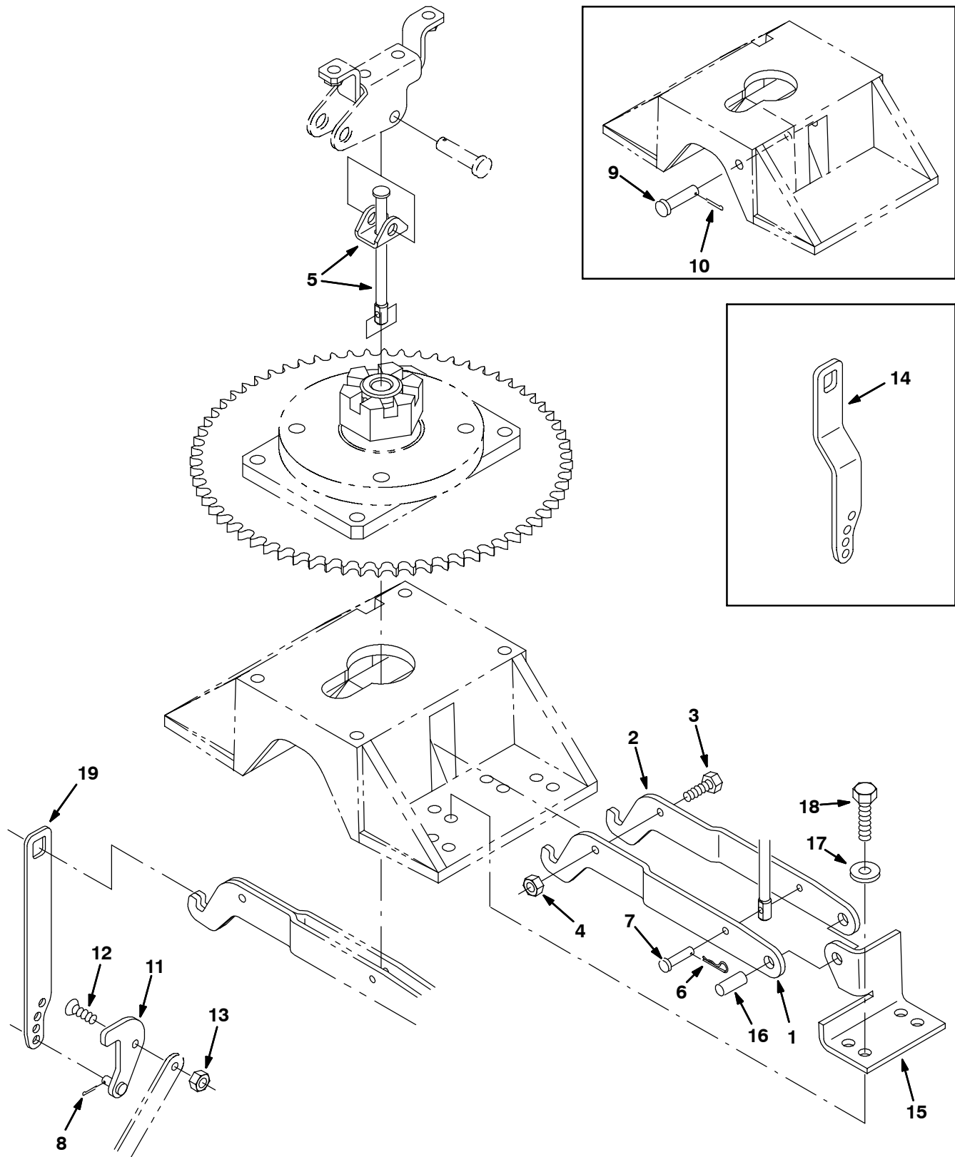
Fig. 12 - Front Brake Linkage Group (00000000-10160409)
