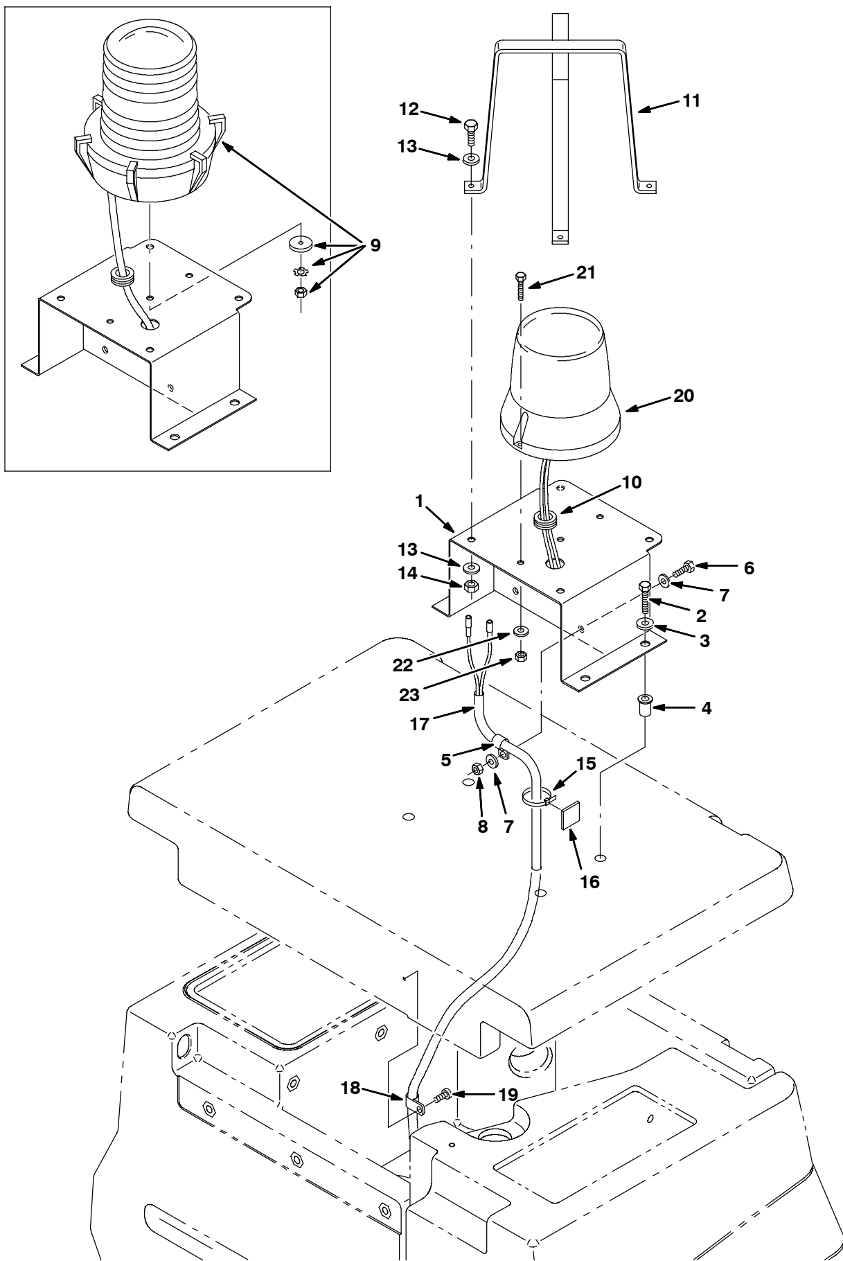
Fig. 45 - Flashing Light Kit
