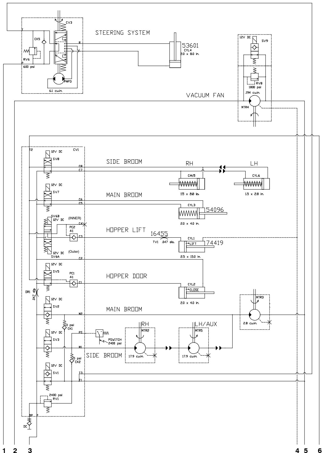
Fig. 66 - Hydraulic Schematic
