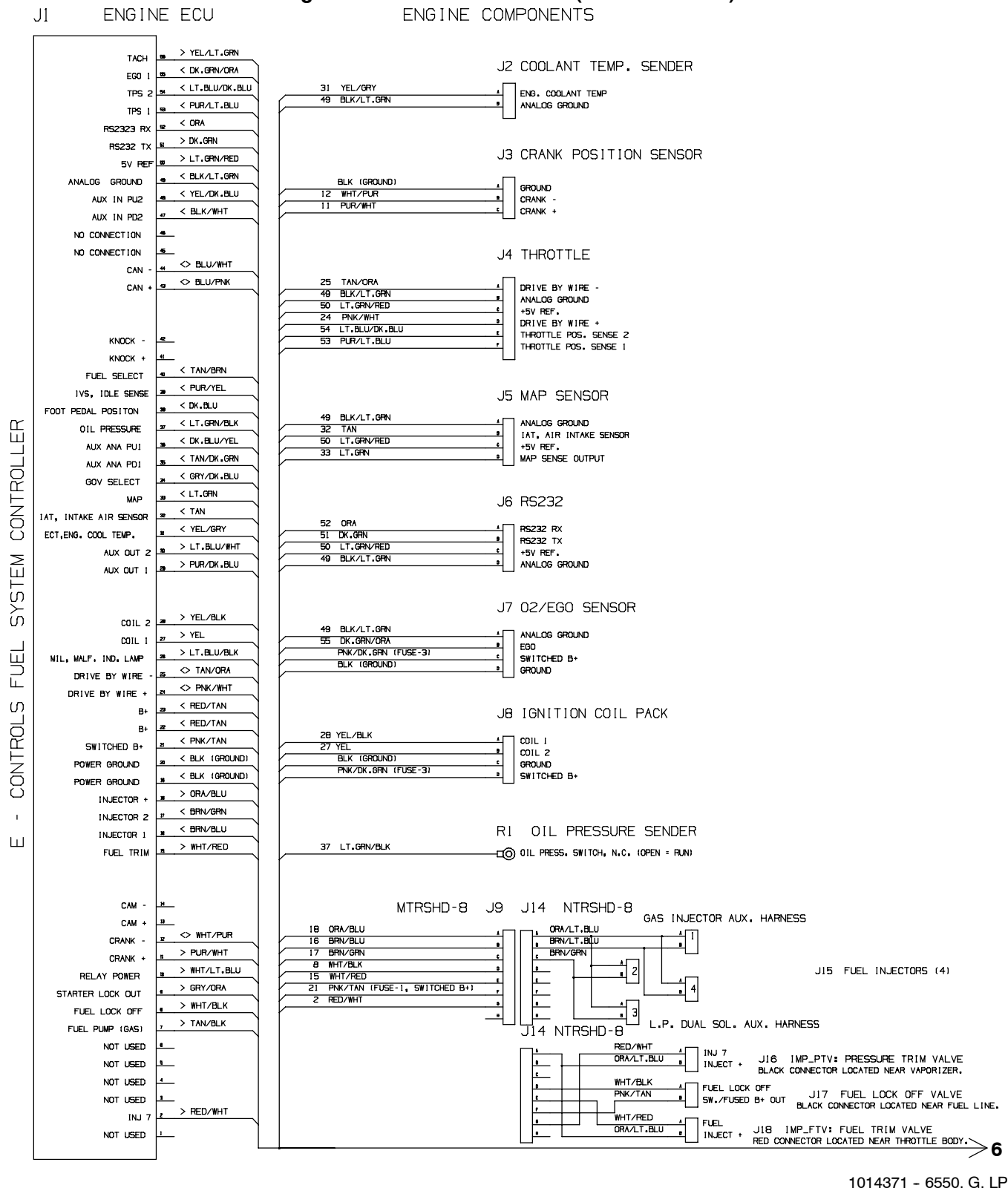
Fig. 74 - Electrical Schematic (010000-014999)
