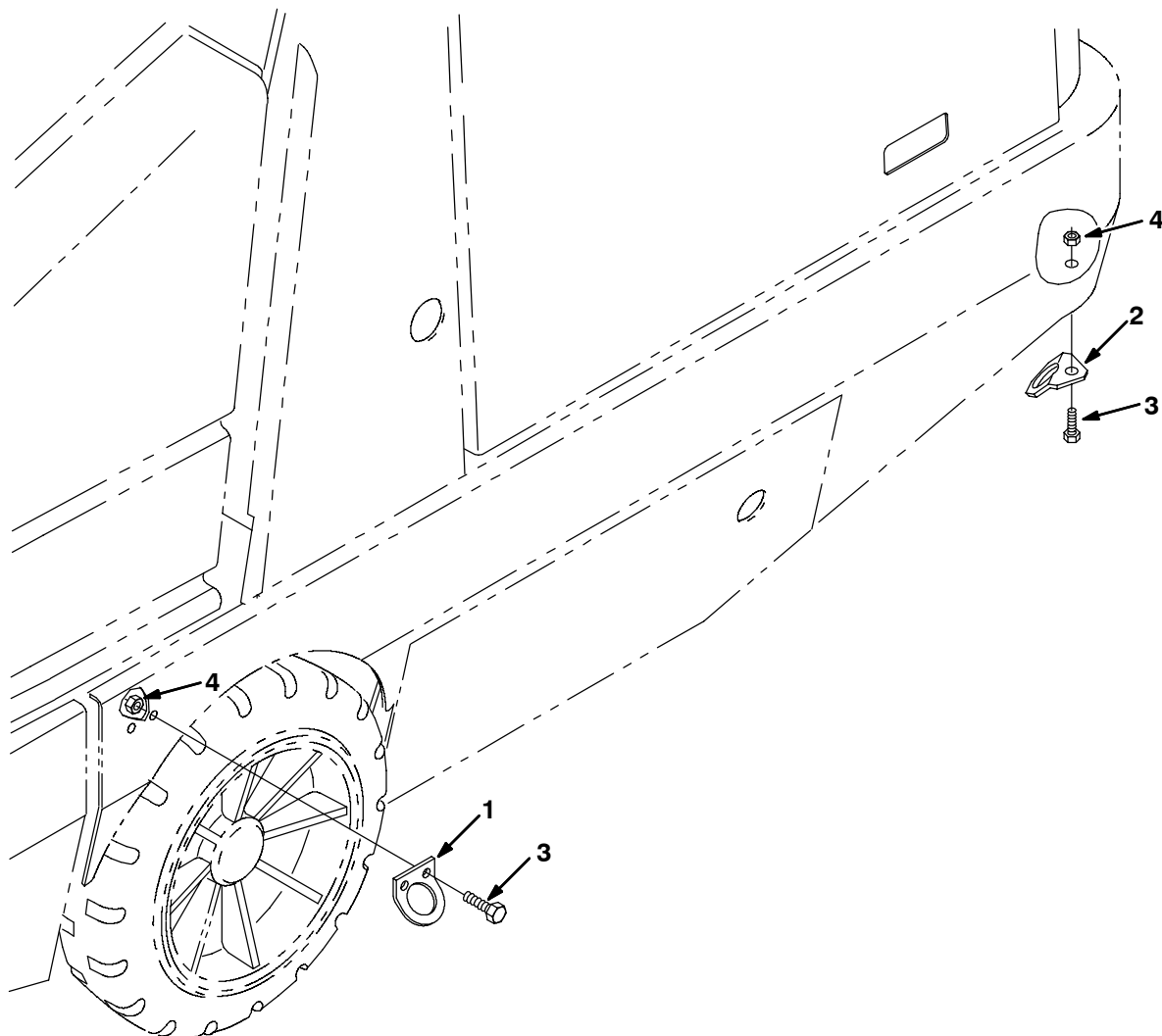
Fig. 50 - Transport Kit
