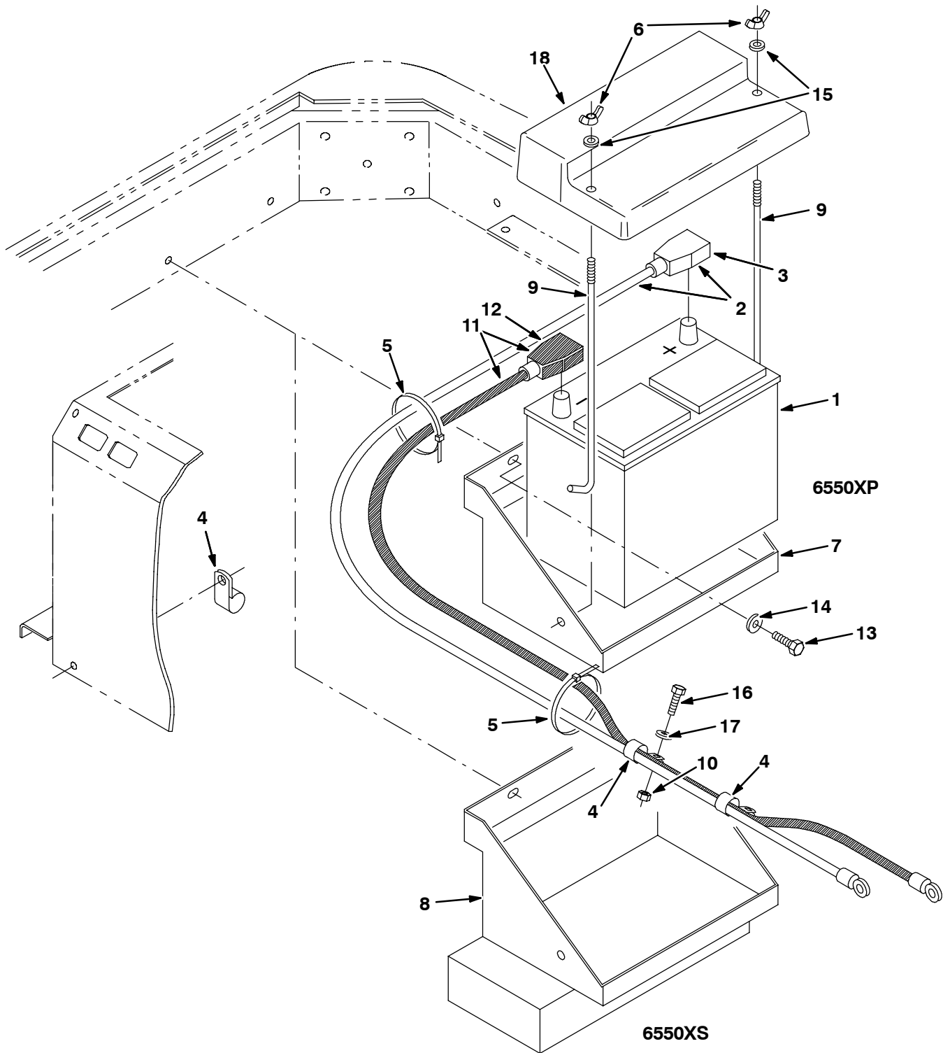
Fig. 44 - Battery Group, LPG
