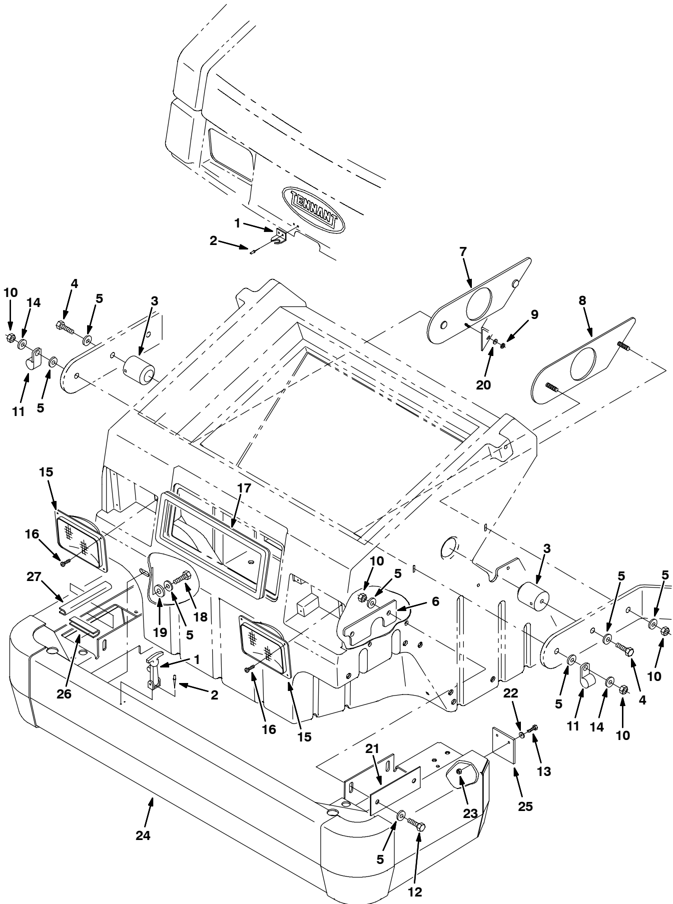
Fig. 56 - Hopper Bumper Group (6650 XP)
