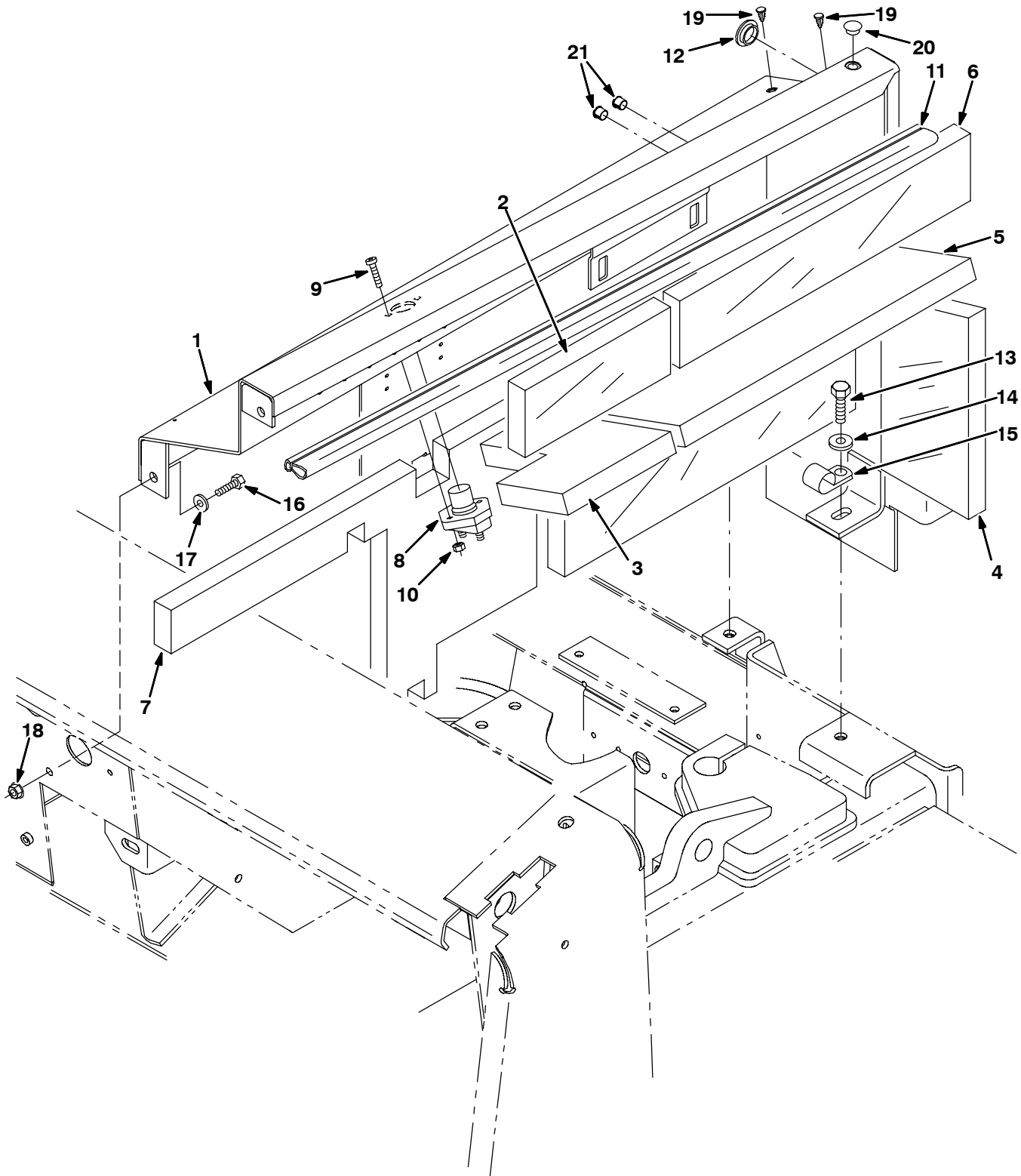
Fig. 13 - Side Instrument Panel Group
