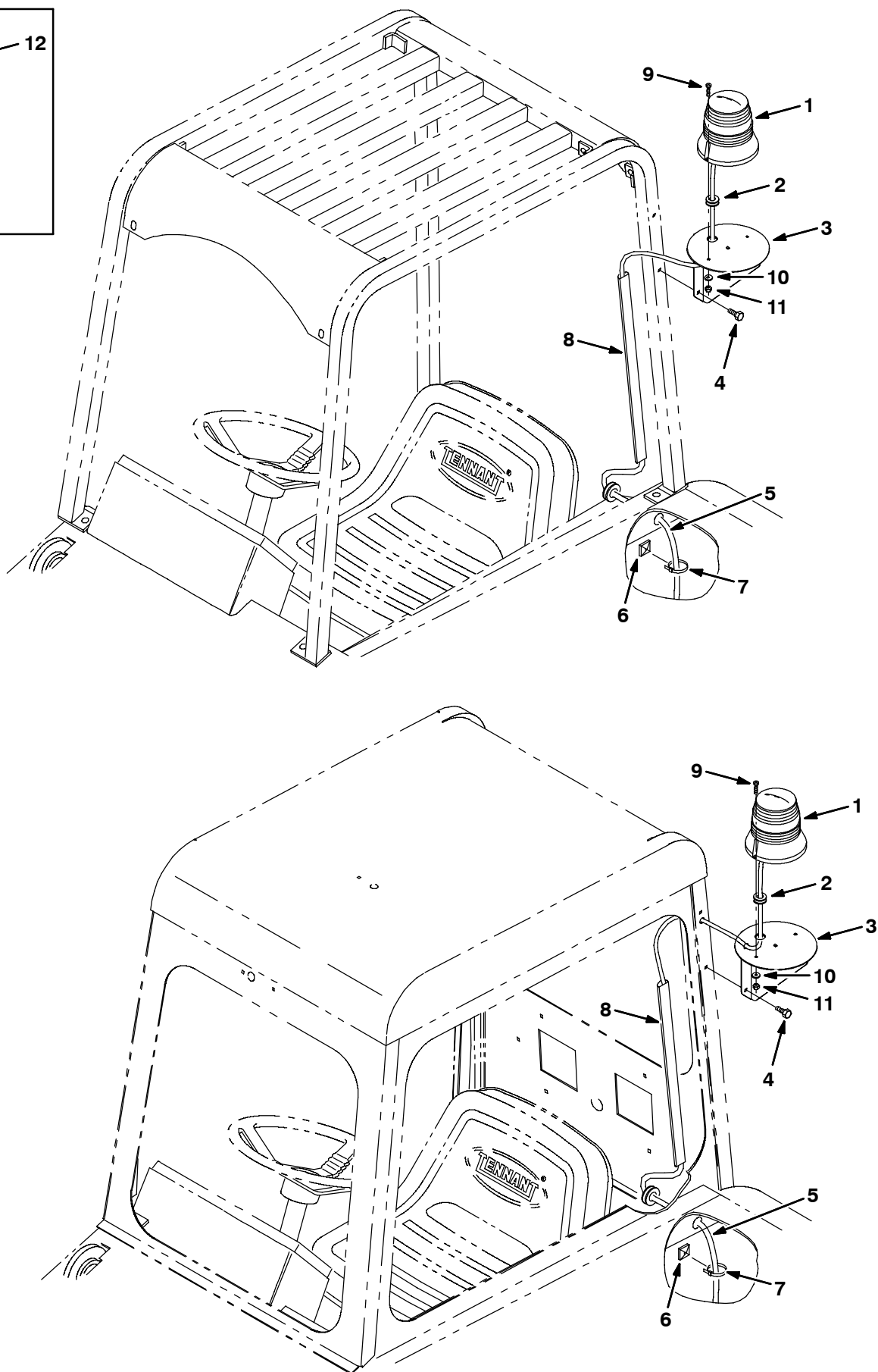
Fig. 9 - Revolving Light Kit, Flush Mounting
