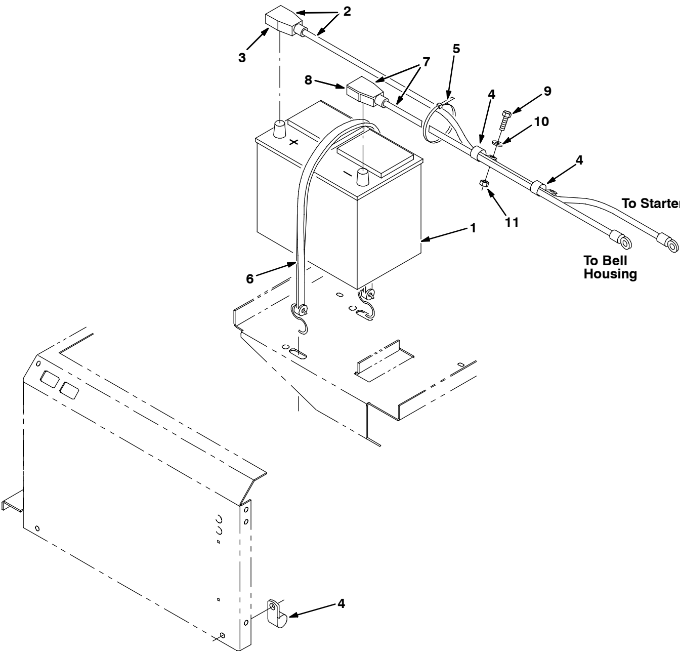
Fig. 43 - Battery Group, Gasoline
