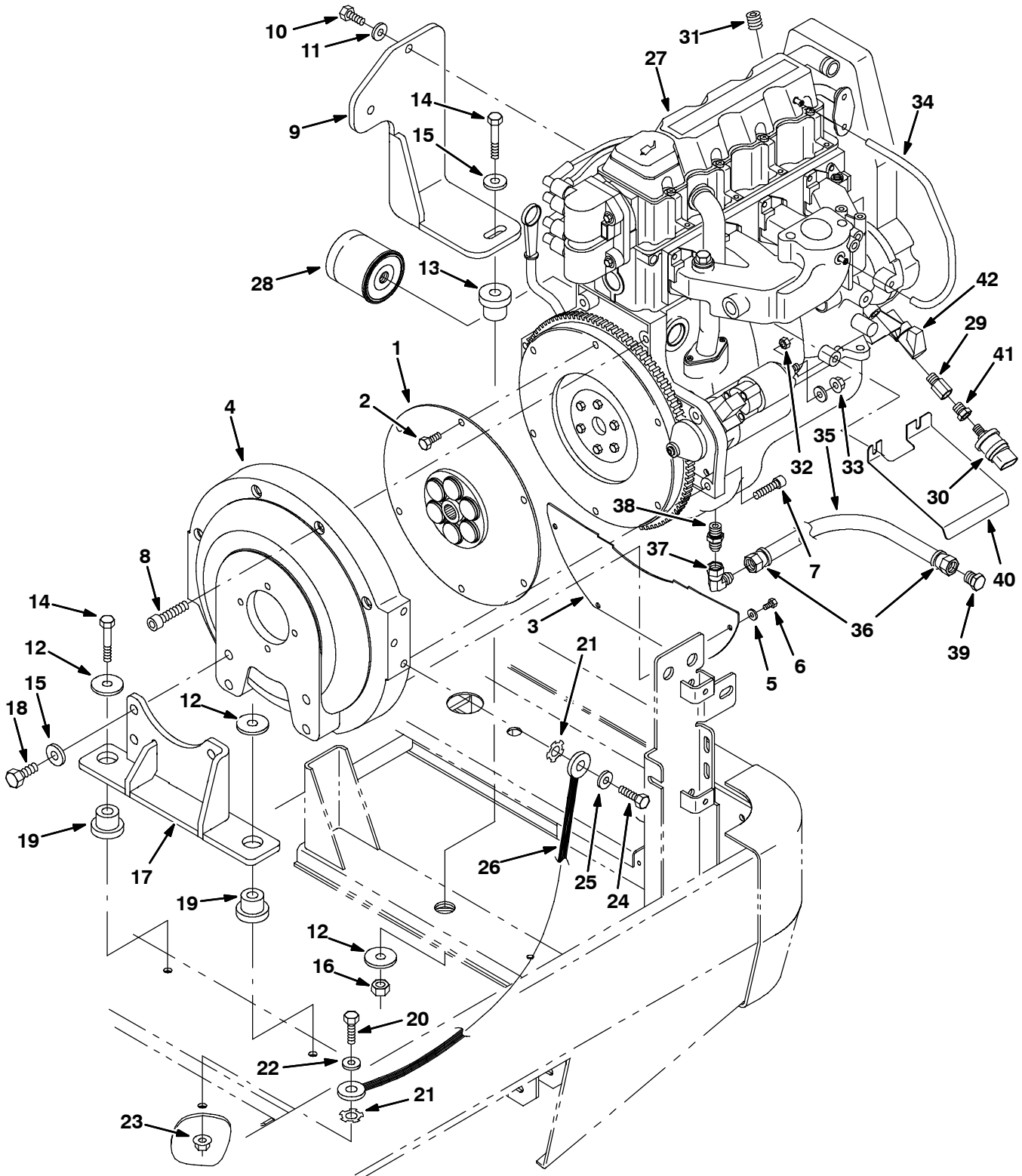
Fig. 15 - Engine Group, Gasoline (000000-009999)
