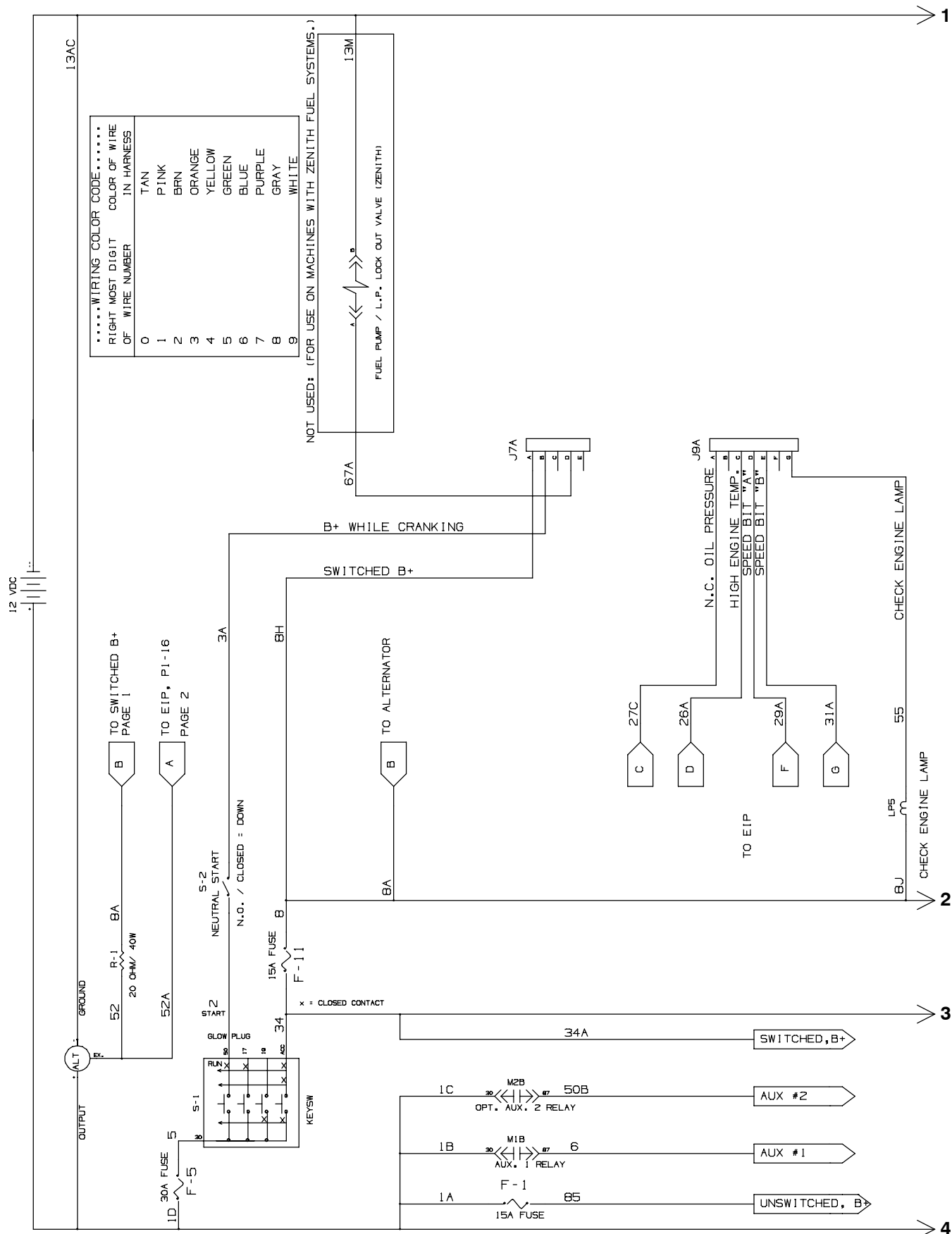
Fig. 75 - Electrical Schematic (015000- )
