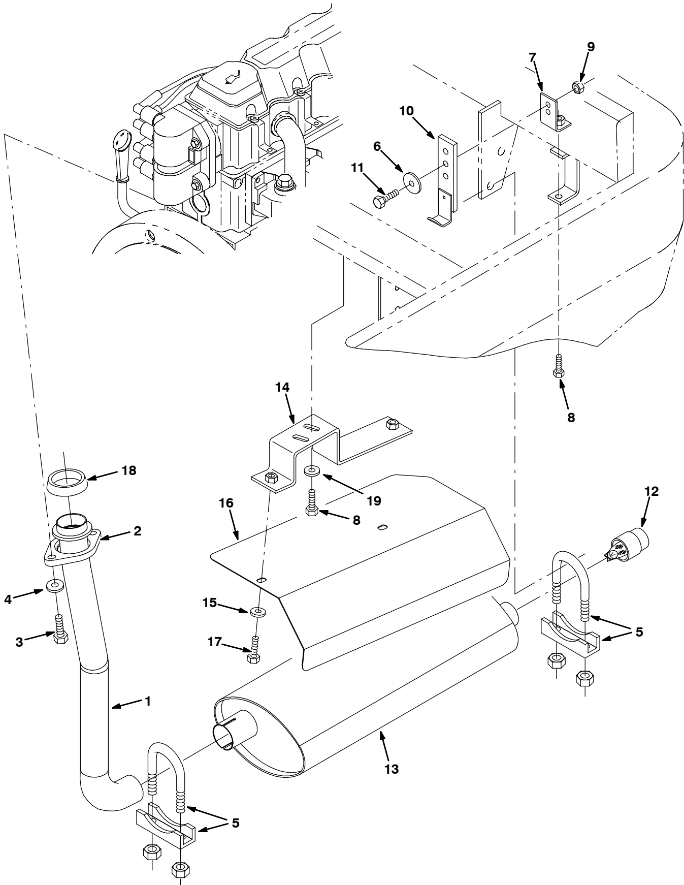
Fig. 31 - Engine Muffler Group (000000-009999)
