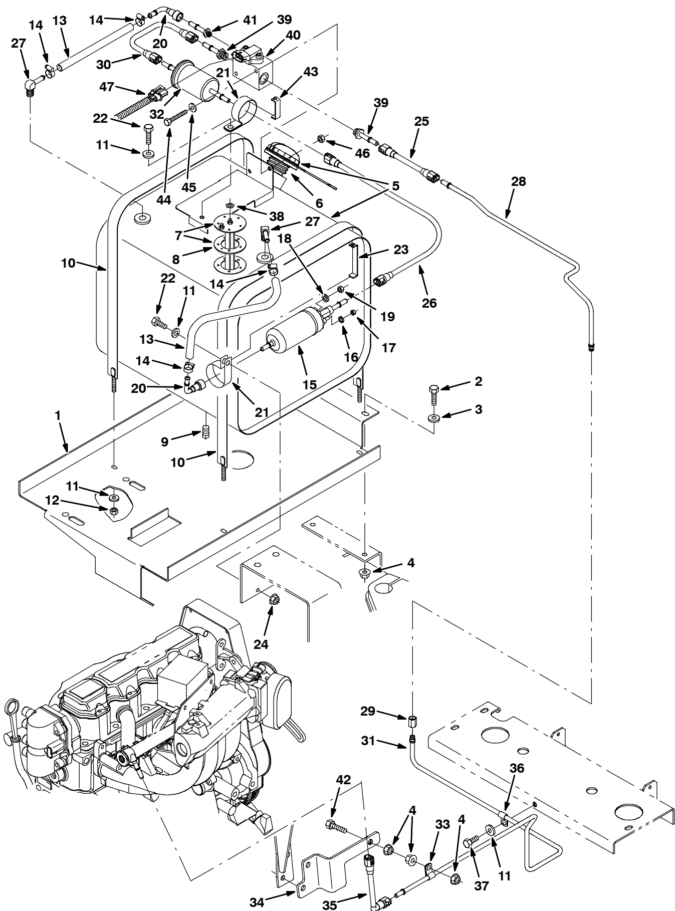
Fig. 36 - Engine Fuel Tank Group, Gasoline (015000- )
