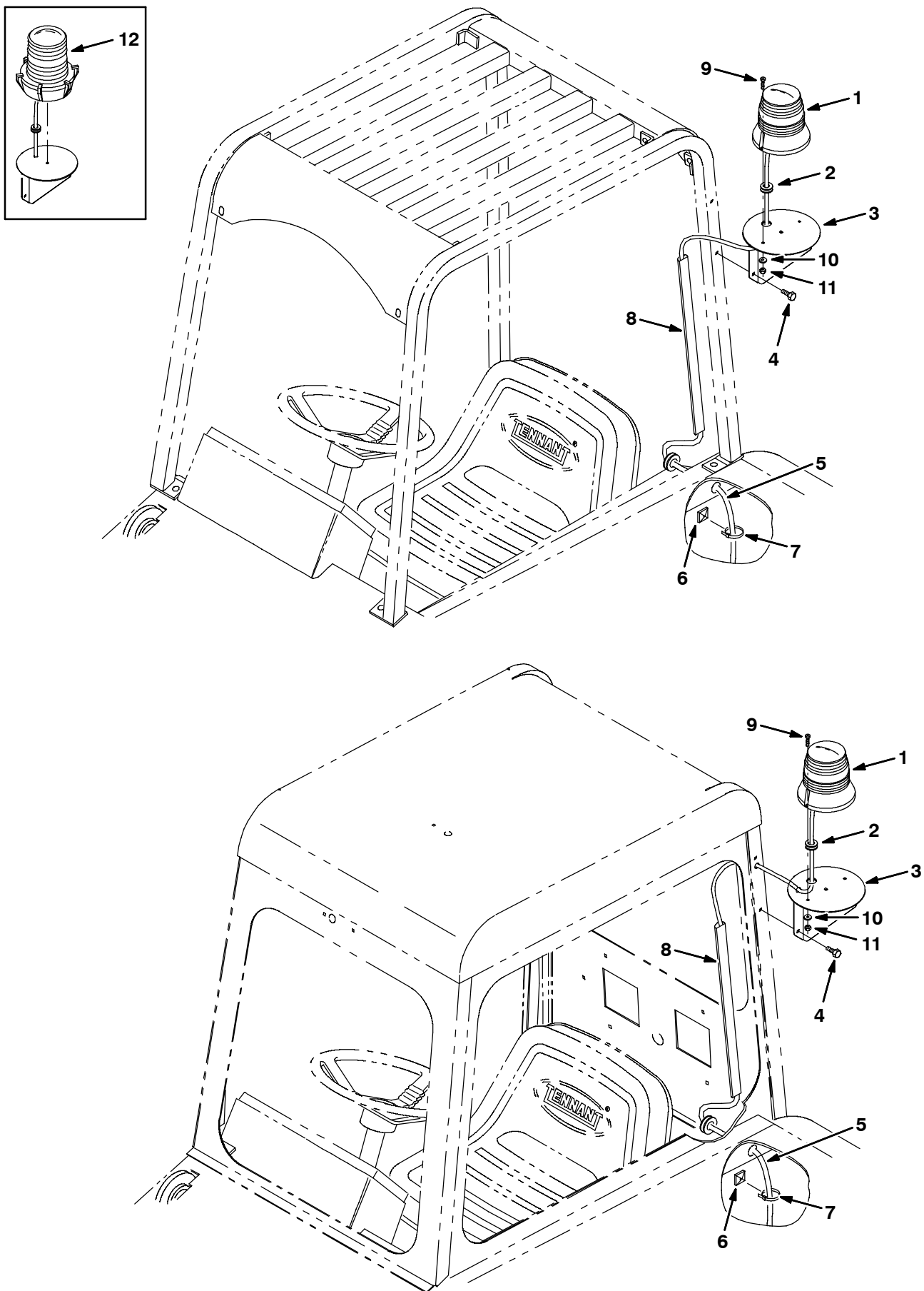
Fig. 8 - Flashing Light Kit, Flush Mounting
