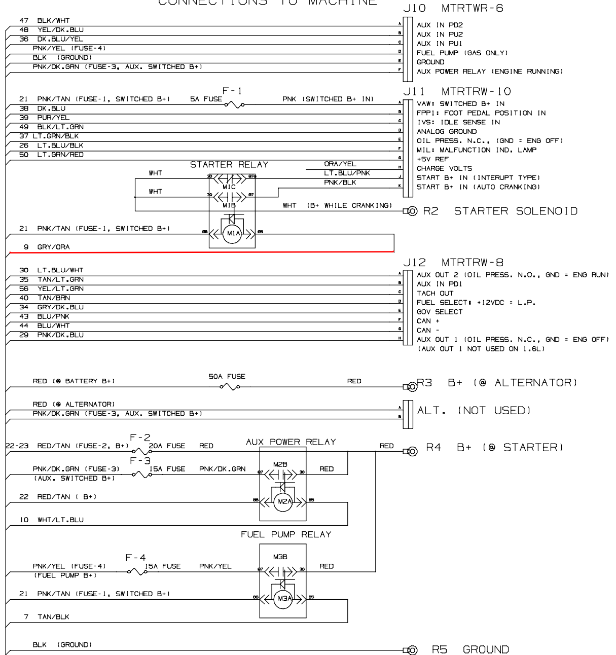
Fig. 74 - Electrical Schematic (010000-014999)
