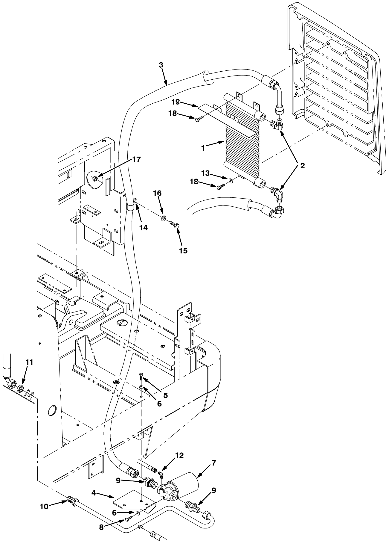
Fig. 69 - Hydraulic Cooler Group (000000-009999)
