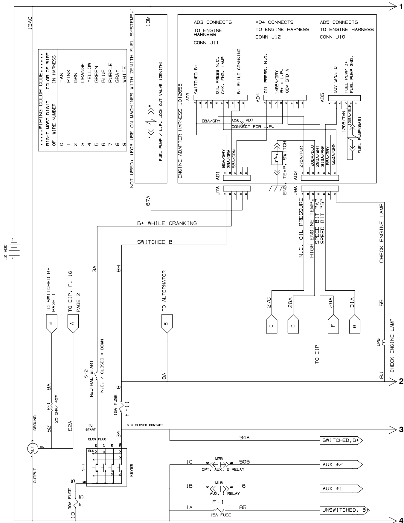
Fig. 74 - Electrical Schematic (010000-014999)
