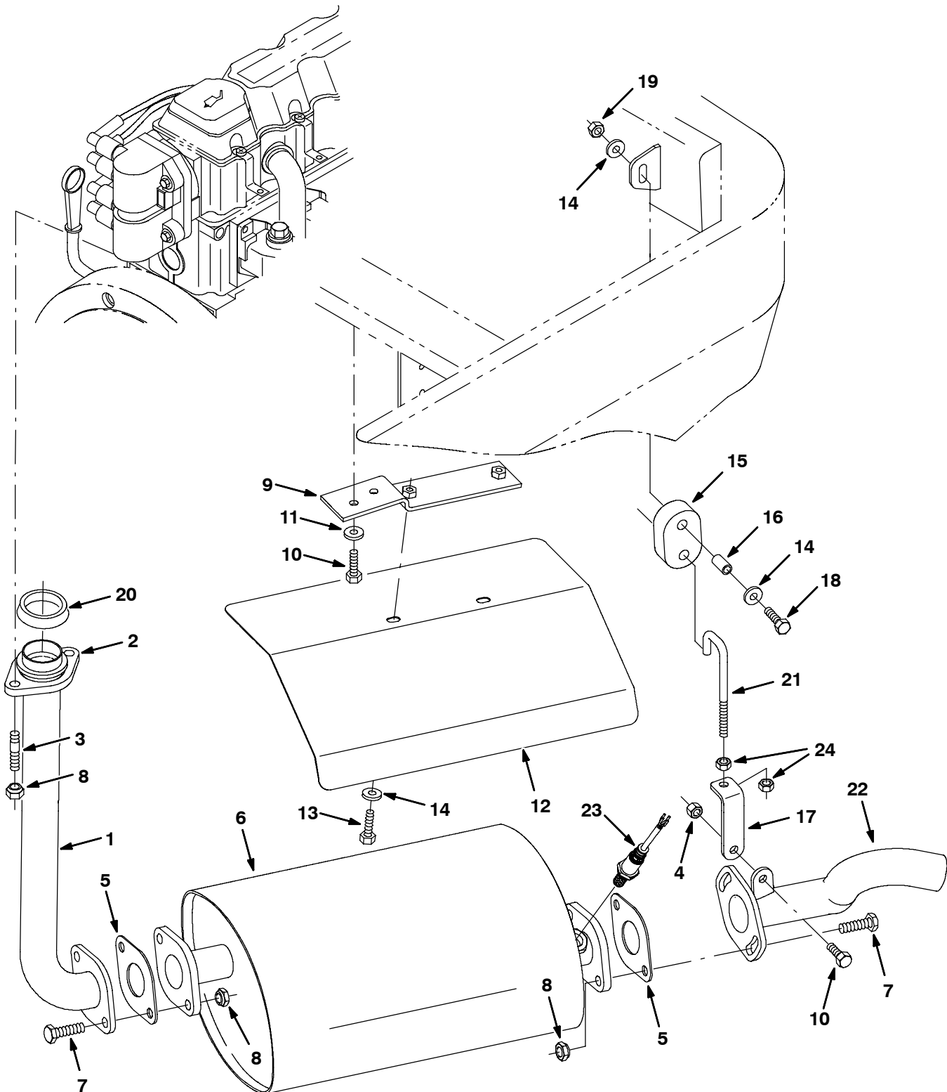
Fig. 33 - Engine Muffler Group (015000- )
