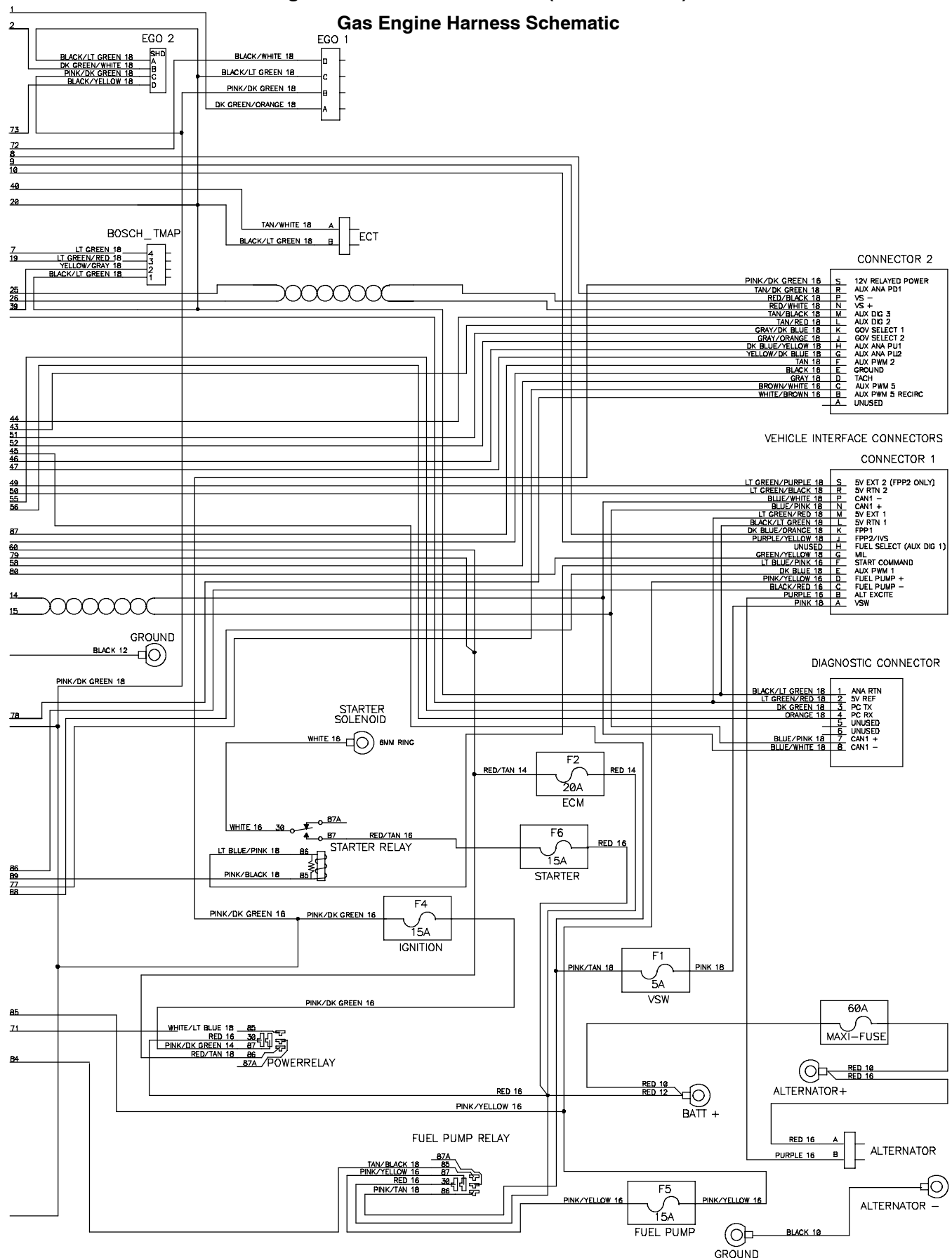
Fig. 75 - Electrical Schematic (015000-
