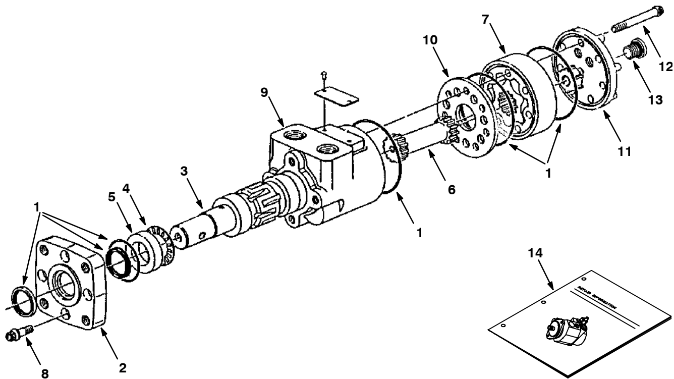
Fig. 6 - Hydraulic Motor Breakdown, 373340
