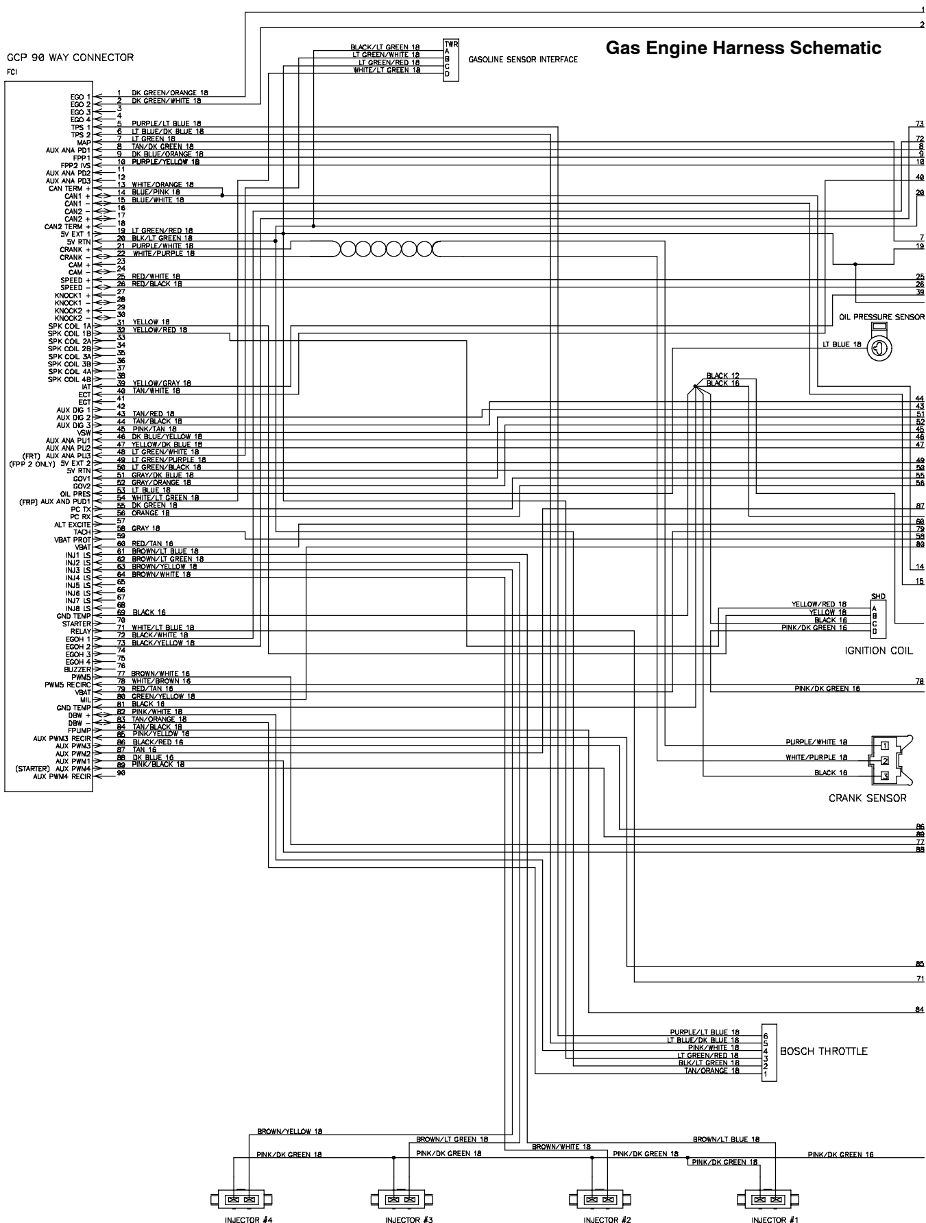
Fig. 75 - Electrical Schematic (015000- )
