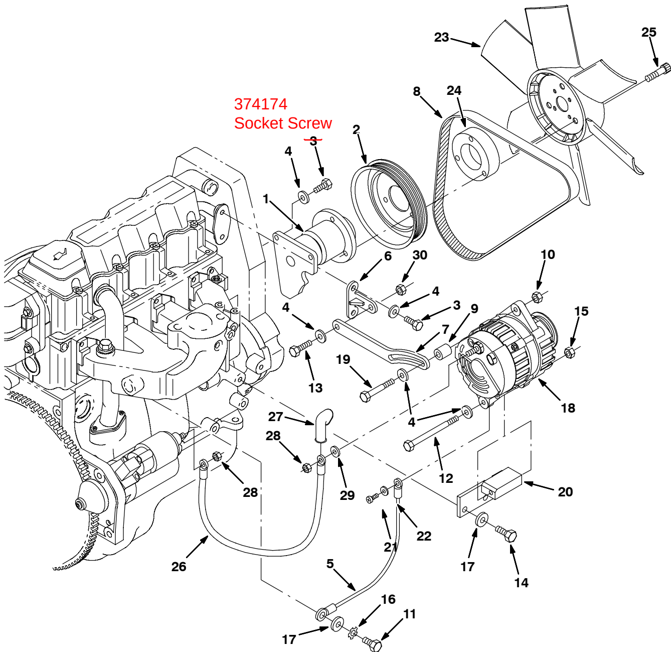
Fig. 29 - Engine Alternator and Engine Fan Group (000000-009999)
