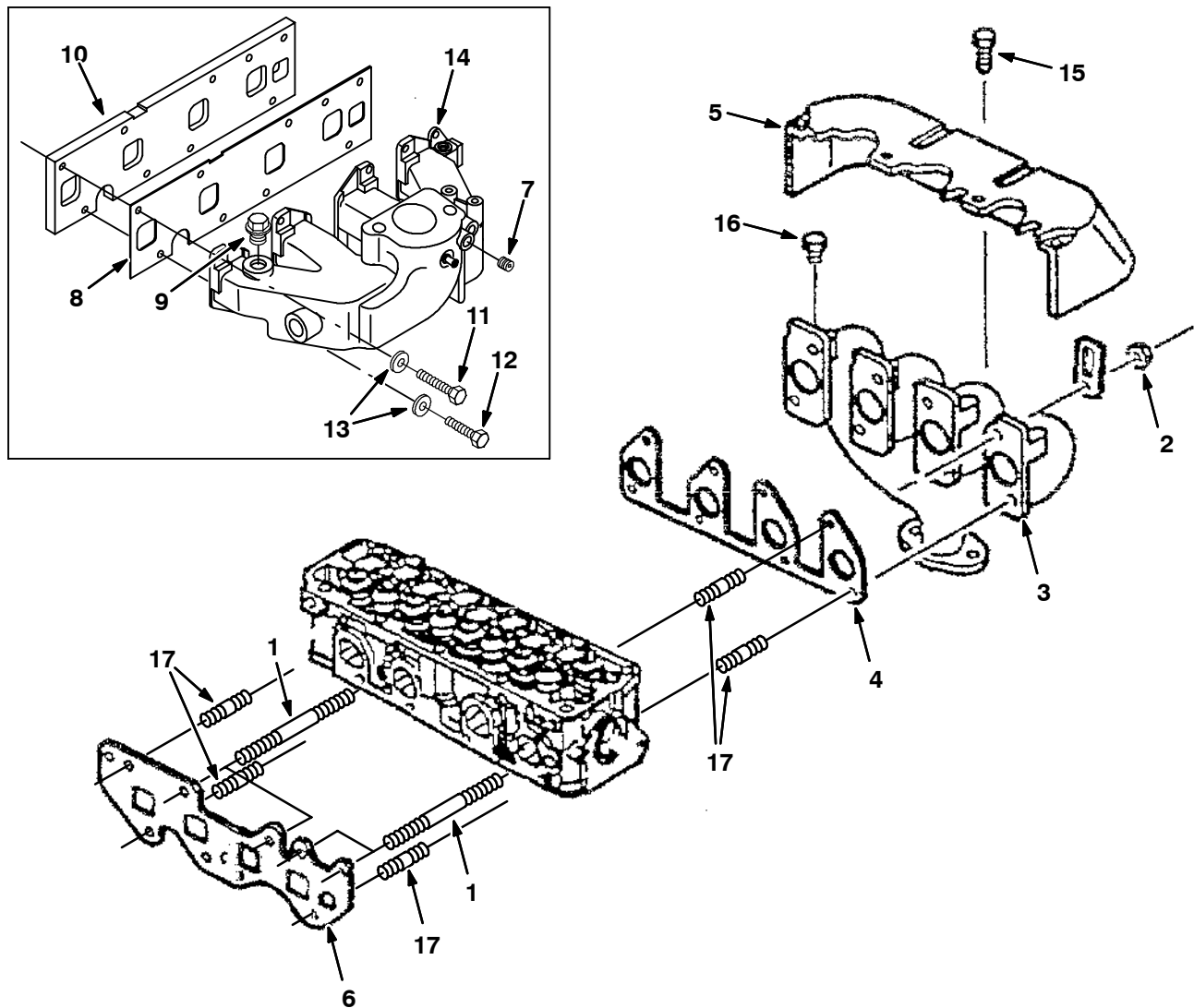
Fig. 5 - Manifold Group
