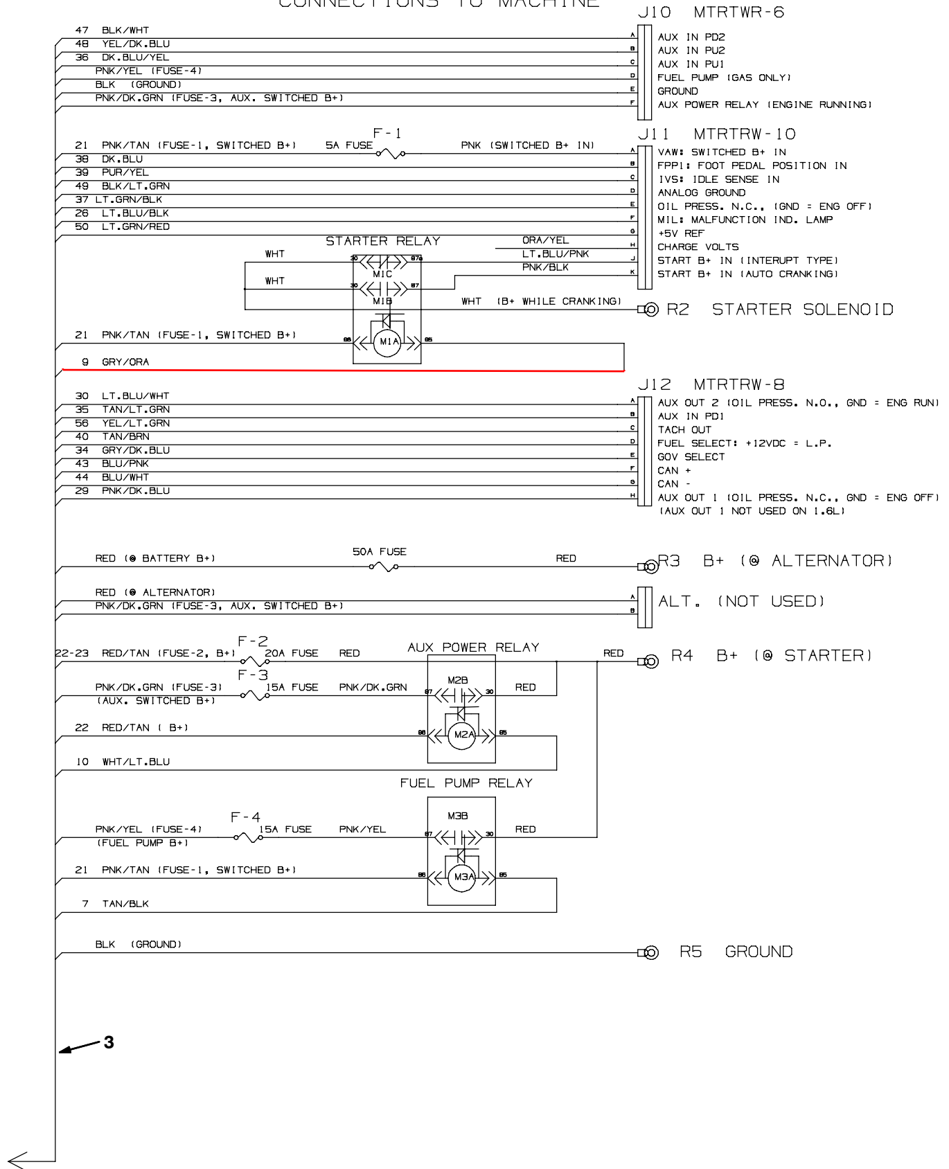
Fig. 76 - Electrical Wire Harness Group CONNECTIONS TO MACHINE
