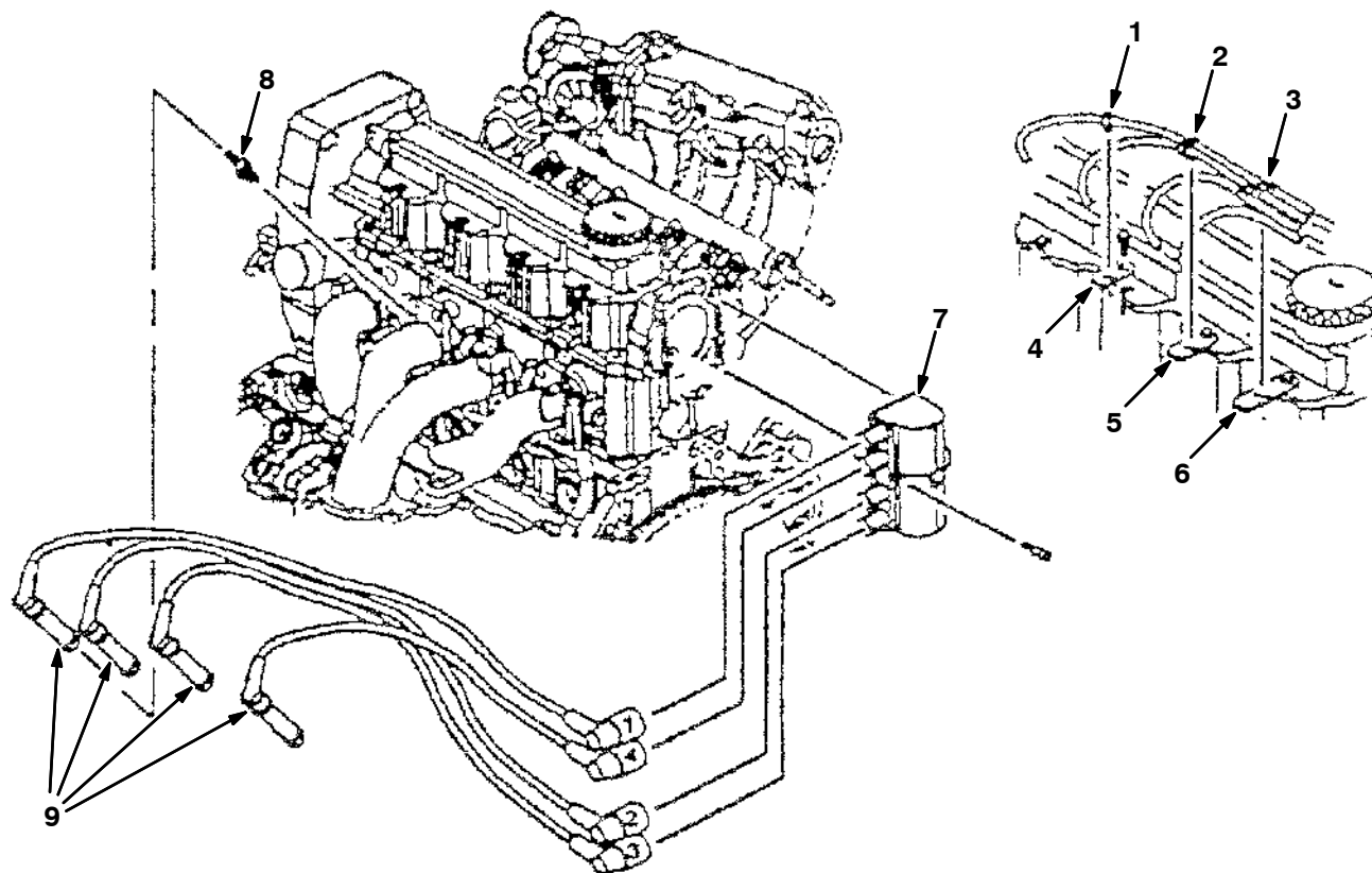
Fig. 7 - Ignition Group
