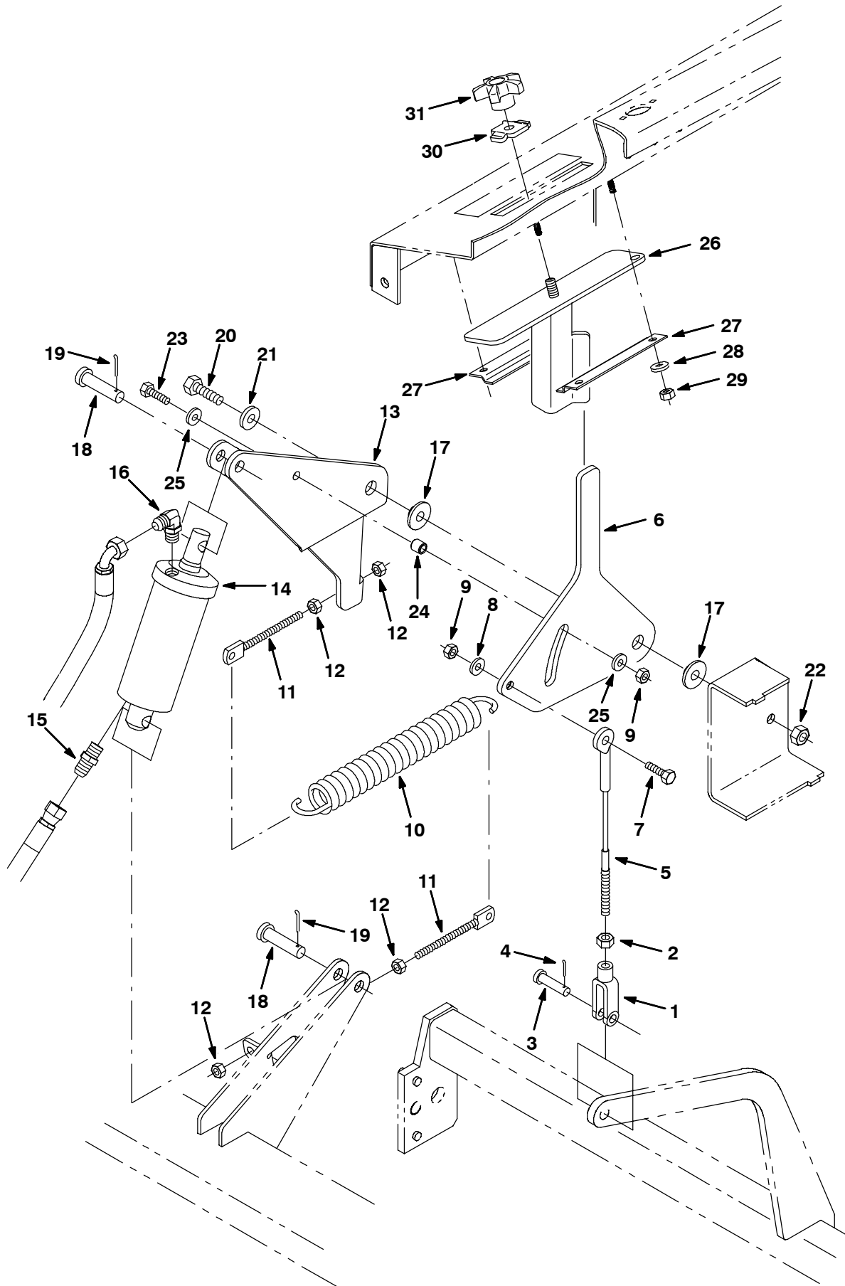
Fig. 63 - Main Brush Lift Group
