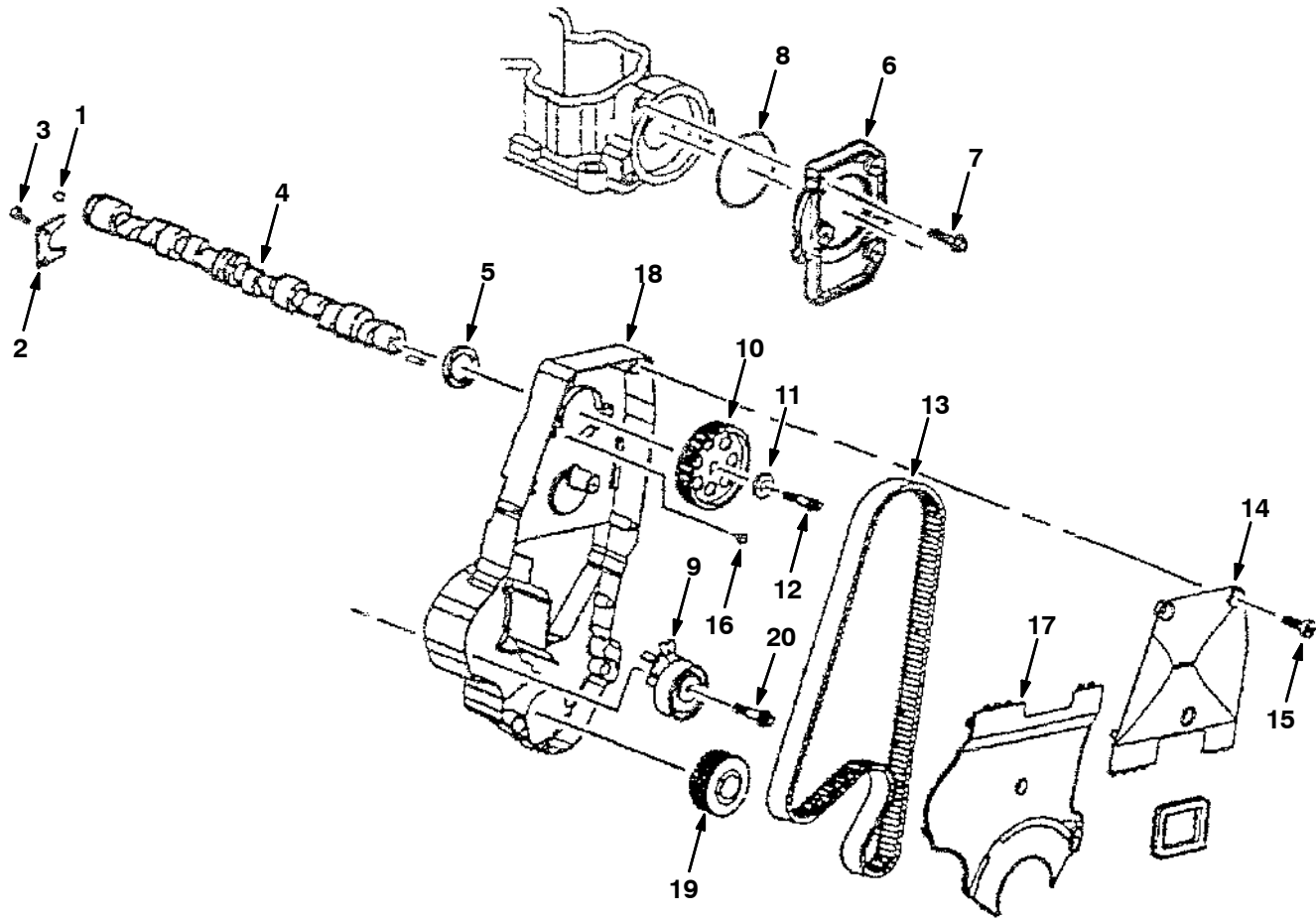
Fig. 6 - Camshaft Group
