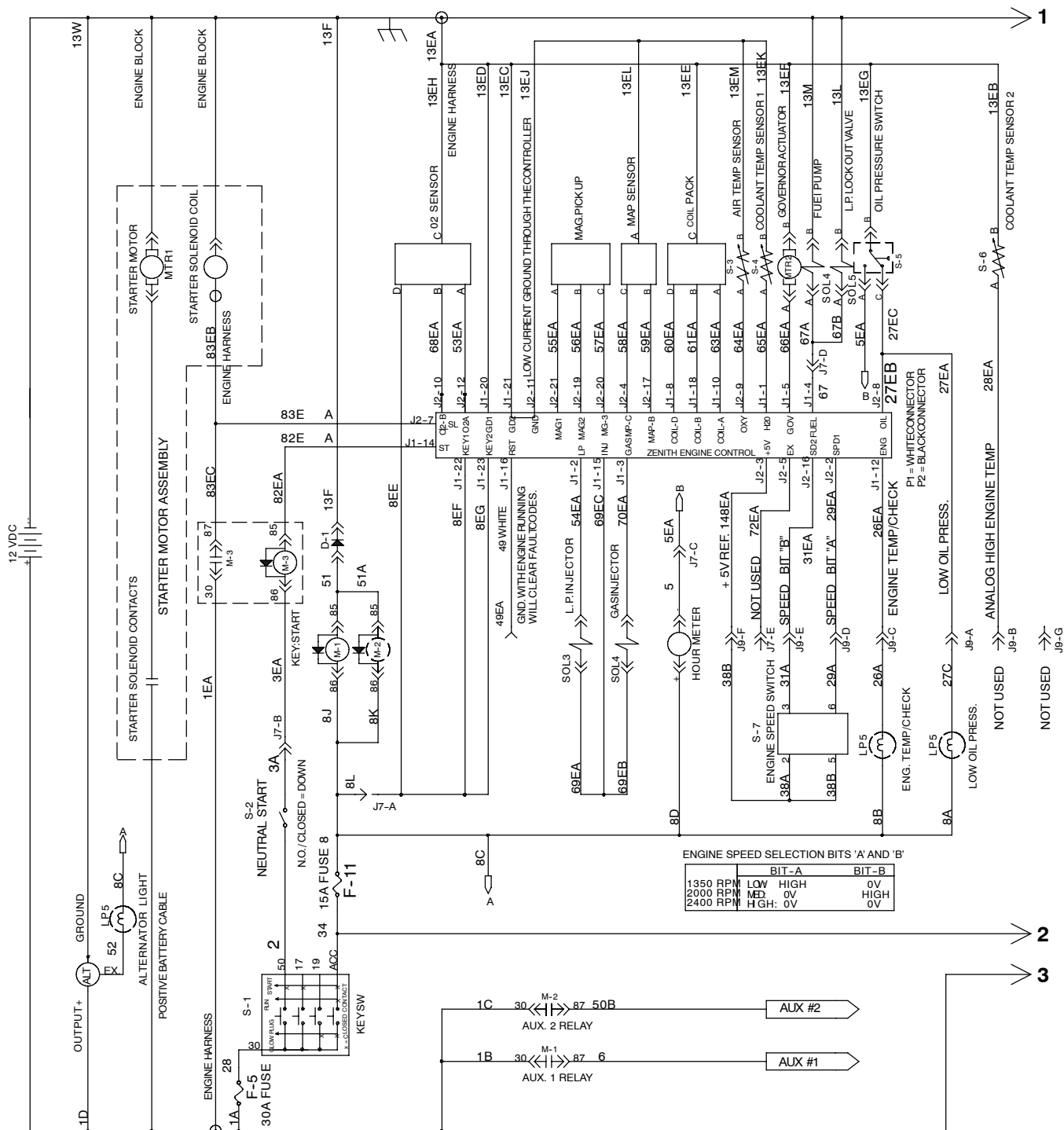
Fig. 69 - Electrical Schematic (000000-024999)
