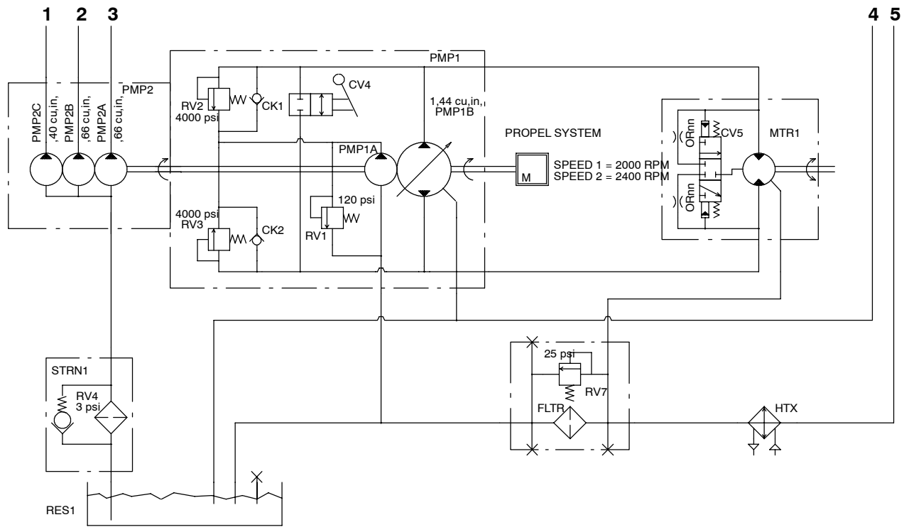
Fig. 62 - Hydraulic Schematic
