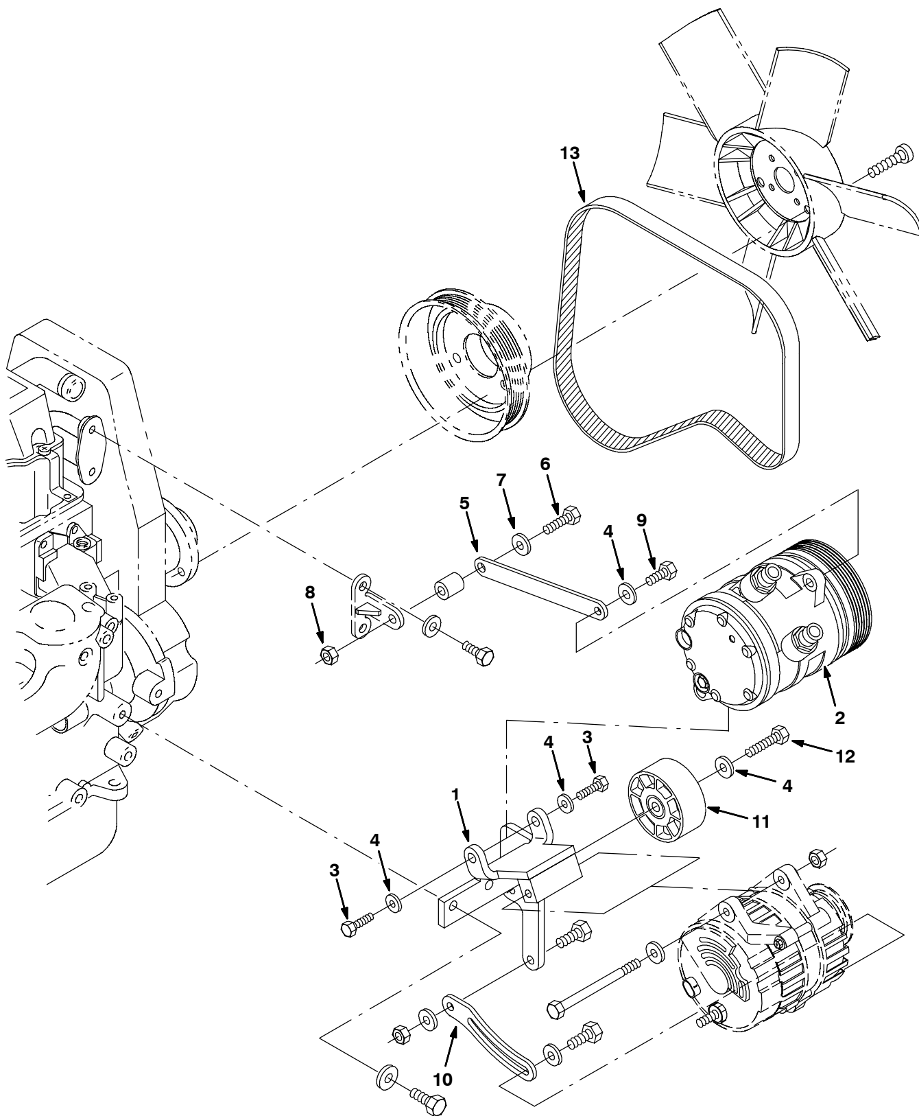
Fig. 25 - Air Conditioning Compressor Group (000000-024999)
