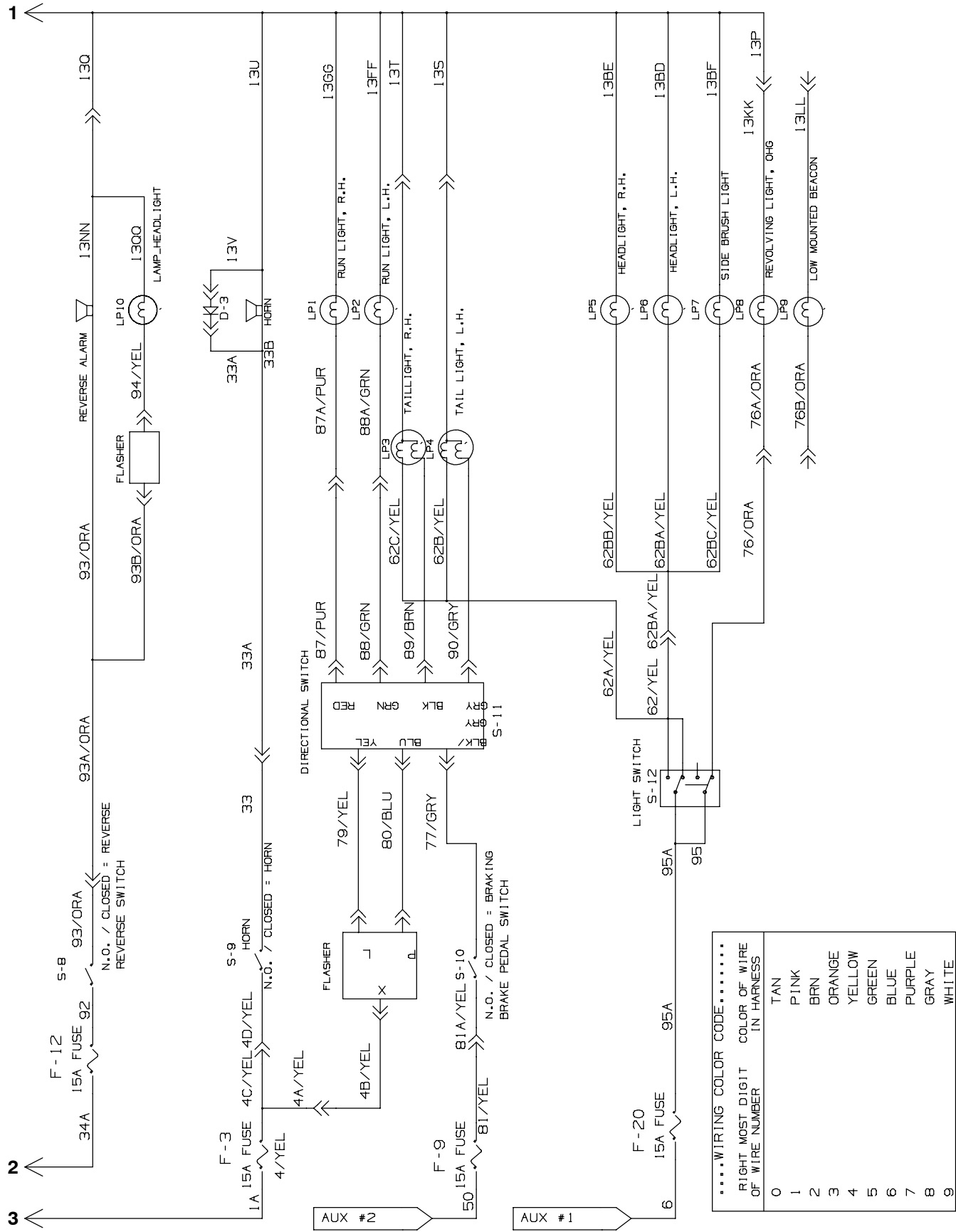
Fig. 71 - Electrical Schematic (030000- )
