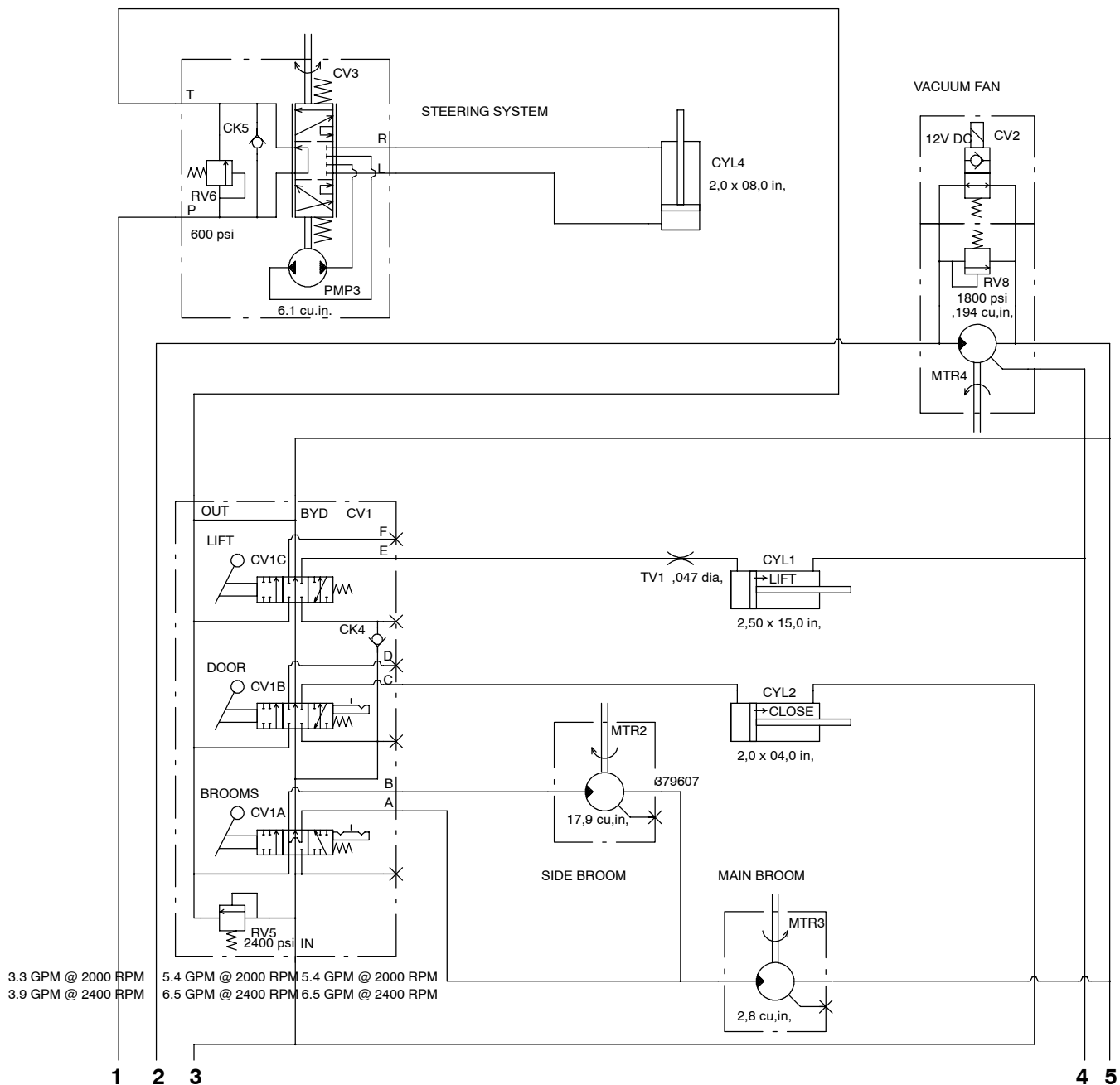
Fig. 62 - Hydraulic Schematic
