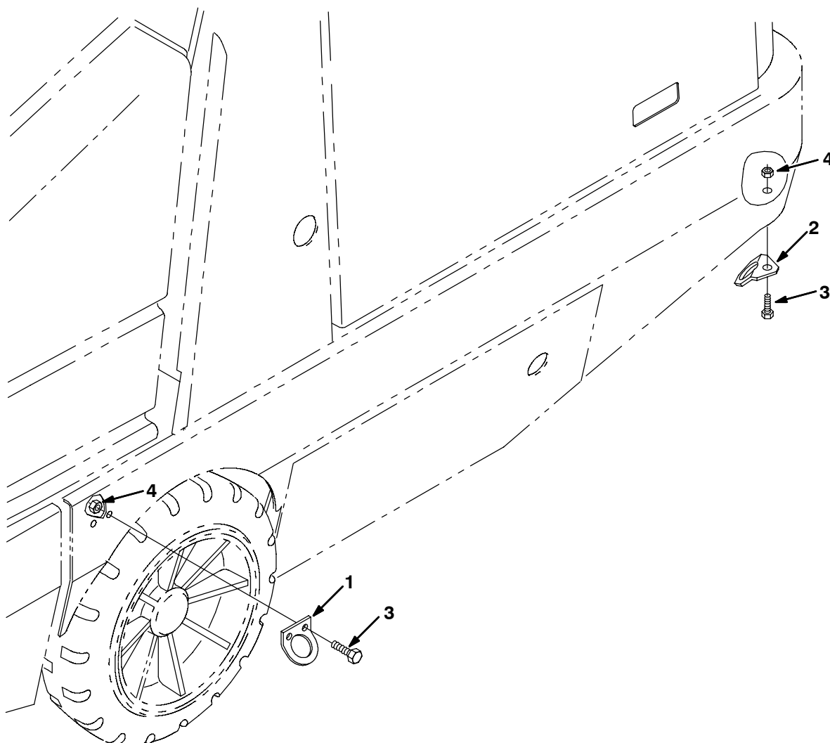
Fig. 45 - Transport Kit
