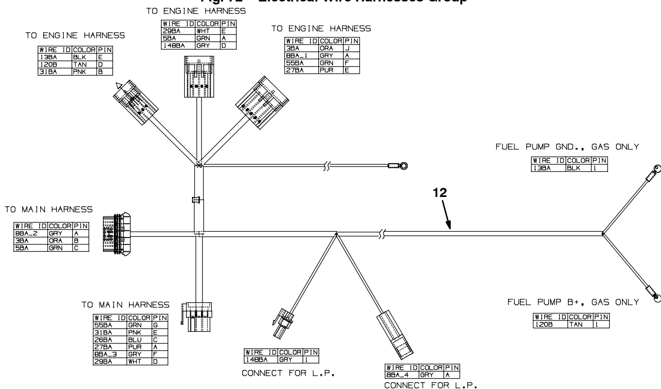
Fig. 72 - Electrical Wire Harnesses Group
