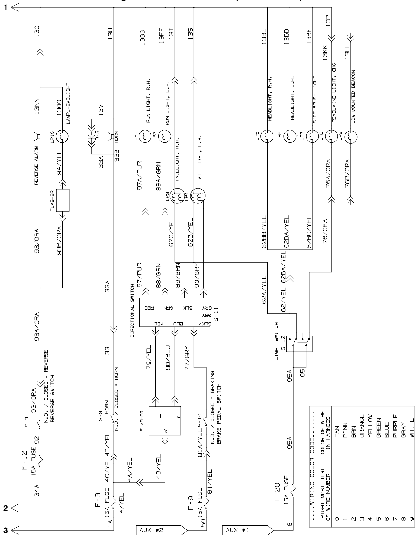
Fig. 70 - Electrical Schematic (025000-029999)
