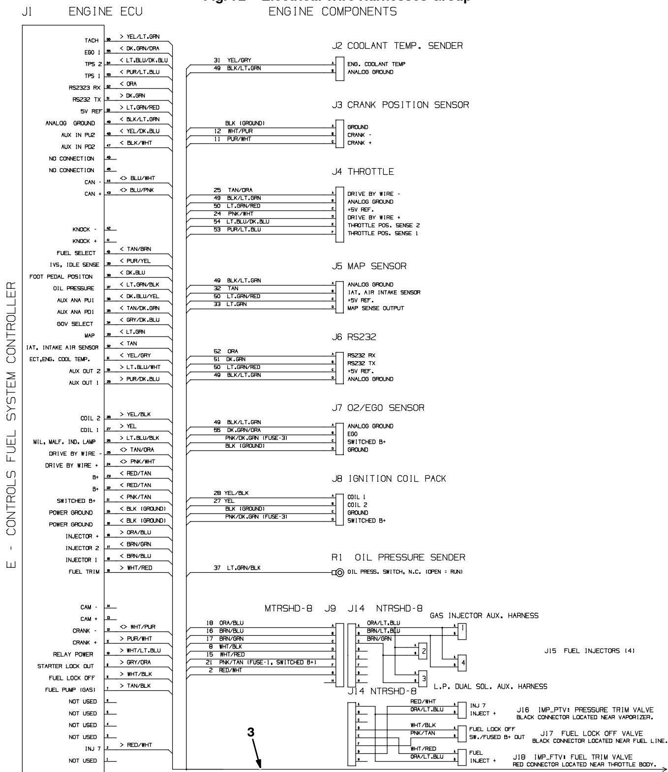
Fig. 72 - Electrical Wire Harnesses Group ENGINE COMPONENTS
