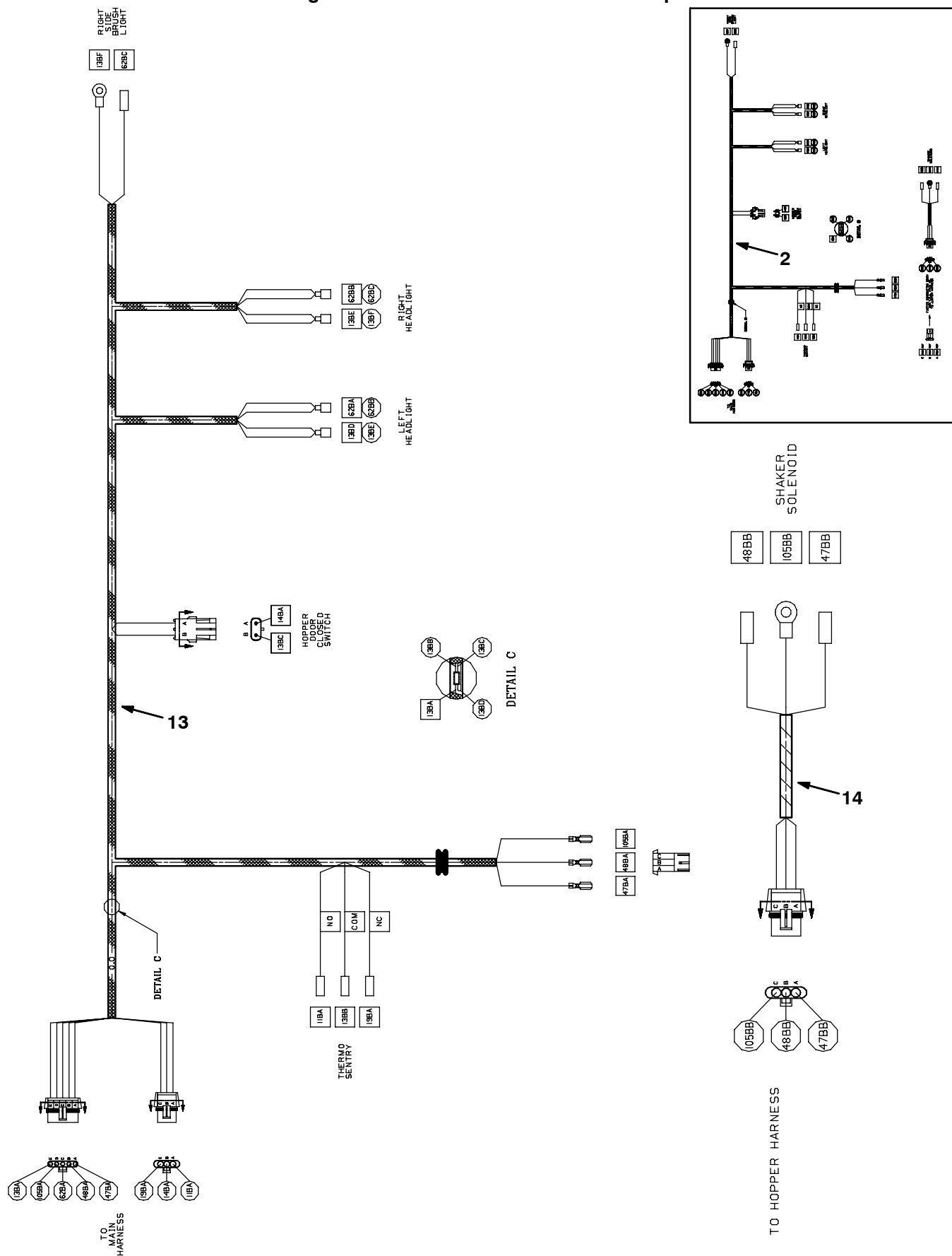
Fig. 72 - Electrical Wire Harnesses Group
