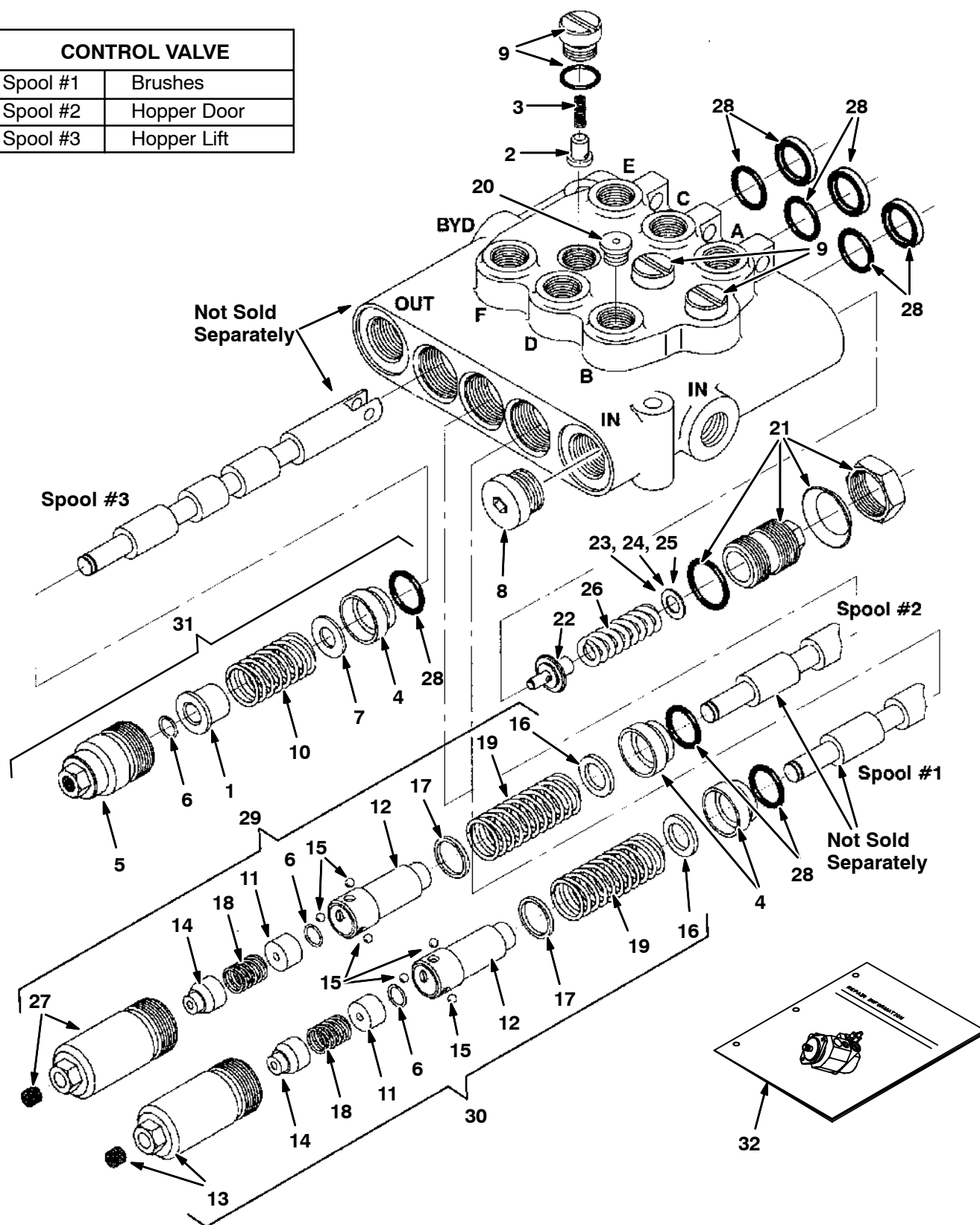
Fig. 7 - Hydraulic Valve Breakdown, 374547
