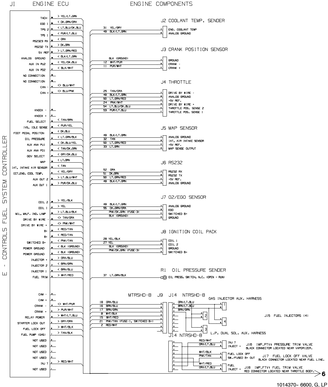
Fig. 70 - Electrical Schematic (025000-029999)
