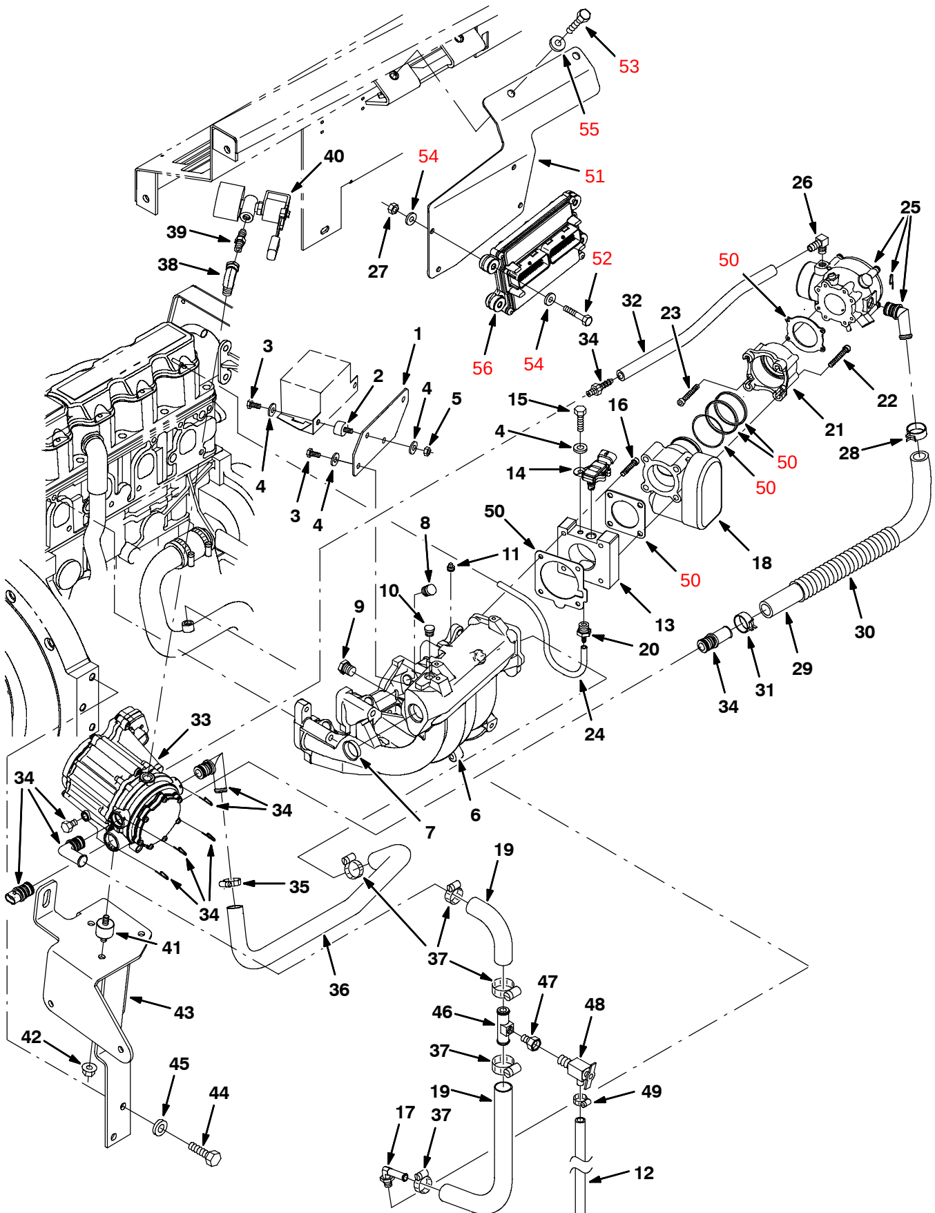
Fig. 25 - Engine EFI and Vaporizer Group, LPG (030000- )
