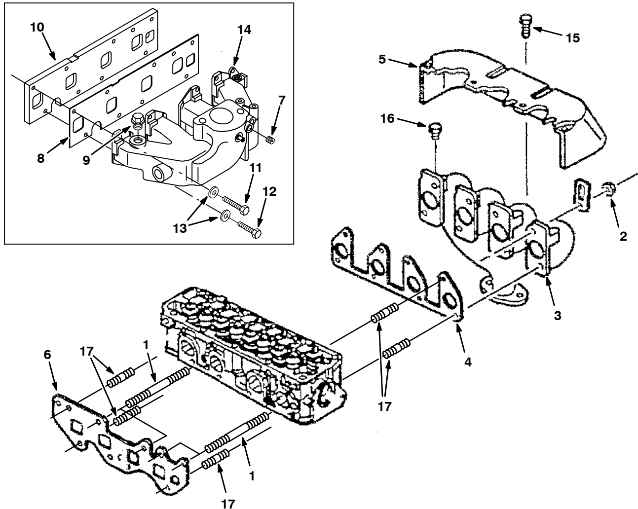
Fig. 5 - Manifold Group
