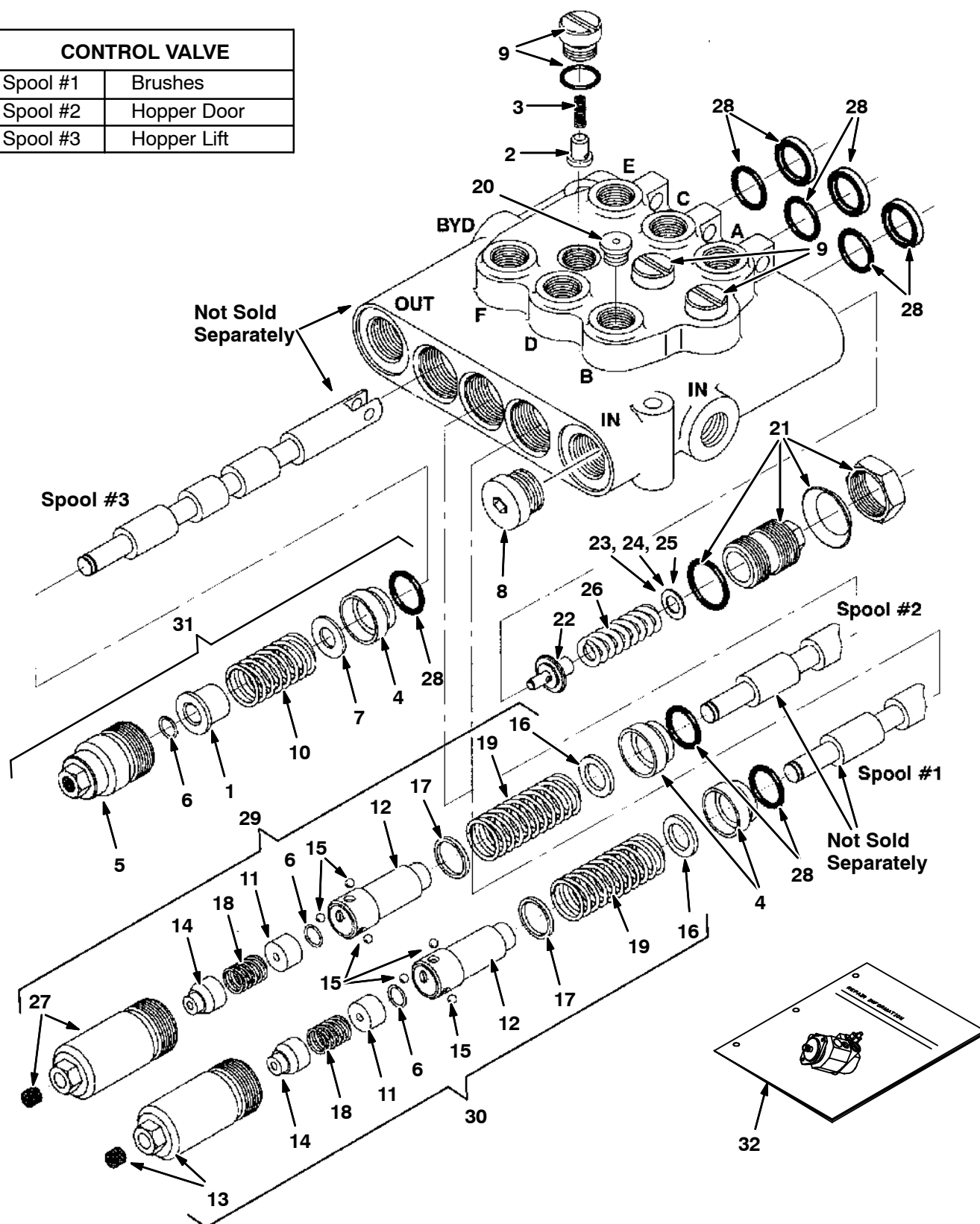
Fig. 8 - Hydraulic Valve Breakdown, 1019961
