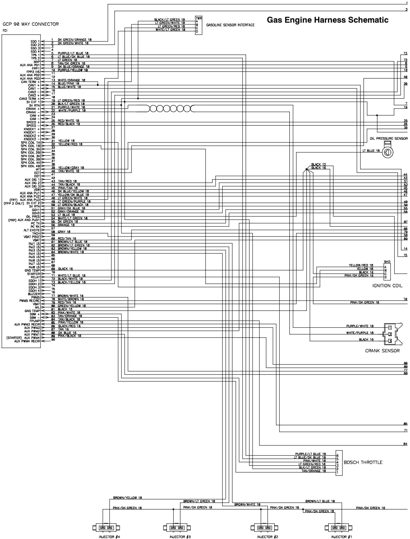
Fig. 71 - Electrical Schematic (030000- )
