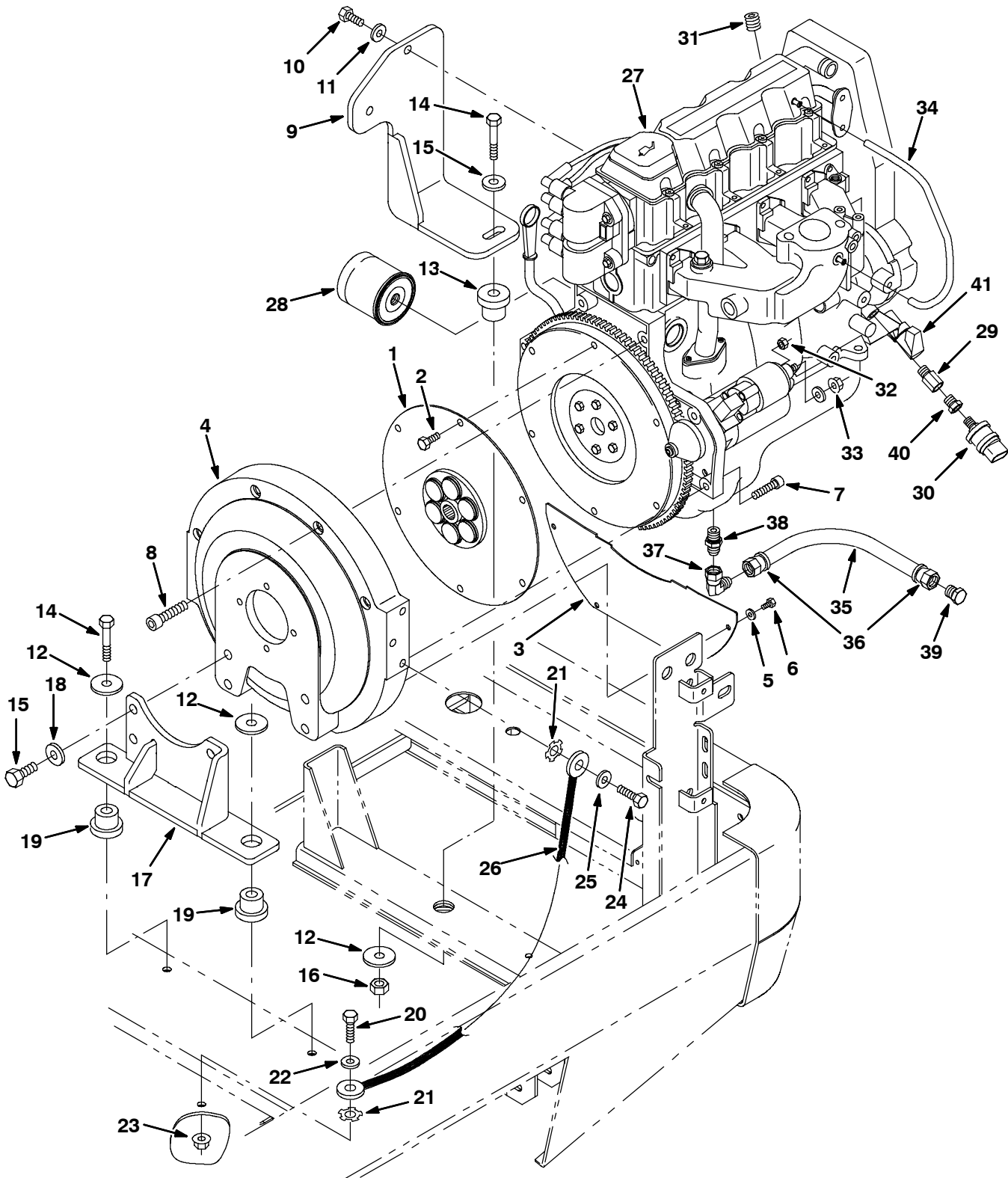
Fig. 17 - Engine Group, LPG (000000-024999)
