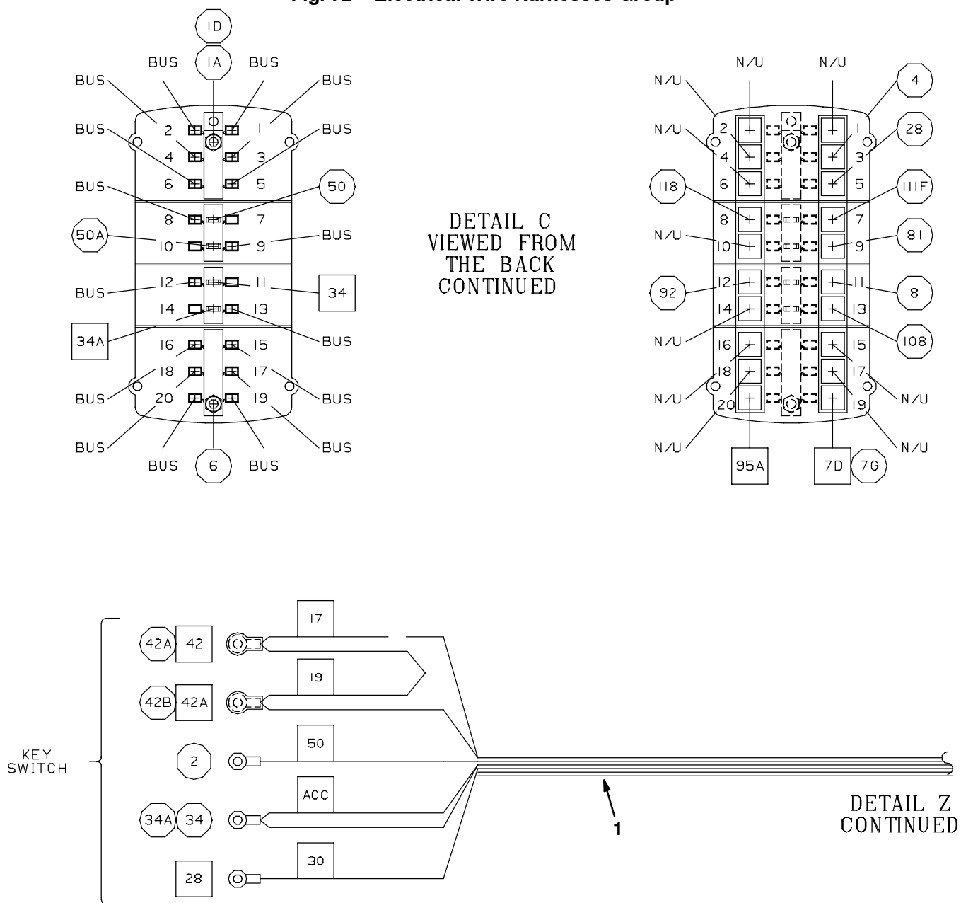
Fig. 72 - Electrical Wire Harnesses Group
