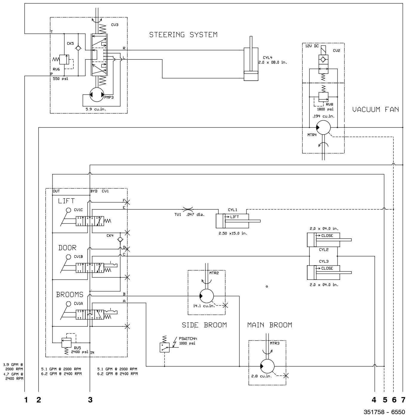
Fig. 48 - Hydraulic Schematic
