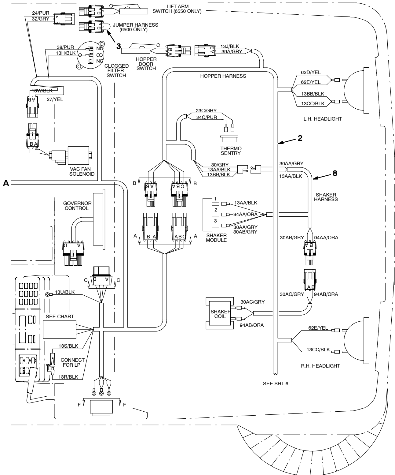
Fig. 56 - Wire Harness Group
