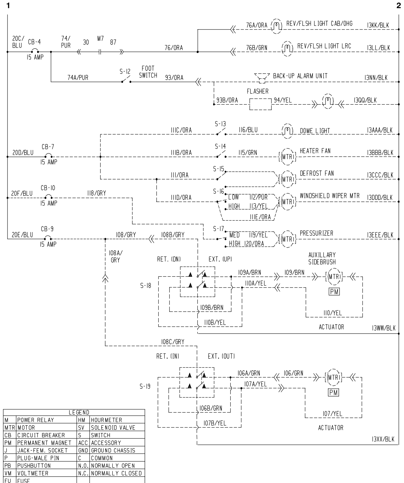
Fig. 55 - Electrical Schematic
