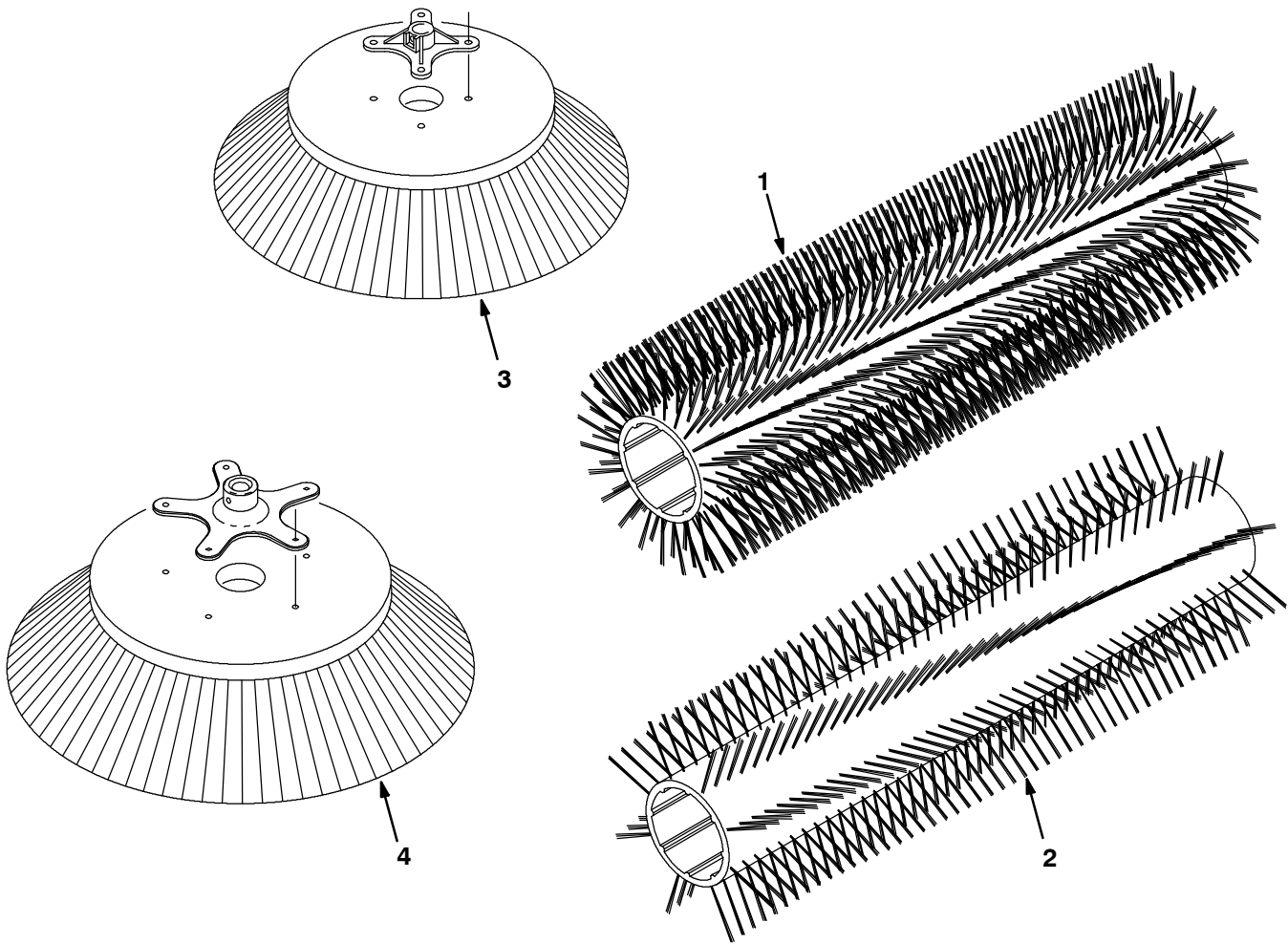
Fig. 2 - Replacement Brushes
