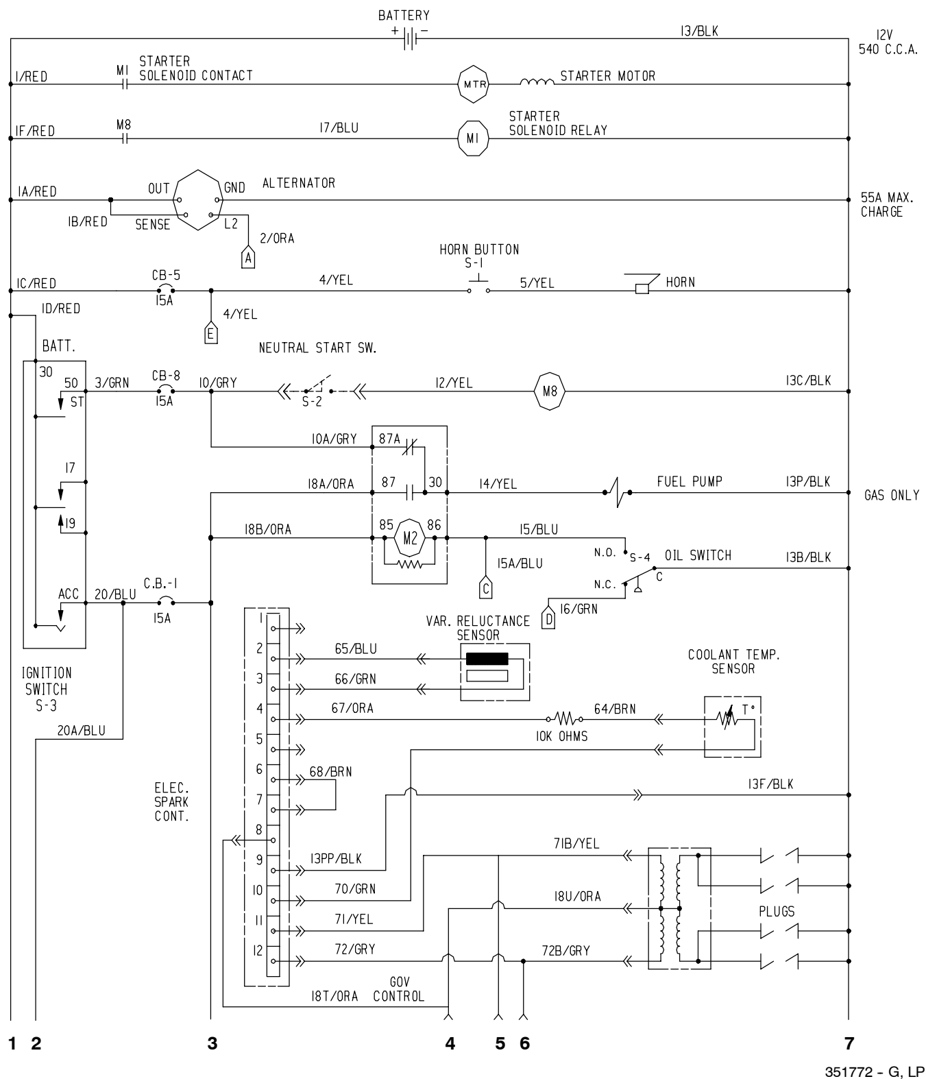
Fig. 55 - Electrical Schematic
