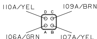
VIEW J-J
