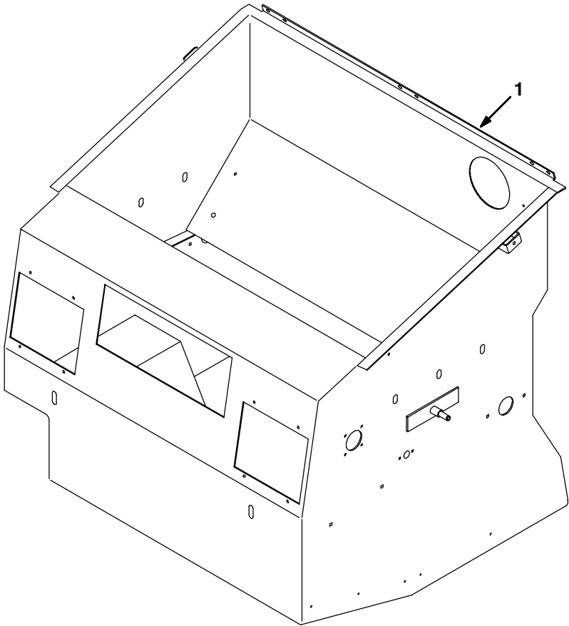
Fig. 44 - Stainless Steel Hopper Group
