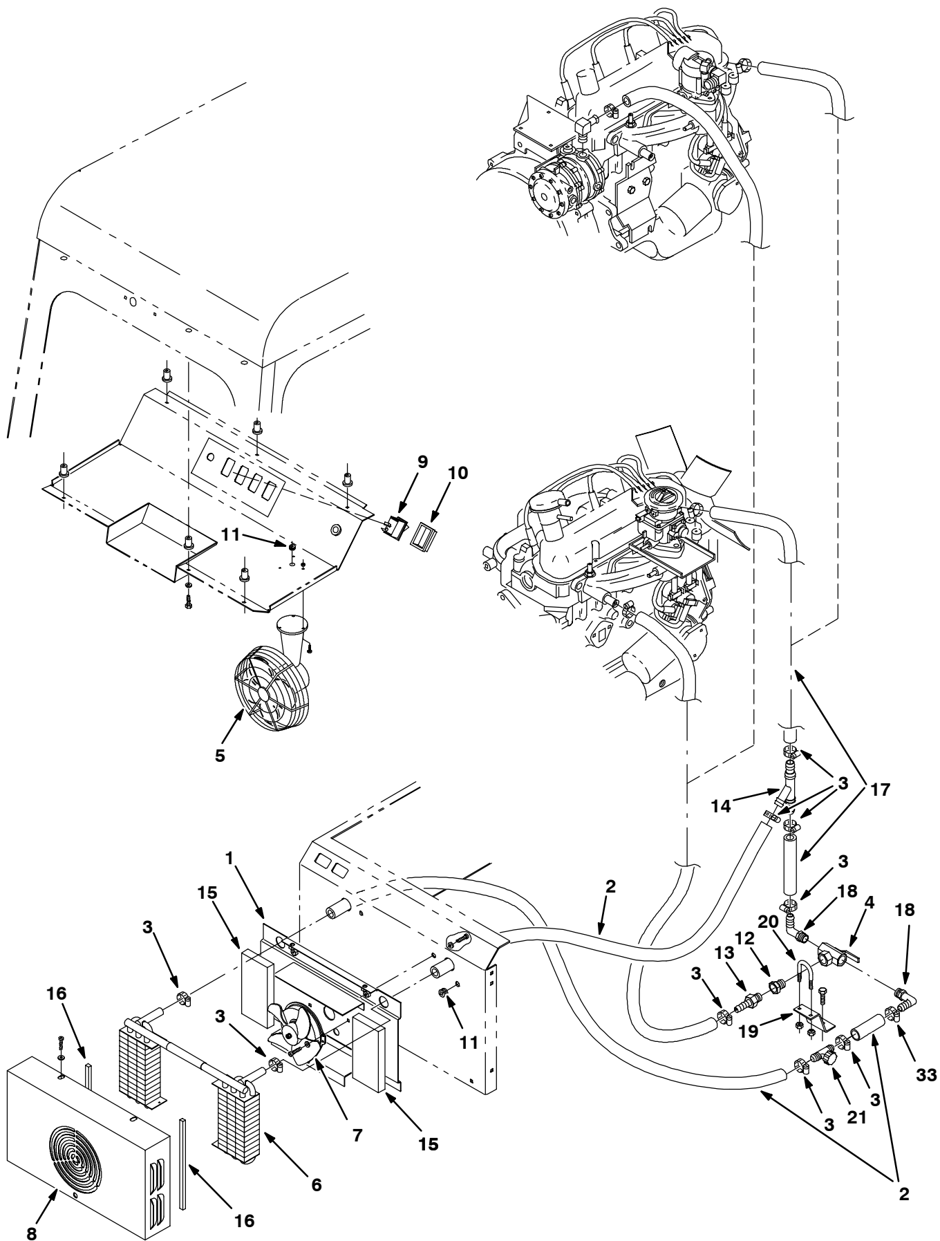
Fig. 21 - Cab Heater Kit (000000-006517)
