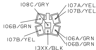
VIEW I-I
