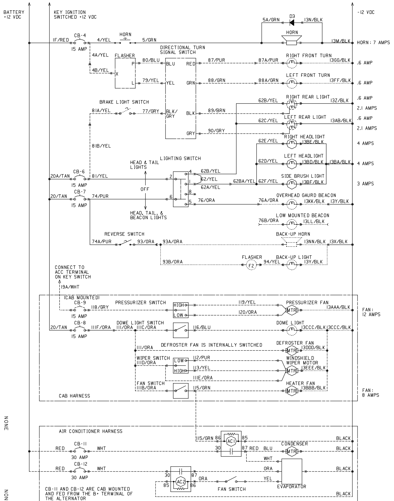
Fig. 62- Electrical Schematic (020000- )
