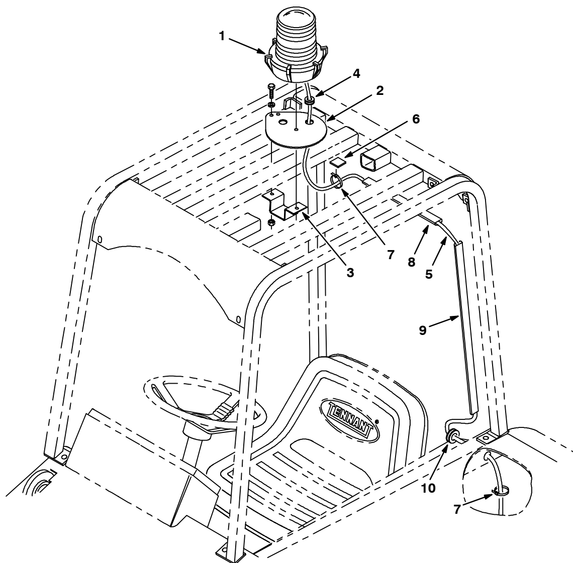
Fig. 4 - Flashing Light Kit, Overhead Guard
