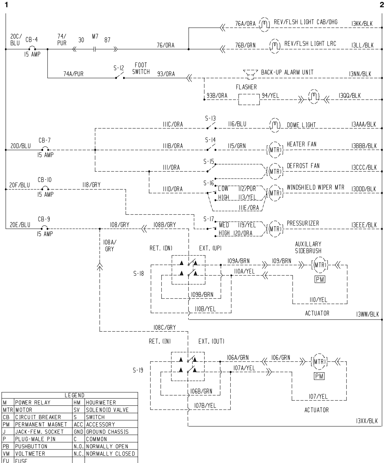
Fig. 61 - Electrical Schematic (000000-019999)
