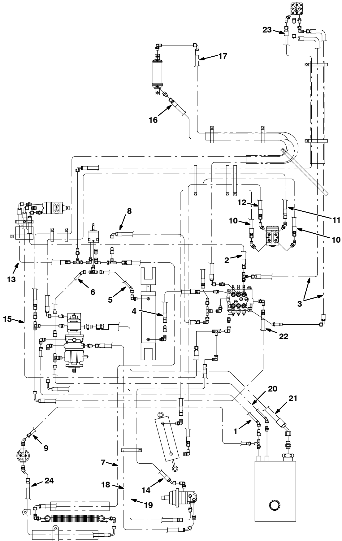
Fig. 57 - Hydraulic Hose Group (Plastic Hopper)
