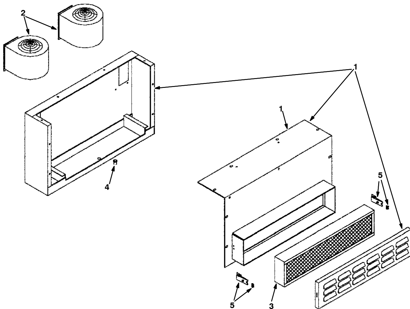
Fig. 17 - Pressurizer Breakdown, 393384
