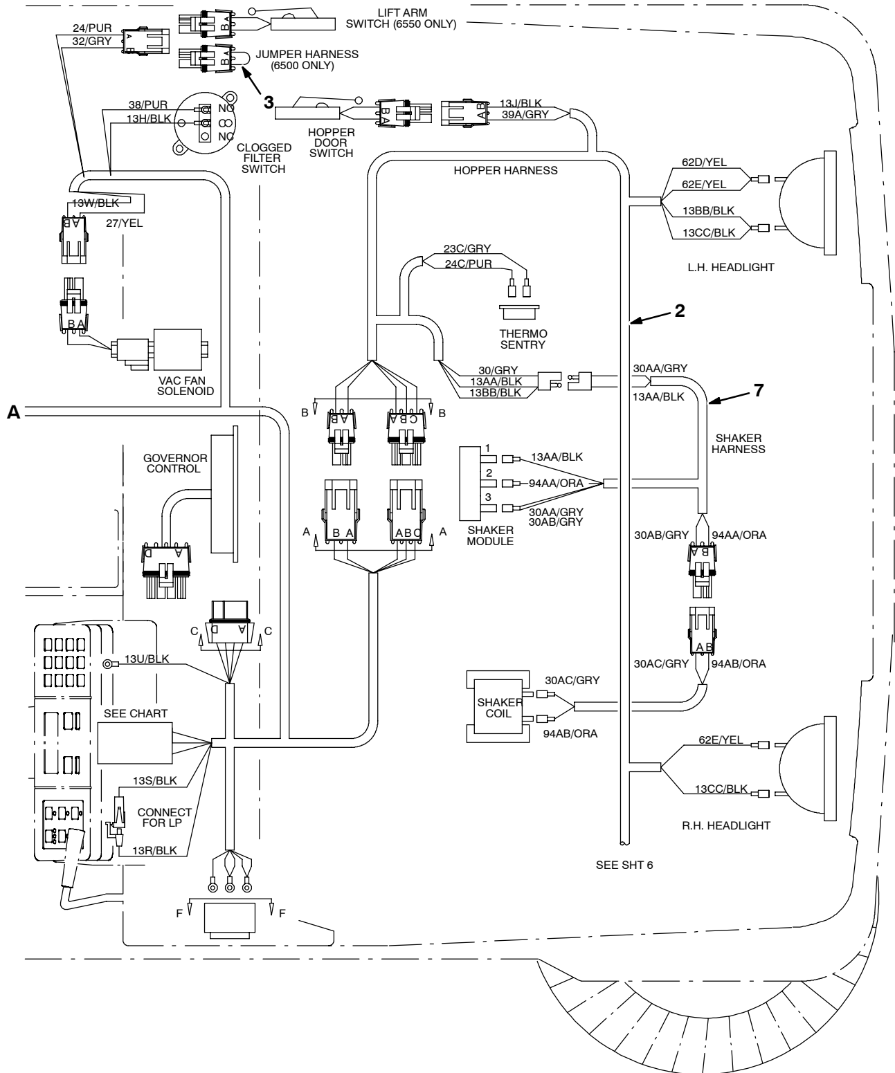
Fig. 63 - Wire Harnesses Group (000000-019999)
