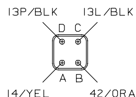
VIEW E-E
