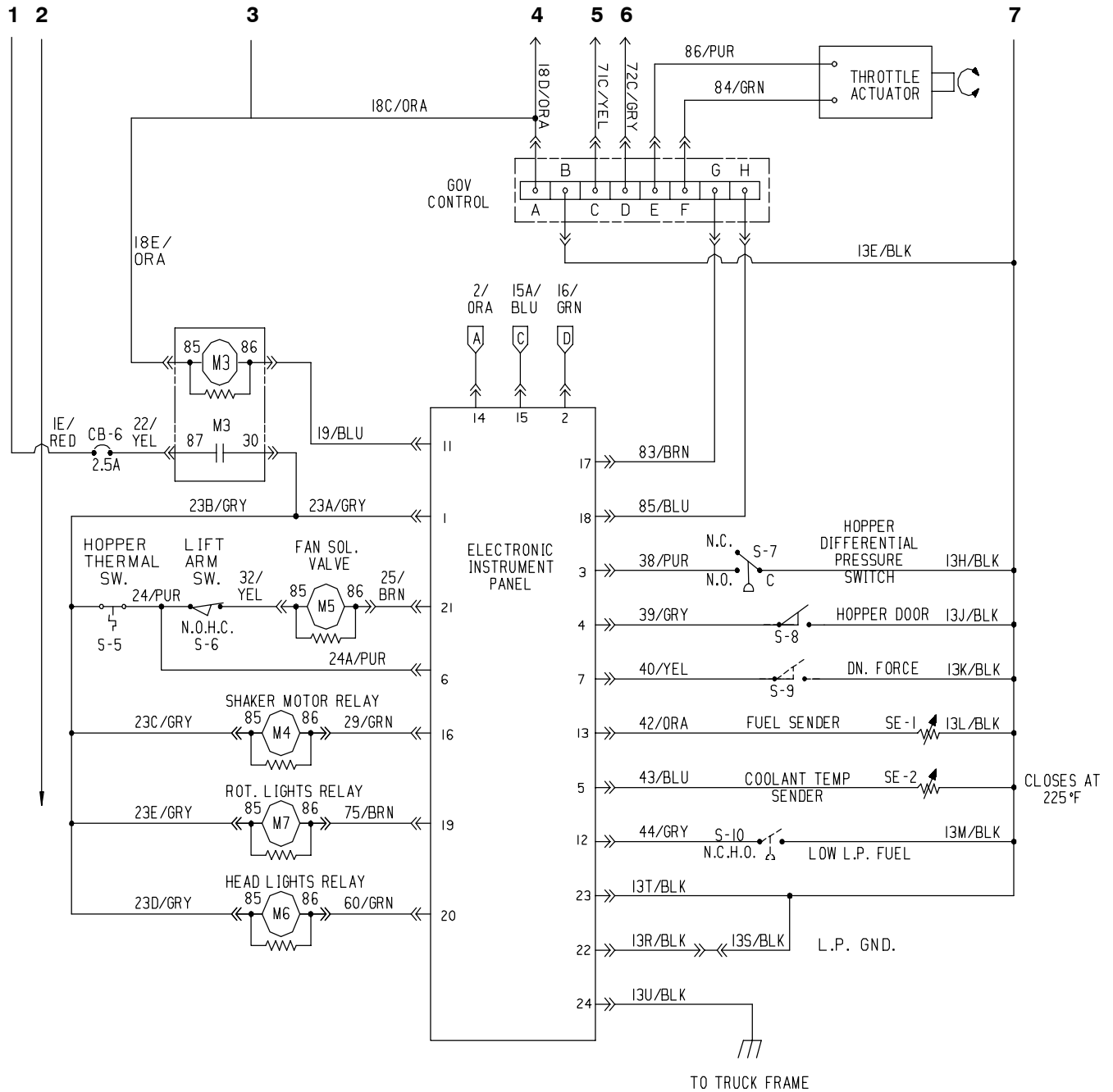
Fig. 61 - Electrical Schematic (000000-019999)
