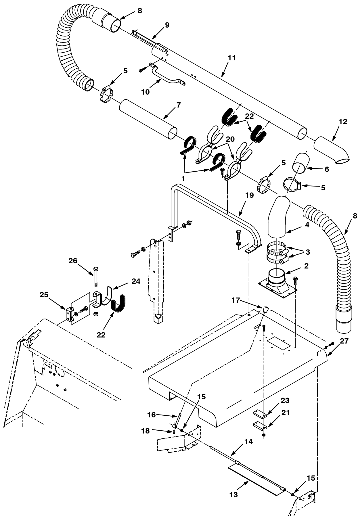
Fig. 30 - Blower Kit
