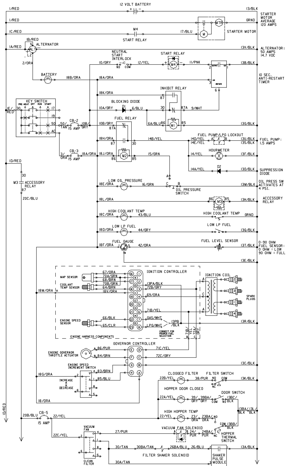
Fig. 62- Electrical Schematic (020000- )
