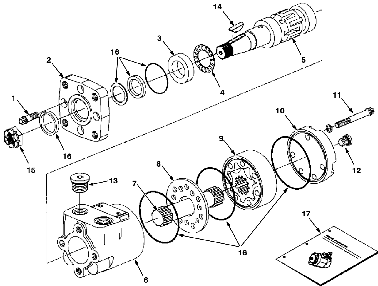
Fig. 7 - Hydraulic Motor Breakdown, 379608
