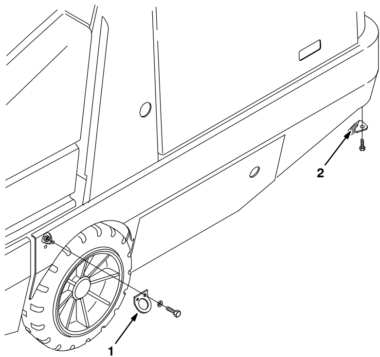
Fig. 46 - Transport Kit (Plastic Hopper)
