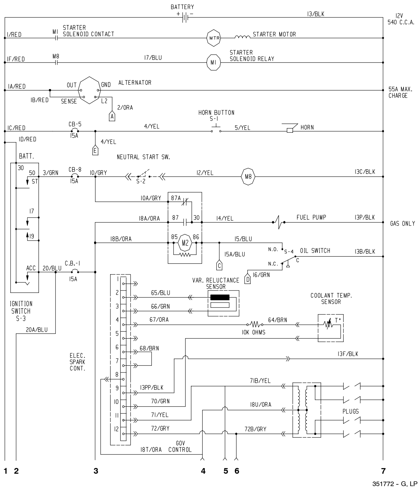
Fig. 61 - Electrical Schematic (000000-019999)
