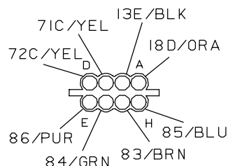
VIEW C-C
