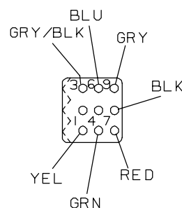
VIEW O-O
