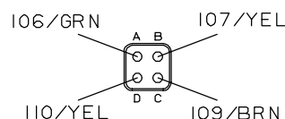
VIEW K-K
