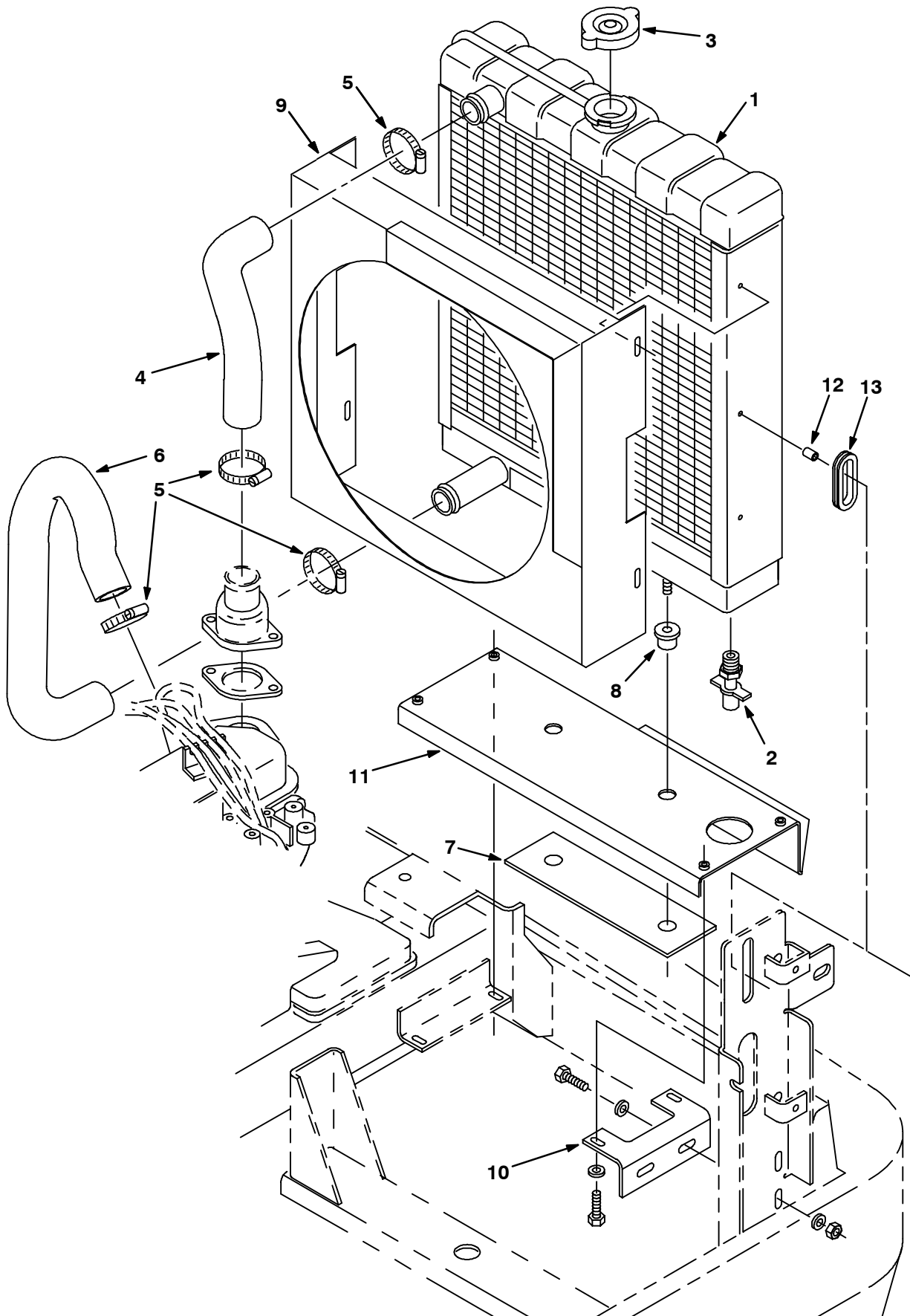
Fig. 26 - Radiator Group
