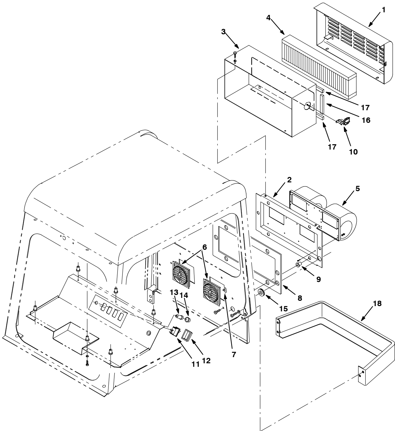
Fig. 20 - Cab Pressurizer Kit (000000-006517)
