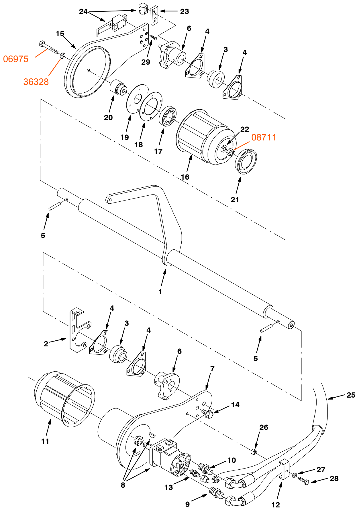
Fig. 50 - Main Brush Drive Group (000000-019999)
