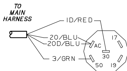
VIEW F-F
