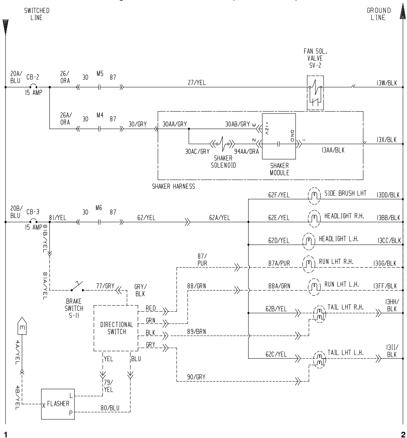
Fig. 61 - Electrical Schematic (000000-019999)
