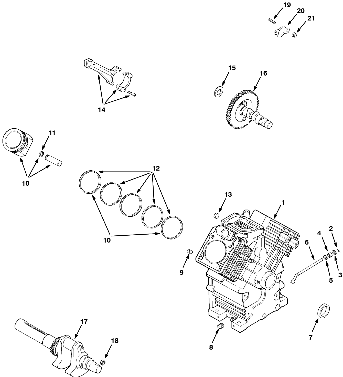
Fig. 1 - Crankcase Group
