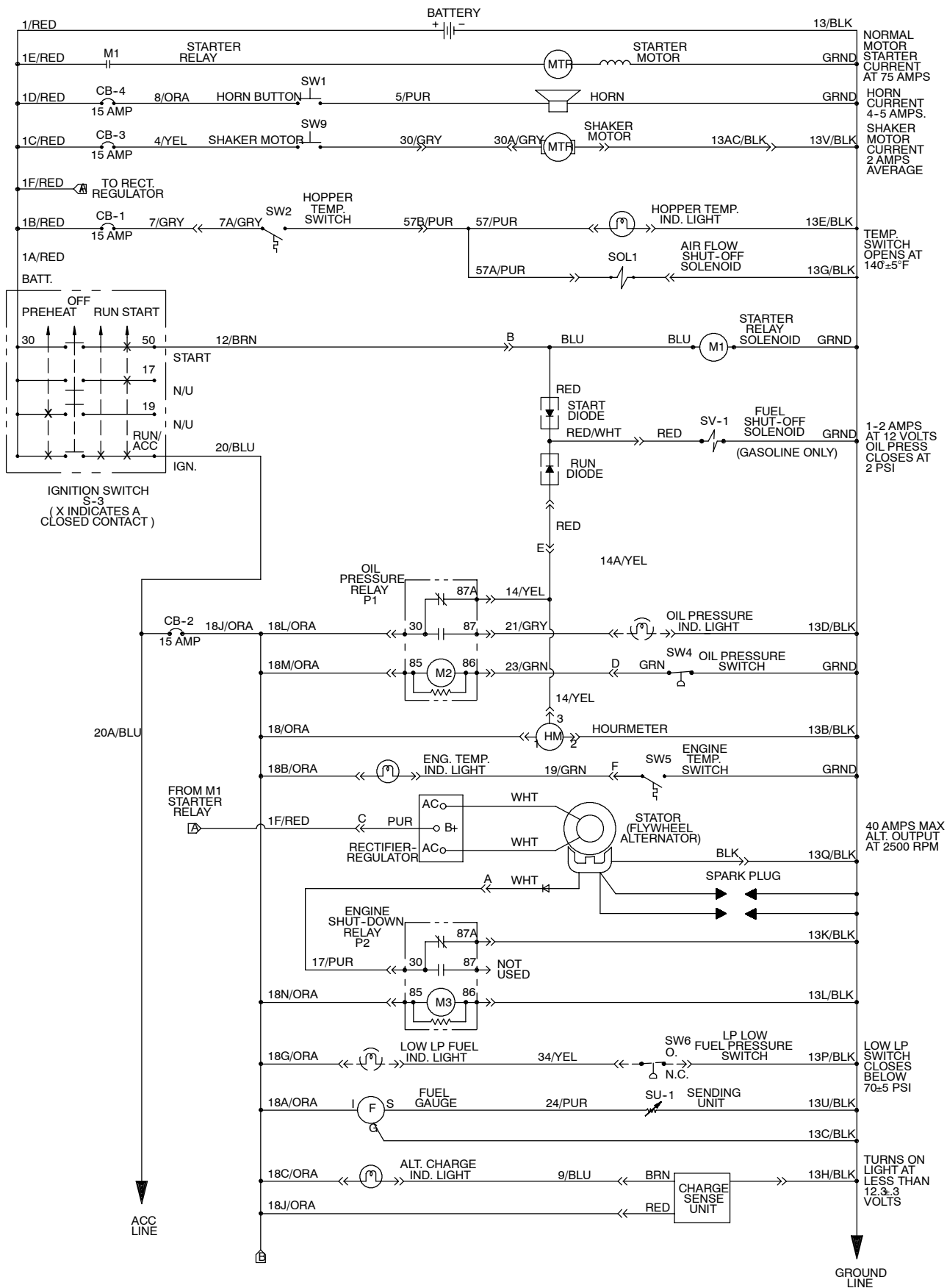
Fig. 39 - Electrical Schematic, G/LP (Air Cooled)
