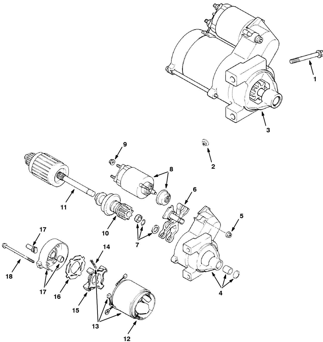
Fig. 6 - Starter Group
