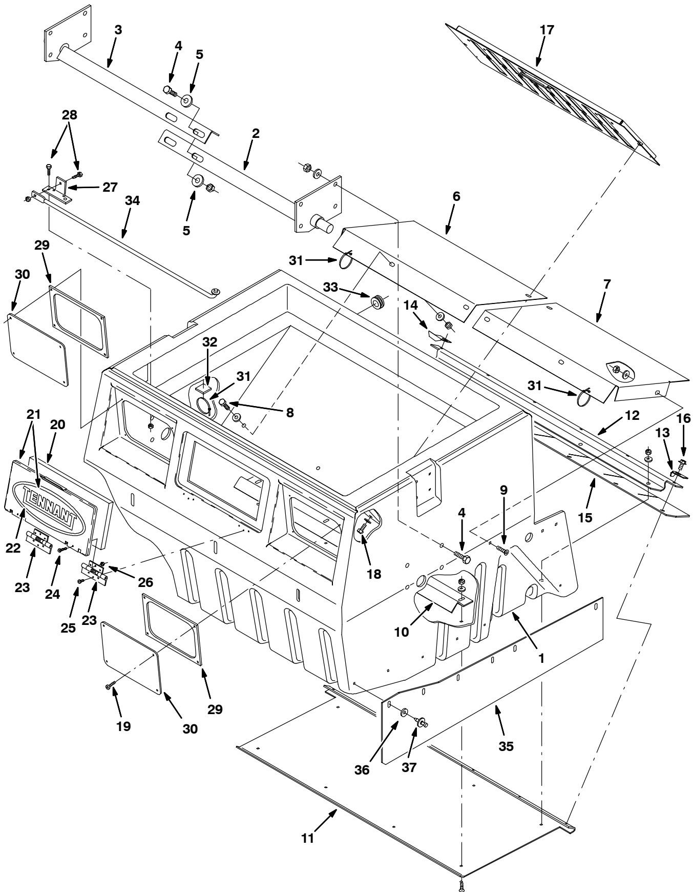
Fig. 28 - Hopper Group
