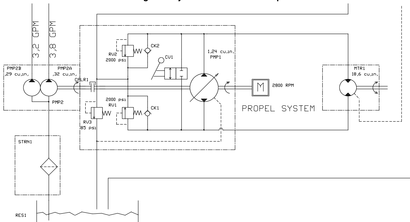
Fig. 37 - Hydraulic Schematic Group
