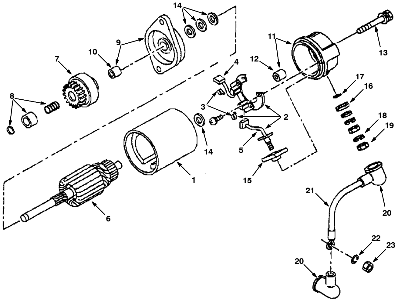
Fig. 12 - Starter Breakdown, 385966
