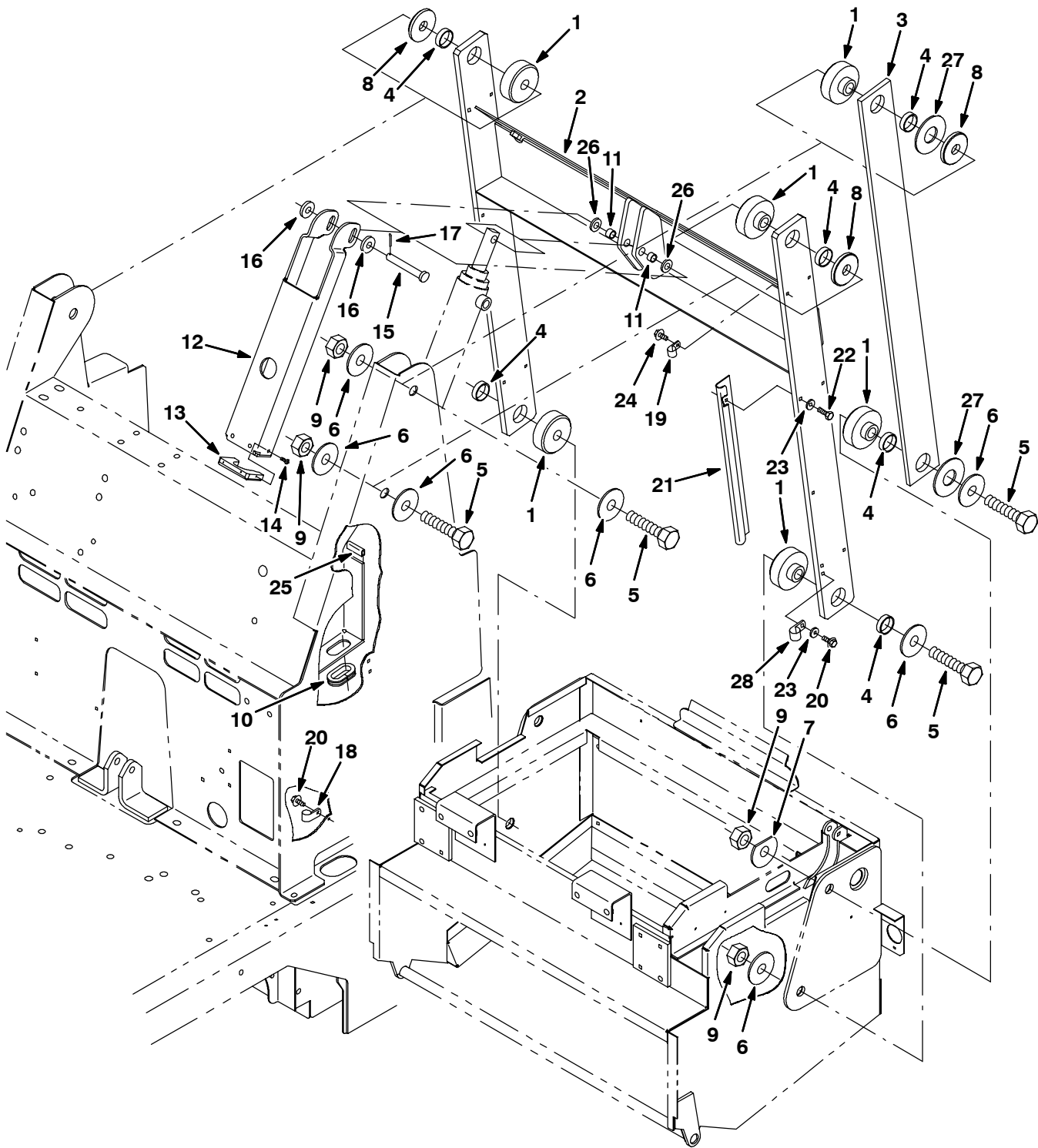
Fig. 39 - Hopper Lift Arms Group
