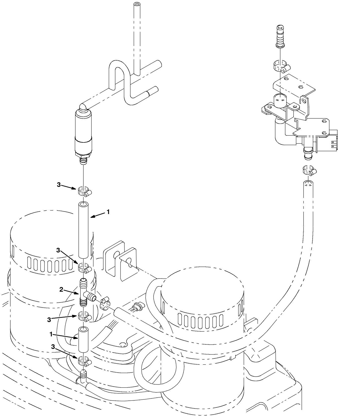
Fig. 5 - FaST Solution Supply Group, Disk Scrub Head (S/N 10000000 - 10361712)
