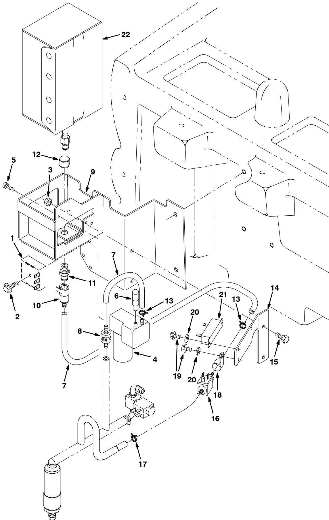
Fig. 3 - FaST Air Pump and Detergent Group (S/N 10000000 - 10361712)
