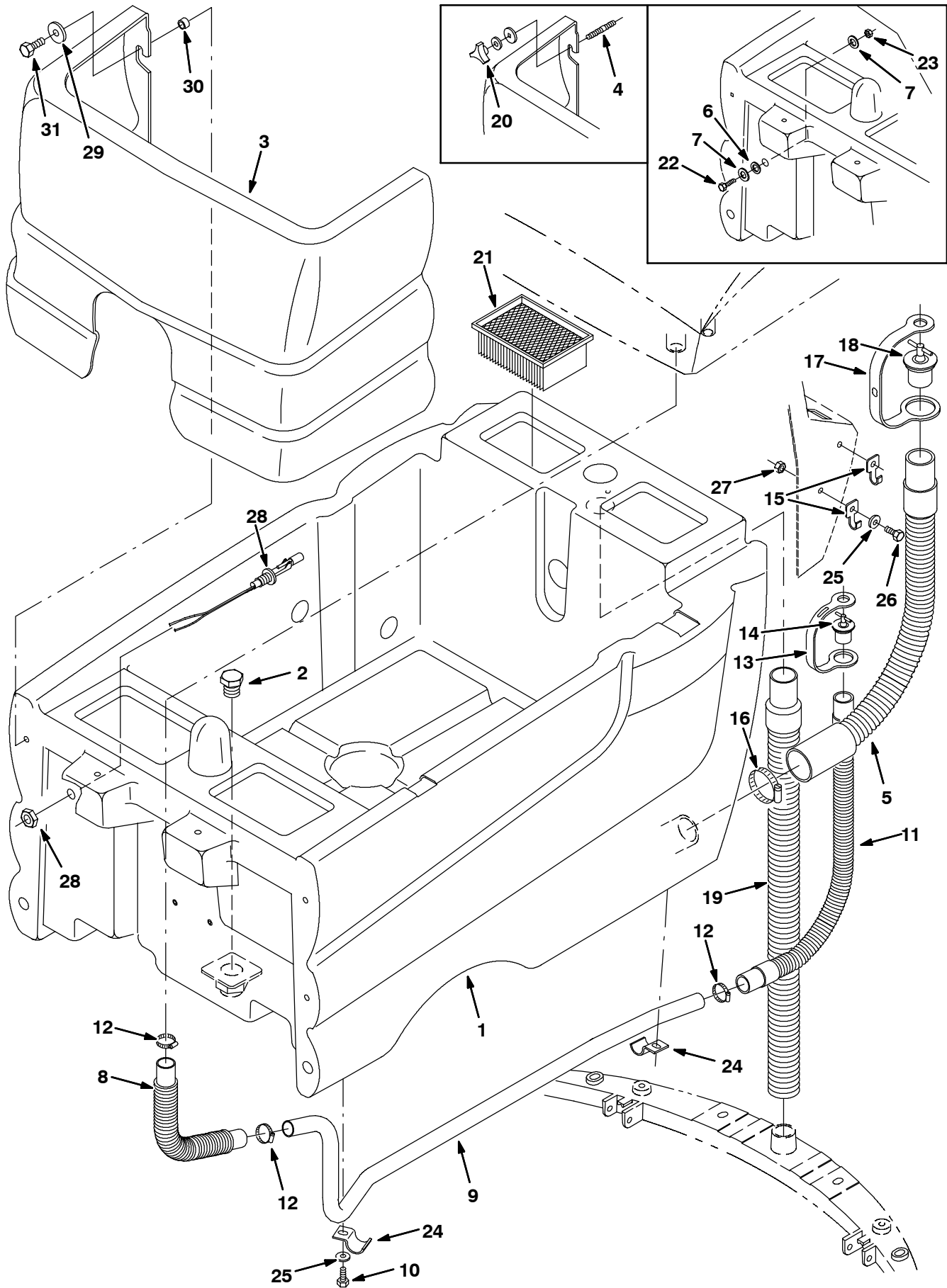
Fig. 10 - Recovery Tank Group (000000-014333)
