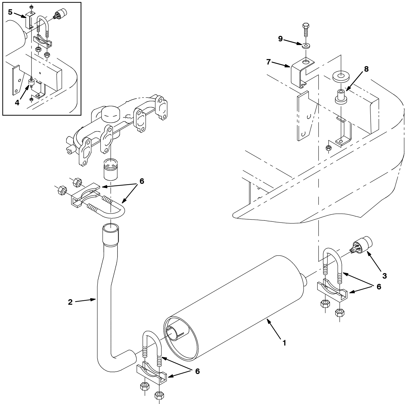
Fig. 22 - Muffler Group
