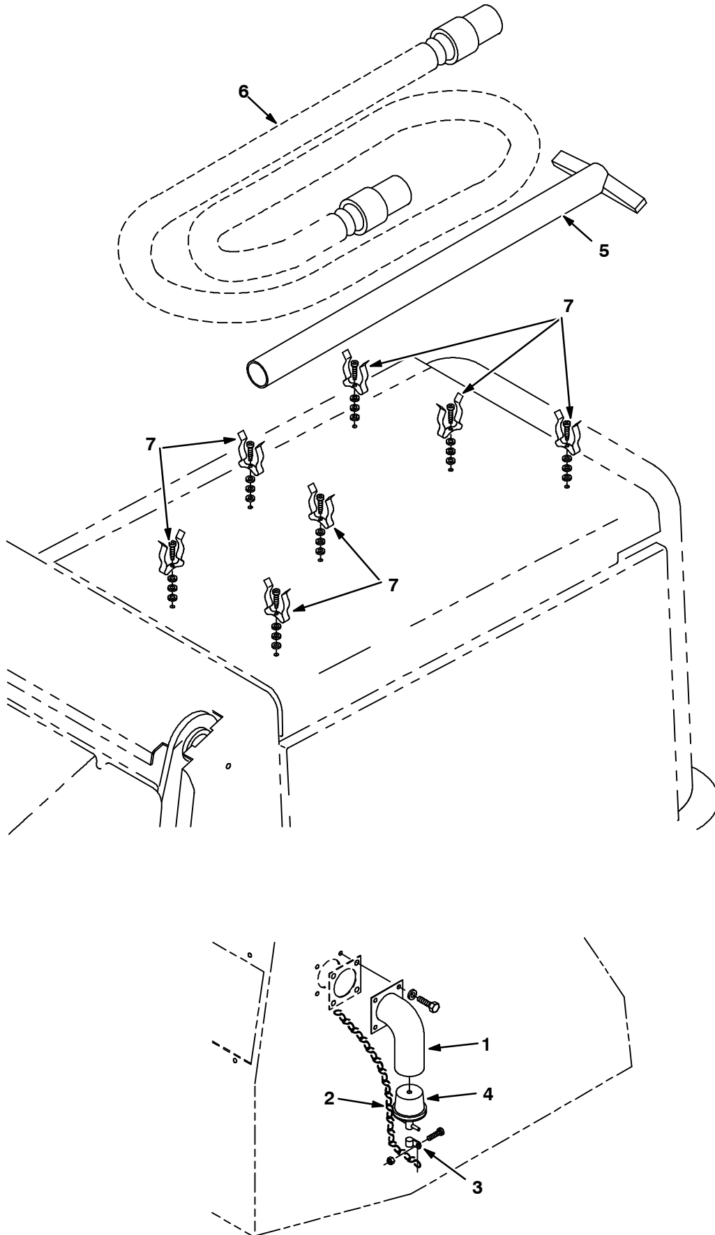
Fig. 21 - Vacuum Wand Kit
