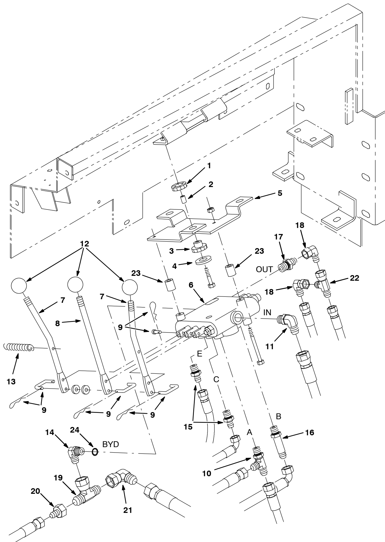
Fig. 55 - Hydraulic Valve Group
