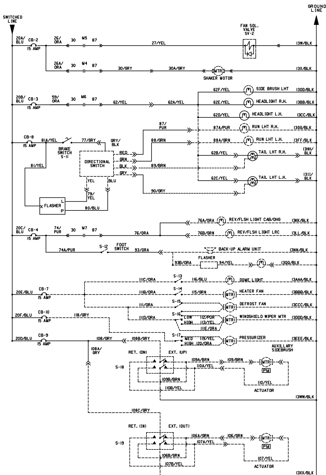
Fig. 58 - Electrical Schematic
