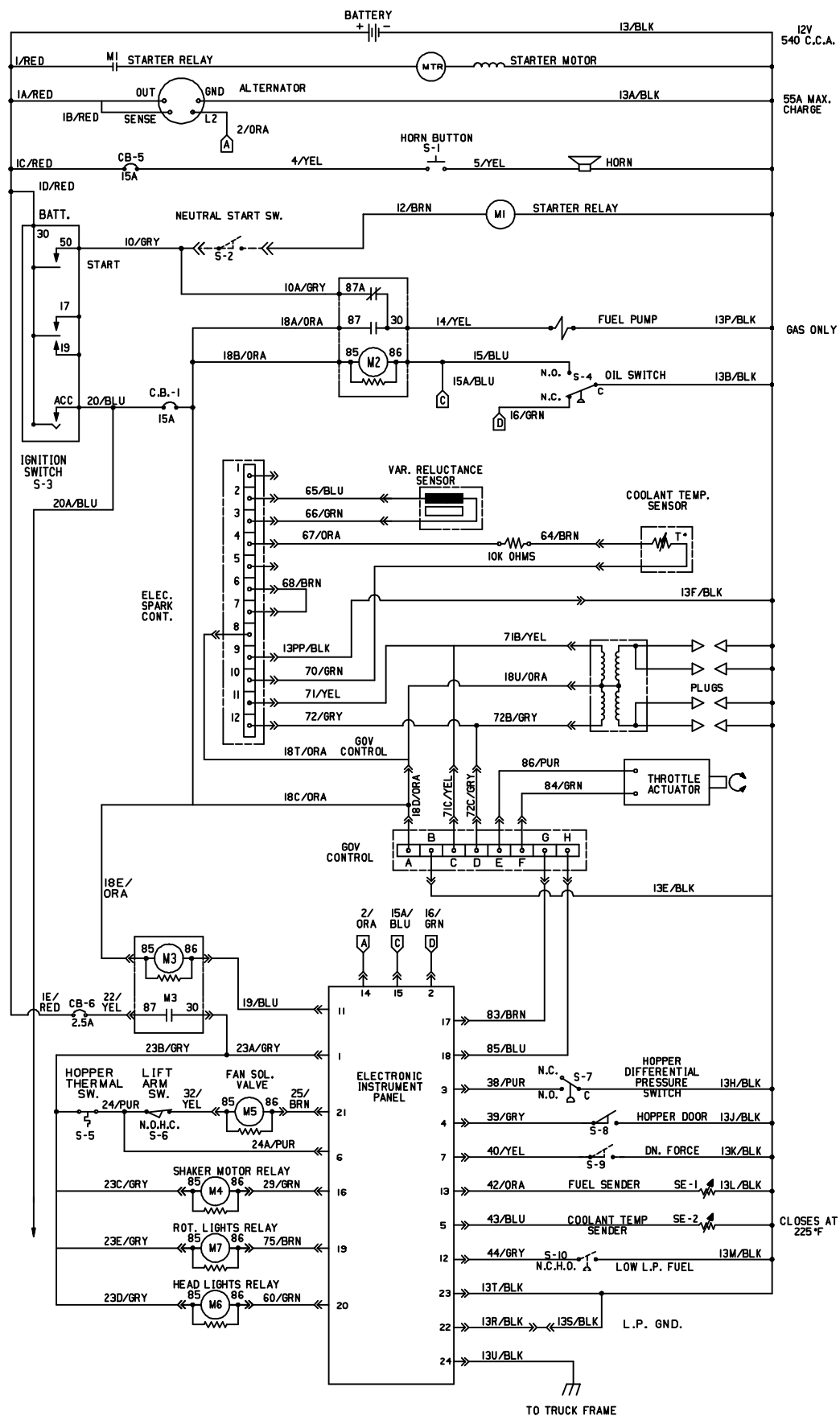
Fig. 58 - Electrical Schematic
