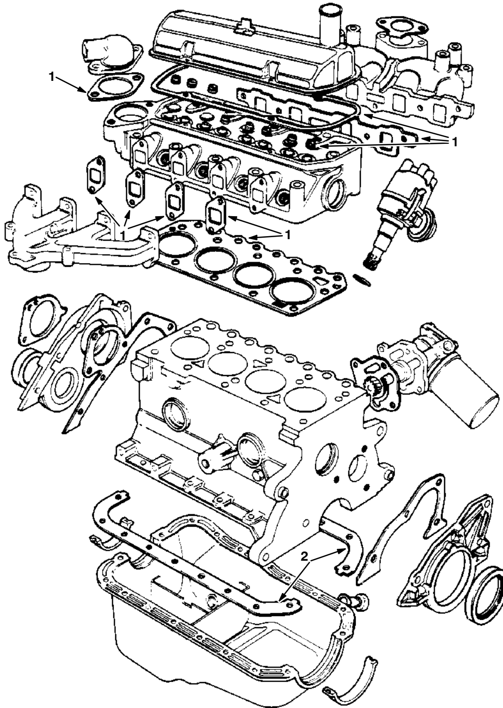
Fig. 10 - Gaskets Group
