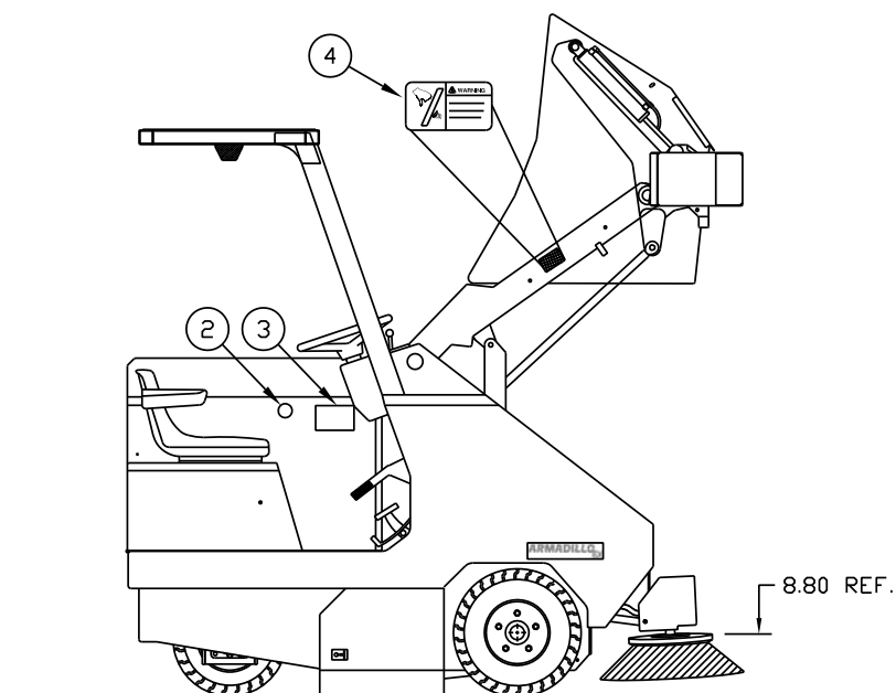
Lift View
