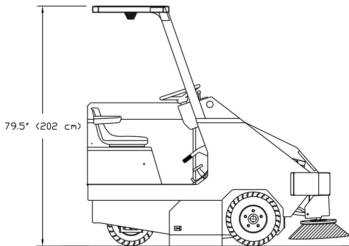
Lift View
