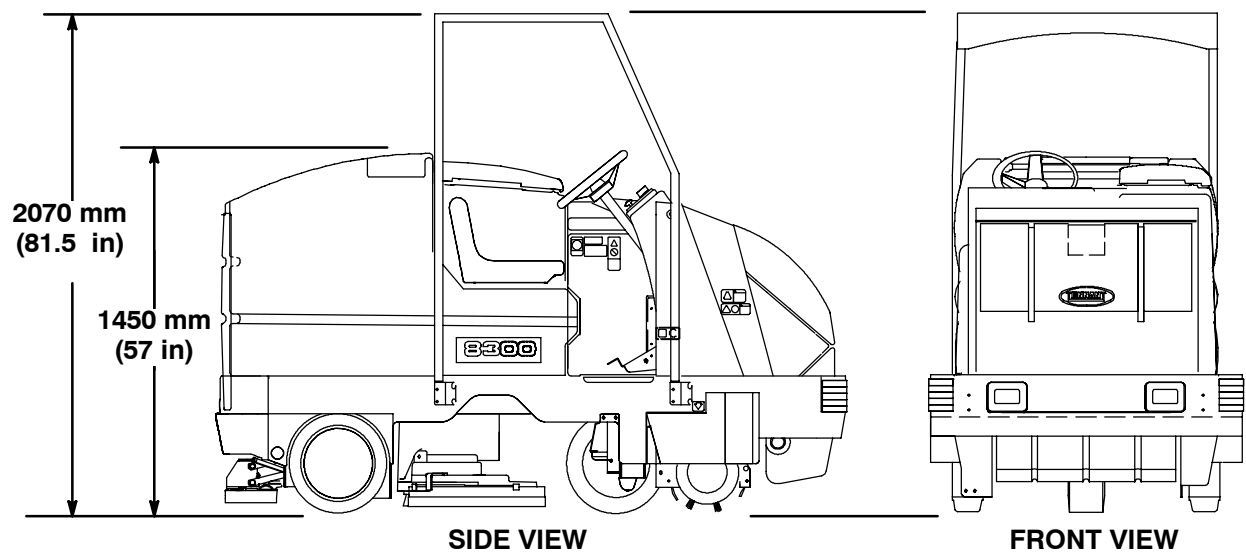
MACHINE DIMENSIONS
