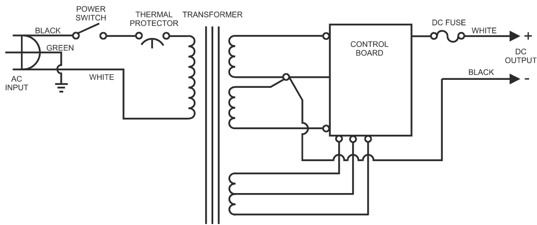
WIRING DIAGRAM
