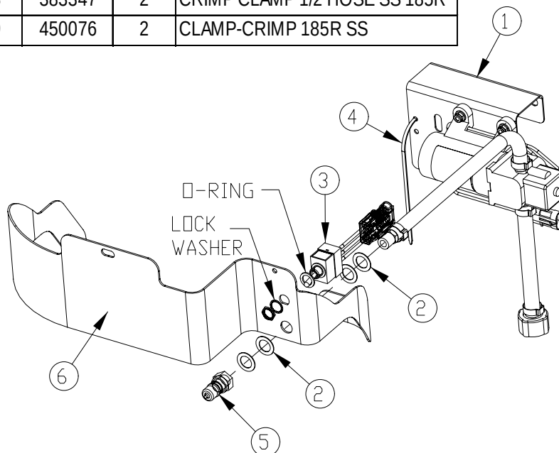
BILL OF MATERIAL - 172402
