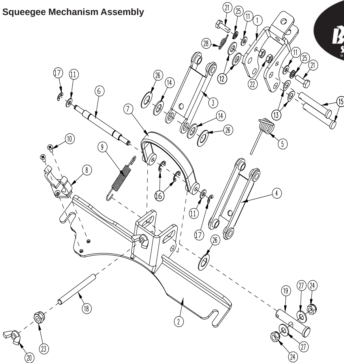
BILL OF MATERIAL - 172150
