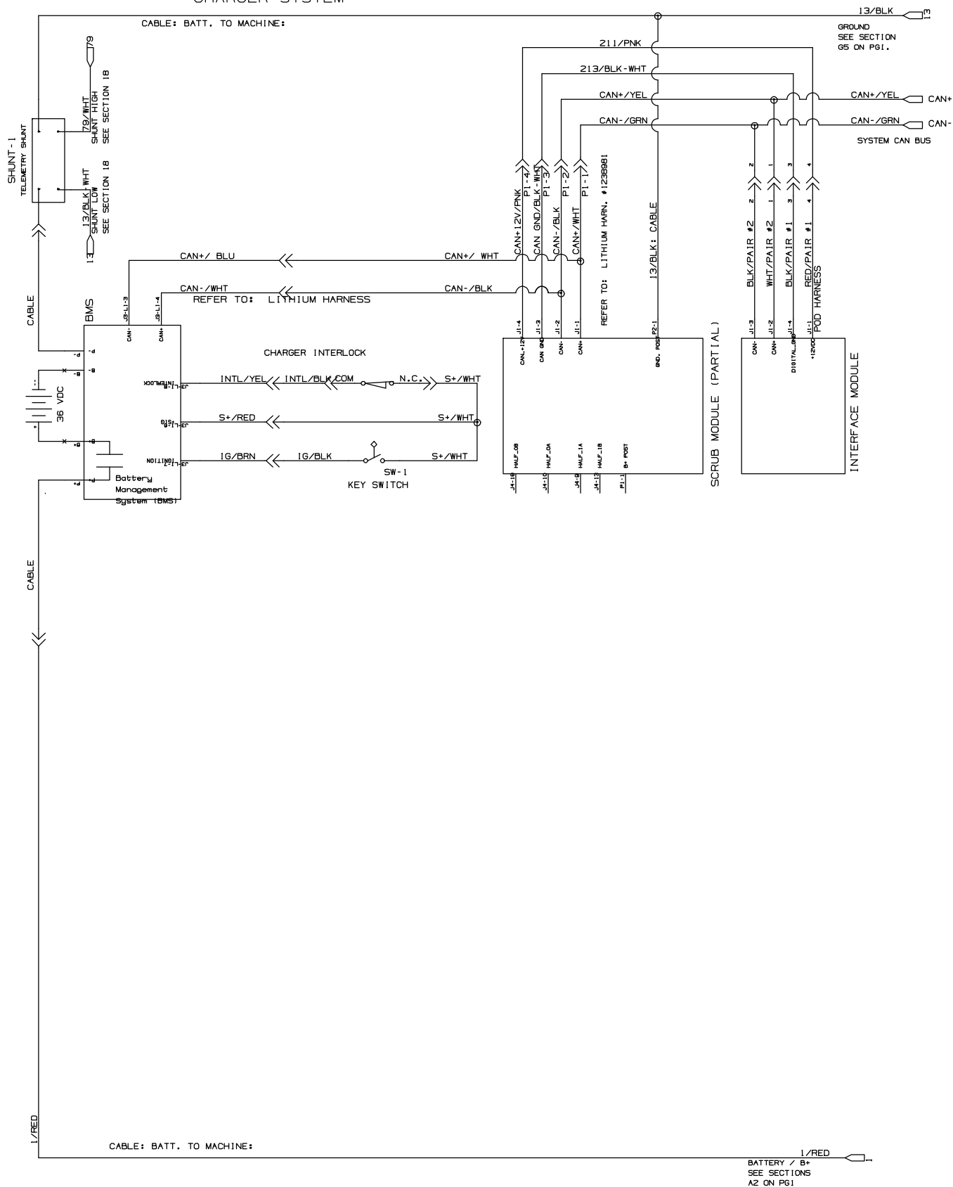
Fig. 53 – Electrical Schematic (012000– )
