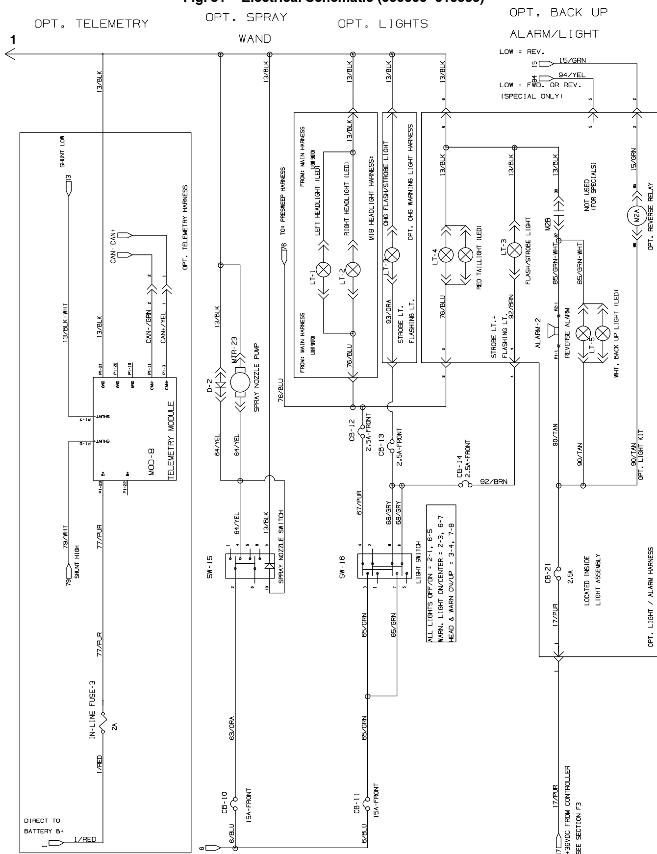
Fig. 51 – Electrical Schematic (000000–010999)
