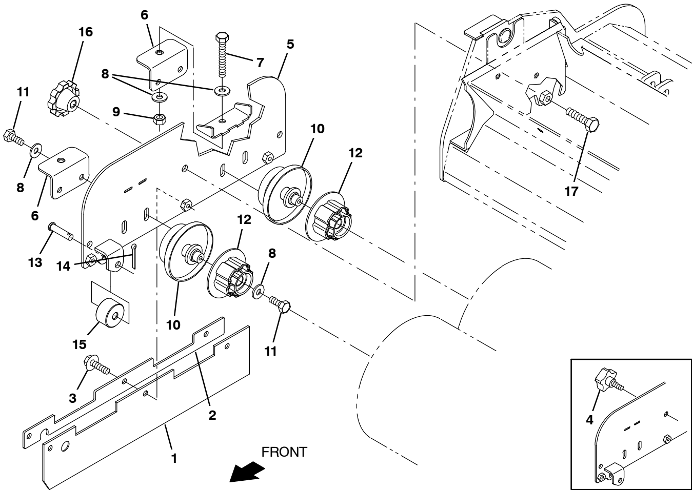
Fig. 15 – Sweeping Main Brush Idler Group
