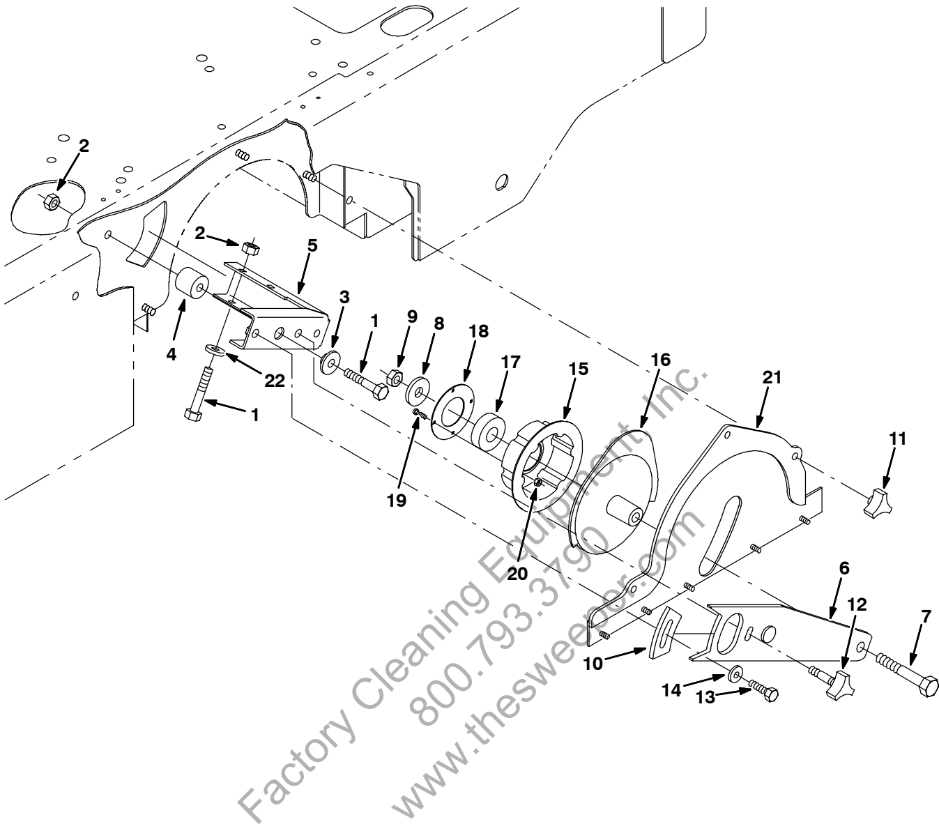
Fig. 31 - Main Brush Idler Group
