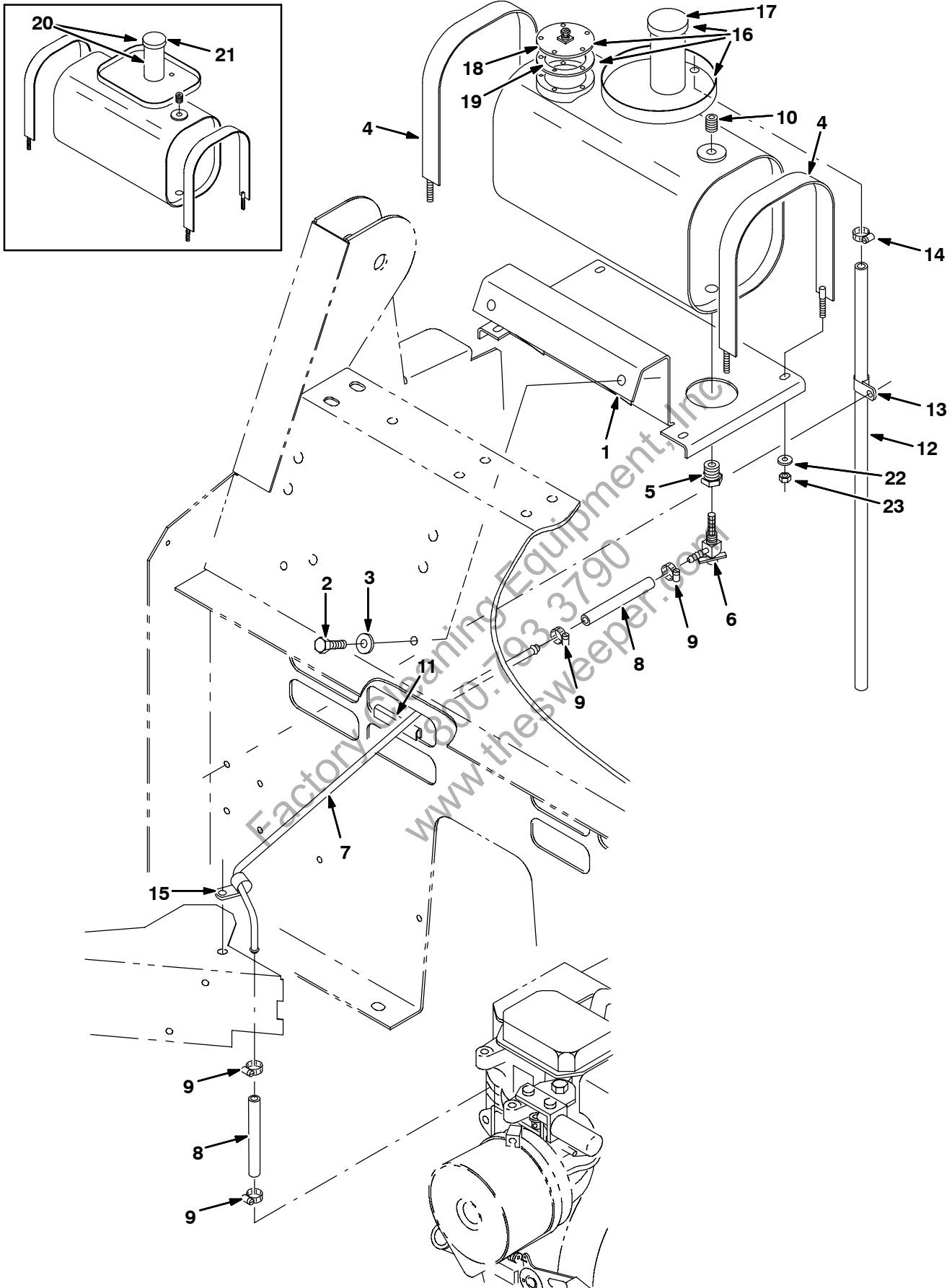
Fig. 12 - Engine Fuel Tank Group, Gas
