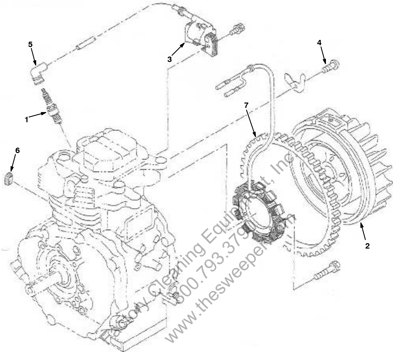
Fig. 9 - Ignition Group, Gasoline
