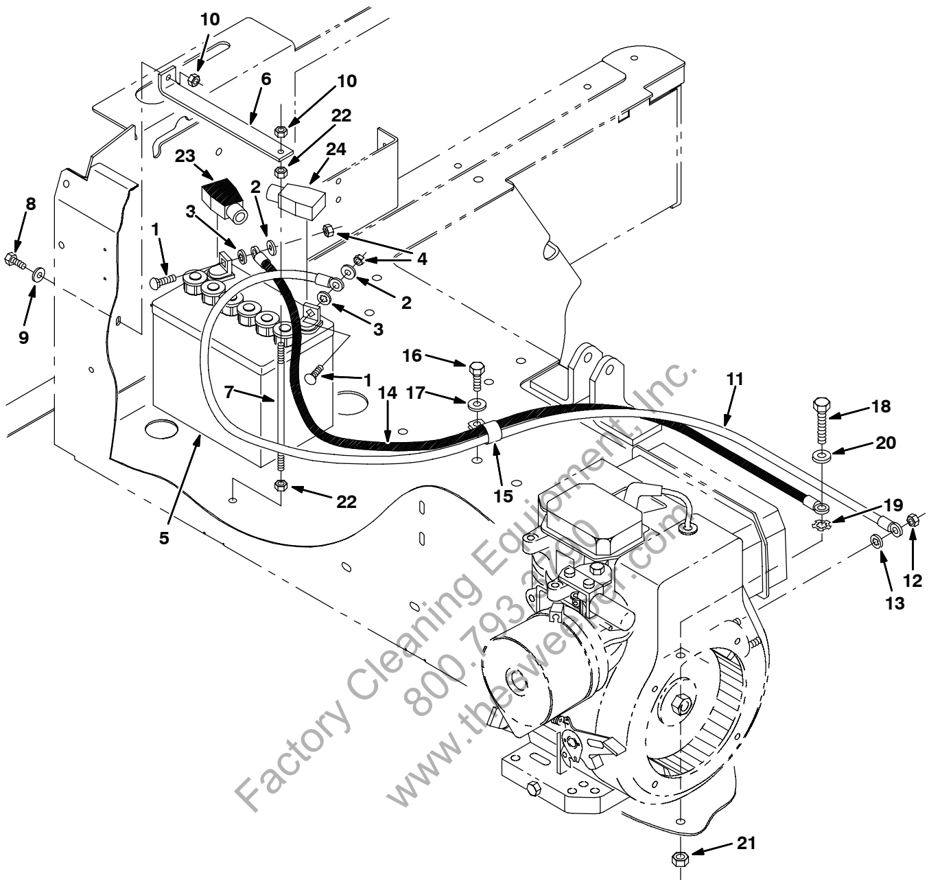
Fig. 17 - Battery Group
