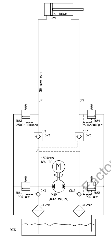
HOPPER LIFT SYSTEM
