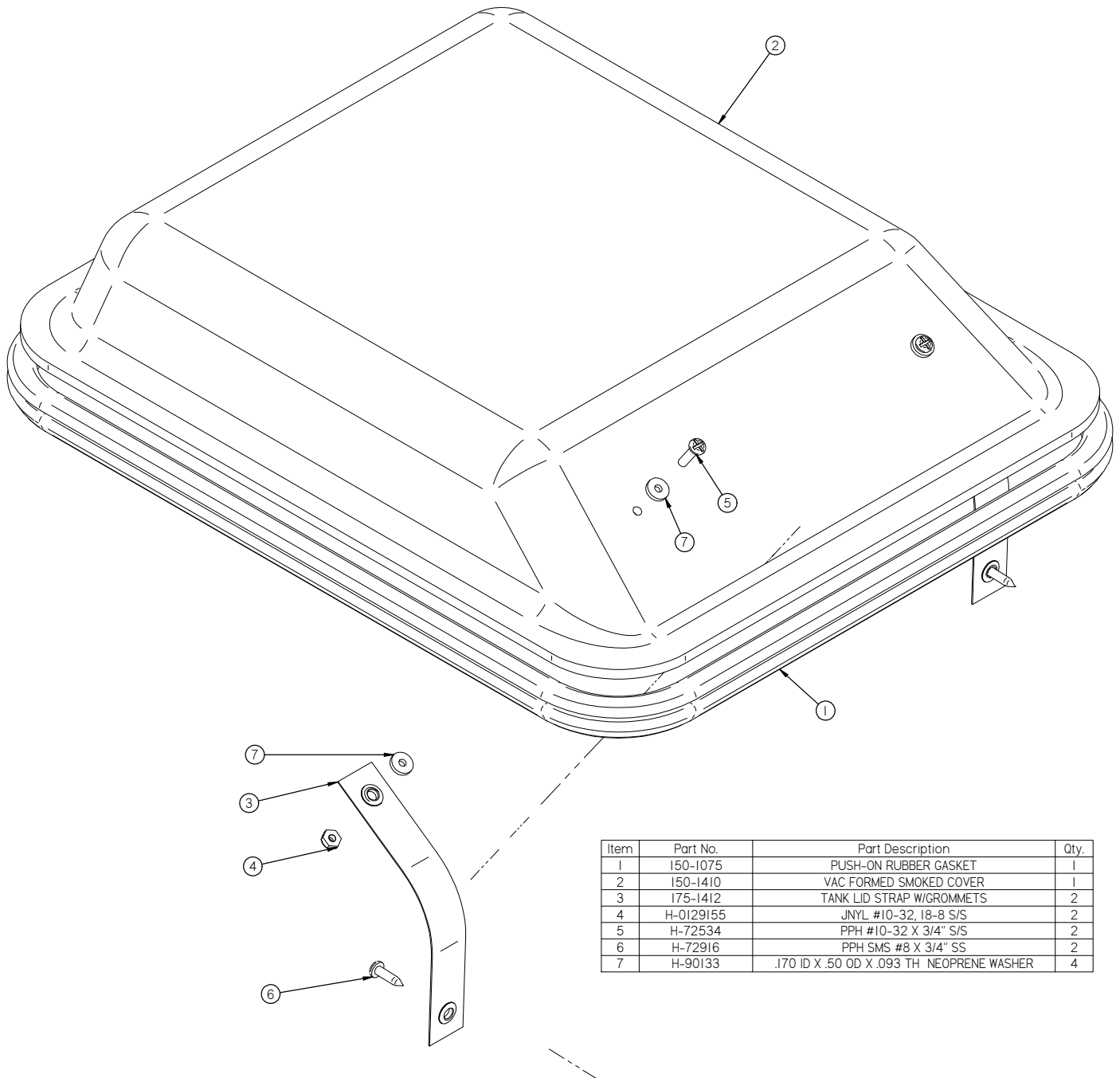
TANK LID ASSEMBLY 150-1410D
